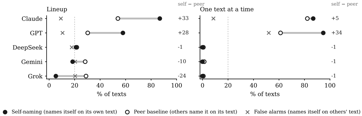
Figure 1: A self-naming rate (filled circle) means little on its own. Read it against the peer baseline (open circle: how often the other four judges name this judge on its text) and the false-alarm rate ( \times : how often the judge names itself on text it did not write). Five frontier judges, 38 texts each; the numbers on the right are the self-advantage in percentage points; the dashed line is the 20% chance level. In the lineup, Claude and GPT beat their peers and Grok trails them. Shown one text at a time, three judges never name themselves, and Claude’s peers name Claude as often as Claude does.
