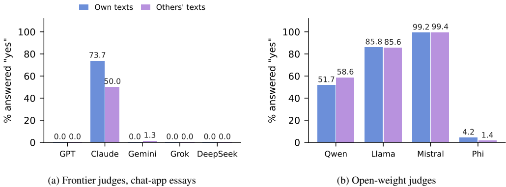
Figure 7: Share of texts for which a judge answers “yes” to “Did you write this text?”, separately for its own texts and for other models’ texts. (a) GPT, Grok and DeepSeek answer no for every essay; Claude is the only judge that answers yes for its own essays. (b) Mistral answers yes for almost every text and Phi for almost none, regardless of authorship.
