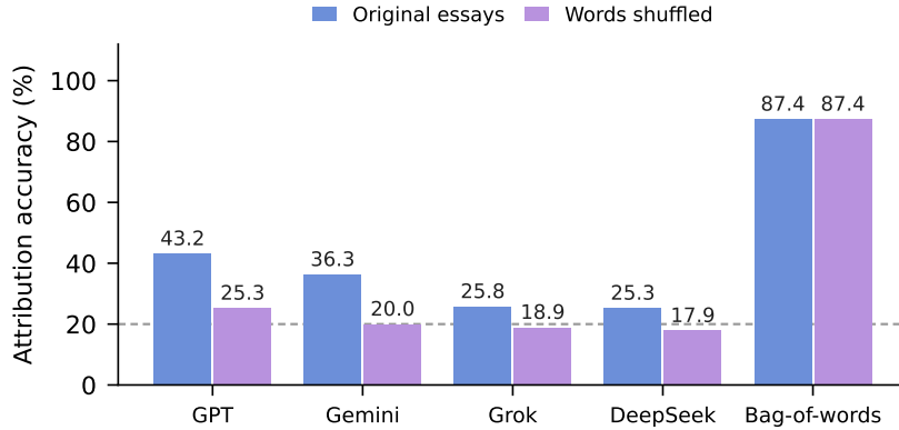
Figure 5: Lineup accuracy of four frontier judges on the chat-app essays in their original form and with the words of each essay shuffled, compared with a bag-of-words classifier on the same essays. With shuffled words the judges’ accuracy is between 17.9% and 25.3%, close to chance (dashed line). The classifier does not use word order, so its two bars are equal by construction. Claude is omitted because its provider refused all shuffled lineups, and Gemini’s shuffled bar is based on 24 of its 38 lineups.
