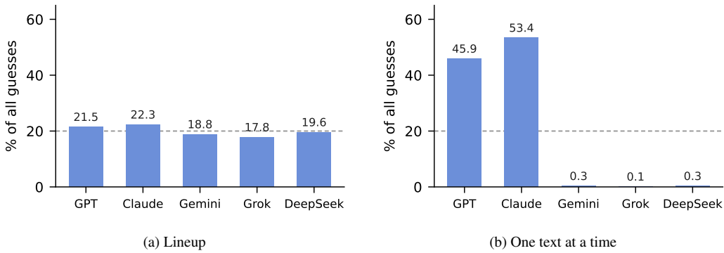
Figure 6: Share of the 950 attributions on the chat-app essays that name each model. In the lineup the shares are close to uniform. One text at a time, GPT and Claude receive 99.3% of attributions and Gemini, Grok and DeepSeek almost none. The dashed line marks a uniform distribution (20%).
