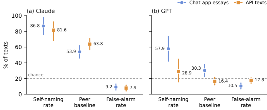
Figure 4: Claude and GPT in the lineup on the 38 prompts shared by the chat-app essays (circles) and the API texts (squares): self-naming rate, peer baseline and false-alarm rate, with 95% bootstrap intervals over prompts. Claude’s self-naming and false-alarm rates are almost the same on the two sets and its peer baseline is higher on the API texts; GPT’s self-naming rate and peer baseline fall and its false-alarm rate rises. The dashed line marks chance (20%).
