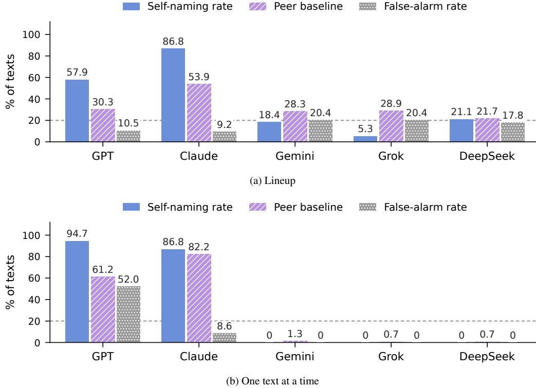
Figure 1: Self-naming rate, peer baseline and false-alarm rate of the five frontier judges on the 38 chat-app essays each wrote. The self-naming rate is the share of its own essays a judge attributes to itself, the peer baseline is the share of those essays the other four judges attribute to it, and the false-alarm rate is the share of other models’ essays it attributes to itself. In the lineup (a), Claude and GPT exceed their peer baselines by 33 and 28 points and Grok falls 24 points below its baseline. When the same essays are shown one at a time (b), Gemini, Grok and DeepSeek never name themselves, GPT names itself on 52% of essays it did not write, and Claude’s peer baseline rises to 82%. The dashed line marks chance (20%).
