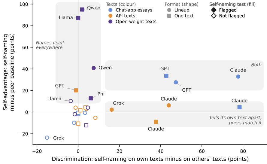
Figure 2: The 28 lineup and one-text cases, placed by discrimination (horizontal) and self-advantage (vertical). Colour gives the text set, shape the format, and filled markers are the 12 cases flagged by the self-naming test. The yes/no cases are omitted because they have no peer baseline. Flagged cases near the vertical axis exceed their peers, by up to +95.0 points, without discriminating; those near the horizontal axis discriminate while their peers name them about as often; three are far from both axes. The grey bands are reading guides; the verdicts come from the tests in Table 2.
