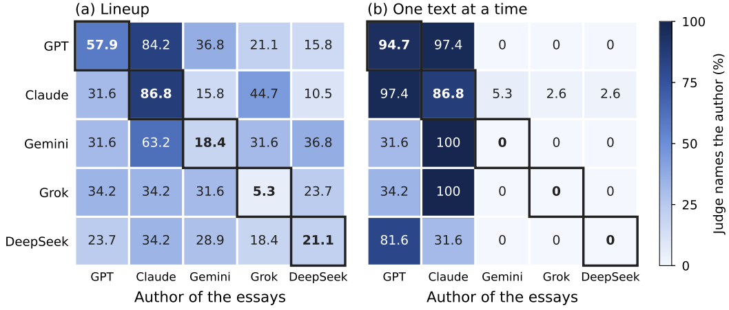
Figure 3: How often each frontier judge (row) names the true author (column) on that author’s 38 chat-app essays, in percent, (a) in the lineup and (b) one text at a time. Outlined cells on the diagonal are self-naming rates, and the mean of the other four cells in a column is that author’s peer baseline.
