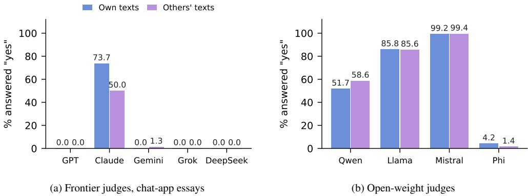
Figure 8: Share of texts for which a judge answers “yes” to “Did you write this text?”, separately for its own texts and for other models’ texts. (a) GPT, Grok and DeepSeek answer no for every essay; Claude is the only judge that answers yes for its own essays. (b) Mistral answers yes for almost every text and Phi for almost none, regardless of authorship.
