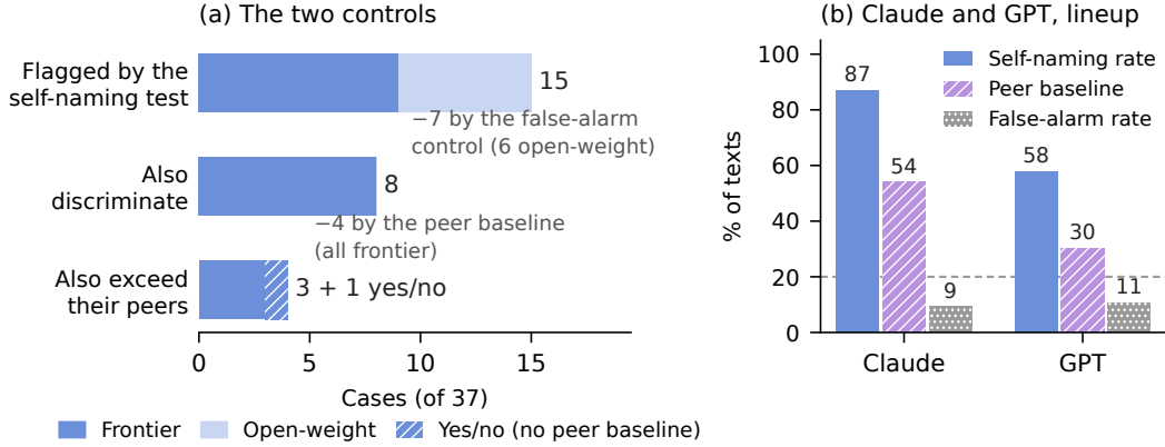
Figure 1: Two controls from the same lineup data remove 11 of the 15 cases that the self-naming test flags. (a) A case is one judge on one set of texts in one question format. The self-naming test flags a case when the judge names itself on its own texts more often than chance. A case discriminates when the judge names itself more often on its own texts than on other models’ texts, and it exceeds its peers when the judge names itself on its texts more often than the other judges name it; under a like-for-like peer comparison 5 cases pass (Table 2). The yes/no format has no peer baseline, and its one case that discriminates (Claude) is significant only with correction within its panel. (b) The two judges that pass both controls in the lineup on the chat-app essays. Claude names itself on 87% of its own essays and 9% of the others, and the other four judges name Claude on 54% of its essays. The dashed line marks chance (20%).
