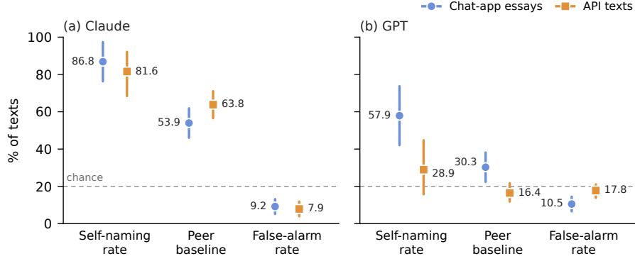
Figure 5: Claude and GPT in the lineup on the 38 prompts shared by the chat-app essays (circles) and the API texts (squares): self-naming rate, peer baseline and false-alarm rate, with 95% bootstrap intervals over prompts. Claude’s self-naming and false-alarm rates are almost the same on the two sets and its peer baseline is higher on the API texts; GPT’s self-naming rate and peer baseline fall and its false-alarm rate rises. The dashed line marks chance (20%).
