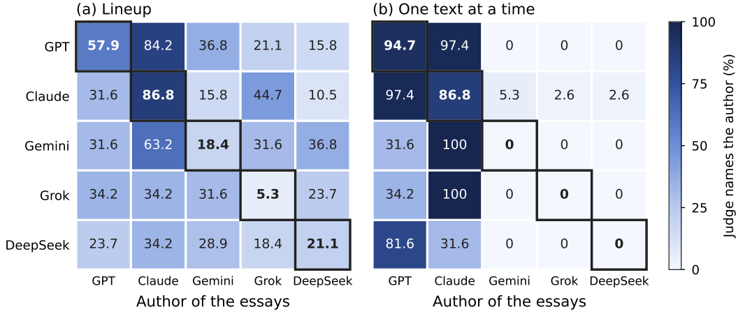
Figure 4: How often each frontier judge (row) names the true author (column) on that author’s 38 chat-app essays, in percent, (a) in the lineup and (b) one text at a time. Outlined cells on the diagonal are self-naming rates, and the mean of the other four cells in a column is that author’s peer baseline.
