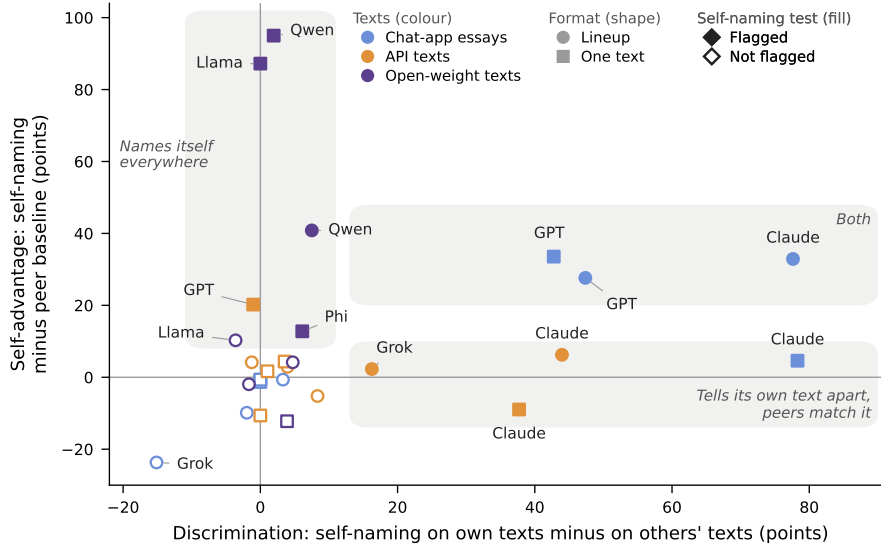
Figure 2: The 28 lineup and one-text cases, placed by discrimination (horizontal) and self-advantage (vertical). Colour gives the text set, shape the format, and filled markers are the 12 cases flagged by the self-naming test. The yes/no cases are omitted because they have no peer baseline. Flagged cases near the vertical axis exceed their peers, by up to +95.0 points, without discriminating; those near the horizontal axis discriminate while their peers name them about as often; three are far from both axes. The grey bands are reading guides; the verdicts come from the tests in Table 2.
