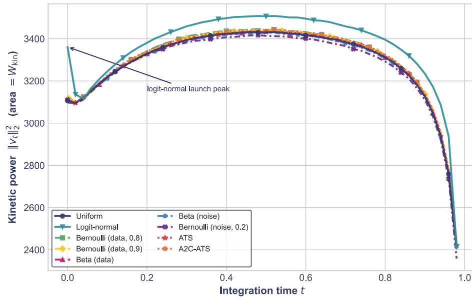
Figure 5.19: Kinetic power \|v_t\|_2^2 along the generation trajectory (Euler, N=50 , 256 trajectories), whose area over t is W_{\text{kin}} . The field starts near the minimum-norm launch value \|x_0\|_2^2 \approx 3072 at t \rightarrow 0 , accelerates to a mid-schedule maximum, and decelerates as it settles onto the data manifold. Logit-normal alone sits systematically above the pack, with a sharp launch peak at the noise boundary its density starves, the clearest trace of a training bias on the learned field, a boundary artifact small against the trajectory-to-trajectory scatter. Curves are means over the 256 paired trajectories, and LTE-ATS is omitted for legibility.
