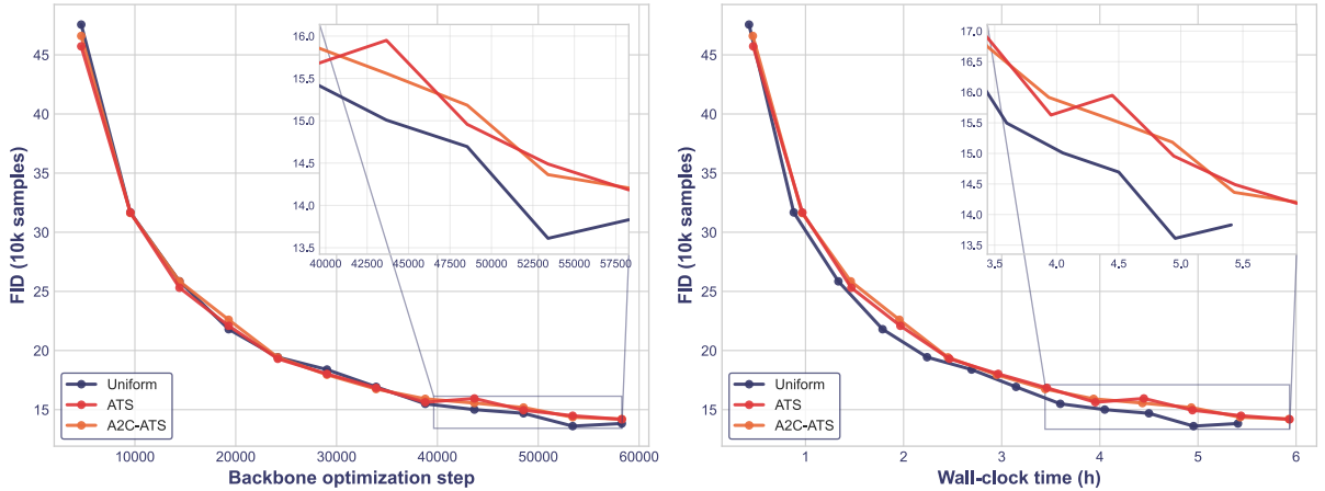
Figure 5.3: Uniform sampling matches or slightly beats adaptive FID at every budget. FID over training (10,000 EMA samples). Left: FID versus optimizer steps. The three strategies overlap, with uniform sampling marginally ahead in the final-third zoom. Right: FID versus wall-clock time. The adaptive strategies spend \approx 10\% longer per epoch, so the uniform curve lies on or slightly below both the ATS and A2C-ATS curves at every compute budget and reaches its final FID notably sooner.
