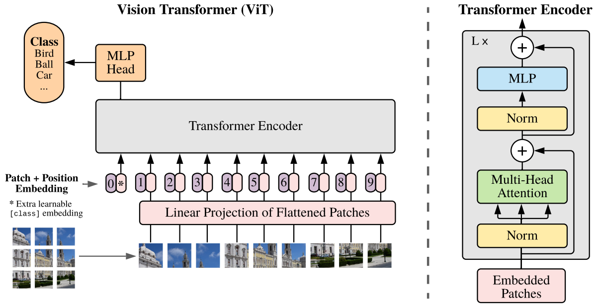
Figure 2.1: The Vision Transformer (ViT). Left: the input image is split into fixed-size patches, each of which is flattened and linearly projected into a token embedding; learned position embeddings are added and an extra learnable [class] token is prepended, after which the sequence is processed by a standard Transformer encoder. In the original classification setting an MLP head reads the class token to predict the label. Right: a single Transformer encoder block applies multi-head self-attention and a position-wise MLP, each preceded by layer normalization and wrapped in a residual connection, repeated L times. Figure from Dosovitskiy et al. (2021).
