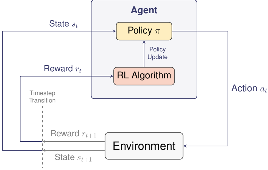
Figure 2.3: The reinforcement learning loop for policy-based model-free methods. The agent internally maps states to actions via a parameterized policy, which is iteratively improved by the RL algorithm using the reward signal. The dashed line delineates the timestep transition from t to t + 1 . This architecture reflects the core learning mechanism utilized by the Adaptive Timestep Sampling (ATS) framework.
