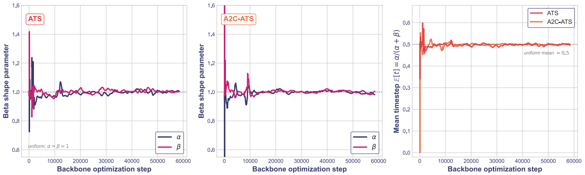
Figure 5.7: The learned policy explores, then reverts to uniform. Policy dynamics of ATS and A2C-ATS over training. Left, center: the batch-averaged Beta shape parameters \alpha (navy) and \beta (magenta) for ATS and A2C-ATS separately; both oscillate during the first \sim 10 epochs, then settle at \alpha \approx \beta \approx 1 (the A2C first-epoch transient reaching \beta \approx 10 runs off-scale). Right: the induced mean timestep \mathbb{E}[t] = \alpha / (\alpha + \beta) swings between 0.34 and 0.60 early (A2C transiently to \approx 0 ), then holds within \pm 2\% of the uniform value 0.5 for the remaining \sim 290 epochs.
