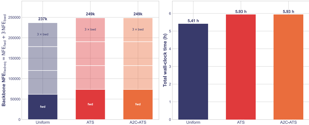
Figure 5.4: Adaptive sampling adds a \approx 10\% compute premium. Training cost of uniform vs. adaptive sampling. Left : theoretical backbone compute in forward-pass equivalents (Equation (5.3)); each bar places the forward passes at the bottom (solid) and stacks the backward passes on top at their 3\times cost, drawn as three translucent tiers. The adaptive methods’ extra forward-only probes are included in the forward block, so the NFE gap over the static samplers stems solely from the additional probe and reward-estimation forward passes. Right : the corresponding measured wall-clock time on 4\times Titan X, where the untracked reinforcement-learning bookkeeping widens the gap to +9.6\% .
