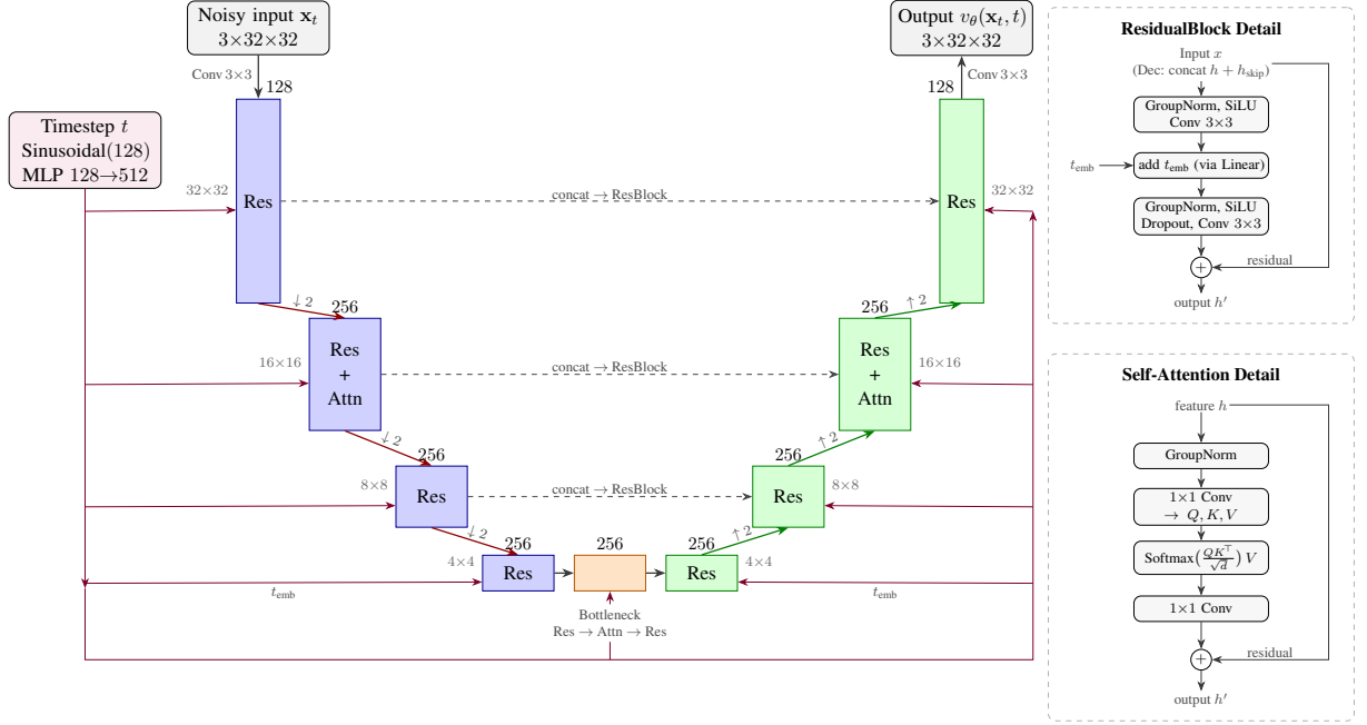
Figure 5.2: The shared U-Net backbone used for all CIFAR-10 runs ( \approx 35.7\text{M} parameters). The architecture follows Kim et al. (2025b). Left/center: The contracting (encoder, blue) and expanding (decoder, green) paths. Each block’s height encodes its spatial resolution ( 32^2 \rightarrow 4^2 ) and its width encodes the channel count ( 128 \rightarrow 256 ). The bottleneck operates at the 4 \times 4 resolution and consists of two ResidualBlocks surrounding a Self-Attention layer. Red/green arrows indicate strided-convolution downsampling ( \downarrow 2 ) and nearest-neighbor upsampling ( \uparrow 2 ). Dashed gray arrows represent skip connections that concatenate encoder feature maps onto the decoder inputs. Right: Internal block details. The decoder ResidualBlocks fuse the concatenated features. Self-Attention is applied at both the 16 \times 16 spatial stages and the 4 \times 4 bottleneck. The sinusoidal timestep embedding t_{\text{emb}} is broadcast along the purple rail and added inside every residual block via a block-specific linear projection to match changing channel dimensions.
