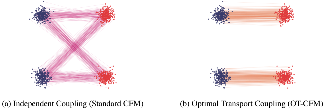
Figure 3.1: Geometric illustration of probability paths under different boundary couplings. (a) Standard independent coupling randomly pairs prior noise representations x_0 (dark purple) with data samples x_1 (red). This randomized assignment results in heavily intersecting trajectories (pink lines) and conflicting vector field targets during training. (b) Mini-batch Optimal Transport coupling dynamically assigns pairs to minimize the approximated 2-Wasserstein distance, measuring the transport cost. This alignment strictly untangles the trajectories, yielding straight, non-overlapping flows (orange lines) that eliminate target ambiguity and reduce stochastic gradient variance (Tong et al., 2024; Pooladian et al., 2023).
