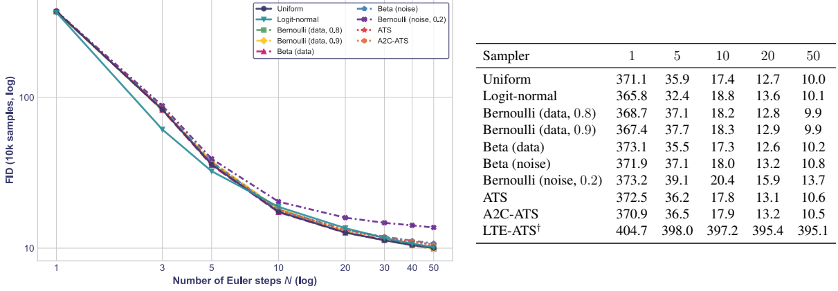
Figure 5.20: FID versus the number of Euler steps N . 10,000 samples with noise paired across N and strategies. Left: log–log curves. Right: values at N \in \{1, 5, 10, 20, 50\} . The nine converged strategies collapse onto a shared curve, so cutting the budget costs each of them the same, while Bernoulli (noise, 0.2) rides a constant offset above the pack and the collapsed LTE-ATS ( † ) stays near 395 at every budget. The absolute scores are a dedicated recomputation on the epoch-300 checkpoints and lie \approx 3.7 FID below the training-time values of Table 5.2, an offset of the separate generation draw rather than a finite-sample effect. It preserves what the comparison rests on, the isolation of Bernoulli (noise, 0.2) and the collapse of LTE-ATS; the re-ordering inside the sub-one-point band of the remaining strategies is itself evidence that those margins are draw noise.
