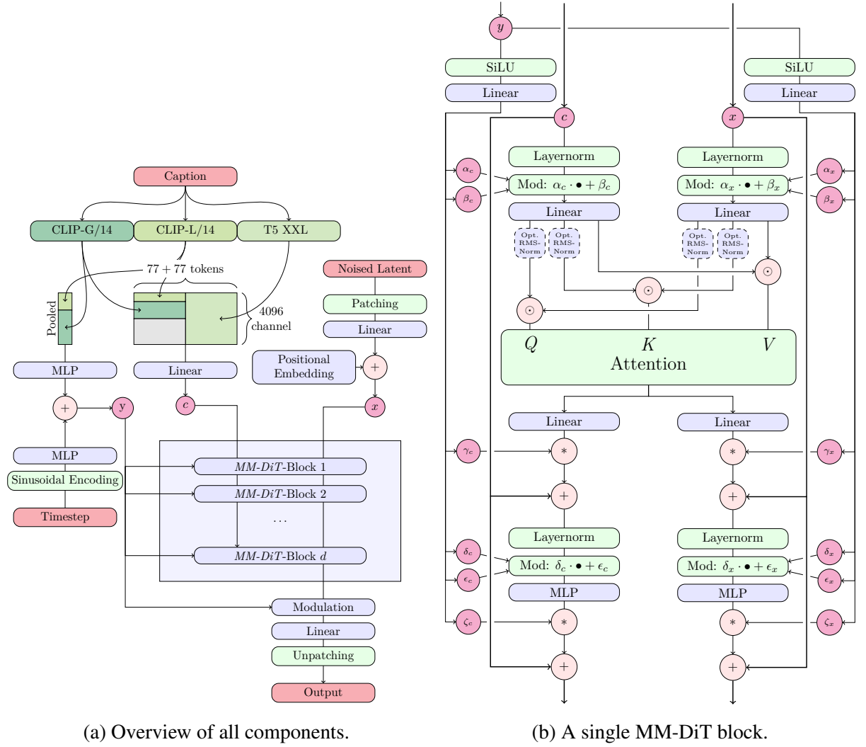
Figure 2.2: The Multimodal Diffusion Transformer (MM-DiT) architecture of Stable Diffusion 3. (a) Caption and noised latent are embedded into a text and an image token stream; the timestep embedding and the pooled text representation form the global modulation signal y . (b) Within each block, the two streams are processed by modality-specific weights and interact exclusively through a joint attention operation over the concatenated token sequences. Concatenation is indicated by \odot and element-wise multiplication by * . Figure from Esser et al. (2024).
