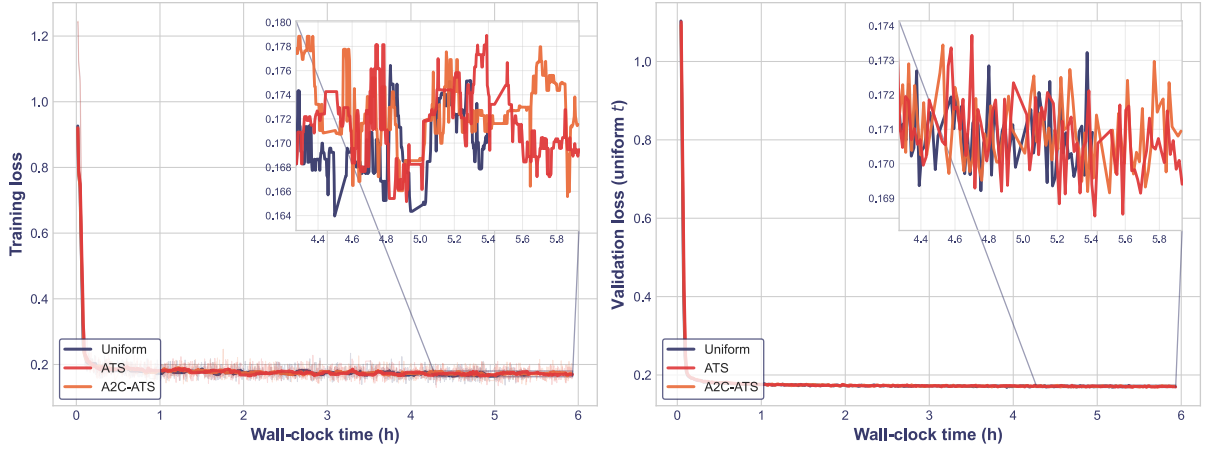
Figure 5.5: Adaptive sampling does not accelerate convergence at equal compute. Backbone loss versus wall-clock time under uniform, ATS, and A2C-ATS sampling. Left: training loss, logged every 40 optimizer steps (raw in faint, 25-point rolling median bold); its high-frequency fluctuation reflects the mini-batch estimation error. Right: the sampler-independent validation loss per epoch. The strategies track one another, and the adaptive curves, shifted right by their \approx 10\% overhead, never lead uniform, as the final-quarter zoom insets confirm.
