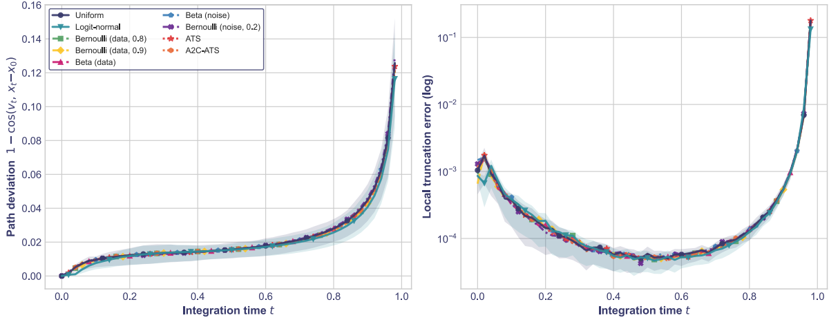
Figure 5.18: Curvature diagnostics of the fully trained models along the generation trajectory (Euler, N=50 , 256 trajectories). Left: path deviation, near 0.02 through the interior and rising to about 0.12 as t \rightarrow 1 . Right: the Euler–Heun truncation-error proxy on a log scale, a U in t minimal near t \approx 0.45 and spiking at t \rightarrow 1 . Line patterns group the sampler families (solid: uniform and logit-normal; dashed: data-biased; dash-dotted: noise-biased; dotted: adaptive) and markers identify the strategies; LTE-ATS is tabulated only (Table 5.5). Shaded bands give the interquartile range over the 256 paired trajectories for uniform and logit-normal, whereas Table 5.5 reports each mean with its standard error. The kinetic power is shown separately in Figure 5.19. The nine converged strategies superimpose on both panels.
