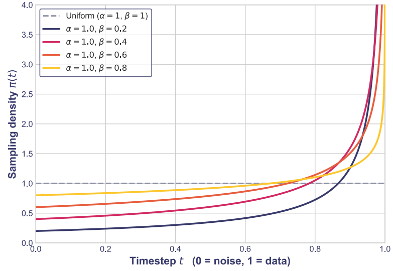
Figure 3.4: Probability density functions for Beta-Tuned timestep sampling, adapted to the continuous Flow Matching temporal domain. By fixing \alpha = 1.0 and decreasing the \beta parameter, a strictly monotonically increasing, J-shaped distribution is induced, asymptotically prioritizing the final trajectory near the data manifold.
