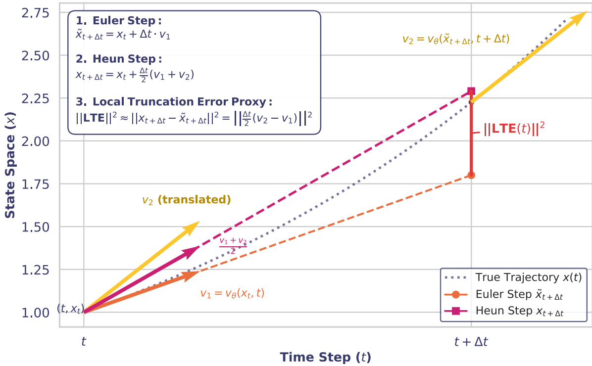
Figure 4.3: Geometric interpretation of the Local Truncation Error (LTE) proxy. The first-order Euler predictor \tilde{x}_{t+\Delta t} extrapolates the state using the instantaneous velocity v_\theta(x_t, t) , assuming a strictly linear trajectory. The second-order Heun corrector evaluates the vector field at this predicted future state to compute a curvature-aware final update x_{t+\Delta t} . The squared magnitude of the spatial discrepancy between these two predictions yields the LTE proxy \widehat{\text{LTE}}_\theta , a quantifiable scalar metric for the underlying geometric curvature of the ODE trajectory.
