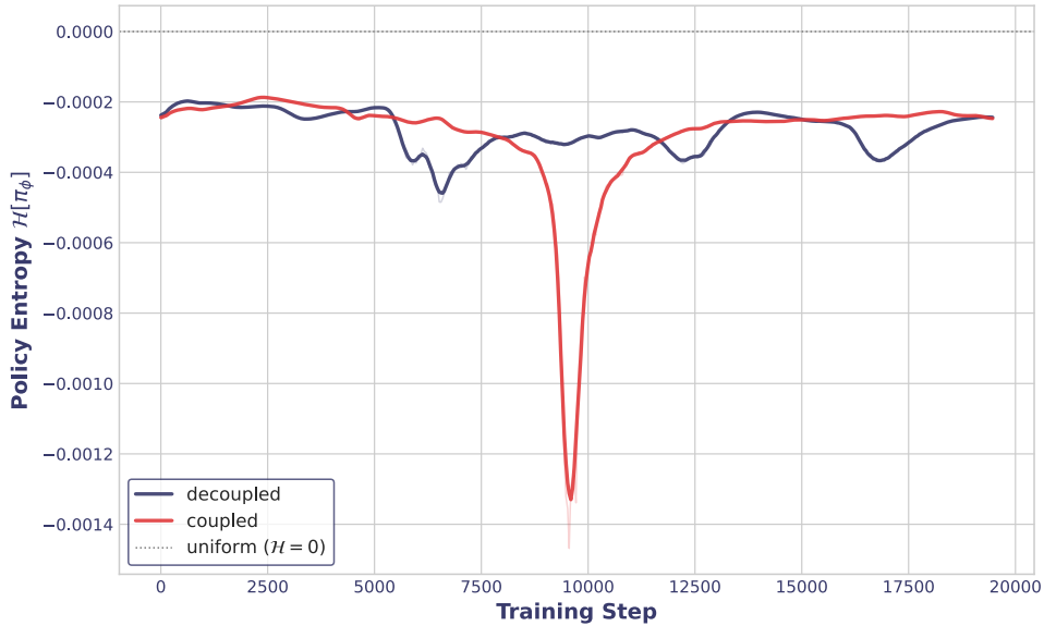
Figure A.2: Policy entropy \mathcal{H}[\pi_\phi] during training for the decoupled and coupled entropy formulations (CondOT-FM with ATS policy, Experimental setup of Section 5.1). Under the coupled entropy formulation, the policy rapidly drifts away from a near-uniform distribution around step 9500. Because the |\mathcal{H}| -gated regularization remains weak, it fails to directly counter this policy drift, resulting in a severe negative spike in entropy. In contrast, the decoupled formulation maintains a distribution much closer to uniform, indicating a more robust and consistent entropy regularization.
