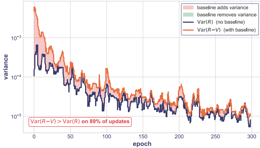
Figure 5.10: Subtracting the baseline increases the centered-reward variance. Per-update reward variance \text{Var}(R) (no baseline) and centered-reward variance \text{Var}(R - V) (with baseline), shown as 25-point rolling medians. The shaded gap is the variance-reduction gain, red where \text{Var}(R - V) > \text{Var}(R) (the baseline adds variance) and green where it removes it. Both variances decay by more than an order of magnitude as the backbone converges, yet \text{Var}(R - V) stays above \text{Var}(R) on 89% of updates across the whole run.
