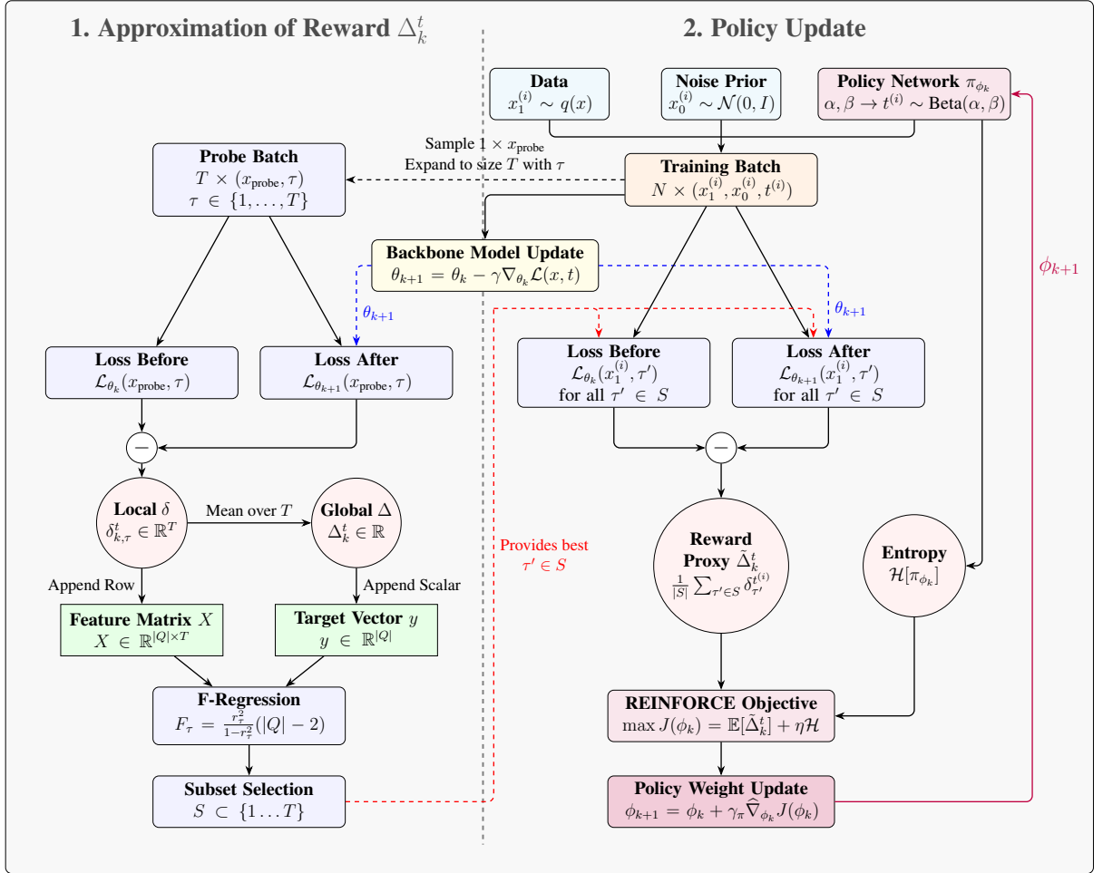
Figure 4.2: Overview of the Adaptive Timestep Sampling Process. The diagram illustrates the interplay between the backbone Flow Matching model and the policy network. The policy network generates a Beta distribution from which a timestep is sampled, while the backbone loss reduction over a subset of timesteps provides the reward to update the policy via REINFORCE.
