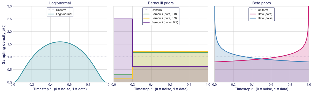
Figure 5.17: Training-time sampling densities, grouped by family on a shared density axis with the uniform density (dotted) as the reference in every panel. Every trajectory launches from the noise manifold at t = 0 , so the density at t \rightarrow 0 measures how much training mass a prior withdraws from the launch regime. Left: logit-normal drives its density to zero at both boundaries. Middle: the data-biased Bernoulli priors drop the noise-boundary density to 0.29 (data, 0.8) and 0.14 (data, 0.9), while Bernoulli (noise, 0.2) raises it to 2.5. Right: Beta (data), though nominally data-biased, keeps a near-uniform density of 0.8 at the noise boundary, far above the data-biased Bernoullis, whereas Beta (noise) concentrates there. The Beta densities diverge at their bias boundary and are clipped at the panel ceiling.
