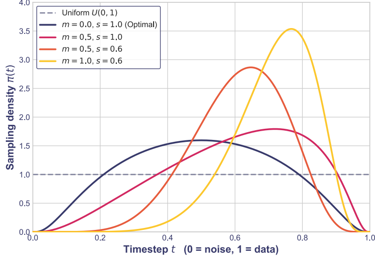
Figure 3.2: Probability density functions for logit-normal timestep sampling. The optimal configuration ( m = 0.0, s = 1.0 ) concentrates training focus heavily on the intermediate steps of the trajectory, compared against alternative parameterizations reported by Esser et al. (2024). The standard uniform distribution \mathcal{U}(0, 1) is provided as a reference baseline.
