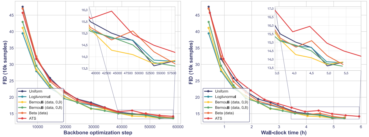
Figure 5.12: Static data-biased priors lead adaptive sampling over most of training. FID over training (10,000 EMA samples) for six representative strategies. Left: FID versus optimizer step. Right: FID versus wall-clock time. The final-portion zoom insets show the strategies converging into a sub-1 FID band, with ATS remaining above the data-biased priors and, on the wall-clock axis, penalized further by its \approx 10\% overhead.
