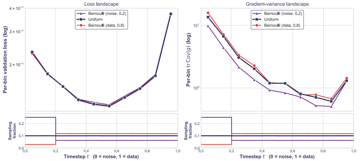
Figure 5.15: Biasing the sampler leaves the loss landscape unchanged and the gradient-variance landscape unchanged in shape. Uniform sampling against the two opposite Bernoulli priors, whose sampling densities (bottom panel, per-bin mean fraction drawn as step lines that are flat within a bin and jump at the bin edge, uniform flat at the reference value 0.1, both Bernoulli densities piecewise-uniform with their break at t = 0.2 ) differ by almost an order of magnitude at the boundaries. Left : per-bin validation loss (uniform-in-bin t , held-out data, mean over the last 20 epochs, log scale), the sampler-independent loss landscape, where the three curves coincide to within 0.007 everywhere. Right : per-bin gradient variance \text{tr Cov}(g) (log scale; mean over the last four probes, which suppresses the \approx 50\% single-probe estimation noise), where the three share the same noise-dominated U shape and differ only by a modest overall level shift.
