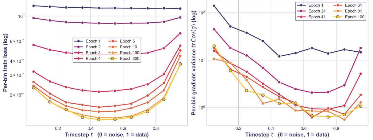
Figure 5.14: The per-timestep loss and gradient variance are both strongly non-uniform in t , both U-shaped, and stationary in shape after the first few epochs, but their peaks sit at opposite ends of the schedule. Left: per-bin training loss of the uniform run at selected epochs. From a nearly flat start the profile shows the U-shape by the second epoch, reaches its final \approx 3\times spread within about five epochs and its final shape by epoch 10, after which it barely moves (epochs 100 and 300 almost coincide), with the data-proximal bin carrying the largest loss throughout. Right: per-sample gradient variance \text{tr Cov}(g) per bin (log scale), estimated every tenth epoch on the instrumented rerun of the same configuration (Equation (5.5)). This profile is U-shaped as well but dominated by the noise boundary, so the loss and the gradient variance place the difficulty at opposite ends. The noise boundary is the highest-variance region at every probe and the shape is preserved, while the overall level, including an elevation at the data boundary during the first training epochs, decays as the fit improves and the interior bins draw together.
