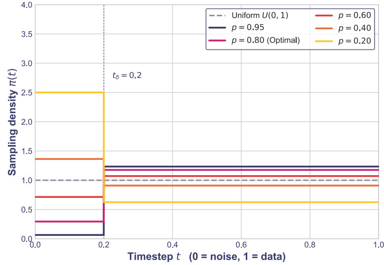
Figure 3.3: Probability density functions for the Bernoulli sampling strategy proposed by Zheng et al. (2024a). The interval threshold is fixed at t_\delta = 0.2 . Values of p > 0.5 progressively shift the network’s training capacity toward the data manifold ( t \rightarrow 1 ), while p < 0.5 biases the distribution toward the prior noise.
