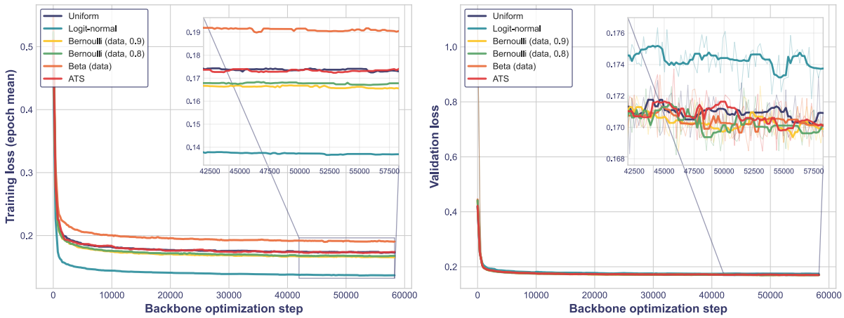
Figure 5.13: The epoch training loss tracks the sampling density, not model quality. Left: epoch-mean training loss under each sampler’s own t -density (raw values with a 9-point rolling median); logit-normal sampling, concentrated on the low-loss mid-range timesteps, posts by far the lowest value. Right: the sampler-independent validation loss at uniform t , on which logit-normal is instead the highest while the remaining strategies collapse onto a common band near 0.170.
