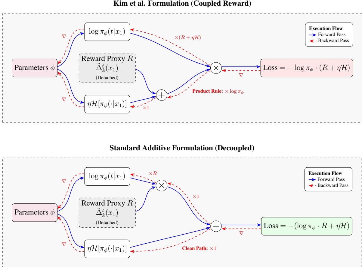
Figure A.1: Computational Graph and Autograd Flow Comparison. Blue solid arrows denote the forward pass, while dashed red arrows denote the flow of gradients during backpropagation. The isolated reward proxy acts as a detached environmental signal. In the Kim et al. (2025b) formulation (top), coupling entropy directly into the reward forces Autograd to apply the product rule, creating an unintentional gradient scaling where \nabla \mathcal{H} is multiplied by \log \pi . Separating them additively in the standard formulation (bottom) provides a clean path for the entropy gradient completely independent of the stochastic log-probability.
