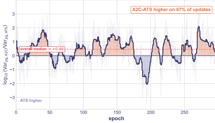
Figure 5.9: The learned critic does not reduce the policy-gradient variance. Step-wise log-ratio \log_{10}(\text{Var}_{\text{pg,A2C}}/\text{Var}_{\text{pg,ATS}}) over training (raw faint, 25-point rolling median bold). Positive values (orange) mark updates where A2C-ATS has the higher variance, negative values (blue) where baseline-free ATS does. The ratio is positive on 67% of updates, so the baseline raises rather than lowers the policy-gradient variance.
