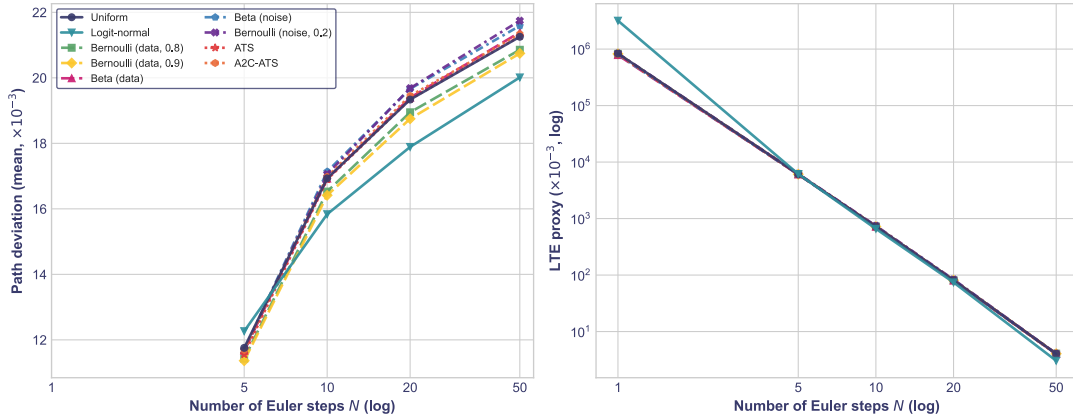
Figure 5.21: Trajectory diagnostics versus the number of Euler steps N (log x -axis). Left: path deviation. Right: the Euler–Heun truncation-error proxy (log scale). Both are recomputed on the epoch-300 models with noise paired across budgets and strategies. The nine converged strategies stay superimposed at every budget, mirroring the FID sweep of Figure 5.20; the truncation error grows as roughly N^{-2} and the path deviation falls as the coarse grid under-samples the late turn. The single-step budget has no interior and is omitted from both, and LTE-ATS is excluded for legitimacy.
