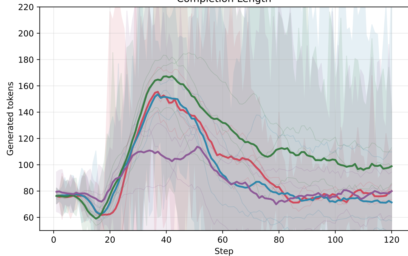
Completion Length
