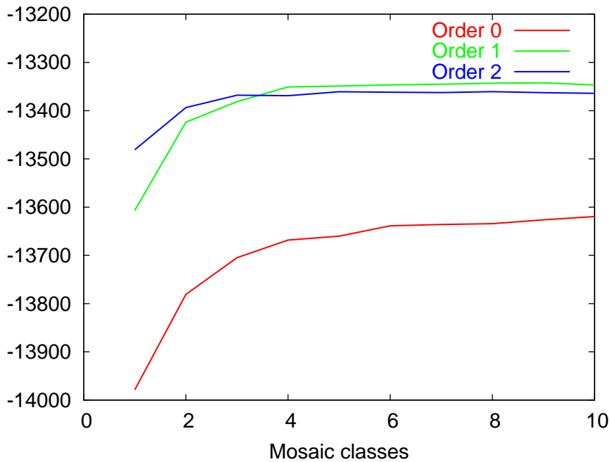
Likelihood of test sequences
