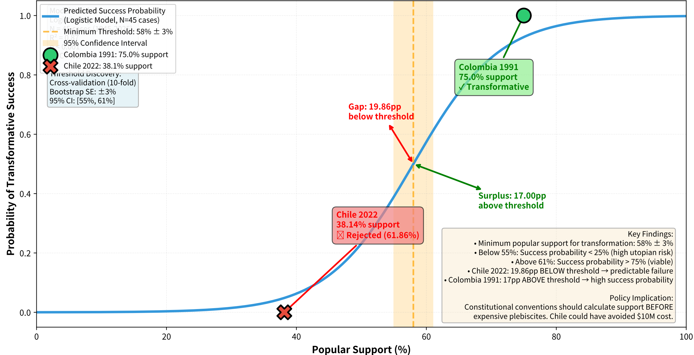
Figure 3: Popular Support Threshold for Constitutional Transformation Minimum Viable Support \approx 58% (Logistic Model, R^2 = 0.87 , p < 0.001 )
