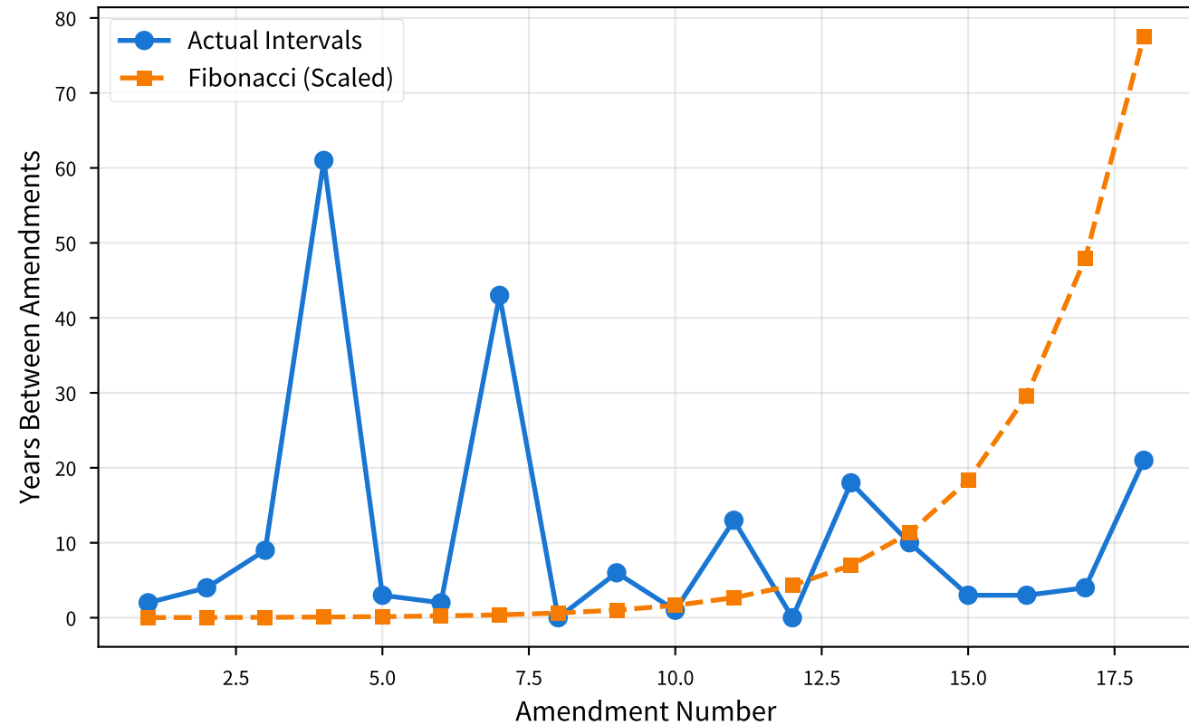
Panel A: Amendment Intervals vs Fibonacci
