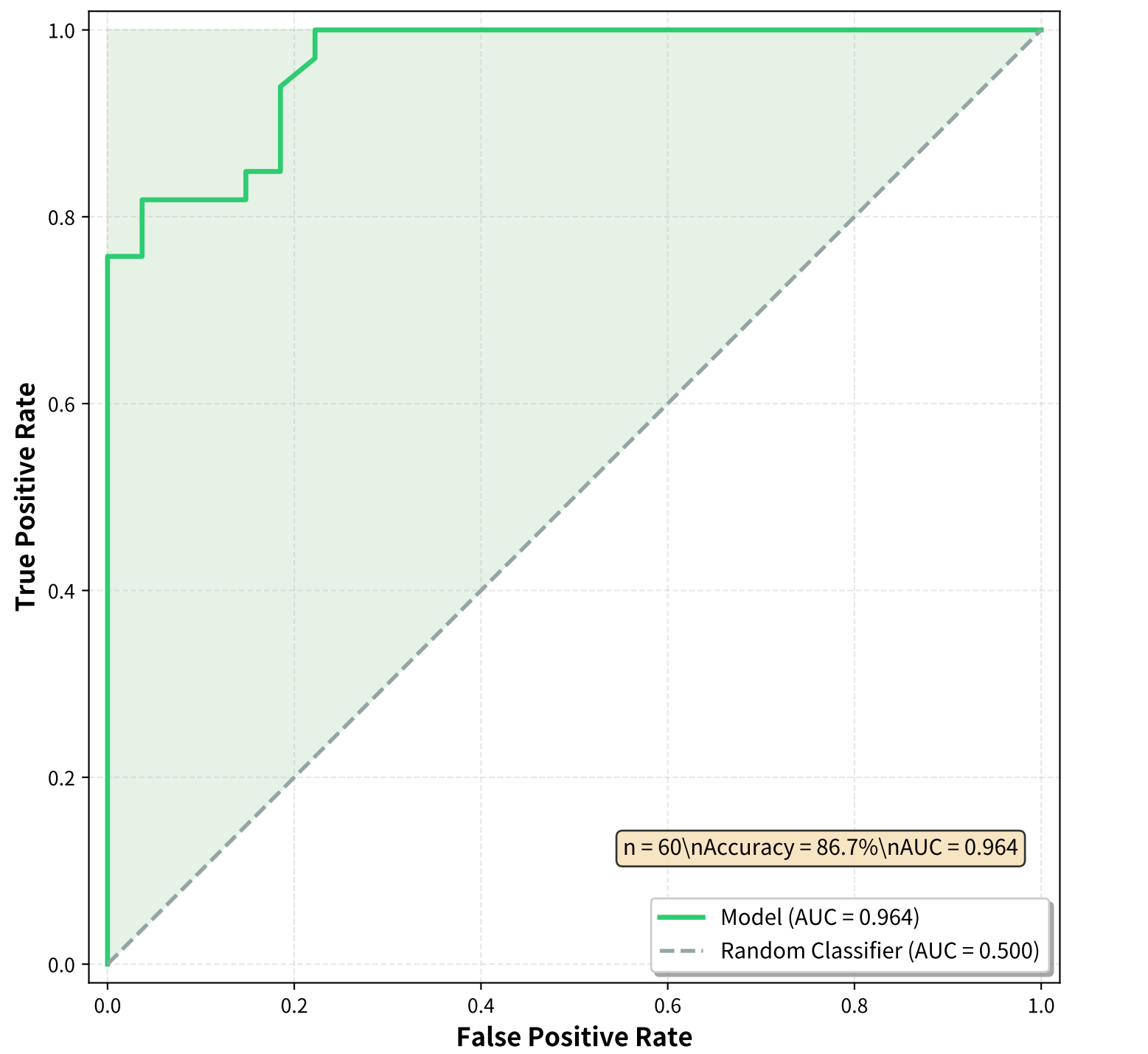
Figure 8.2: ROC Curve - Transplant Success Prediction Logistic Regression: success ~ d_φ
