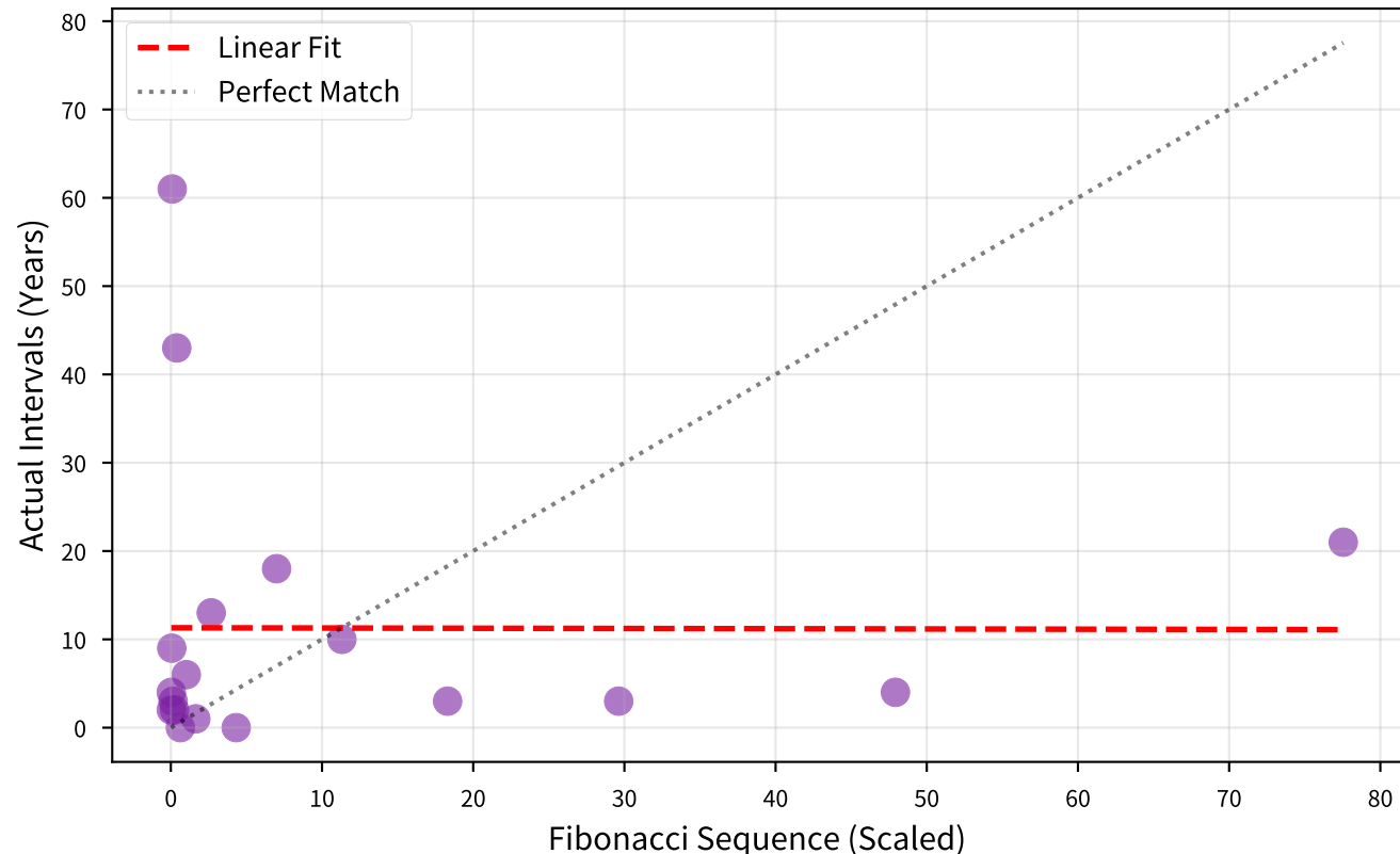
Panel B: Correlation ( r = -0.003 , p = 0.989 )
