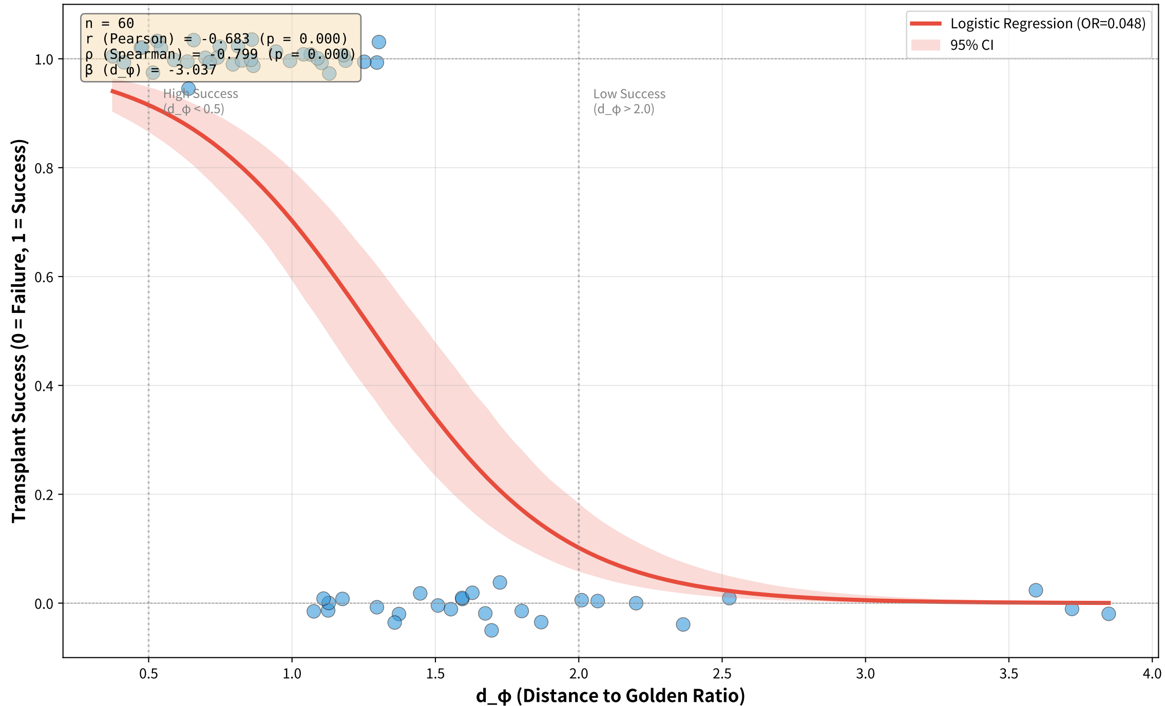
Figure 8.1: Constitutional Transplant Success vs Distance to \phi Lower d_\phi predicts higher success rate
