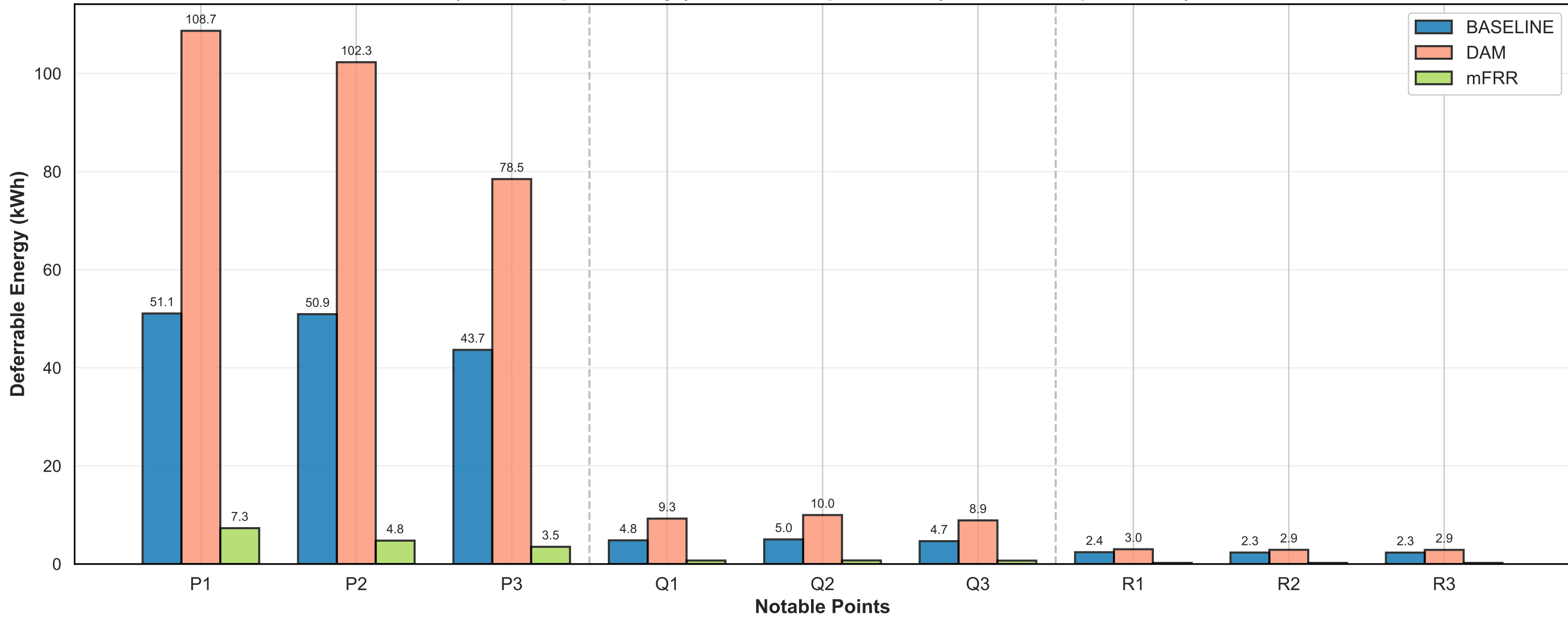
Comparison of 9 Notable Points Across Scenarios (P1-P3: Top flexibility | Q1-Q3: 75th percentile | R1-R3: 50th percentile)
