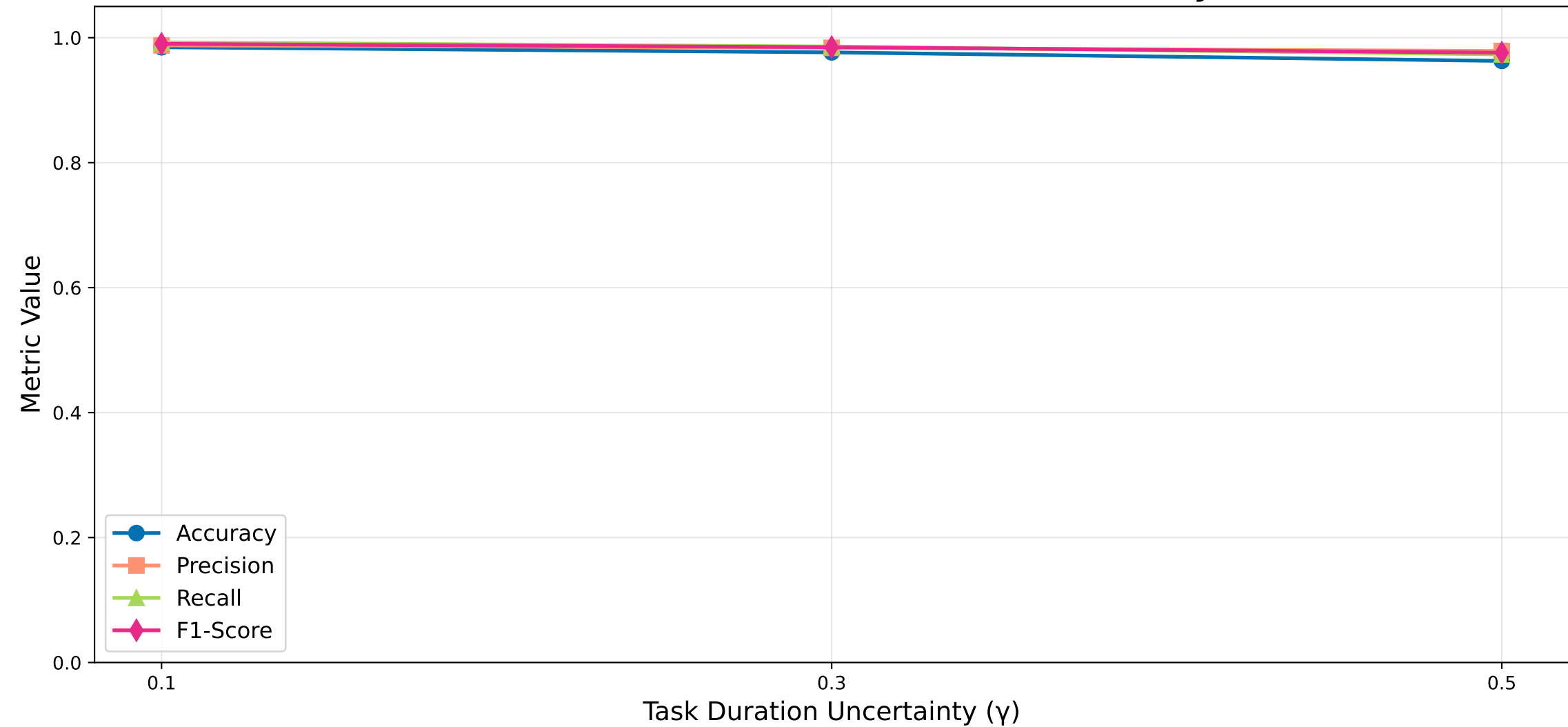
Classification Metrics vs Duration Uncertainty
