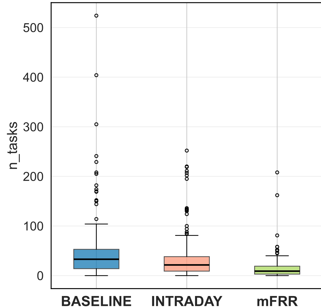
Task Count
