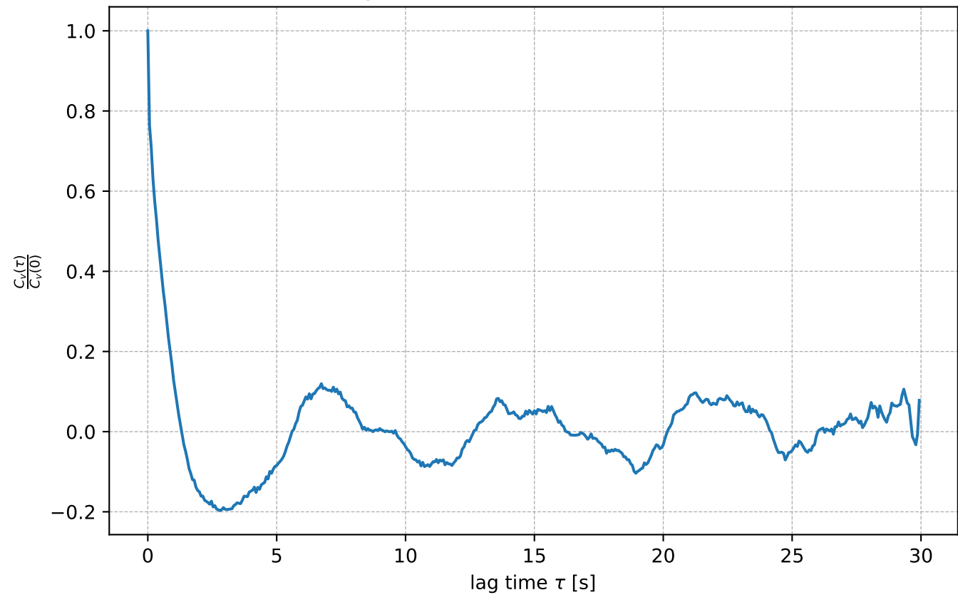
Temporal autocorrelation of velocities
