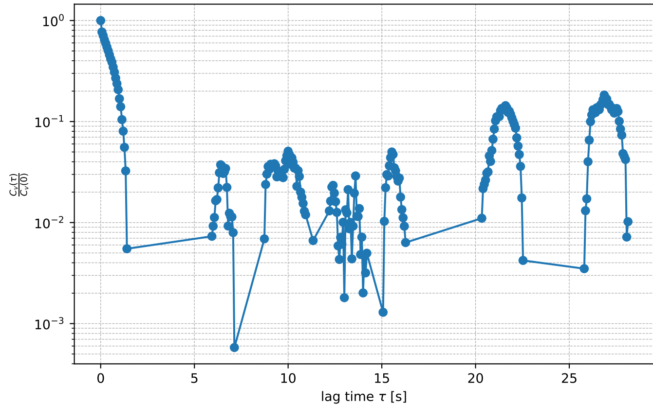
Temporal autocorrelation of velocities in semilog scale
