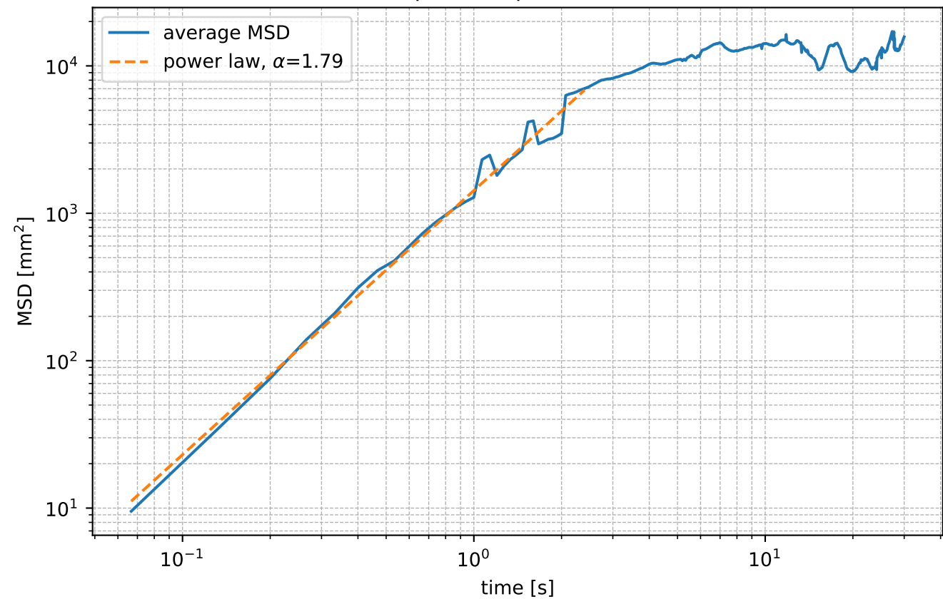
Mean Square Displacement (MSD)
