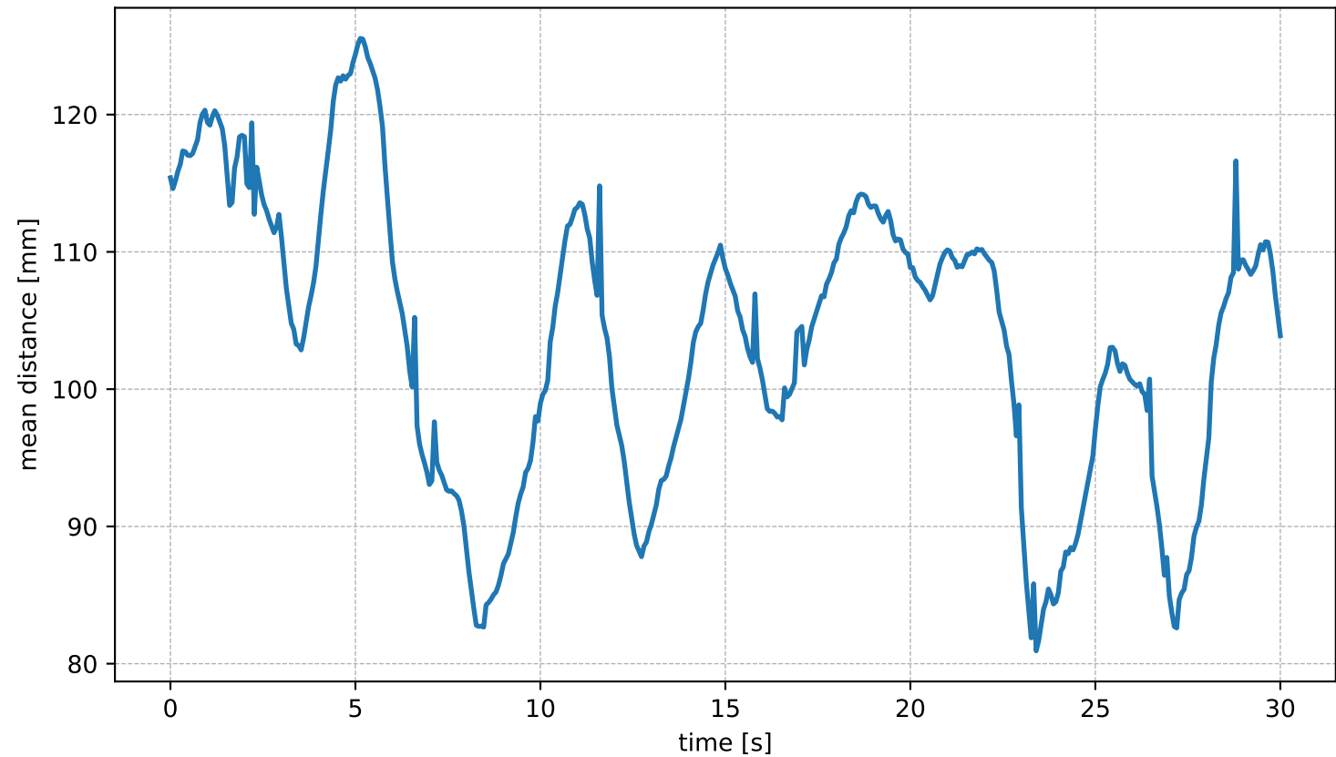
Mean pairwise distance between fish frame by frame
