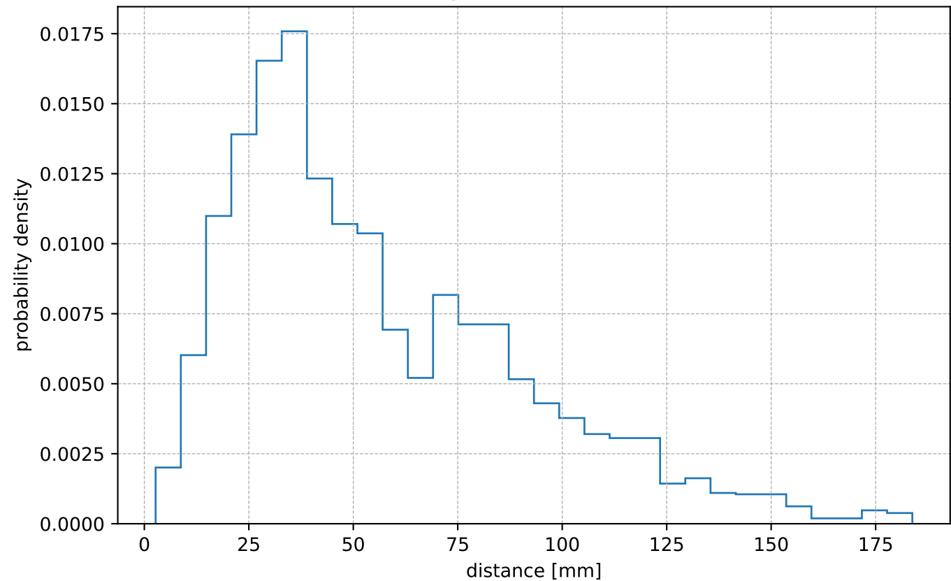
Nearest neighbor distance distribution
