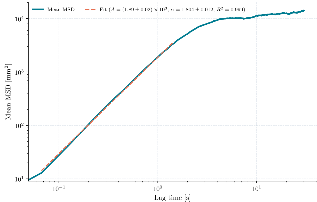
Mean square displacement, fit up to 1.5 s
