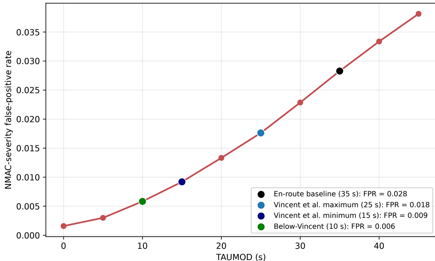
NMAC-Severity False-Alarm Rate vs. TAUMOD (ZTHR = 450 ft; N = 60,000 sample encounters)
