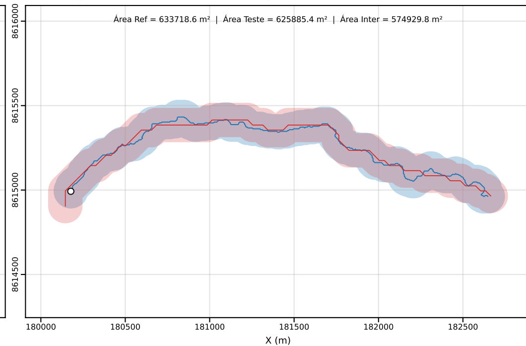
Classe D | PEC-PCD (Horizontal)=100.00 m | dm = 29.51
