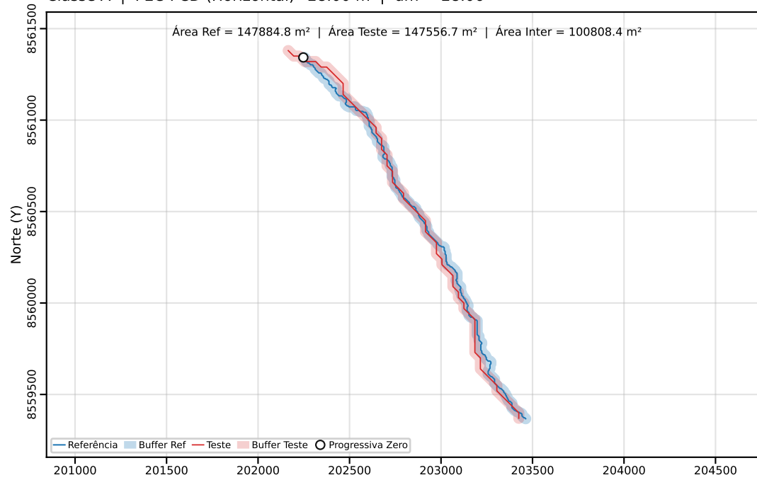
Classe C | PEC-PCD (Horizontal)=80.00 m | dm = 28.02
