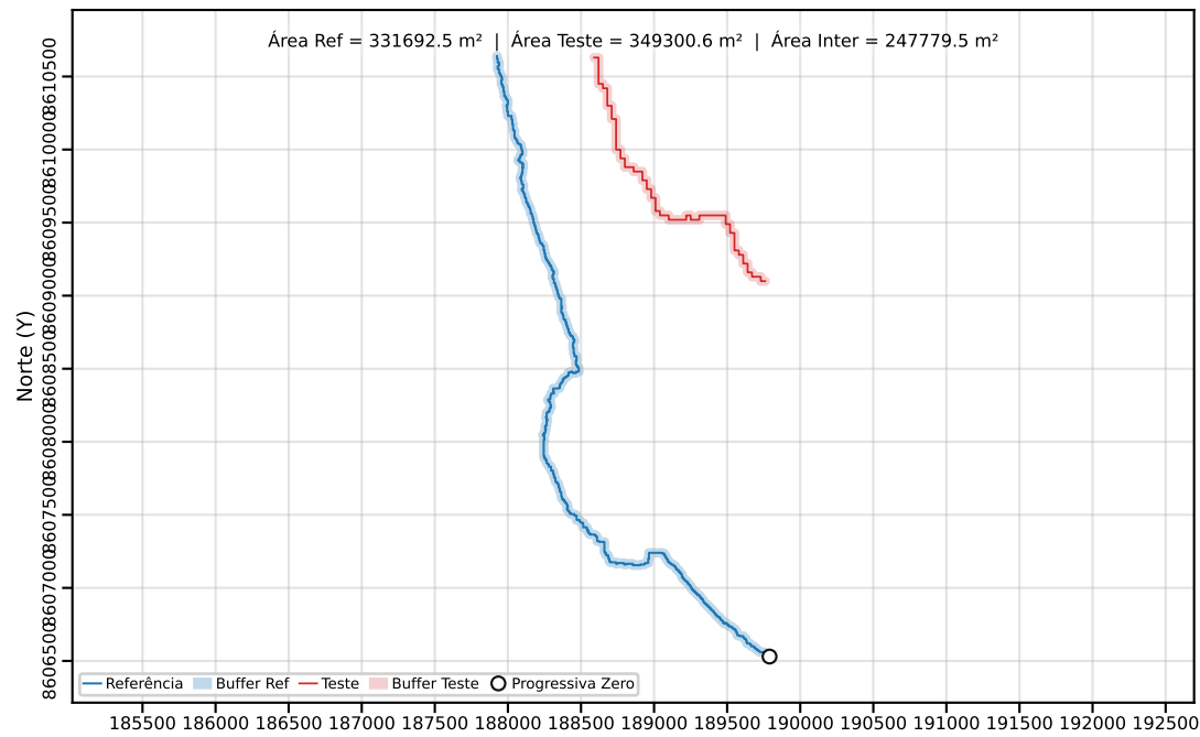
Classe C | PEC-PCD (Horizontal)=80.00 m | dm = 20.83
