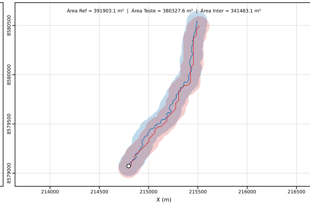
Classe D | PEC-PCD (Horizontal)=100.00 m | dm = 41.65
