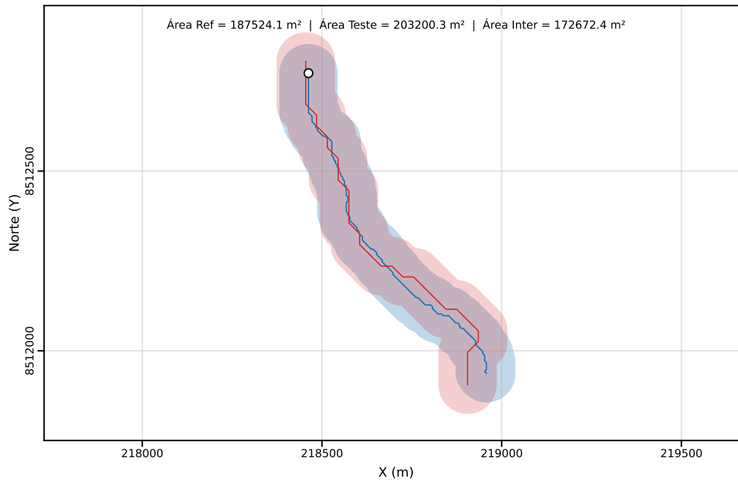
Classe C | PEC-PCD (Horizontal)=80.00 m | dm = 18.37
