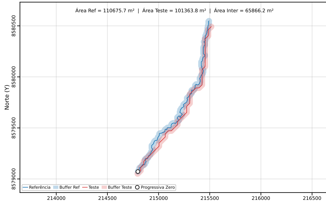
Classe C | PEC-PCD (Horizontal)=80.00 m | dm = 41.05
