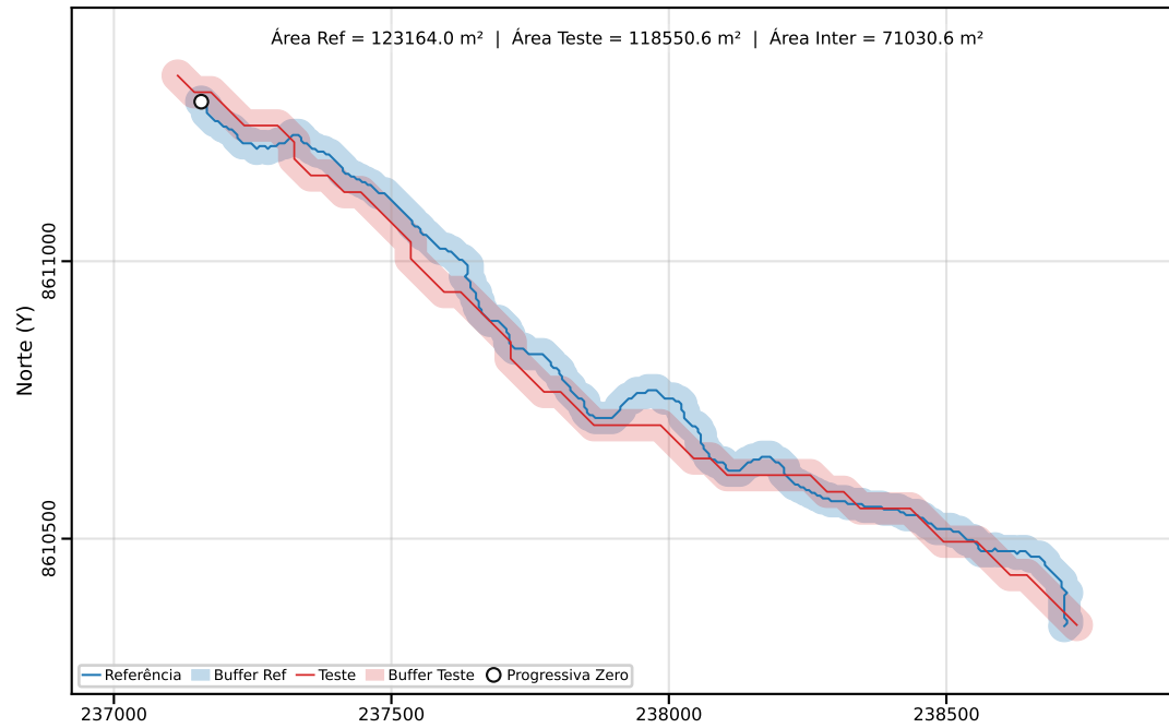
Classe C | PEC-PCD (Horizontal)=80.00 m | dm = 39.39
