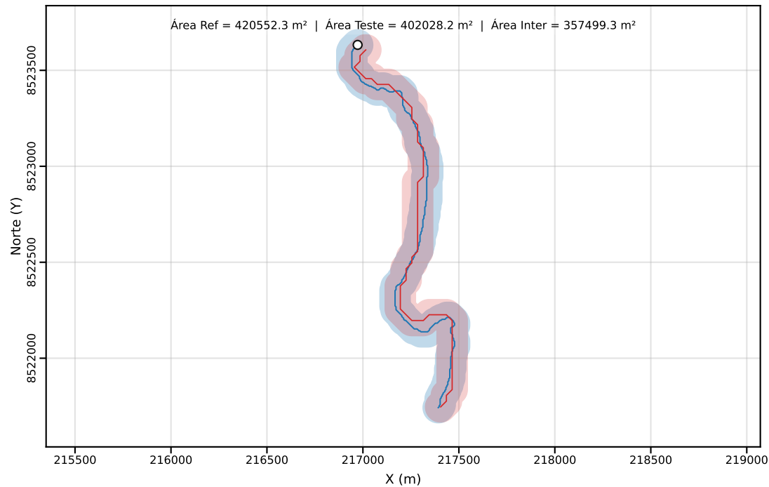
Classe C | PEC-PCD (Horizontal)=80.00 m | dm = 39.42
