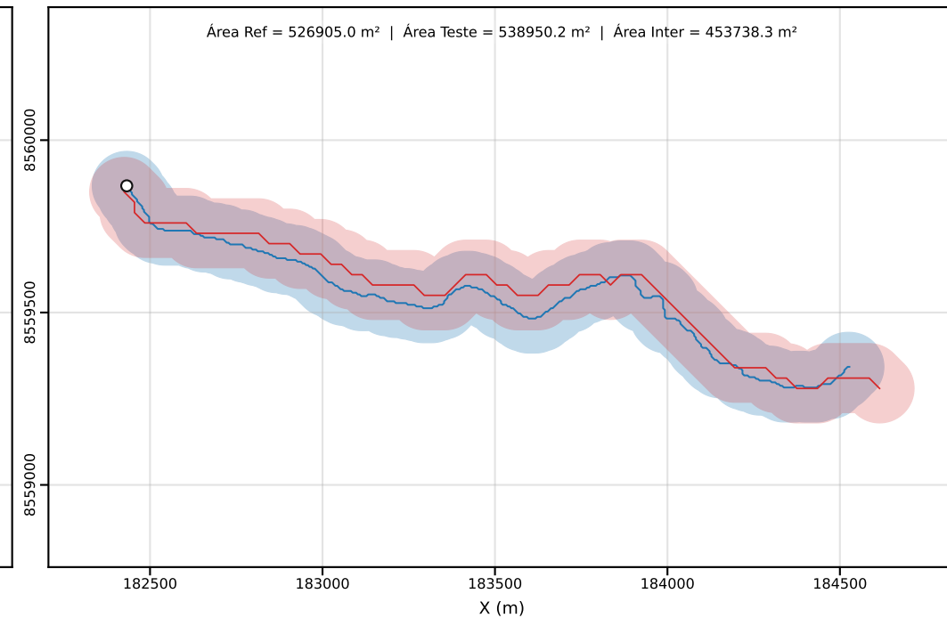
Classe D | PEC-PCD (Horizontal)=100.00 m | dm = 42.65
