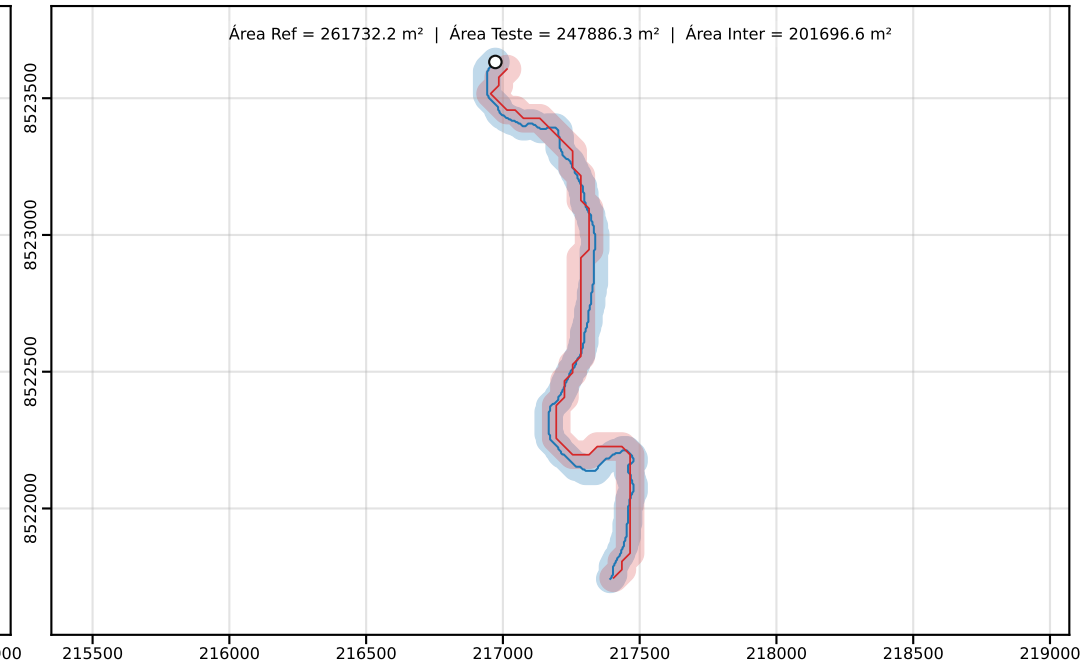
Classe D | PEC-PCD (Horizontal)=100.00 m | dm = 40.05
