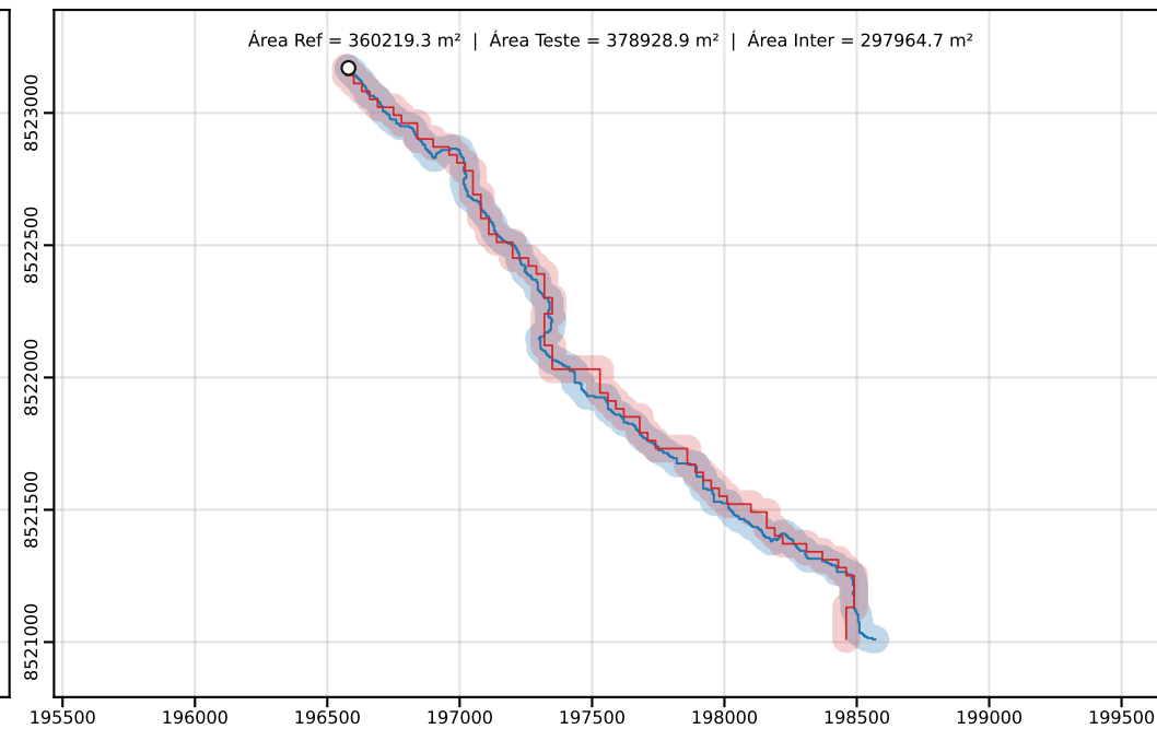
Classe D | PEC-PCD (Horizontal)=100.00 m | dm = 27.90
