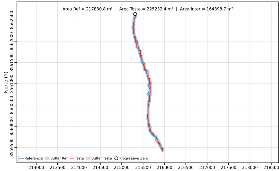
Classe C | PEC-PCD (Horizontal)=80.00 m | dm = 19.84
