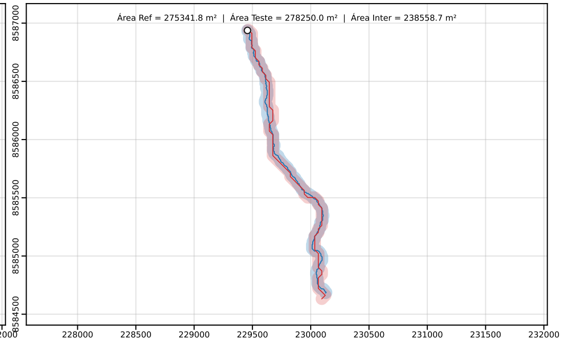
Classe D | PEC-PCD (Horizontal)=100.00 m | dm = 19.49
