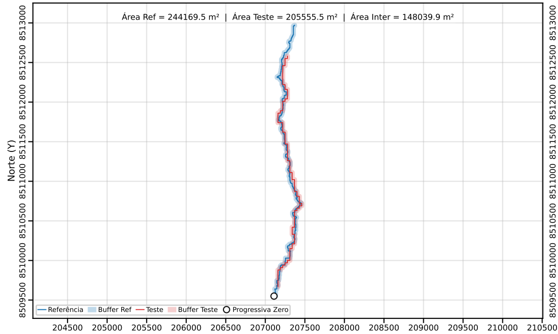
Classe C | PEC-PCD (Horizontal)=80.00 m | dm = 68.70
