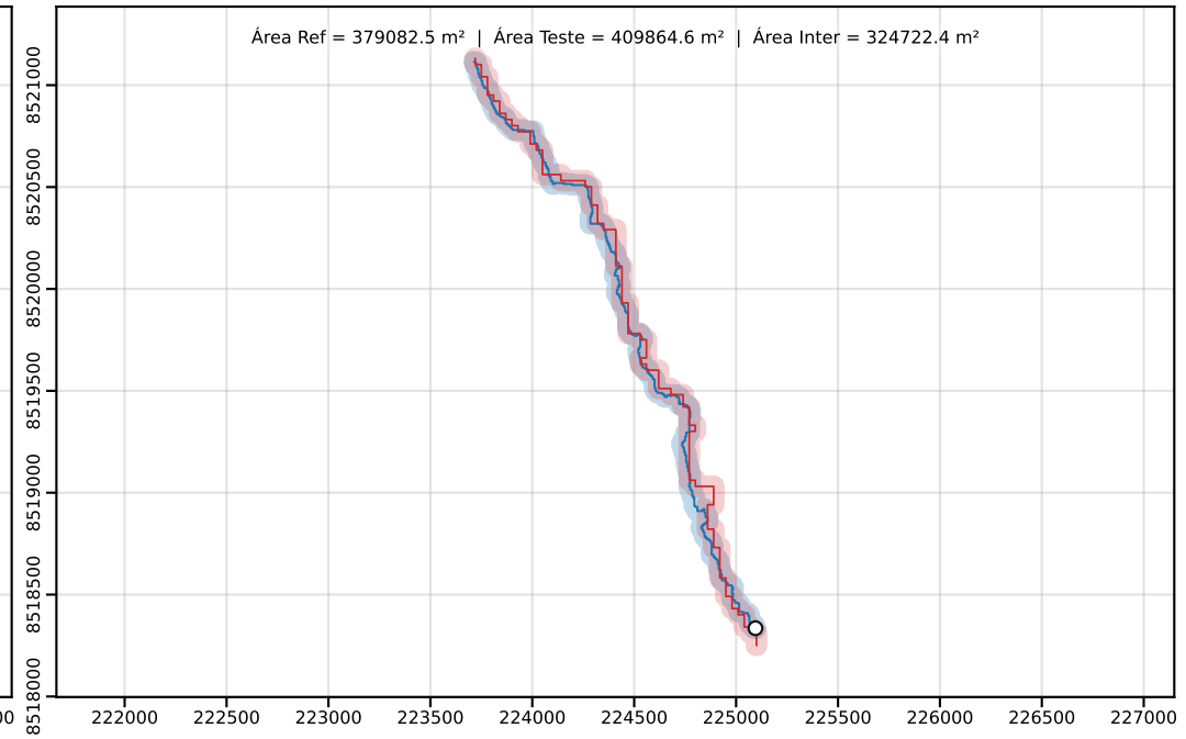
Classe D | PEC-PCD (Horizontal)=100.00 m | dm = 20.34
