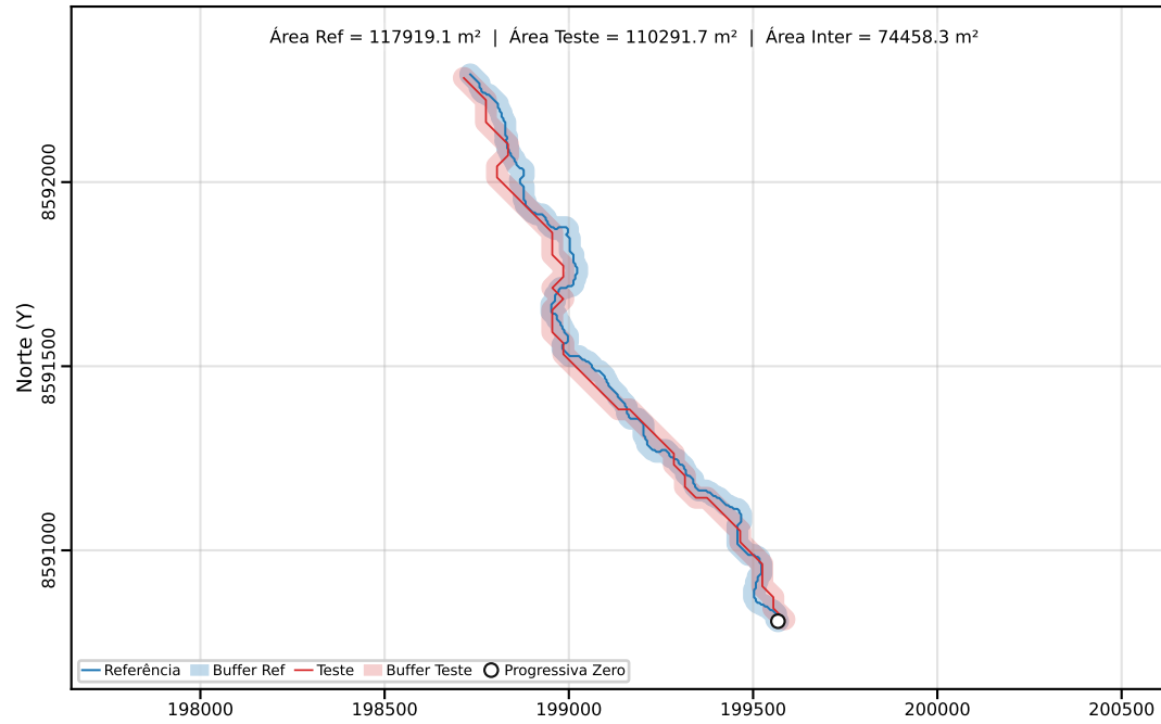
Classe C | PEC-PCD (Horizontal)=80.00 m | dm = 36.05
