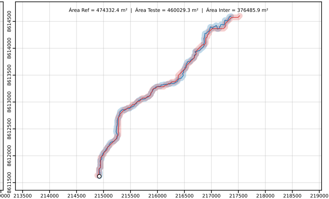
Classe D | PEC-PCD (Horizontal)=100.00 m | dm = 35.35
