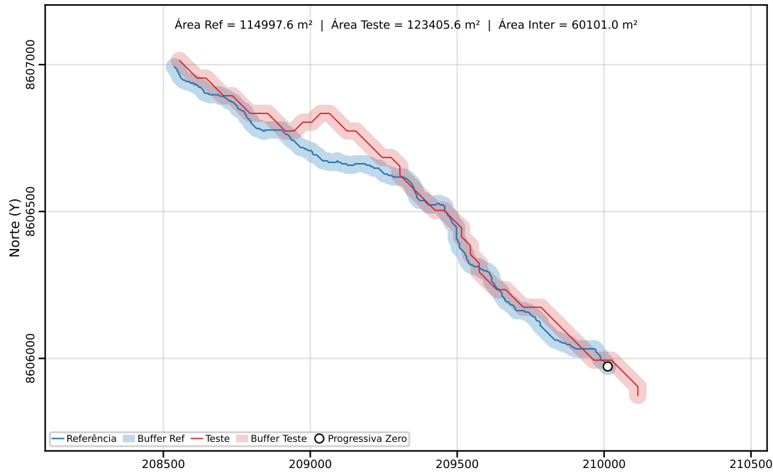
Classe C | PEC-PCD (Horizontal)=80.00 m | dm = 45.85
