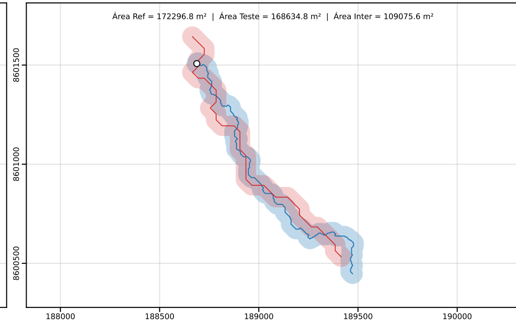
Classe D | PEC-PCD (Horizontal)=100.00 m | dm = 65.72
