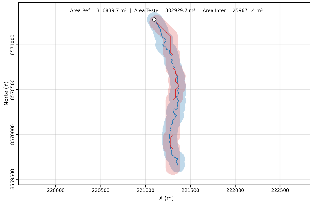
Classe C | PEC-PCD (Horizontal)=80.00 m | dm = 47.43
