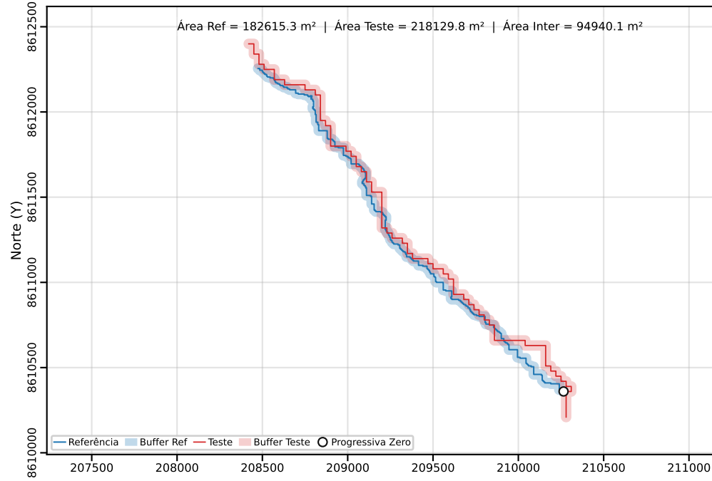
Classe C | PEC-PCD (Horizontal)=80.00 m | dm = 36.07
