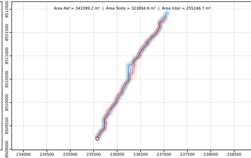
Classe D | PEC-PCD (Horizontal)=100.00 m | dm = 49.17
