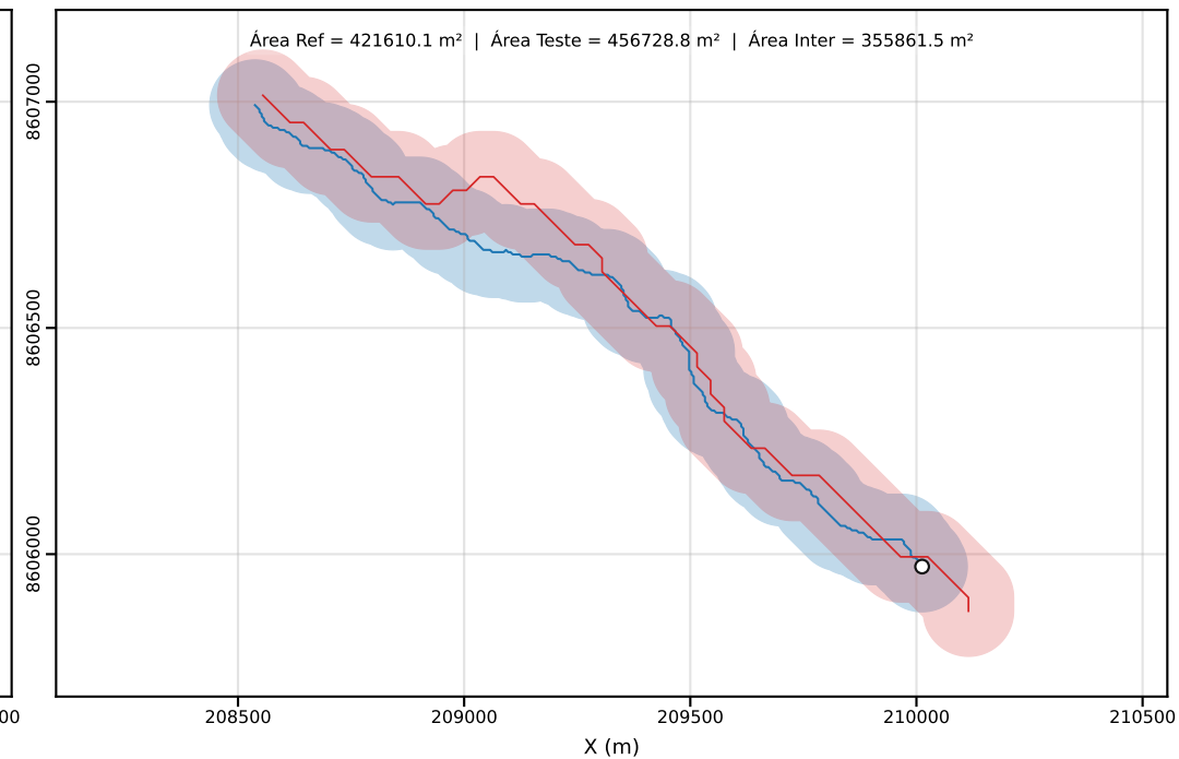
Classe D | PEC-PCD (Horizontal)=100.00 m | dm = 45.22
