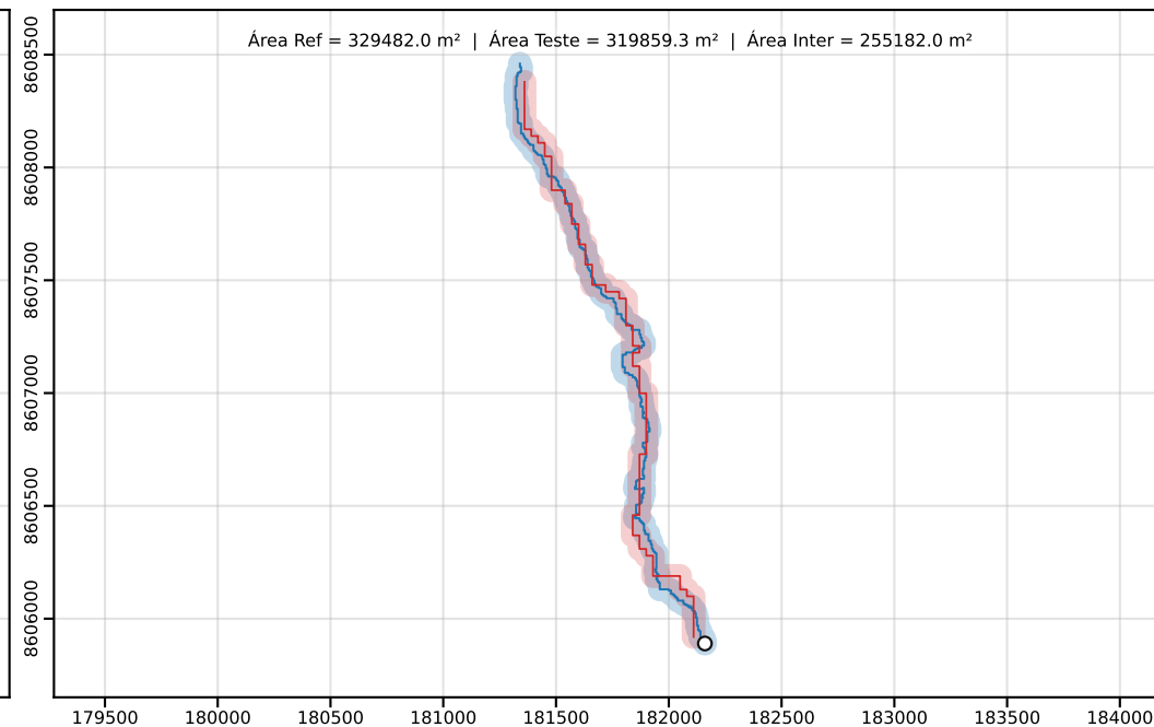
Classe D | PEC-PCD (Horizontal)=100.00 m | dm = 42.53
