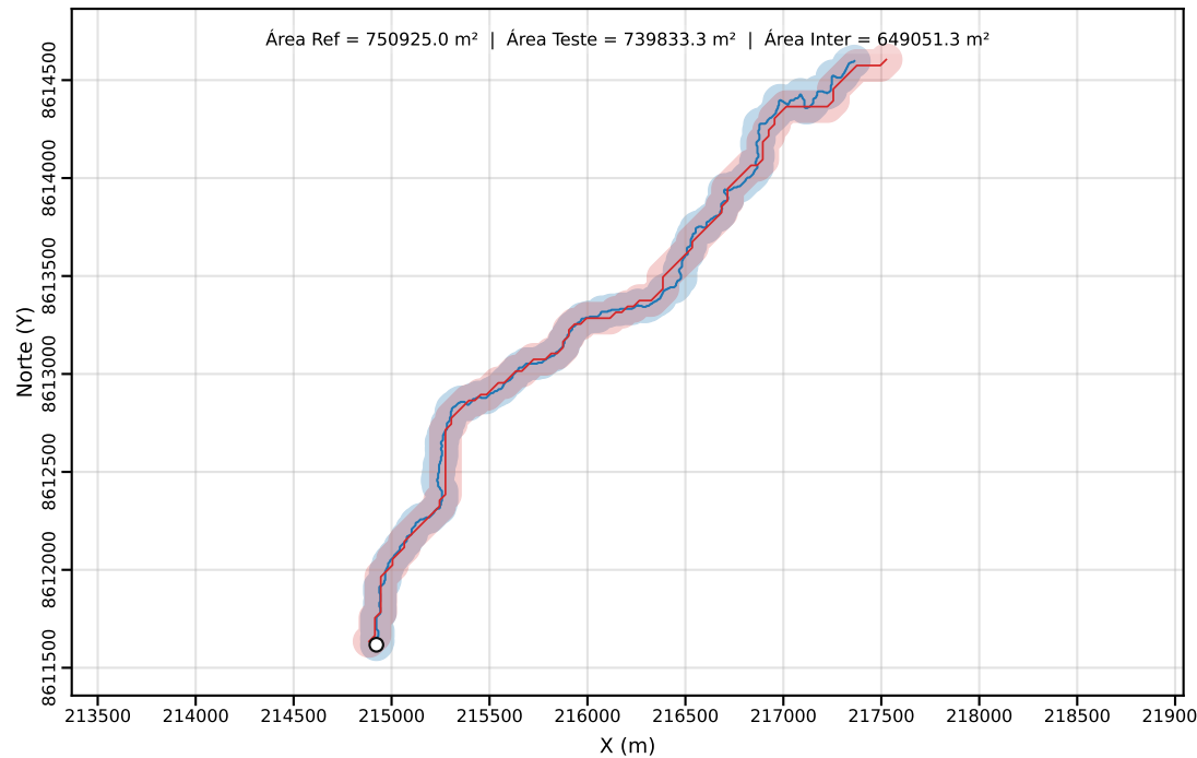
Classe C | PEC-PCD (Horizontal)=80.00 m | dm = 34.61
