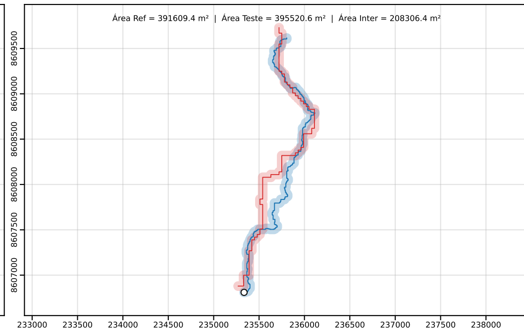
Classe D | PEC-PCD (Horizontal)=100.00 m | dm = 90.64
