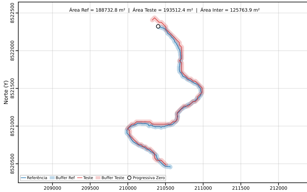
Classe C | PEC-PCD (Horizontal)=80.00 m | dm = 30.16
