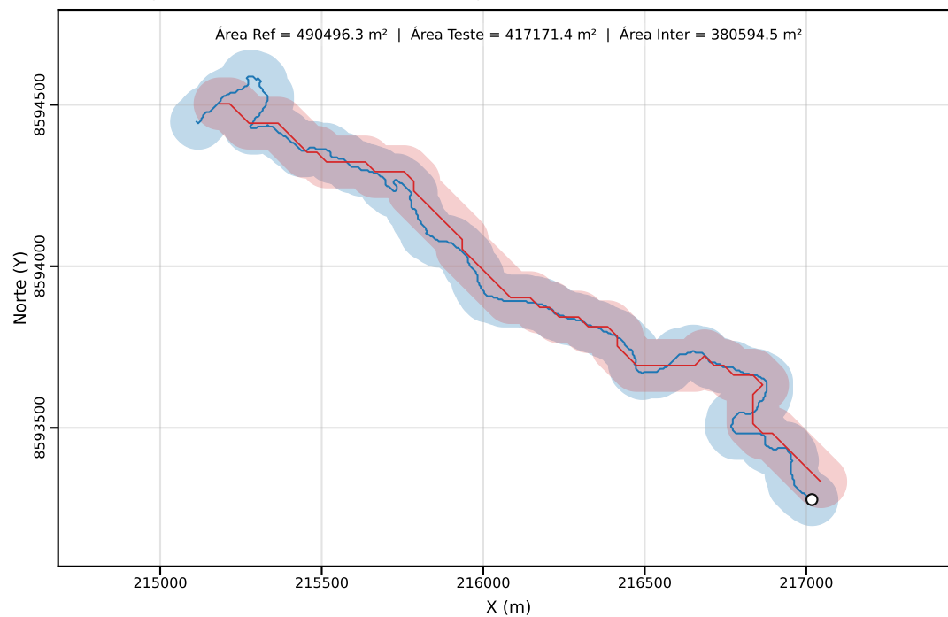
Classe C | PEC-PCD (Horizontal)=80.00 m | dm = 66.21
