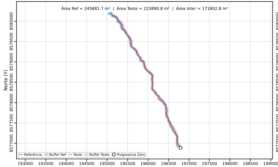
Classe C | PEC-PCD (Horizontal)=80.00 m | dm = 35.04
