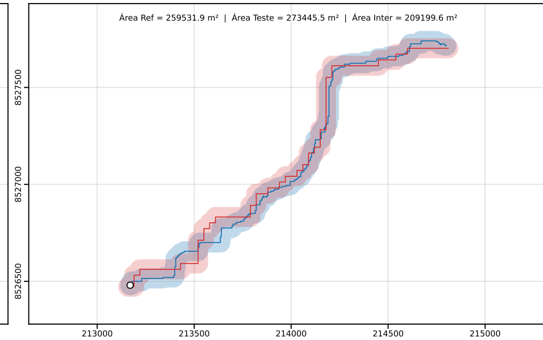
Classe D | PEC-PCD (Horizontal)=100.00 m | dm = 26.92
