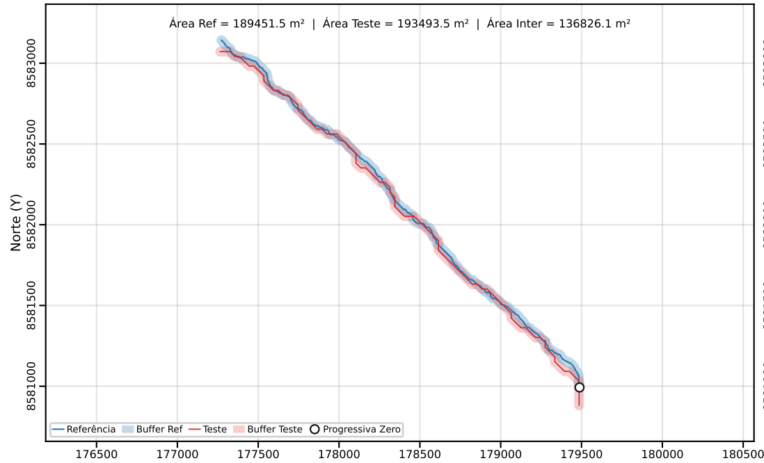
Classe C | PEC-PCD (Horizontal)=80.00 m | dm = 23.80
