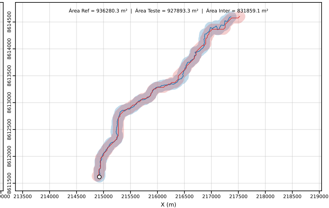
Classe D | PEC-PCD (Horizontal)=100.00 m | dm = 35.35
