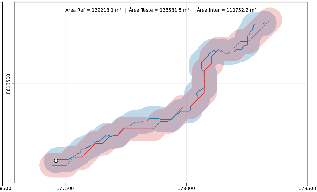
Classe D | PEC-PCD (Horizontal)=100.00 m | dm = 22.16
