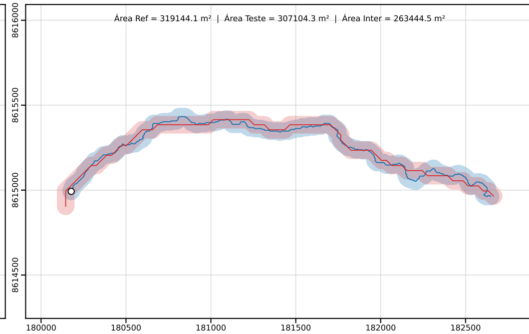
Classe D | PEC-PCD (Horizontal)=100.00 m | dm = 29.51
