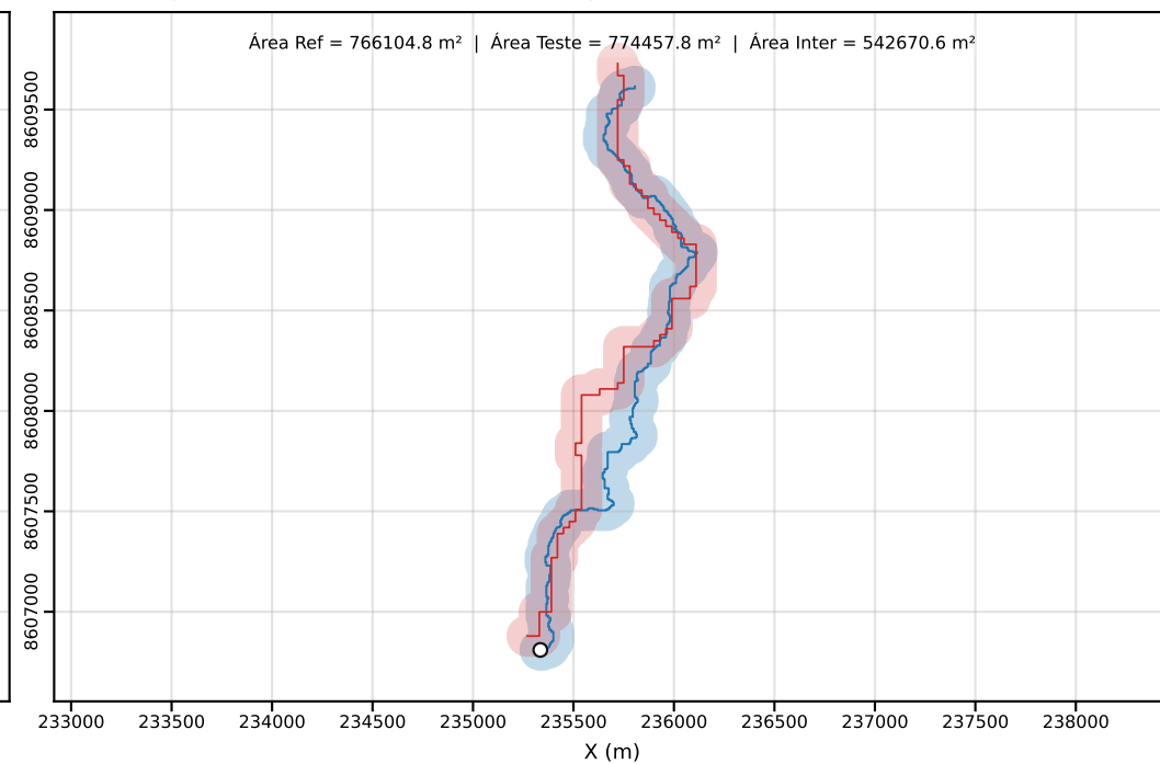
Classe D | PEC-PCD (Horizontal)=100.00 m | dm = 90.64
