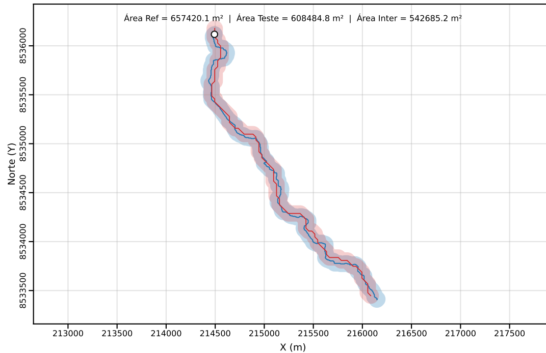
Classe C | PEC-PCD (Horizontal)=80.00 m | dm = 47.39
