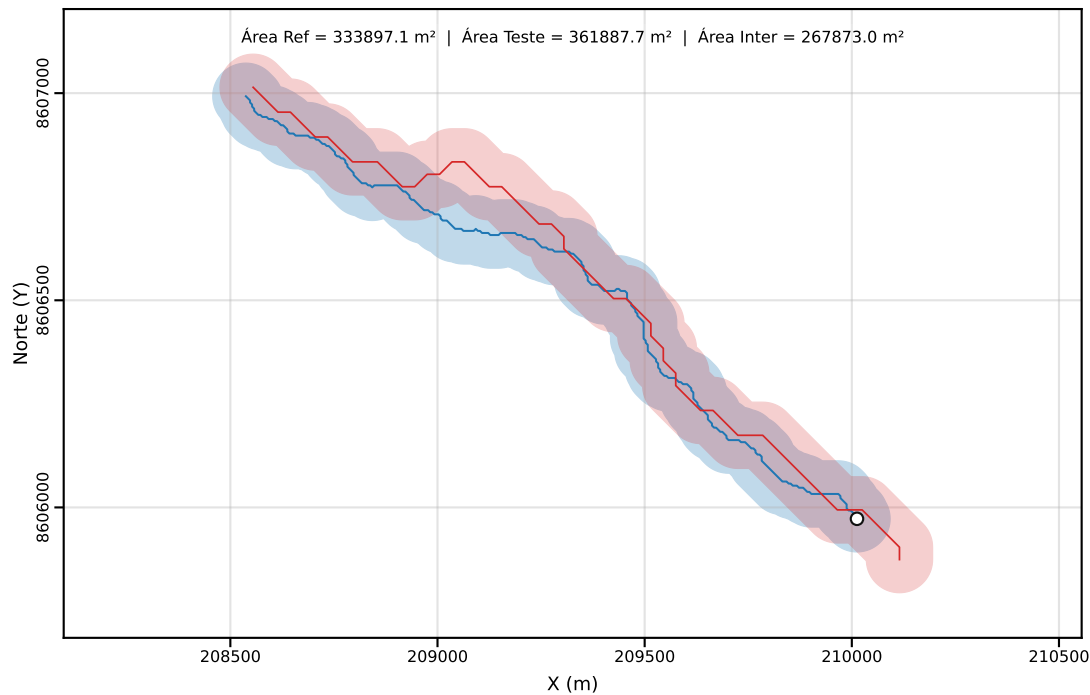
Classe C | PEC-PCD (Horizontal)=80.00 m | dm = 45.85
