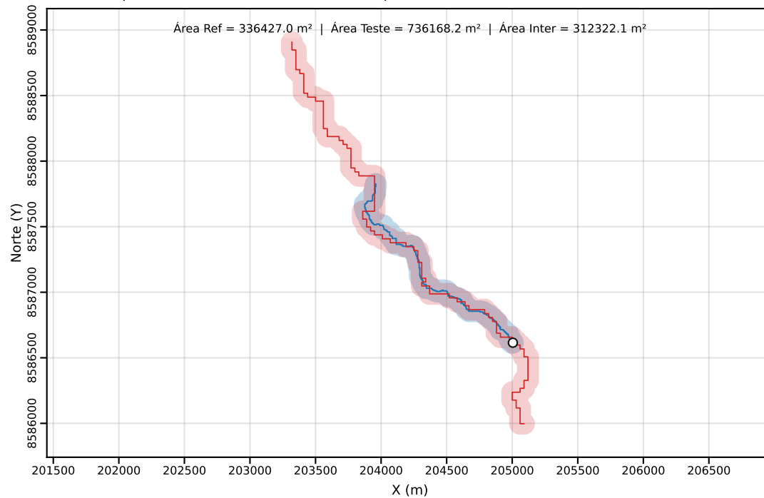
Classe C | PEC-PCD (Horizontal)=80.00 m | dm = 8.23
