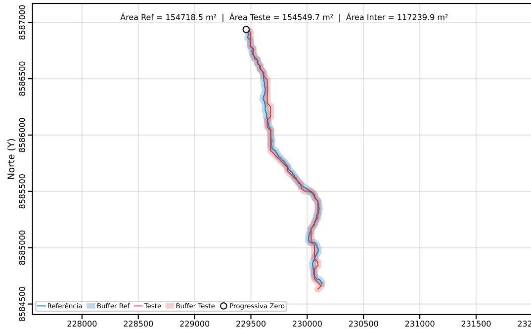
Classe C | PEC-PCD (Horizontal)=80.00 m | dm = 19.95
