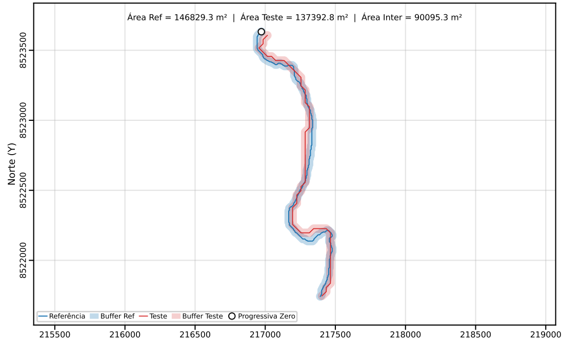
Classe C | PEC-PCD (Horizontal)=80.00 m | dm = 39.42
