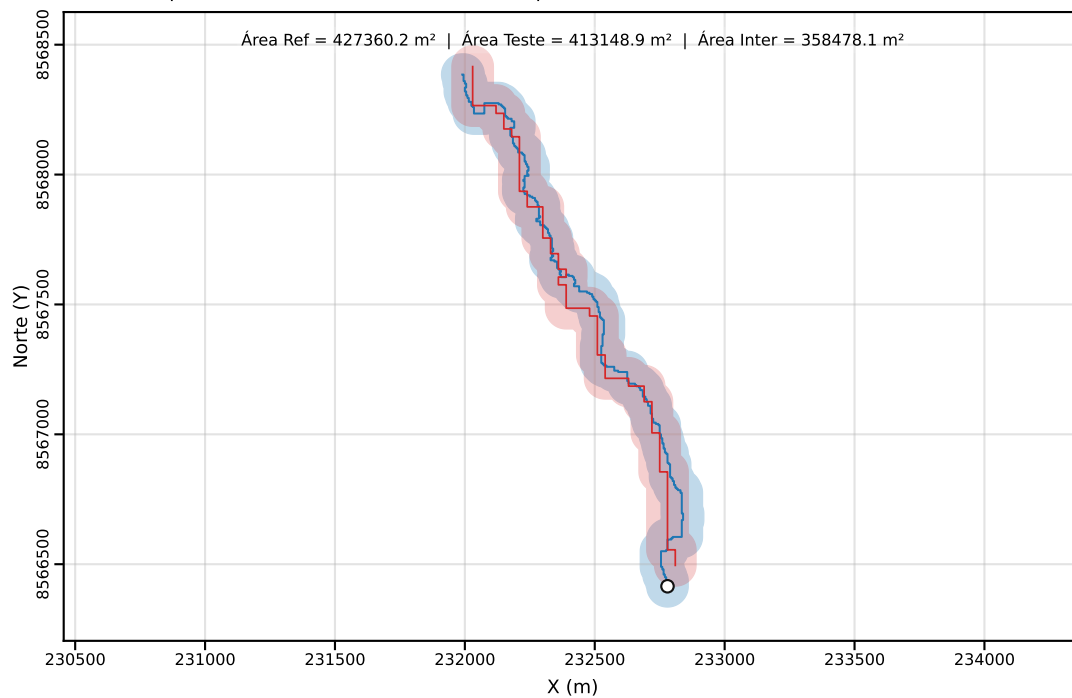
Classe C | PEC-PCD (Horizontal)=80.00 m | dm = 41.90
