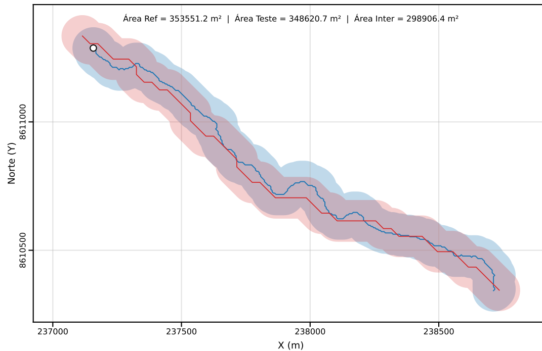
Classe C | PEC-PCD (Horizontal)=80.00 m | dm = 39.39
