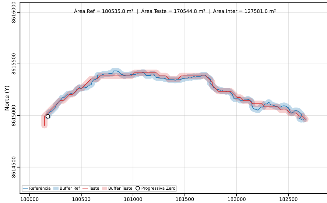
Classe C | PEC-PCD (Horizontal)=80.00 m | dm = 29.28
