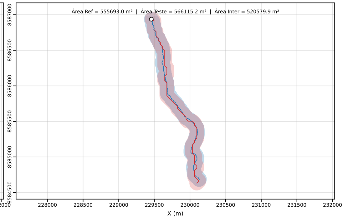
Classe D | PEC-PCD (Horizontal)=100.00 m | dm = 19.49
