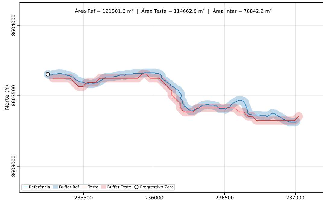
Classe C | PEC-PCD (Horizontal)=80.00 m | dm = 44.40
