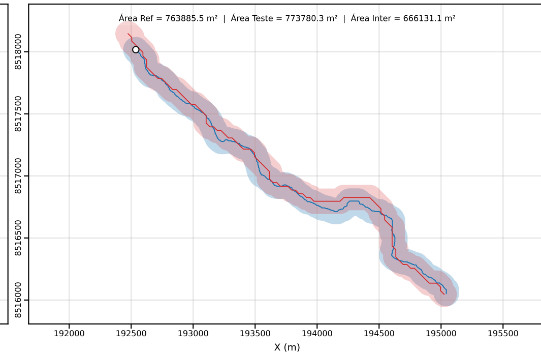
Classe D | PEC-PCD (Horizontal)=100.00 m | dm = 39.69
