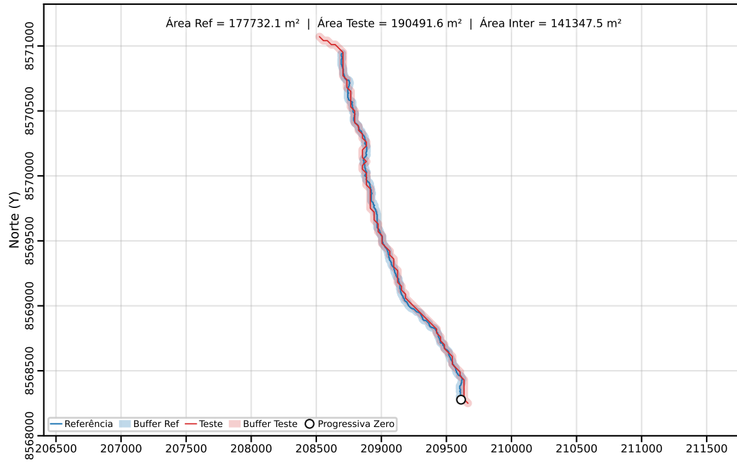
Classe C | PEC-PCD (Horizontal)=80.00 m | dm = 15.26
