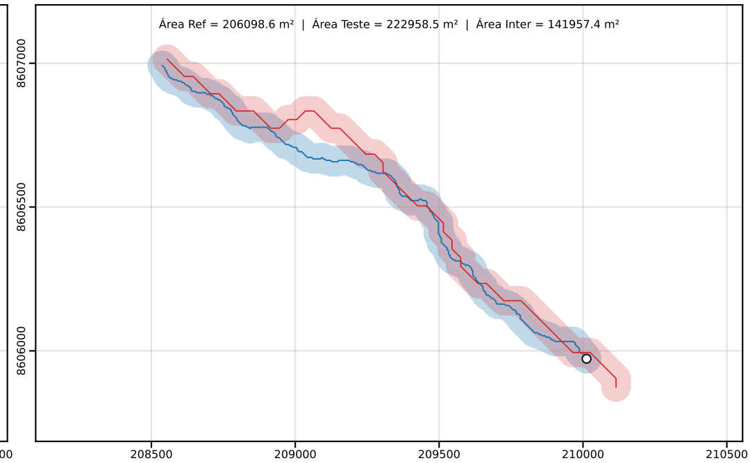
Classe D | PEC-PCD (Horizontal)=100.00 m | dm = 45.22
