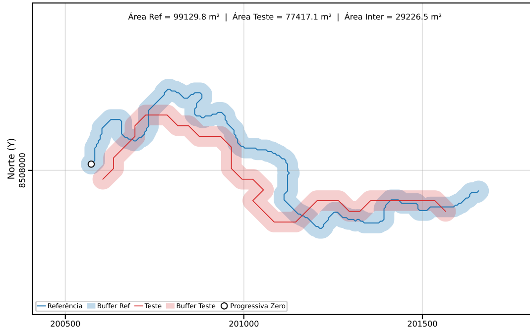
Classe C | PEC-PCD (Horizontal)=80.00 m | dm = 100.75
