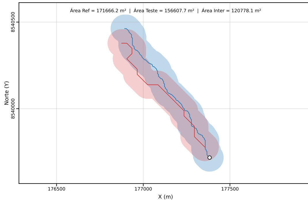
Classe C | PEC-PCD (Horizontal)=80.00 m | dm = 81.67
