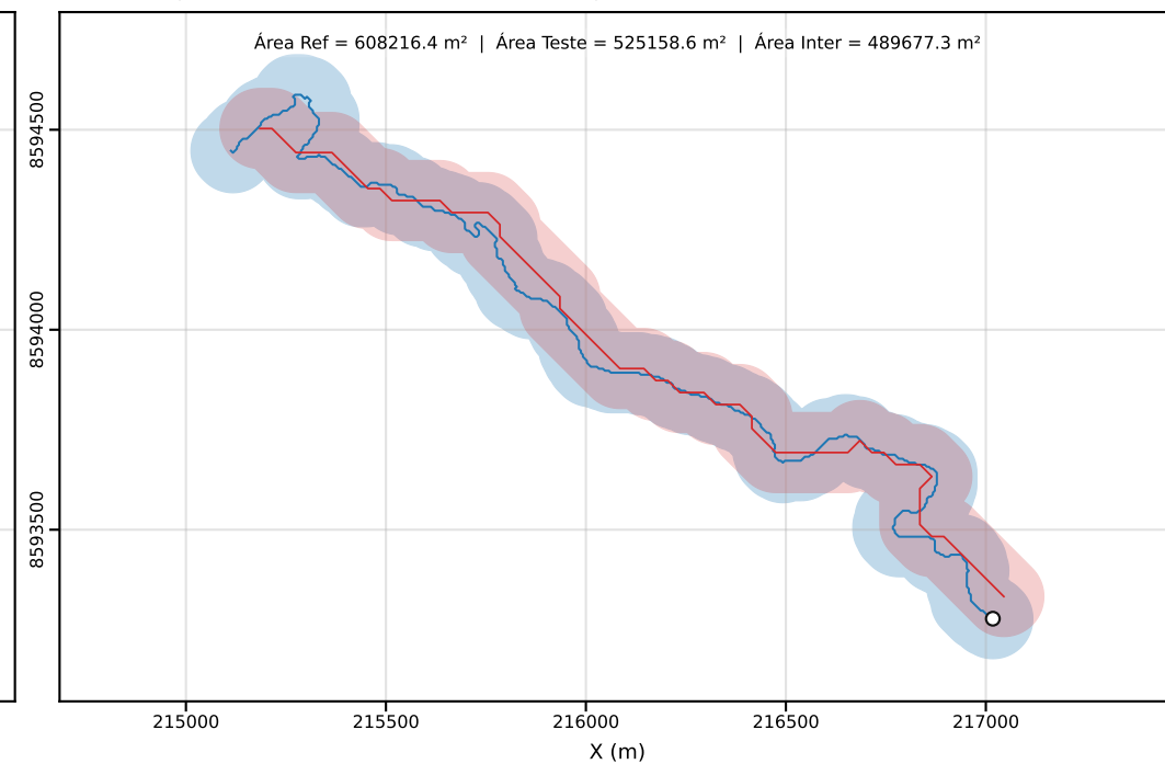
Classe D | PEC-PCD (Horizontal)=100.00 m | dm = 70.91
