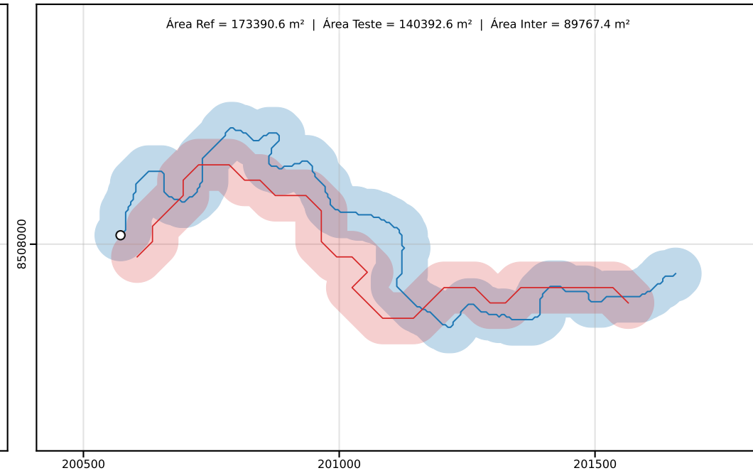
Classe D | PEC-PCD (Horizontal)=100.00 m | dm = 106.26
