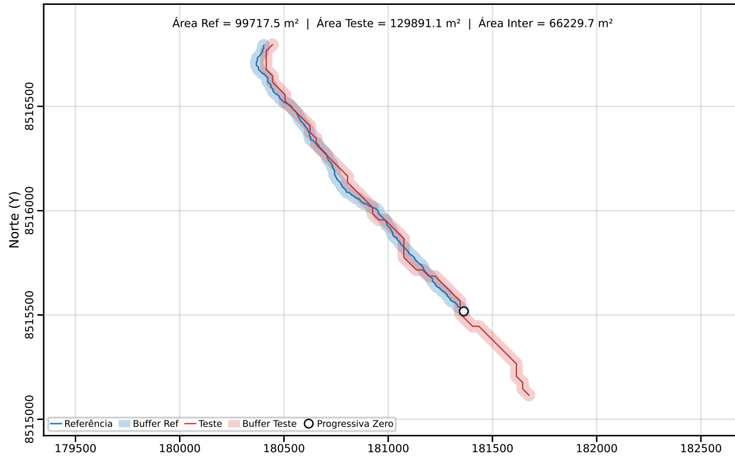
Classe C | PEC-PCD (Horizontal)=80.00 m | dm = 22.28
