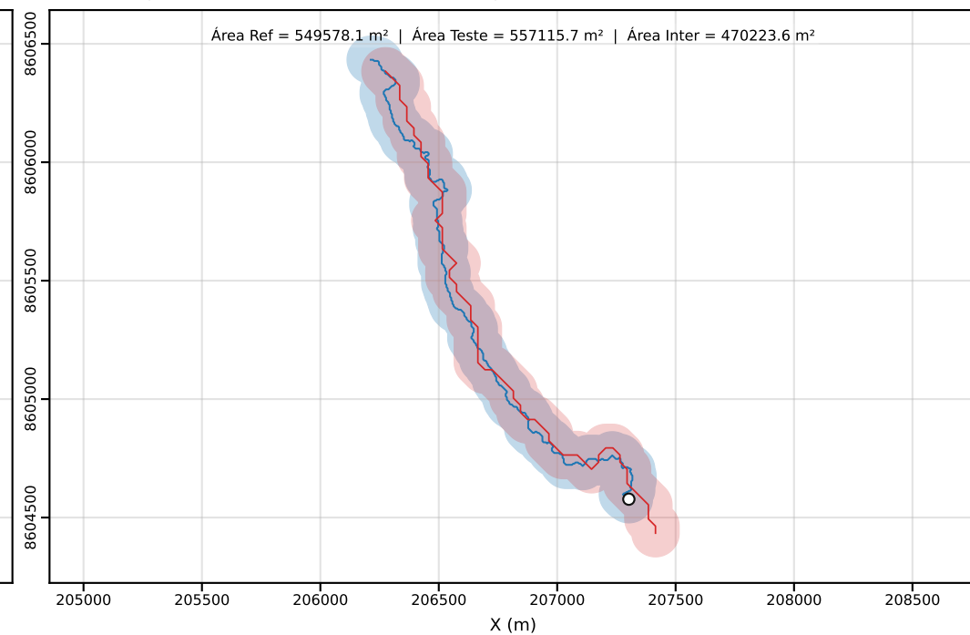
Classe D | PEC-PCD (Horizontal)=100.00 m | dm = 44.75
