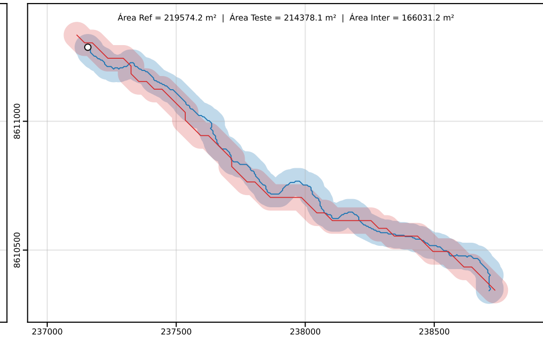
Classe D | PEC-PCD (Horizontal)=100.00 m | dm = 39.42
