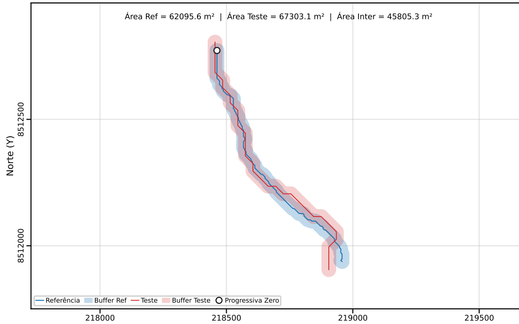
Classe C | PEC-PCD (Horizontal)=80.00 m | dm = 18.37
