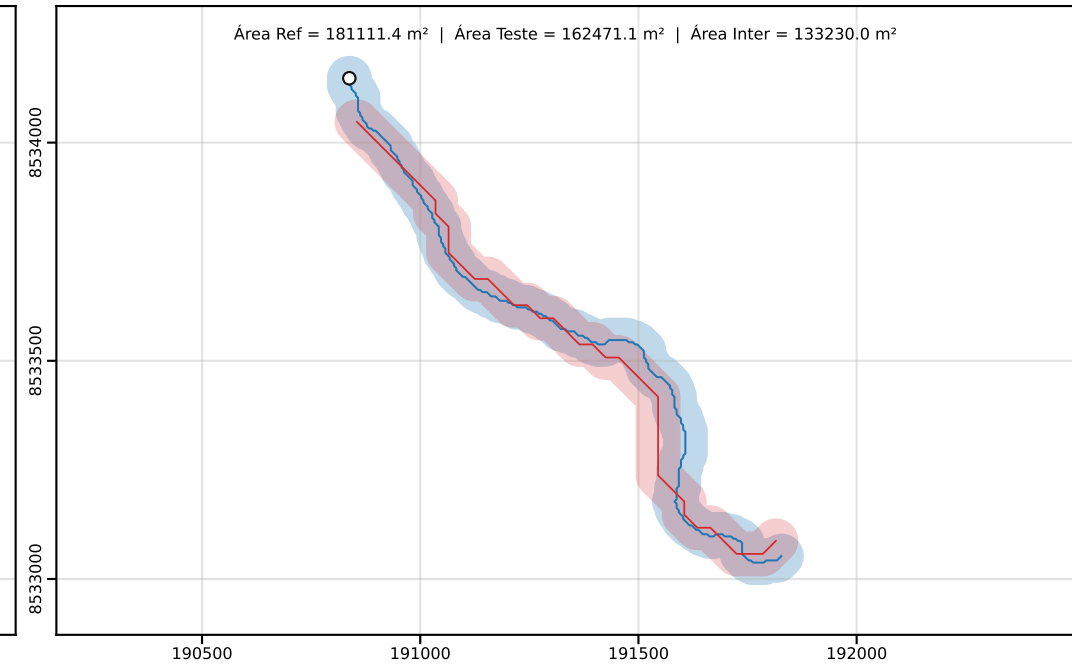
Classe D | PEC-PCD (Horizontal)=100.00 m | dm = 56.99
