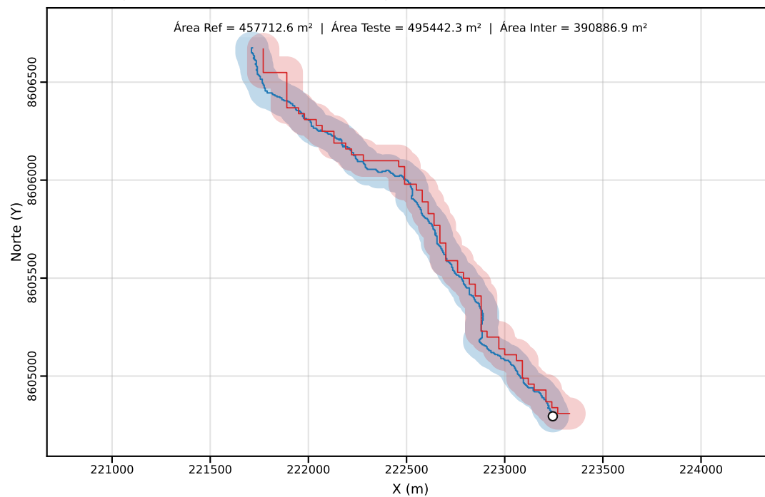
Classe C | PEC-PCD (Horizontal)=80.00 m | dm = 33.90
