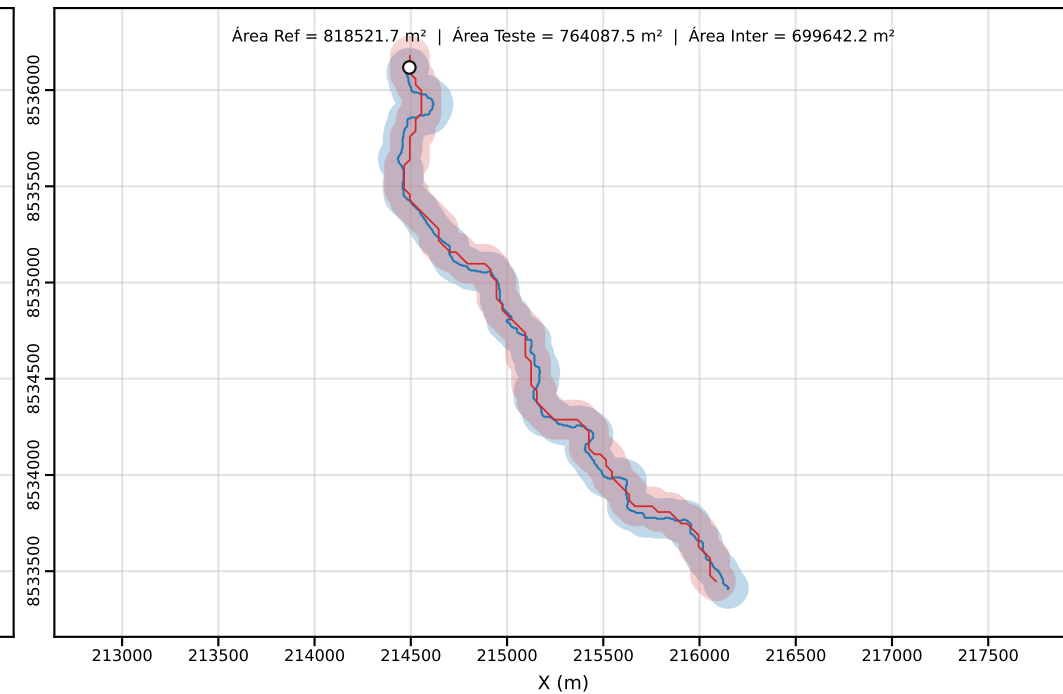
Classe D | PEC-PCD (Horizontal)=100.00 m | dm = 48.88
