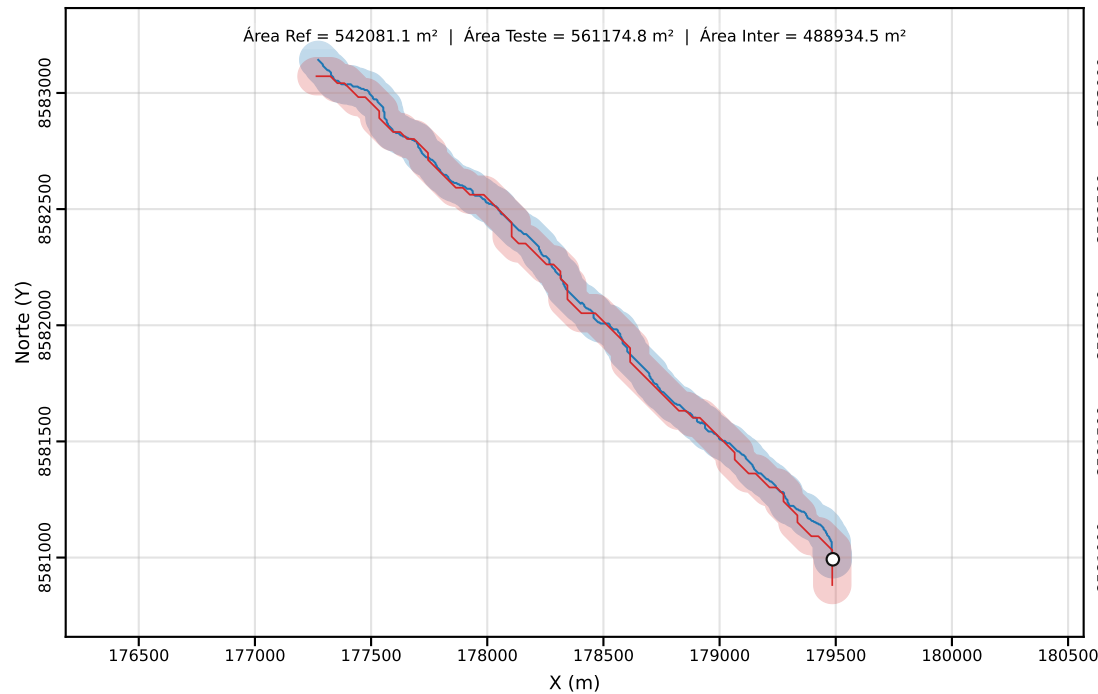
Classe C | PEC-PCD (Horizontal)=80.00 m | dm = 23.80
