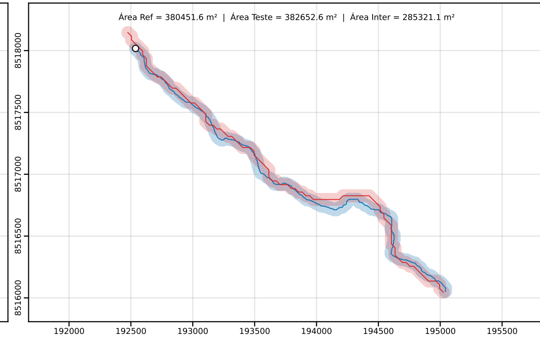
Classe D | PEC-PCD (Horizontal)=100.00 m | dm = 39.69
