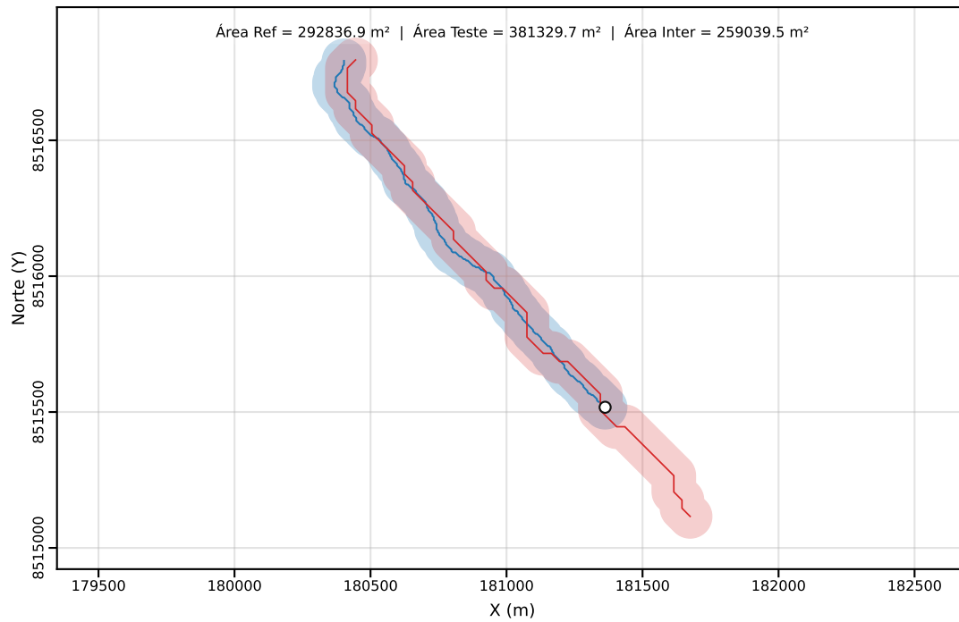
Classe C | PEC-PCD (Horizontal)=80.00 m | dm = 22.28
