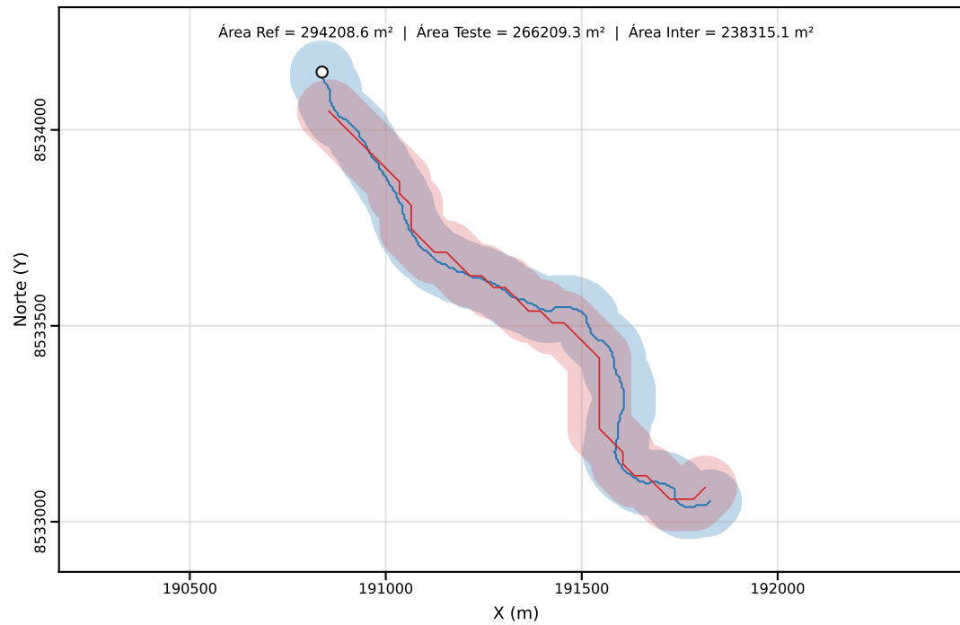
Classe C | PEC-PCD (Horizontal)=80.00 m | dm = 52.77
