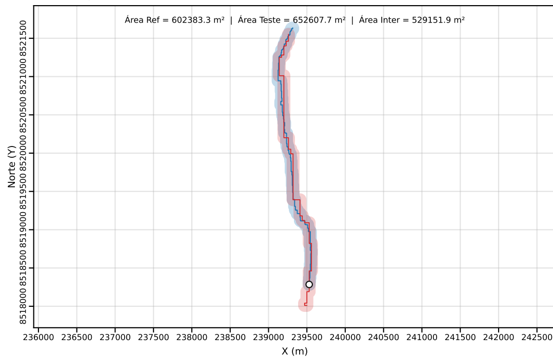
Classe C | PEC-PCD (Horizontal)=80.00 m | dm = 28.20
