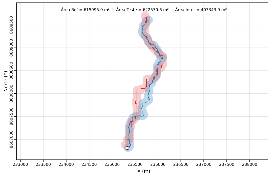
Classe C | PEC-PCD (Horizontal)=80.00 m | dm = 85.85
