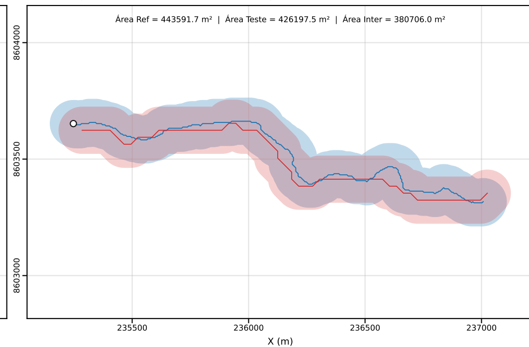
Classe D | PEC-PCD (Horizontal)=100.00 m | dm = 46.35
