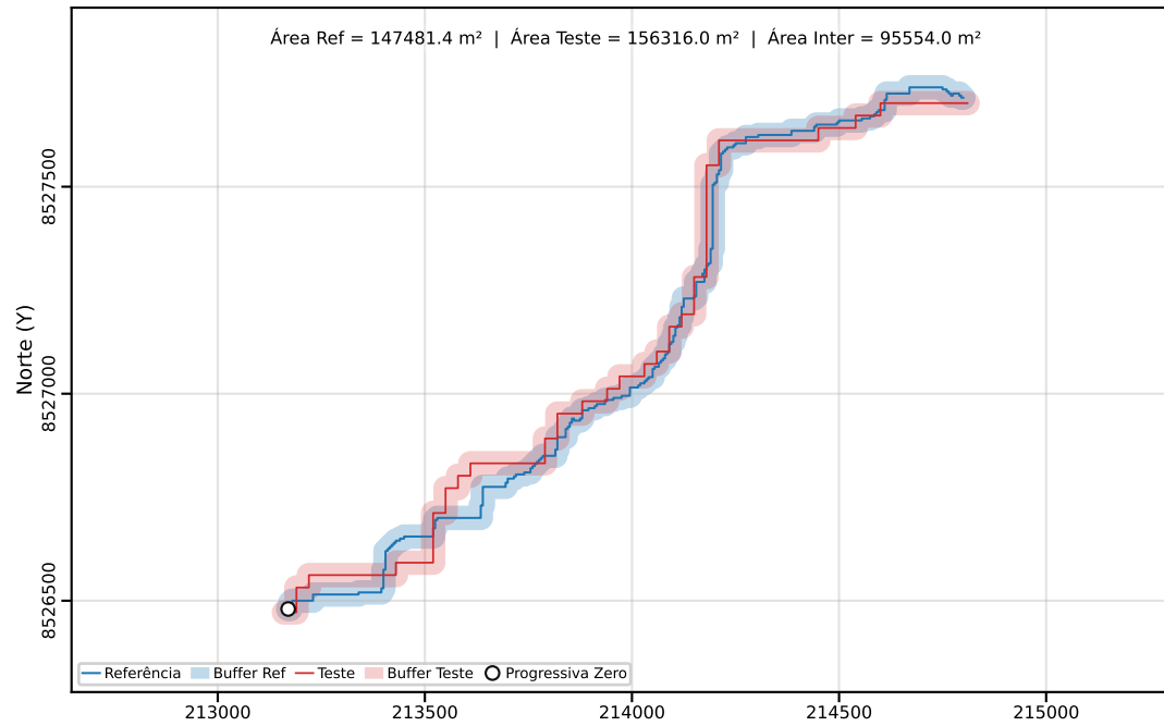
Classe C | PEC-PCD (Horizontal)=80.00 m | dm = 27.76
