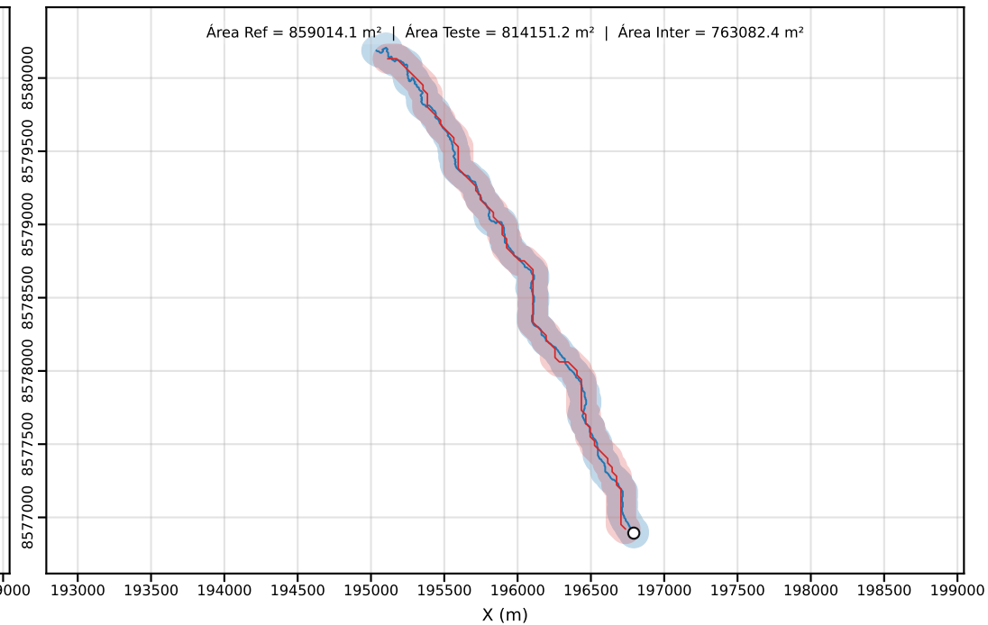
Classe D | PEC-PCD (Horizontal)=100.00 m | dm = 37.02
