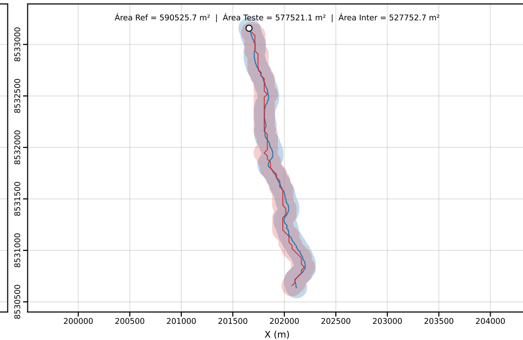
Classe D | PEC-PCD (Horizontal)=100.00 m | dm = 34.15
