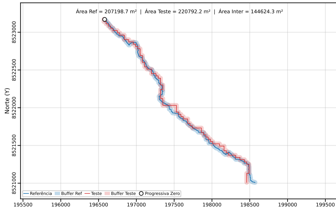
Classe C | PEC-PCD (Horizontal)=80.00 m | dm = 27.06
