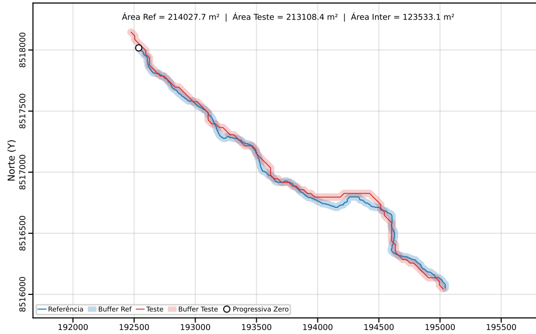
Classe C | PEC-PCD (Horizontal)=80.00 m | dm = 39.43
