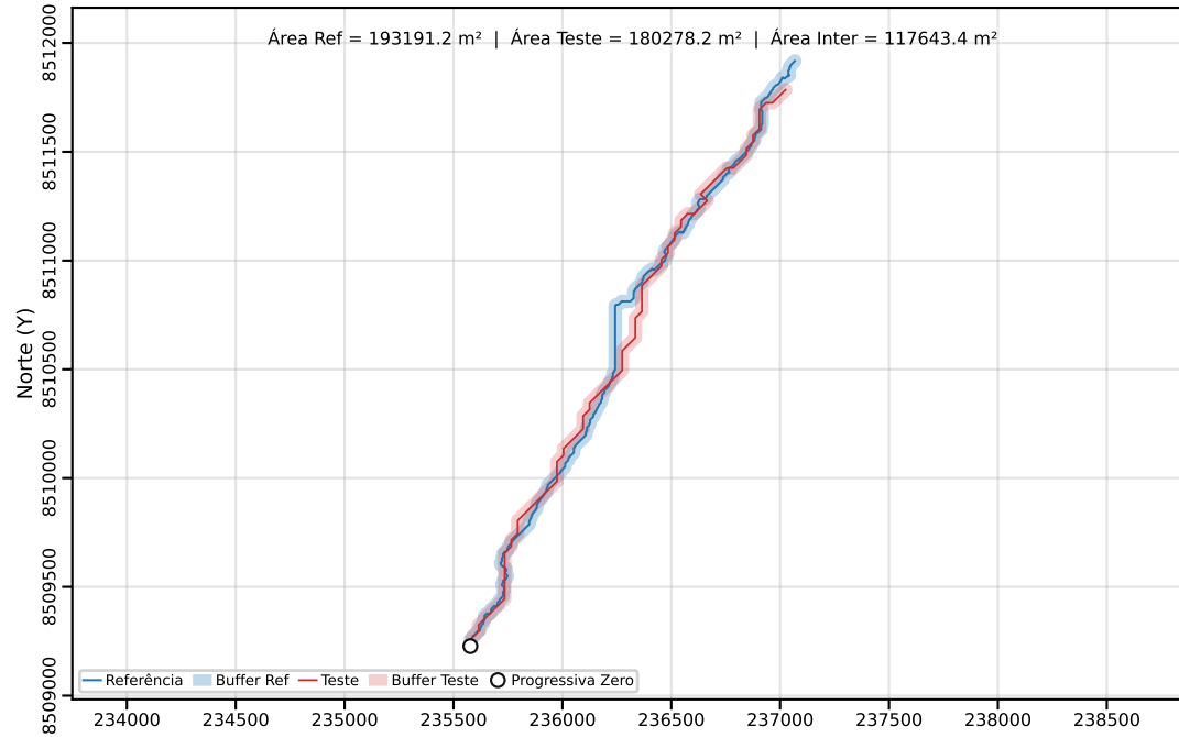
Classe C | PEC-PCD (Horizontal)=80.00 m | dm = 46.53
