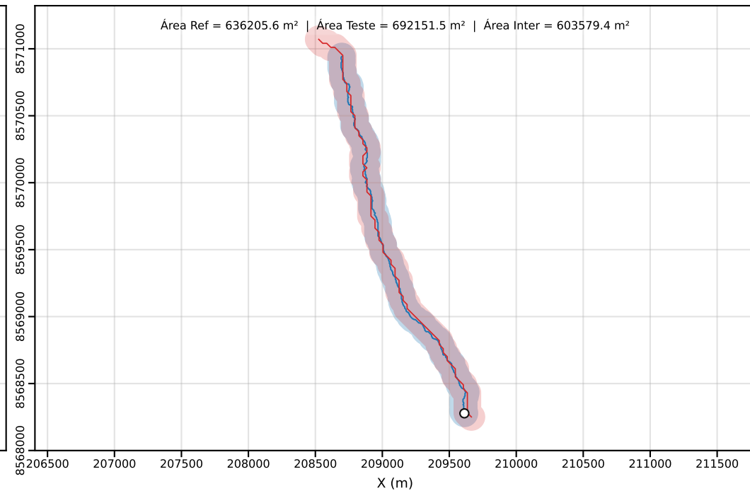
Classe D | PEC-PCD (Horizontal)=100.00 m | dm = 14.81
