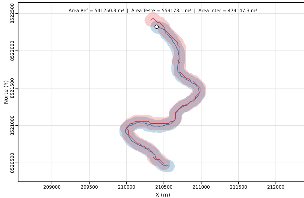
Classe C | PEC-PCD (Horizontal)=80.00 m | dm = 30.16
