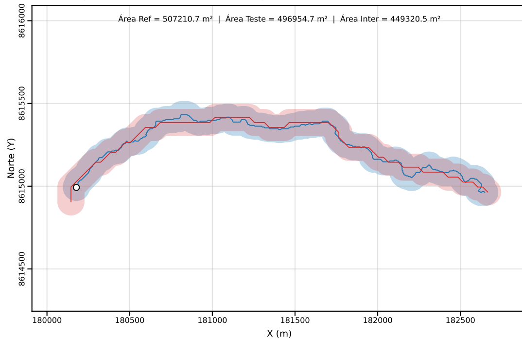
Classe C | PEC-PCD (Horizontal)=80.00 m | dm = 29.28
