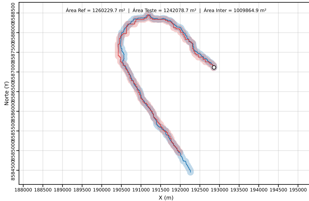
Classe C | PEC-PCD (Horizontal)=80.00 m | dm = 50.66
