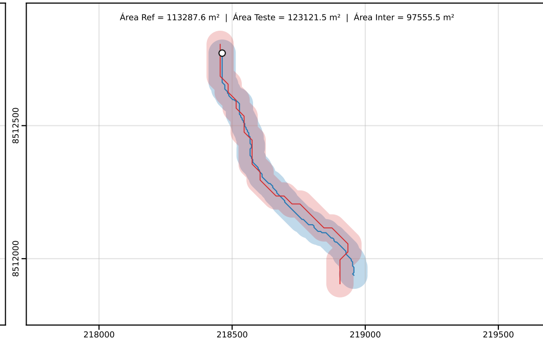
Classe D | PEC-PCD (Horizontal)=100.00 m | dm = 17.74
