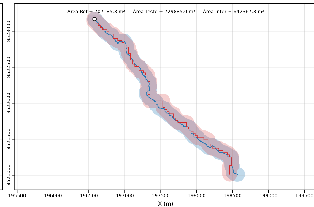
Classe D | PEC-PCD (Horizontal)=100.00 m | dm = 27.90
