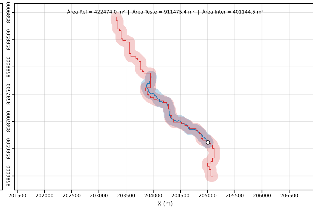
Classe D | PEC-PCD (Horizontal)=100.00 m | dm = 7.35
