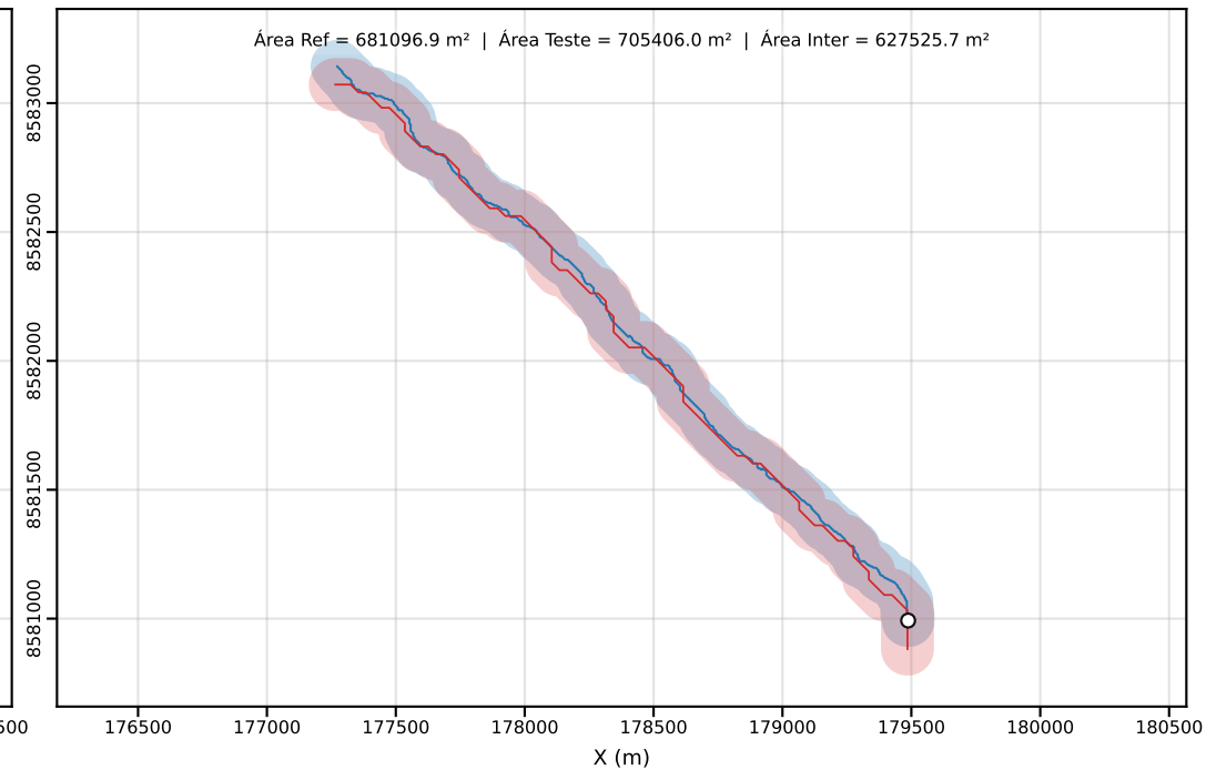
Classe D | PEC-PCD (Horizontal)=100.00 m | dm = 23.86
