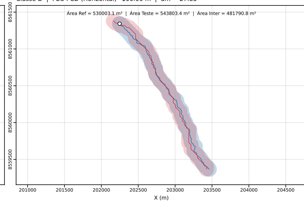
Classe D | PEC-PCD (Horizontal)=100.00 m | dm = 27.85
