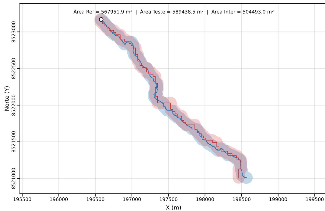
Classe C | PEC-PCD (Horizontal)=80.00 m | dm = 27.06
