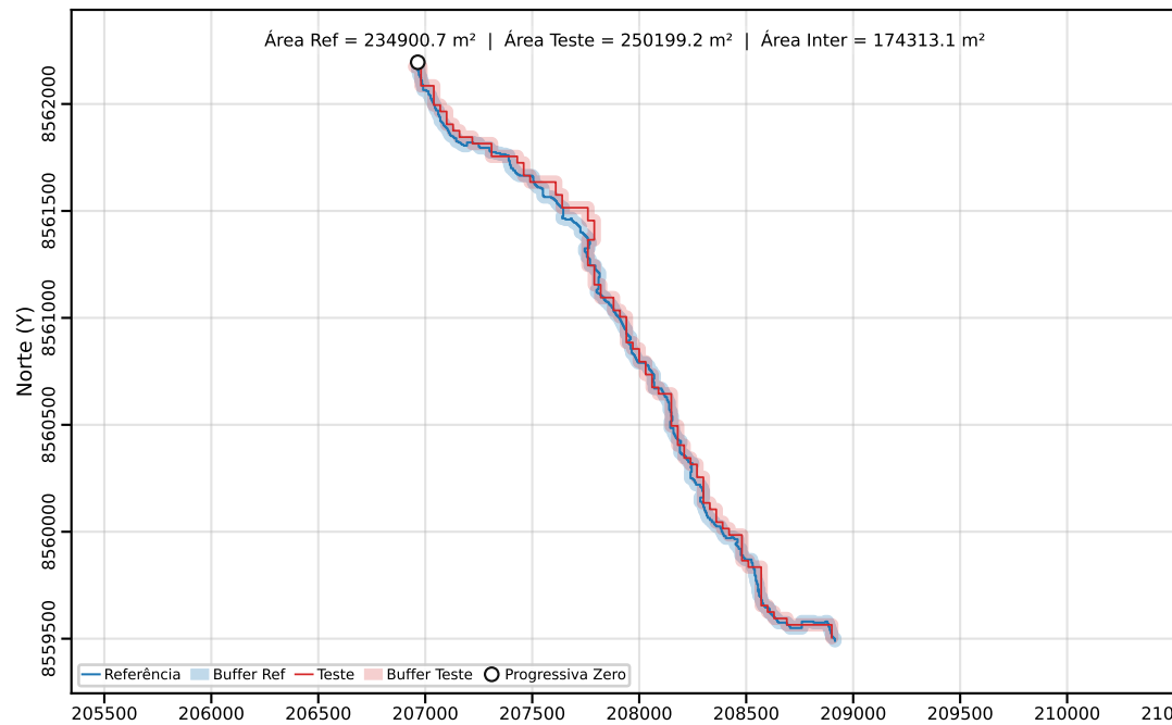
Classe C | PEC-PCD (Horizontal)=80.00 m | dm = 19.43
