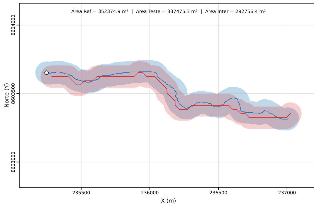
Classe C | PEC-PCD (Horizontal)=80.00 m | dm = 44.40
