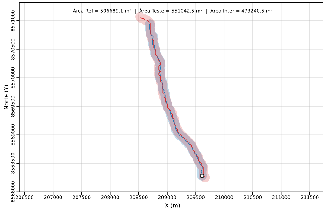
Classe C | PEC-PCD (Horizontal)=80.00 m | dm = 15.26
