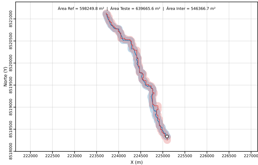
Classe C | PEC-PCD (Horizontal)=80.00 m | dm = 20.39
