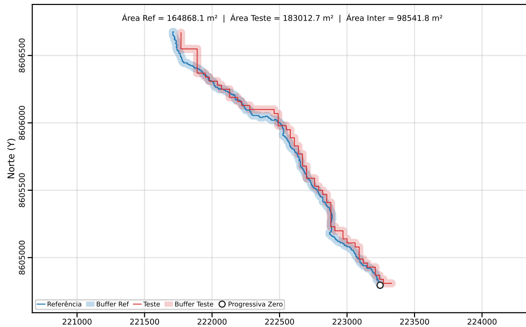
Classe C | PEC-PCD (Horizontal)=80.00 m | dm = 33.90
