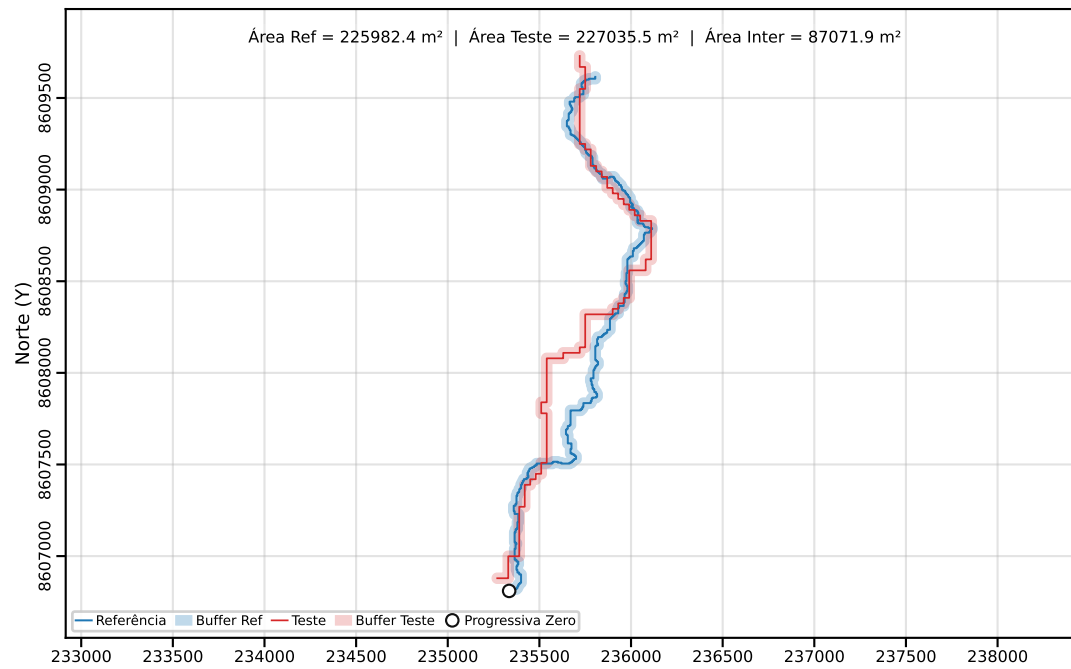
Classe C | PEC-PCD (Horizontal)=80.00 m | dm = 85.85
