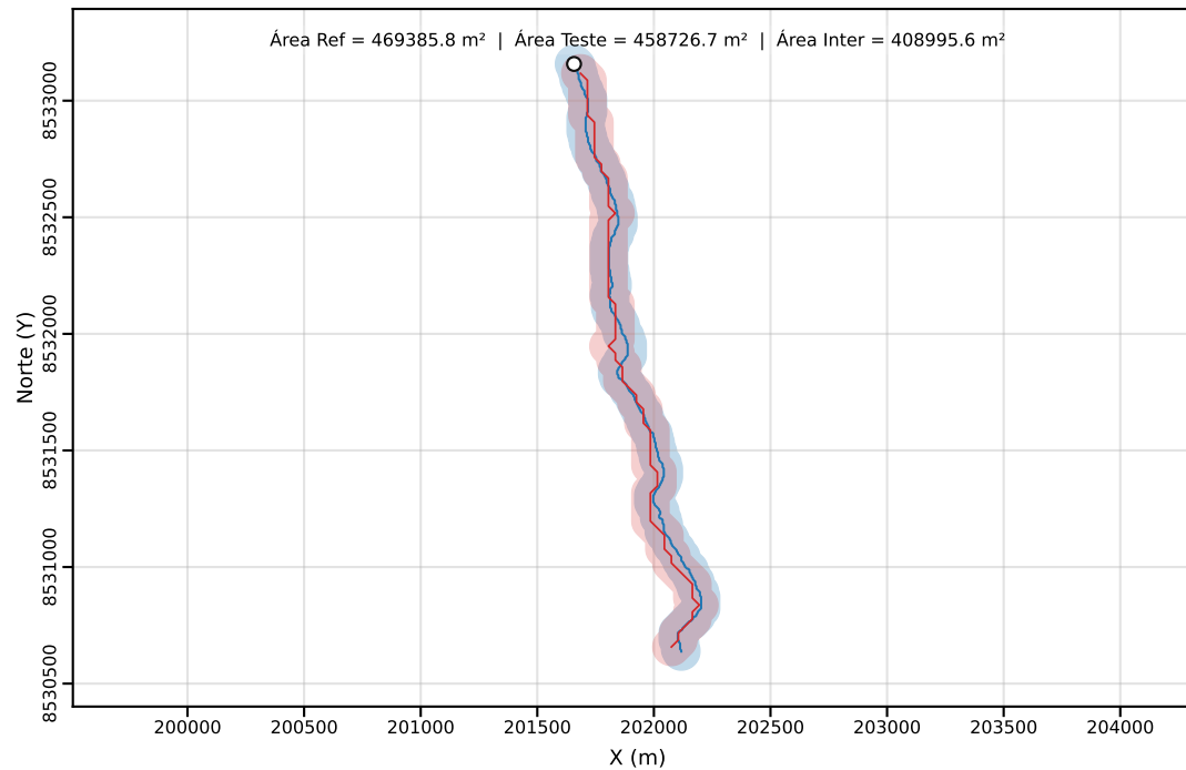
Classe C | PEC-PCD (Horizontal)=80.00 m | dm = 33.09
