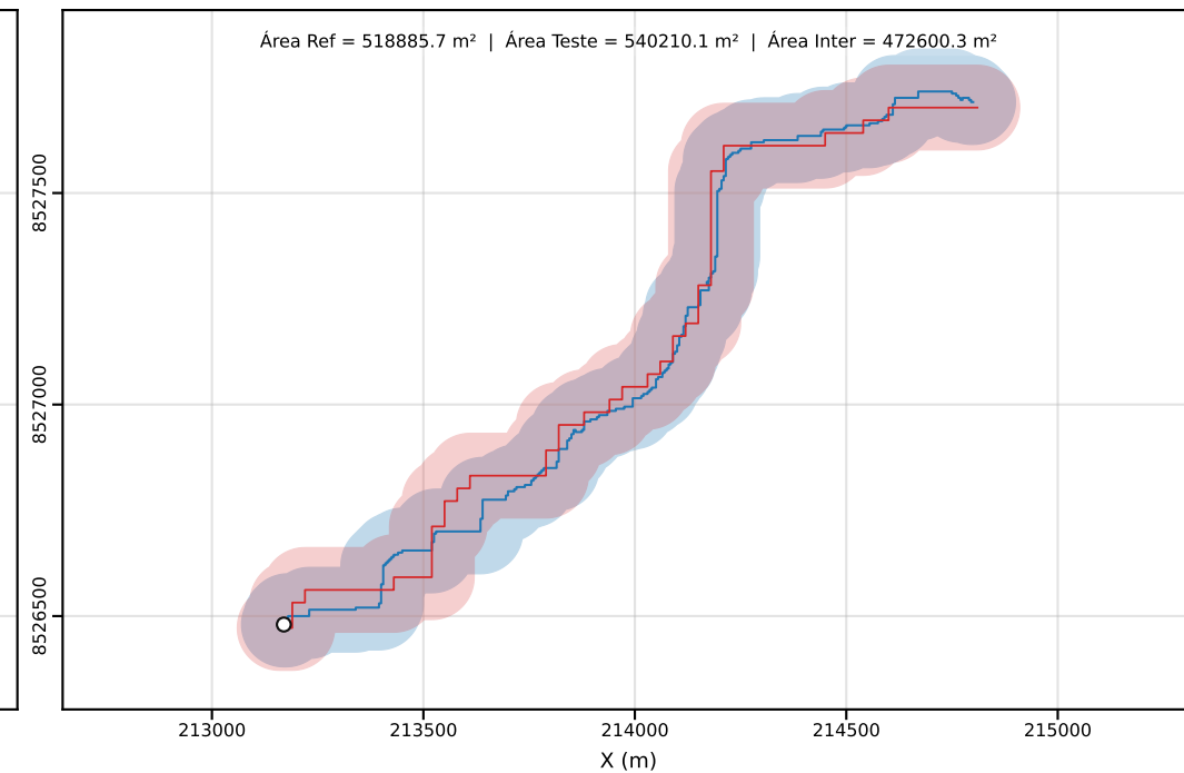
Classe D | PEC-PCD (Horizontal)=100.00 m | dm = 26.92
