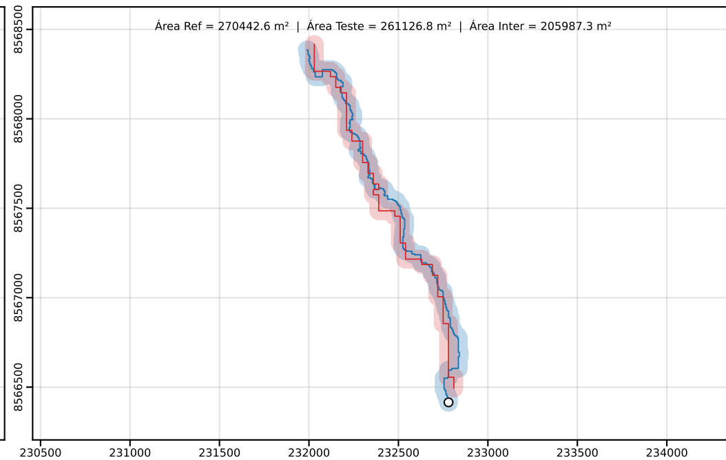
Classe D | PEC-PCD (Horizontal)=100.00 m | dm = 44.00
