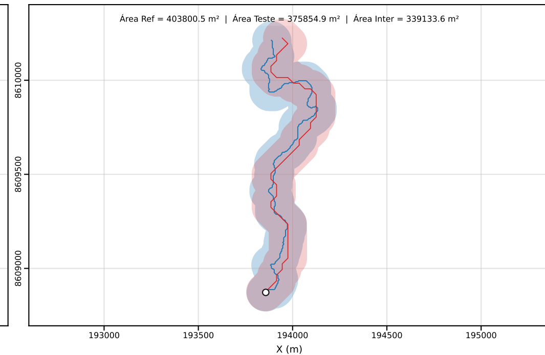
Classe D | PEC-PCD (Horizontal)=100.00 m | dm = 54.05
