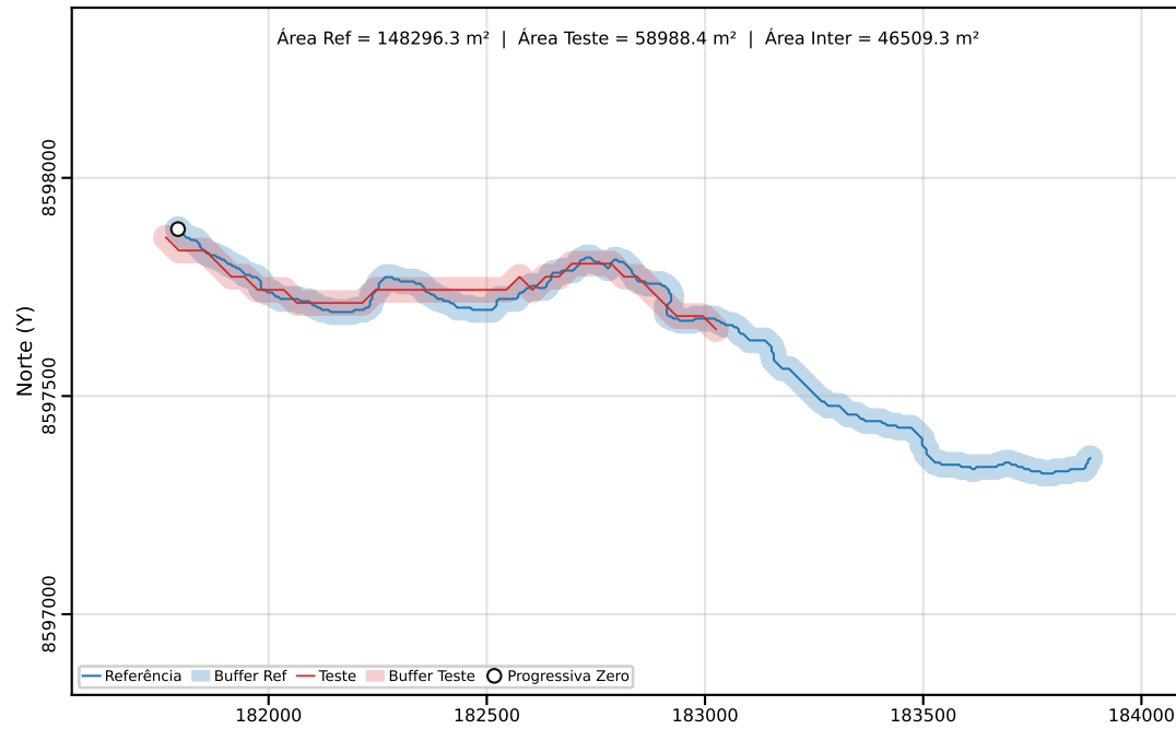
Classe C | PEC-PCD (Horizontal)=80.00 m | dm = 359.29
