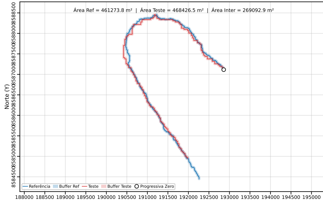
Classe C | PEC-PCD (Horizontal)=80.00 m | dm = 50.66
