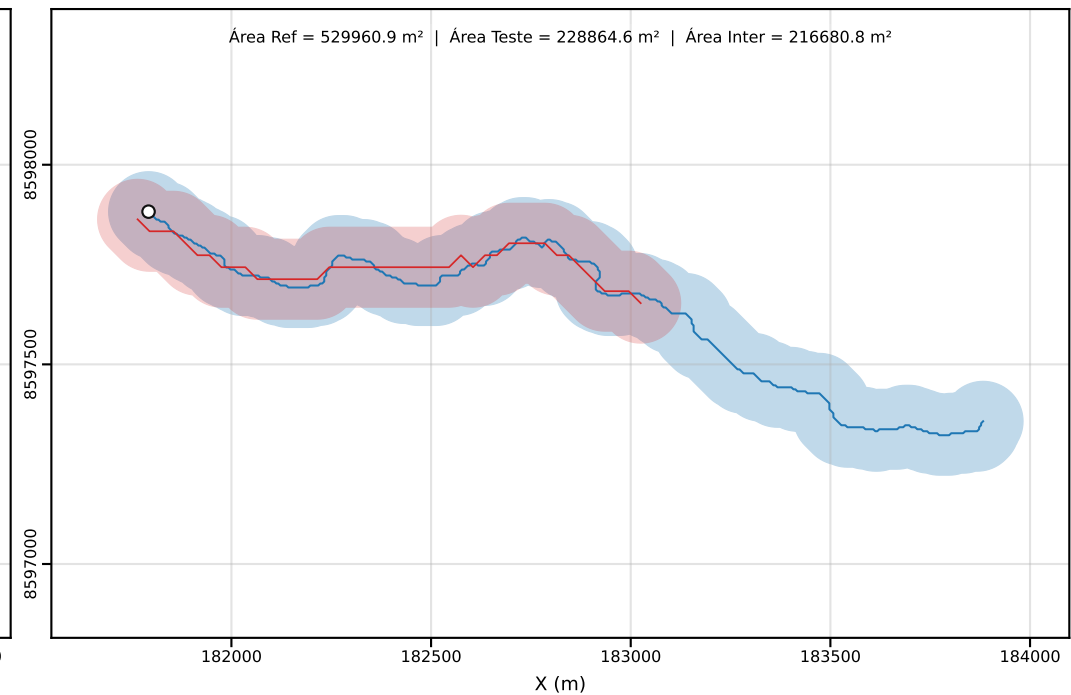
Classe D | PEC-PCD (Horizontal)=100.00 m | dm = 430.04
