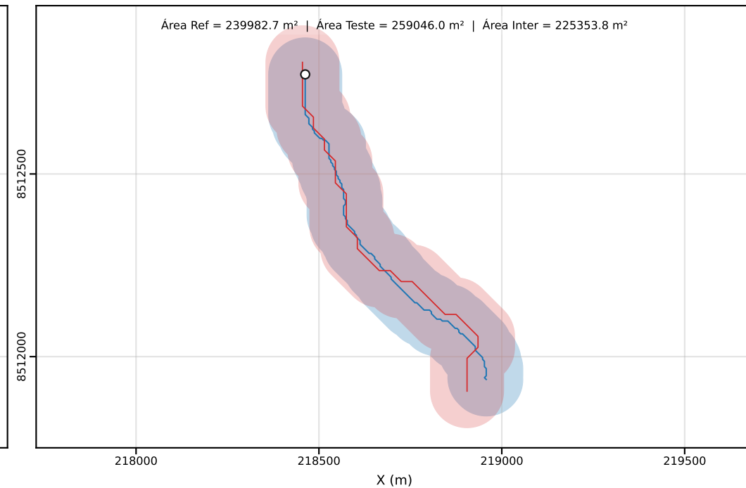
Classe D | PEC-PCD (Horizontal)=100.00 m | dm = 17.74
