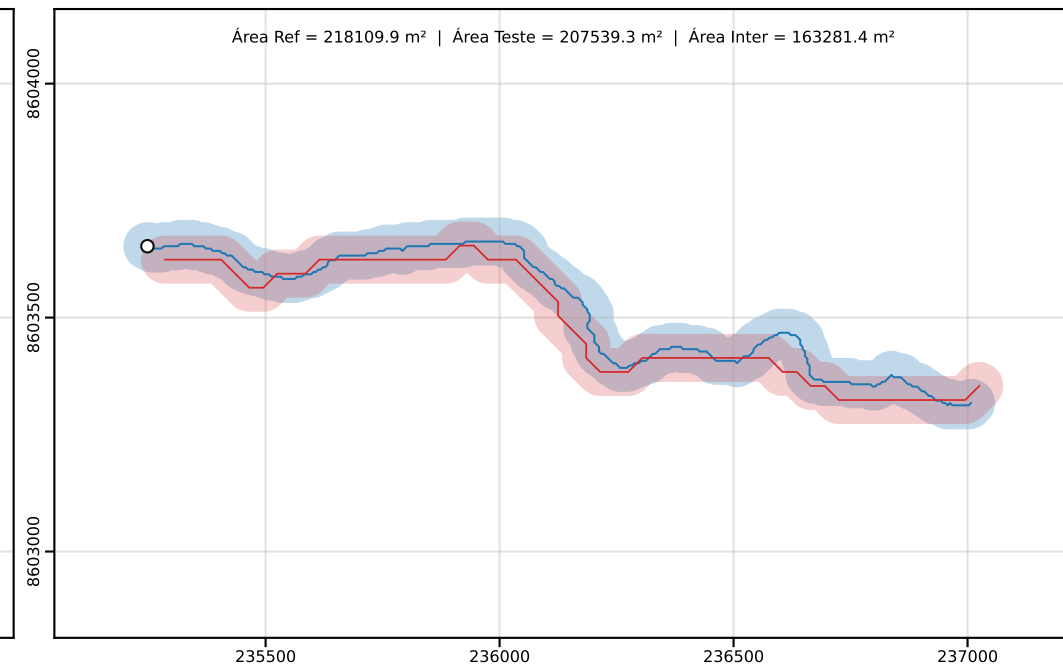
Classe D | PEC-PCD (Horizontal)=100.00 m | dm = 46.35
