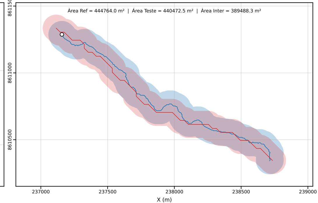
Classe D | PEC-PCD (Horizontal)=100.00 m | dm = 39.42
