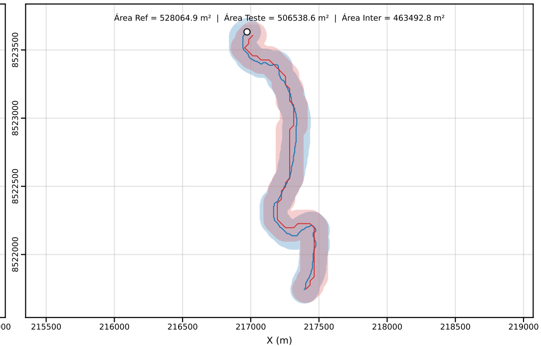
Classe D | PEC-PCD (Horizontal)=100.00 m | dm = 40.05
