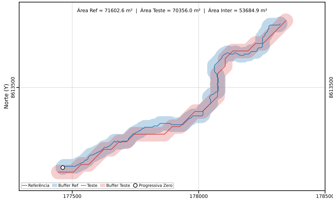
Classe C | PEC-PCD (Horizontal)=80.00 m | dm = 22.31
