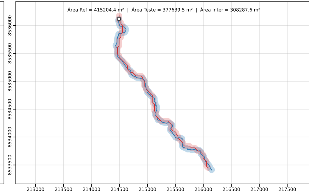
Classe D | PEC-PCD (Horizontal)=100.00 m | dm = 48.88
