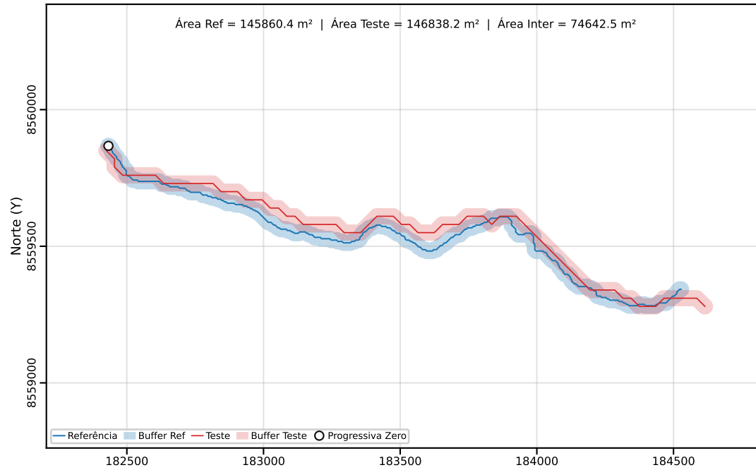
Classe C | PEC-PCD (Horizontal)=80.00 m | dm = 42.59
