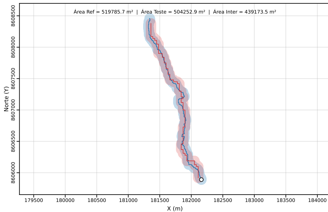
Classe C | PEC-PCD (Horizontal)=80.00 m | dm = 40.18
