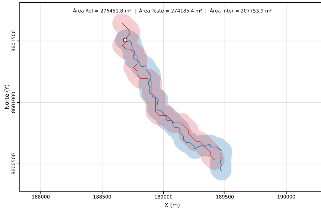
Classe C | PEC-PCD (Horizontal)=80.00 m | dm = 62.97
