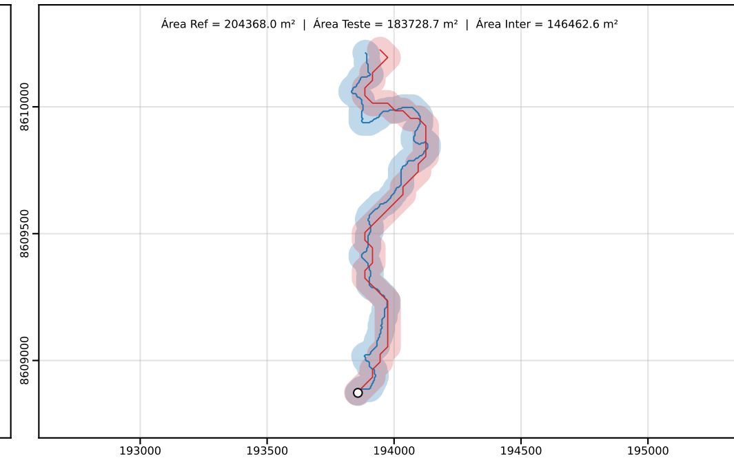
Classe D | PEC-PCD (Horizontal)=100.00 m | dm = 54.05
