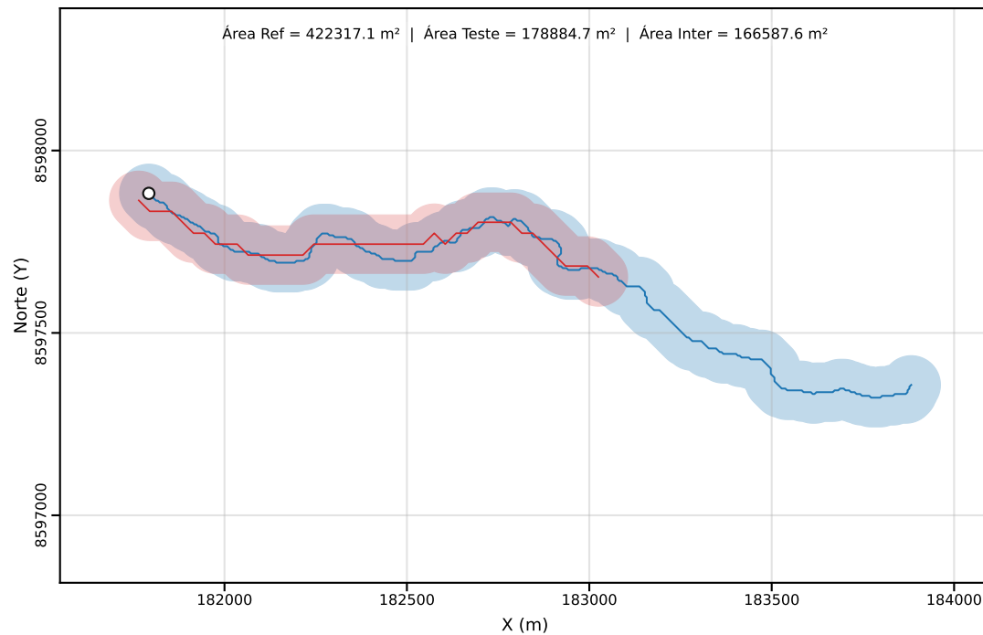
Classe C | PEC-PCD (Horizontal)=80.00 m | dm = 359.29
