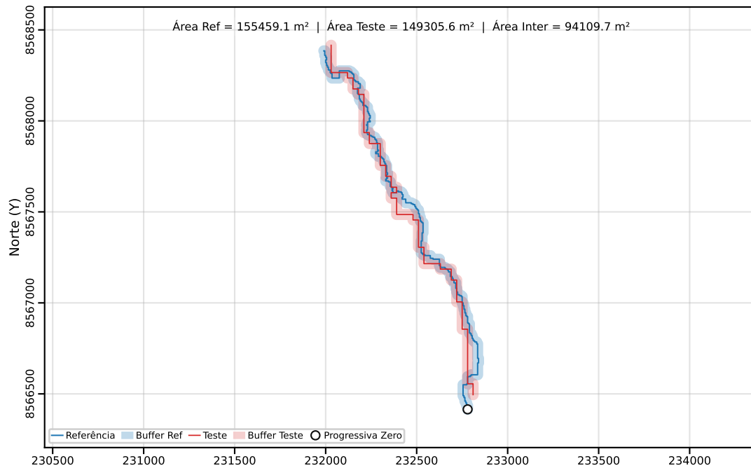
Classe C | PEC-PCD (Horizontal)=80.00 m | dm = 41.90
