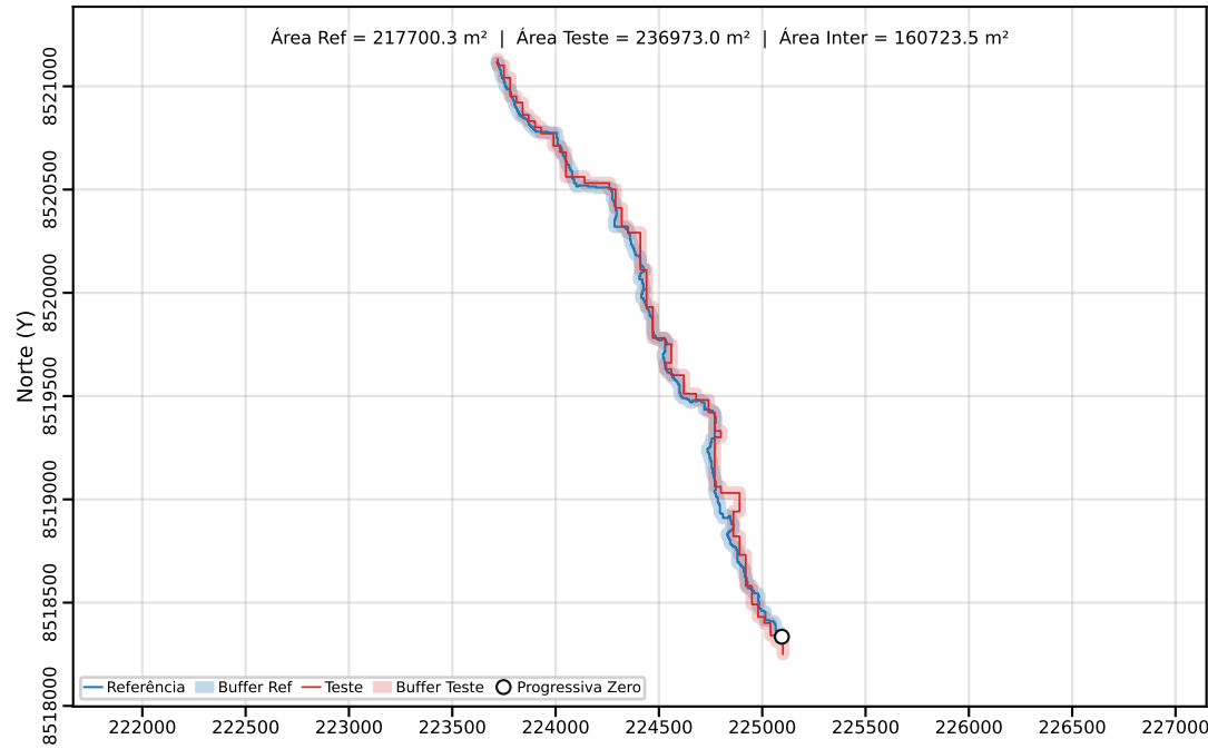
Classe C | PEC-PCD (Horizontal)=80.00 m | dm = 20.39
