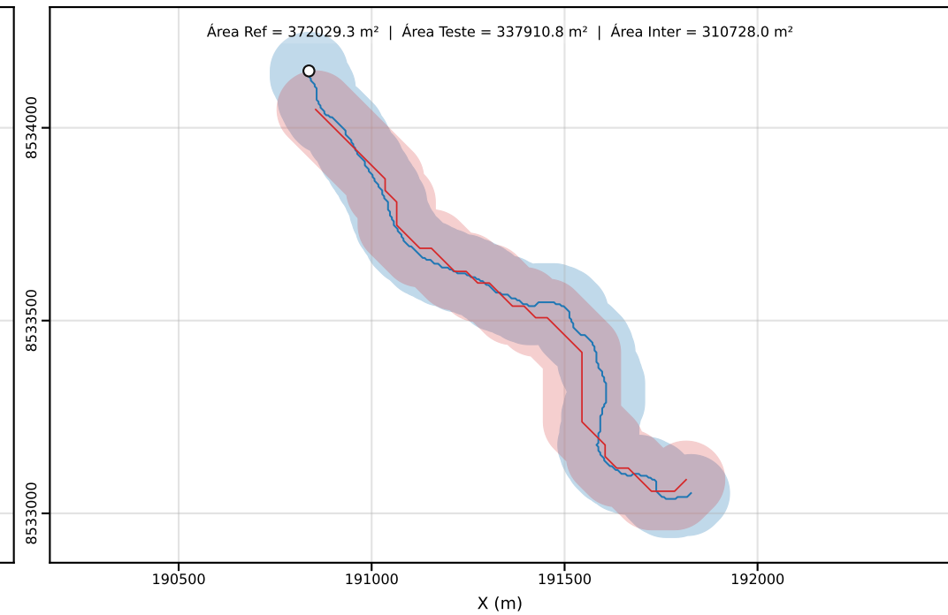
Classe D | PEC-PCD (Horizontal)=100.00 m | dm = 56.99
