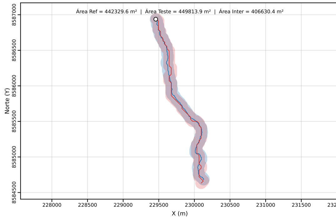
Classe C | PEC-PCD (Horizontal)=80.00 m | dm = 19.95
