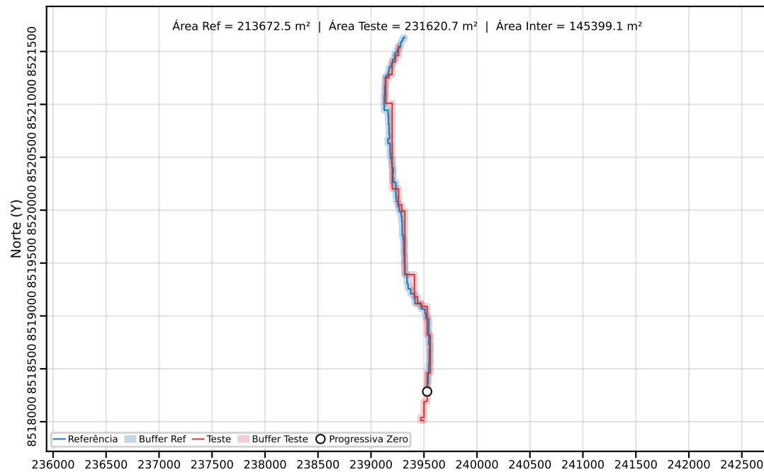
Classe C | PEC-PCD (Horizontal)=80.00 m | dm = 28.20
