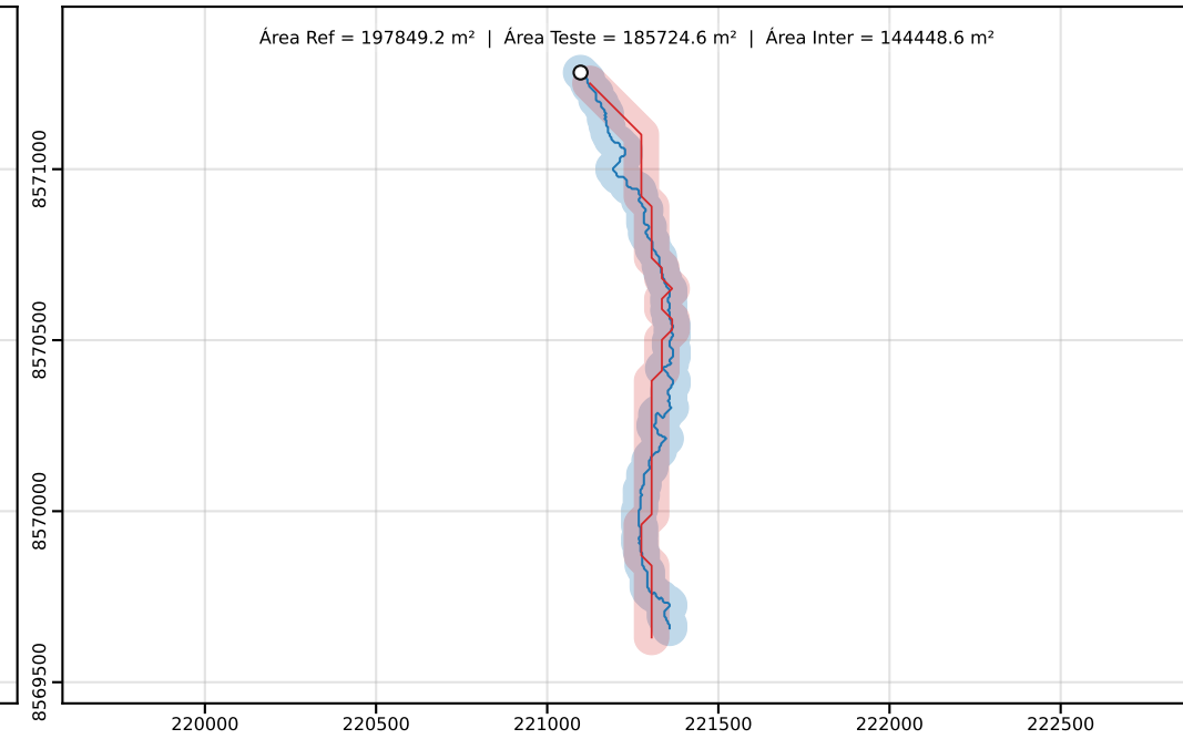
Classe D | PEC-PCD (Horizontal)=100.00 m | dm = 48.73
