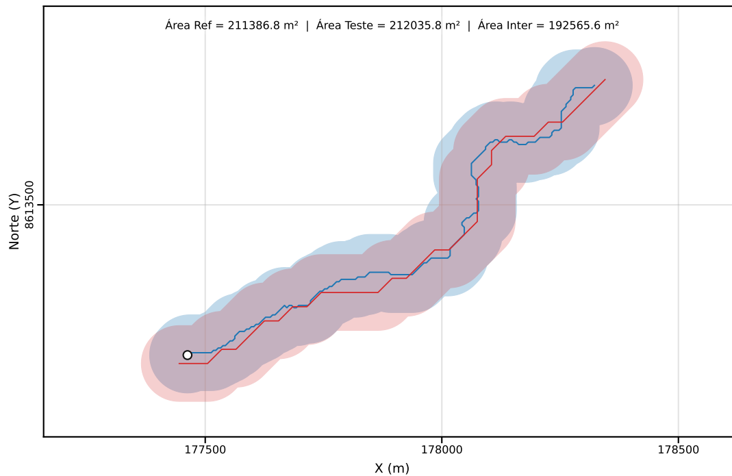
Classe C | PEC-PCD (Horizontal)=80.00 m | dm = 22.31
