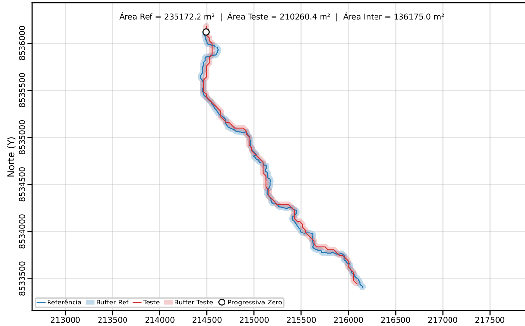
Classe C | PEC-PCD (Horizontal)=80.00 m | dm = 47.39
