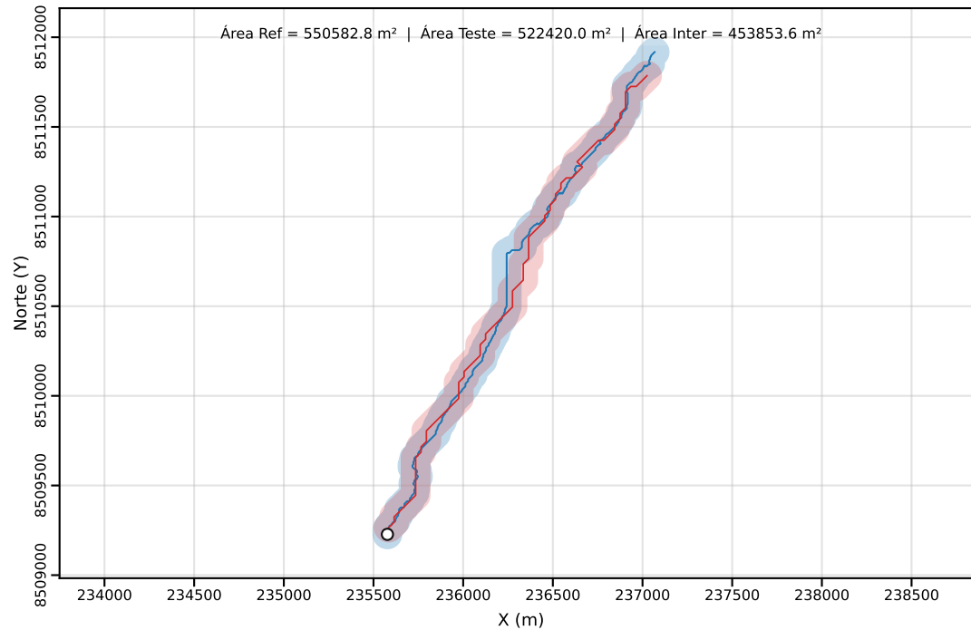
Classe C | PEC-PCD (Horizontal)=80.00 m | dm = 46.53
