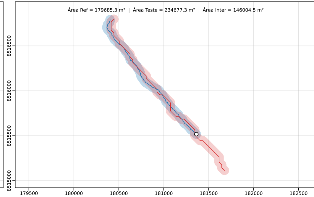
Classe D | PEC-PCD (Horizontal)=100.00 m | dm = 22.12
