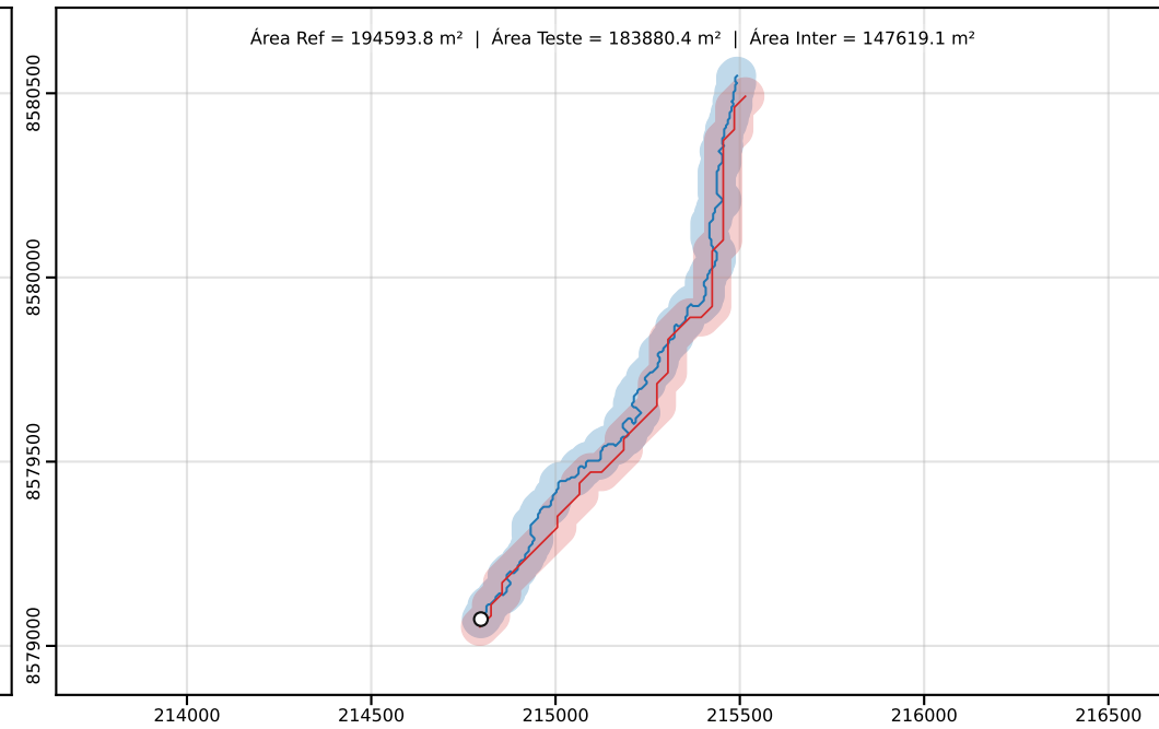
Classe D | PEC-PCD (Horizontal)=100.00 m | dm = 41.65
