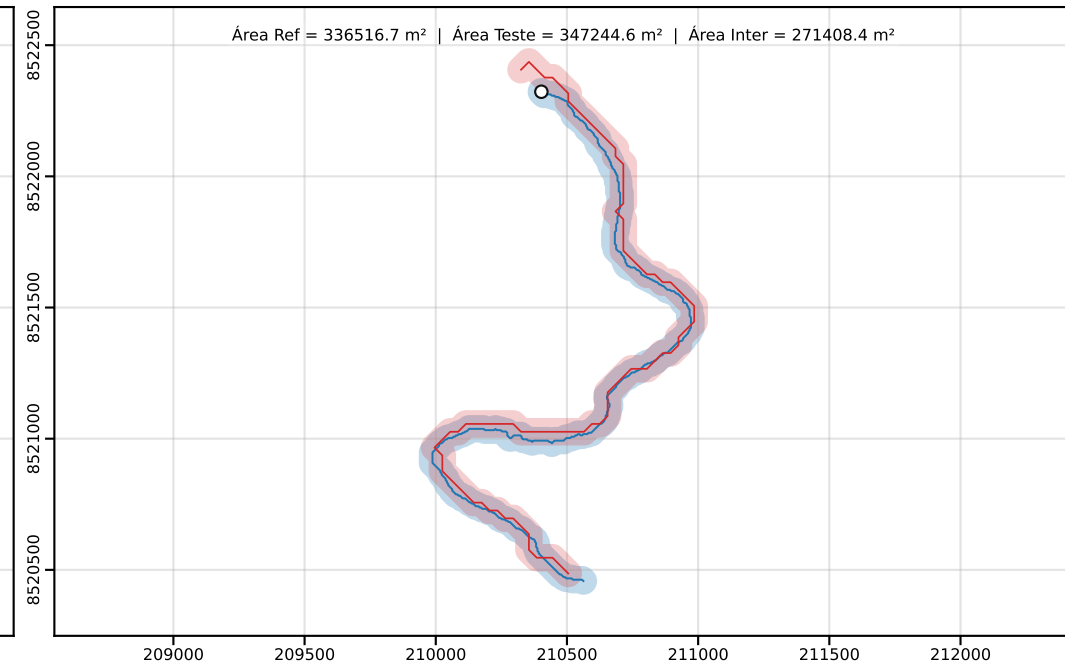
Classe D | PEC-PCD (Horizontal)=100.00 m | dm = 30.67
