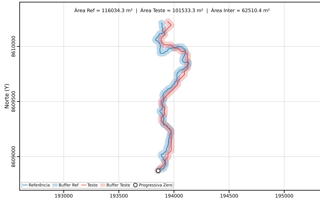
Classe C | PEC-PCD (Horizontal)=80.00 m | dm = 52.43
