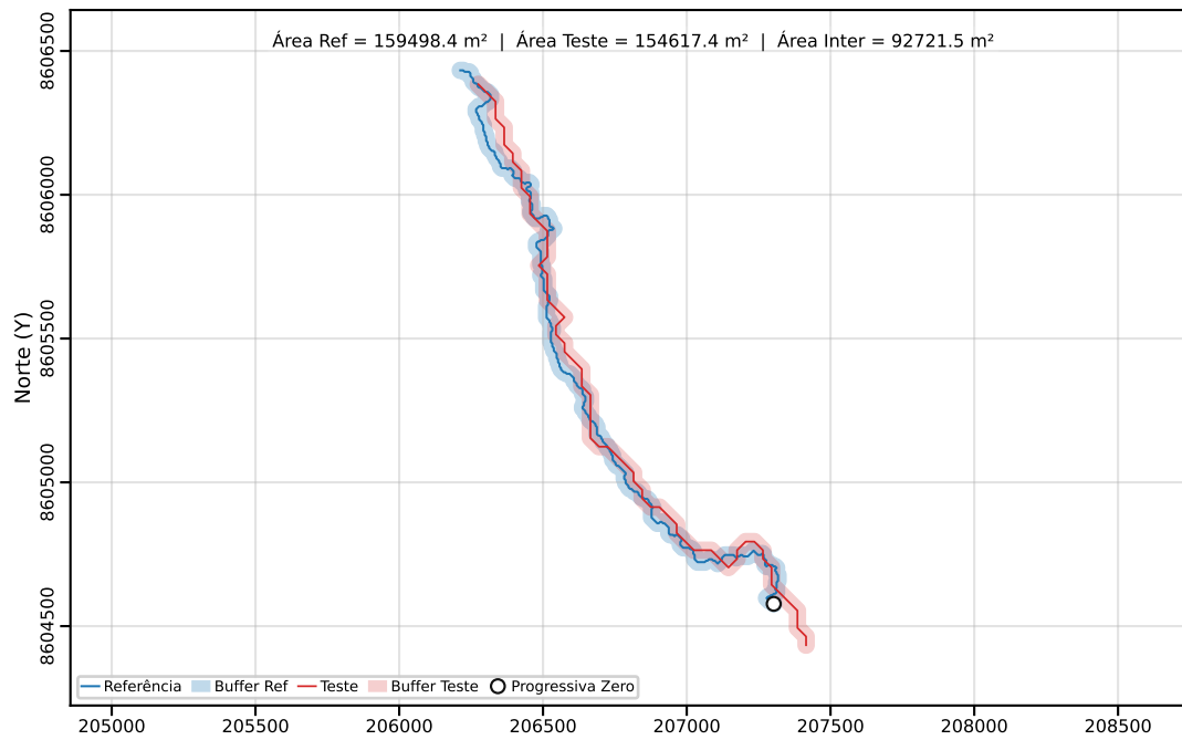
Classe C | PEC-PCD (Horizontal)=80.00 m | dm = 43.15
