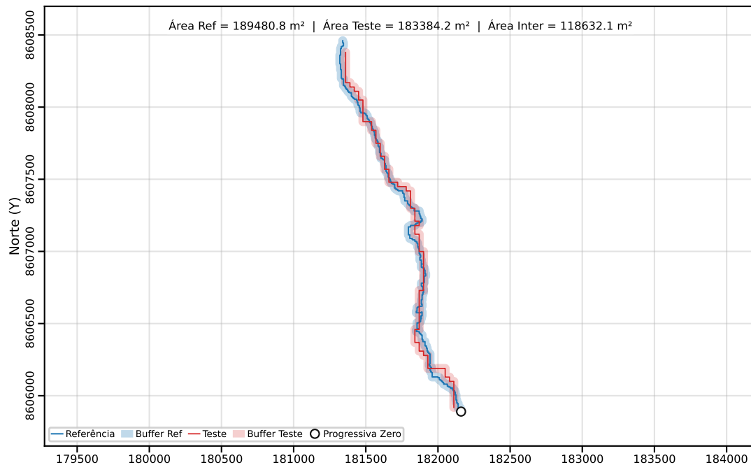
Classe C | PEC-PCD (Horizontal)=80.00 m | dm = 40.18
