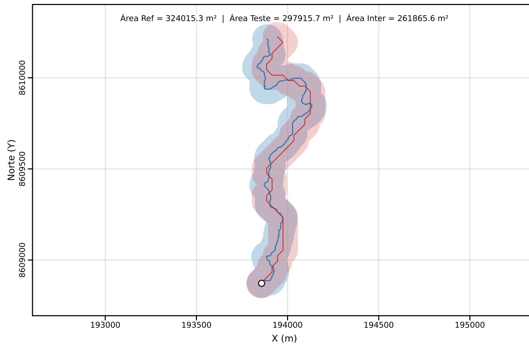
Classe C | PEC-PCD (Horizontal)=80.00 m | dm = 52.43
