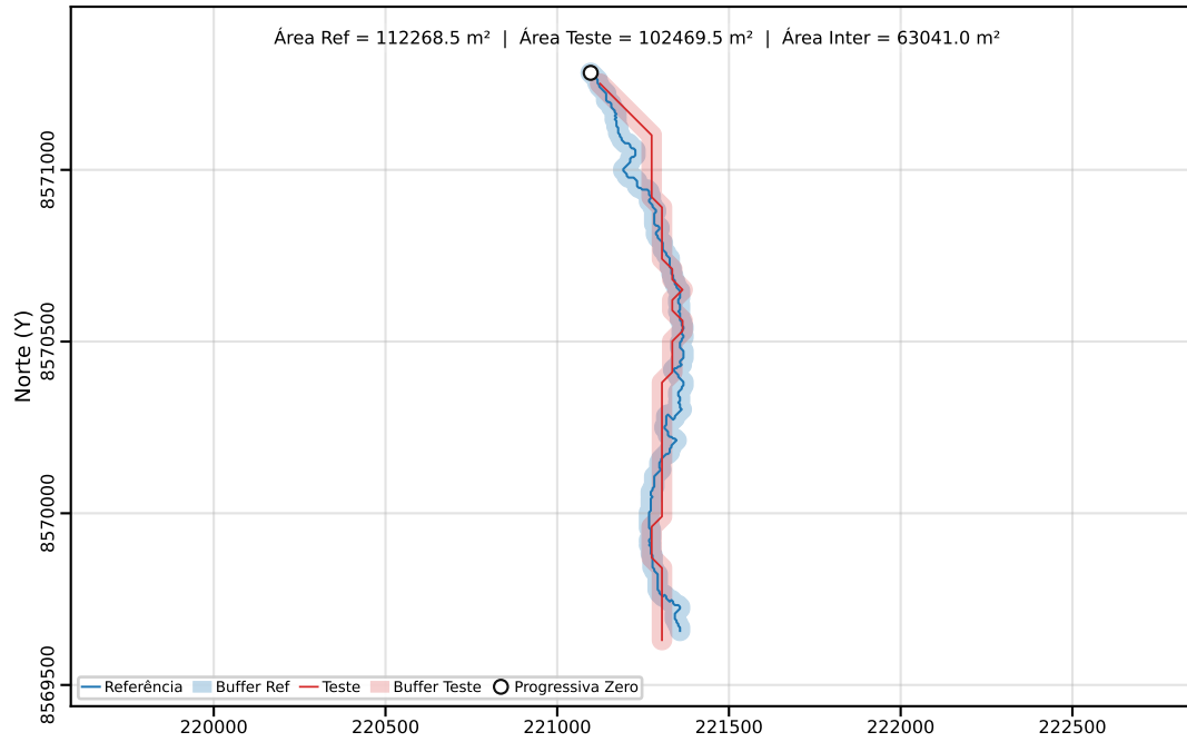
Classe C | PEC-PCD (Horizontal)=80.00 m | dm = 47.43
