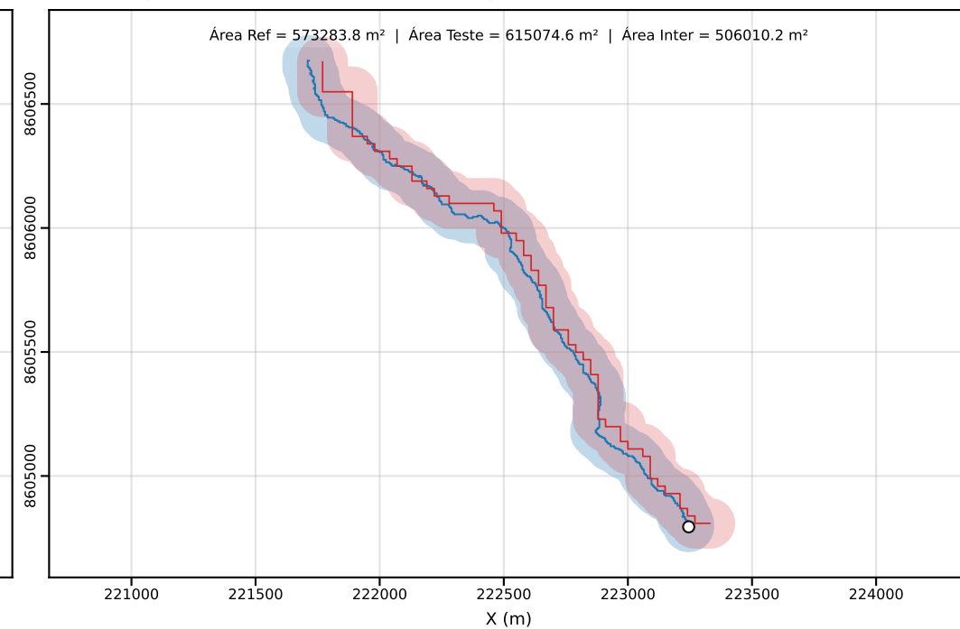
Classe D | PEC-PCD (Horizontal)=100.00 m | dm = 34.36
