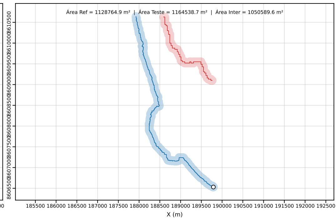
Classe D | PEC-PCD (Horizontal)=100.00 m | dm = 21.09
