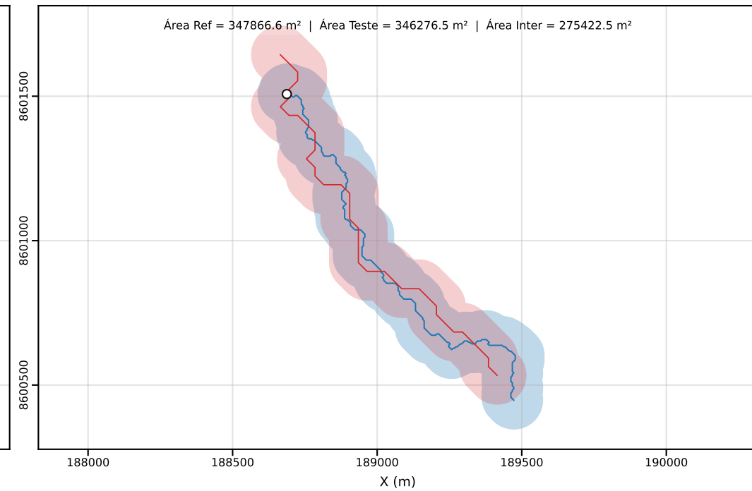
Classe D | PEC-PCD (Horizontal)=100.00 m | dm = 65.72
