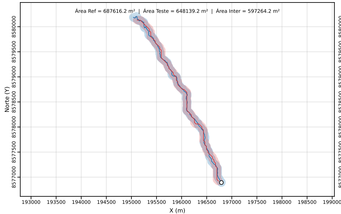
Classe C | PEC-PCD (Horizontal)=80.00 m | dm = 35.04
