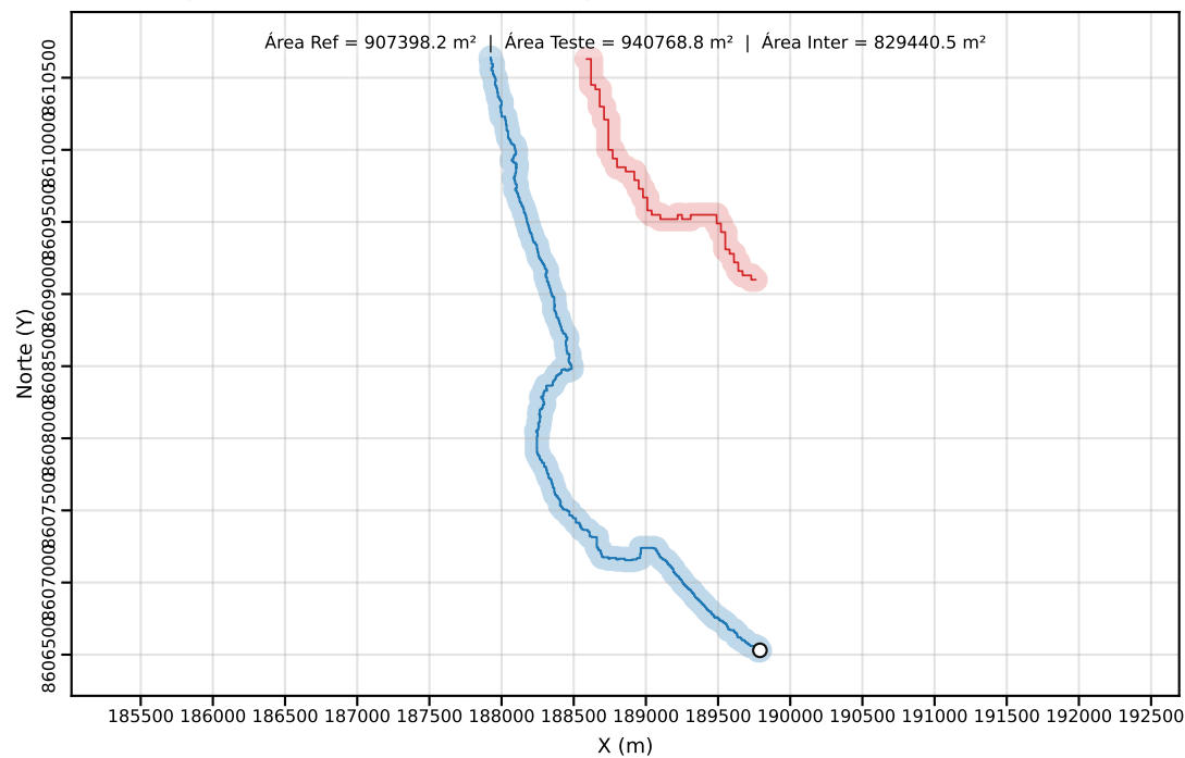
Classe C | PEC-PCD (Horizontal)=80.00 m | dm = 20.83
