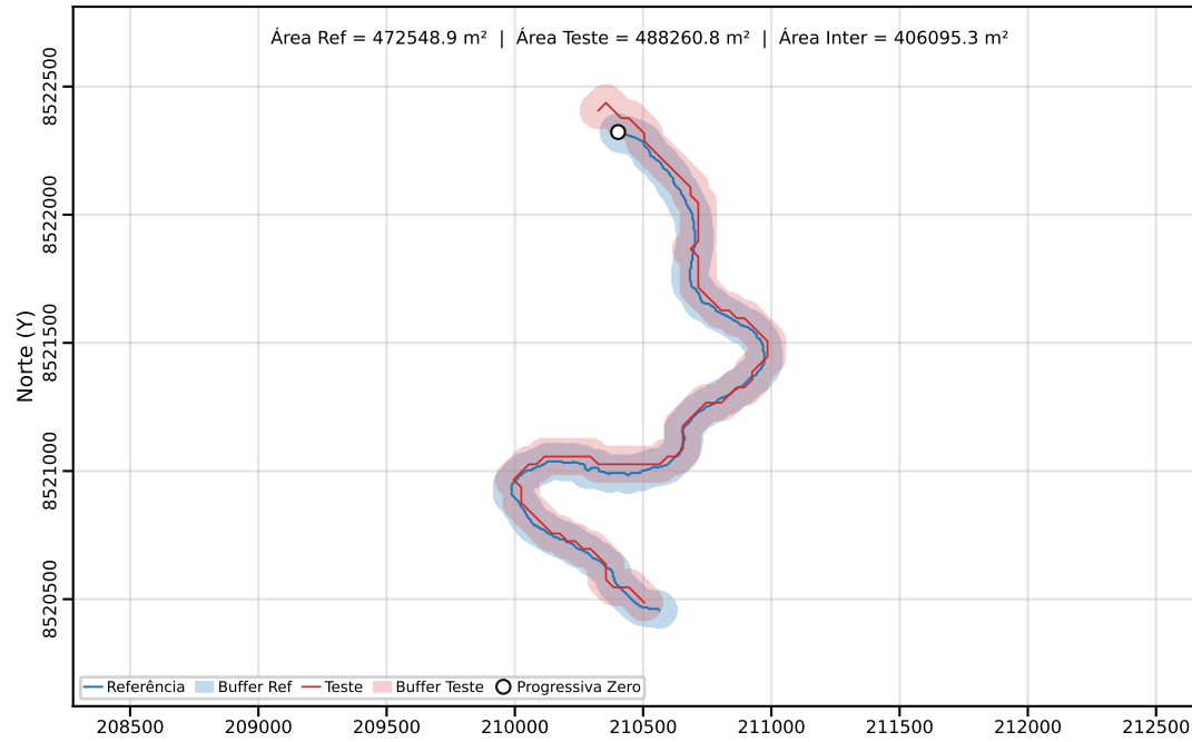
Classe C | PEC-PCD (Horizontal)=200.00 m | dm = 30.01
