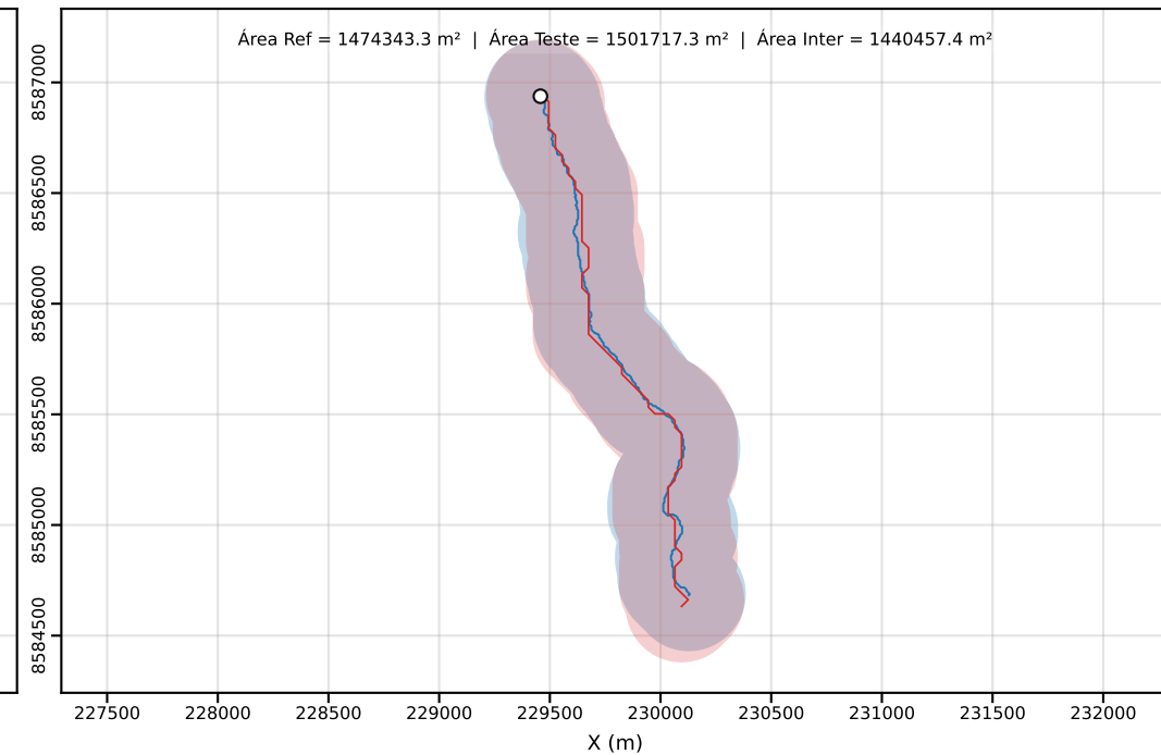
Classe D | PEC-PCD (Horizontal)=250.00 m | dm = 17.72
