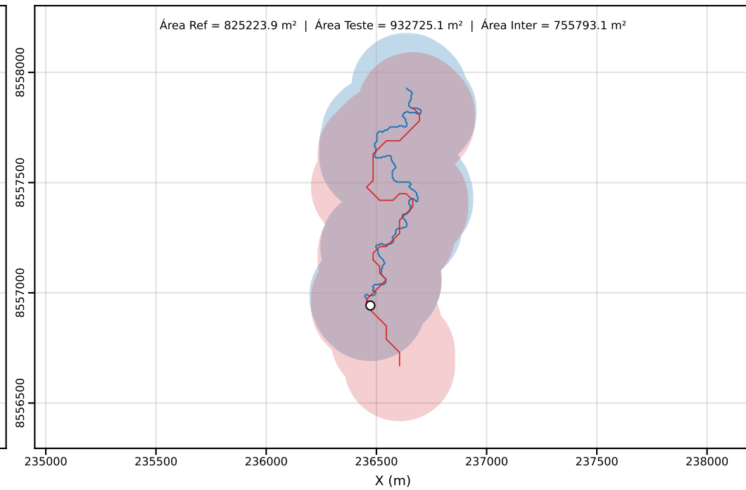
Classe D | PEC-PCD (Horizontal)=250.00 m | dm = 58.46
