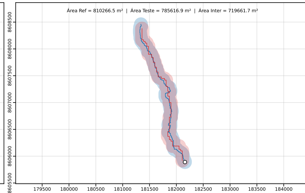
Classe D | PEC-PCD (Horizontal)=250.00 m | dm = 57.47
