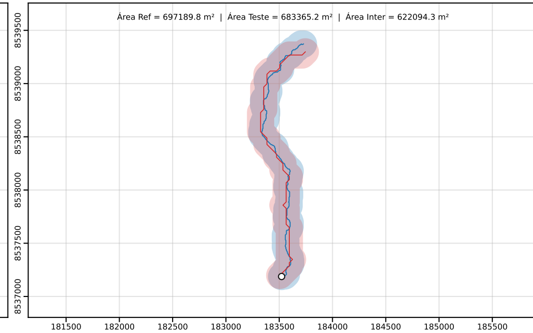
Classe D | PEC-PCD (Horizontal)=250.00 m | dm = 47.32
