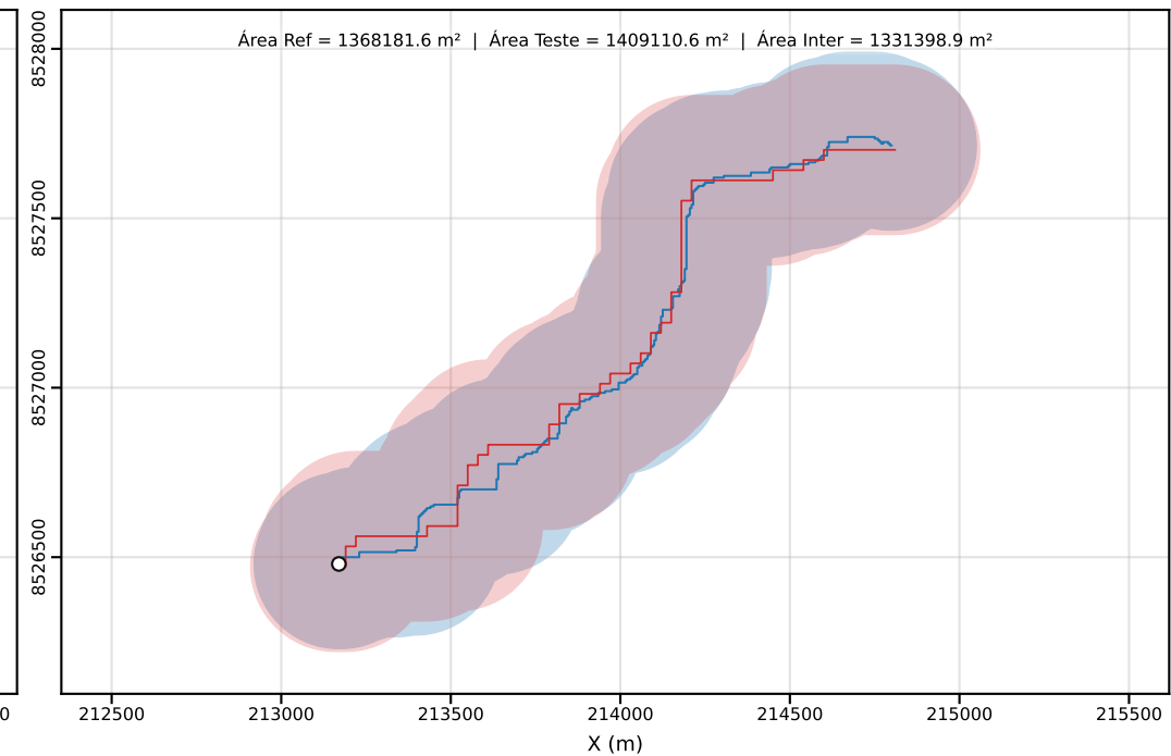
Classe D | PEC-PCD (Horizontal)=250.00 m | dm = 20.50
