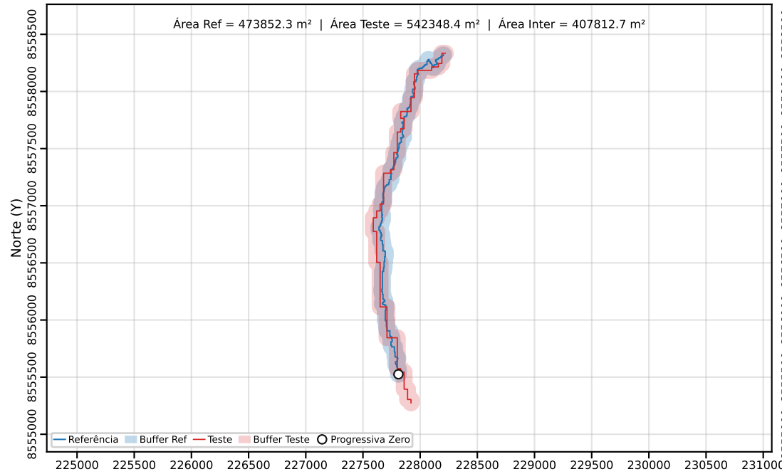
Classe C | PEC-PCD (Horizontal)=200.00 m | dm = 20.70
