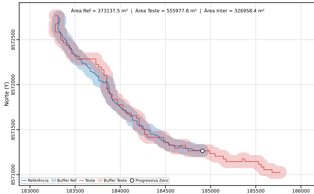
Classe C | PEC-PCD (Horizontal)=200.00 m | dm = 12.71
