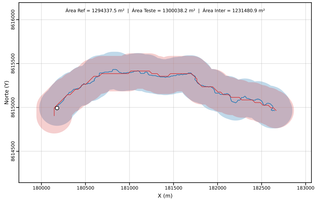
Classe C | PEC-PCD (Horizontal)=200.00 m | dm = 30.38
