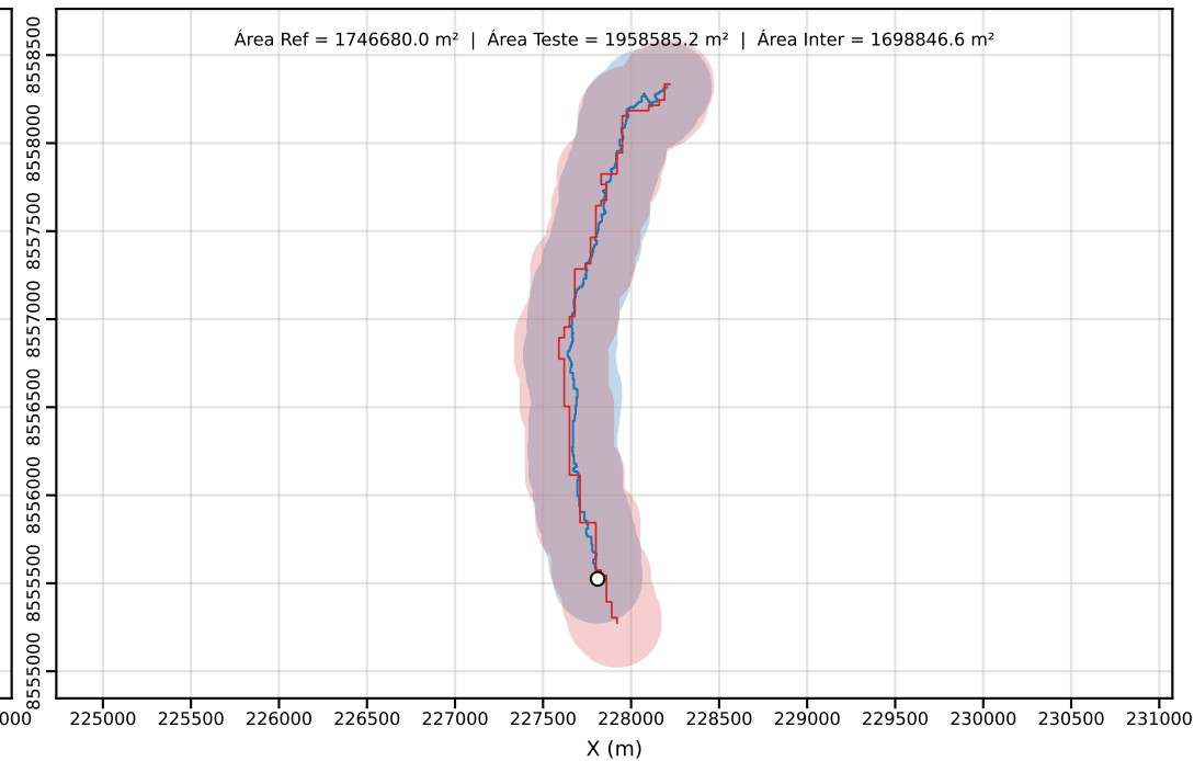
Classe D | PEC-PCD (Horizontal)=250.00 m | dm = 19.18
