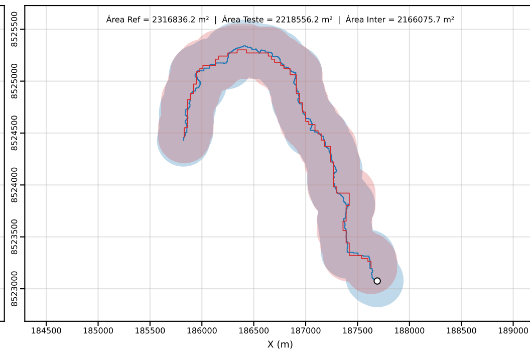
Classe D | PEC-PCD (Horizontal)=250.00 m | dm = 53.37
