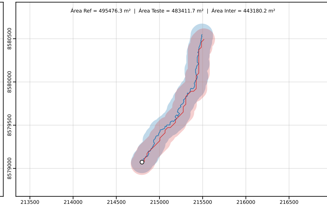
Classe D | PEC-PCD (Horizontal)=250.00 m | dm = 47.17
