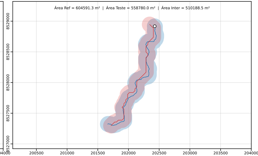
Classe D | PEC-PCD (Horizontal)=250.00 m | dm = 80.80
