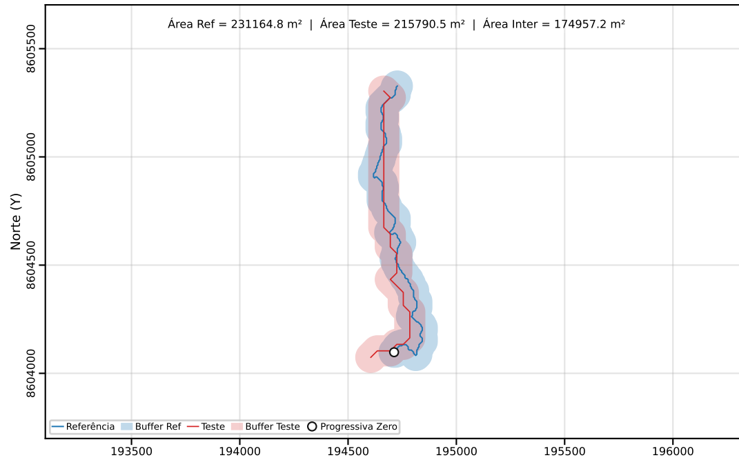
Classe C | PEC-PCD (Horizontal)=200.00 m | dm = 79.55
