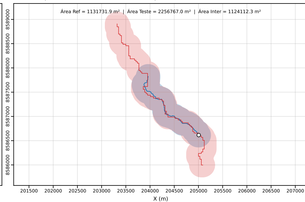
Classe D | PEC-PCD (Horizontal)=250.00 m | dm = 2.65
