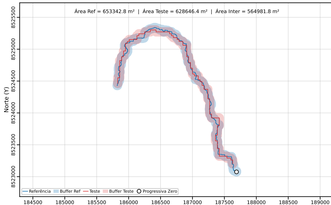
Classe C | PEC-PCD (Horizontal)=200.00 m | dm = 47.37
