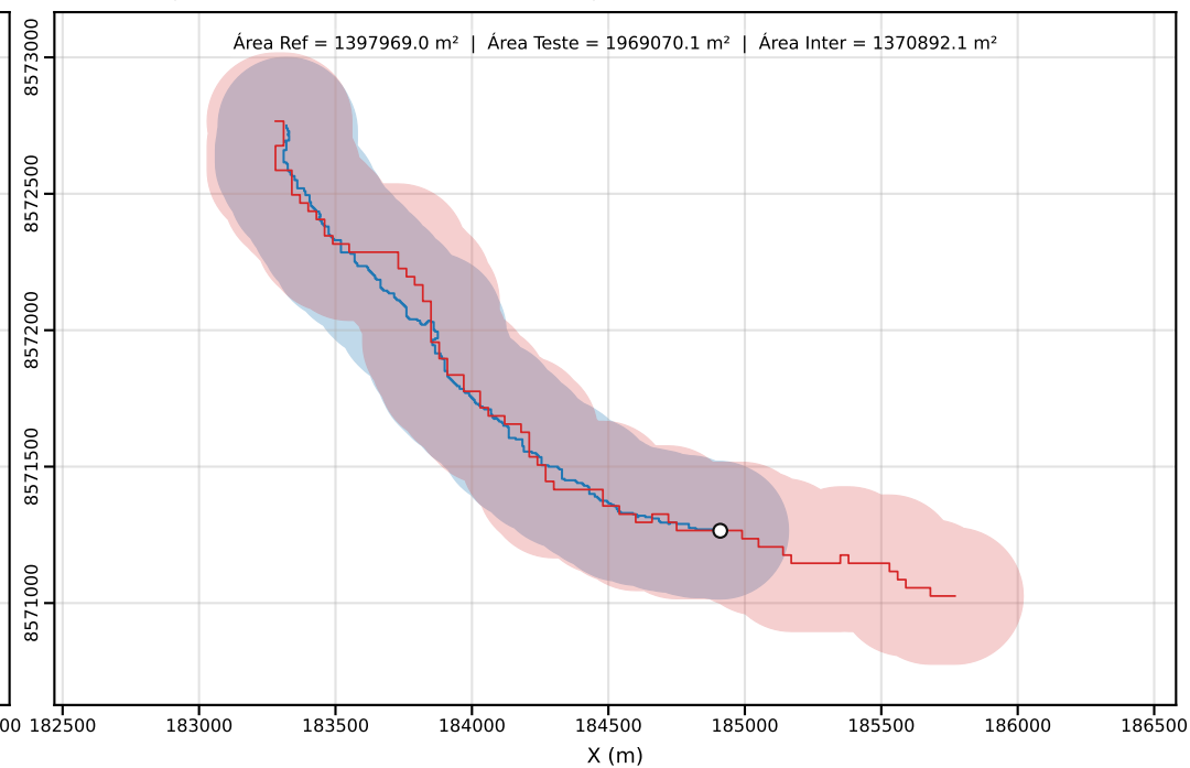
Classe D | PEC-PCD (Horizontal)=250.00 m | dm = 10.80
