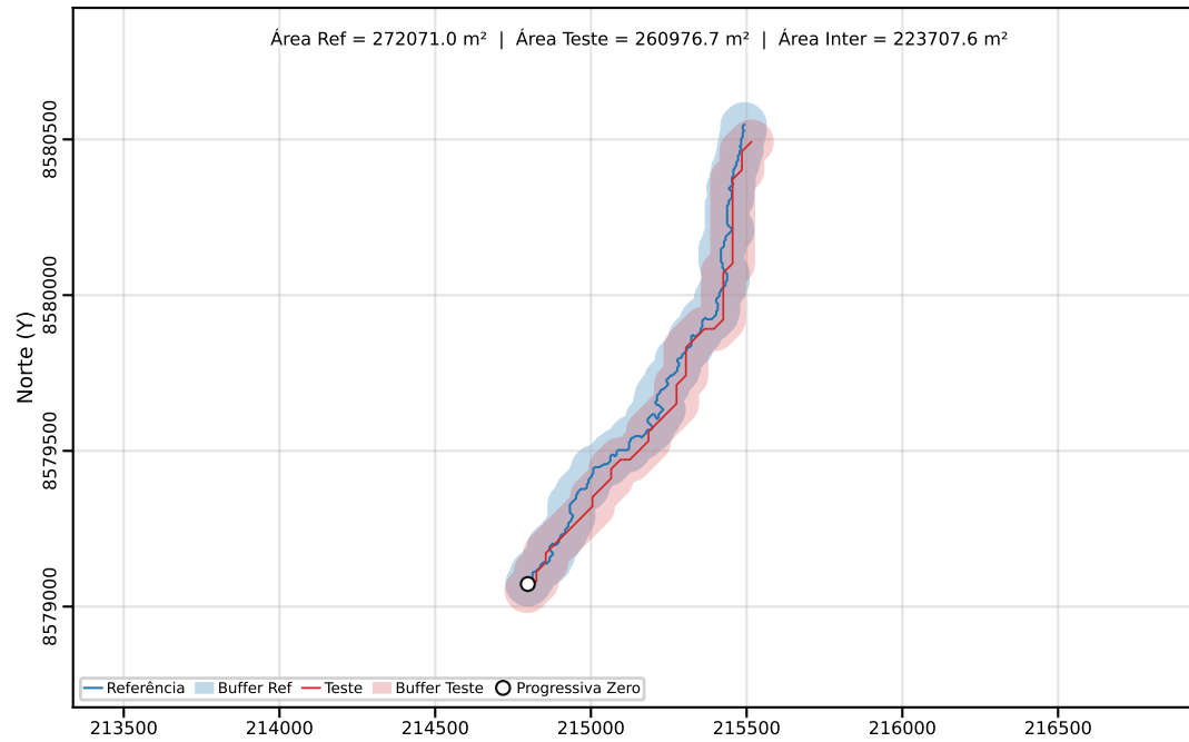
Classe C | PEC-PCD (Horizontal)=200.00 m | dm = 45.33
