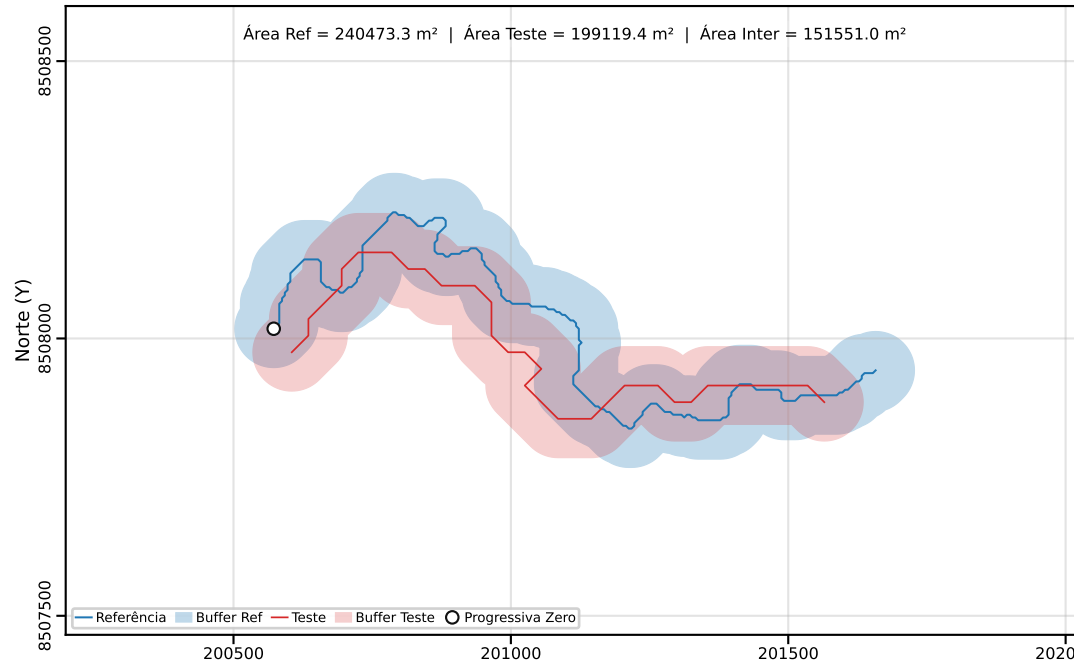
Classe C | PEC-PCD (Horizontal)=200.00 m | dm = 130.76
