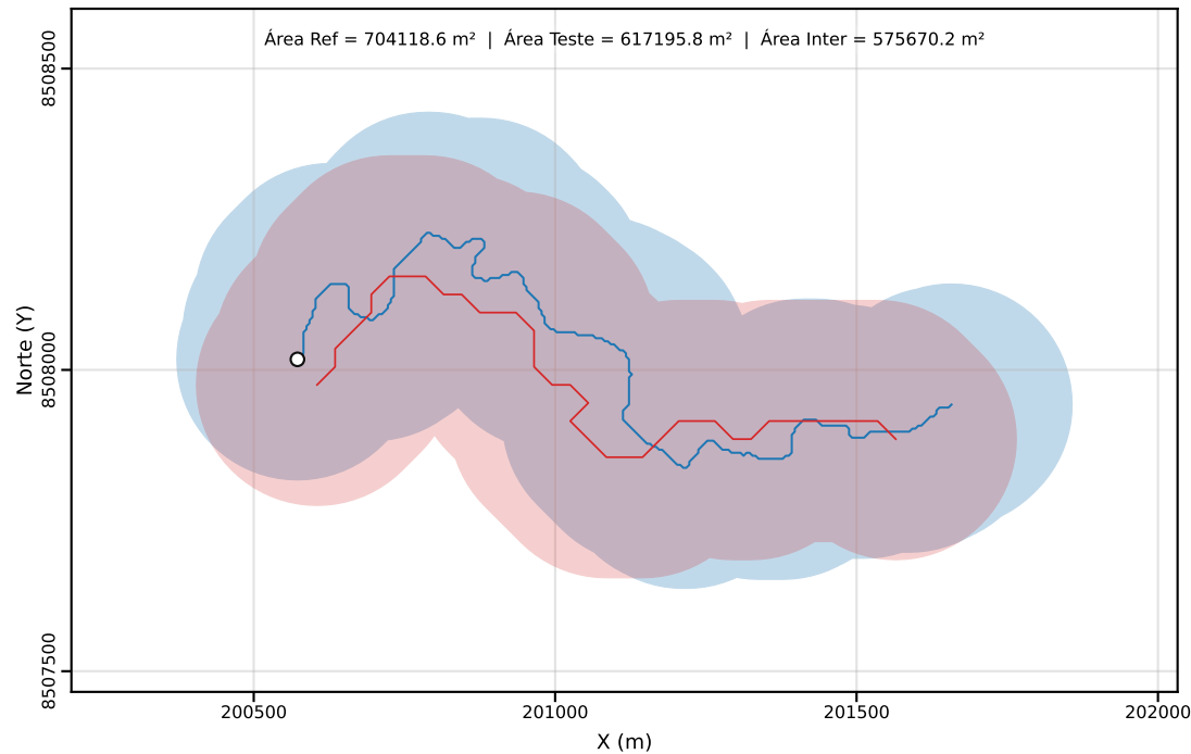
Classe C | PEC-PCD (Horizontal)=200.00 m | dm = 130.76
