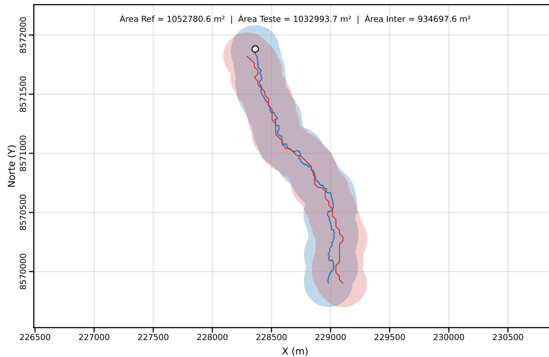
Classe C | PEC-PCD (Horizontal)=200.00 m | dm = 71.82
