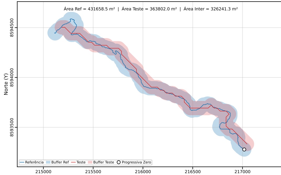
Classe C | PEC-PCD (Horizontal)=200.00 m | dm = 88.91
