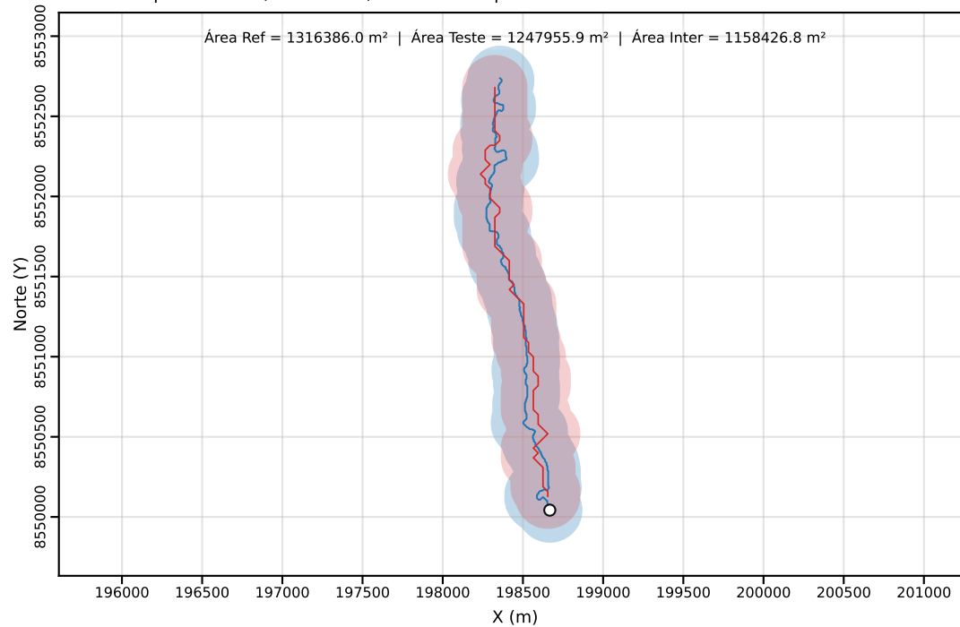
Classe C | PEC-PCD (Horizontal)=200.00 m | dm = 79.53
