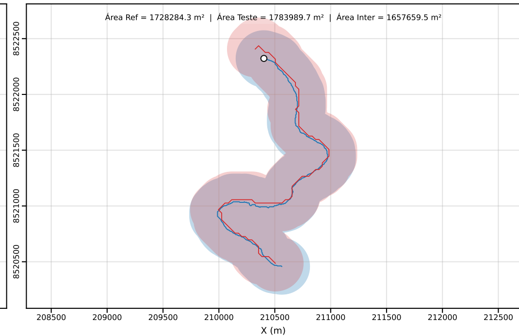
Classe D | PEC-PCD (Horizontal)=250.00 m | dm = 31.09
