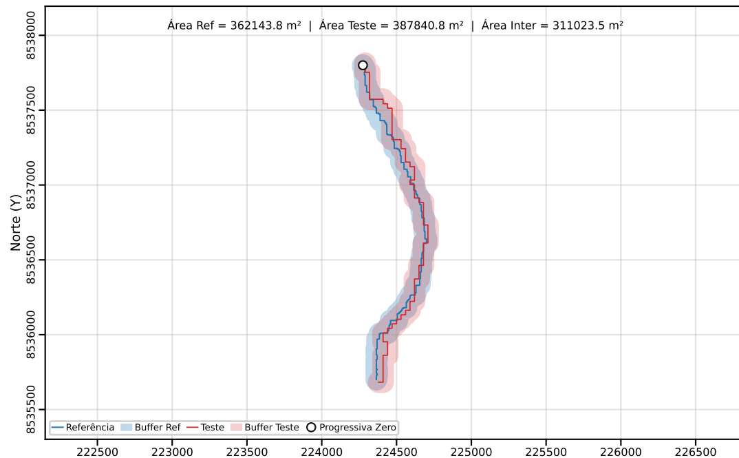
Classe C | PEC-PCD (Horizontal)=200.00 m | dm = 24.61
