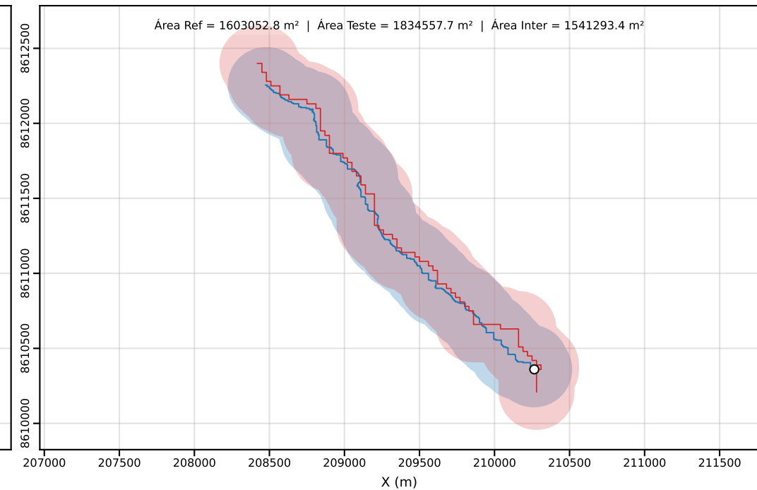
Classe D | PEC-PCD (Horizontal)=250.00 m | dm = 26.44
