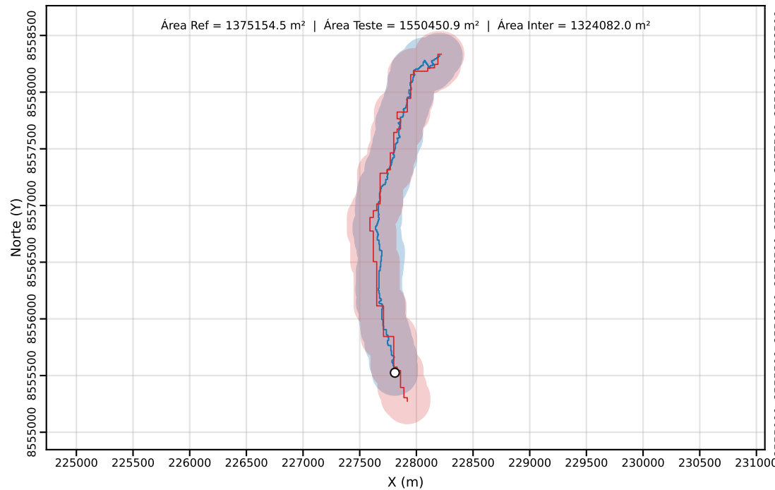
Classe C | PEC-PCD (Horizontal)=200.00 m | dm = 20.70
