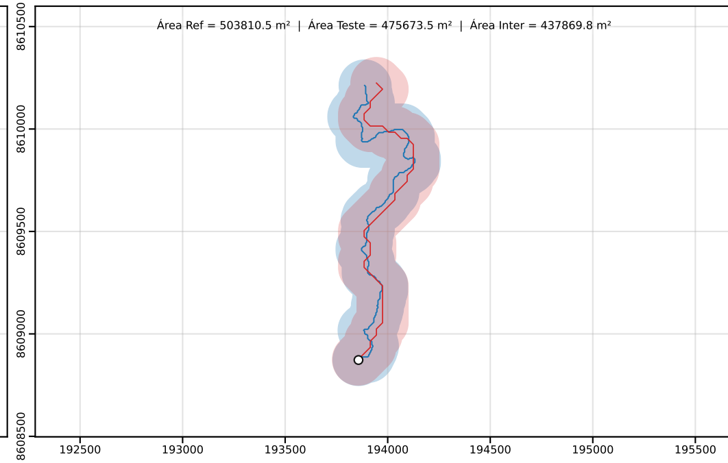
Classe D | PEC-PCD (Horizontal)=250.00 m | dm = 47.72
