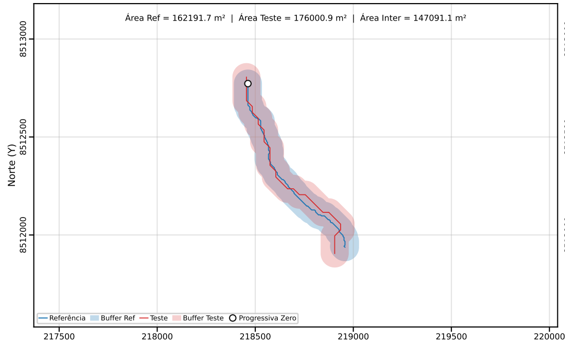
Classe C | PEC-PCD (Horizontal)=200.00 m | dm = 16.53
