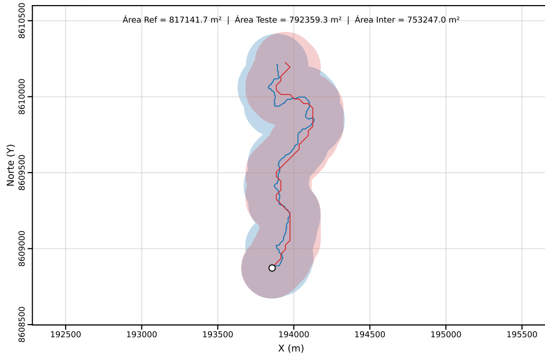
Classe C | PEC-PCD (Horizontal)=200.00 m | dm = 50.67
