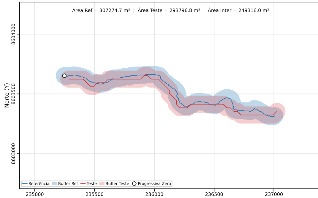
Classe C | PEC-PCD (Horizontal)=200.00 m | dm = 52.42
