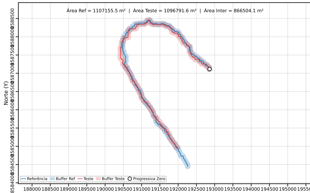
Classe C | PEC-PCD (Horizontal)=200.00 m | dm = 78.76
