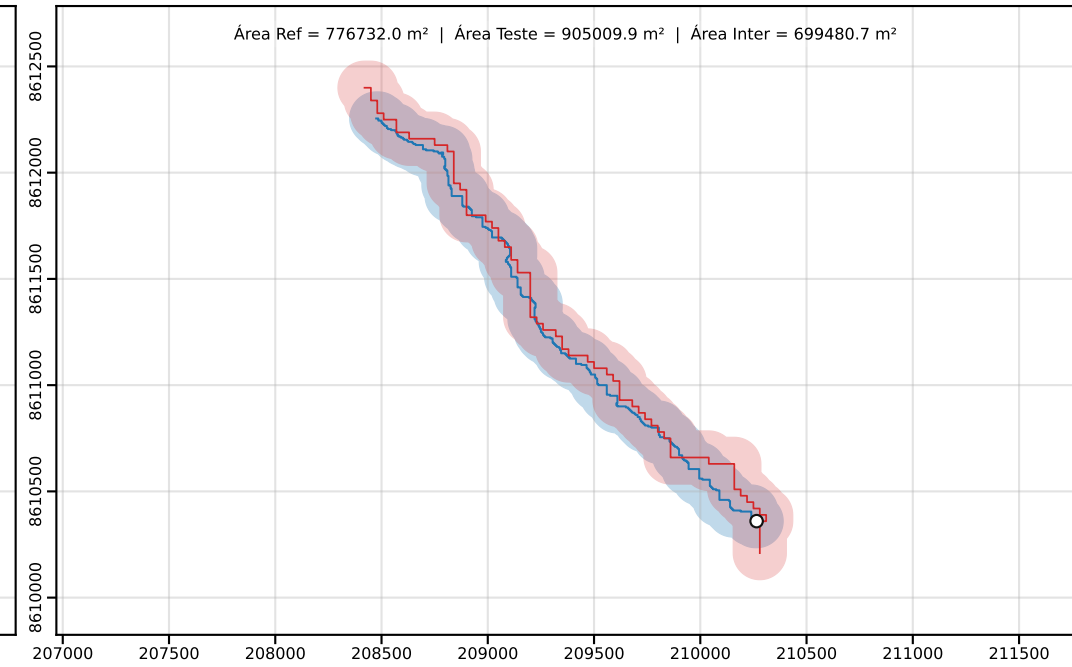
Classe D | PEC-PCD (Horizontal)=250.00 m | dm = 26.44
