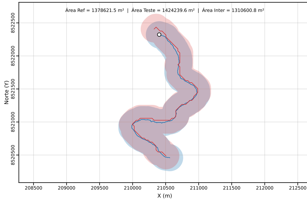
Classe C | PEC-PCD (Horizontal)=200.00 m | dm = 30.01
