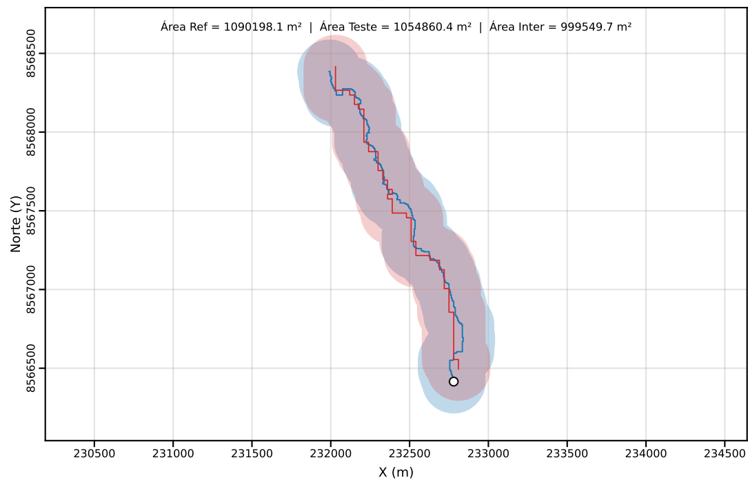
Classe C | PEC-PCD (Horizontal)=200.00 m | dm = 53.99
