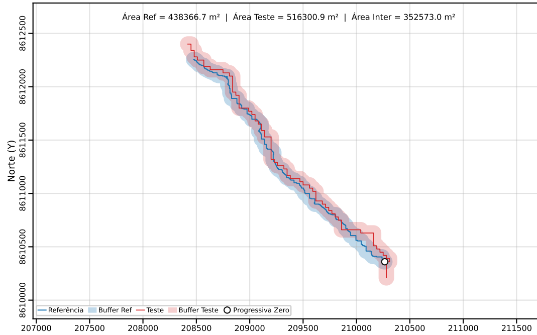
Classe C | PEC-PCD (Horizontal)=200.00 m | dm = 29.02
