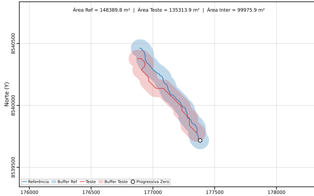
Classe C | PEC-PCD (Horizontal)=200.00 m | dm = 111.76
