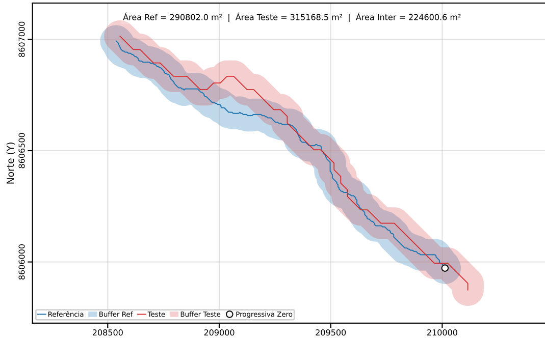
Classe C | PEC-PCD (Horizontal)=200.00 m | dm = 42.50
