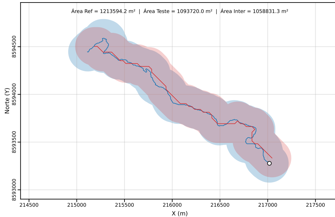
Classe C | PEC-PCD (Horizontal)=200.00 m | dm = 88.91
