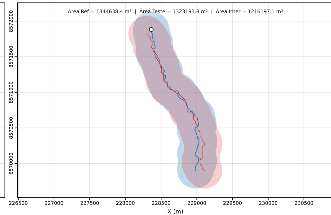
Classe D | PEC-PCD (Horizontal)=250.00 m | dm = 76.24
