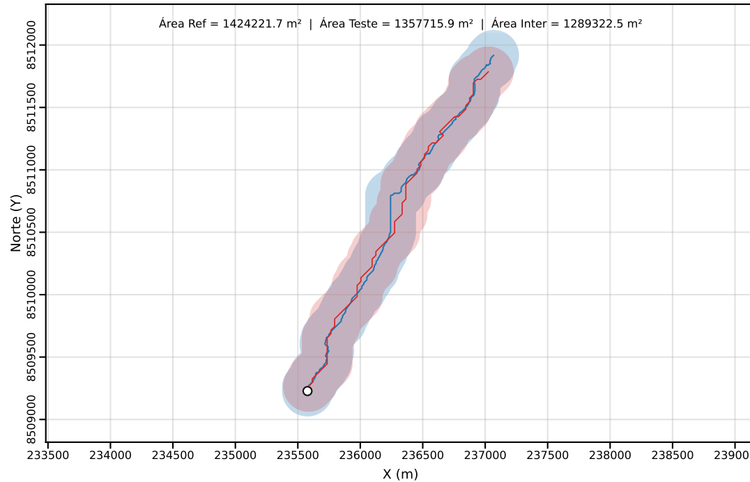
Classe C | PEC-PCD (Horizontal)=200.00 m | dm = 62.43
