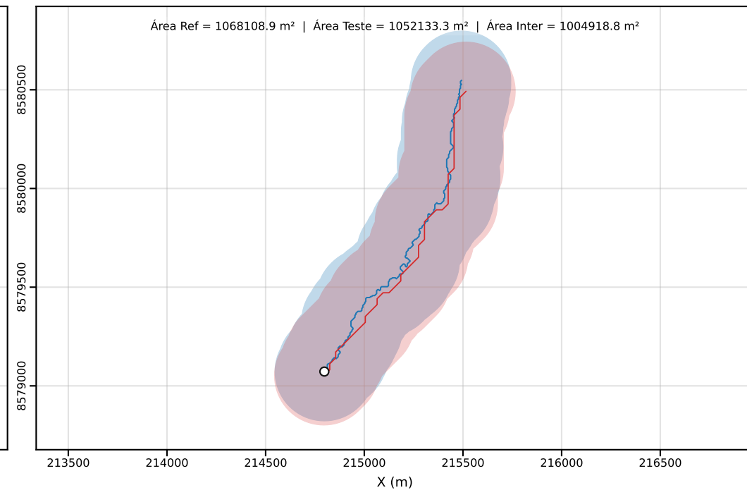
Classe D | PEC-PCD (Horizontal)=250.00 m | dm = 47.17
