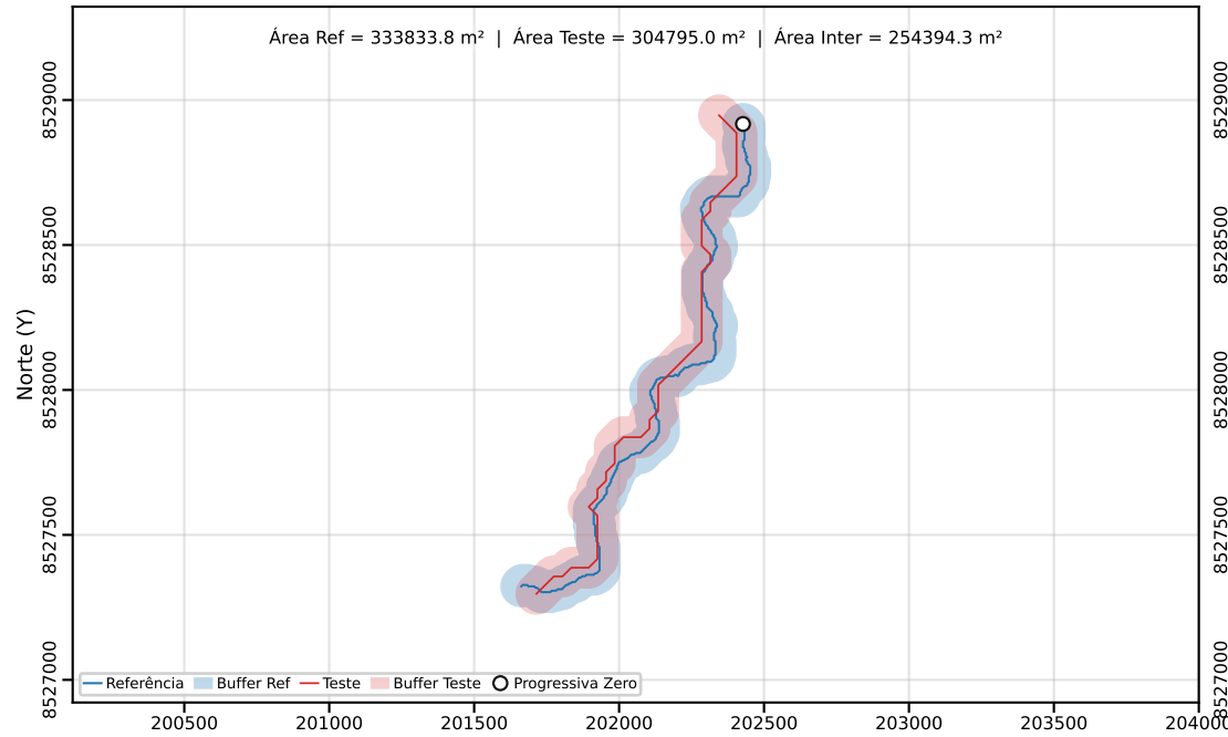
Classe C | PEC-PCD (Horizontal)=200.00 m | dm = 75.76
