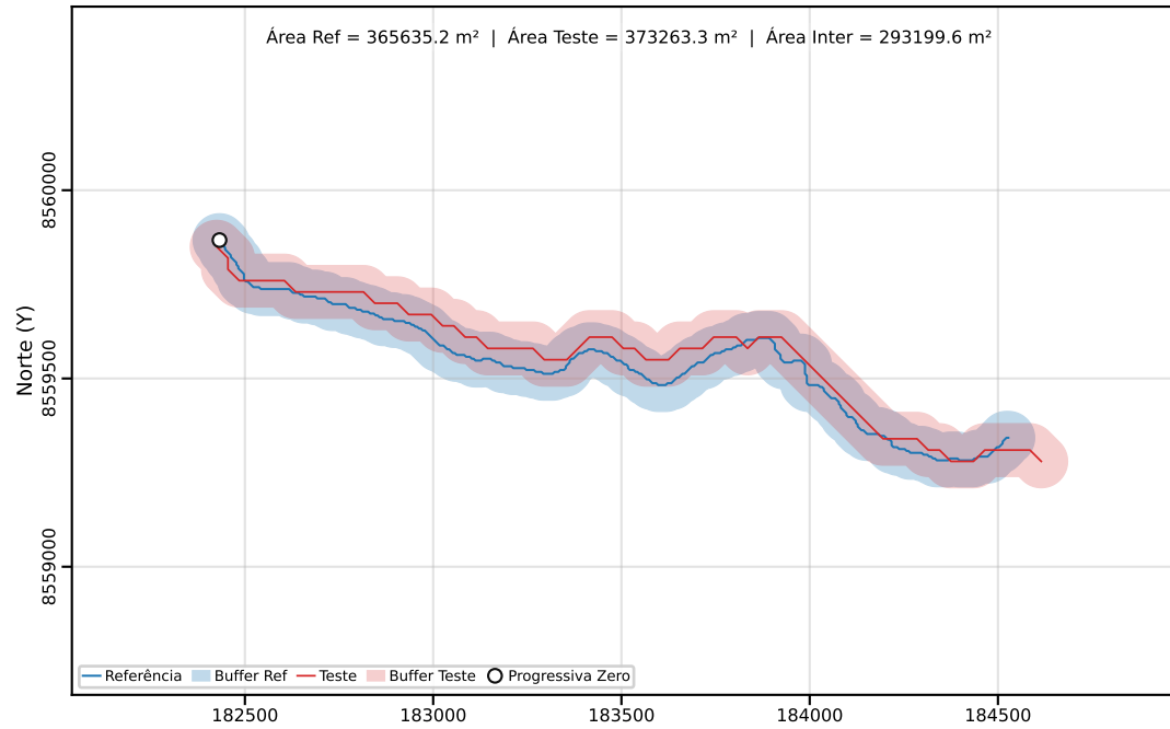
Classe C | PEC-PCD (Horizontal)=200.00 m | dm = 43.90
