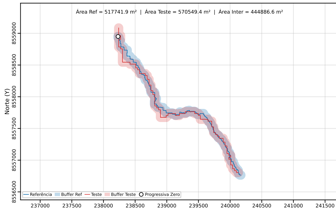
Classe C | PEC-PCD (Horizontal)=200.00 m | dm = 28.13
