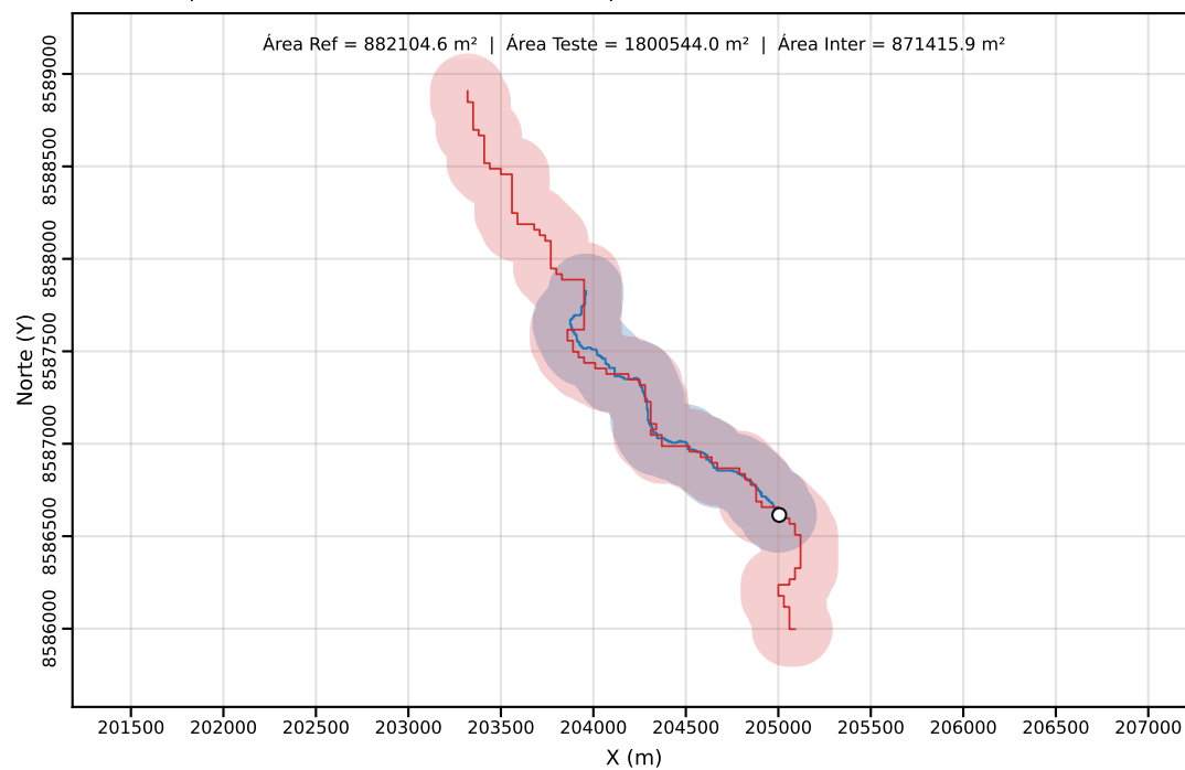
Classe C | PEC-PCD (Horizontal)=200.00 m | dm = 3.73
