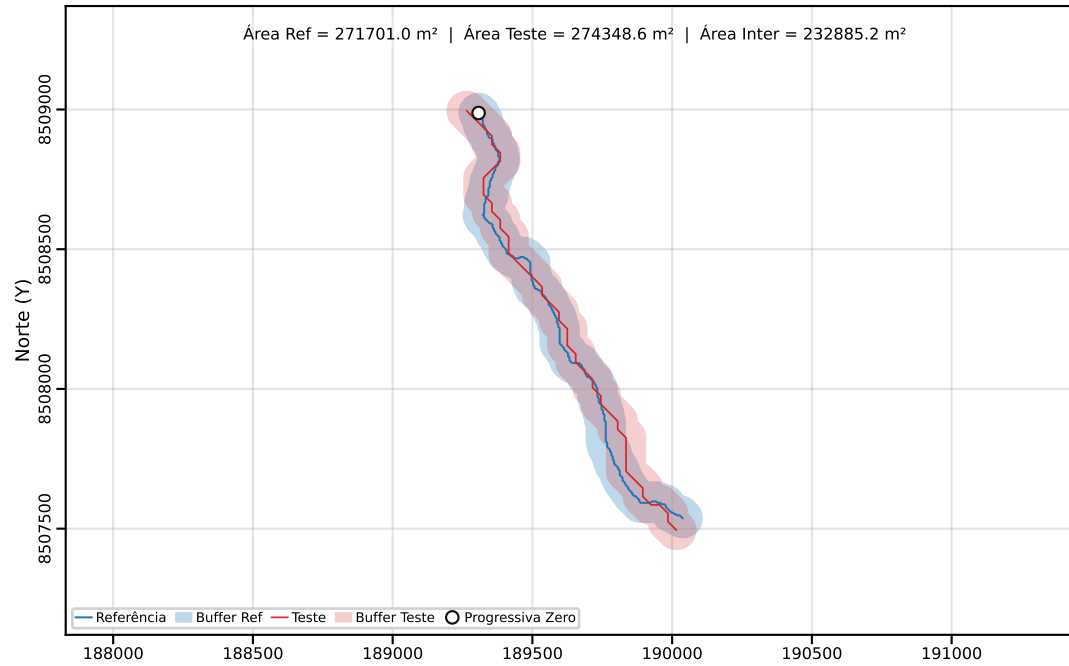
Classe C | PEC-PCD (Horizontal)=200.00 m | dm = 33.98
