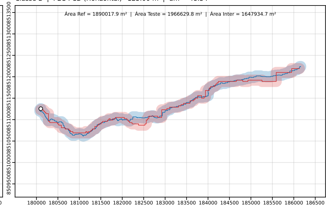
Classe D | PEC-PCD (Horizontal)=250.00 m | dm = 45.43
