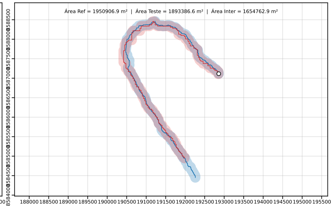
Classe D | PEC-PCD (Horizontal)=250.00 m | dm = 90.11
