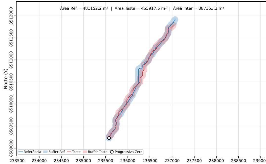
Classe C | PEC-PCD (Horizontal)=200.00 m | dm = 62.43
