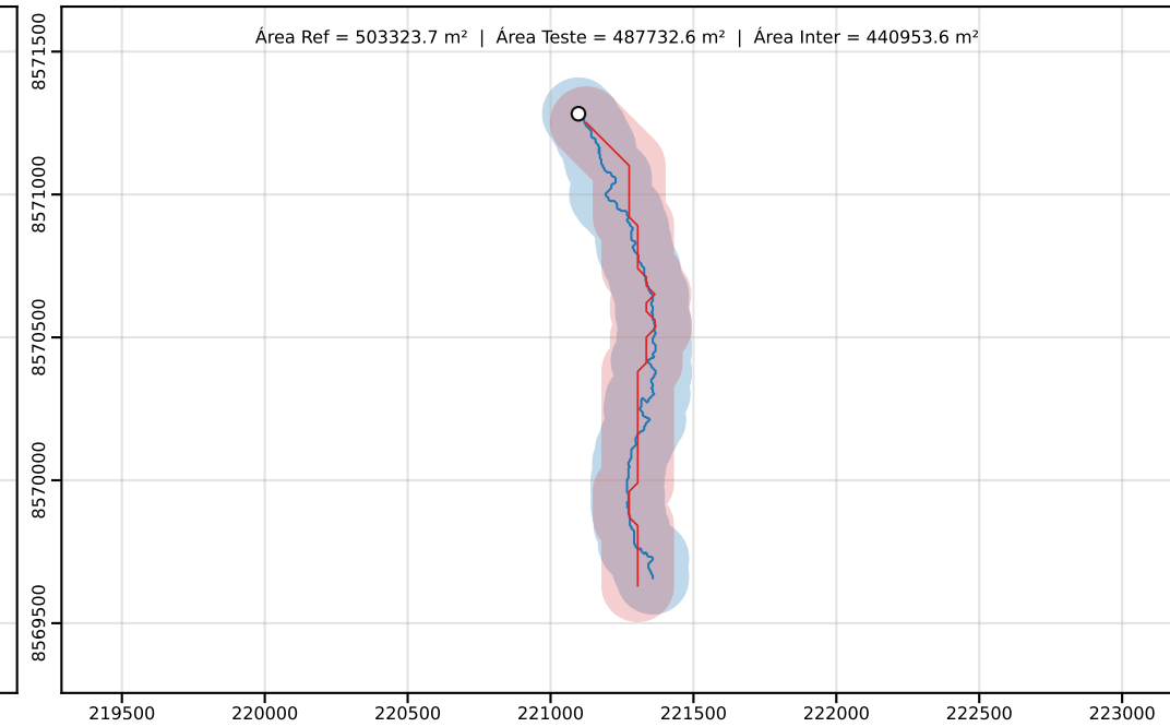
Classe D | PEC-PCD (Horizontal)=250.00 m | dm = 56.40
