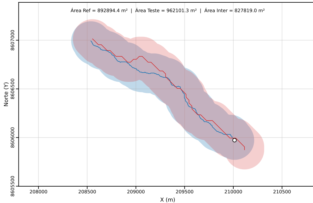
Classe C | PEC-PCD (Horizontal)=200.00 m | dm = 42.50
