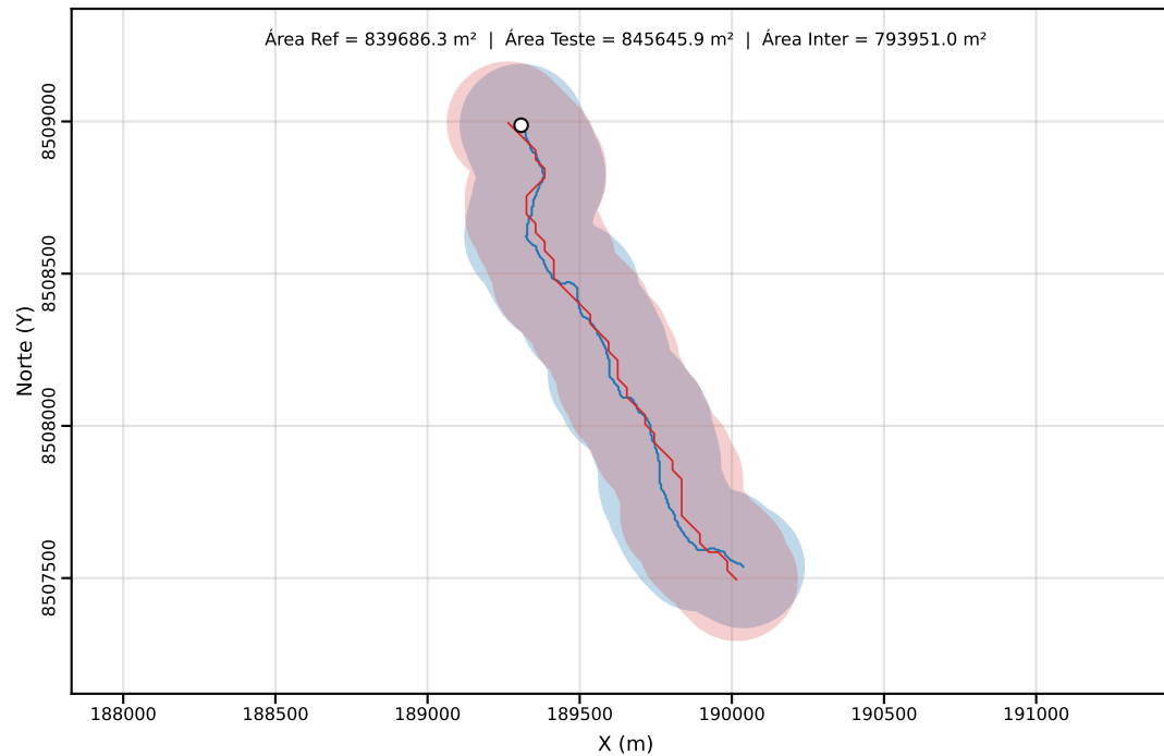
Classe C | PEC-PCD (Horizontal)=200.00 m | dm = 33.98
