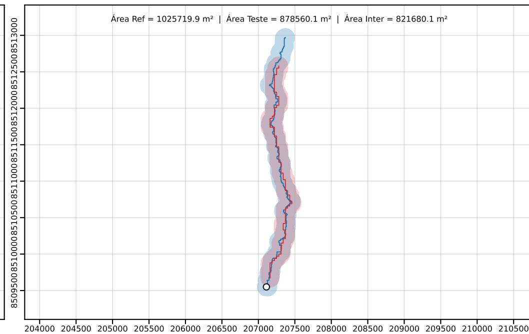
Classe D | PEC-PCD (Horizontal)=250.00 m | dm = 148.48
