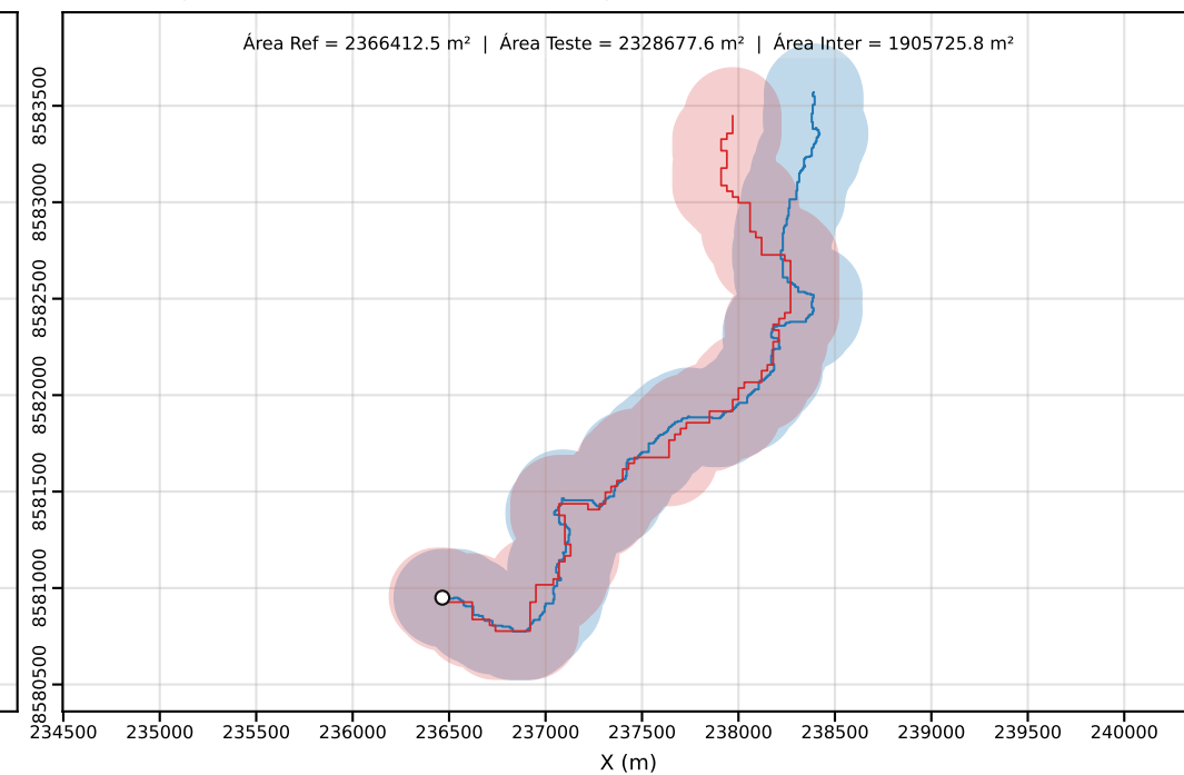
Classe D | PEC-PCD (Horizontal)=250.00 m | dm = 155.38
