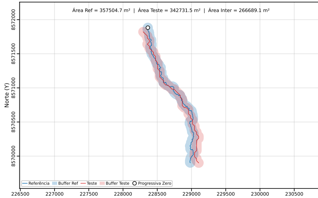
Classe C | PEC-PCD (Horizontal)=200.00 m | dm = 71.82
