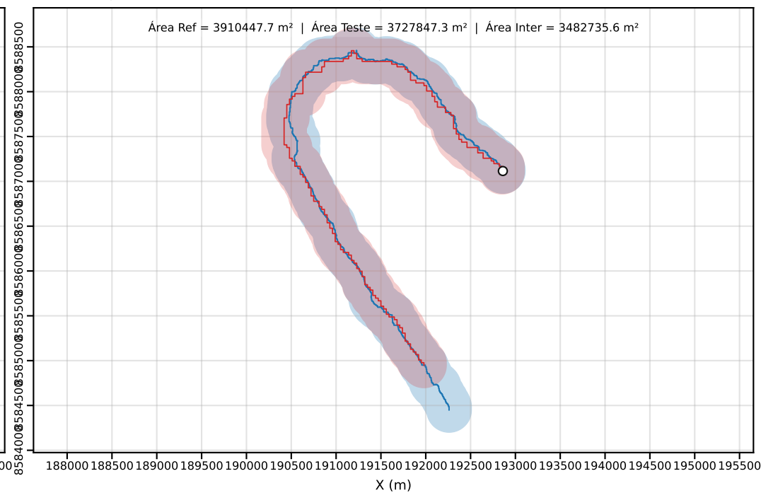
Classe D | PEC-PCD (Horizontal)=250.00 m | dm = 90.11
