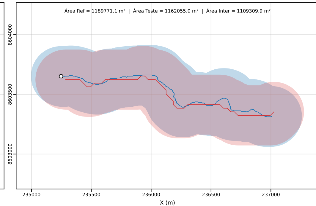
Classe D | PEC-PCD (Horizontal)=250.00 m | dm = 54.38
