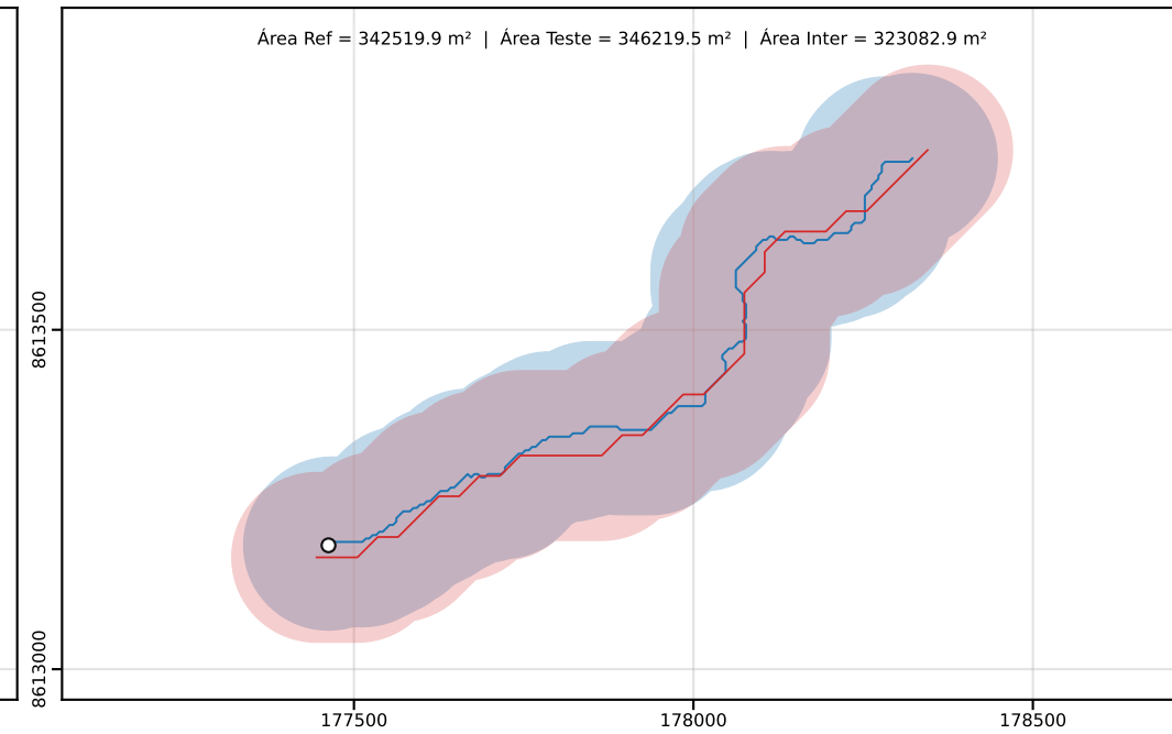
Classe D | PEC-PCD (Horizontal)=250.00 m | dm = 20.94
