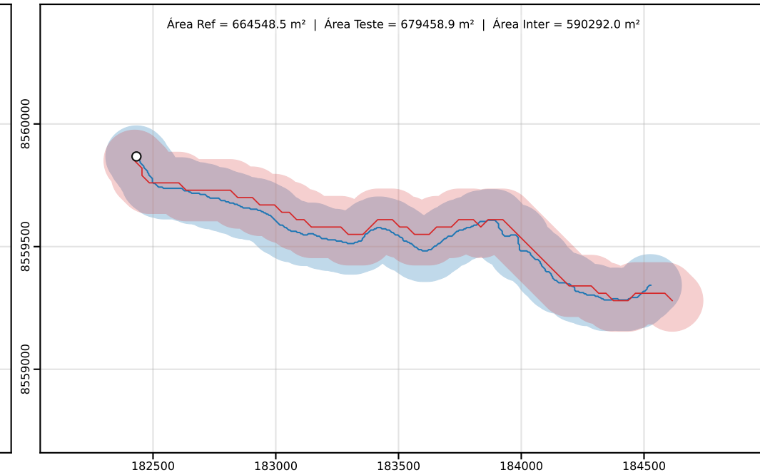
Classe D | PEC-PCD (Horizontal)=250.00 m | dm = 44.36
