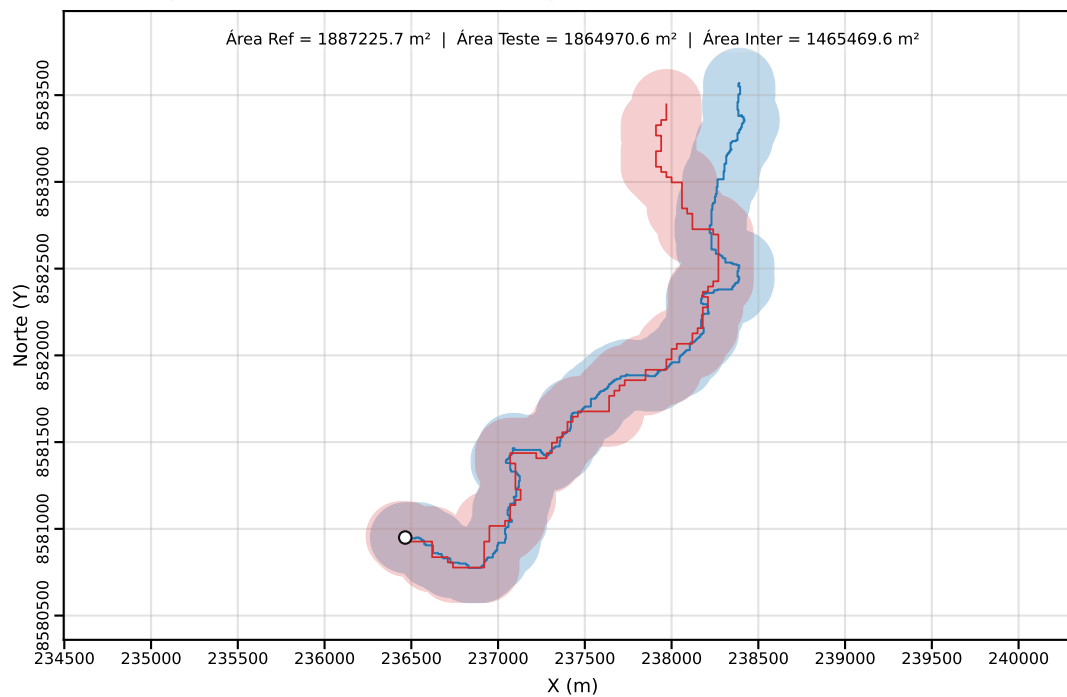
Classe C | PEC-PCD (Horizontal)=200.00 m | dm = 142.09
