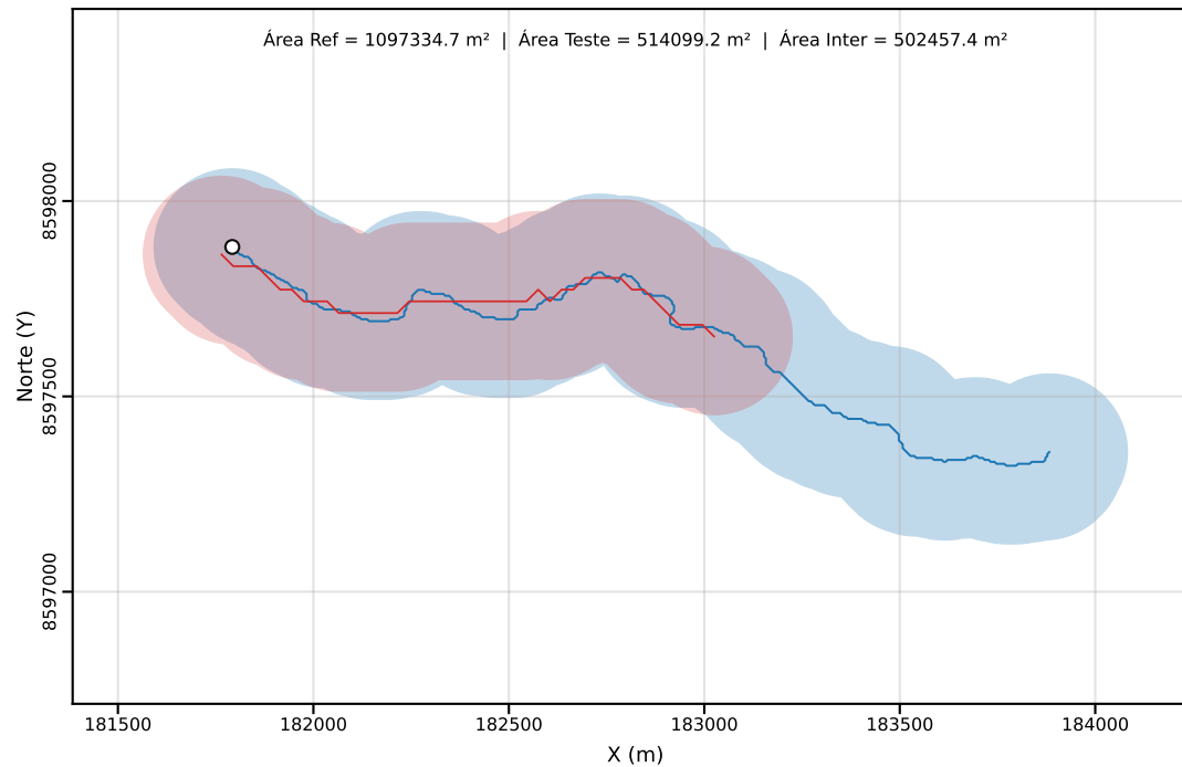
Classe C | PEC-PCD (Horizontal)=200.00 m | dm = 727.04
