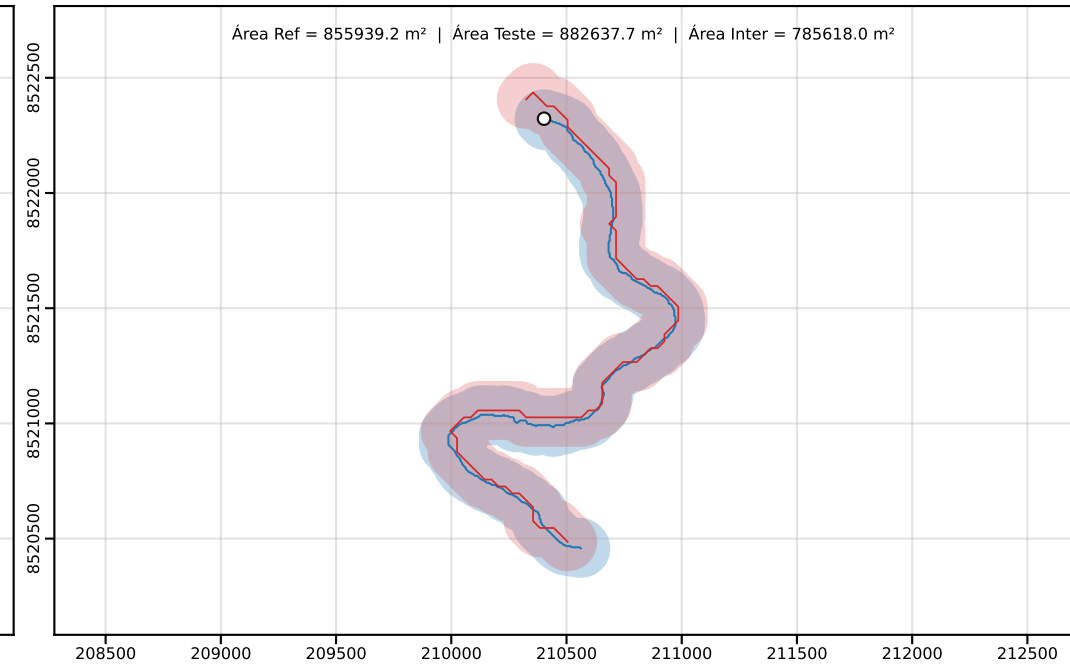
Classe D | PEC-PCD (Horizontal)=250.00 m | dm = 31.09
