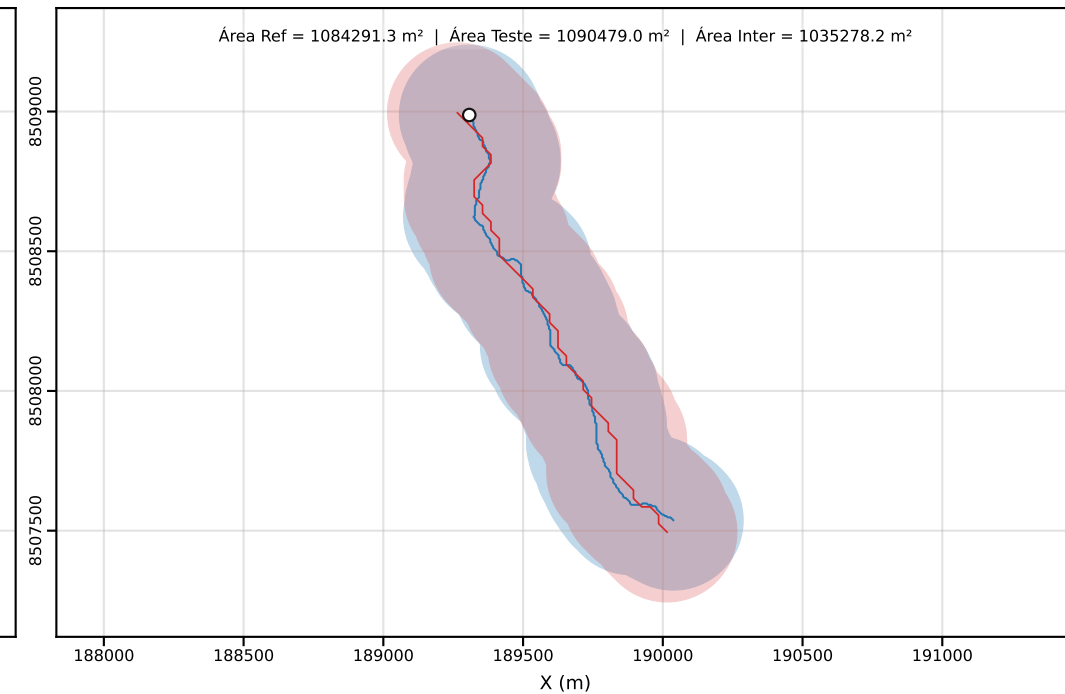
Classe D | PEC-PCD (Horizontal)=250.00 m | dm = 35.30
