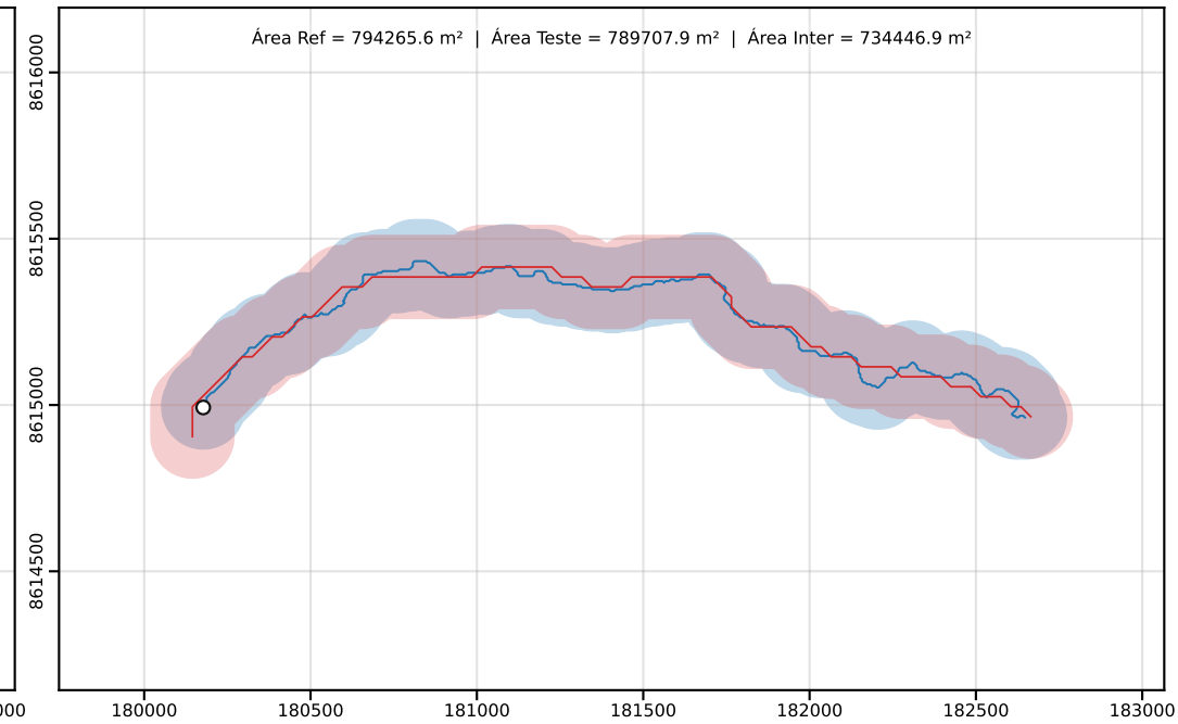
Classe D | PEC-PCD (Horizontal)=250.00 m | dm = 30.54
