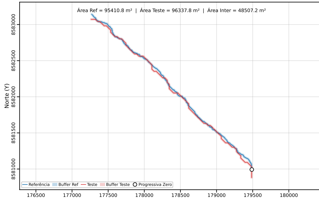
Classe C | PEC-PCD (Horizontal)=40.00 m | dm = 23.96
