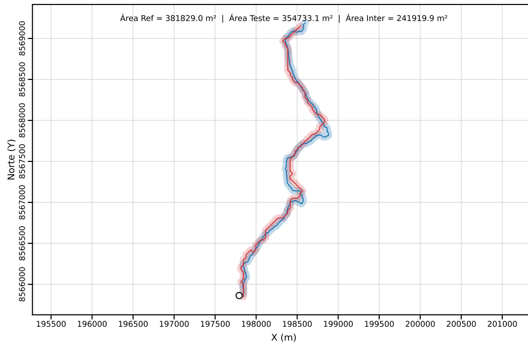
Classe C | PEC-PCD (Horizontal)=40.00 m | dm = 49.56
