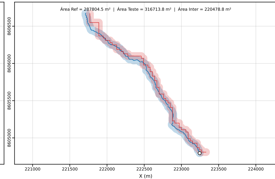
Classe D | PEC-PCD (Horizontal)=50.00 m | dm = 33.39
