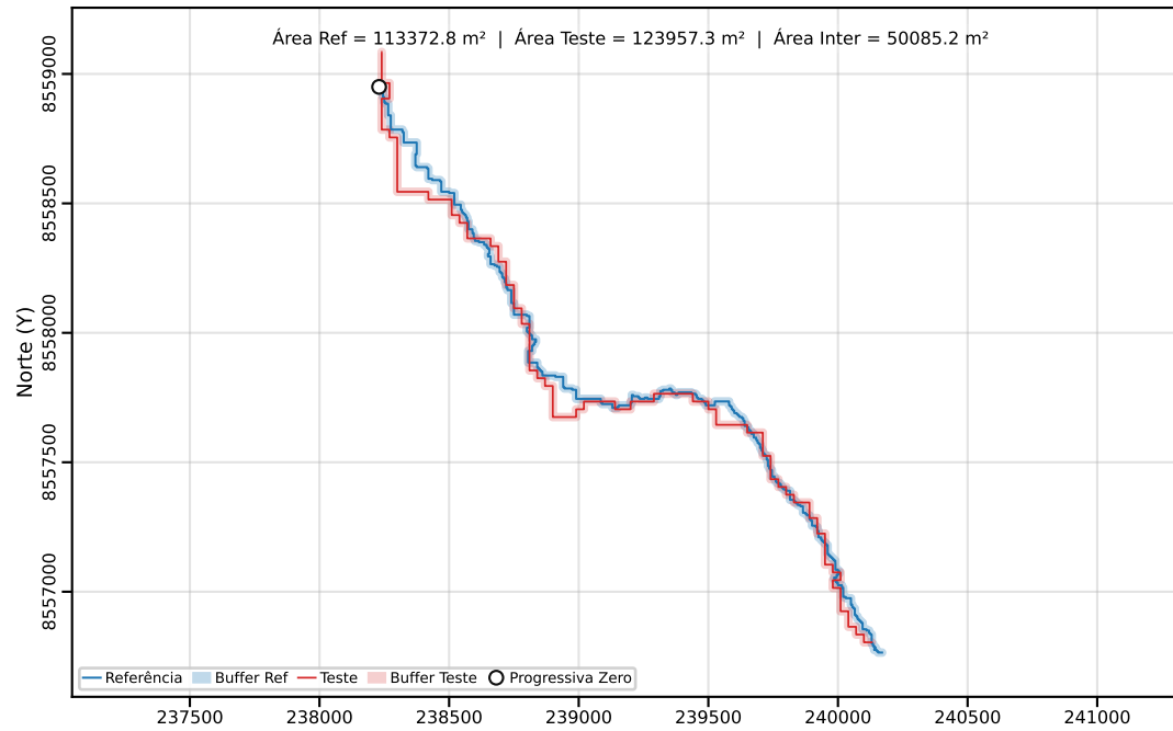
Classe C | PEC-PCD (Horizontal)=40.00 m | dm = 28.42
