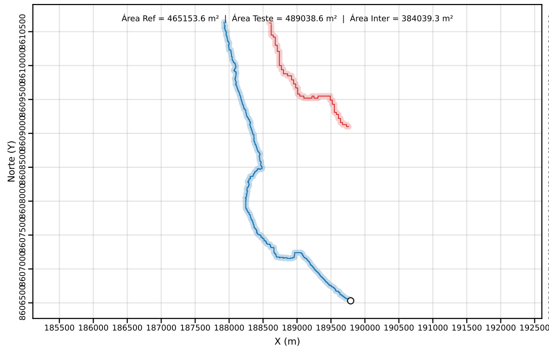
Classe C | PEC-PCD (Horizontal)=40.00 m | dm = 20.84
