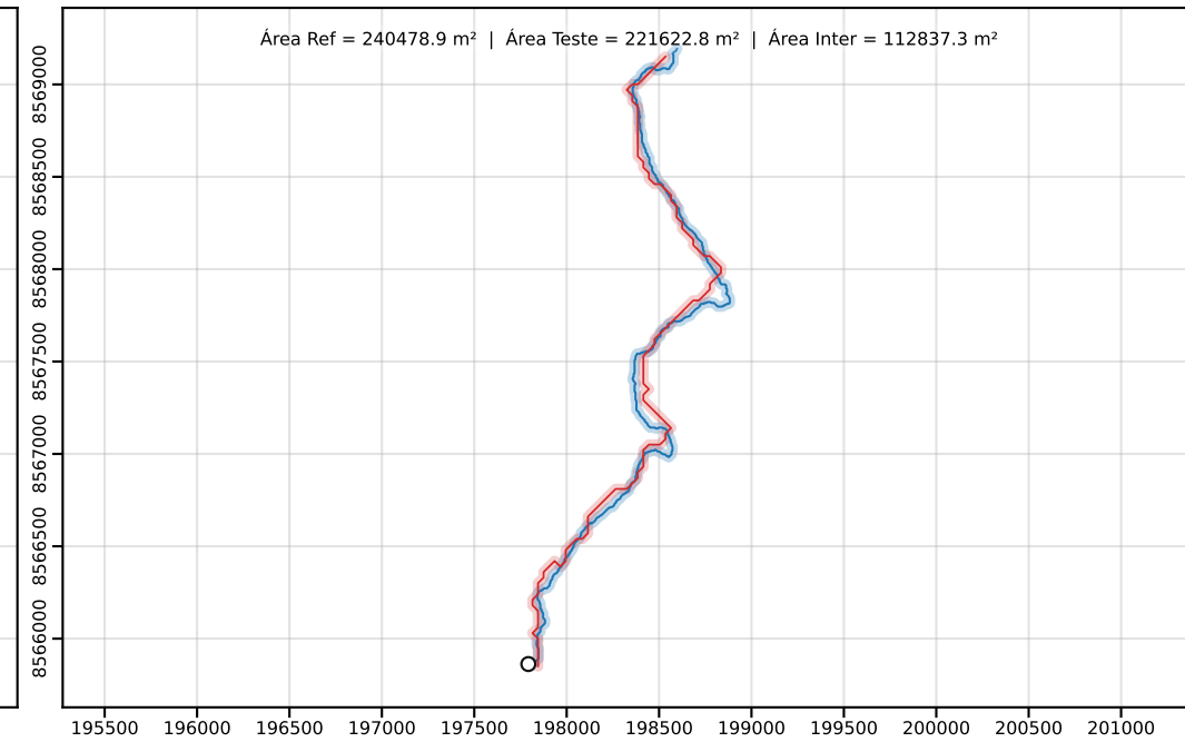
Classe D | PEC-PCD (Horizontal)=50.00 m | dm = 50.85
