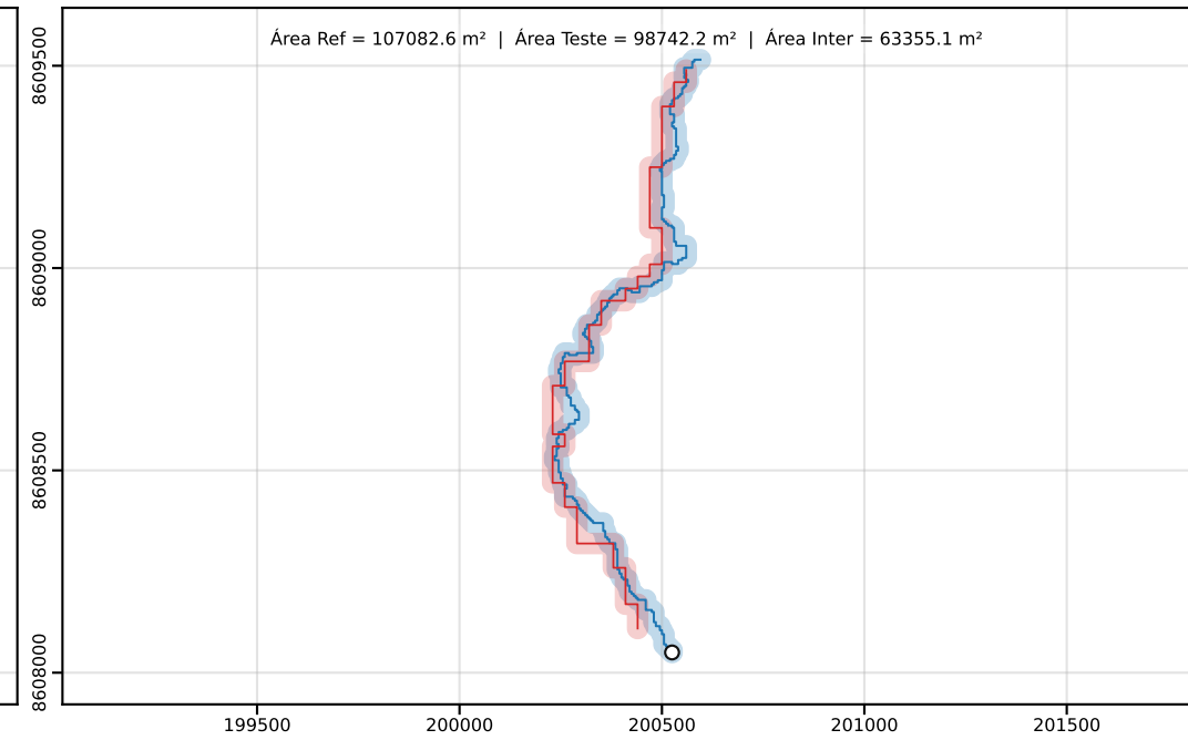
Classe D | PEC-PCD (Horizontal)=50.00 m | dm = 40.79
