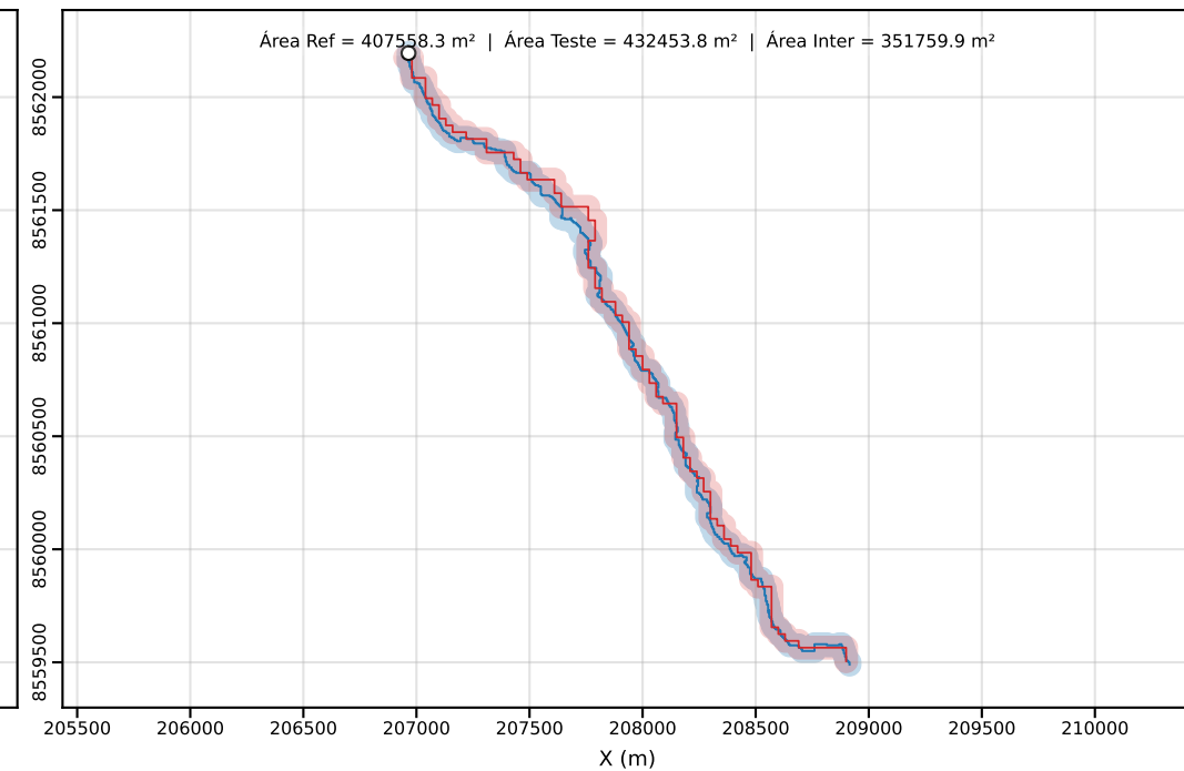
Classe D | PEC-PCD (Horizontal)=50.00 m | dm = 20.27
