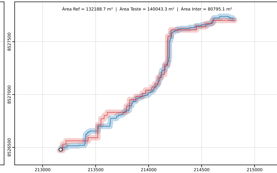
Classe D | PEC-PCD (Horizontal)=50.00 m | dm = 28.91
