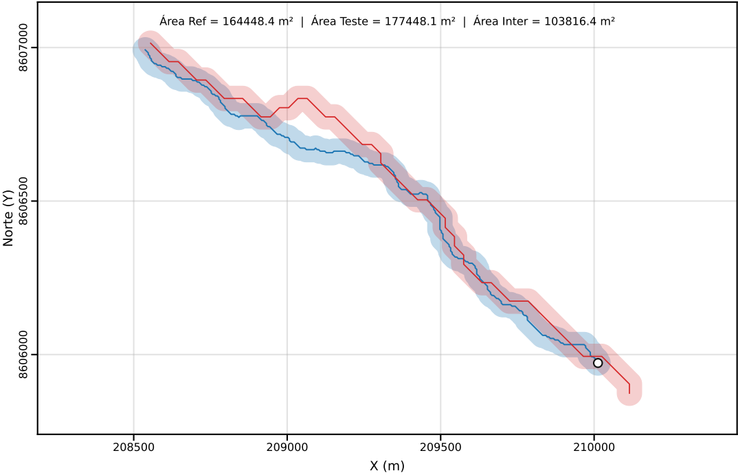
Classe C | PEC-PCD (Horizontal)=40.00 m | dm = 42.94
