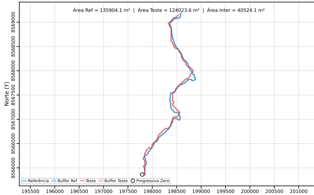
Classe C | PEC-PCD (Horizontal)=40.00 m | dm = 49.56
