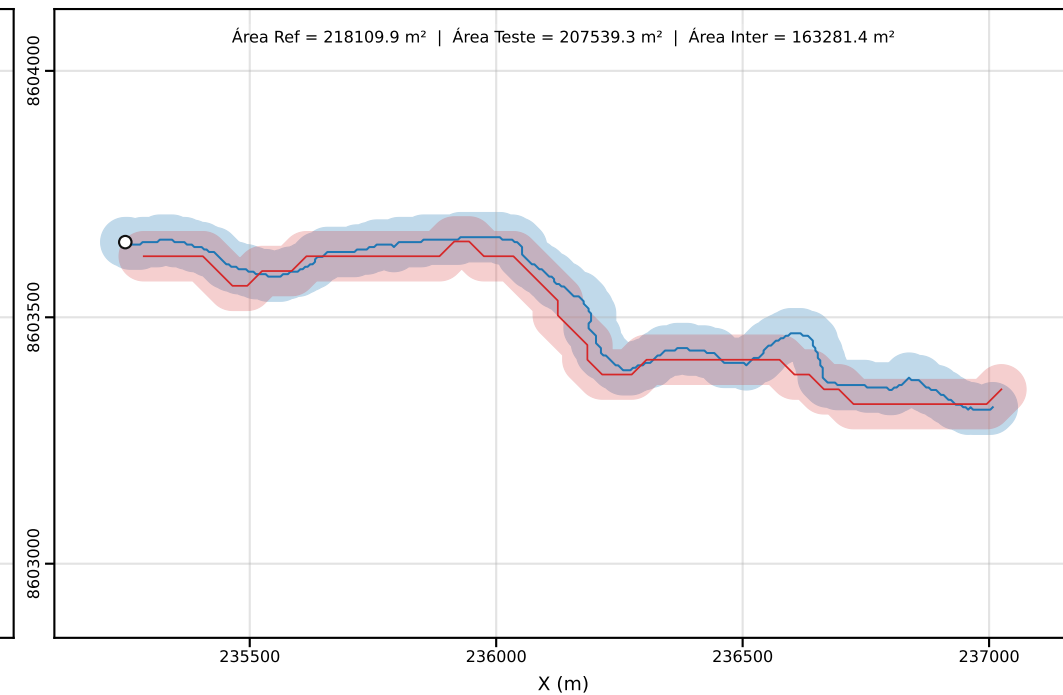
Classe D | PEC-PCD (Horizontal)=50.00 m | dm = 41.50
