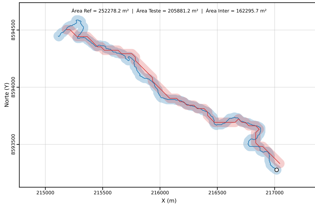
Classe C | PEC-PCD (Horizontal)=40.00 m | dm = 54.92
