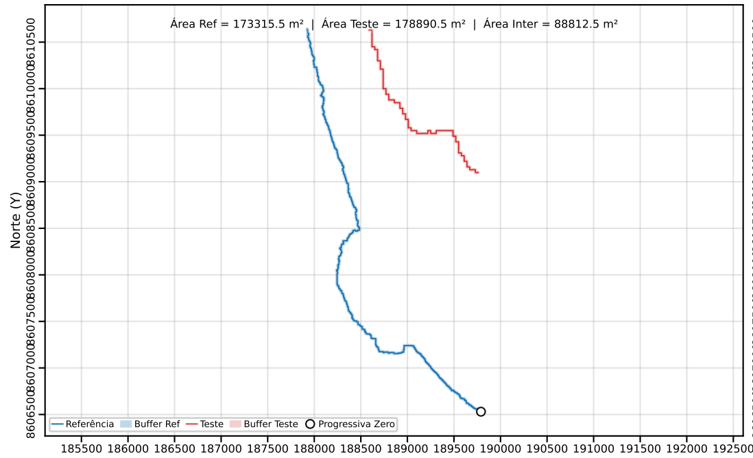
Classe C | PEC-PCD (Horizontal)=40.00 m | dm = 20.84
