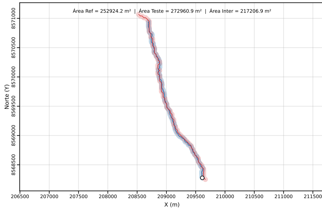
Classe C | PEC-PCD (Horizontal)=40.00 m | dm = 16.44
