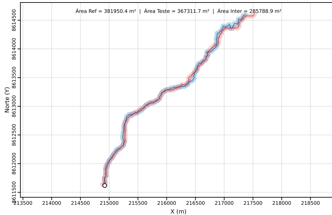
Classe C | PEC-PCD (Horizontal)=40.00 m | dm = 32.90
