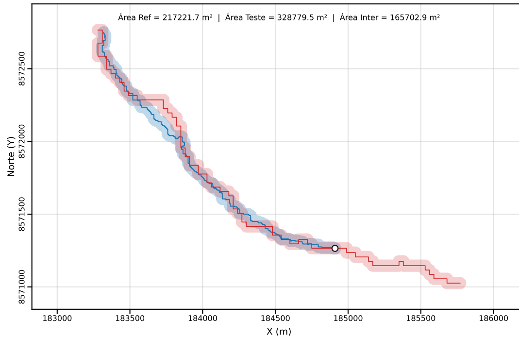
Classe C | PEC-PCD (Horizontal)=40.00 m | dm = 19.69
