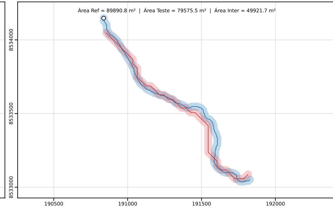
Classe D | PEC-PCD (Horizontal)=50.00 m | dm = 46.29
