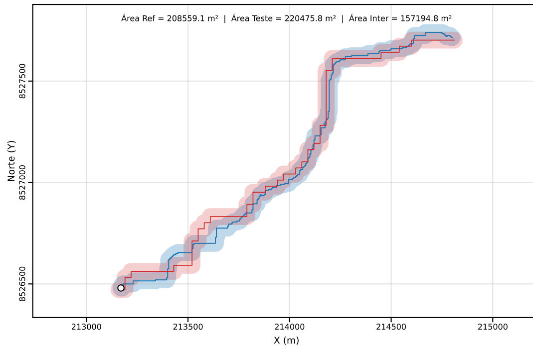
Classe C | PEC-PCD (Horizontal)=40.00 m | dm = 29.28
