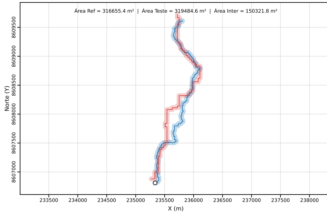
Classe C | PEC-PCD (Horizontal)=40.00 m | dm = 65.42
