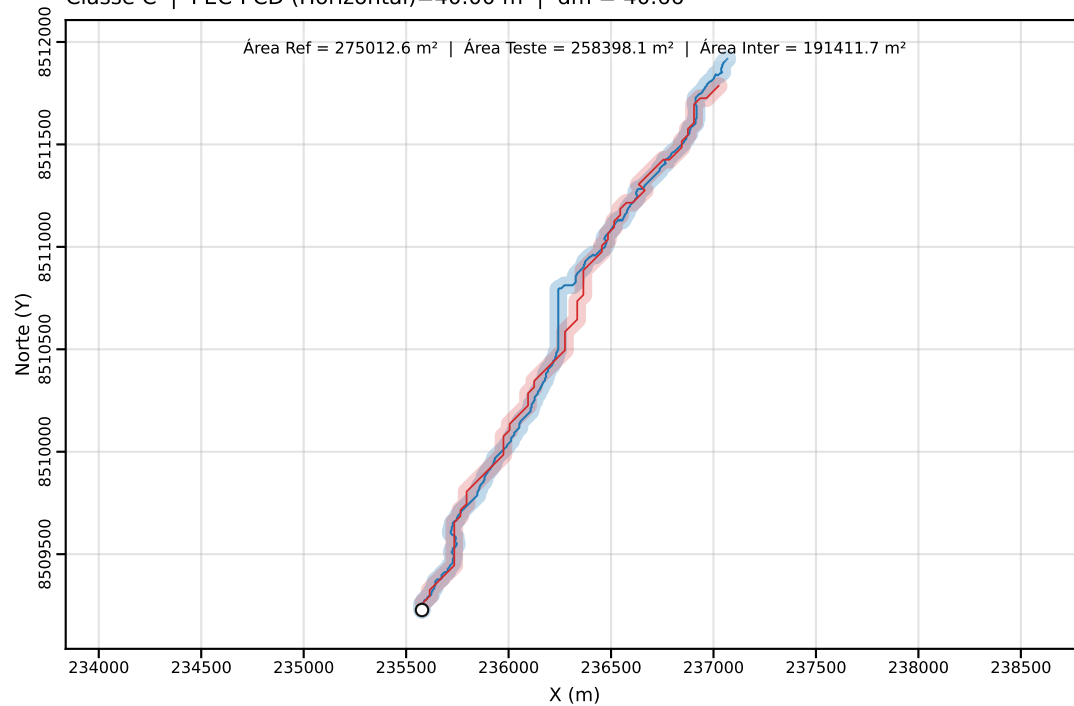
Classe C | PEC-PCD (Horizontal)=40.00 m | dm = 40.66
