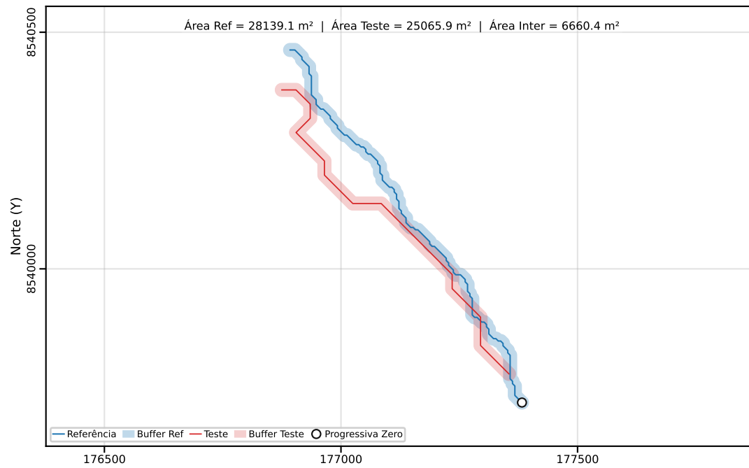
Classe C | PEC-PCD (Horizontal)=40.00 m | dm = 67.17
