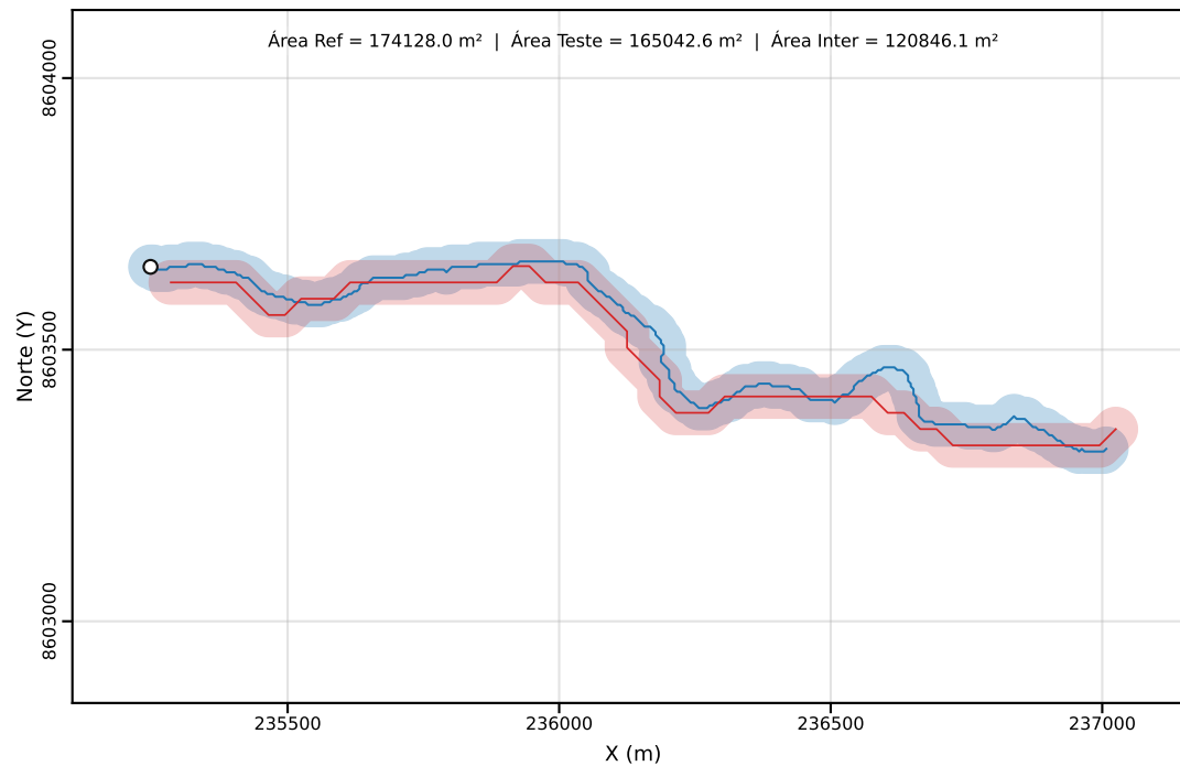
Classe C | PEC-PCD (Horizontal)=40.00 m | dm = 40.57
