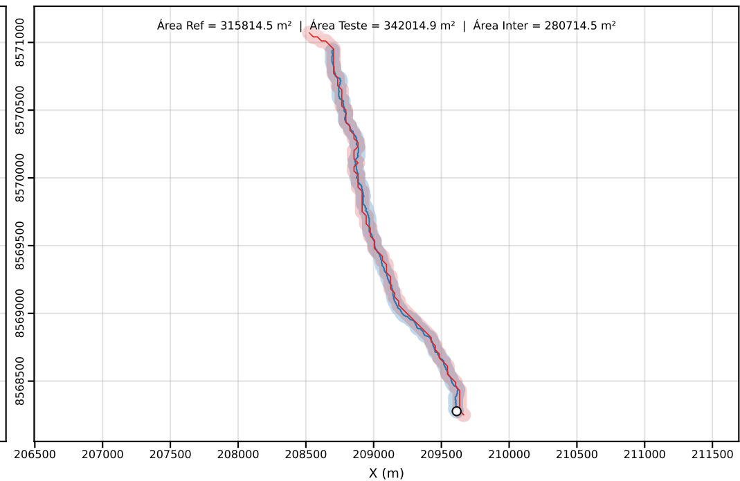
Classe D | PEC-PCD (Horizontal)=50.00 m | dm = 16.12
