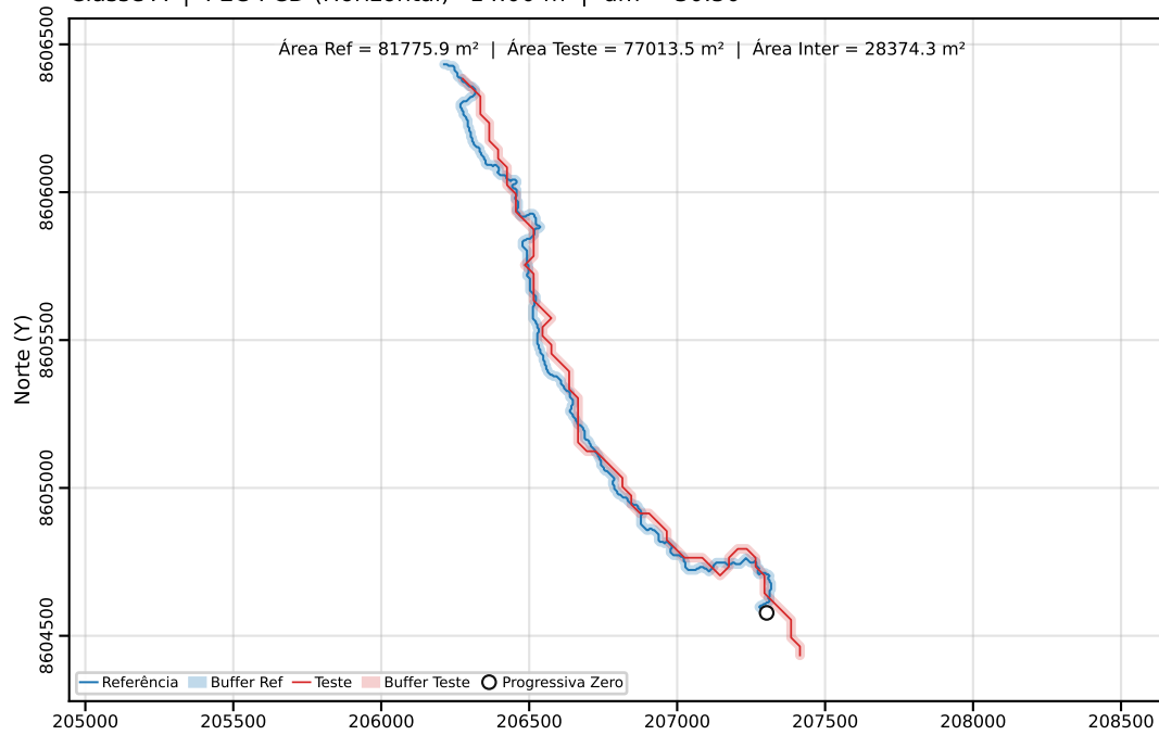
Classe C | PEC-PCD (Horizontal)=40.00 m | dm = 39.35
