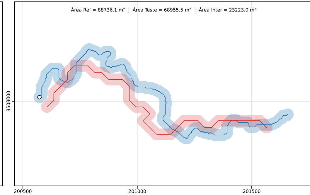
Classe D | PEC-PCD (Horizontal)=50.00 m | dm = 93.56
