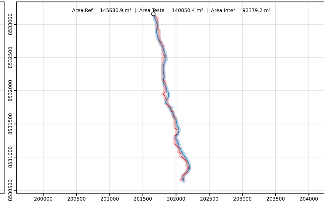
Classe D | PEC-PCD (Horizontal)=50.00 m | dm = 31.48
