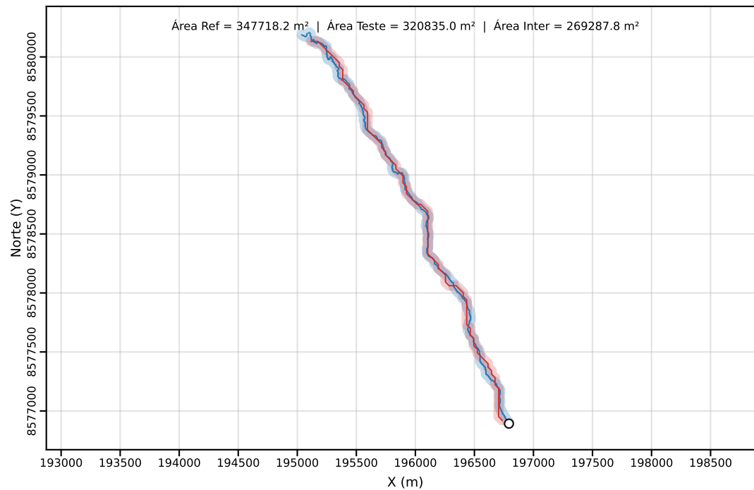
Classe C | PEC-PCD (Horizontal)=40.00 m | dm = 30.72
