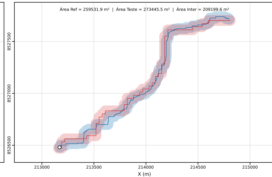
Classe D | PEC-PCD (Horizontal)=50.00 m | dm = 28.91
