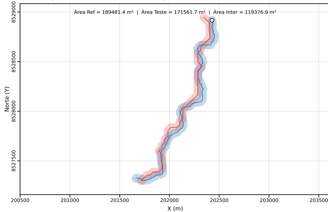
Classe C | PEC-PCD (Horizontal)=40.00 m | dm = 51.35
