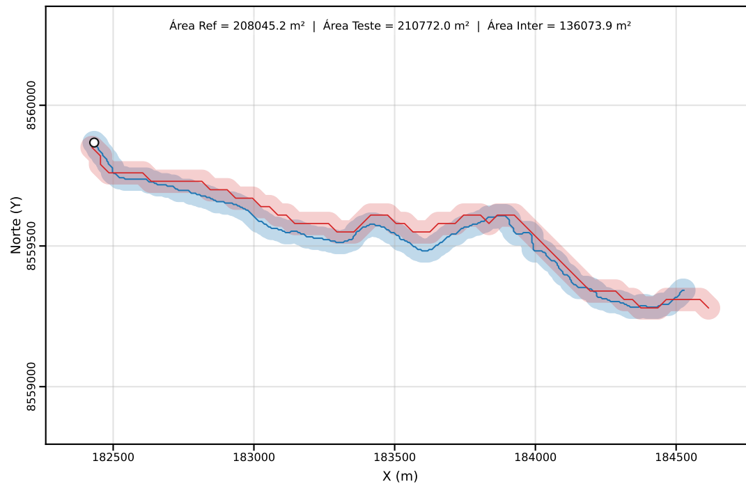
Classe C | PEC-PCD (Horizontal)=40.00 m | dm = 42.91
