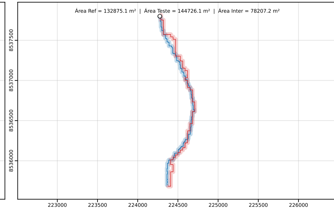
Classe D | PEC-PCD (Horizontal)=50.00 m | dm = 29.85
