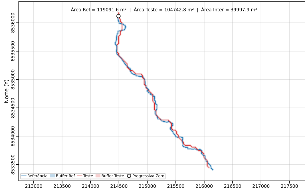
Classe C | PEC-PCD (Horizontal)=40.00 m | dm = 43.20
