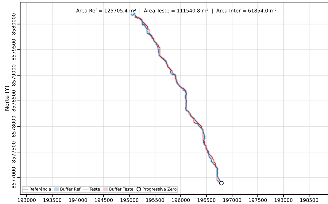
Classe C | PEC-PCD (Horizontal)=40.00 m | dm = 30.72
