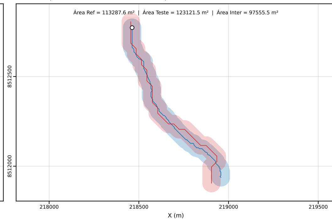
Classe D | PEC-PCD (Horizontal)=50.00 m | dm = 20.07
