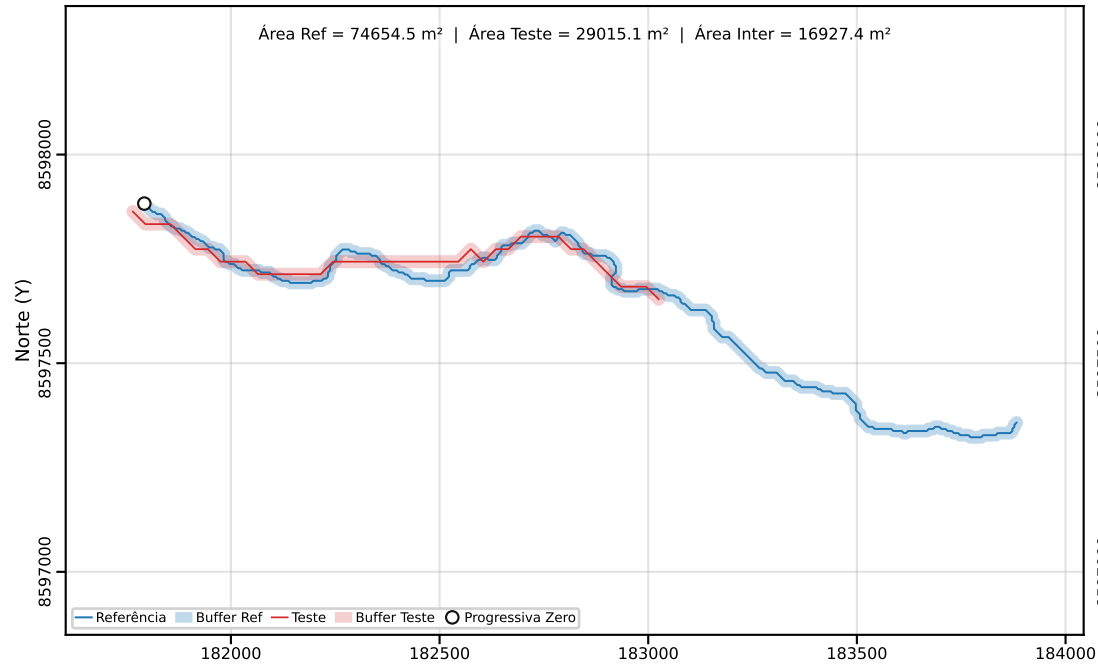
Classe C | PEC-PCD (Horizontal)=40.00 m | dm = 203.31
