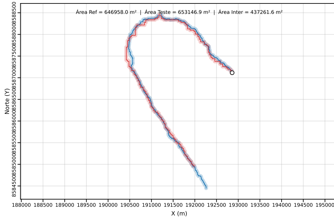
Classe C | PEC-PCD (Horizontal)=40.00 m | dm = 40.35
