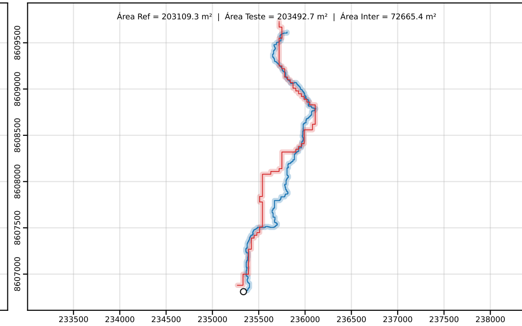
Classe D | PEC-PCD (Horizontal)=50.00 m | dm = 72.80
