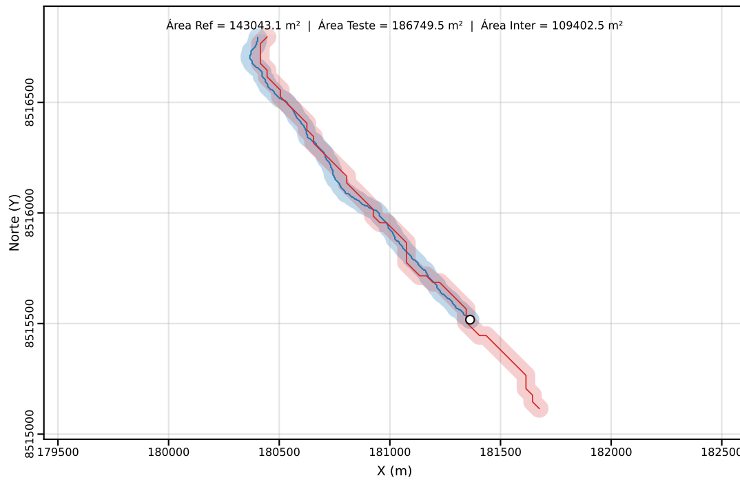
Classe C | PEC-PCD (Horizontal)=40.00 m | dm = 22.64
