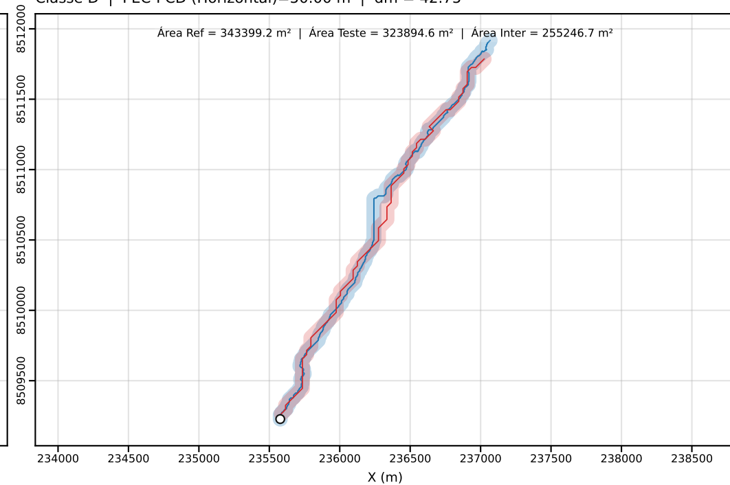
Classe D | PEC-PCD (Horizontal)=50.00 m | dm = 42.75
