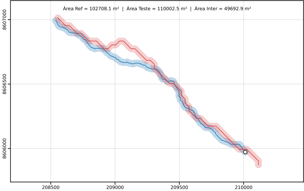
Classe D | PEC-PCD (Horizontal)=50.00 m | dm = 45.19
