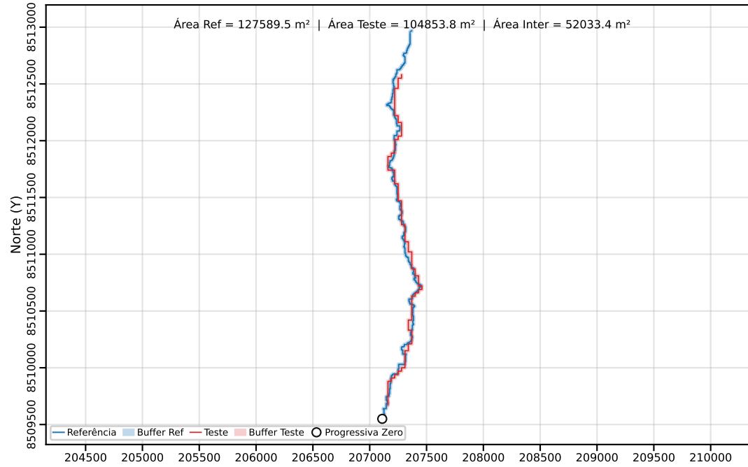
Classe C | PEC-PCD (Horizontal)=40.00 m | dm = 47.71
