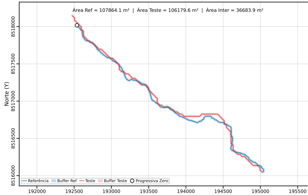
Classe C | PEC-PCD (Horizontal)=40.00 m | dm = 38.90
