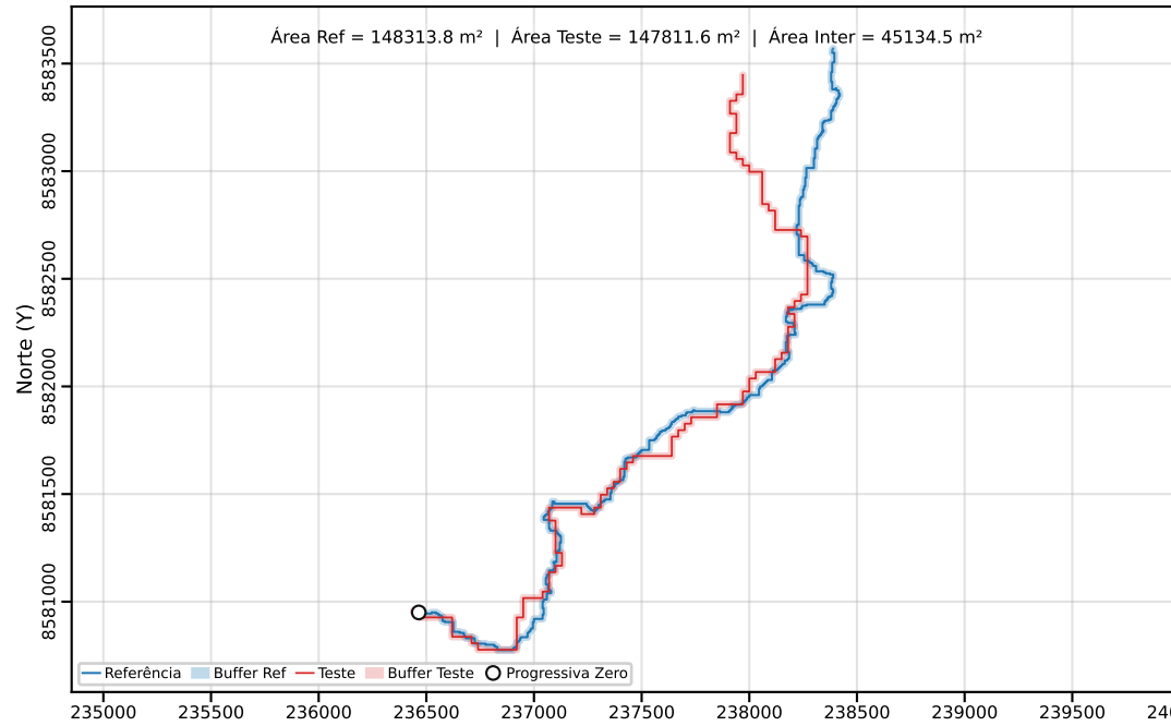
Classe C | PEC-PCD (Horizontal)=40.00 m | dm = 54.66
