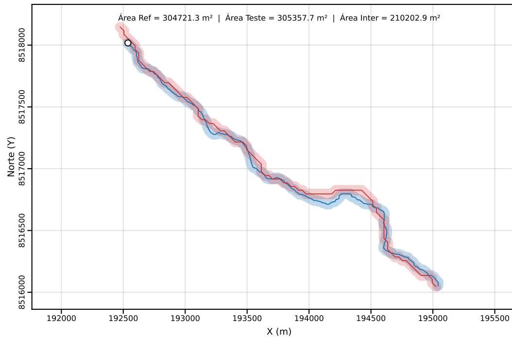
Classe C | PEC-PCD (Horizontal)=40.00 m | dm = 38.90
