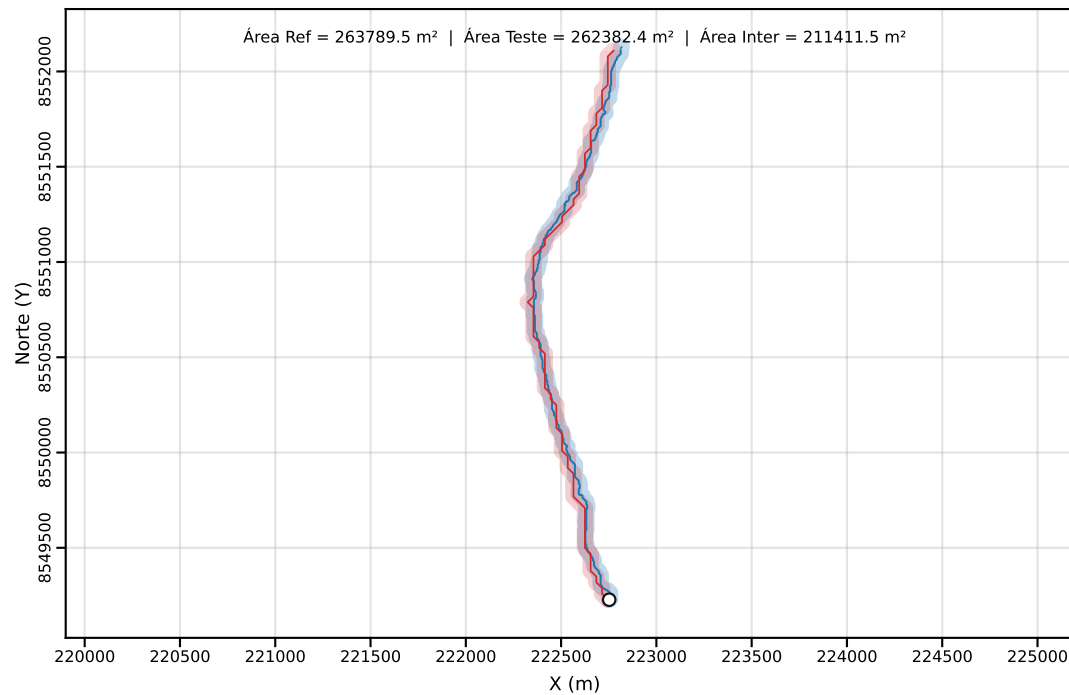
Classe C | PEC-PCD (Horizontal)=40.00 m | dm = 25.09
