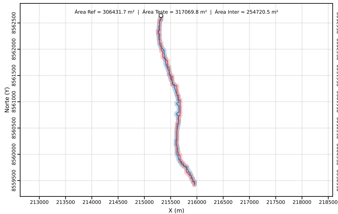
Classe C | PEC-PCD (Horizontal)=40.00 m | dm = 20.49
