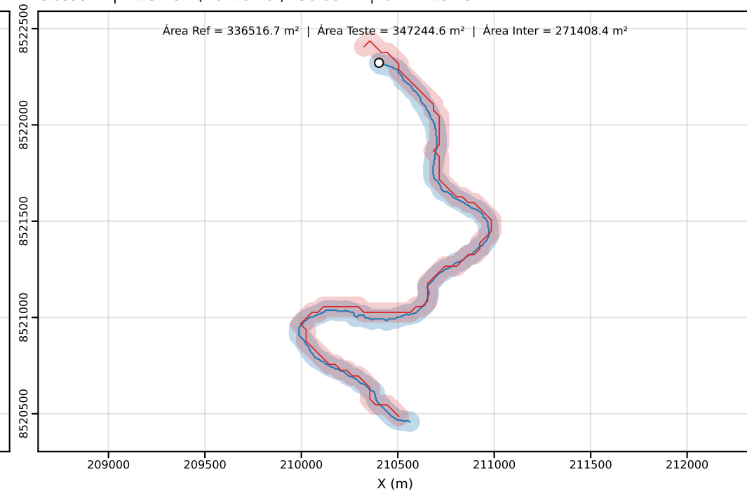
Classe D | PEC-PCD (Horizontal)=50.00 m | dm = 29.45
