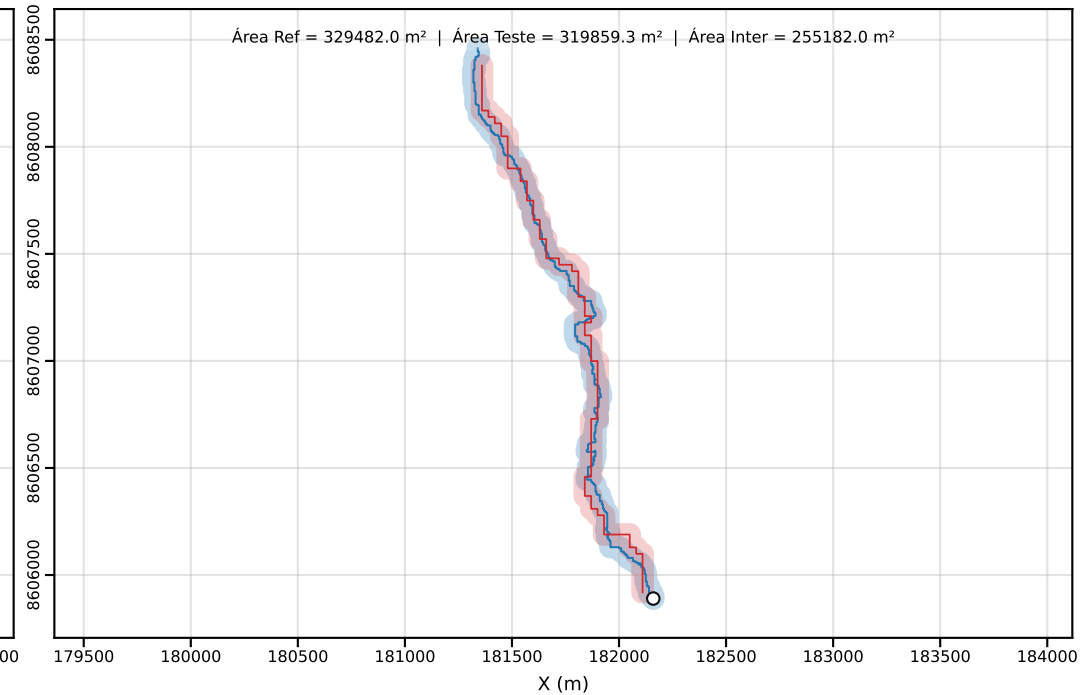
Classe D | PEC-PCD (Horizontal)=50.00 m | dm = 36.49
