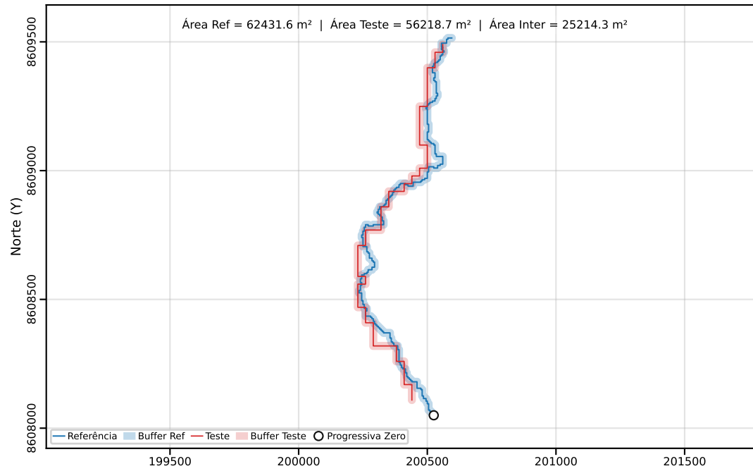
Classe C | PEC-PCD (Horizontal)=40.00 m | dm = 38.40
