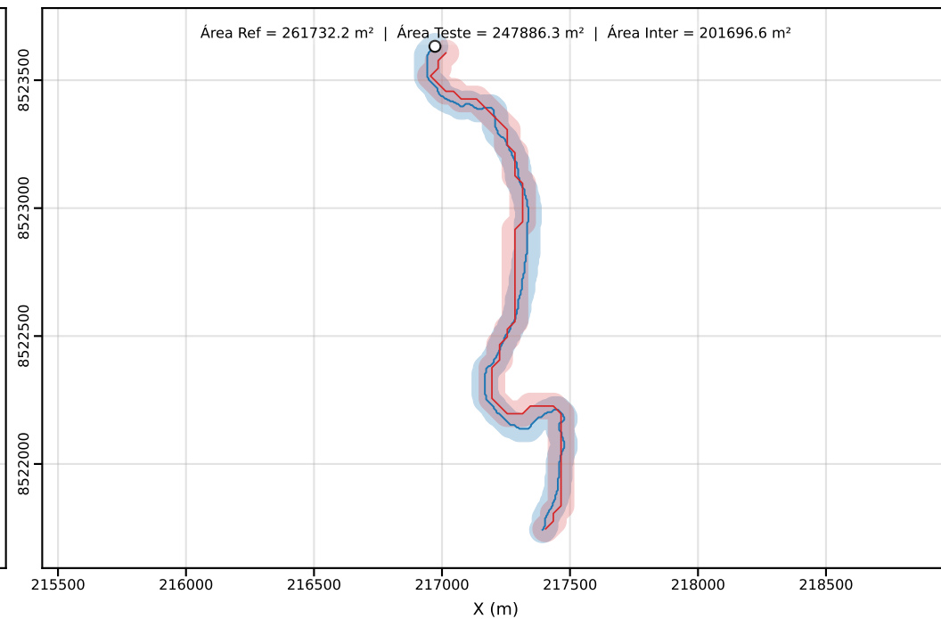
Classe D | PEC-PCD (Horizontal)=50.00 m | dm = 38.04
