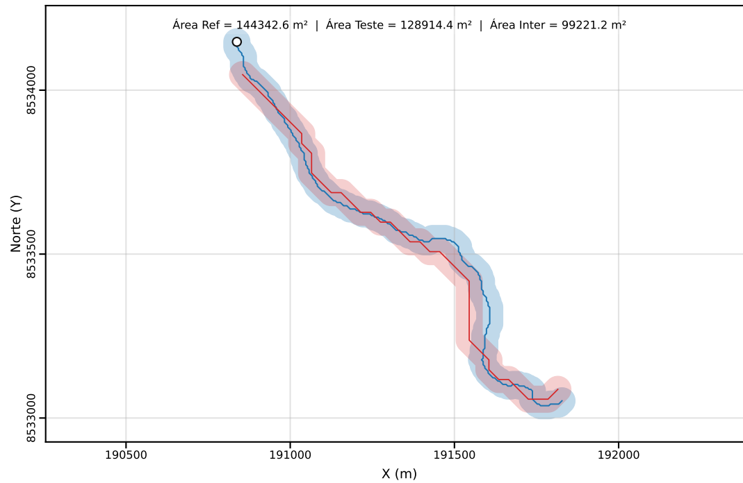
Classe C | PEC-PCD (Horizontal)=40.00 m | dm = 43.98
