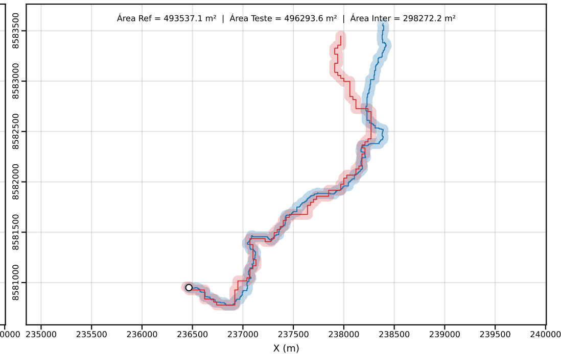
Classe D | PEC-PCD (Horizontal)=50.00 m | dm = 61.80
