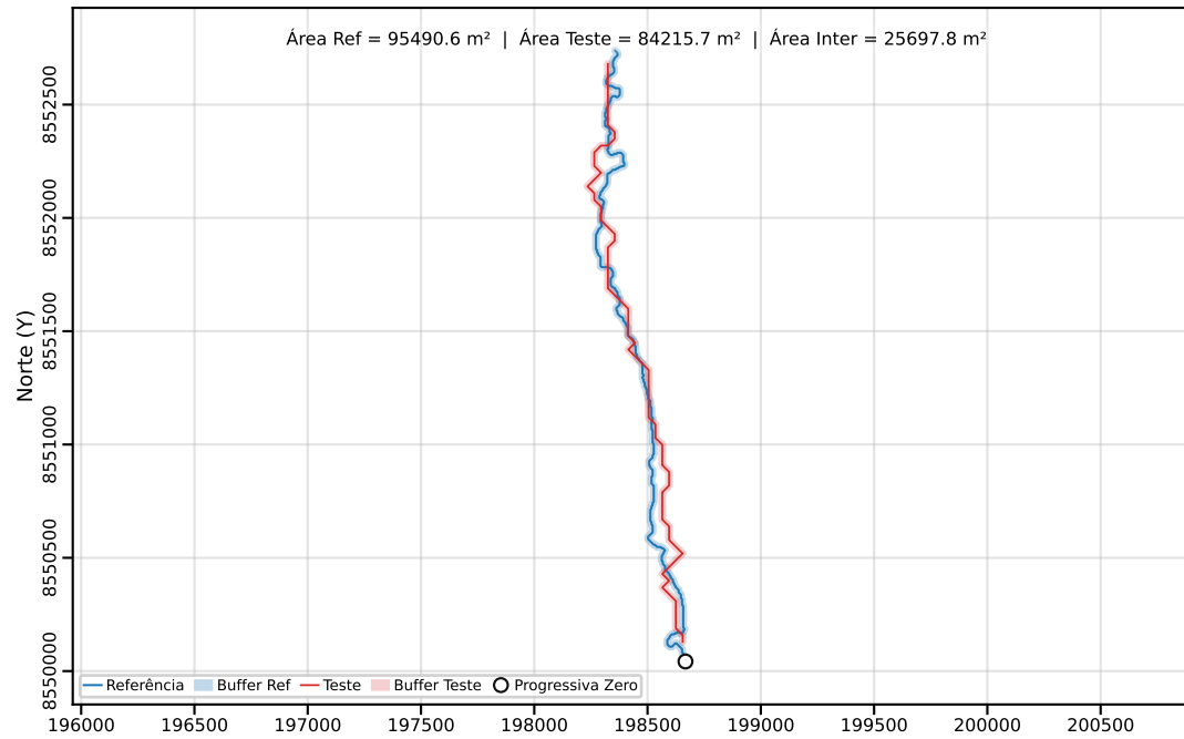
Classe C | PEC-PCD (Horizontal)=40.00 m | dm = 56.47
