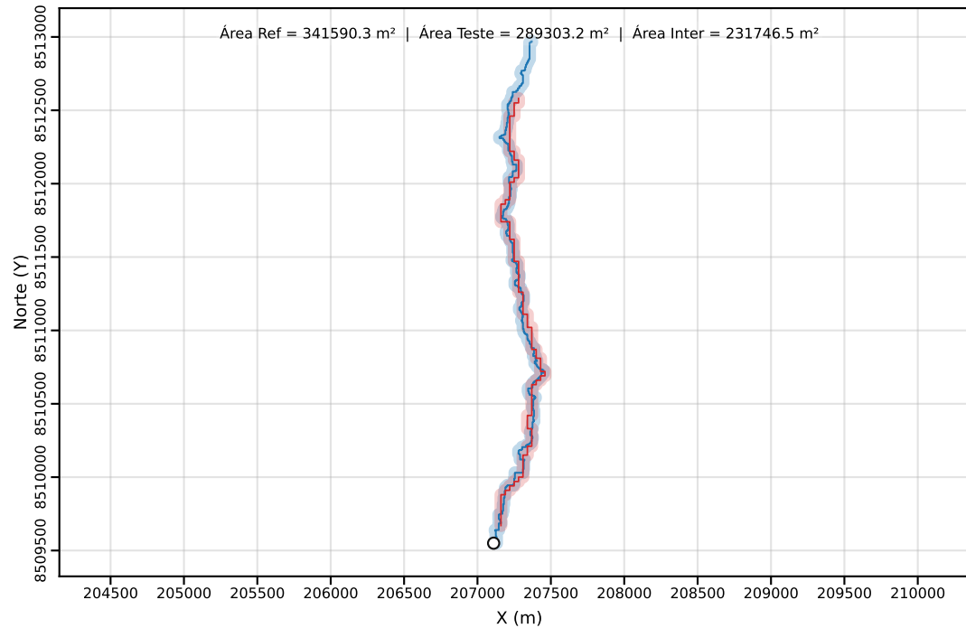
Classe C | PEC-PCD (Horizontal)=40.00 m | dm = 47.71
