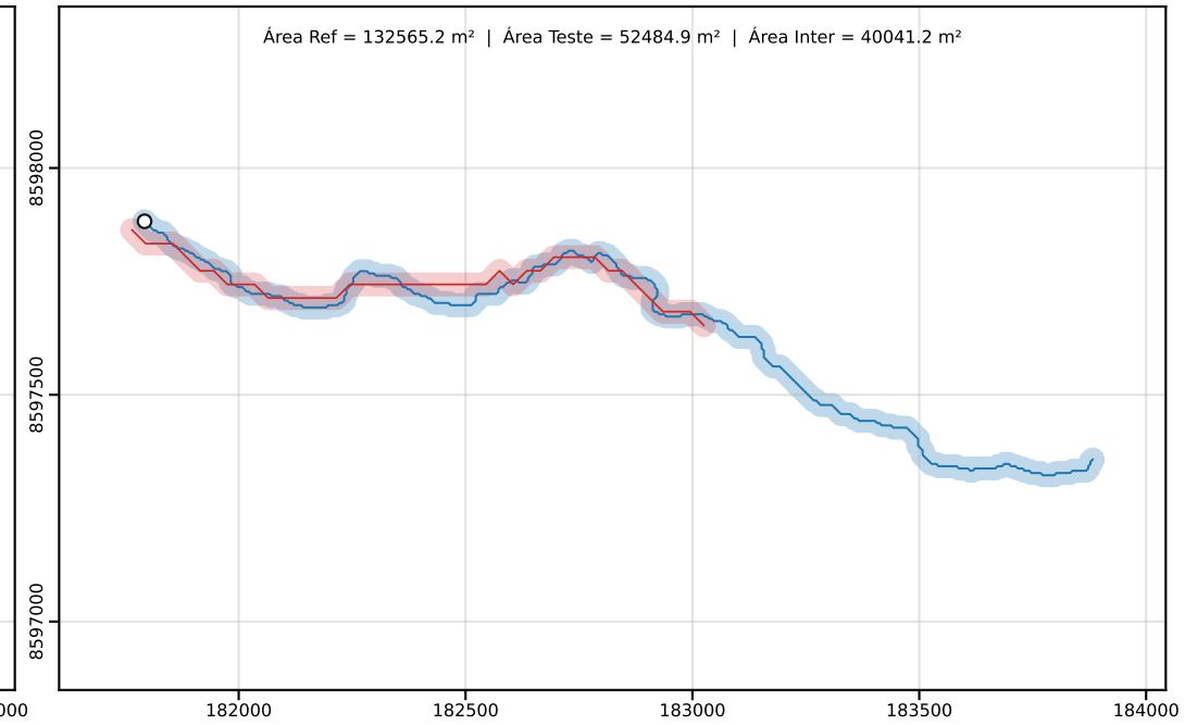
Classe D | PEC-PCD (Horizontal)=50.00 m | dm = 244.28
