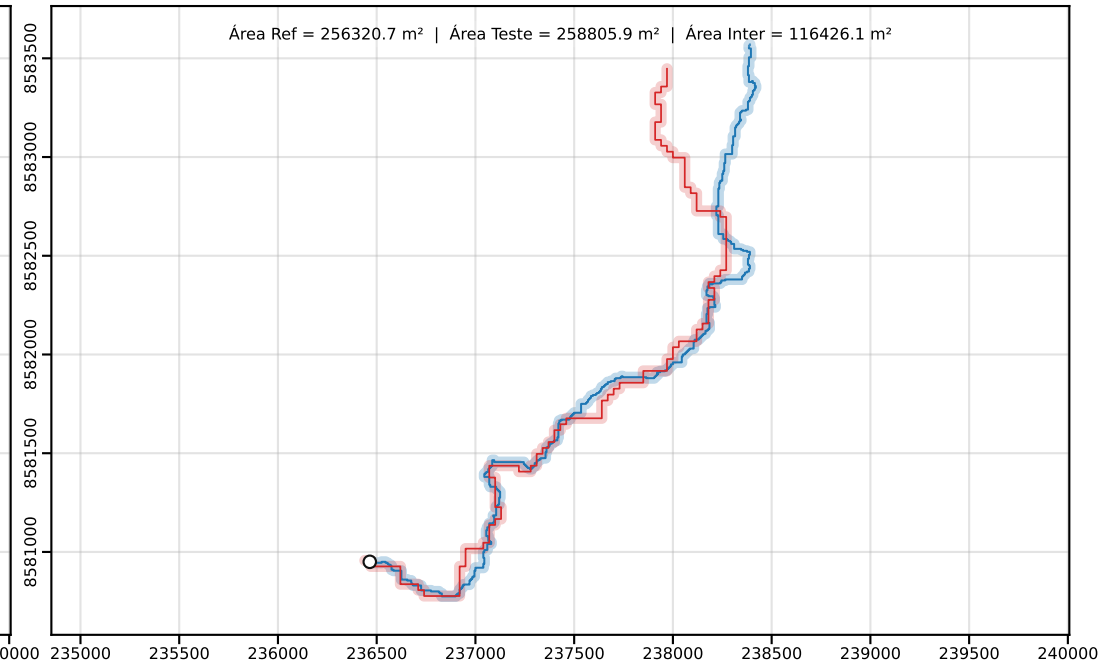
Classe D | PEC-PCD (Horizontal)=50.00 m | dm = 61.80
