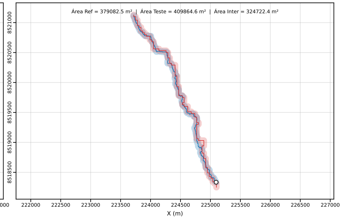
Classe D | PEC-PCD (Horizontal)=50.00 m | dm = 20.83
