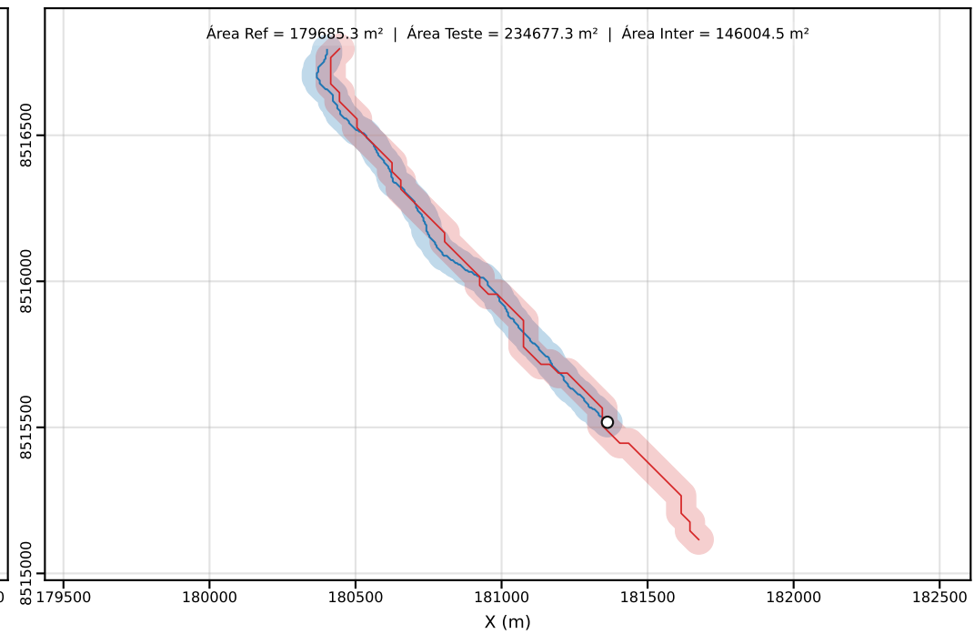
Classe D | PEC-PCD (Horizontal)=50.00 m | dm = 22.54
