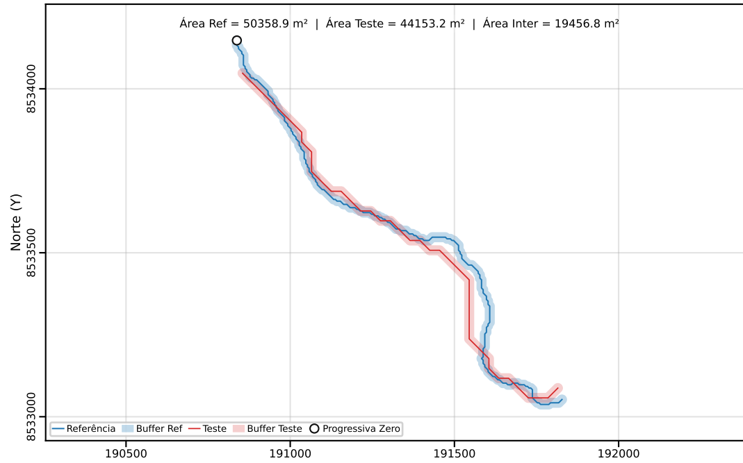
Classe C | PEC-PCD (Horizontal)=40.00 m | dm = 43.98
