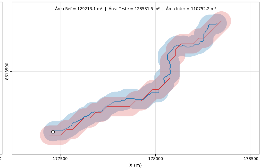
Classe D | PEC-PCD (Horizontal)=50.00 m | dm = 22.55
