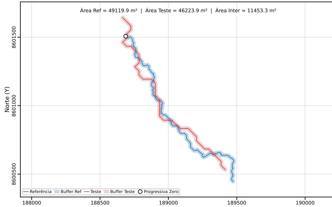
Classe C | PEC-PCD (Horizontal)=40.00 m | dm = 57.16
