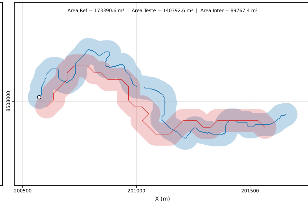
Classe D | PEC-PCD (Horizontal)=50.00 m | dm = 93.56
