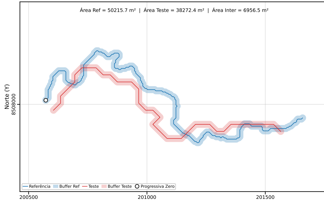
Classe C | PEC-PCD (Horizontal)=40.00 m | dm = 89.58
