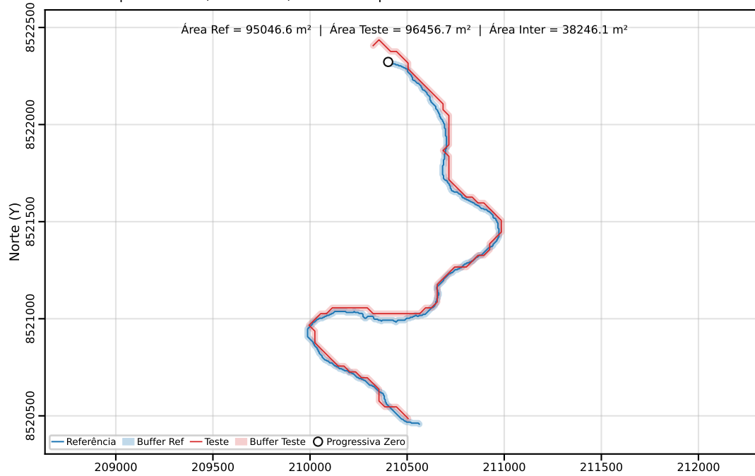
Classe C | PEC-PCD (Horizontal)=40.00 m | dm = 29.16
