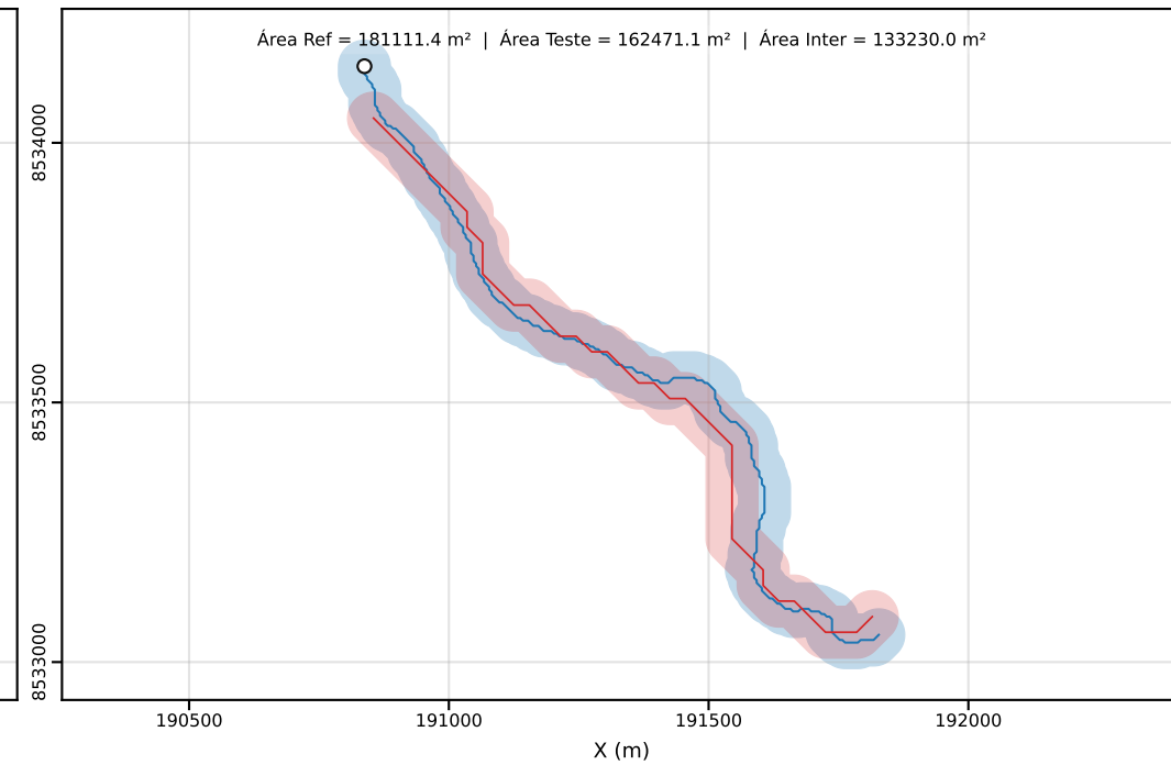
Classe D | PEC-PCD (Horizontal)=50.00 m | dm = 46.29
