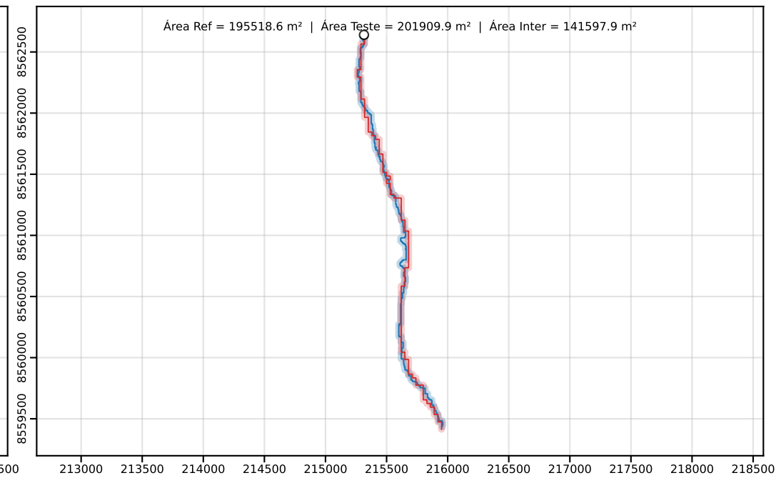
Classe D | PEC-PCD (Horizontal)=50.00 m | dm = 20.28
