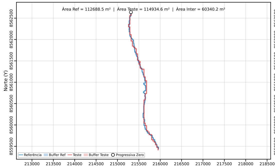
Classe C | PEC-PCD (Horizontal)=40.00 m | dm = 20.49
