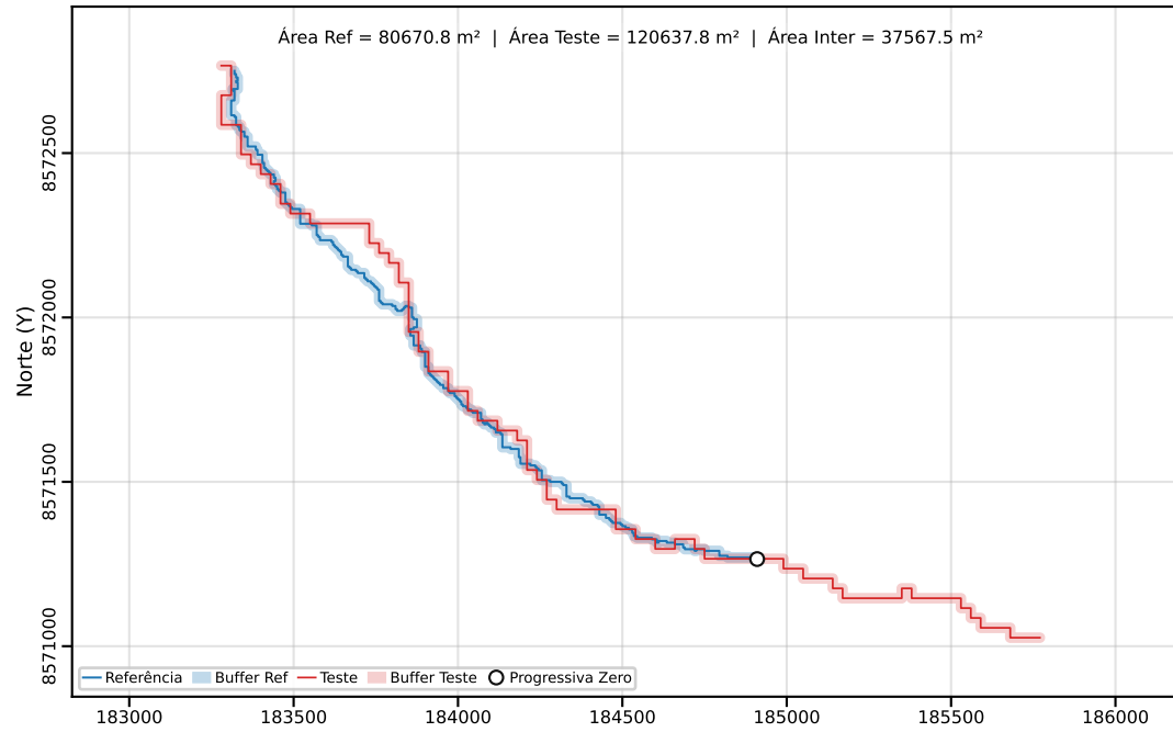
Classe C | PEC-PCD (Horizontal)=40.00 m | dm = 19.69
