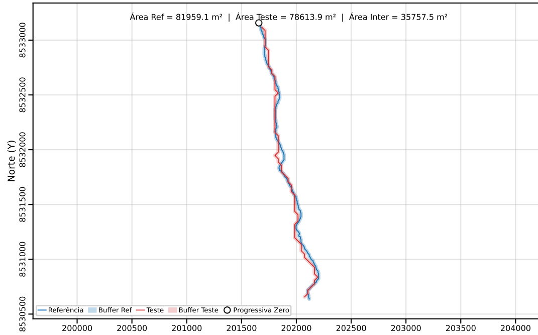
Classe C | PEC-PCD (Horizontal)=40.00 m | dm = 30.90
