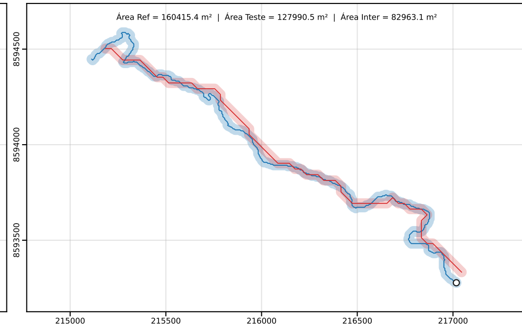
Classe D | PEC-PCD (Horizontal)=50.00 m | dm = 58.19
