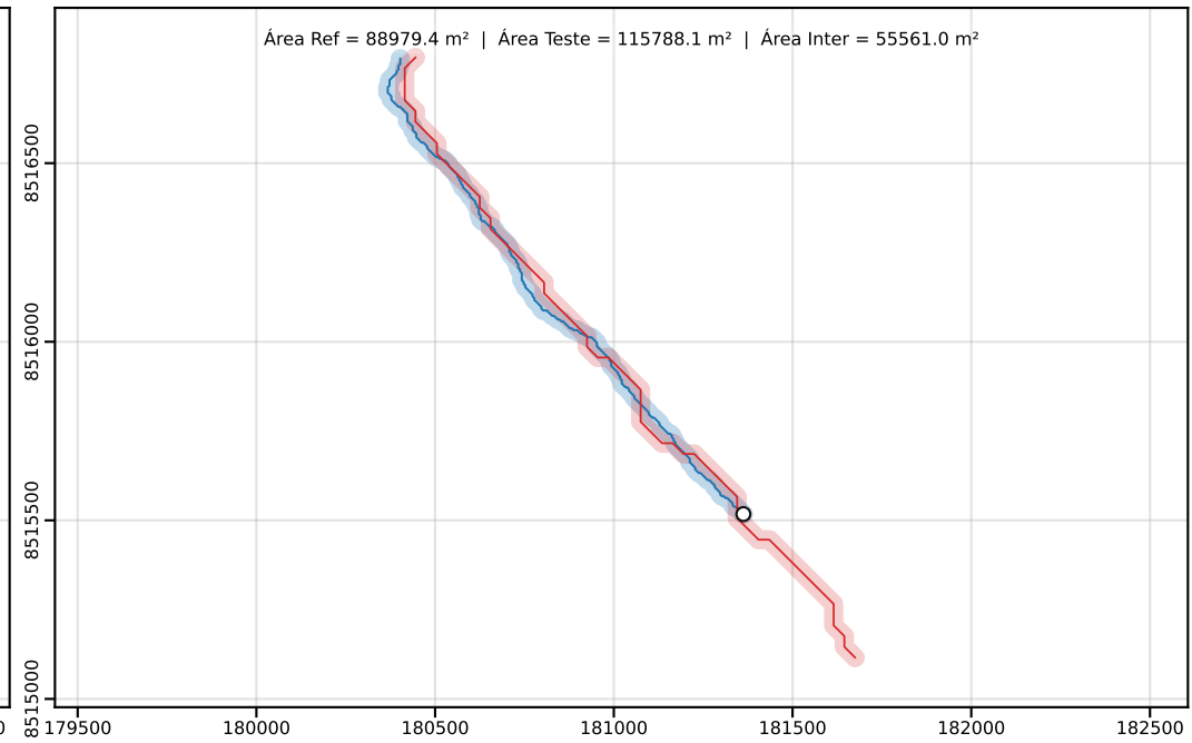
Classe D | PEC-PCD (Horizontal)=50.00 m | dm = 22.54
