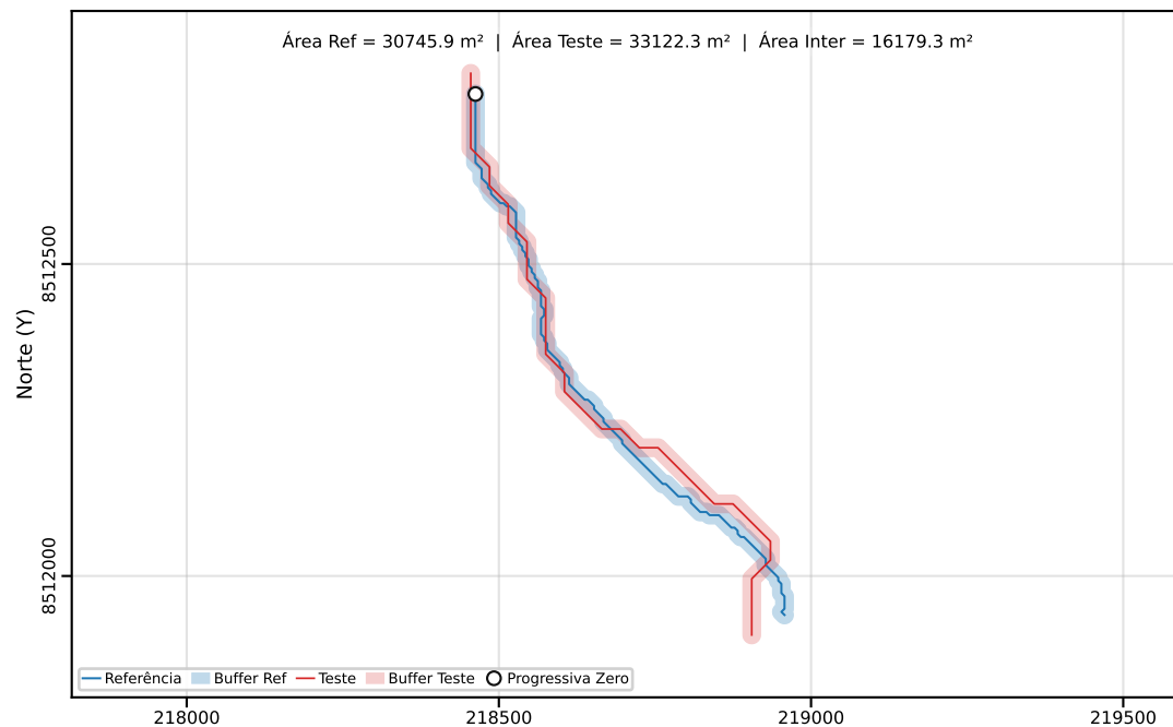
Classe C | PEC-PCD (Horizontal)=40.00 m | dm = 20.70
