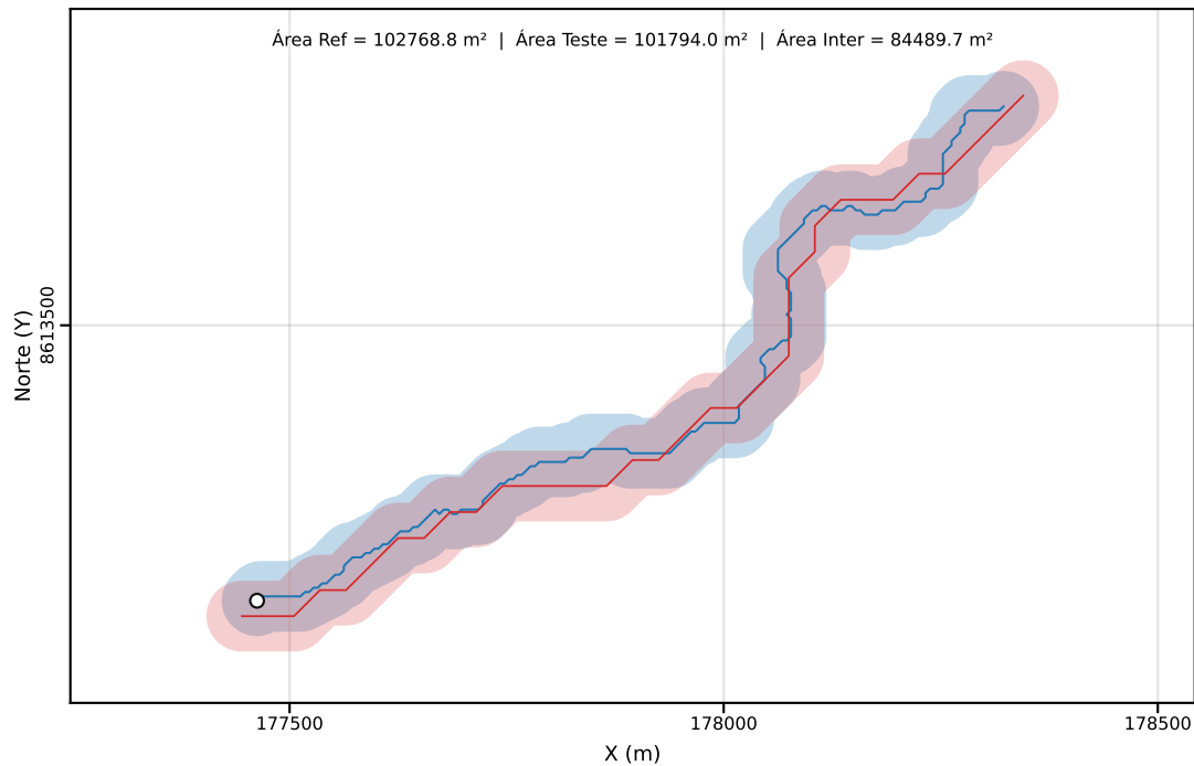
Classe C | PEC-PCD (Horizontal)=40.00 m | dm = 22.57
