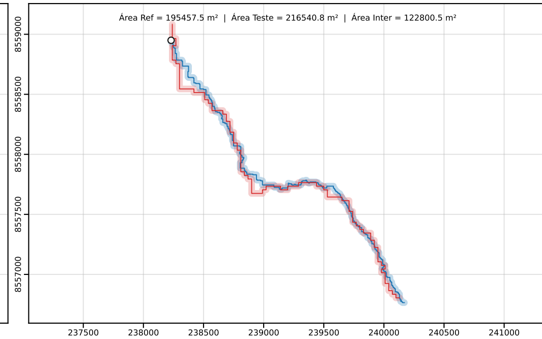
Classe D | PEC-PCD (Horizontal)=50.00 m | dm = 28.53
