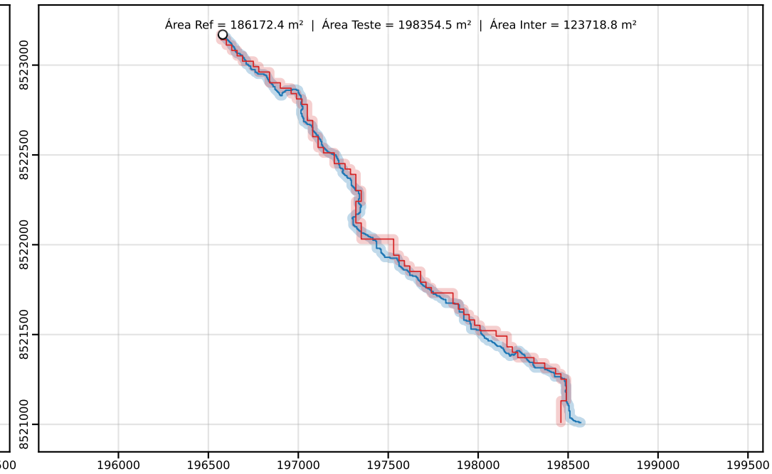
Classe D | PEC-PCD (Horizontal)=50.00 m | dm = 25.81
