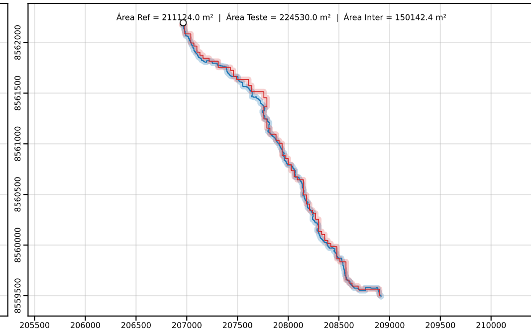
Classe D | PEC-PCD (Horizontal)=50.00 m | dm = 20.27
