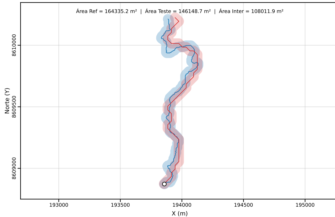
Classe C | PEC-PCD (Horizontal)=40.00 m | dm = 48.43
