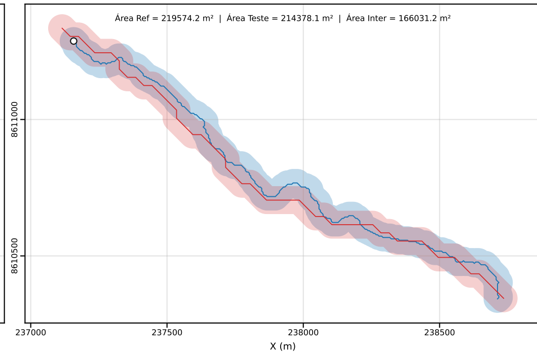
Classe D | PEC-PCD (Horizontal)=50.00 m | dm = 39.23
