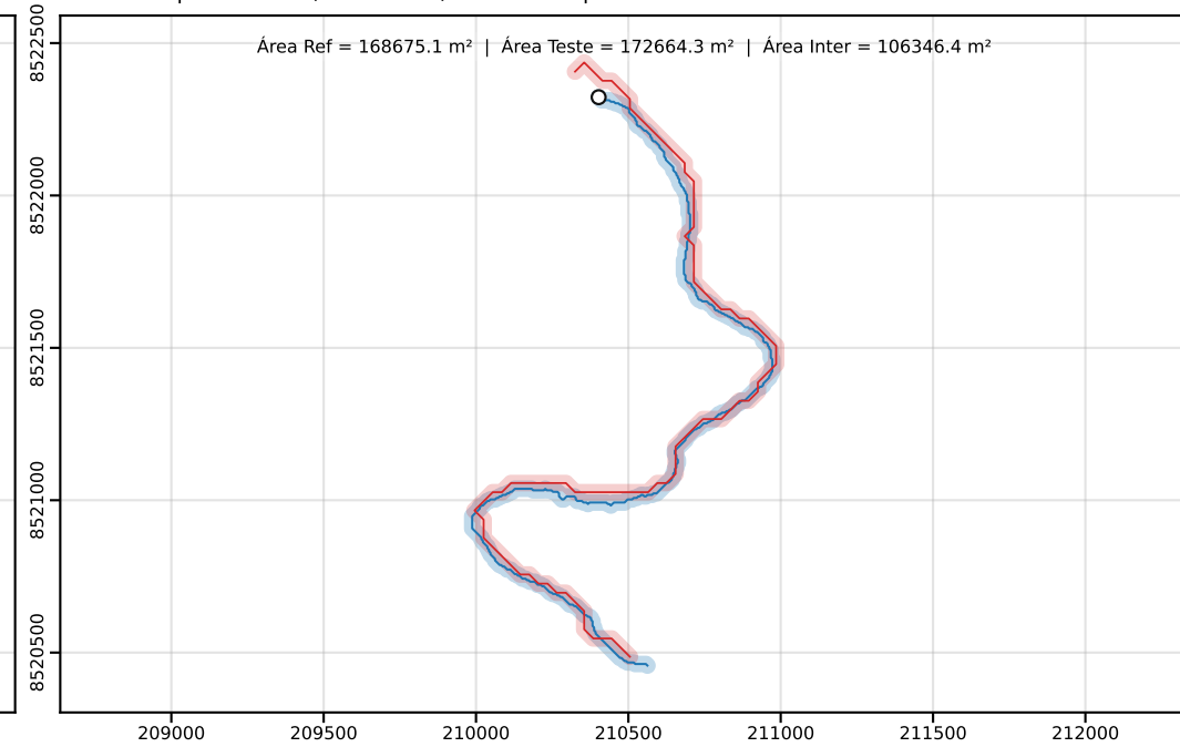
Classe D | PEC-PCD (Horizontal)=50.00 m | dm = 29.45
