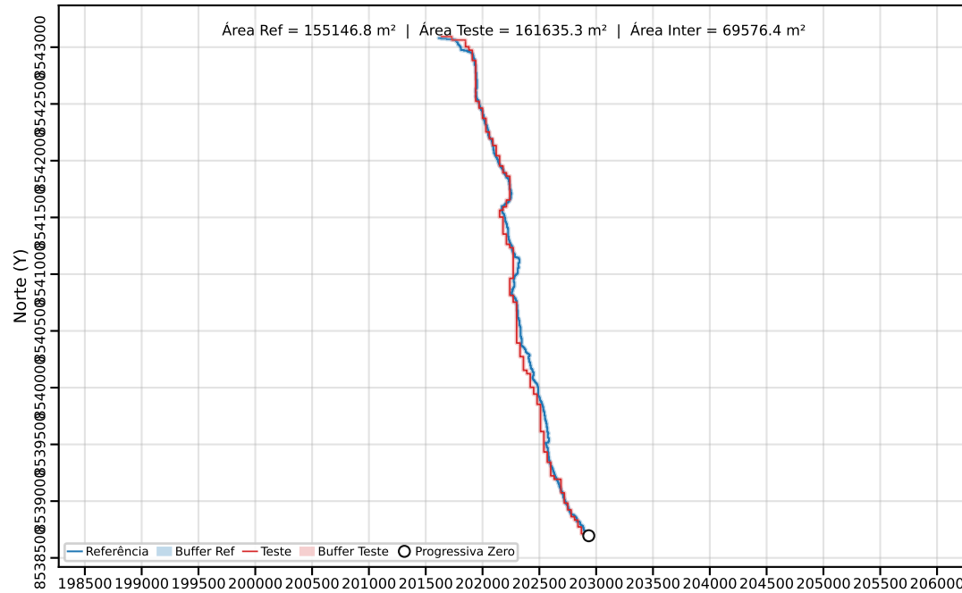
Classe C | PEC-PCD (Horizontal)=40.00 m | dm = 26.75
