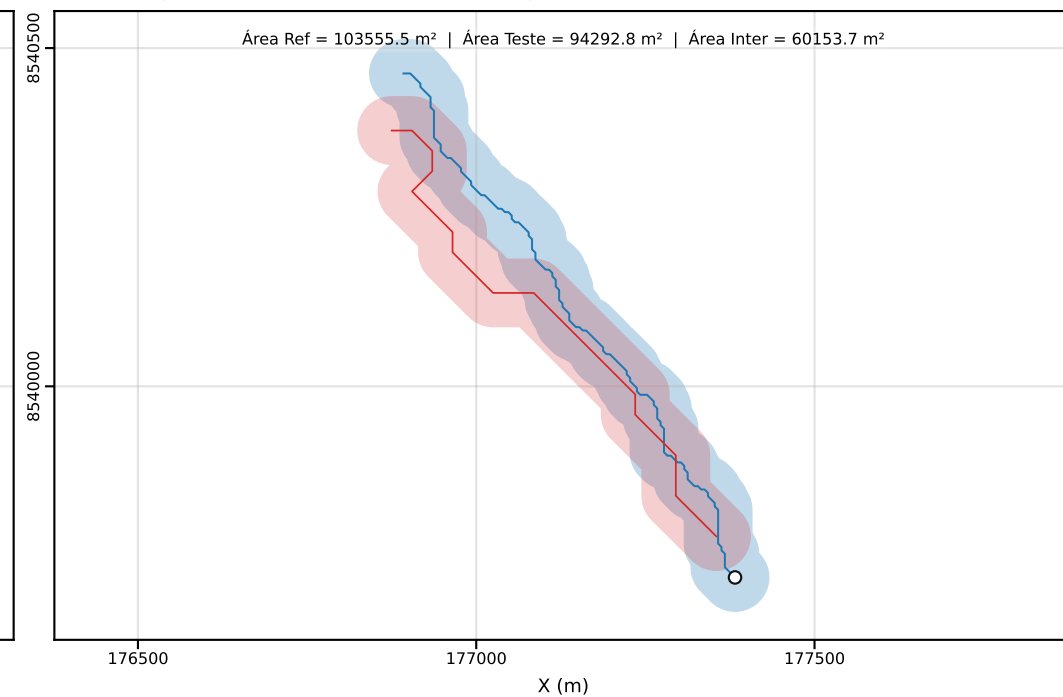
Classe D | PEC-PCD (Horizontal)=50.00 m | dm = 72.30
