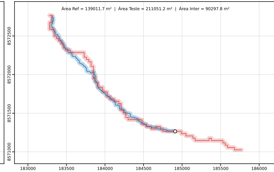
Classe D | PEC-PCD (Horizontal)=50.00 m | dm = 19.31
