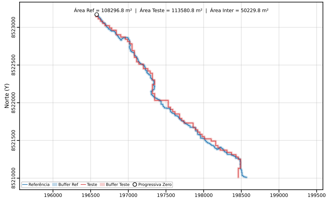
Classe C | PEC-PCD (Horizontal)=40.00 m | dm = 25.44
