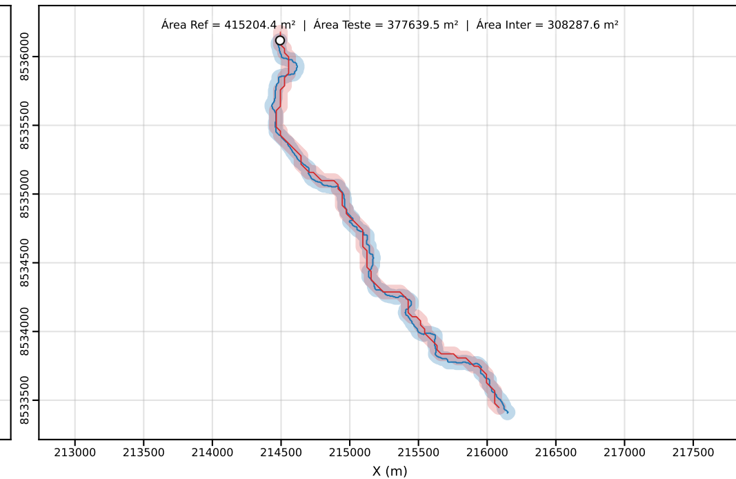
Classe D | PEC-PCD (Horizontal)=50.00 m | dm = 44.47
