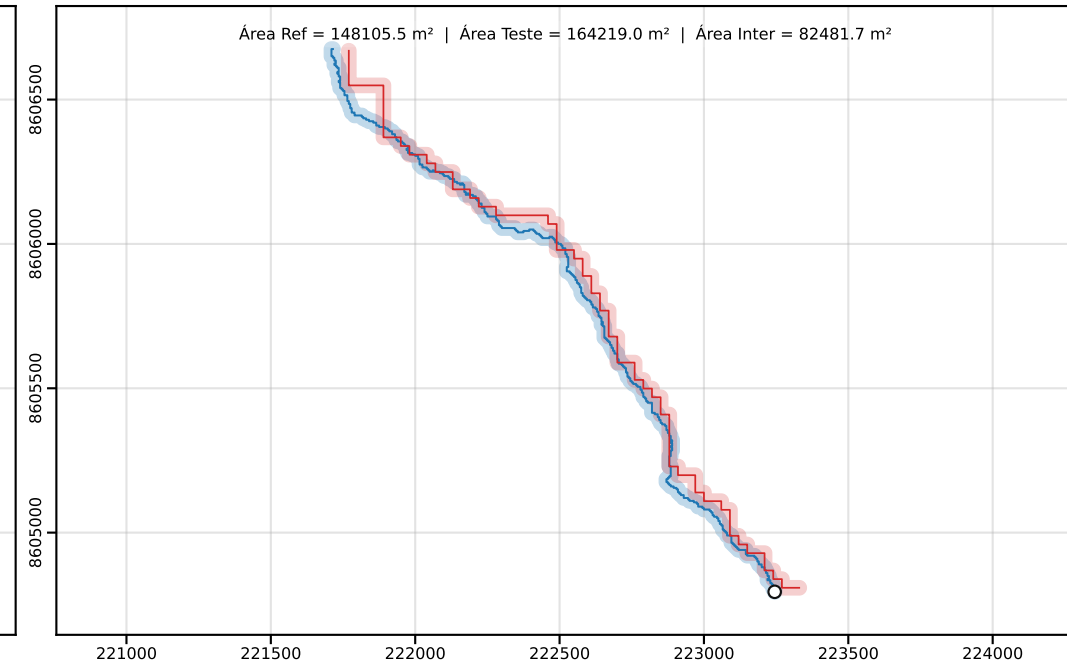
Classe D | PEC-PCD (Horizontal)=50.00 m | dm = 33.39
