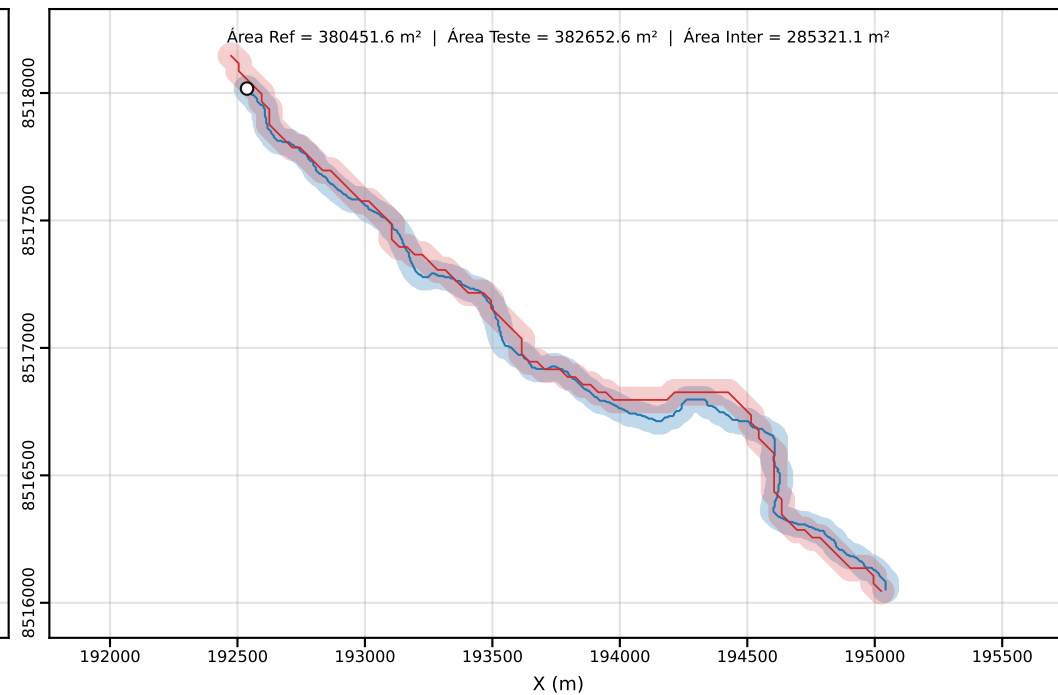
Classe D | PEC-PCD (Horizontal)=50.00 m | dm = 39.05
