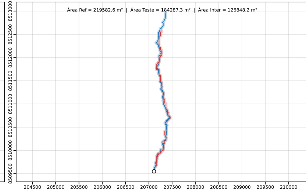
Classe D | PEC-PCD (Horizontal)=50.00 m | dm = 53.11
