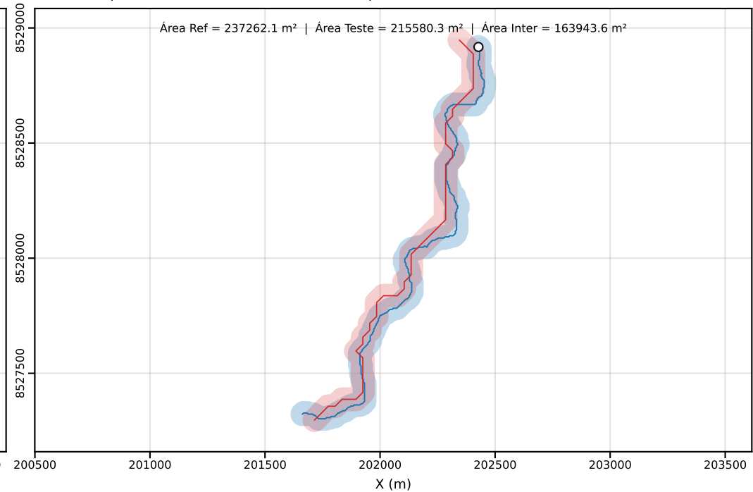
Classe D | PEC-PCD (Horizontal)=50.00 m | dm = 53.42
