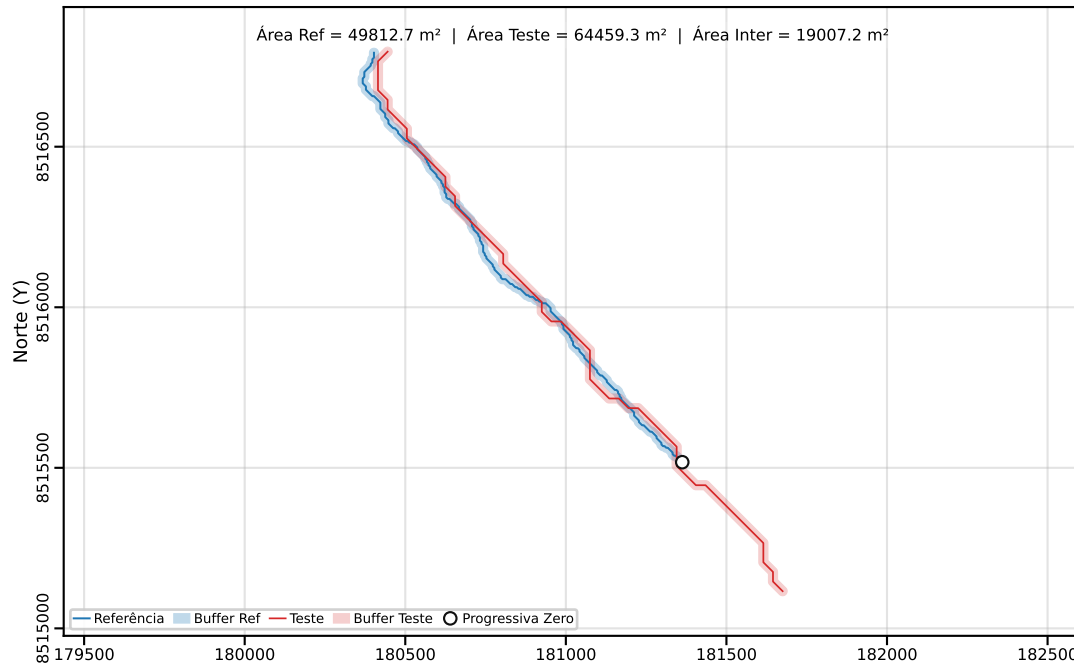
Classe C | PEC-PCD (Horizontal)=40.00 m | dm = 22.64
