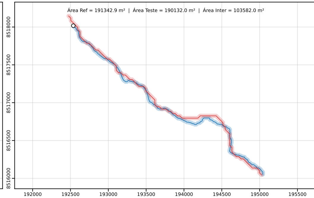
Classe D | PEC-PCD (Horizontal)=50.00 m | dm = 39.05
