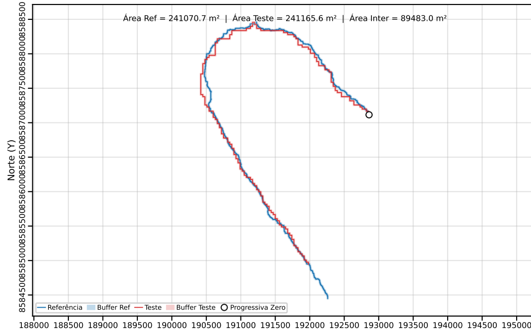
Classe C | PEC-PCD (Horizontal)=40.00 m | dm = 40.35
