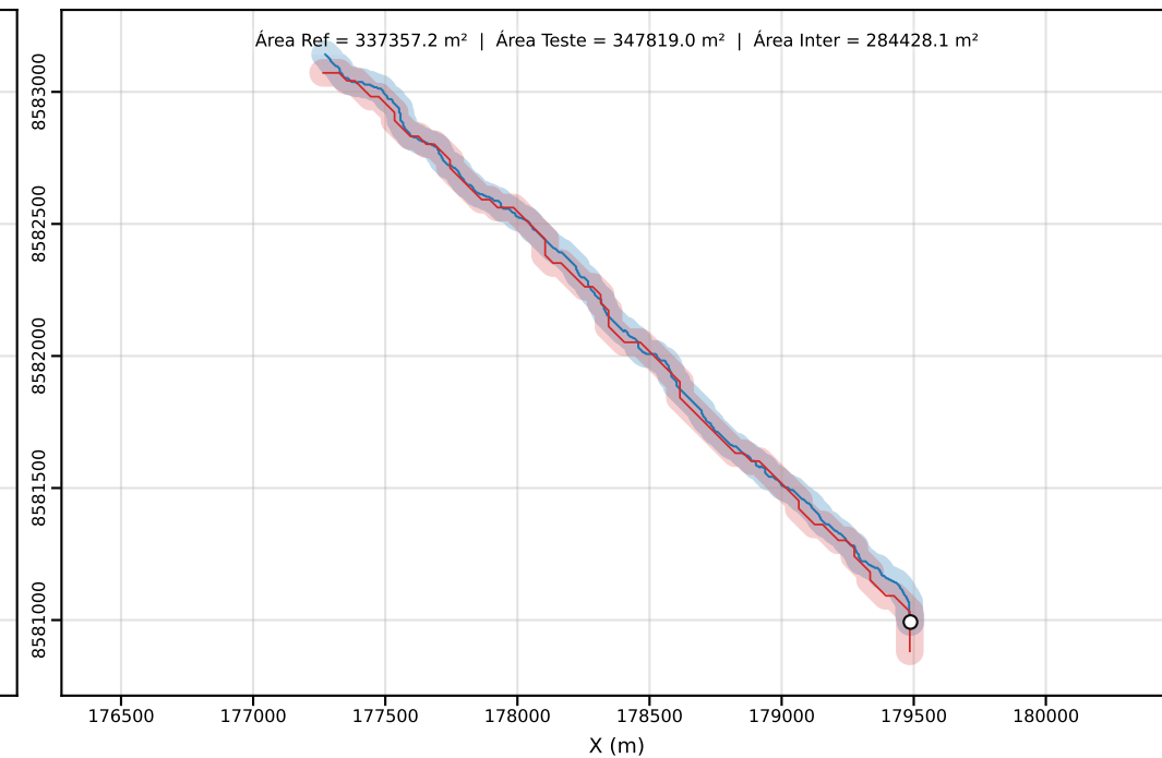
Classe D | PEC-PCD (Horizontal)=50.00 m | dm = 23.90
