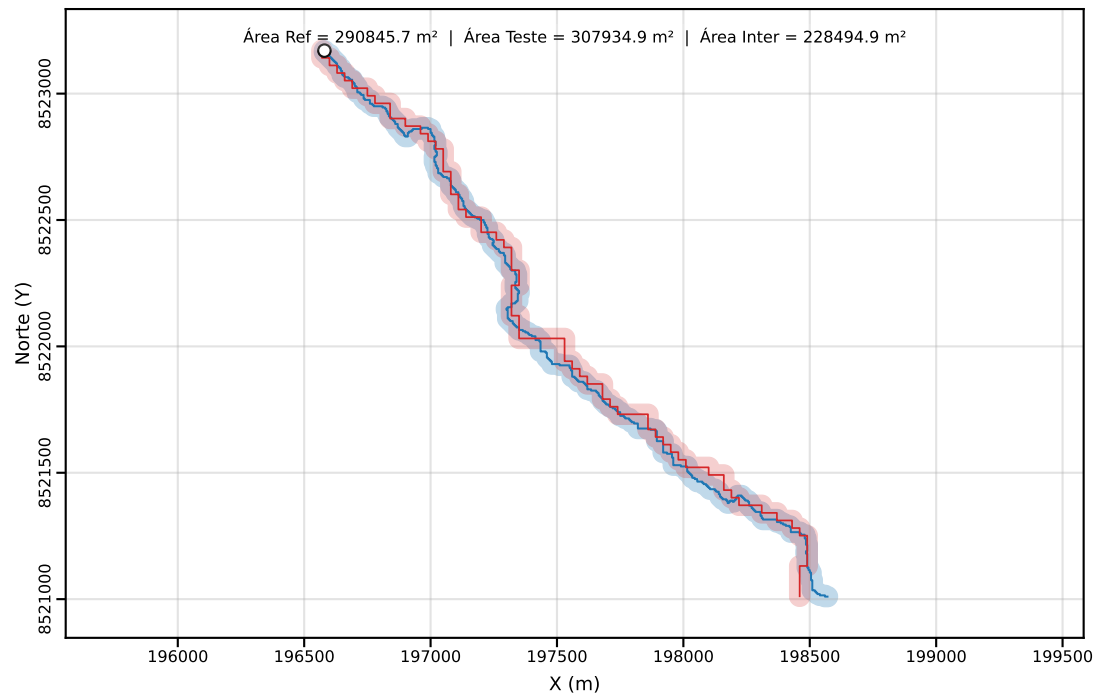
Classe C | PEC-PCD (Horizontal)=40.00 m | dm = 25.44
