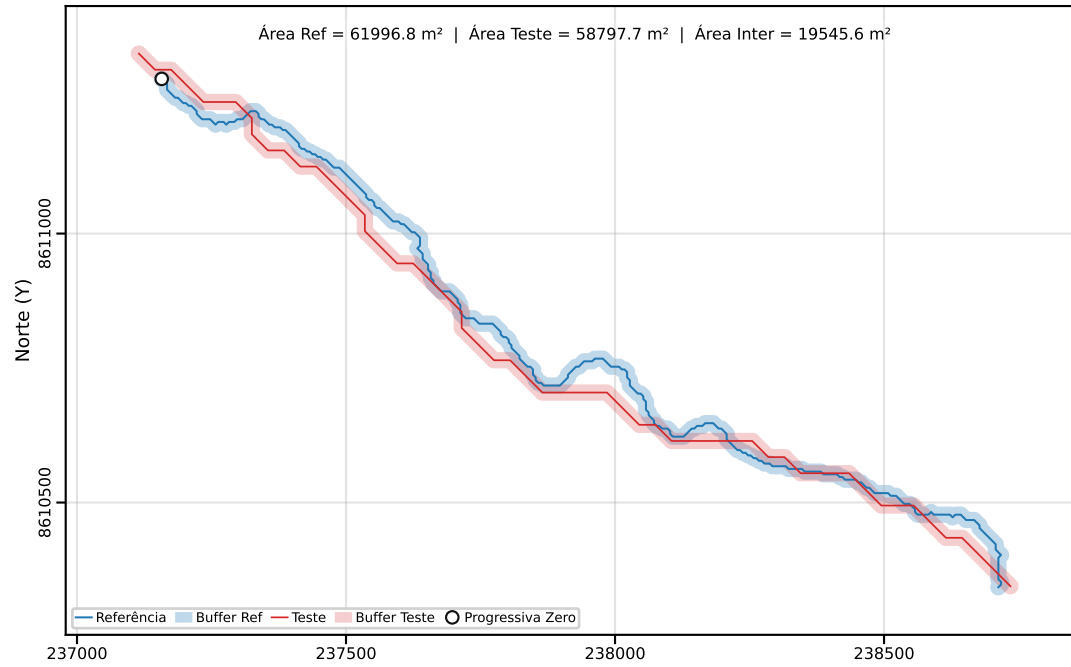
Classe C | PEC-PCD (Horizontal)=40.00 m | dm = 39.13
