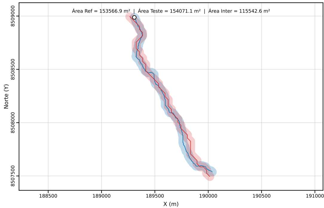
Classe C | PEC-PCD (Horizontal)=40.00 m | dm = 31.01
