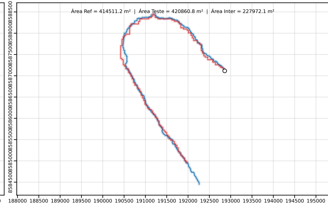
Classe D | PEC-PCD (Horizontal)=50.00 m | dm = 43.24
