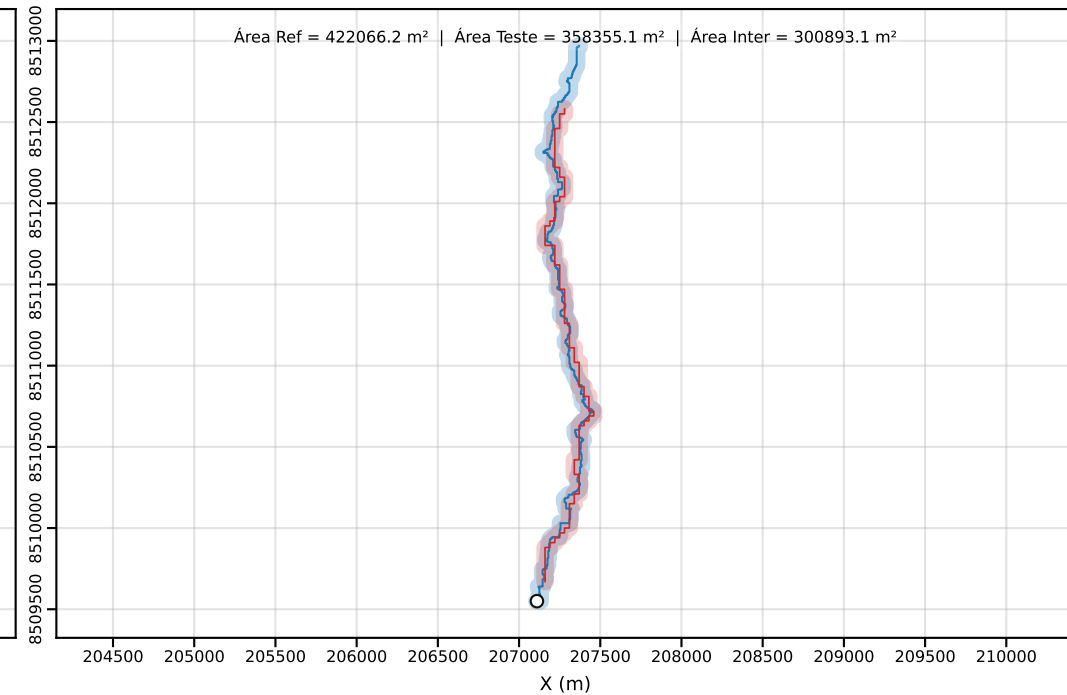
Classe D | PEC-PCD (Horizontal)=50.00 m | dm = 53.11
