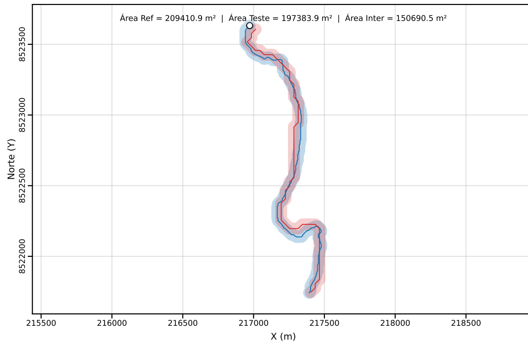
Classe C | PEC-PCD (Horizontal)=40.00 m | dm = 37.38
