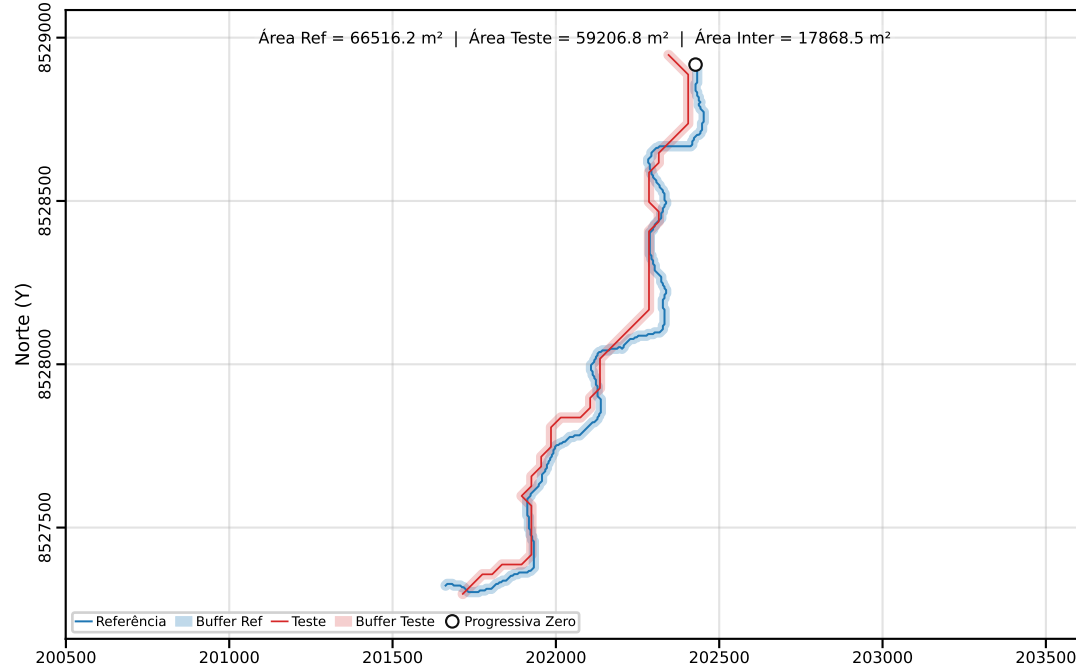
Classe C | PEC-PCD (Horizontal)=40.00 m | dm = 51.35
