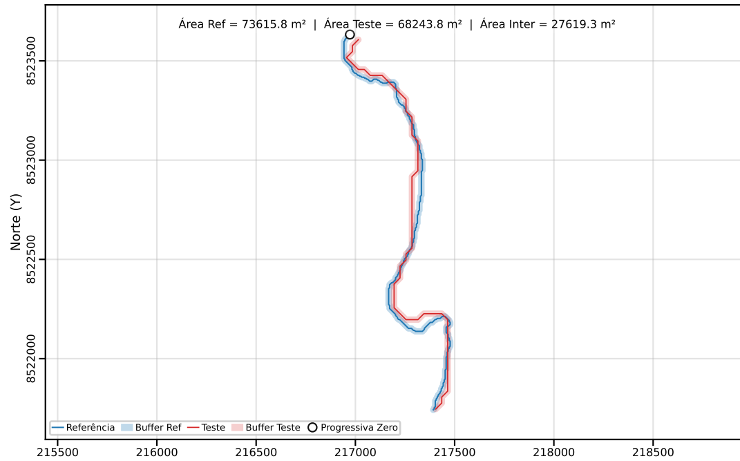
Classe C | PEC-PCD (Horizontal)=40.00 m | dm = 37.38
