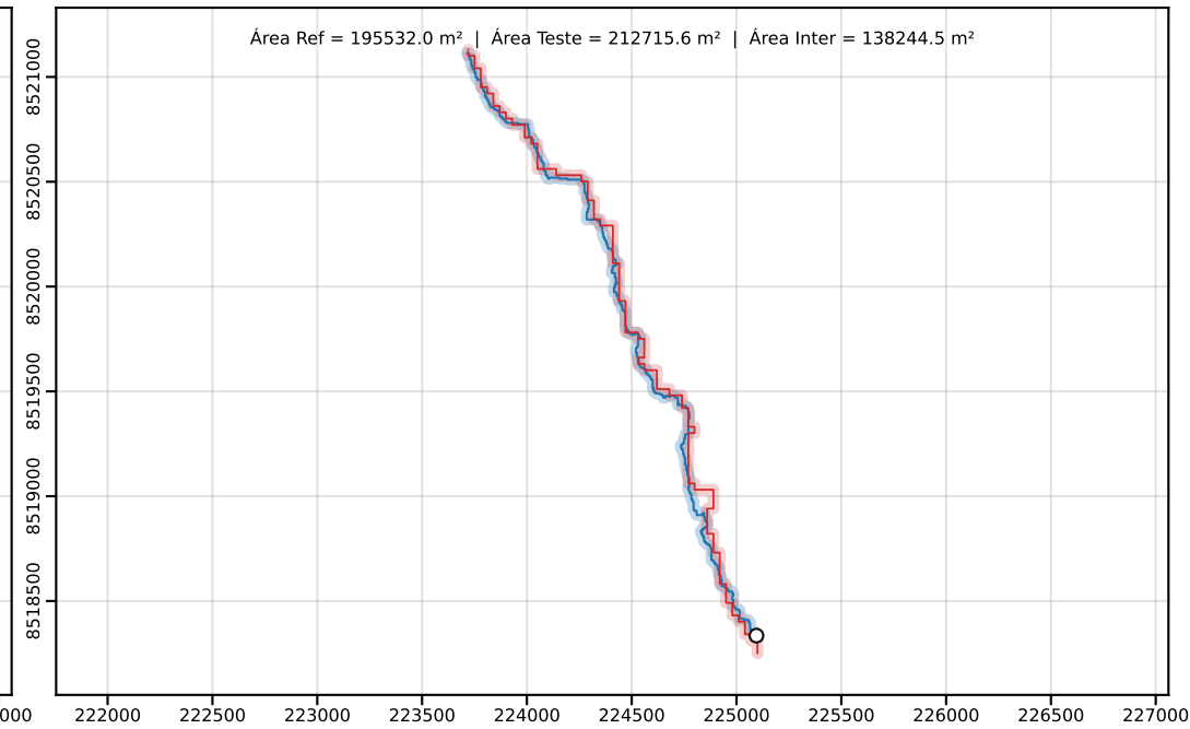
Classe D | PEC-PCD (Horizontal)=50.00 m | dm = 20.83
