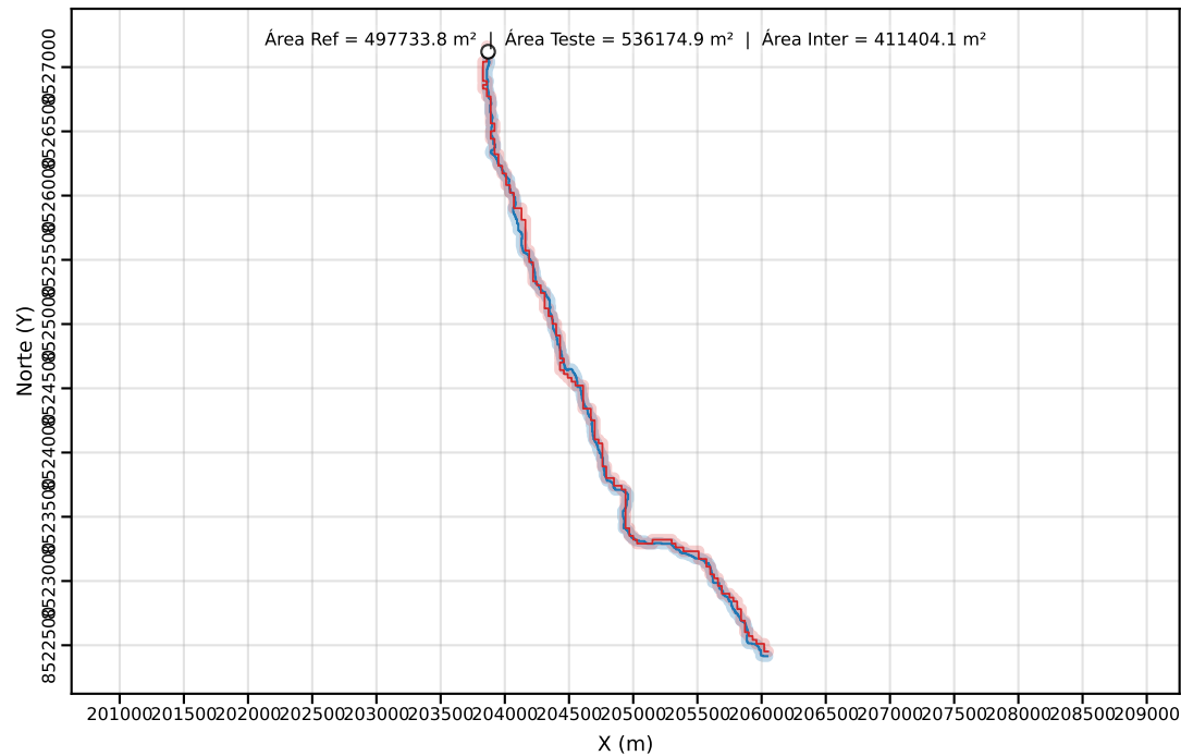
Classe C | PEC-PCD (Horizontal)=40.00 m | dm = 20.23
