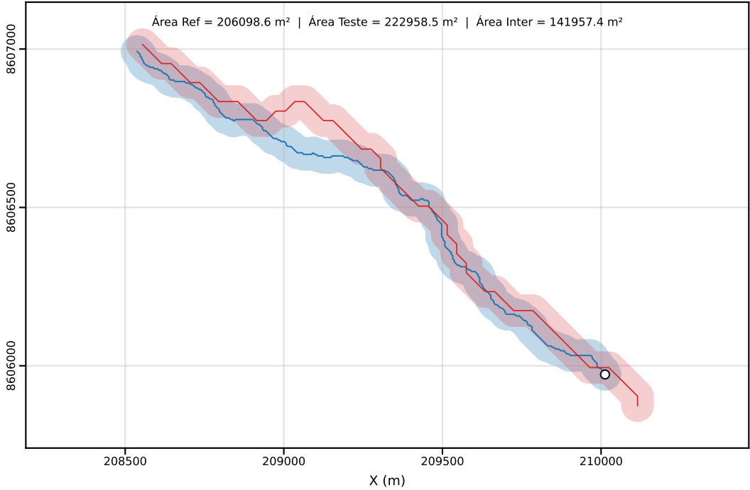
Classe D | PEC-PCD (Horizontal)=50.00 m | dm = 45.19
