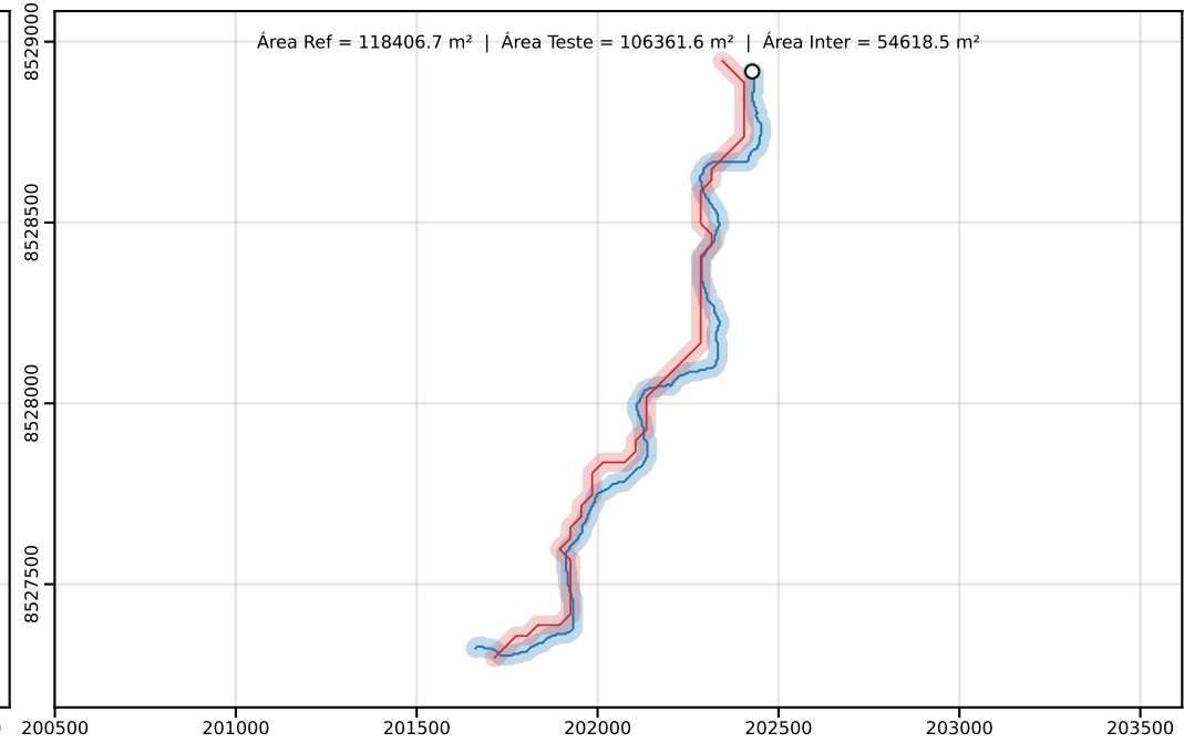
Classe D | PEC-PCD (Horizontal)=50.00 m | dm = 53.42
