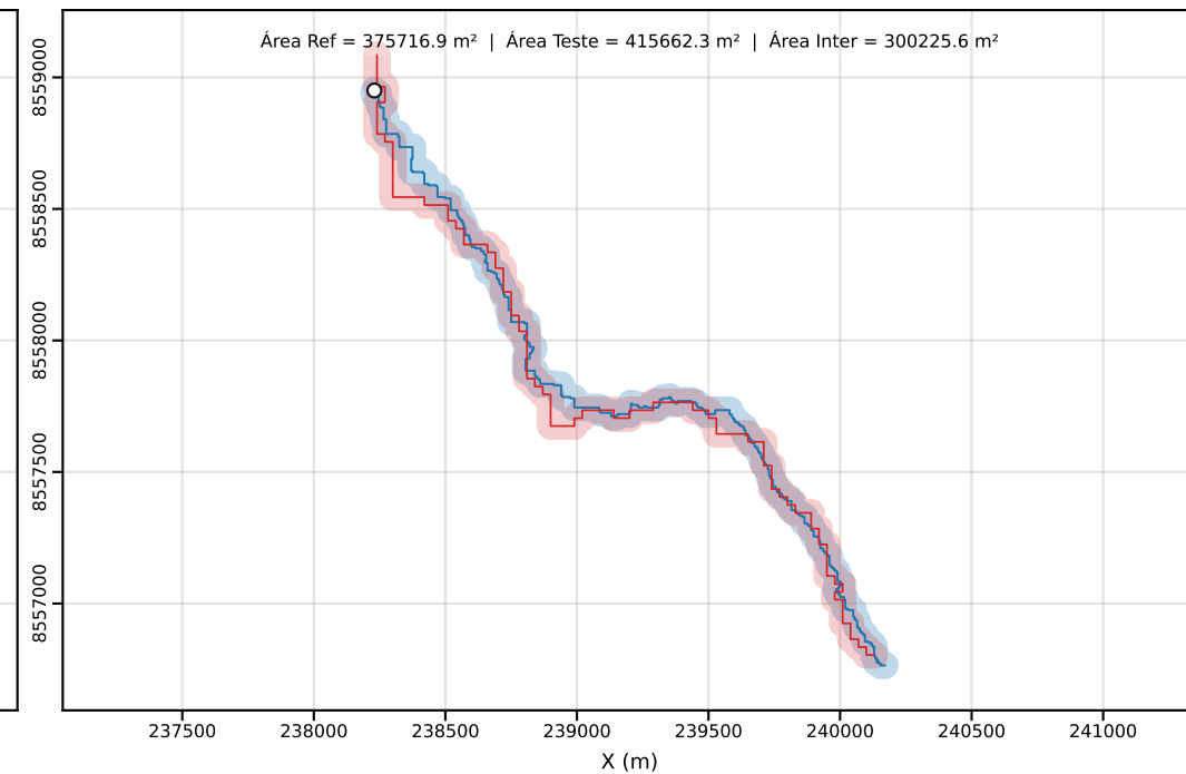
Classe D | PEC-PCD (Horizontal)=50.00 m | dm = 28.53
