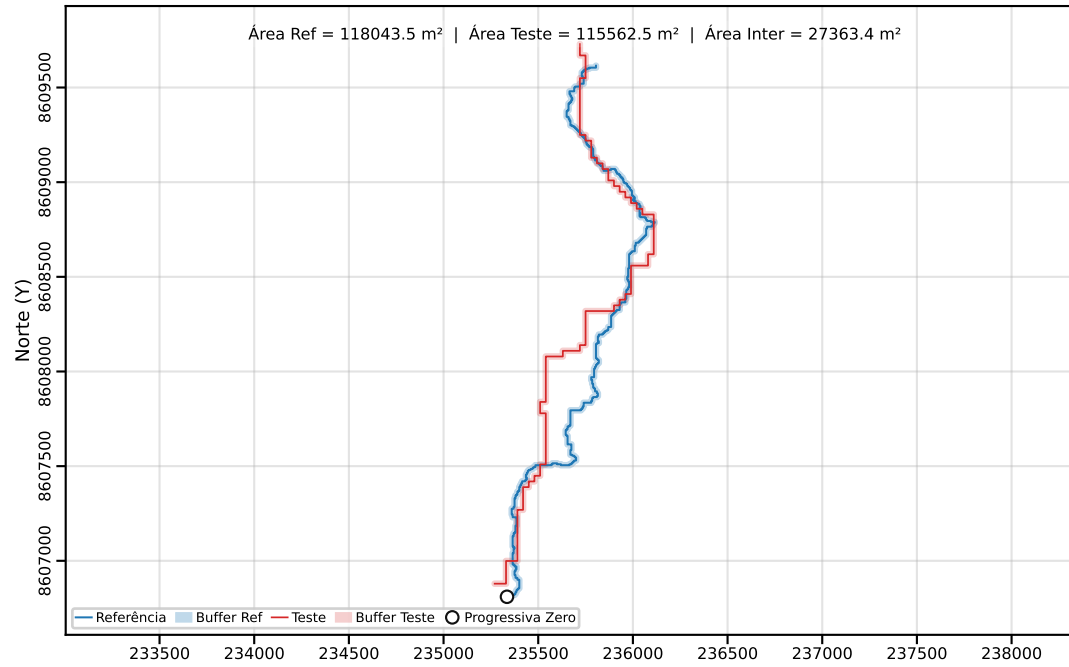
Classe C | PEC-PCD (Horizontal)=40.00 m | dm = 65.42
