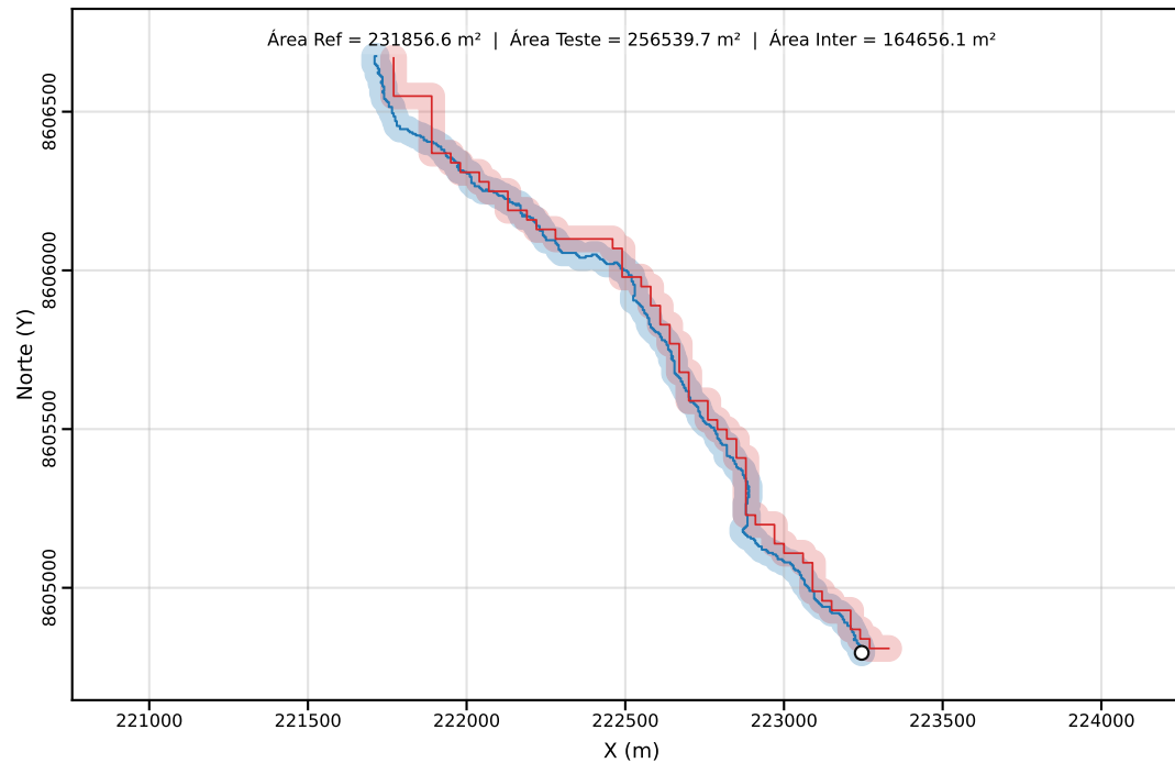
Classe C | PEC-PCD (Horizontal)=40.00 m | dm = 32.92
