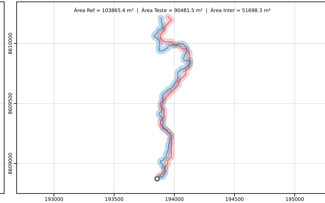
Classe D | PEC-PCD (Horizontal)=50.00 m | dm = 49.51
