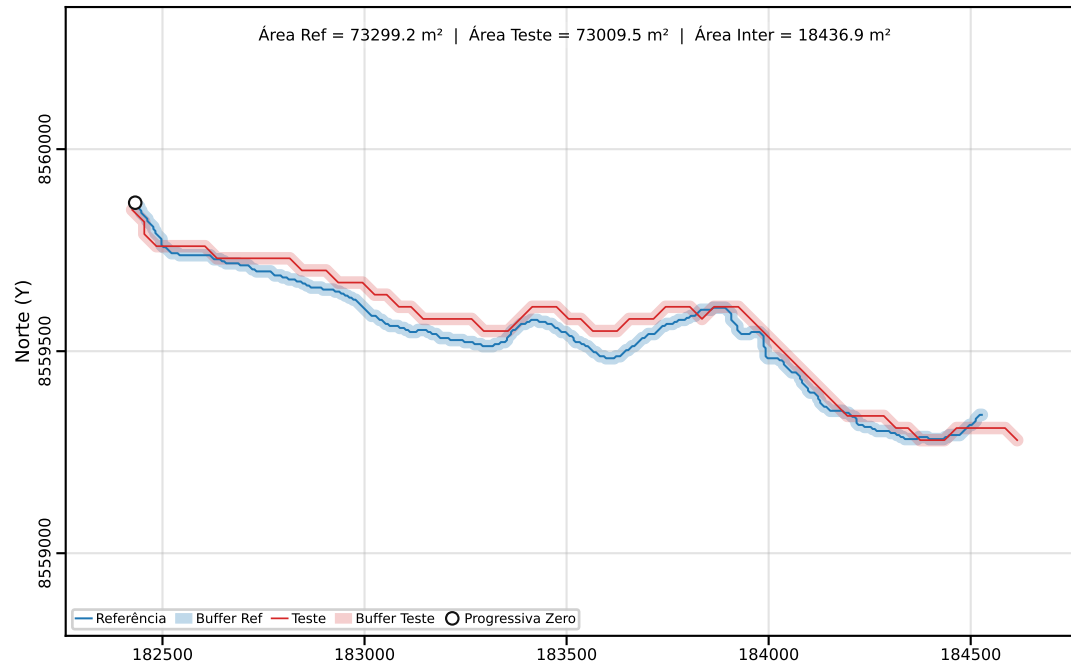
Classe C | PEC-PCD (Horizontal)=40.00 m | dm = 42.91
