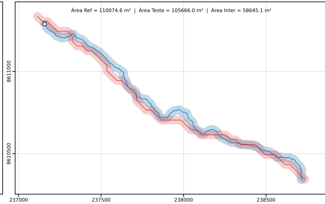
Classe D | PEC-PCD (Horizontal)=50.00 m | dm = 39.23
