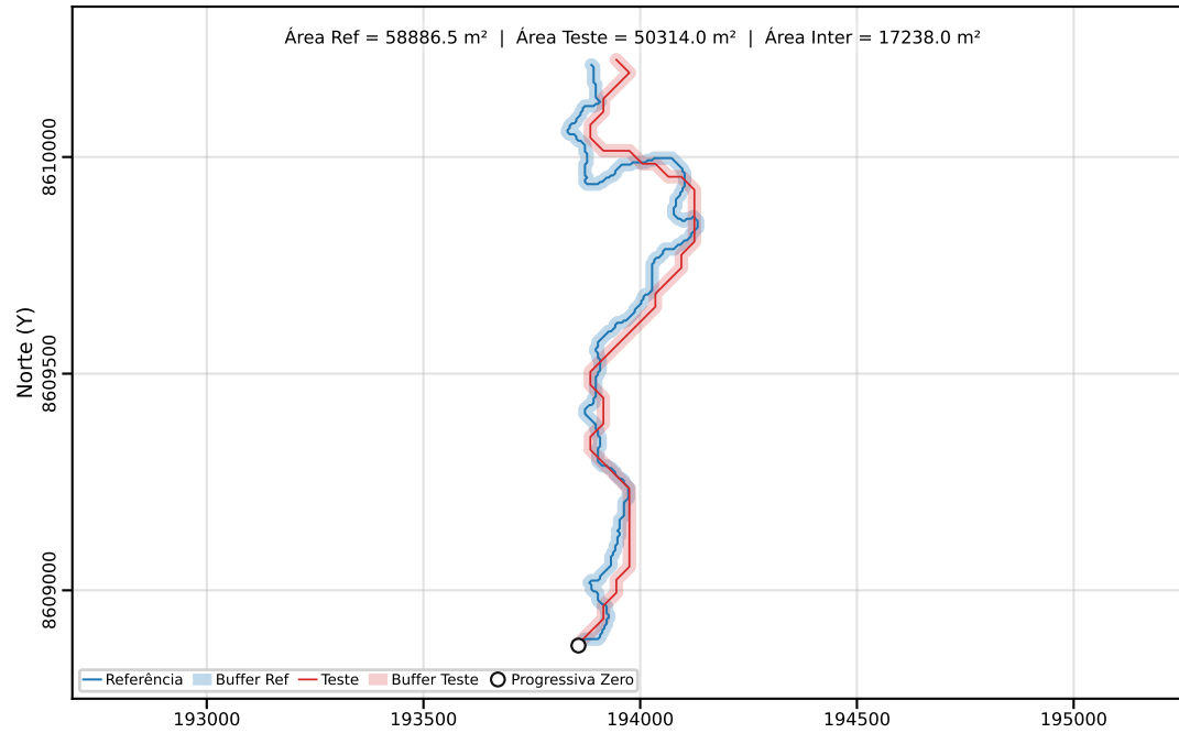
Classe C | PEC-PCD (Horizontal)=40.00 m | dm = 48.43
