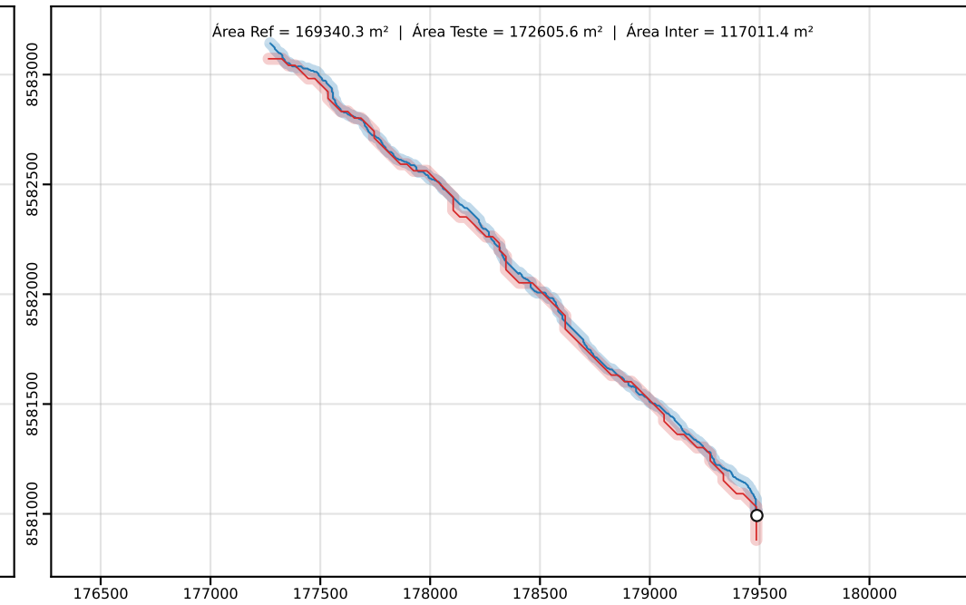
Classe D | PEC-PCD (Horizontal)=50.00 m | dm = 23.90
