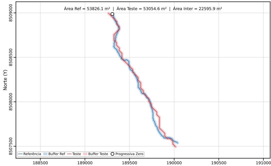
Classe C | PEC-PCD (Horizontal)=40.00 m | dm = 31.01
