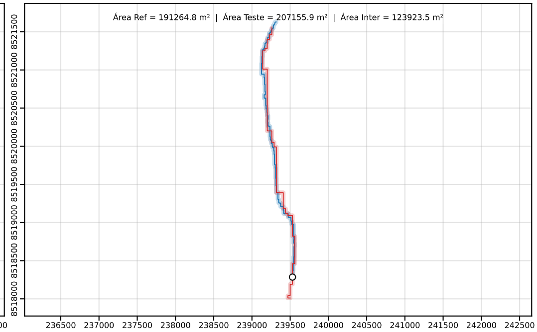
Classe D | PEC-PCD (Horizontal)=50.00 m | dm = 27.03
