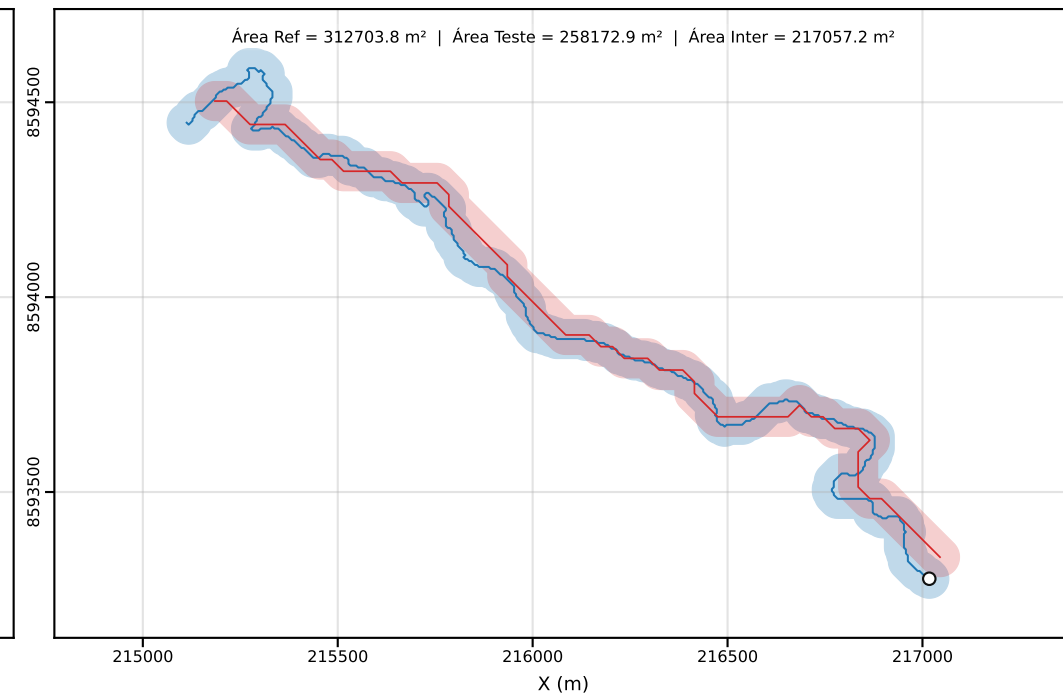
Classe D | PEC-PCD (Horizontal)=50.00 m | dm = 58.19
