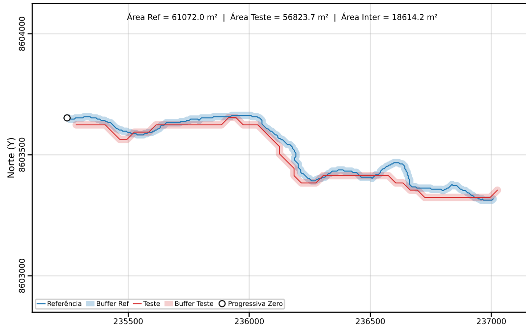
Classe C | PEC-PCD (Horizontal)=40.00 m | dm = 40.57
