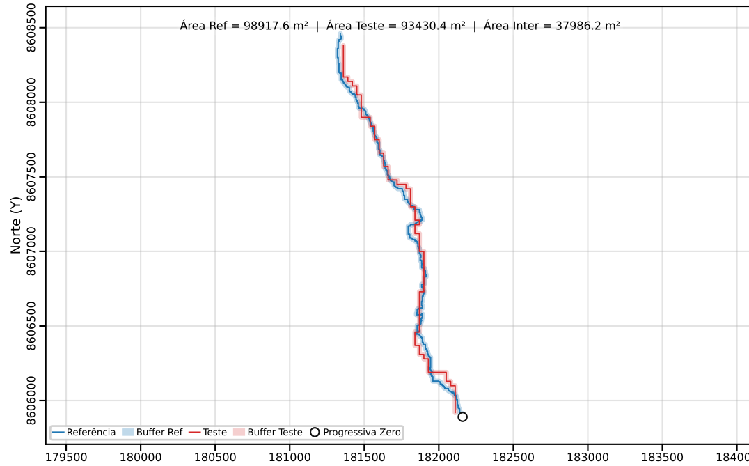
Classe C | PEC-PCD (Horizontal)=40.00 m | dm = 35.32
