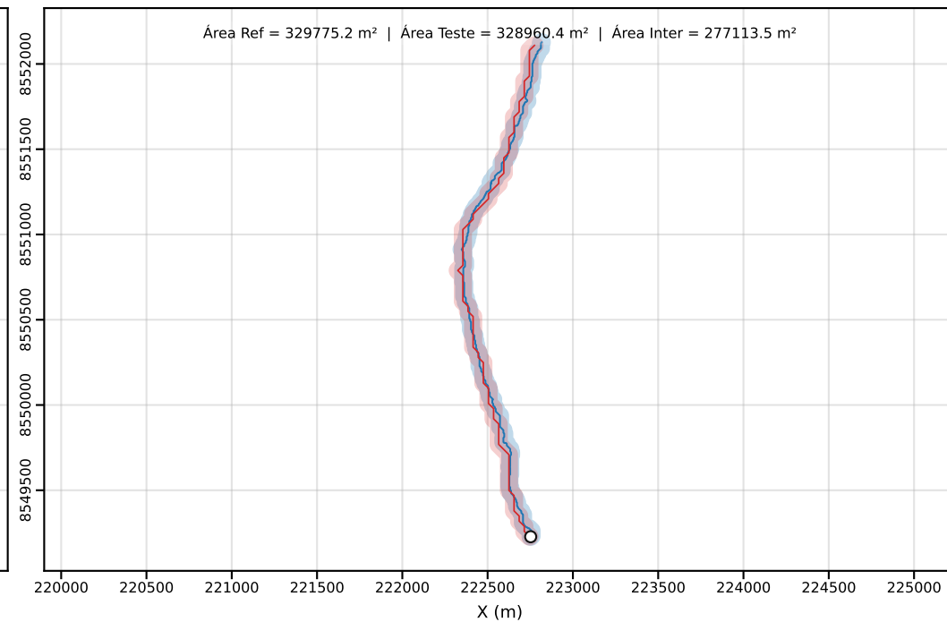
Classe D | PEC-PCD (Horizontal)=50.00 m | dm = 25.15
