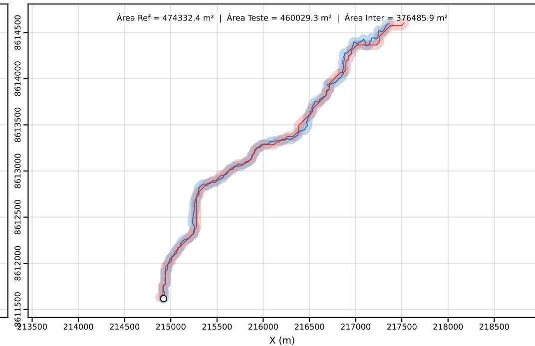
Classe D | PEC-PCD (Horizontal)=50.00 m | dm = 33.41
