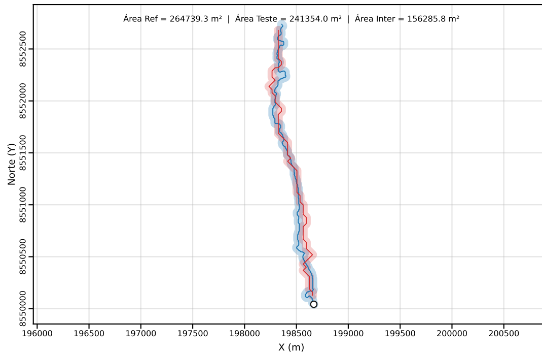
Classe C | PEC-PCD (Horizontal)=40.00 m | dm = 56.47
