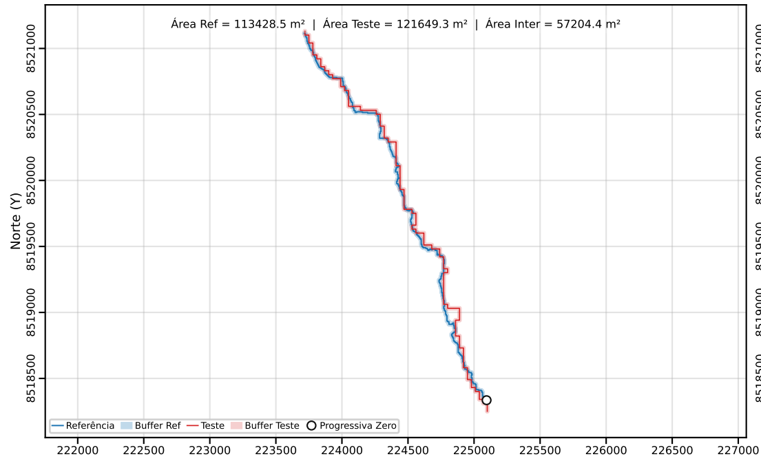
Classe C | PEC-PCD (Horizontal)=40.00 m | dm = 21.13
