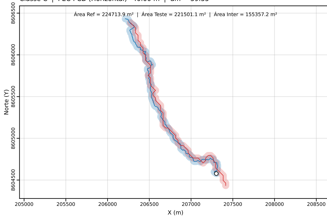
Classe C | PEC-PCD (Horizontal)=40.00 m | dm = 39.35
