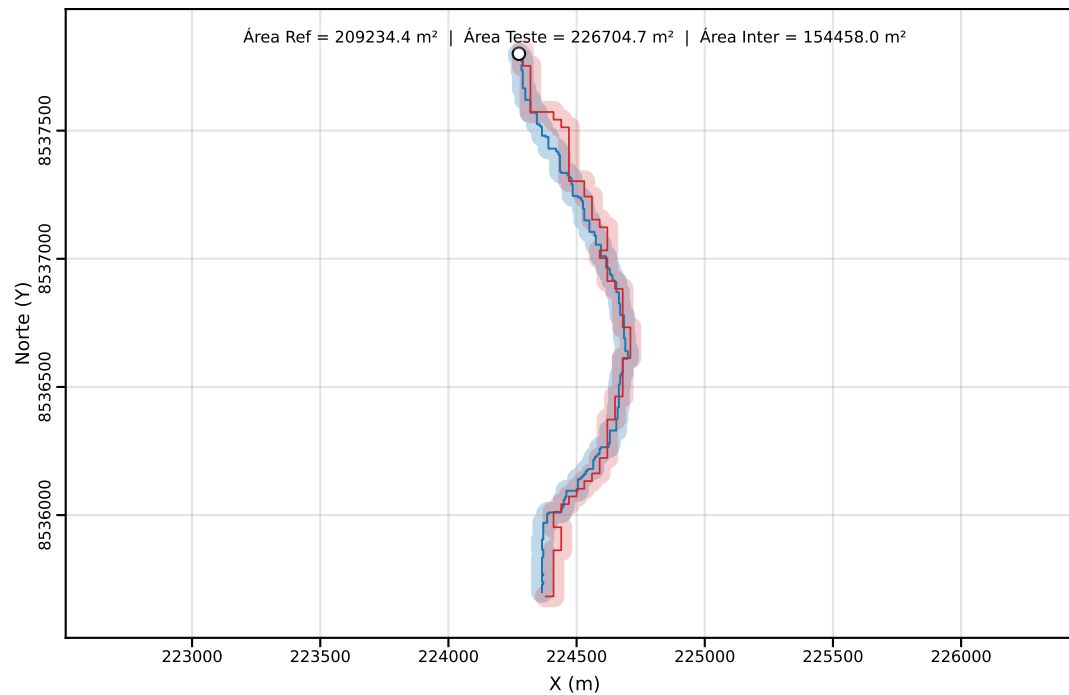
Classe C | PEC-PCD (Horizontal)=40.00 m | dm = 30.36
