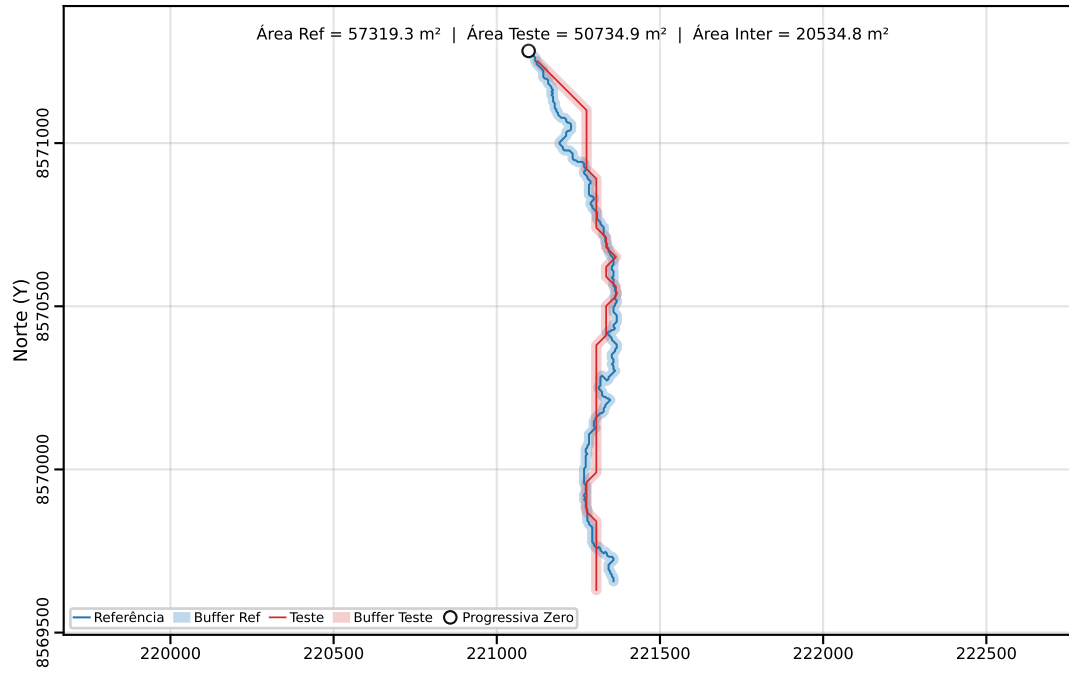
Classe C | PEC-PCD (Horizontal)=40.00 m | dm = 44.26
