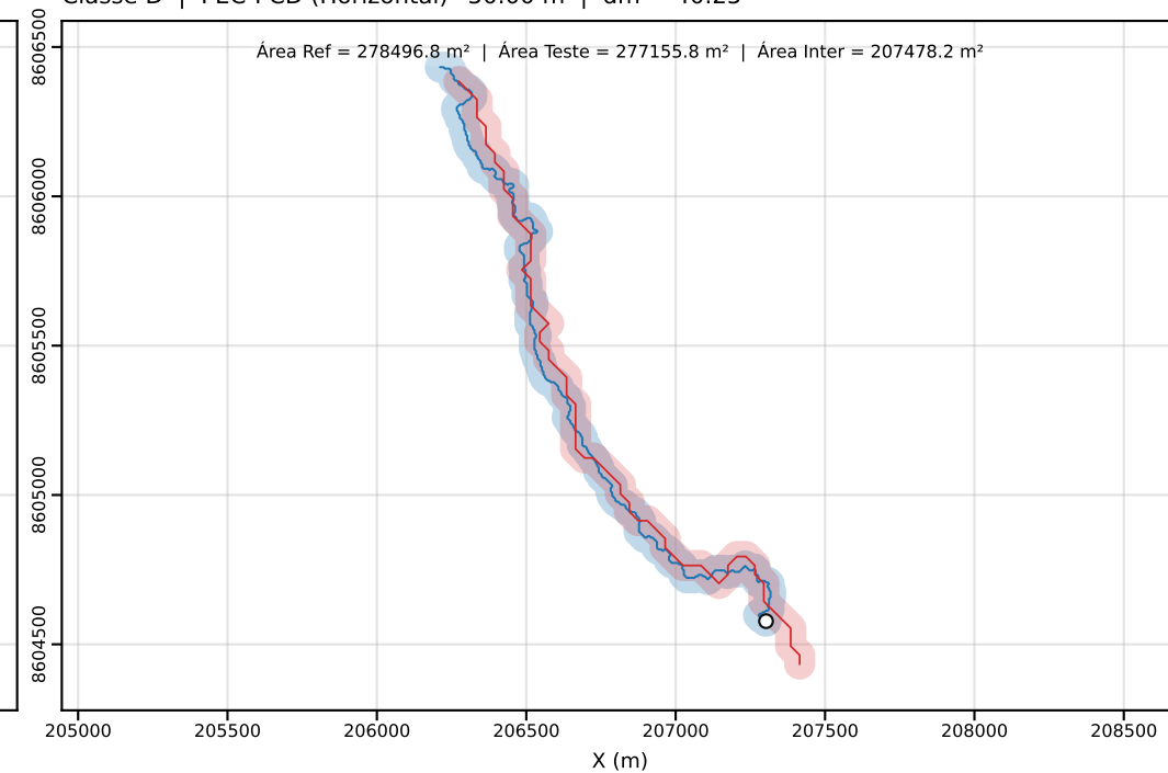
Classe D | PEC-PCD (Horizontal)=50.00 m | dm = 40.25
