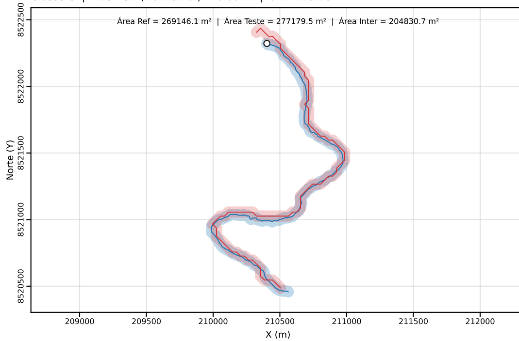
Classe C | PEC-PCD (Horizontal)=40.00 m | dm = 29.16
