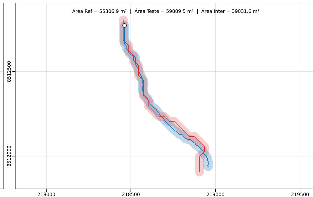
Classe D | PEC-PCD (Horizontal)=50.00 m | dm = 20.07
