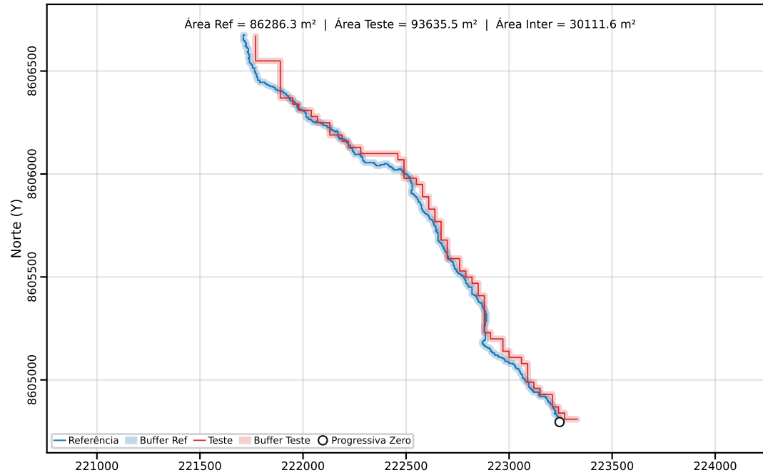
Classe C | PEC-PCD (Horizontal)=40.00 m | dm = 32.92
