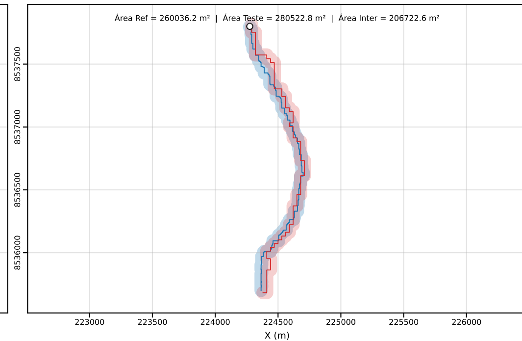
Classe D | PEC-PCD (Horizontal)=50.00 m | dm = 29.85
