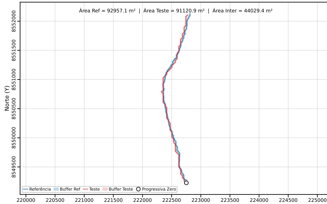
Classe C | PEC-PCD (Horizontal)=40.00 m | dm = 25.09
