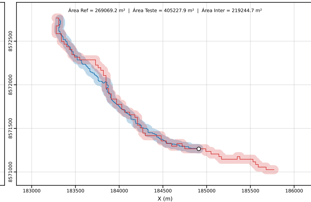
Classe D | PEC-PCD (Horizontal)=50.00 m | dm = 19.31
