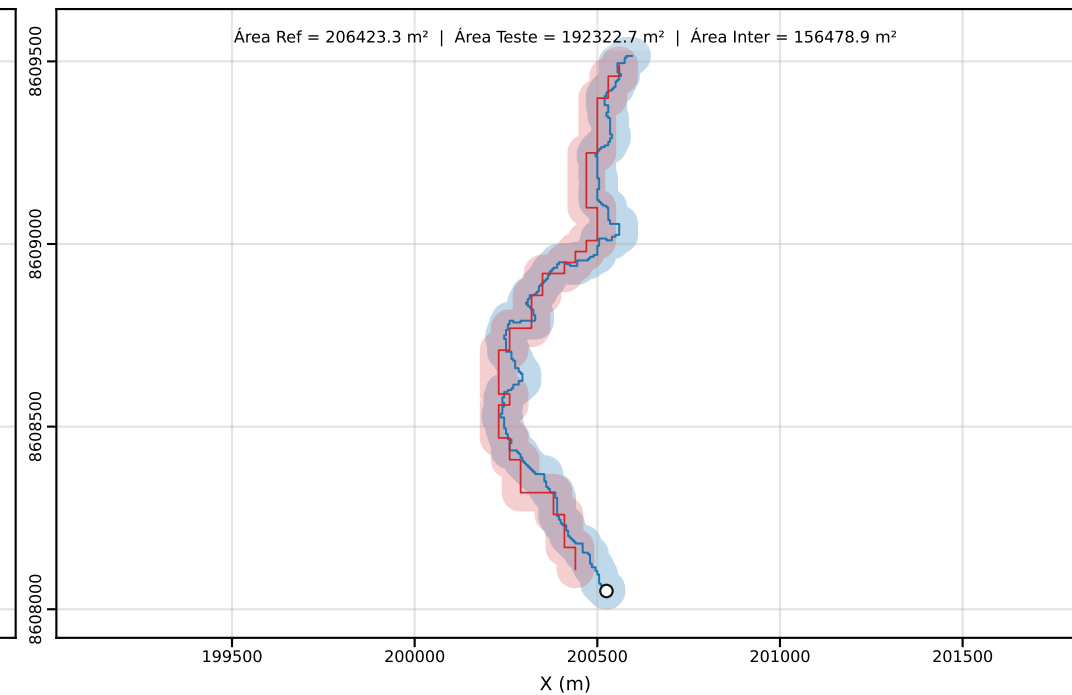
Classe D | PEC-PCD (Horizontal)=50.00 m | dm = 40.79
