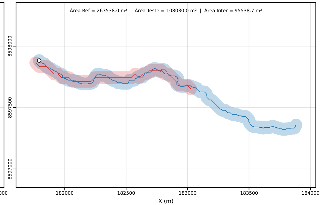
Classe D | PEC-PCD (Horizontal)=50.00 m | dm = 244.28
