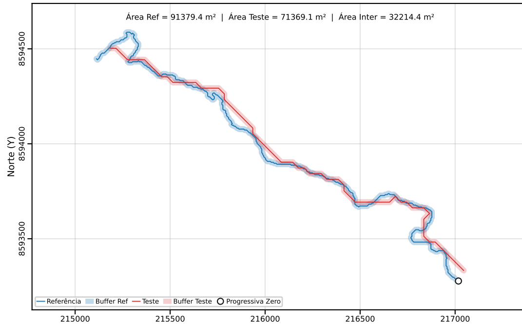
Classe C | PEC-PCD (Horizontal)=40.00 m | dm = 54.92
