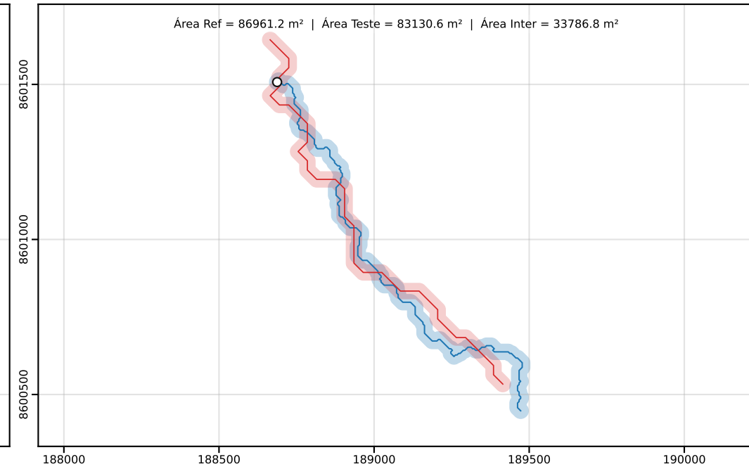
Classe D | PEC-PCD (Horizontal)=50.00 m | dm = 58.89
