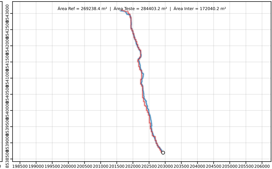
Classe D | PEC-PCD (Horizontal)=50.00 m | dm = 26.80
