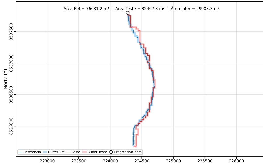
Classe C | PEC-PCD (Horizontal)=40.00 m | dm = 30.36
