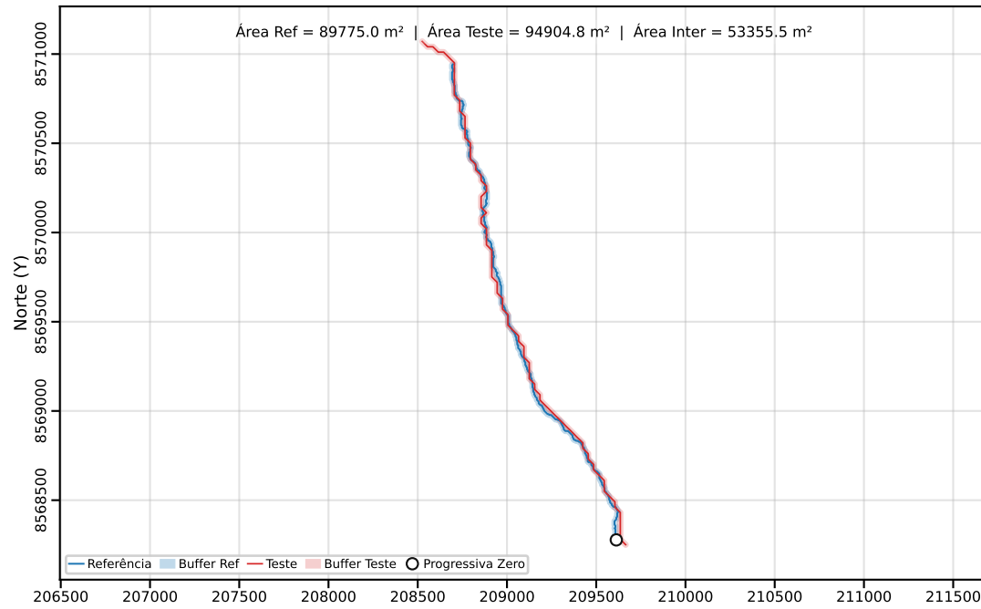
Classe C | PEC-PCD (Horizontal)=40.00 m | dm = 16.44
