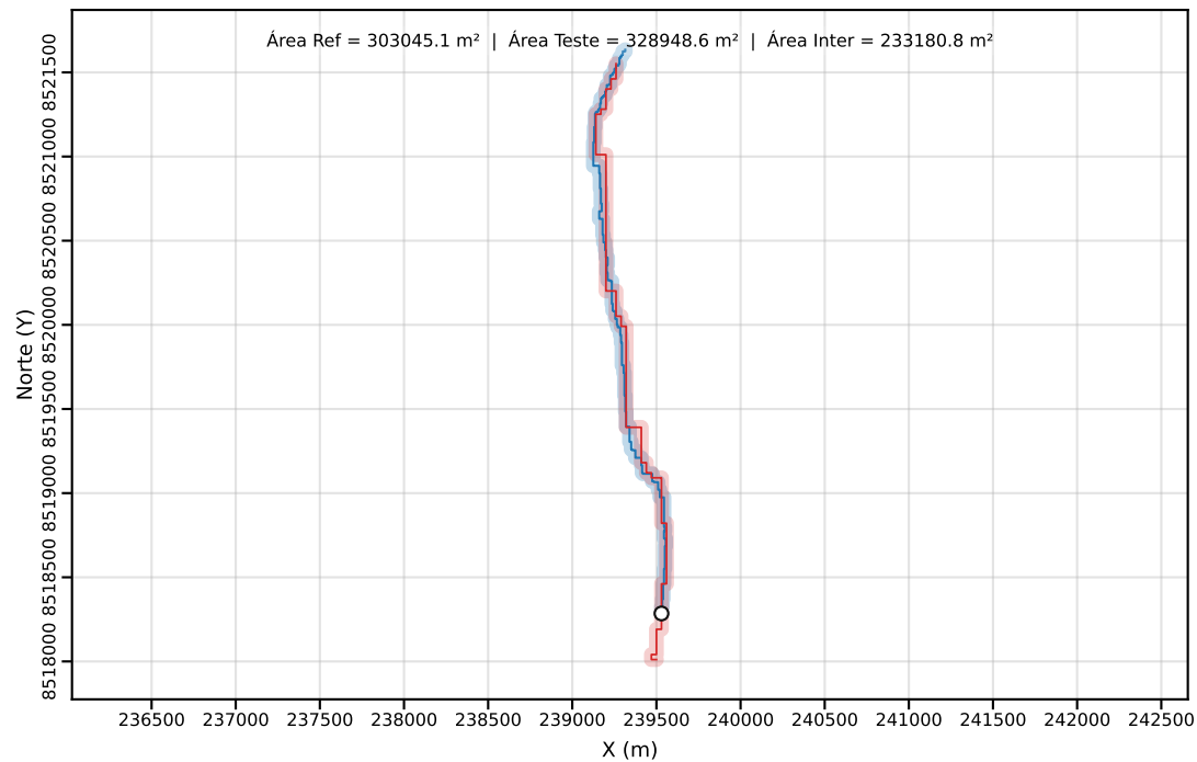
Classe C | PEC-PCD (Horizontal)=40.00 m | dm = 26.69
