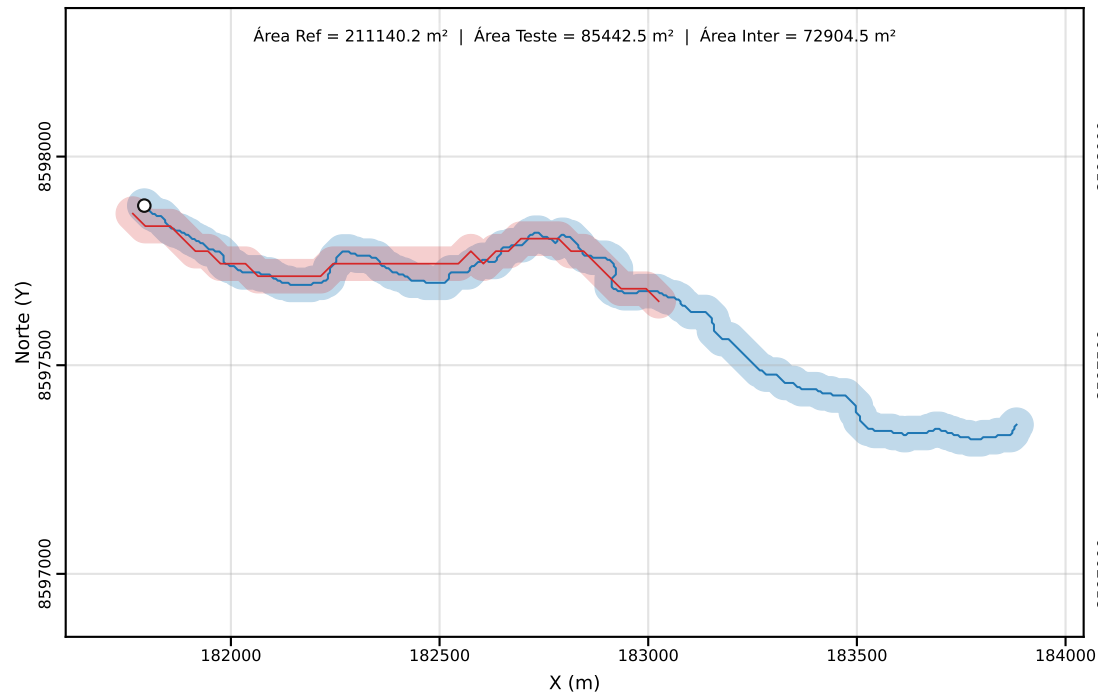
Classe C | PEC-PCD (Horizontal)=40.00 m | dm = 203.31
