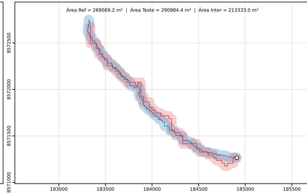
Classe D | PEC-PCD (Horizontal)=100.00 m | dm = 31.45
