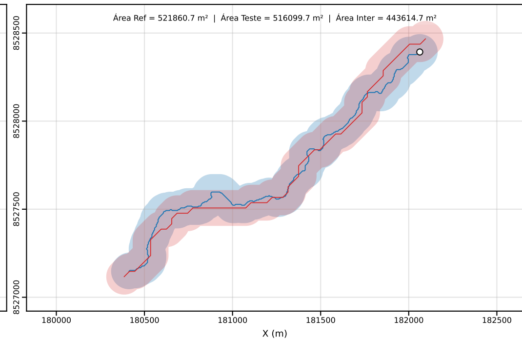
Classe D | PEC-PCD (Horizontal)=100.00 m | dm = 47.63
