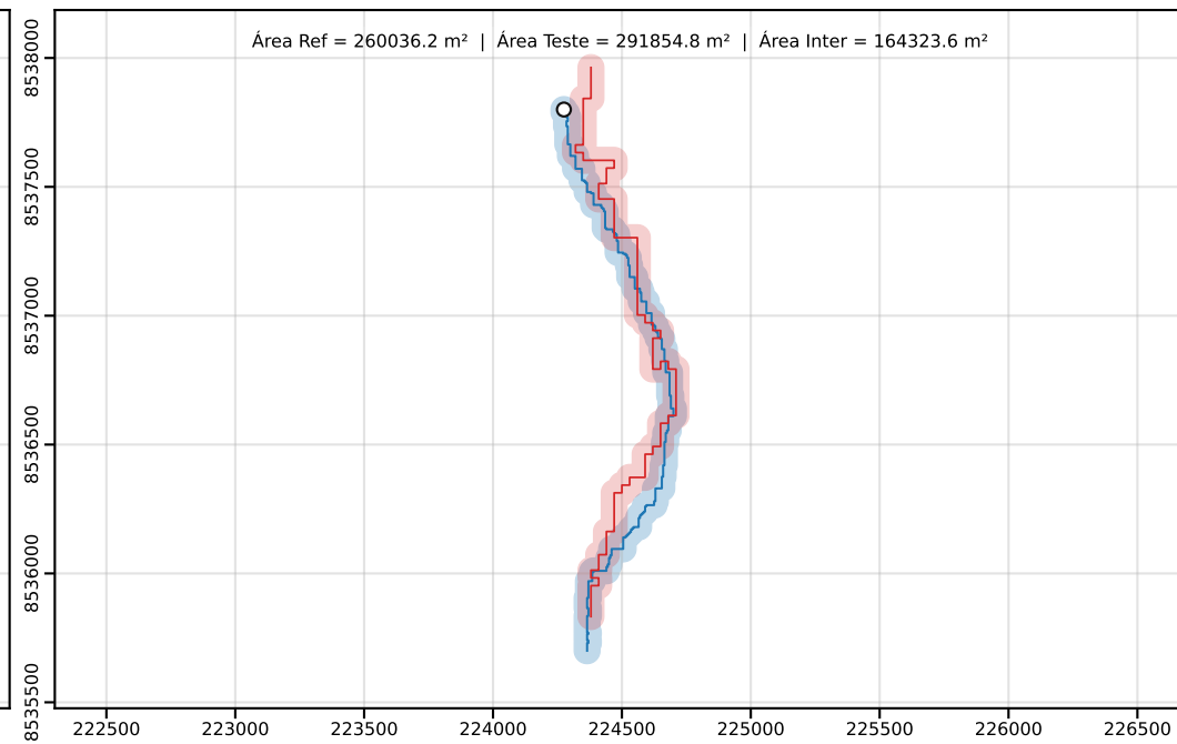
Classe D | PEC-PCD (Horizontal)=100.00 m | dm = 59.11
