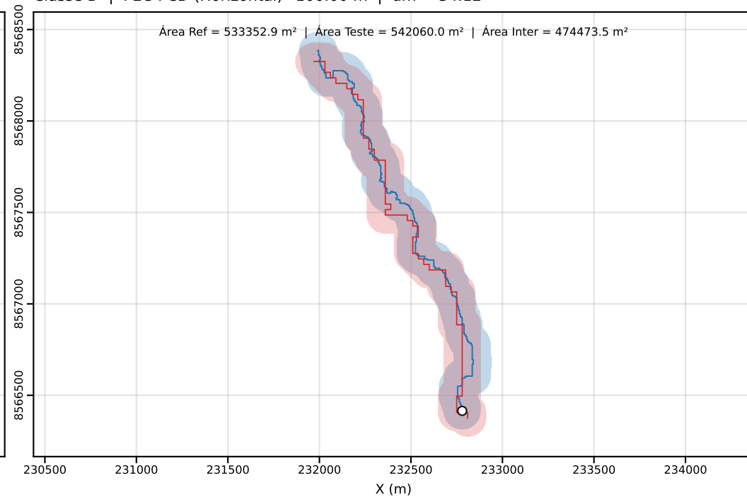
Classe D | PEC-PCD (Horizontal)=100.00 m | dm = 34.12
