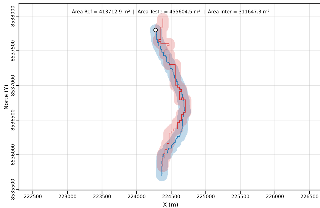
Classe C | PEC-PCD (Horizontal)=80.00 m | dm = 56.30
