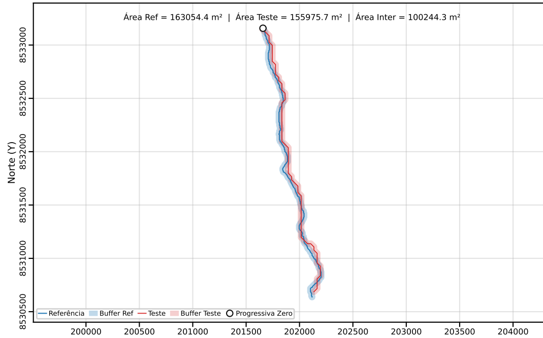
Classe C | PEC-PCD (Horizontal)=80.00 m | dm = 38.18
