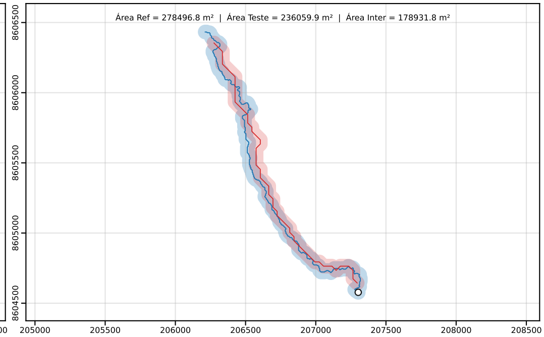
Classe D | PEC-PCD (Horizontal)=100.00 m | dm = 77.88
