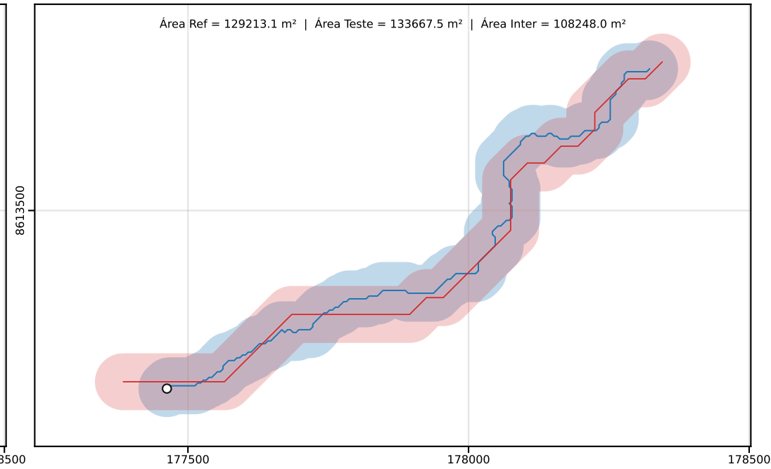
Classe D | PEC-PCD (Horizontal)=100.00 m | dm = 24.44
