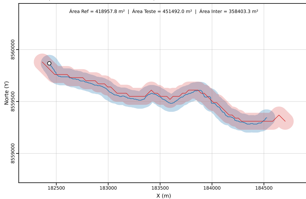
Classe C | PEC-PCD (Horizontal)=80.00 m | dm = 33.71
