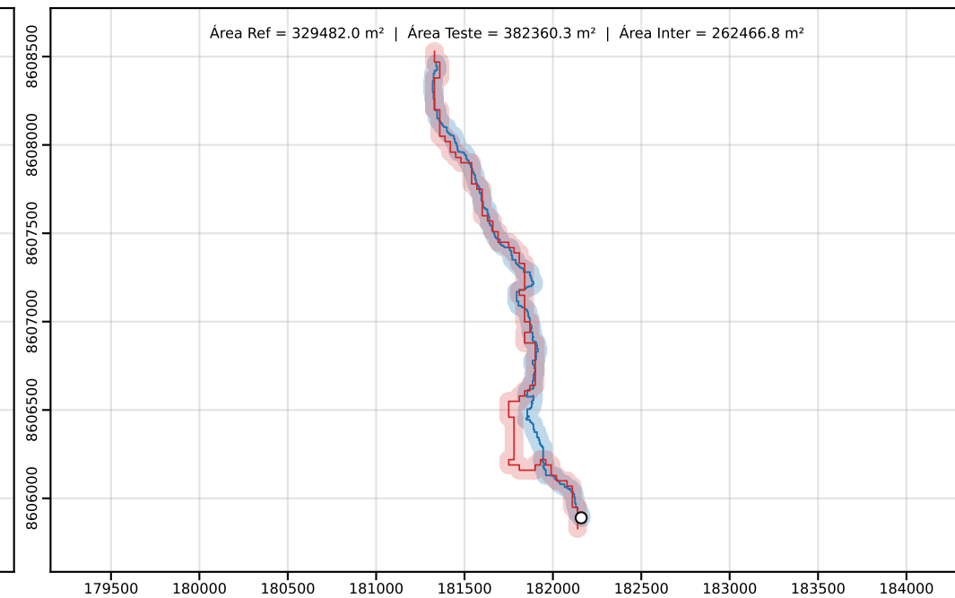
Classe D | PEC-PCD (Horizontal)=100.00 m | dm = 25.88
