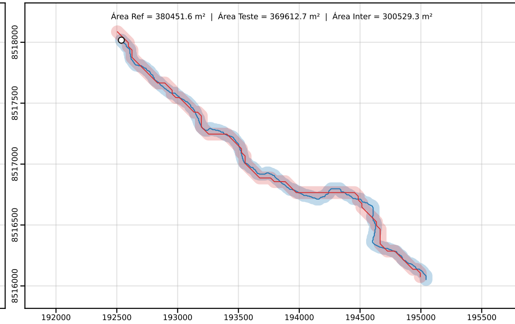
Classe D | PEC-PCD (Horizontal)=100.00 m | dm = 35.80
