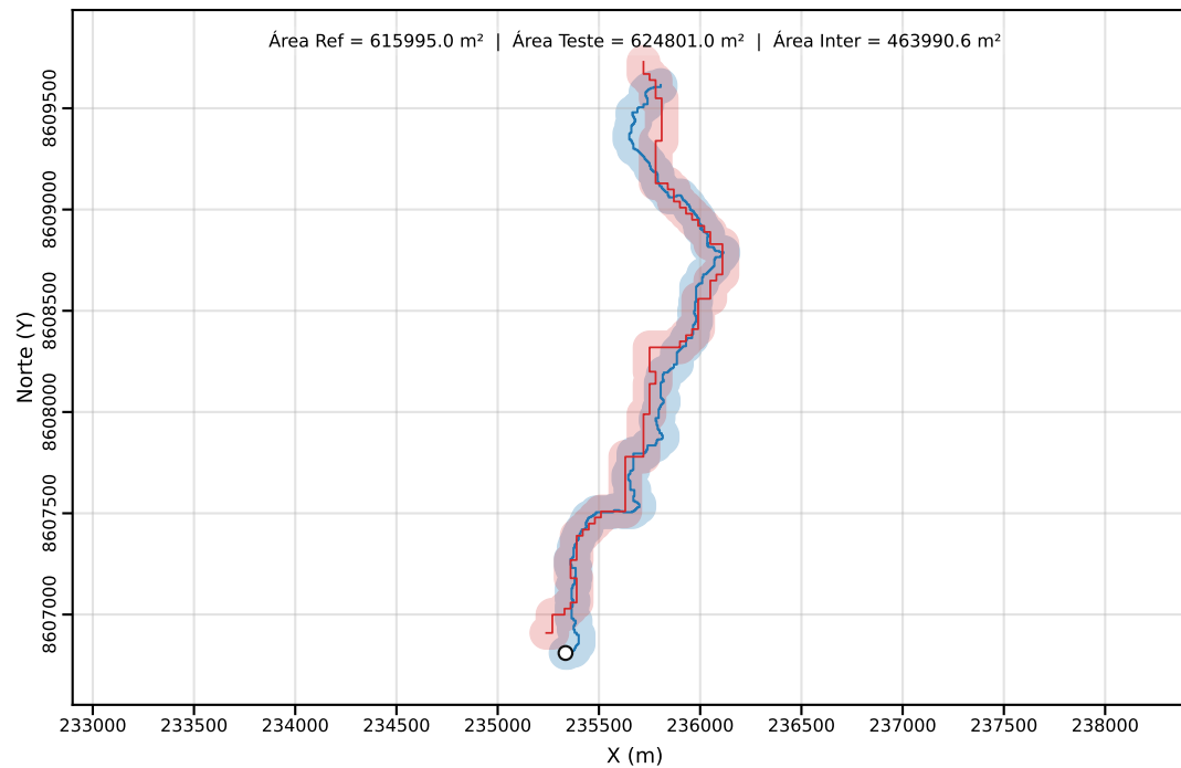
Classe C | PEC-PCD (Horizontal)=80.00 m | dm = 61.14
