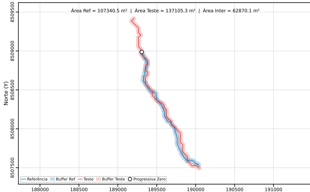
Classe C | PEC-PCD (Horizontal)=80.00 m | dm = 25.88
