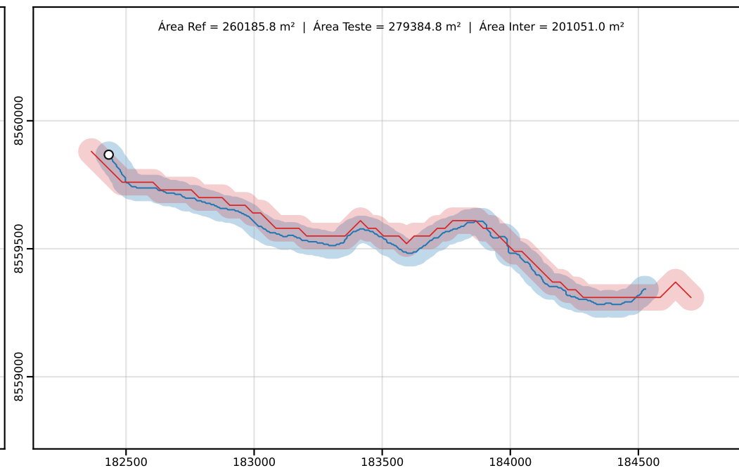
Classe D | PEC-PCD (Horizontal)=100.00 m | dm = 33.83
