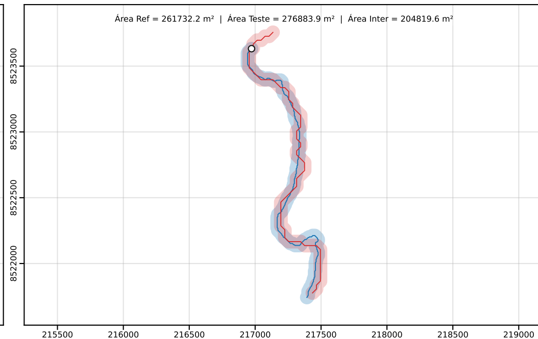
Classe D | PEC-PCD (Horizontal)=100.00 m | dm = 33.25
