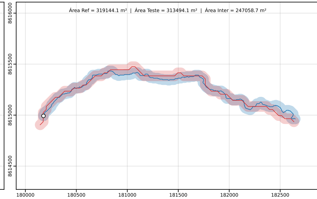
Classe D | PEC-PCD (Horizontal)=100.00 m | dm = 36.76
