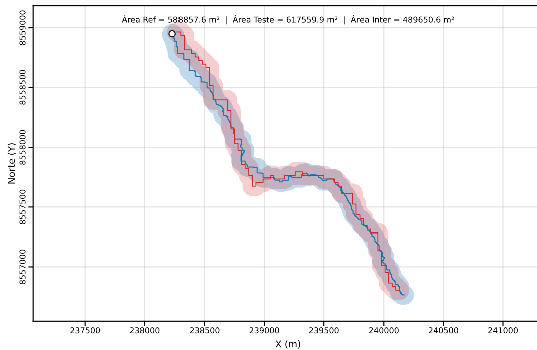
Classe C | PEC-PCD (Horizontal)=80.00 m | dm = 40.37
