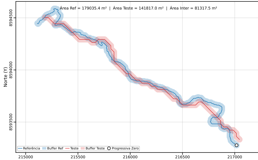
Classe C | PEC-PCD (Horizontal)=80.00 m | dm = 77.04
