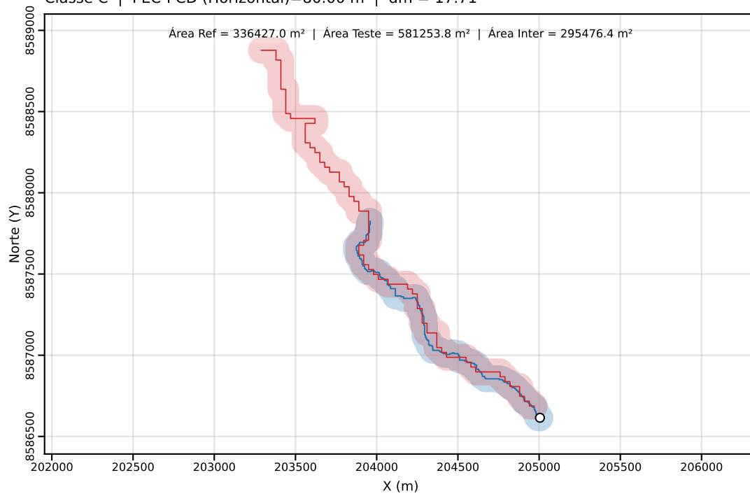
Classe C | PEC-PCD (Horizontal)=80.00 m | dm = 17.71
