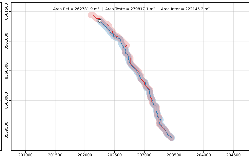
Classe D | PEC-PCD (Horizontal)=100.00 m | dm = 20.72
