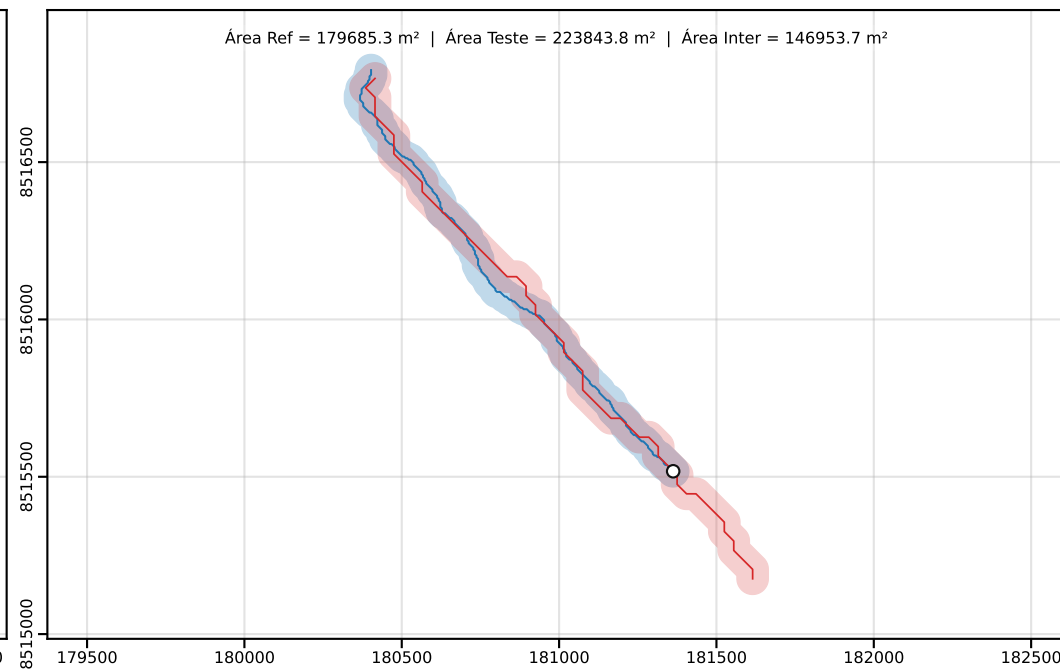
Classe D | PEC-PCD (Horizontal)=100.00 m | dm = 23.41
