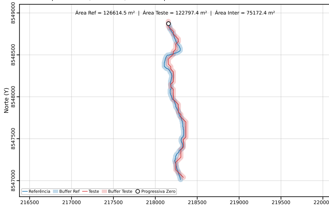
Classe C | PEC-PCD (Horizontal)=80.00 m | dm = 38.40
