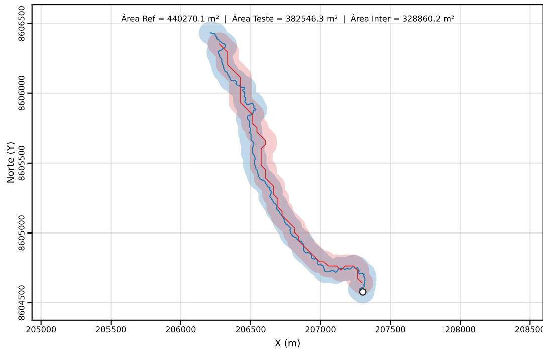
Classe C | PEC-PCD (Horizontal)=80.00 m | dm = 73.19
