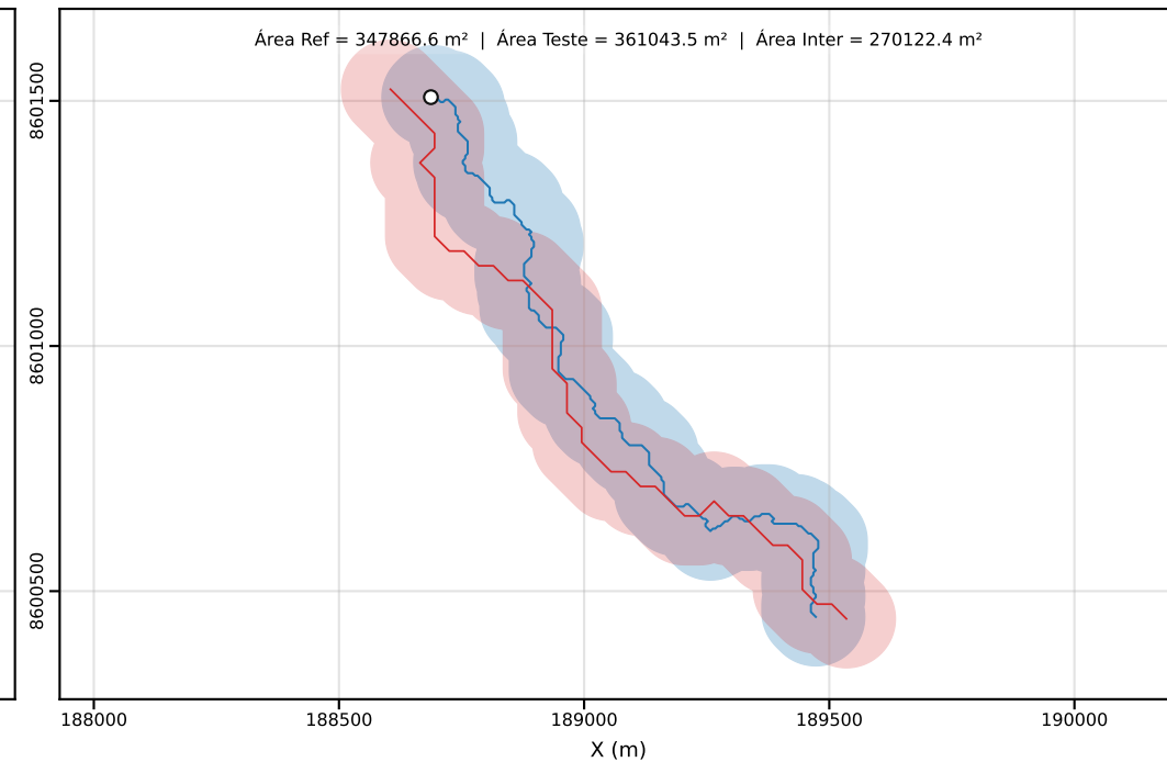
Classe D | PEC-PCD (Horizontal)=100.00 m | dm = 67.65
