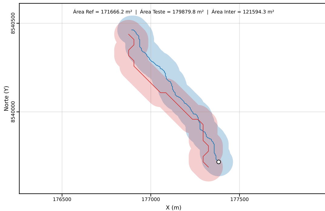
Classe C | PEC-PCD (Horizontal)=80.00 m | dm = 69.96
