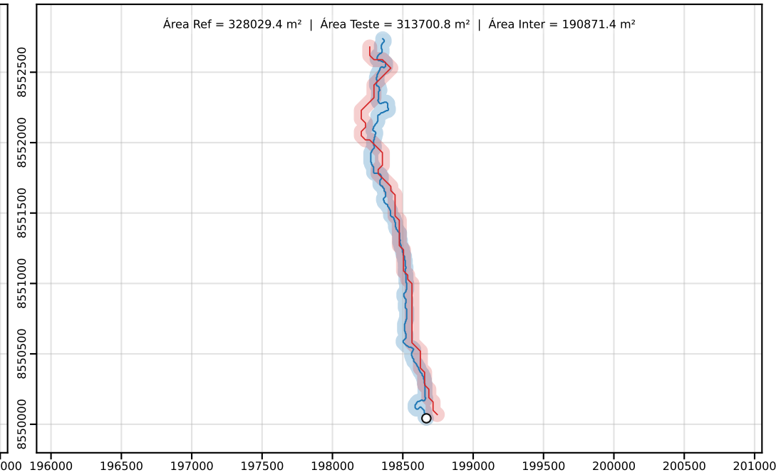
Classe D | PEC-PCD (Horizontal)=100.00 m | dm = 73.09
