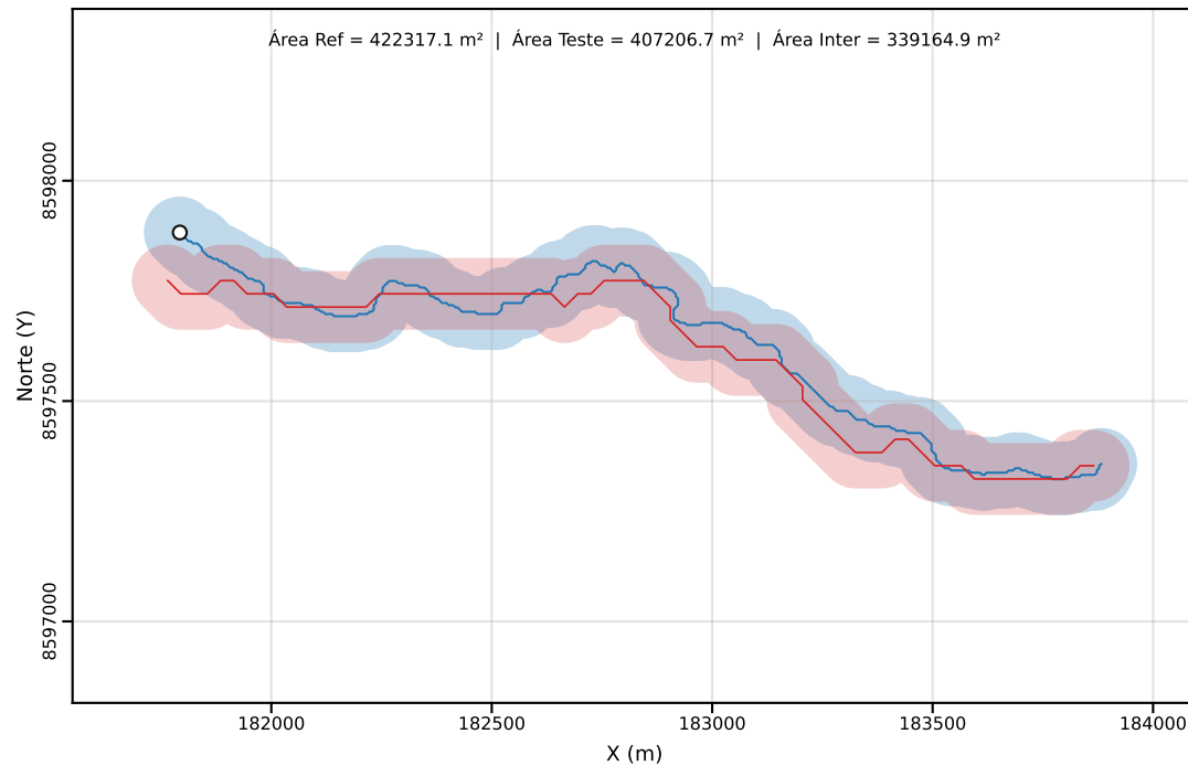
Classe C | PEC-PCD (Horizontal)=80.00 m | dm = 51.32
