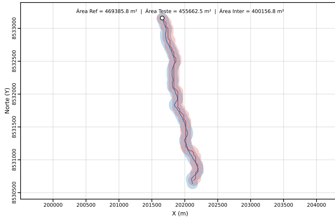
Classe C | PEC-PCD (Horizontal)=80.00 m | dm = 38.18
