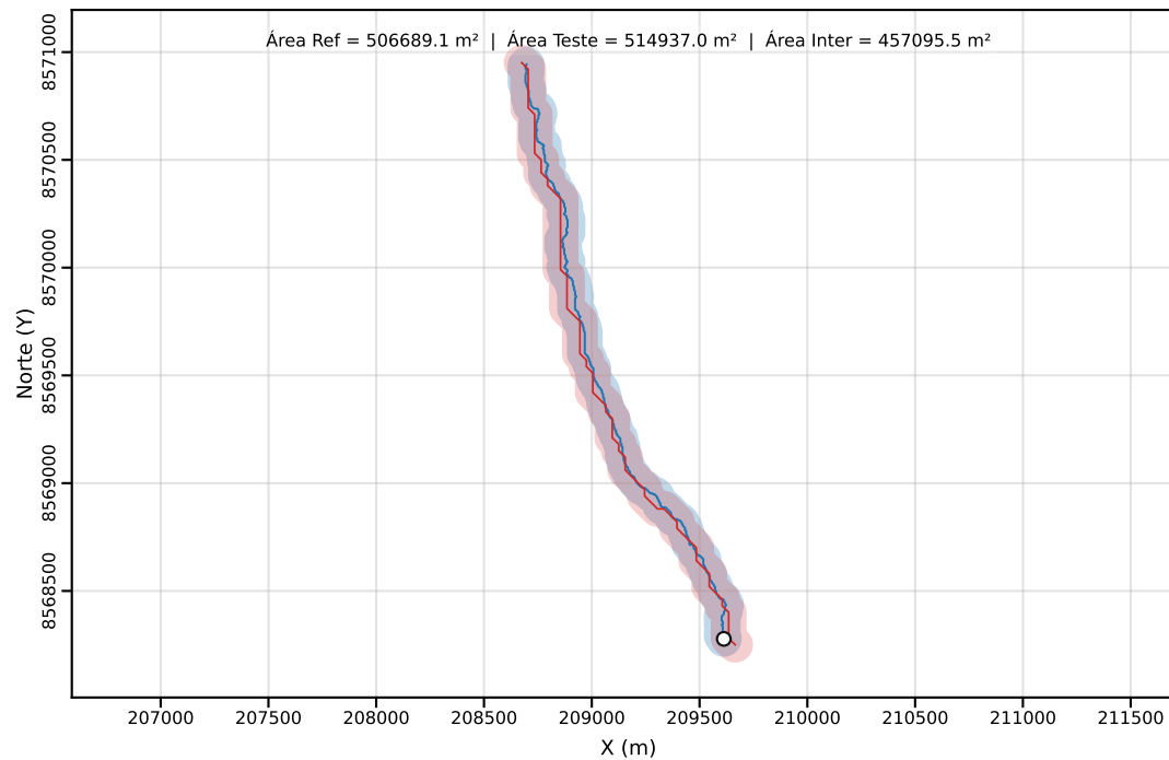
Classe C | PEC-PCD (Horizontal)=80.00 m | dm = 24.21
