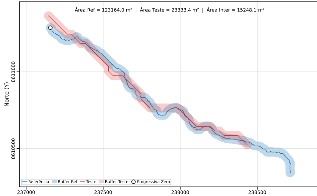
Classe C | PEC-PCD (Horizontal)=80.00 m | dm = 903.54
