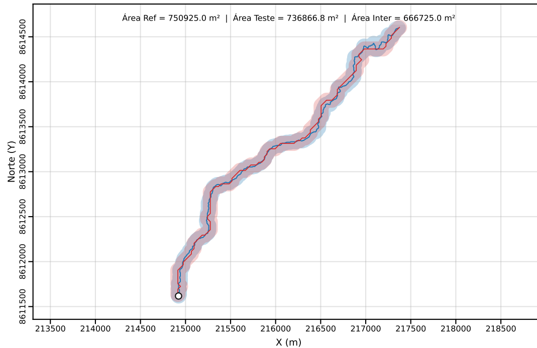
Classe C | PEC-PCD (Horizontal)=80.00 m | dm = 28.72
