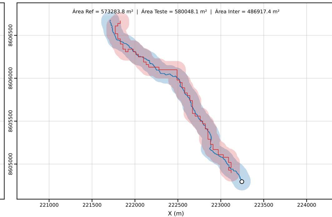
Classe D | PEC-PCD (Horizontal)=100.00 m | dm = 46.78
