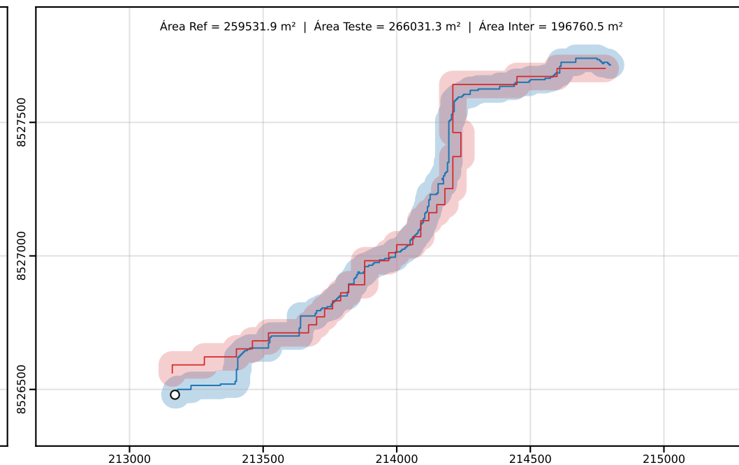
Classe D | PEC-PCD (Horizontal)=100.00 m | dm = 41.82
