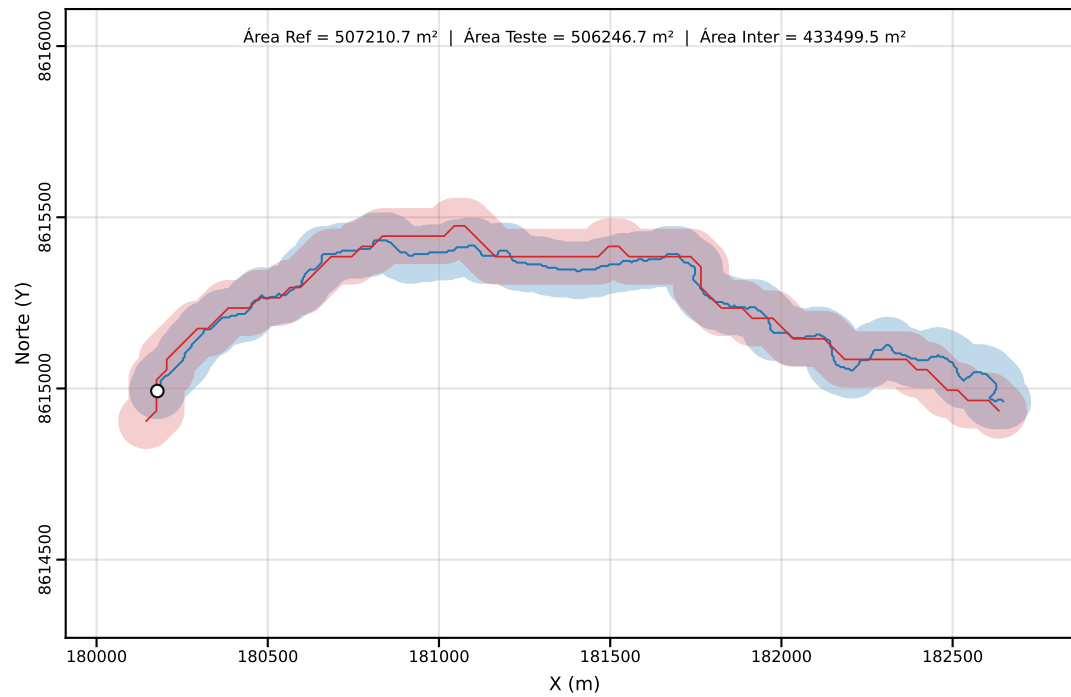
Classe C | PEC-PCD (Horizontal)=80.00 m | dm = 36.59
