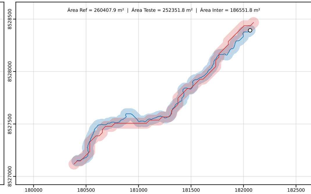
Classe D | PEC-PCD (Horizontal)=100.00 m | dm = 47.63
