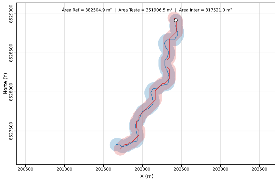
Classe C | PEC-PCD (Horizontal)=80.00 m | dm = 46.41
