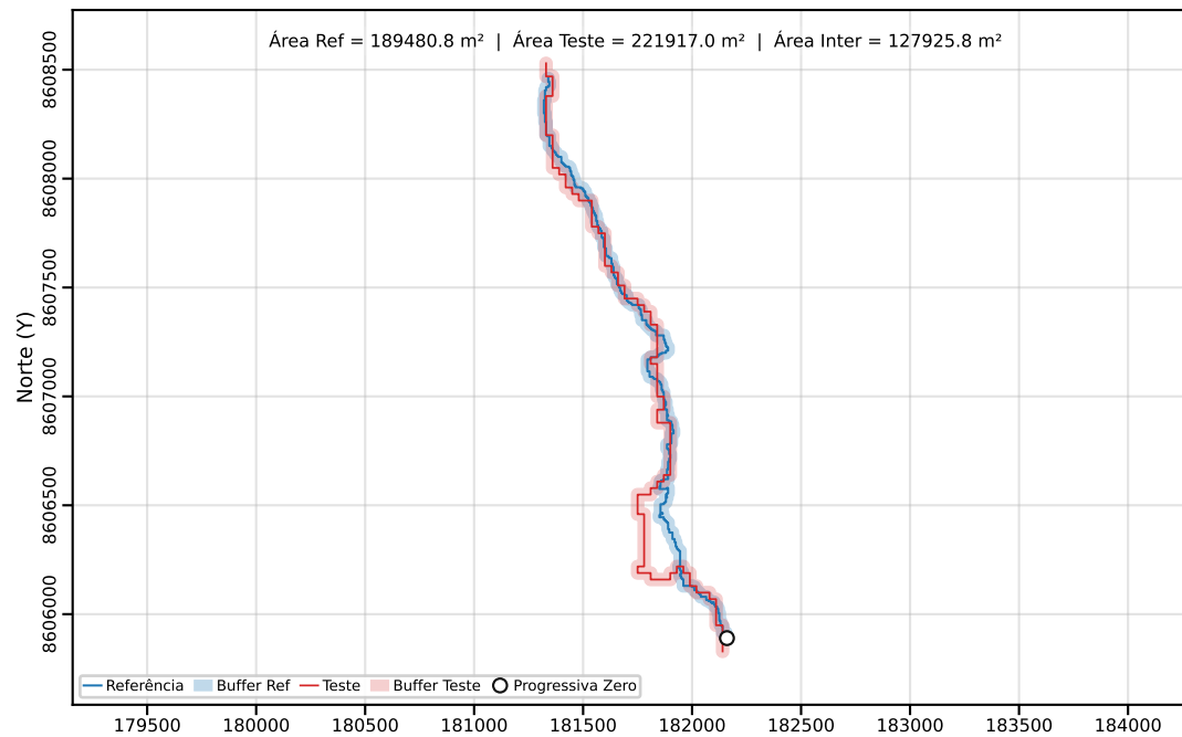
Classe C | PEC-PCD (Horizontal)=80.00 m | dm = 27.55
