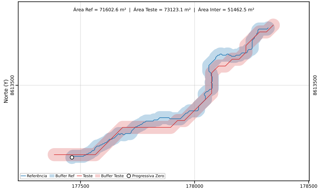
Classe C | PEC-PCD (Horizontal)=80.00 m | dm = 24.67
