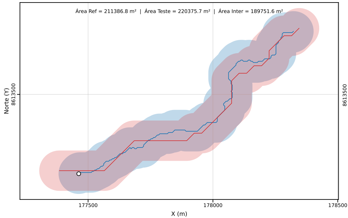
Classe C | PEC-PCD (Horizontal)=80.00 m | dm = 24.67
