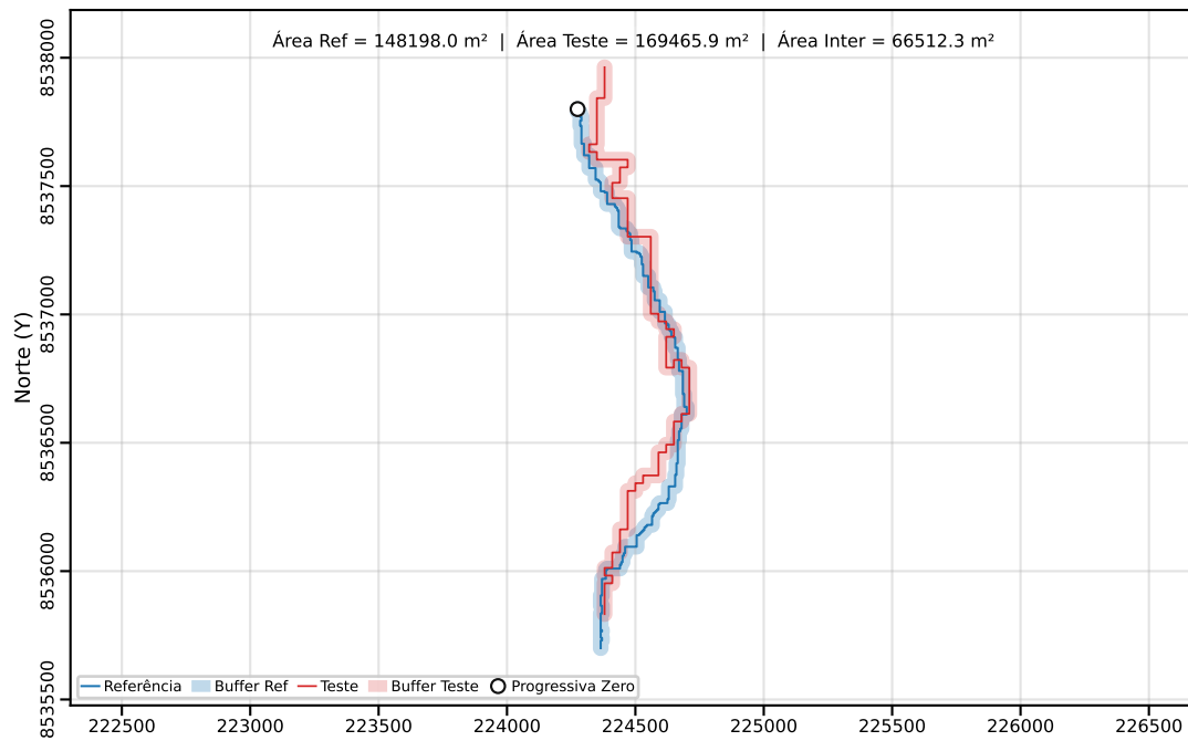
Classe C | PEC-PCD (Horizontal)=80.00 m | dm = 56.30
