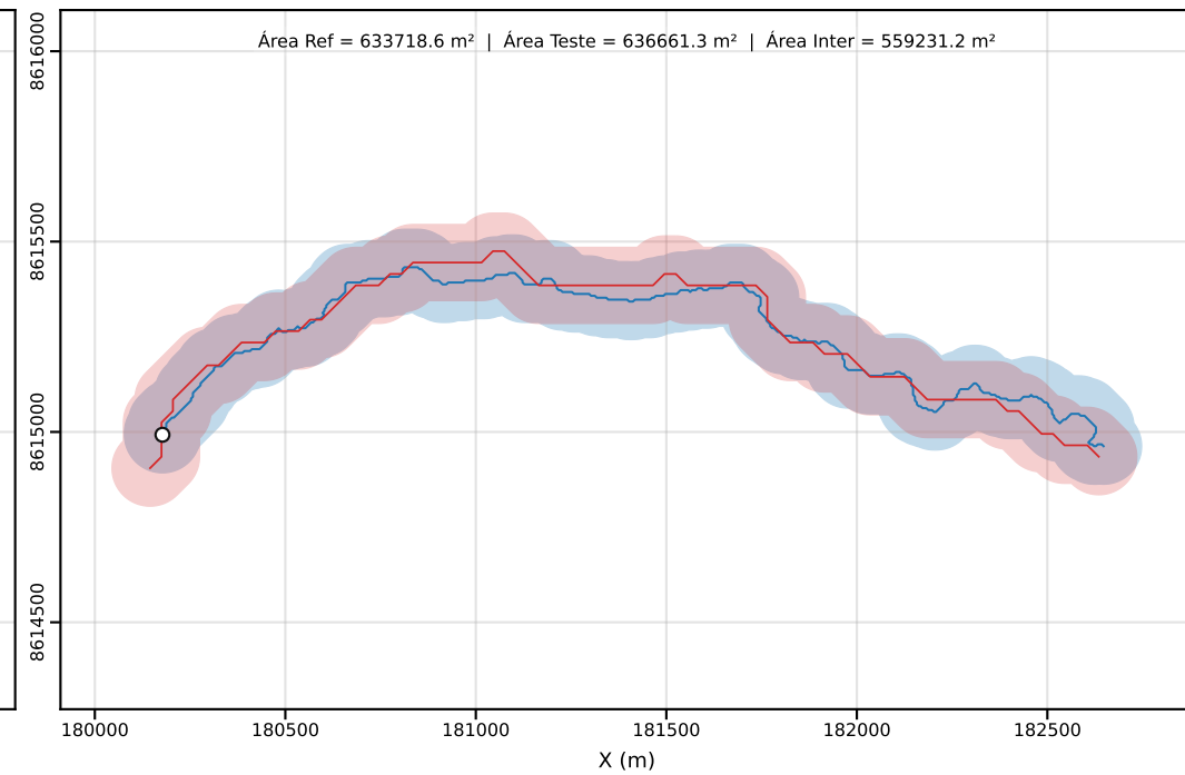
Classe D | PEC-PCD (Horizontal)=100.00 m | dm = 36.76
