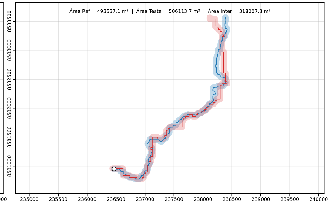
Classe D | PEC-PCD (Horizontal)=100.00 m | dm = 64.60
