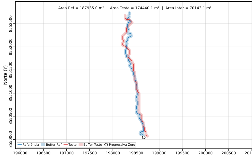
Classe C | PEC-PCD (Horizontal)=80.00 m | dm = 71.49
