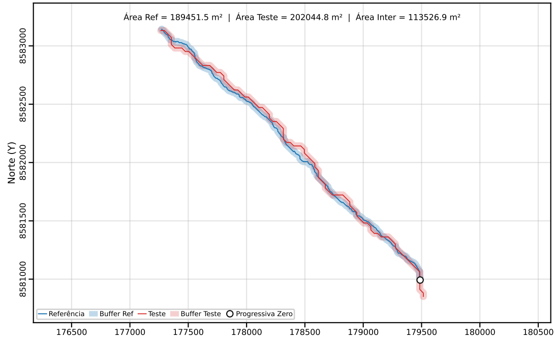
Classe C | PEC-PCD (Horizontal)=80.00 m | dm = 29.49
