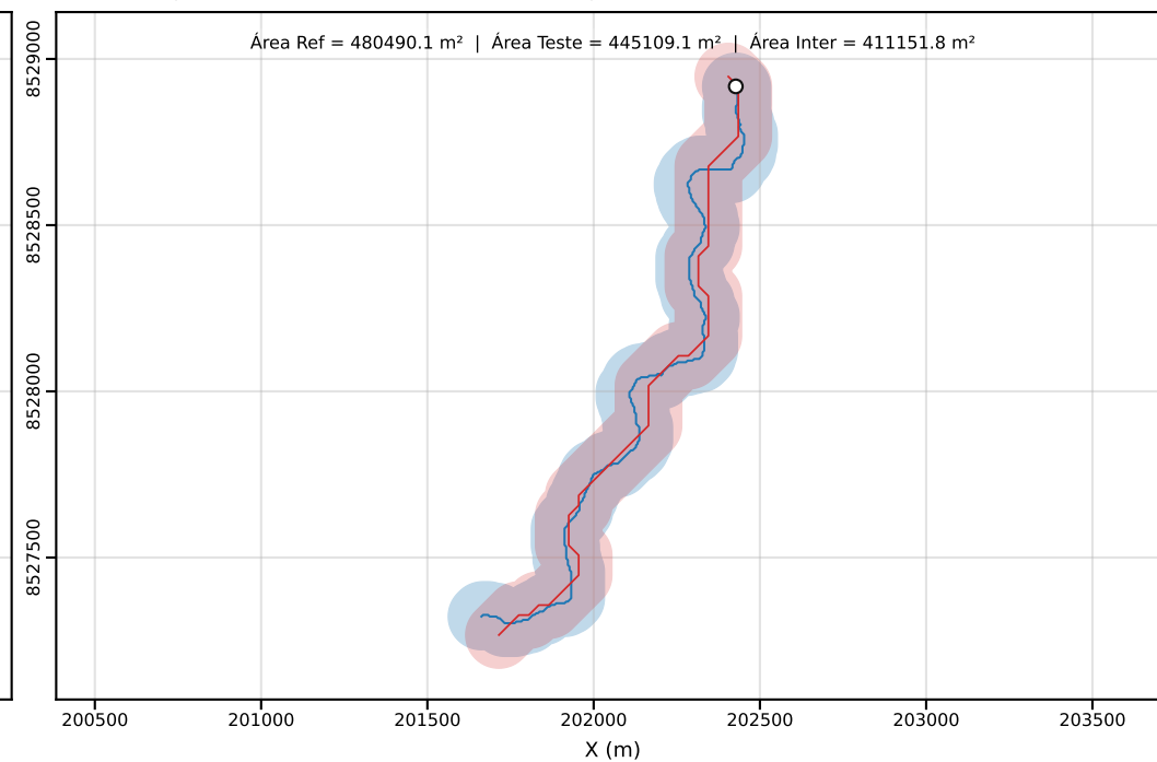
Classe D | PEC-PCD (Horizontal)=100.00 m | dm = 48.94
