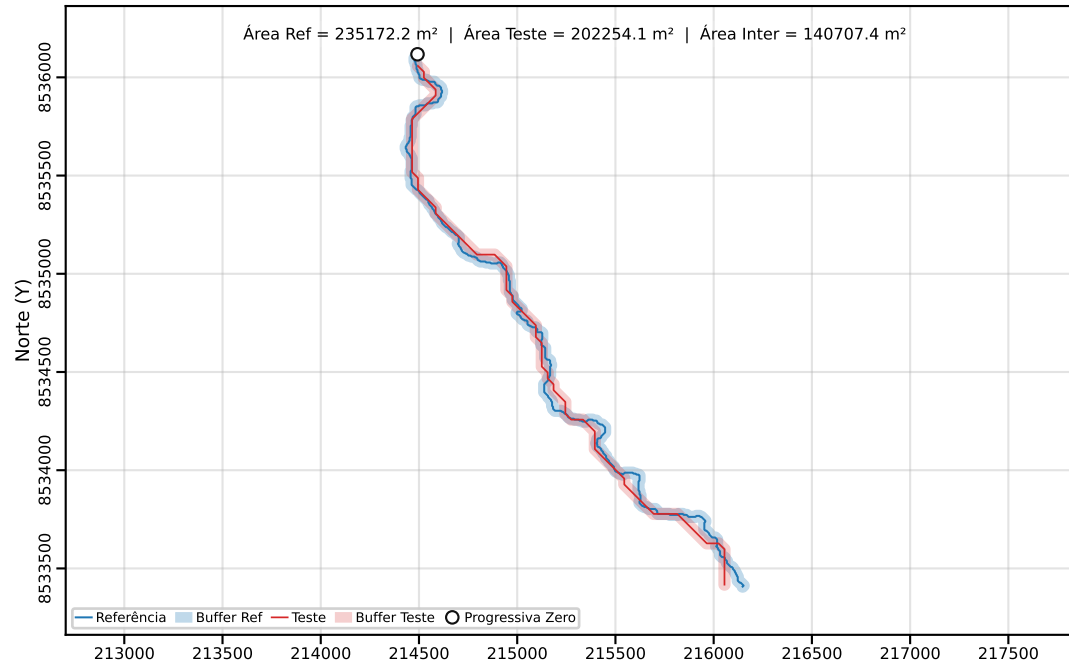
Classe C | PEC-PCD (Horizontal)=80.00 m | dm = 52.98
