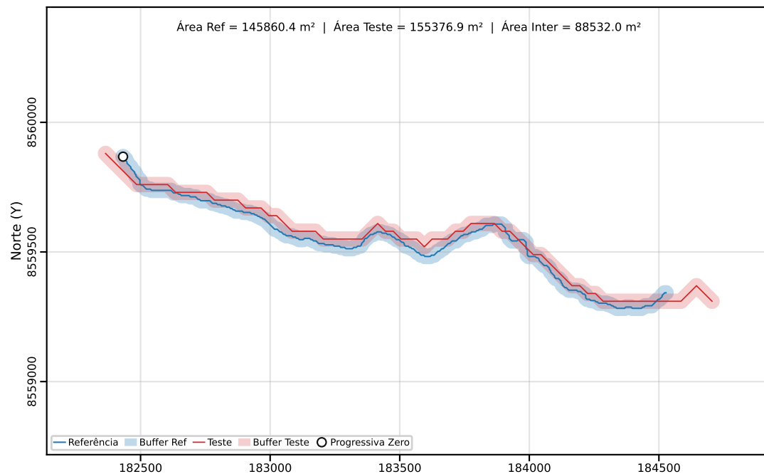
Classe C | PEC-PCD (Horizontal)=80.00 m | dm = 33.71
