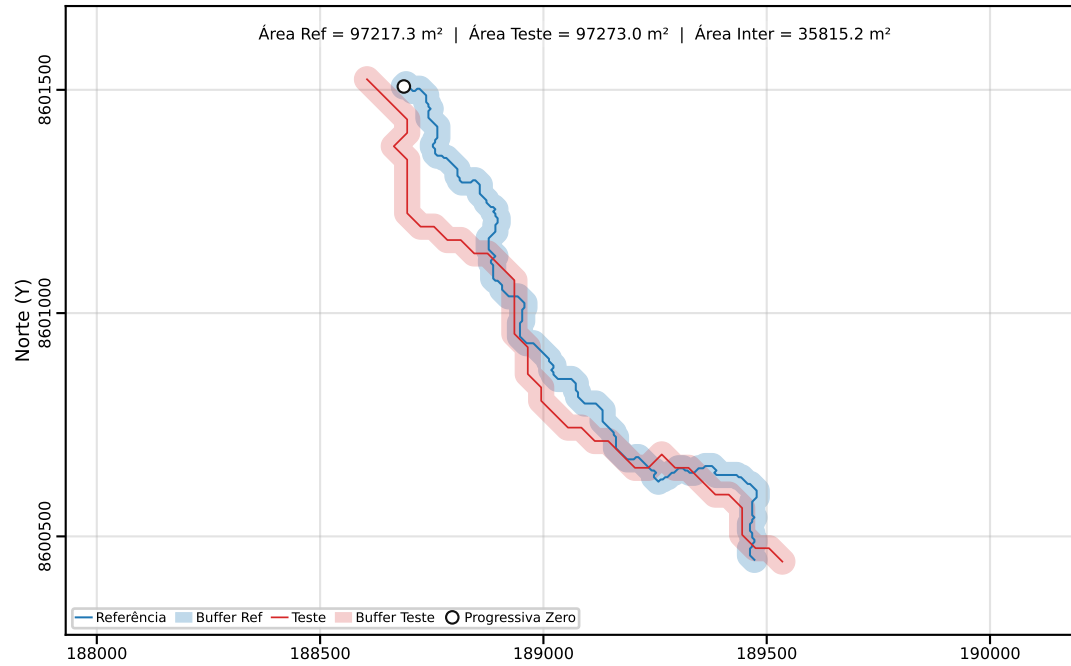
Classe C | PEC-PCD (Horizontal)=80.00 m | dm = 68.01
