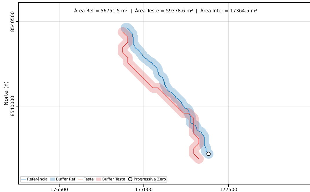
Classe C | PEC-PCD (Horizontal)=80.00 m | dm = 69.96
