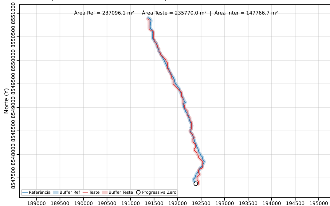
Classe C | PEC-PCD (Horizontal)=80.00 m | dm = 33.87
