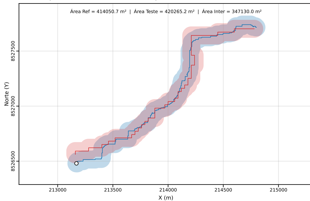
Classe C | PEC-PCD (Horizontal)=80.00 m | dm = 40.02
