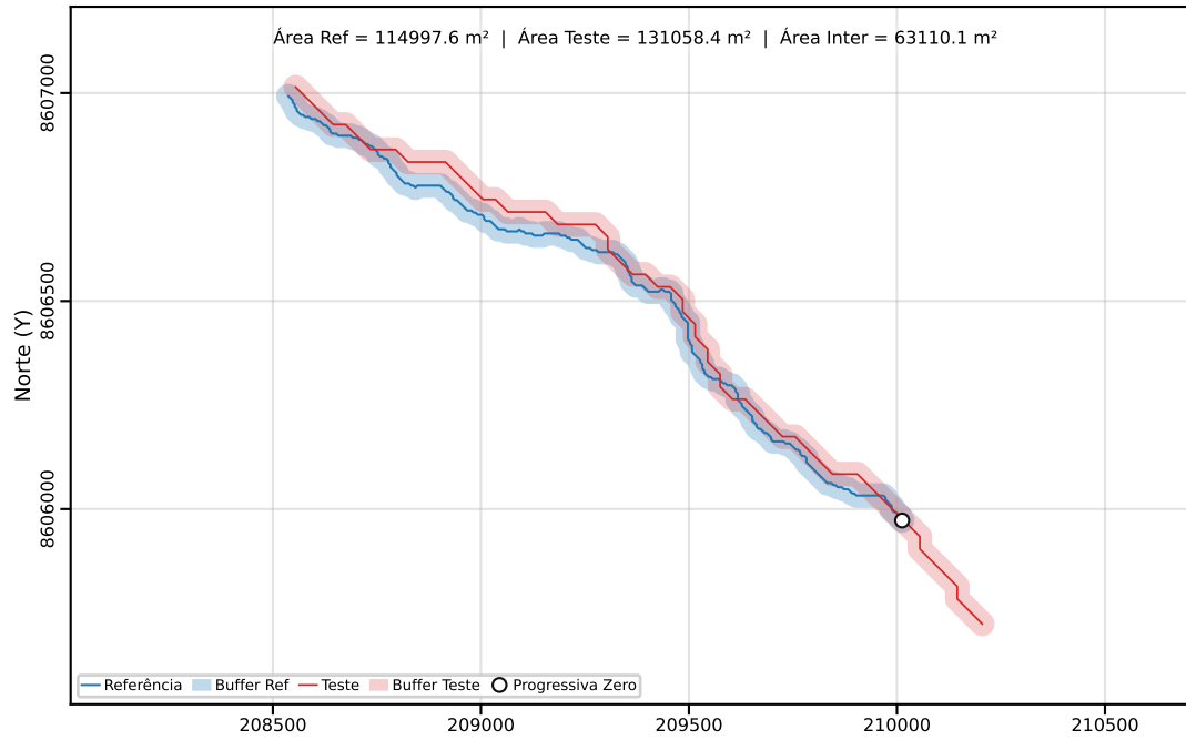
Classe C | PEC-PCD (Horizontal)=80.00 m | dm = 34.12
