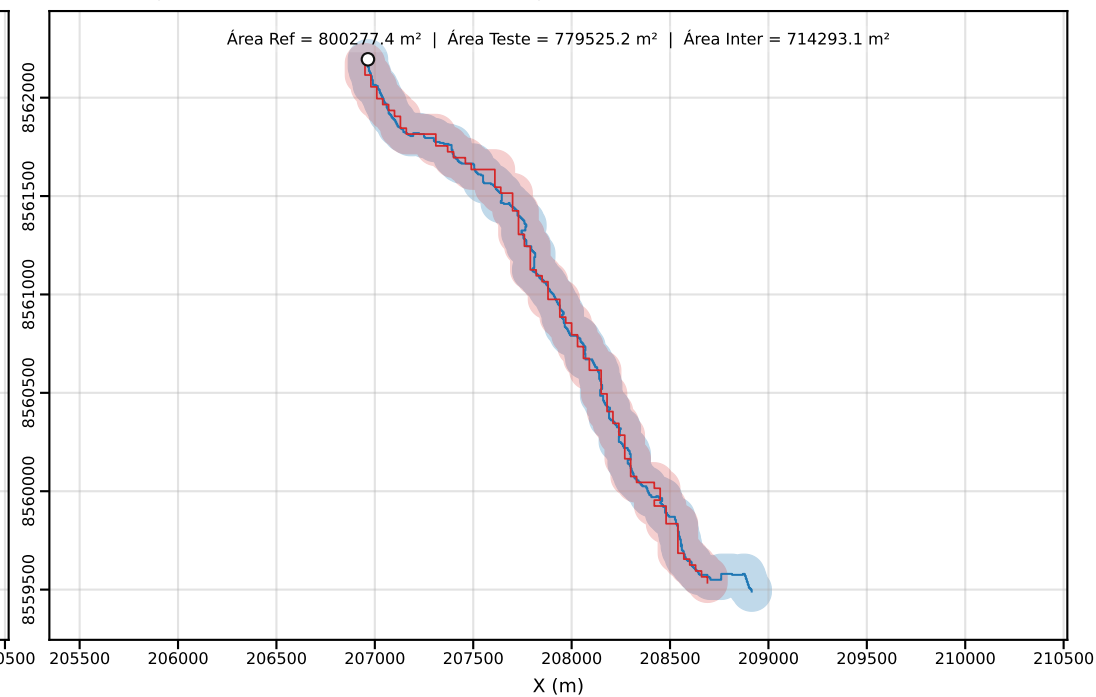
Classe D | PEC-PCD (Horizontal)=100.00 m | dm = 34.65
