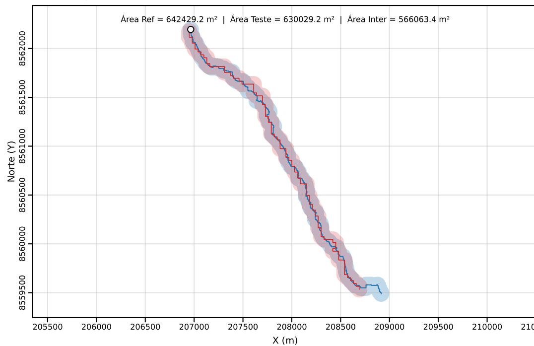
Classe C | PEC-PCD (Horizontal)=80.00 m | dm = 30.46
