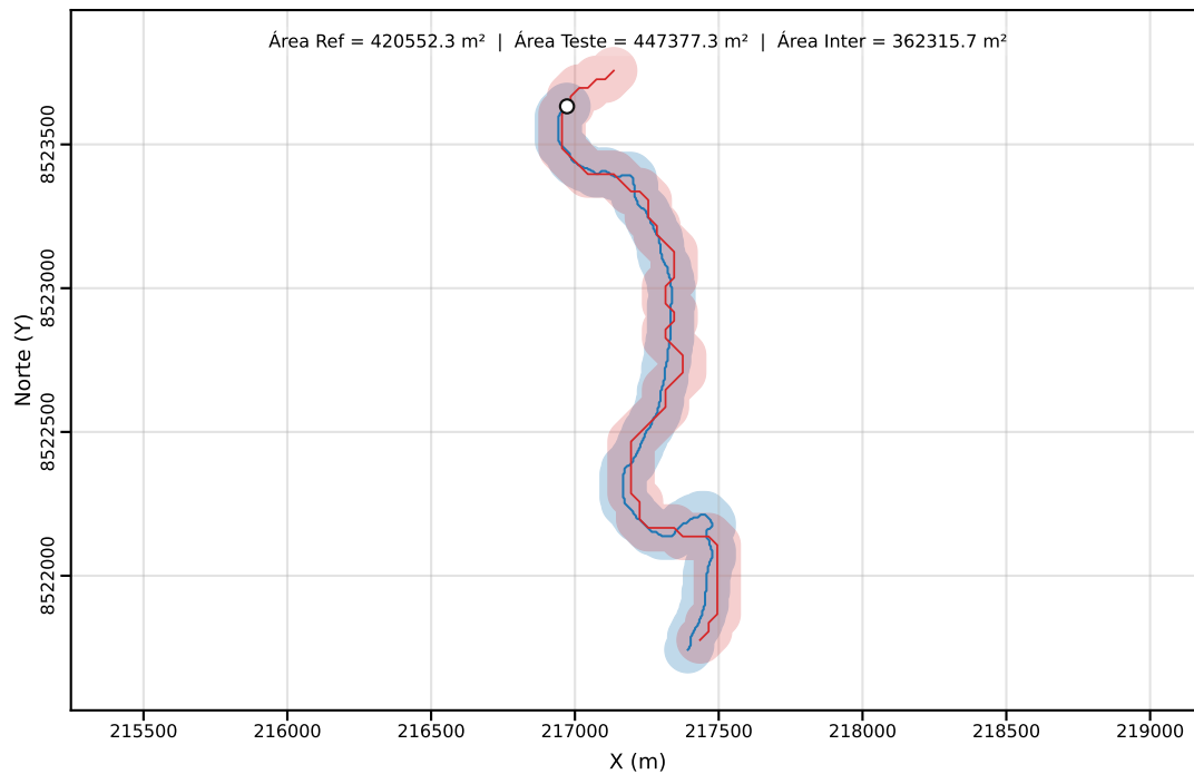
Classe C | PEC-PCD (Horizontal)=80.00 m | dm = 32.72
