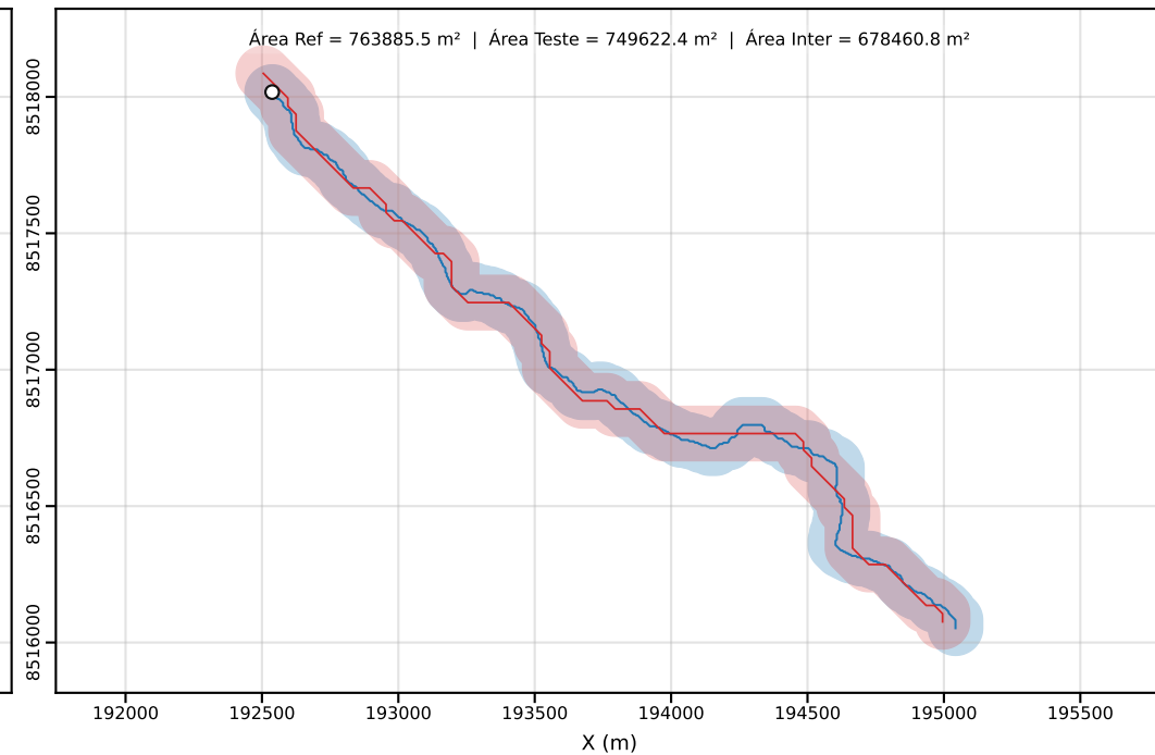
Classe D | PEC-PCD (Horizontal)=100.00 m | dm = 35.80
