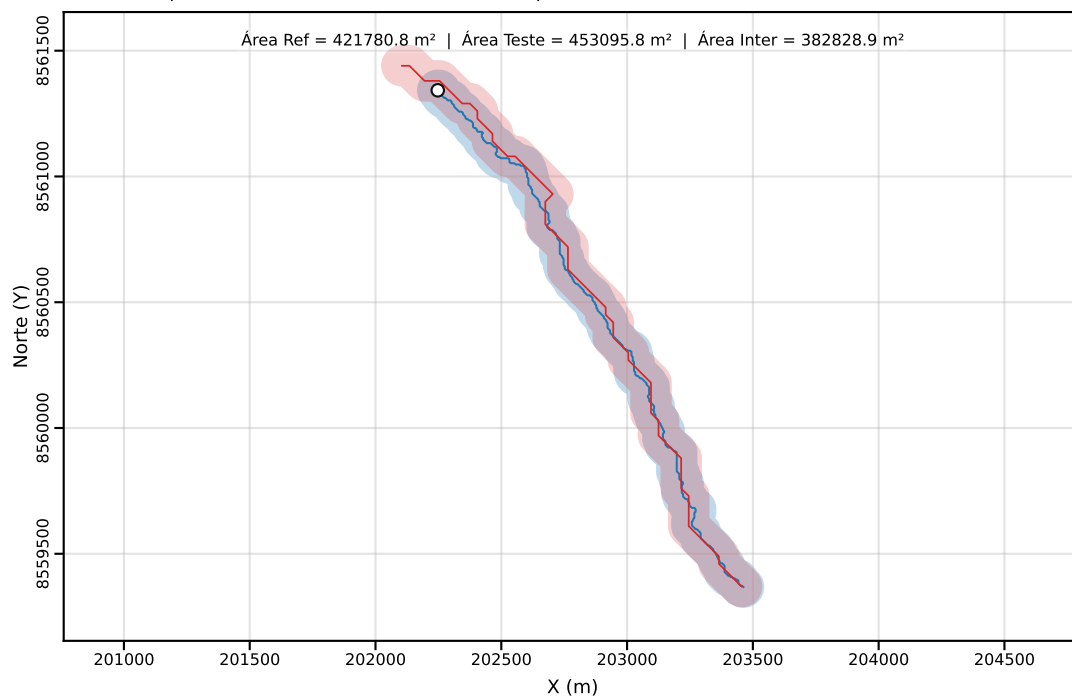
Classe C | PEC-PCD (Horizontal)=80.00 m | dm = 21.61
