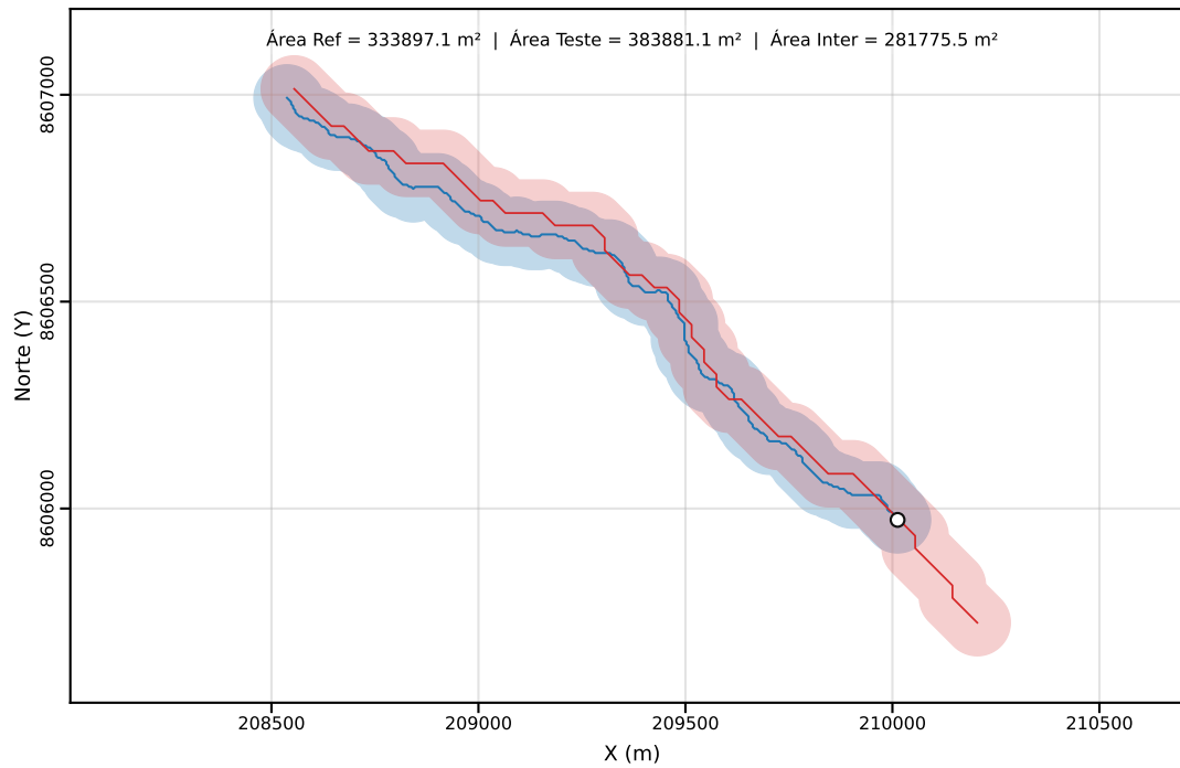
Classe C | PEC-PCD (Horizontal)=80.00 m | dm = 34.12
