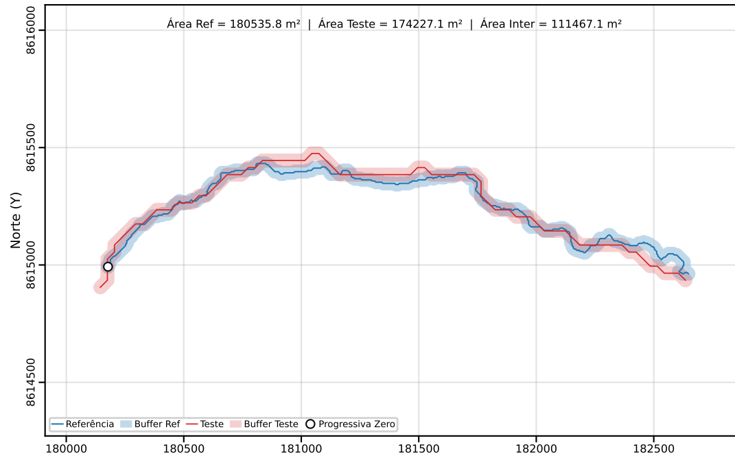
Classe C | PEC-PCD (Horizontal)=80.00 m | dm = 36.59
