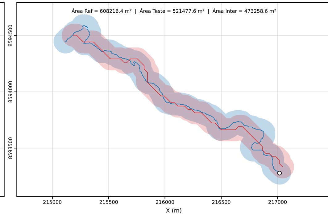
Classe D | PEC-PCD (Horizontal)=100.00 m | dm = 81.30
