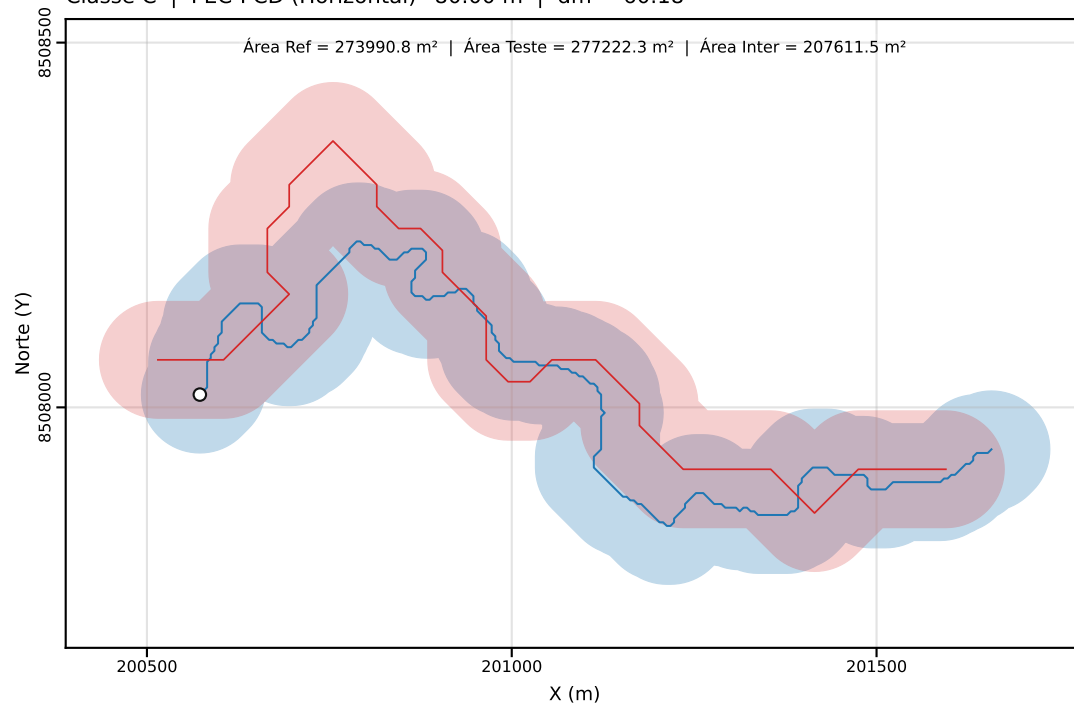
Classe C | PEC-PCD (Horizontal)=80.00 m | dm = 60.18
