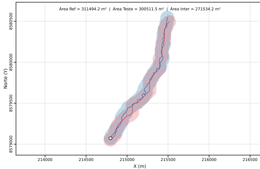
Classe C | PEC-PCD (Horizontal)=80.00 m | dm = 33.42
