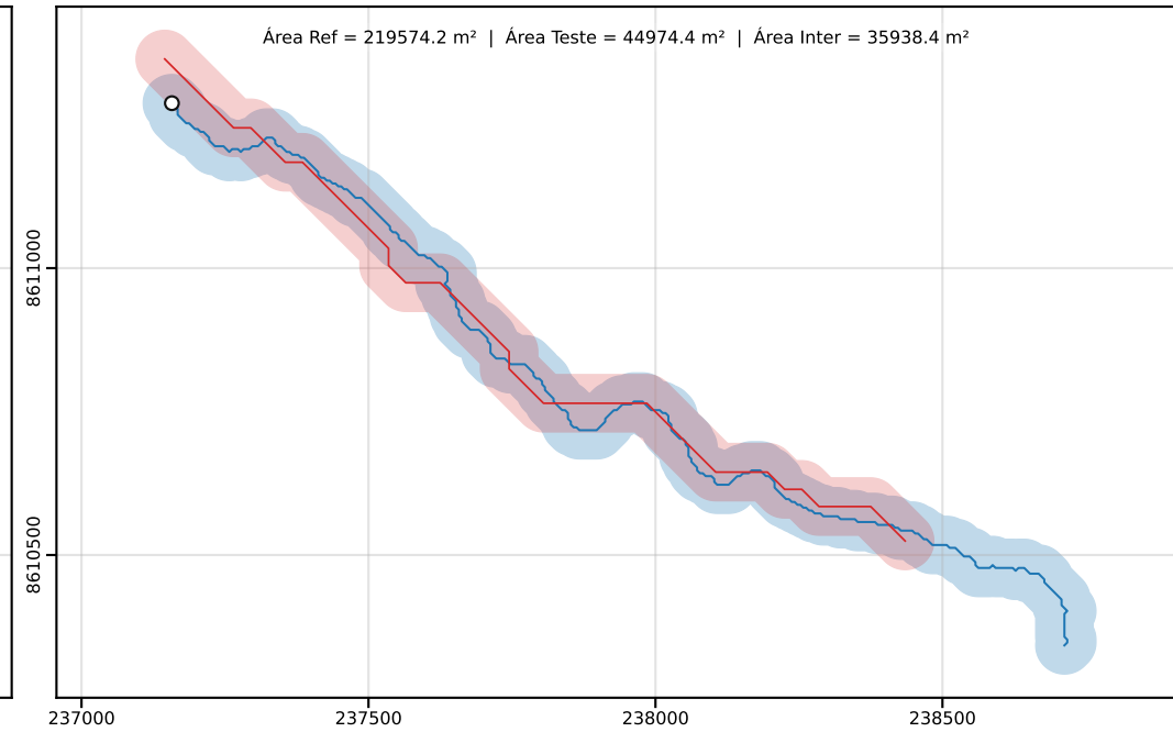
Classe D | PEC-PCD (Horizontal)=100.00 m | dm = 1049.74
