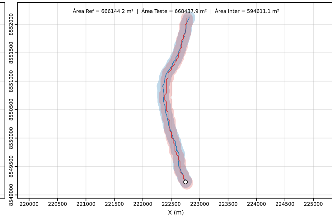
Classe D | PEC-PCD (Horizontal)=100.00 m | dm = 33.62
