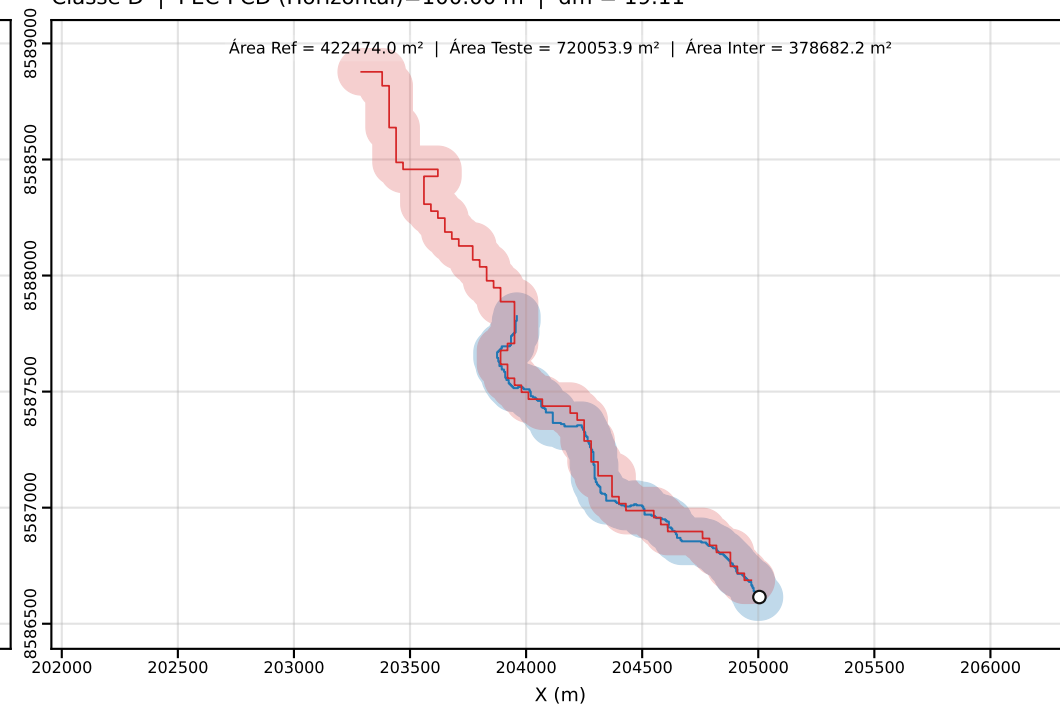
Classe D | PEC-PCD (Horizontal)=100.00 m | dm = 19.11
