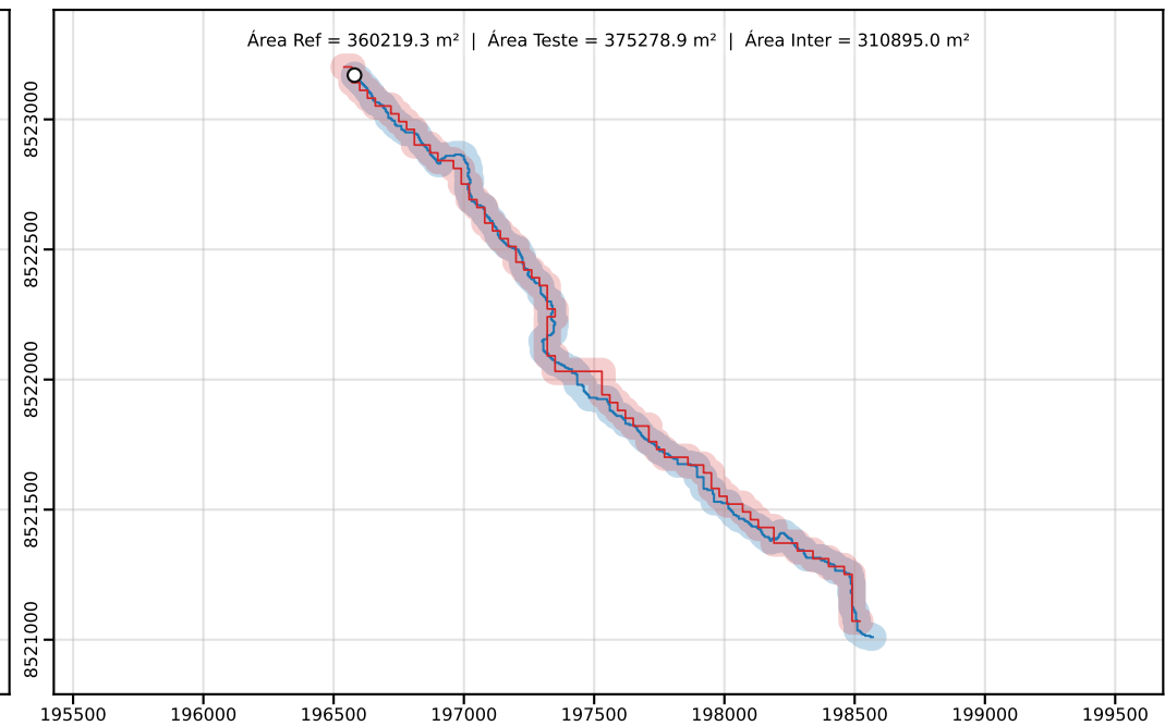
Classe D | PEC-PCD (Horizontal)=100.00 m | dm = 23.58
