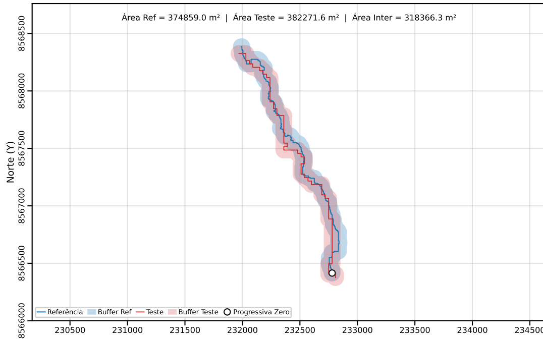
Classe C | PEC-PCD (Horizontal)=200.00 m | dm = 36.95
