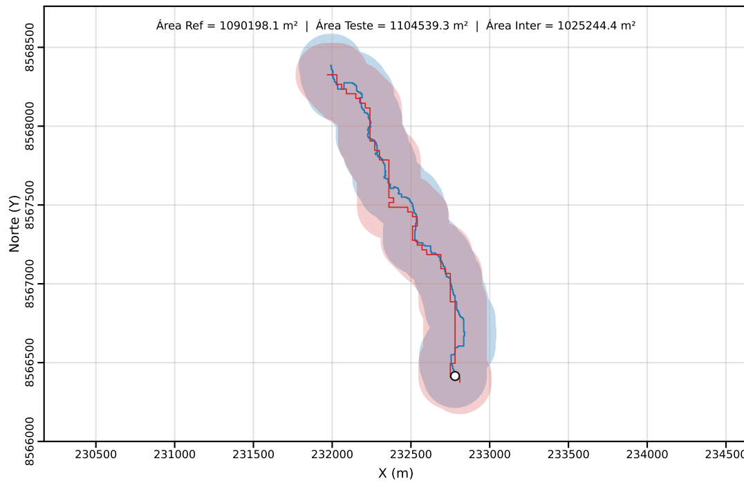
Classe C | PEC-PCD (Horizontal)=200.00 m | dm = 36.95
