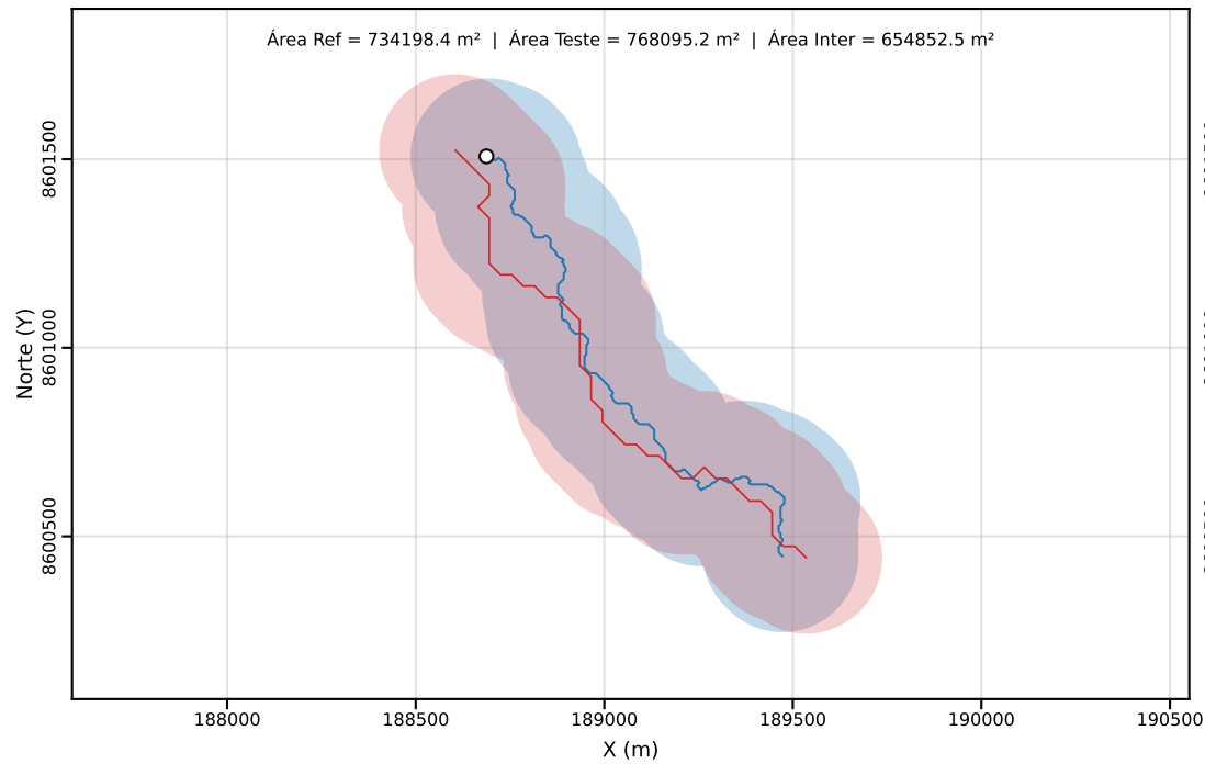
Classe C | PEC-PCD (Horizontal)=200.00 m | dm = 64.91
