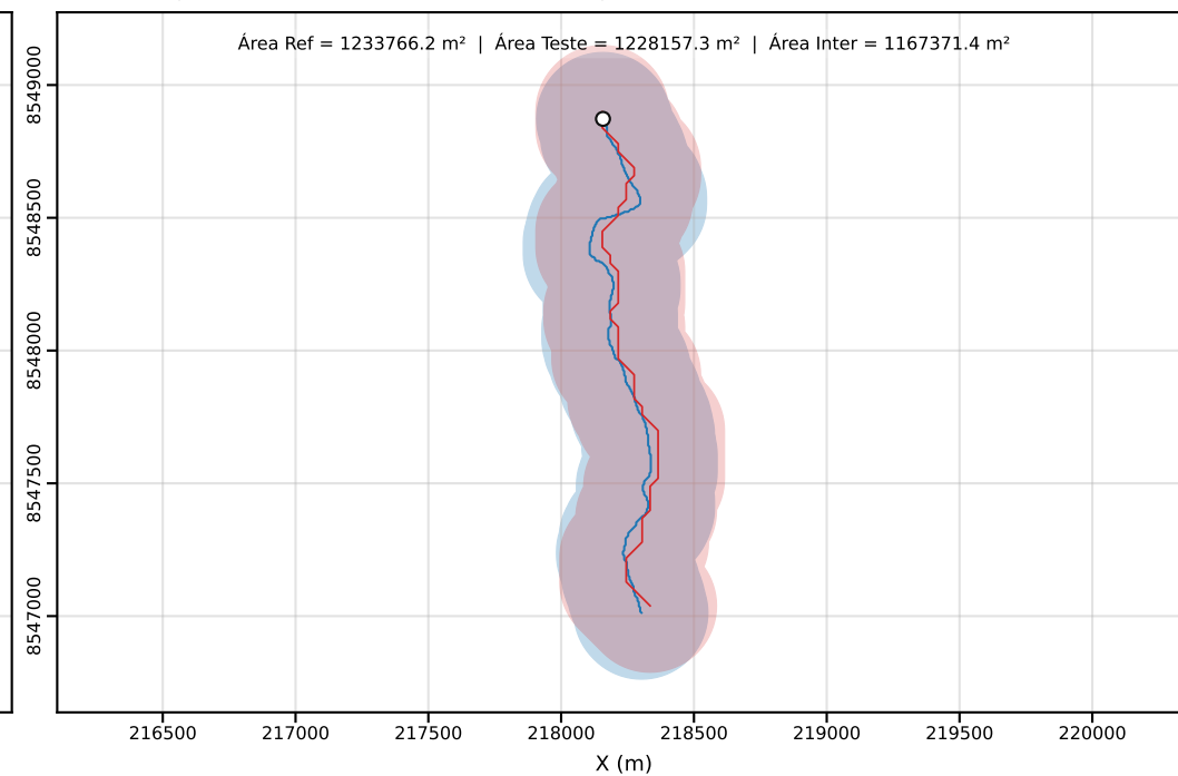
Classe D | PEC-PCD (Horizontal)=250.00 m | dm = 42.46
