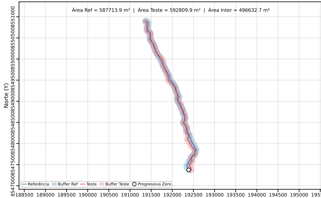
Classe C | PEC-PCD (Horizontal)=200.00 m | dm = 36.85
