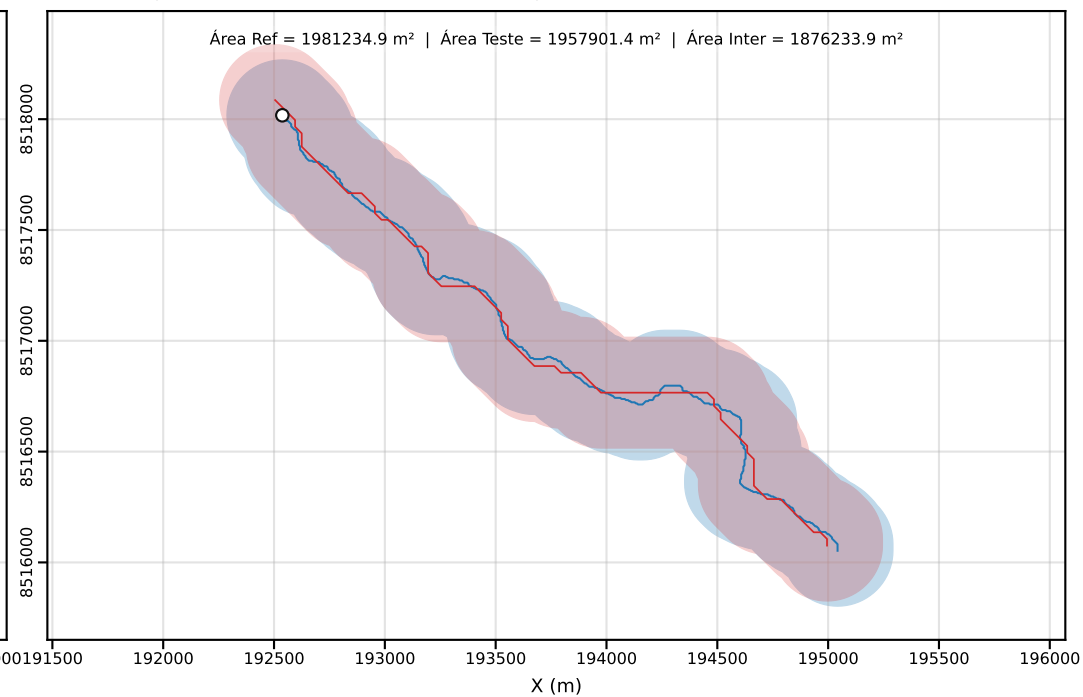
Classe D | PEC-PCD (Horizontal)=250.00 m | dm = 42.12
