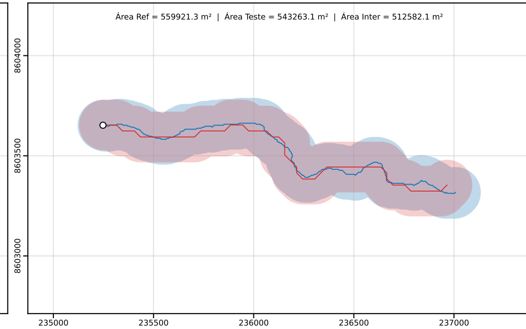
Classe D | PEC-PCD (Horizontal)=250.00 m | dm = 38.70
