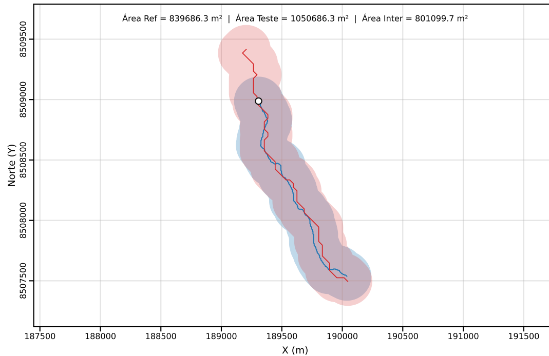
Classe C | PEC-PCD (Horizontal)=200.00 m | dm = 23.08
