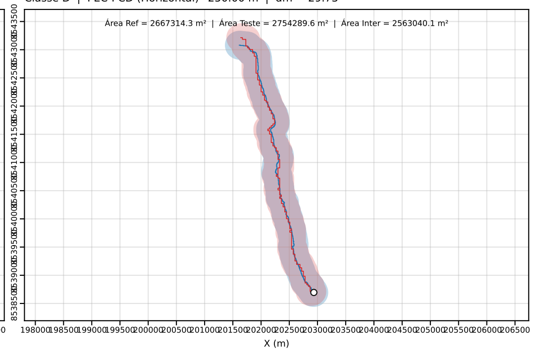
Classe D | PEC-PCD (Horizontal)=250.00 m | dm = 29.73
