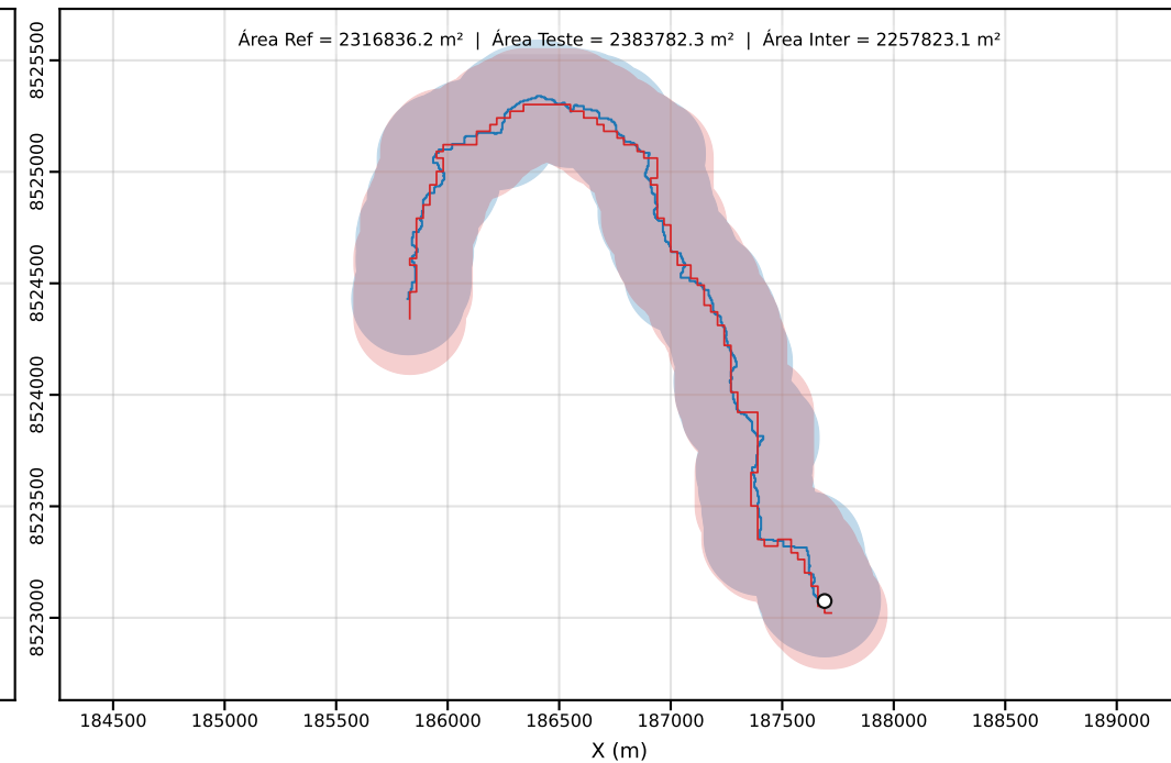
Classe D | PEC-PCD (Horizontal)=250.00 m | dm = 19.44
