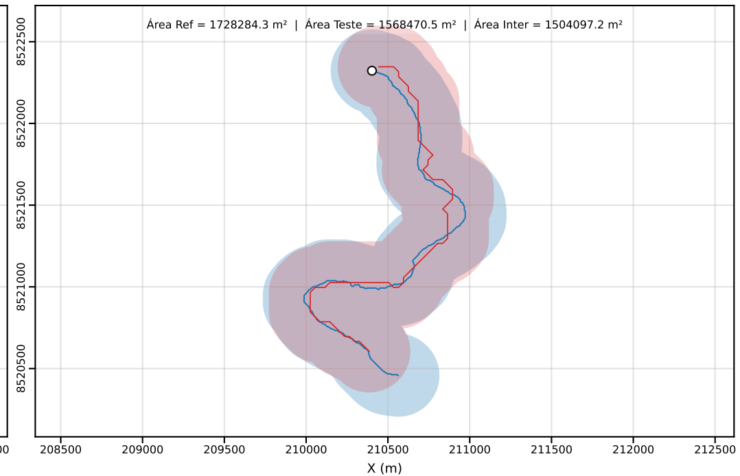
Classe D | PEC-PCD (Horizontal)=250.00 m | dm = 112.26
