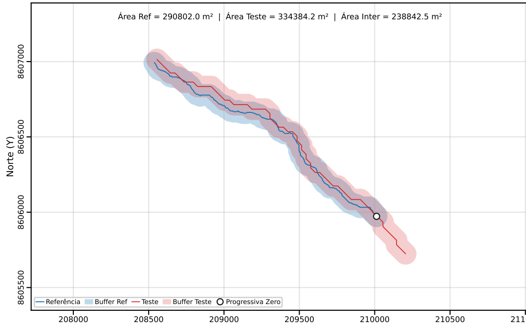
Classe C | PEC-PCD (Horizontal)=200.00 m | dm = 34.13
