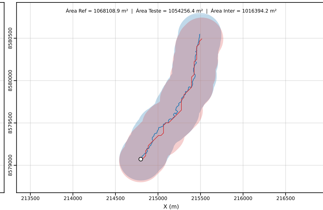
Classe D | PEC-PCD (Horizontal)=250.00 m | dm = 38.53
