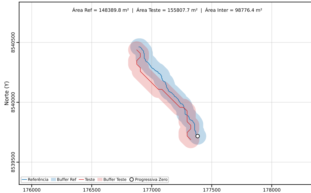
Classe C | PEC-PCD (Horizontal)=200.00 m | dm = 69.81
