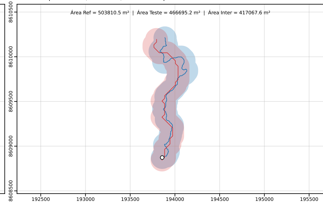
Classe D | PEC-PCD (Horizontal)=250.00 m | dm = 75.89
