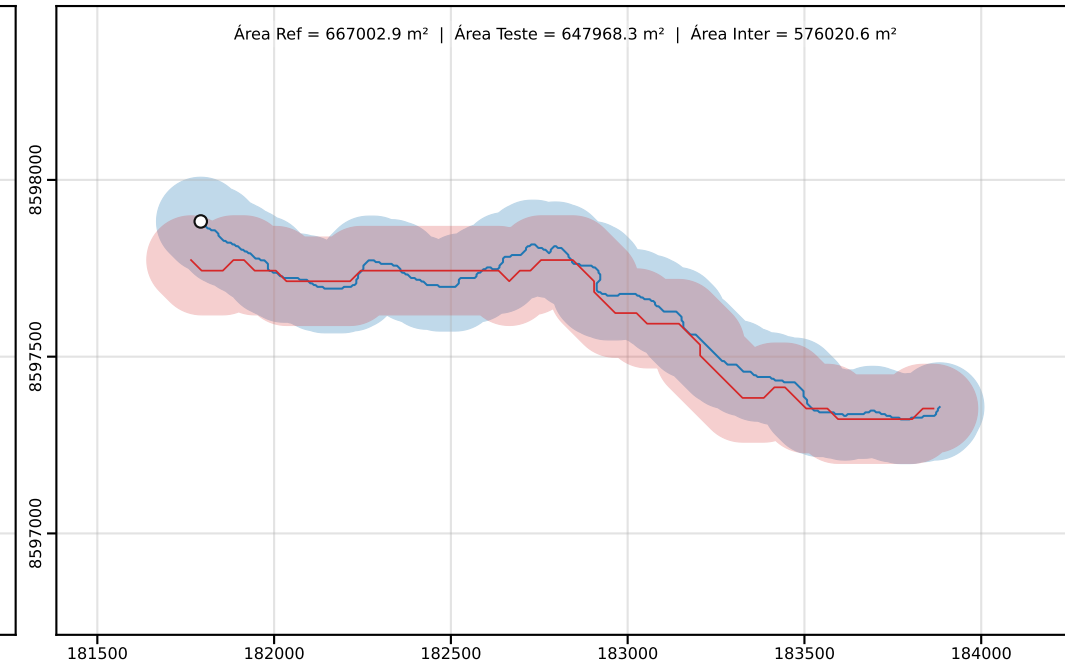
Classe D | PEC-PCD (Horizontal)=250.00 m | dm = 65.00
