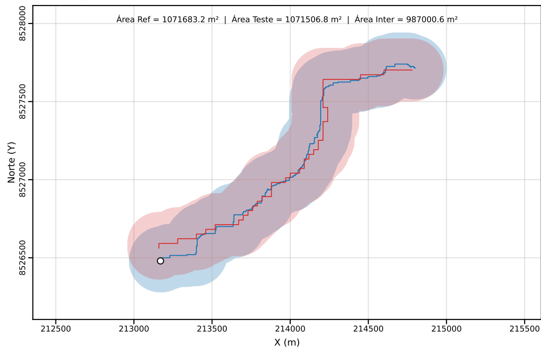
Classe C | PEC-PCD (Horizontal)=200.00 m | dm = 49.66
