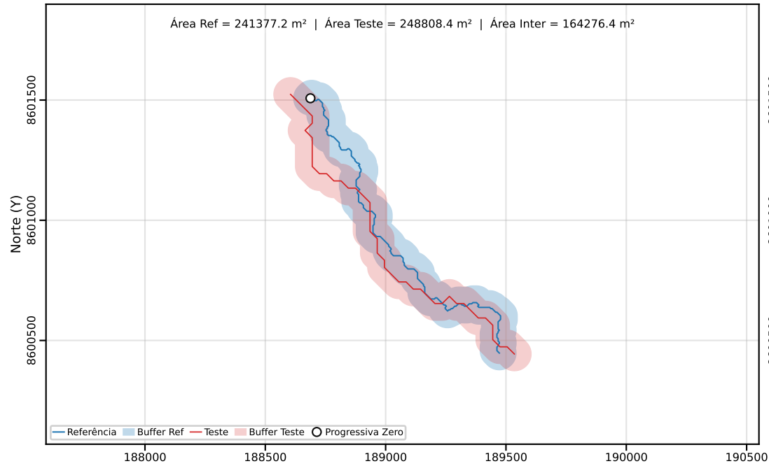
Classe C | PEC-PCD (Horizontal)=200.00 m | dm = 64.91
