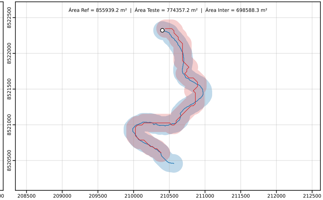
Classe D | PEC-PCD (Horizontal)=250.00 m | dm = 112.26
