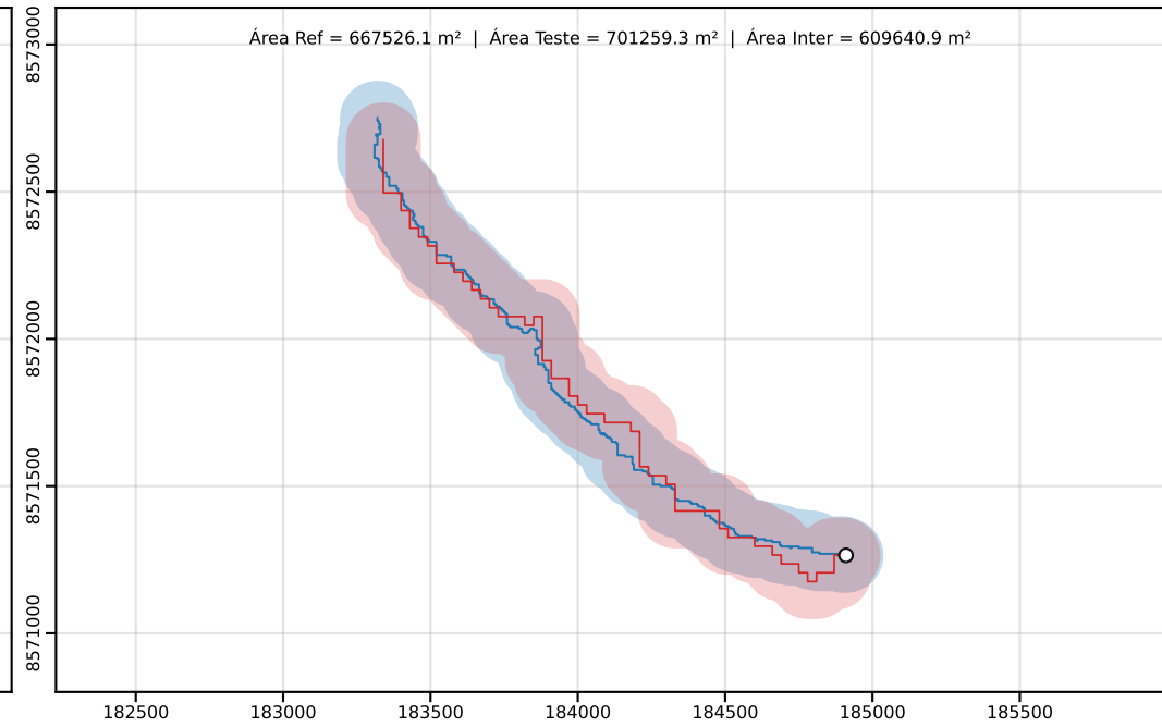
Classe D | PEC-PCD (Horizontal)=250.00 m | dm = 39.83
