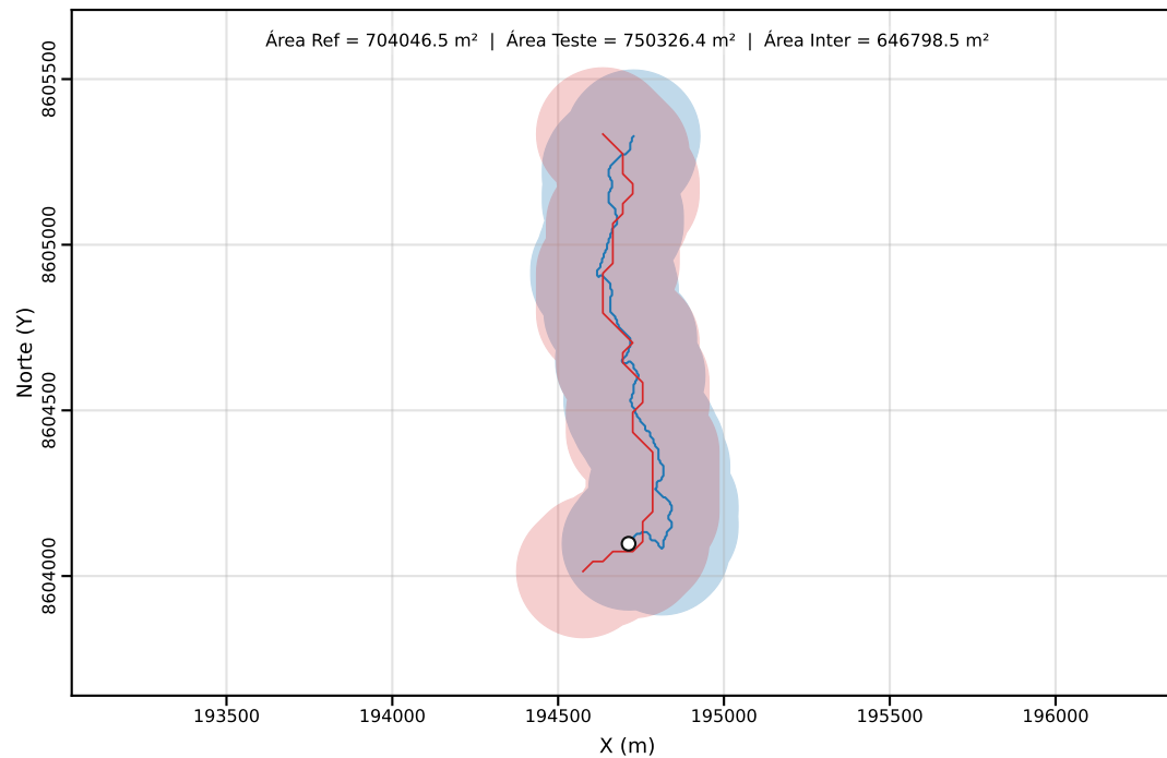
Classe C | PEC-PCD (Horizontal)=200.00 m | dm = 47.94
