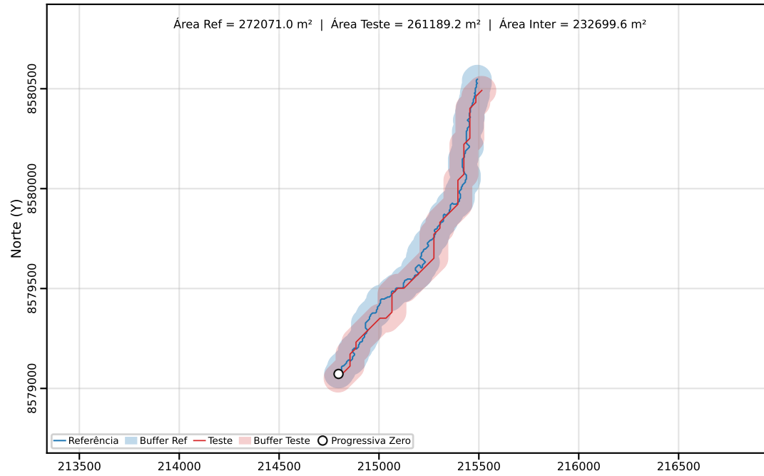
Classe C | PEC-PCD (Horizontal)=200.00 m | dm = 36.98
