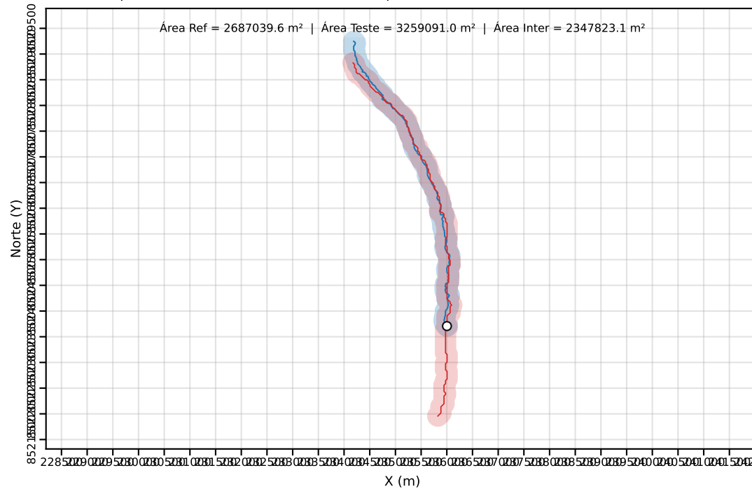
Classe C | PEC-PCD (Horizontal)=200.00 m | dm = 65.40
