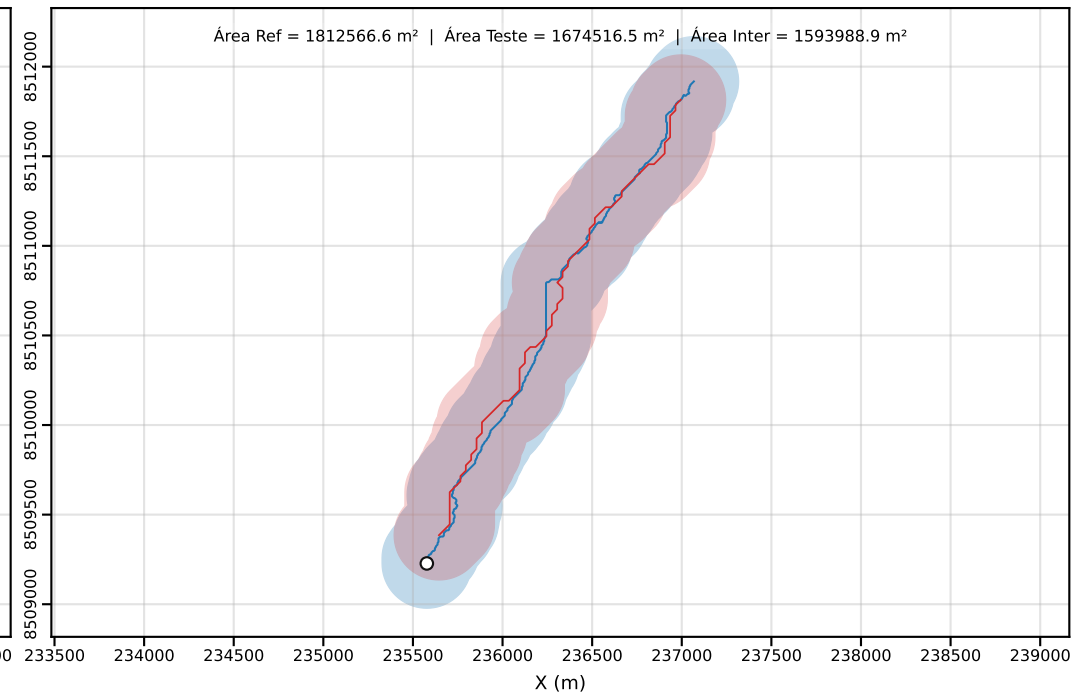
Classe D | PEC-PCD (Horizontal)=250.00 m | dm = 102.52
