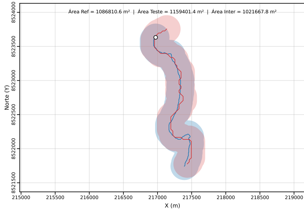
Classe C | PEC-PCD (Horizontal)=200.00 m | dm = 35.30
