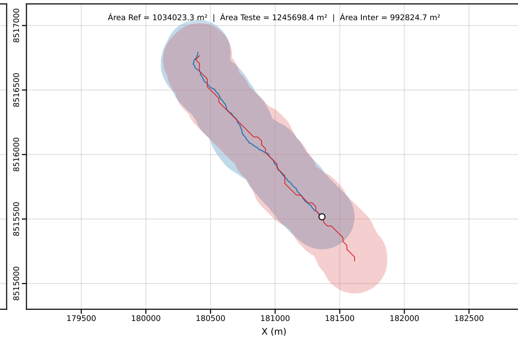
Classe D | PEC-PCD (Horizontal)=250.00 m | dm = 25.98
