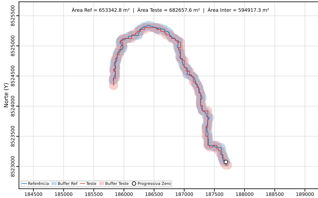
Classe C | PEC-PCD (Horizontal)=200.00 m | dm = 19.34
