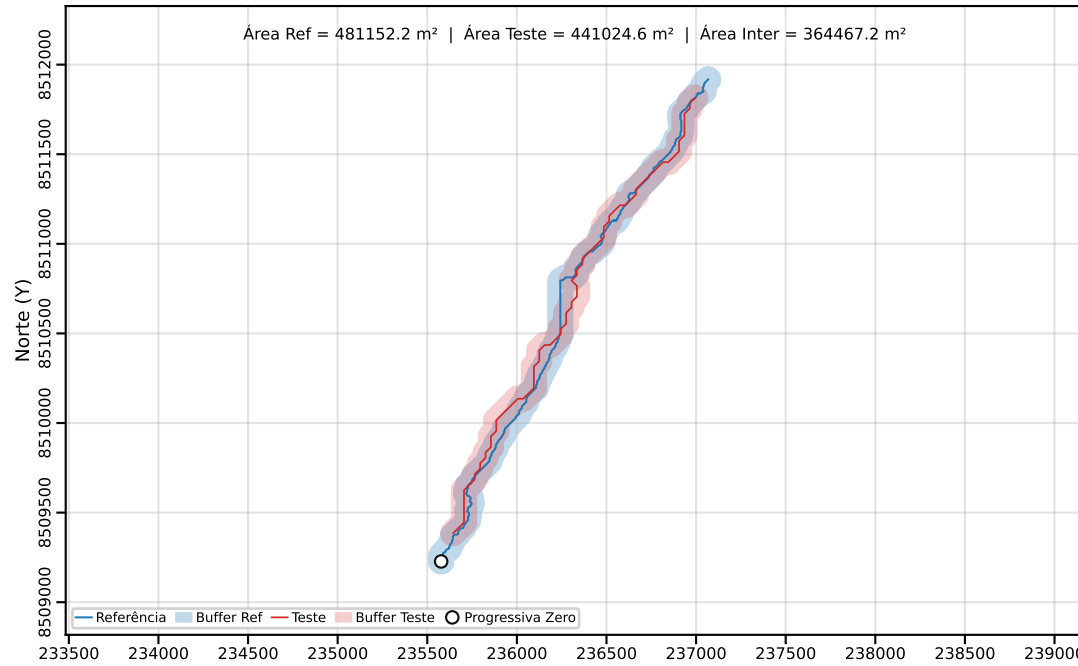
Classe C | PEC-PCD (Horizontal)=200.00 m | dm = 90.65
