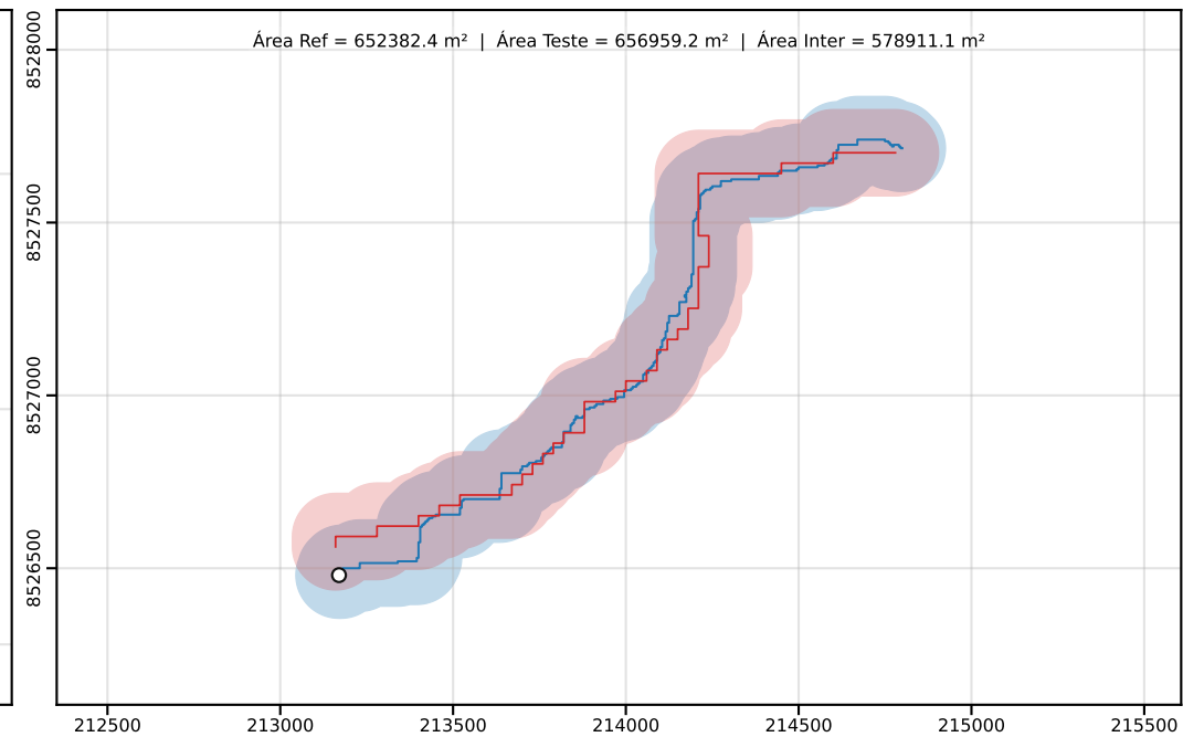
Classe D | PEC-PCD (Horizontal)=250.00 m | dm = 53.24
