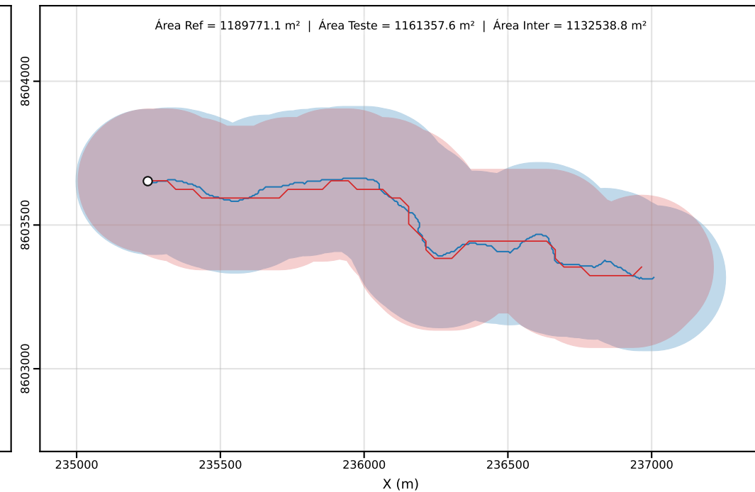
Classe D | PEC-PCD (Horizontal)=250.00 m | dm = 38.70
