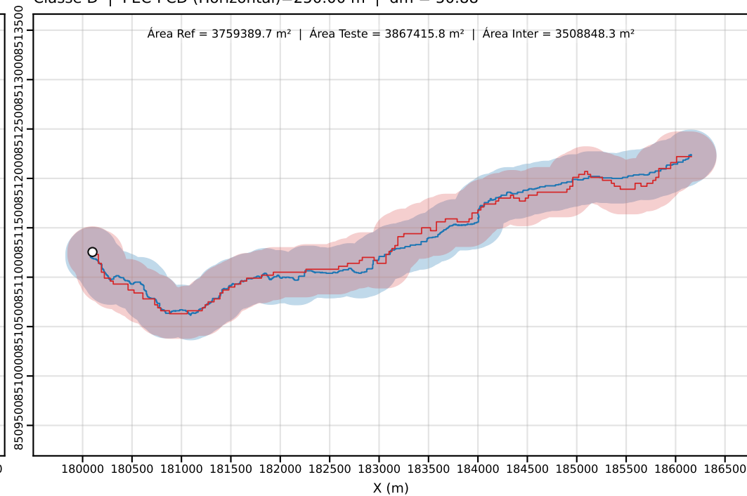
Classe D | PEC-PCD (Horizontal)=250.00 m | dm = 50.88
