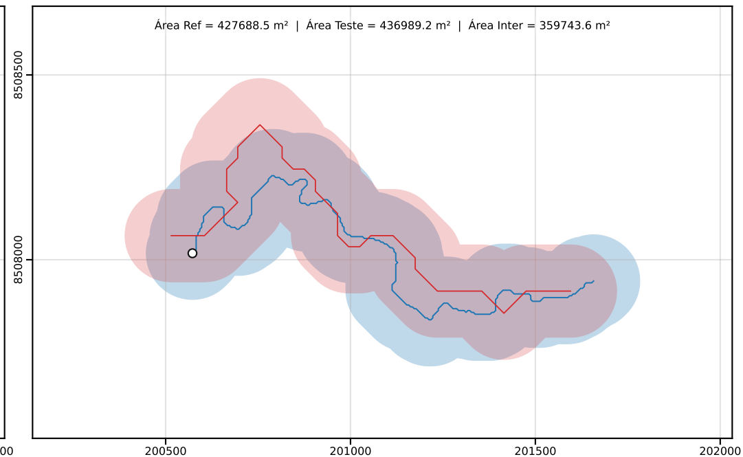
Classe D | PEC-PCD (Horizontal)=250.00 m | dm = 72.02
