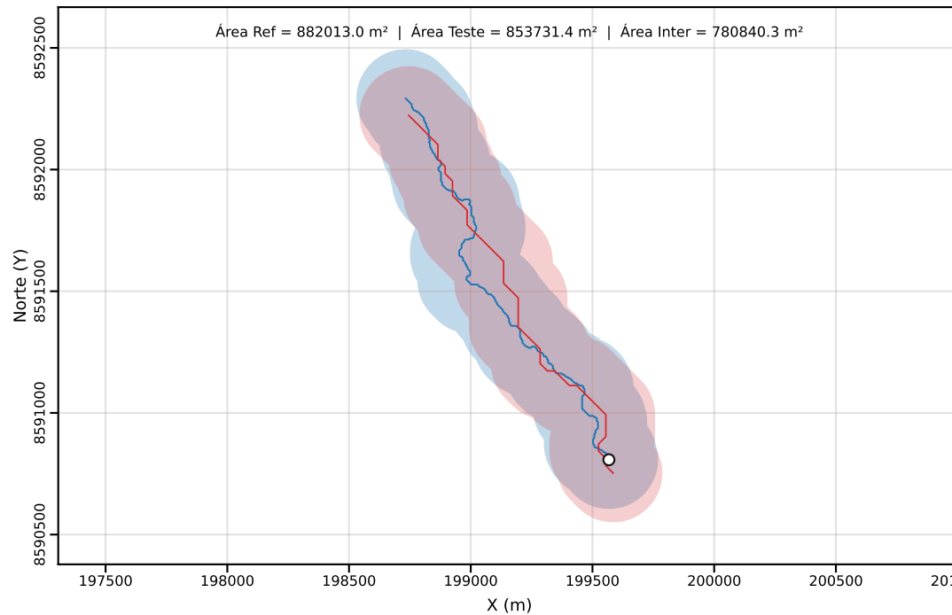
Classe C | PEC-PCD (Horizontal)=200.00 m | dm = 74.46
