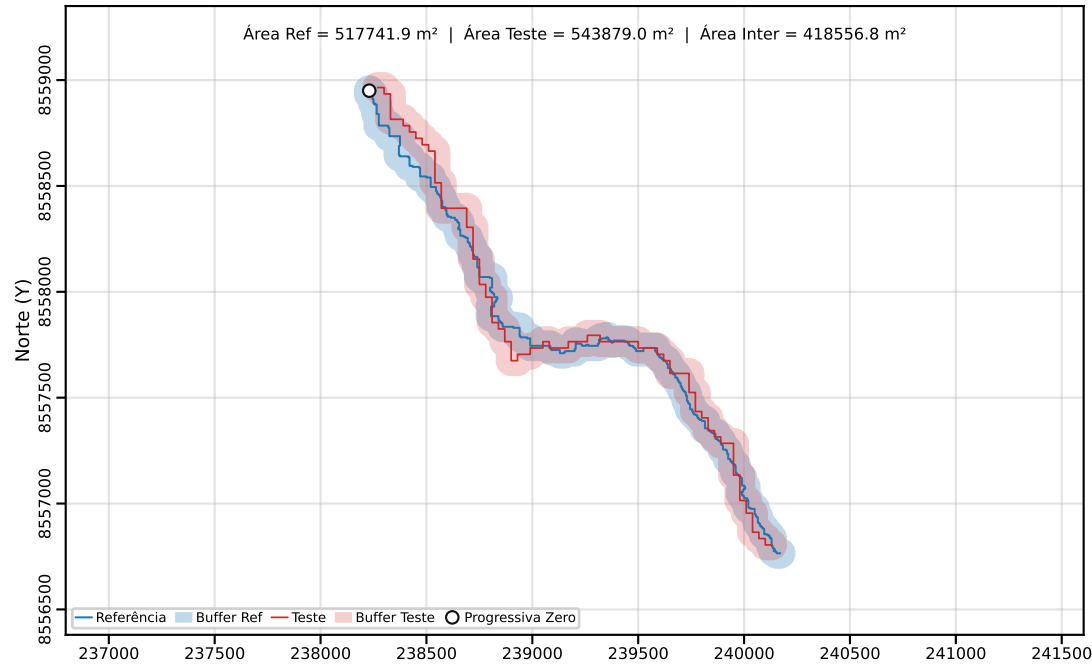
Classe C | PEC-PCD (Horizontal)=200.00 m | dm = 42.58
