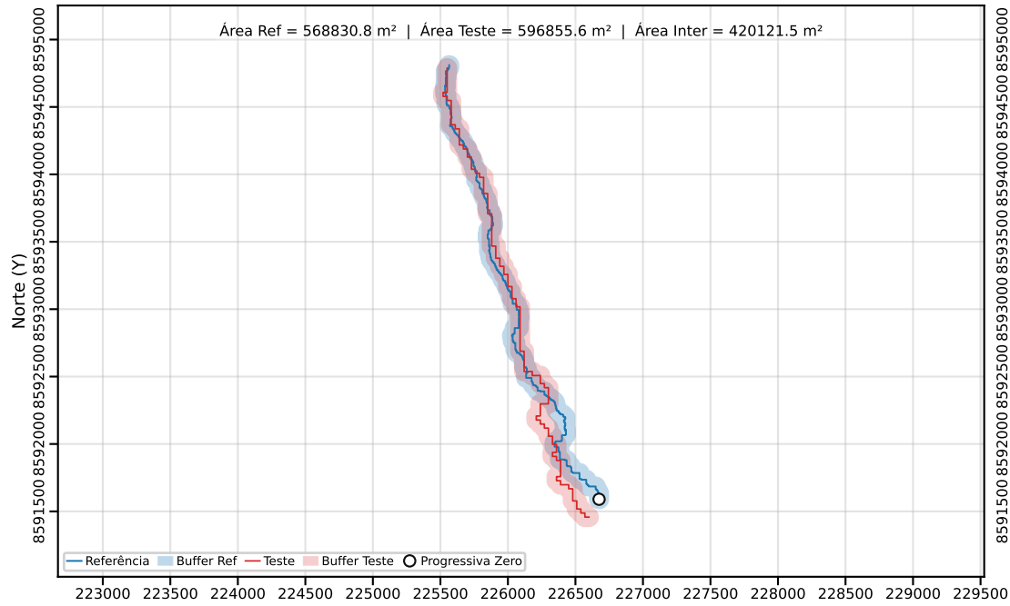
Classe C | PEC-PCD (Horizontal)=200.00 m | dm = 61.79
