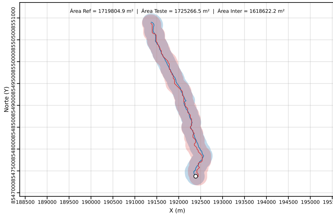
Classe C | PEC-PCD (Horizontal)=200.00 m | dm = 36.85
