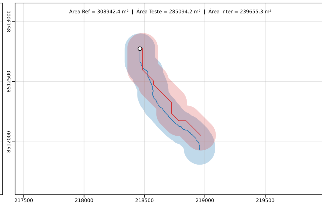
Classe D | PEC-PCD (Horizontal)=250.00 m | dm = 115.66
