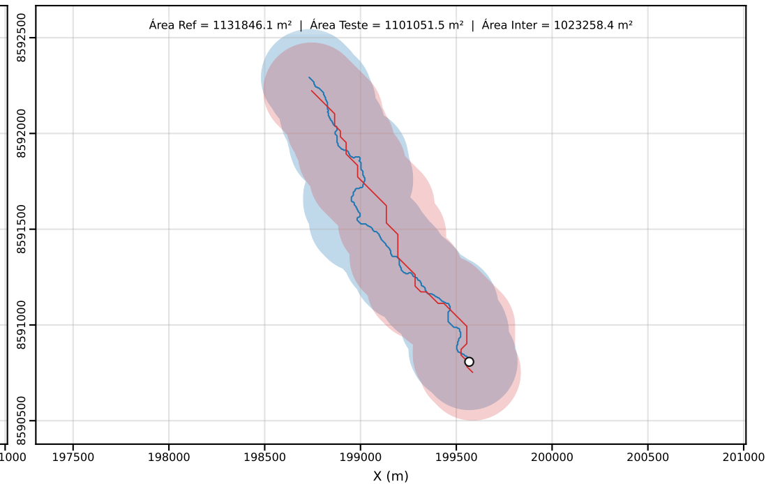
Classe D | PEC-PCD (Horizontal)=250.00 m | dm = 77.46
