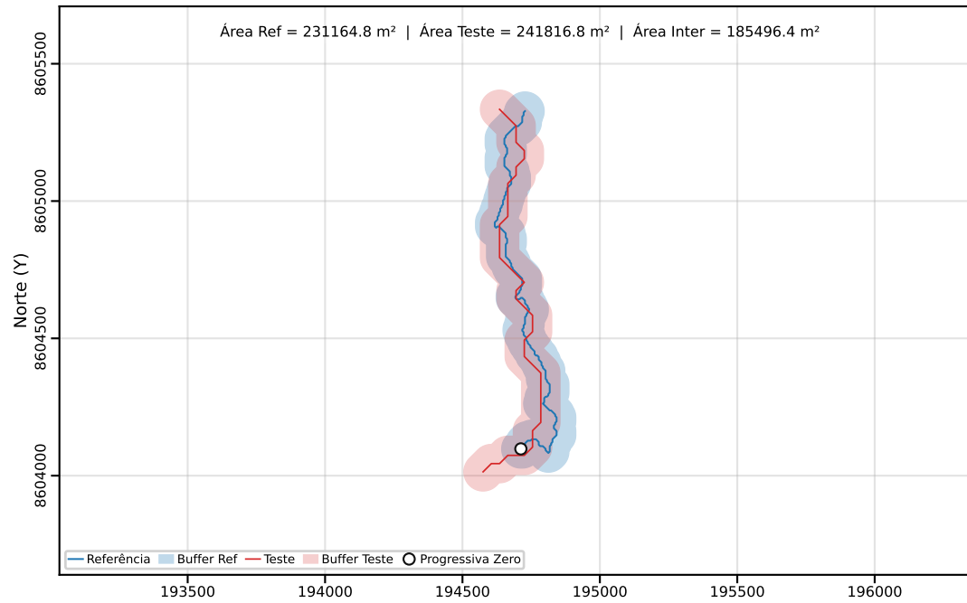
Classe C | PEC-PCD (Horizontal)=200.00 m | dm = 47.94
