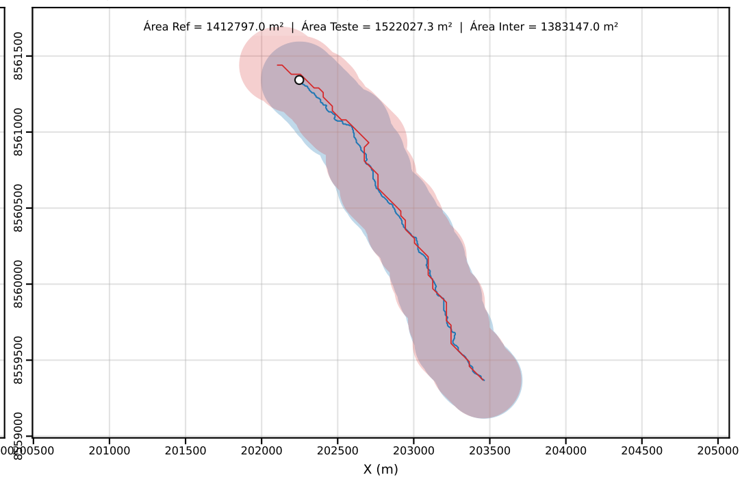
Classe D | PEC-PCD (Horizontal)=250.00 m | dm = 15.30
