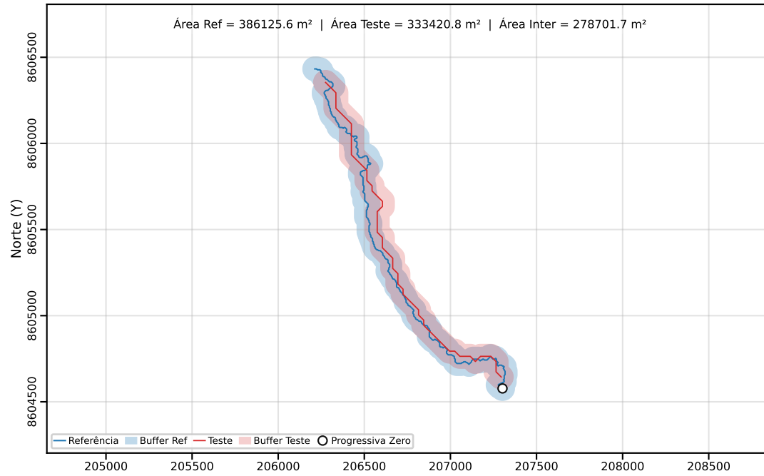
Classe C | PEC-PCD (Horizontal)=200.00 m | dm = 97.24
