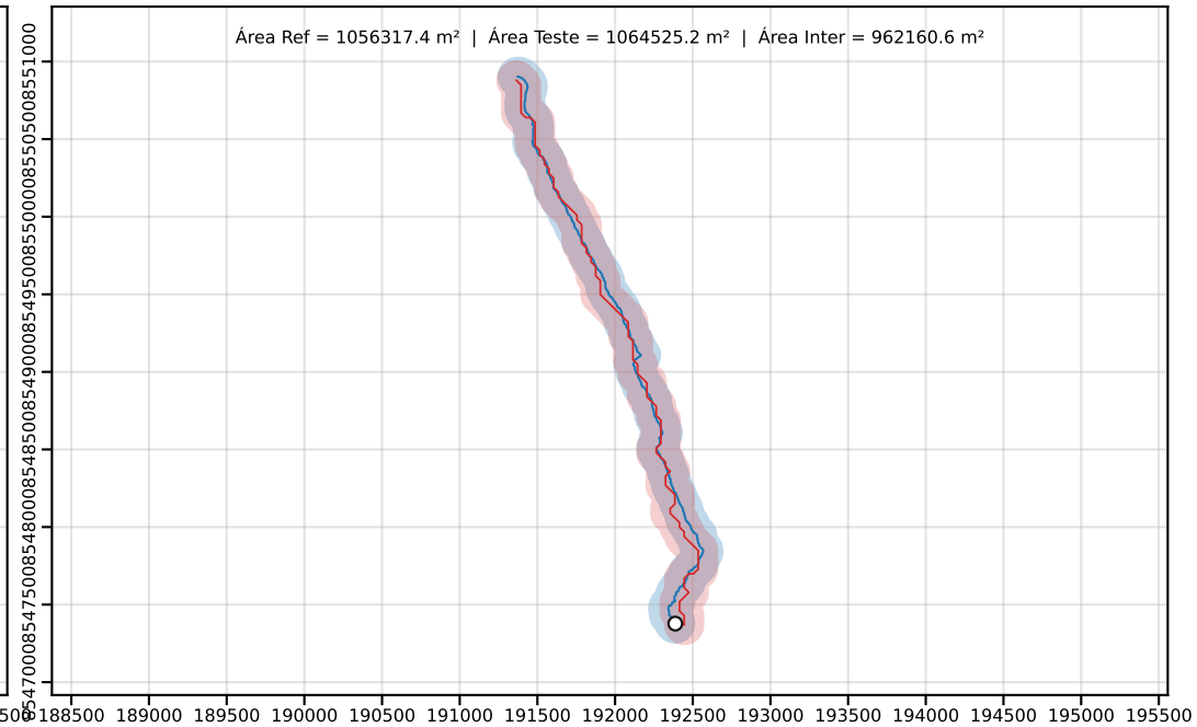
Classe D | PEC-PCD (Horizontal)=250.00 m | dm = 38.47
