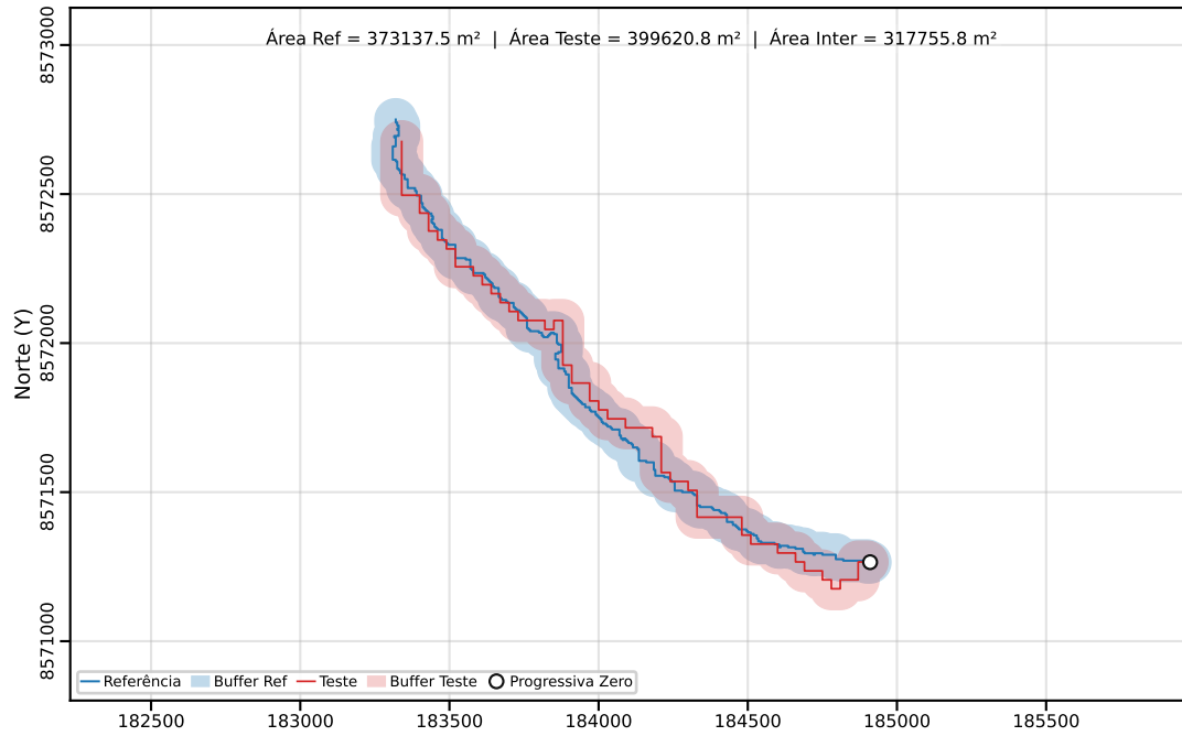
Classe C | PEC-PCD (Horizontal)=200.00 m | dm = 36.56
