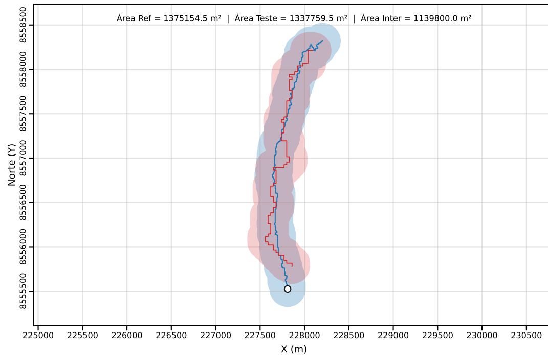
Classe C | PEC-PCD (Horizontal)=200.00 m | dm = 110.54
