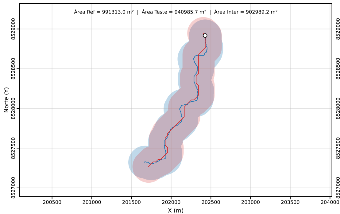
Classe C | PEC-PCD (Horizontal)=200.00 m | dm = 58.98
