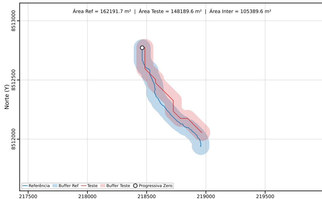
Classe C | PEC-PCD (Horizontal)=200.00 m | dm = 108.31
