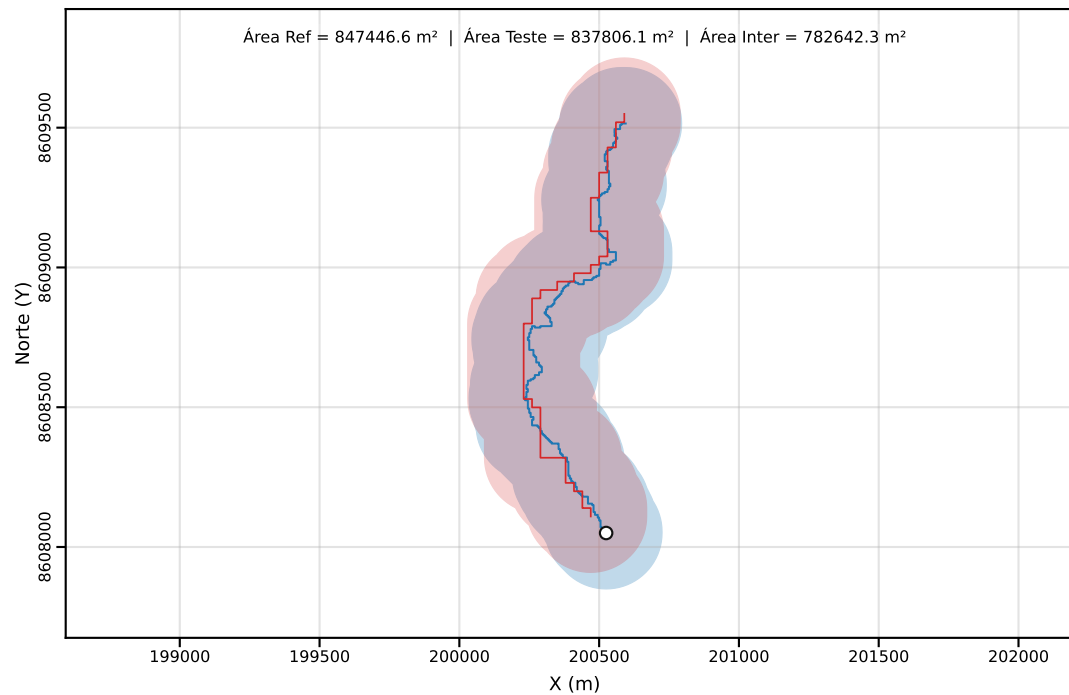
Classe C | PEC-PCD (Horizontal)=200.00 m | dm = 48.60
