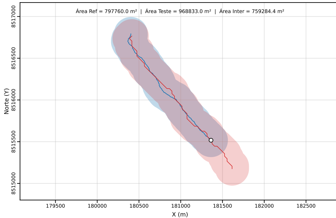
Classe C | PEC-PCD (Horizontal)=200.00 m | dm = 24.95
