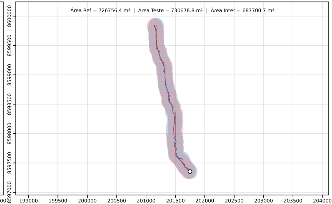
Classe D | PEC-PCD (Horizontal)=250.00 m | dm = 20.89
