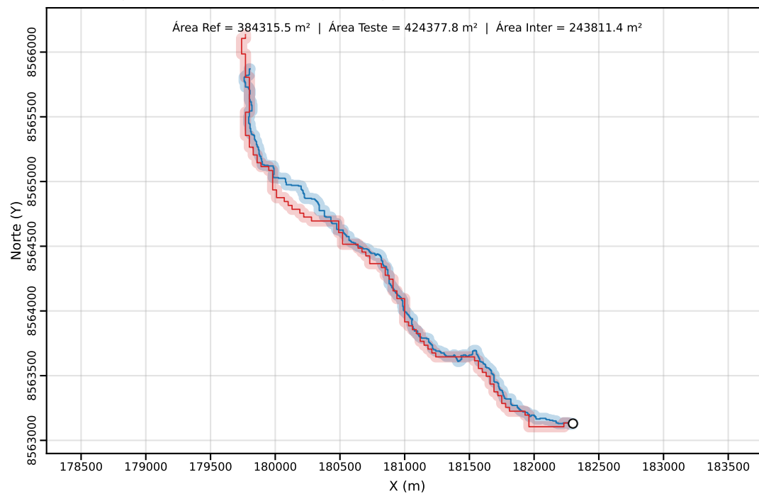
Classe C | PEC-PCD (Horizontal)=40.00 m | dm = 41.61
