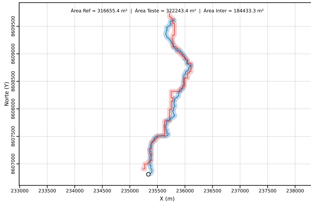
Classe C | PEC-PCD (Horizontal)=40.00 m | dm = 51.56
