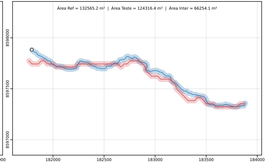
Classe D | PEC-PCD (Horizontal)=50.00 m | dm = 48.22
