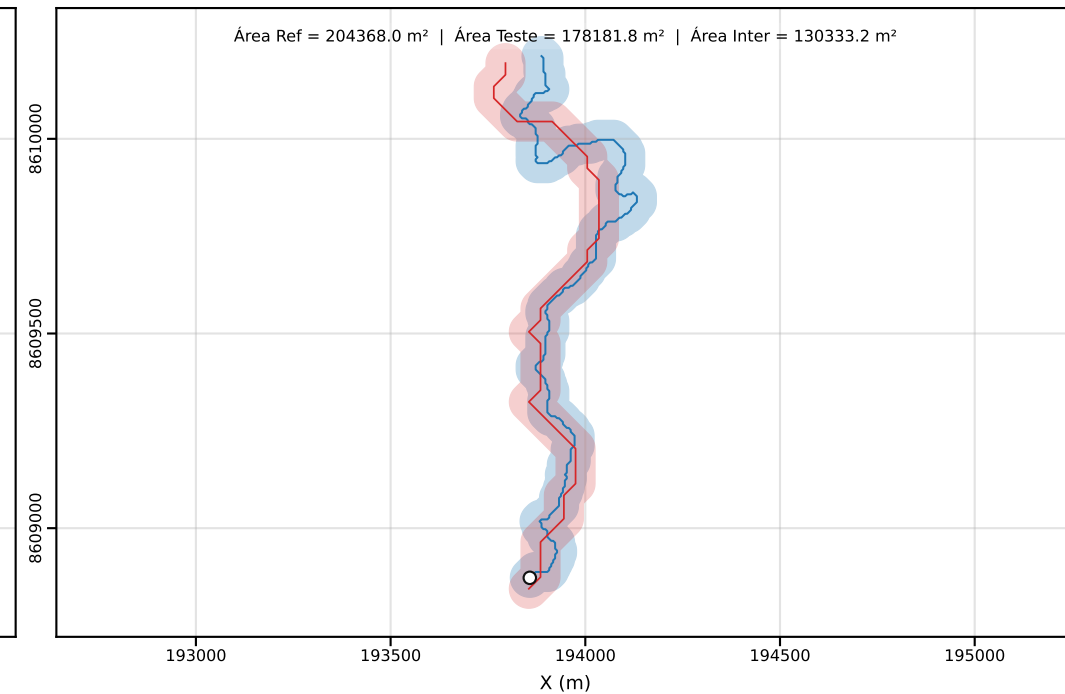
Classe D | PEC-PCD (Horizontal)=50.00 m | dm = 65.27
