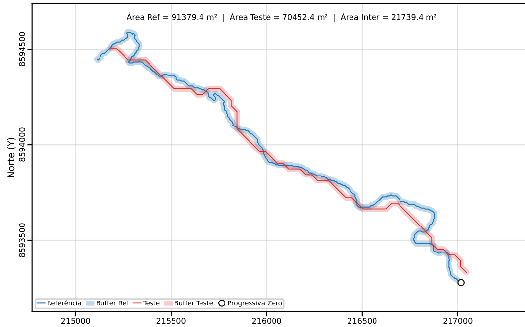
Classe C | PEC-PCD (Horizontal)=40.00 m | dm = 66.80
