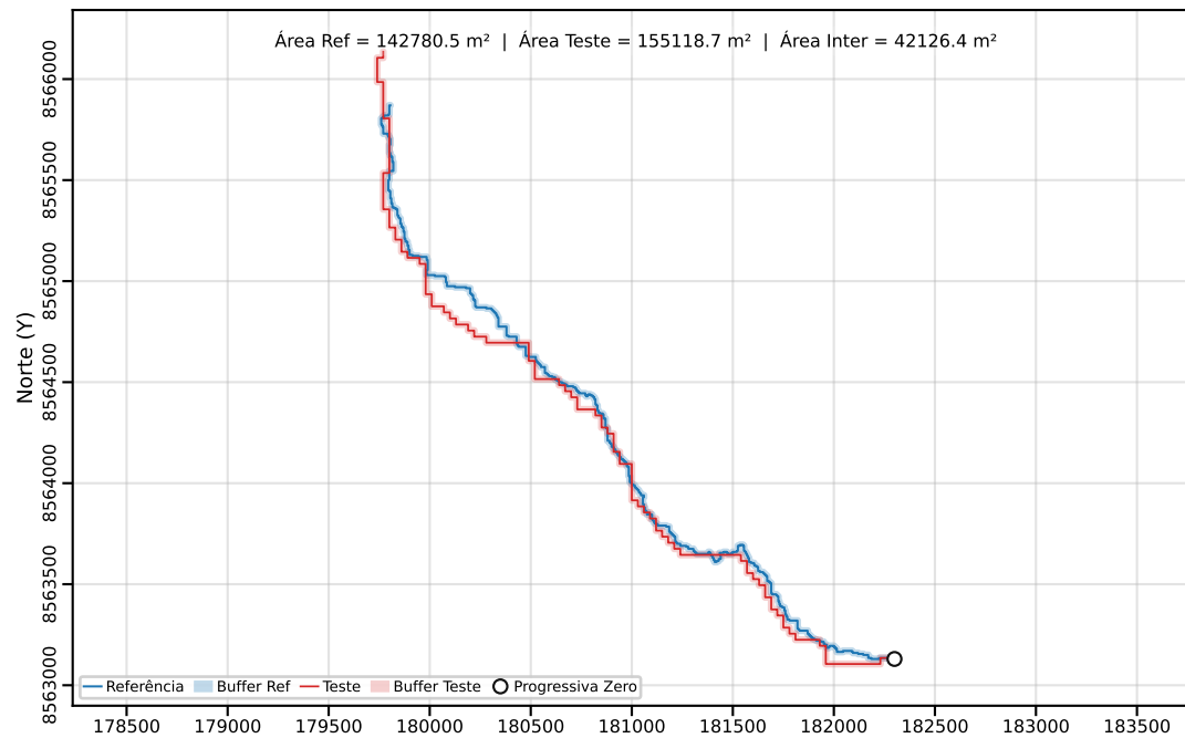
Classe C | PEC-PCD (Horizontal)=40.00 m | dm = 41.61
