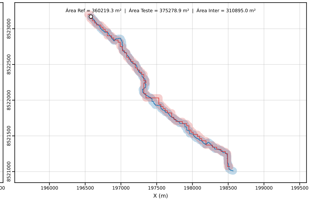
Classe D | PEC-PCD (Horizontal)=50.00 m | dm = 20.65
