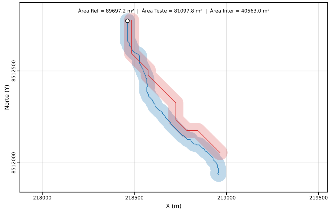
Classe C | PEC-PCD (Horizontal)=40.00 m | dm = 76.14
