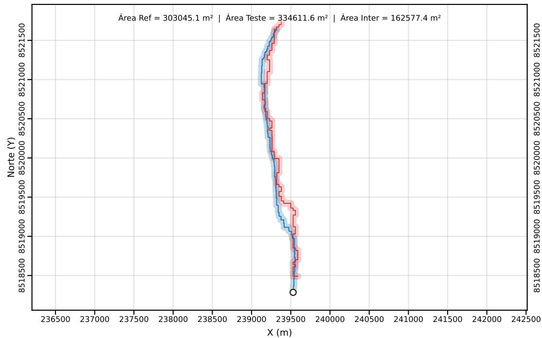
Classe C | PEC-PCD (Horizontal)=40.00 m | dm = 52.75
