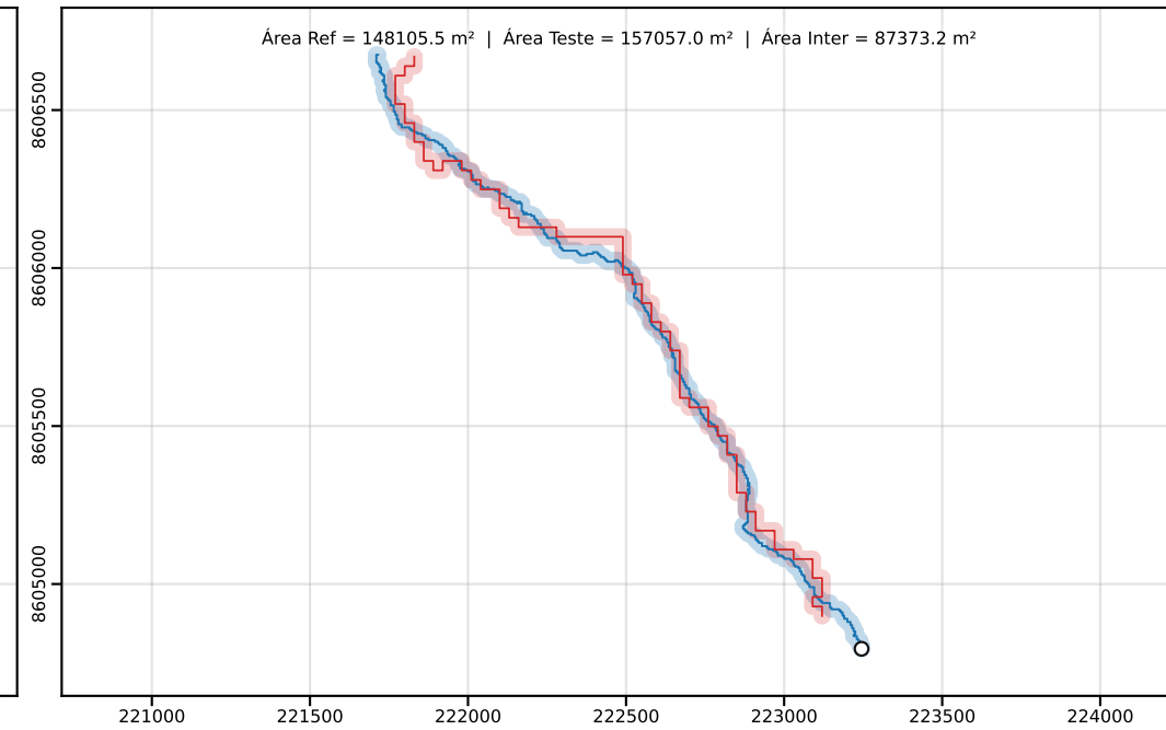
Classe D | PEC-PCD (Horizontal)=50.00 m | dm = 36.18
