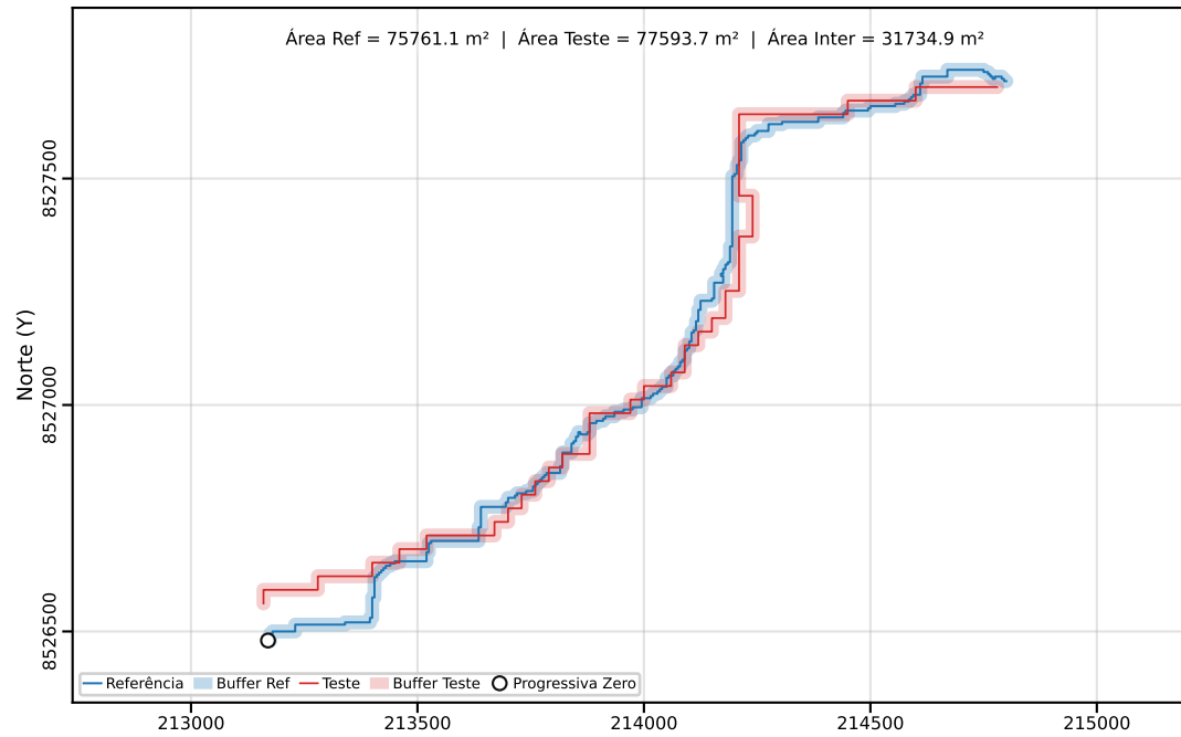
Classe C | PEC-PCD (Horizontal)=40.00 m | dm = 35.43
