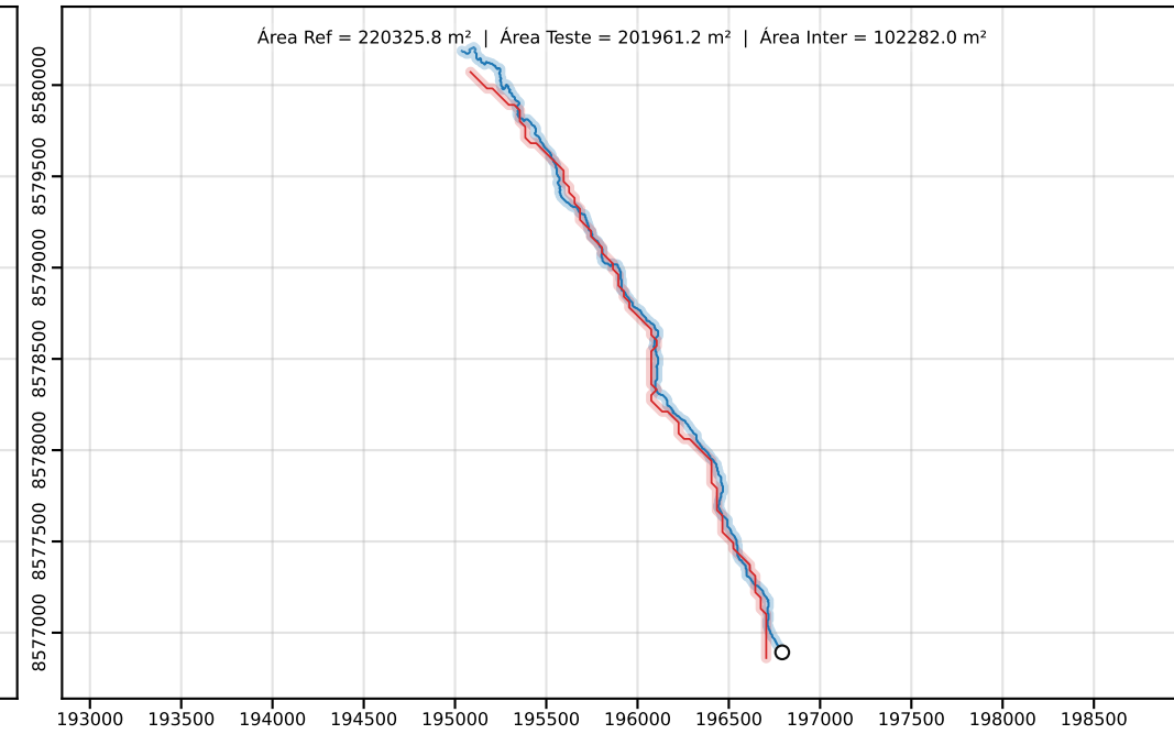
Classe D | PEC-PCD (Horizontal)=50.00 m | dm = 53.50
