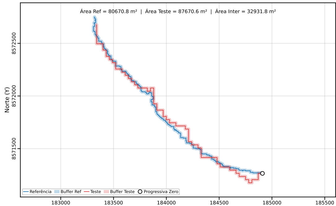
Classe C | PEC-PCD (Horizontal)=40.00 m | dm = 29.96
