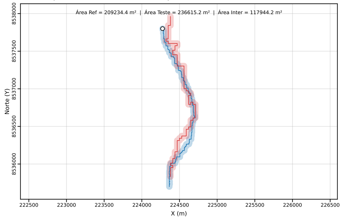
Classe C | PEC-PCD (Horizontal)=40.00 m | dm = 48.48
