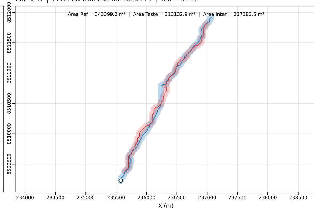
Classe D | PEC-PCD (Horizontal)=50.00 m | dm = 53.18
