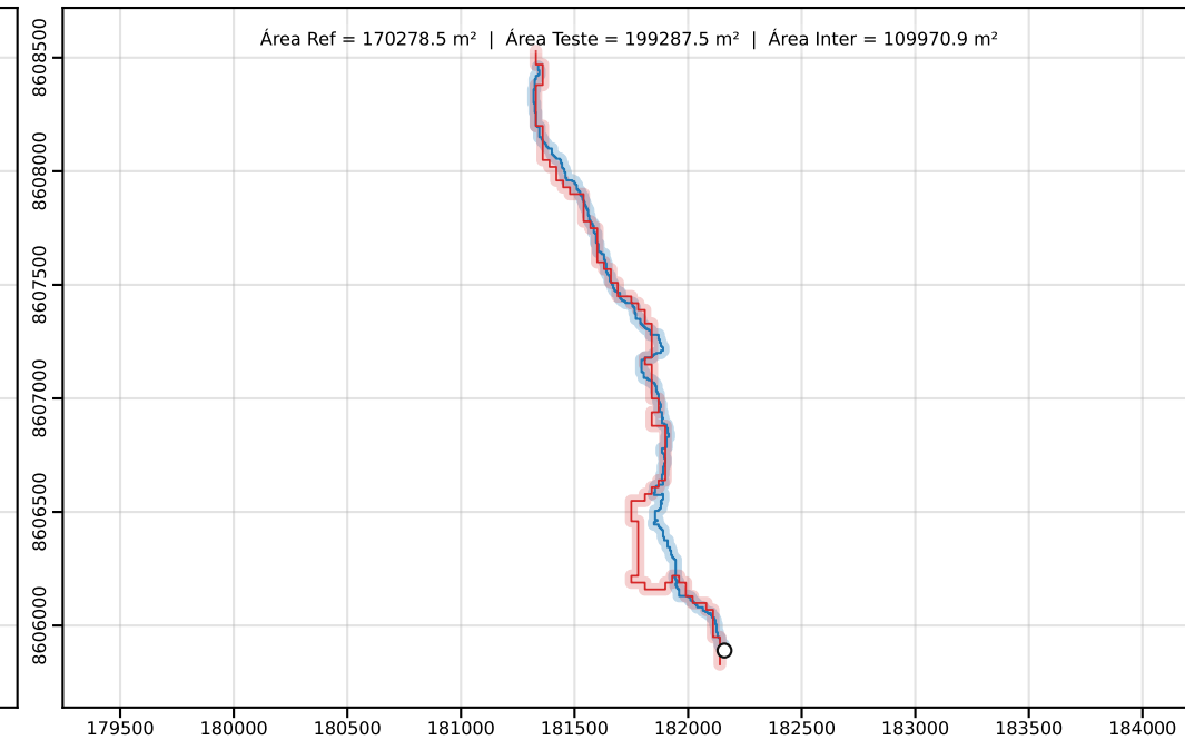
Classe D | PEC-PCD (Horizontal)=50.00 m | dm = 27.53
