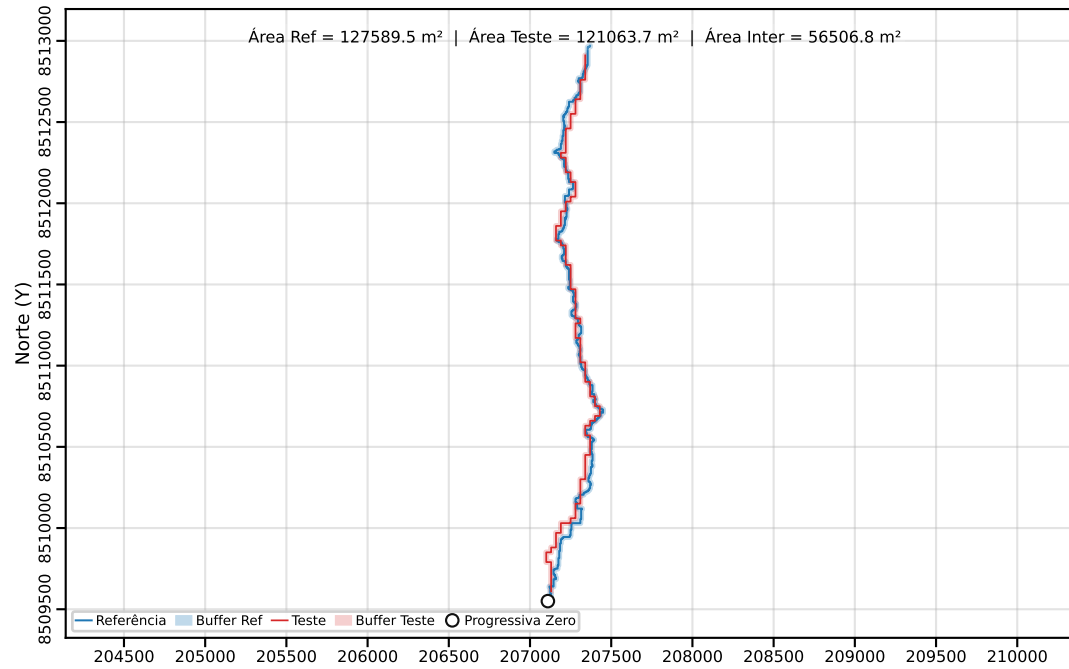
Classe C | PEC-PCD (Horizontal)=40.00 m | dm = 32.27
