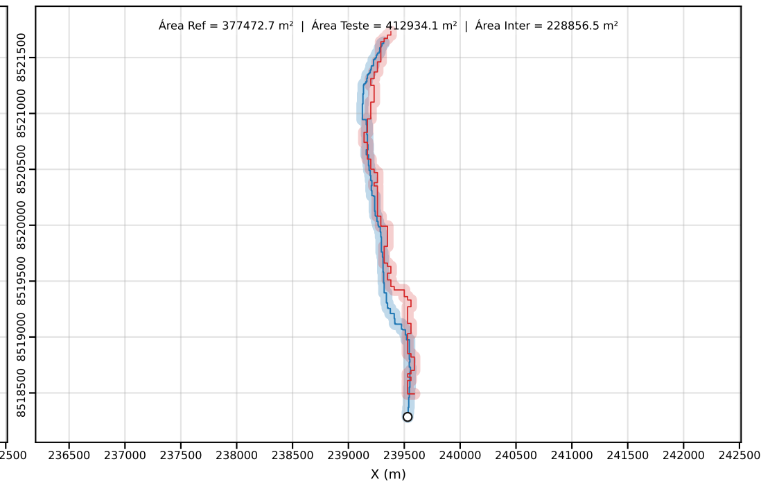
Classe D | PEC-PCD (Horizontal)=50.00 m | dm = 56.53
