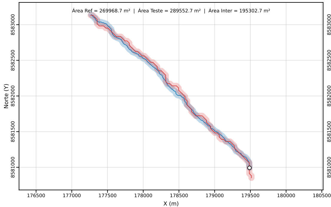
Classe C | PEC-PCD (Horizontal)=40.00 m | dm = 32.40
