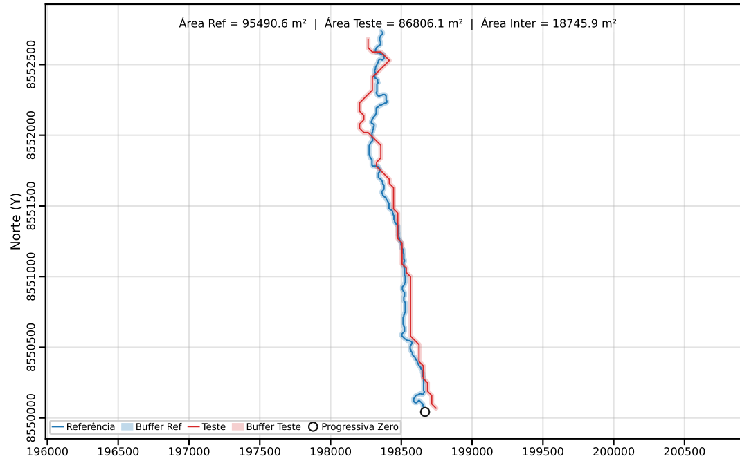
Classe C | PEC-PCD (Horizontal)=40.00 m | dm = 66.35
