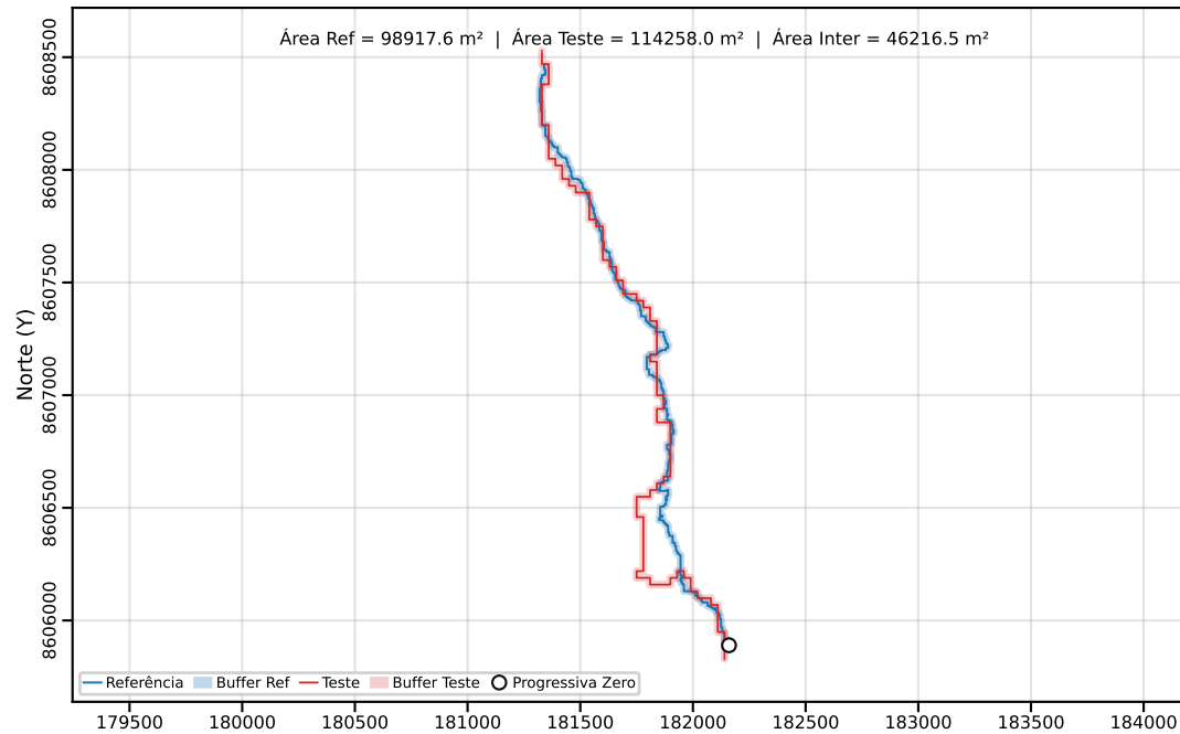
Classe C | PEC-PCD (Horizontal)=40.00 m | dm = 26.60
