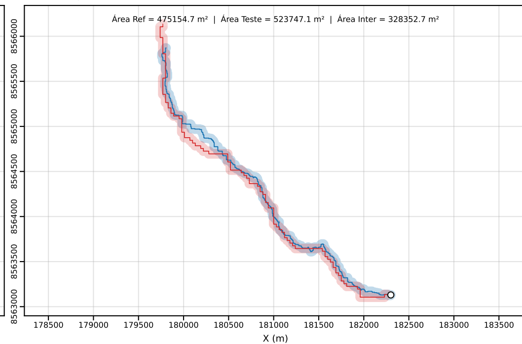
Classe D | PEC-PCD (Horizontal)=50.00 m | dm = 44.03
