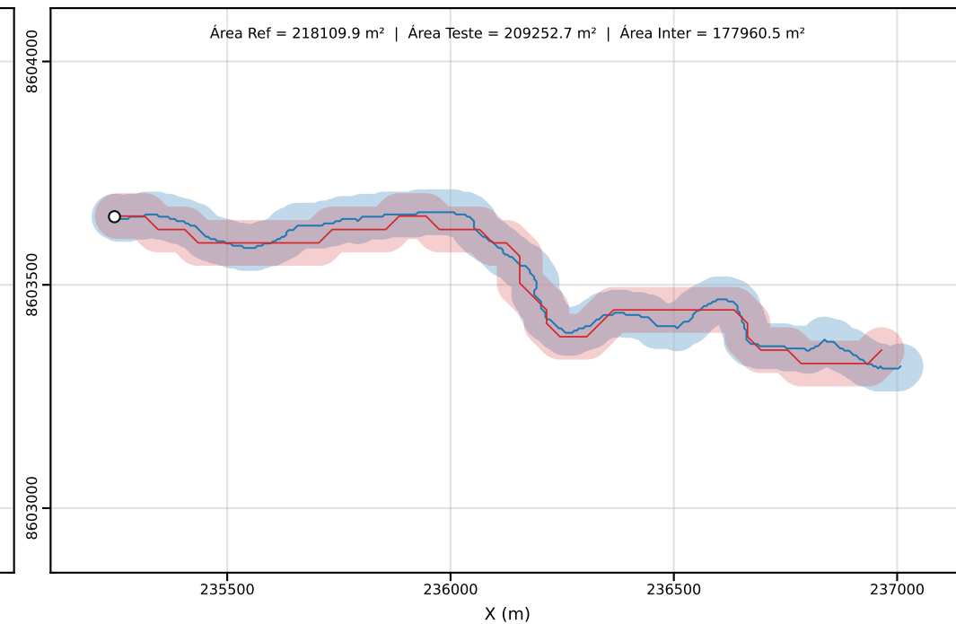
Classe D | PEC-PCD (Horizontal)=50.00 m | dm = 30.14
