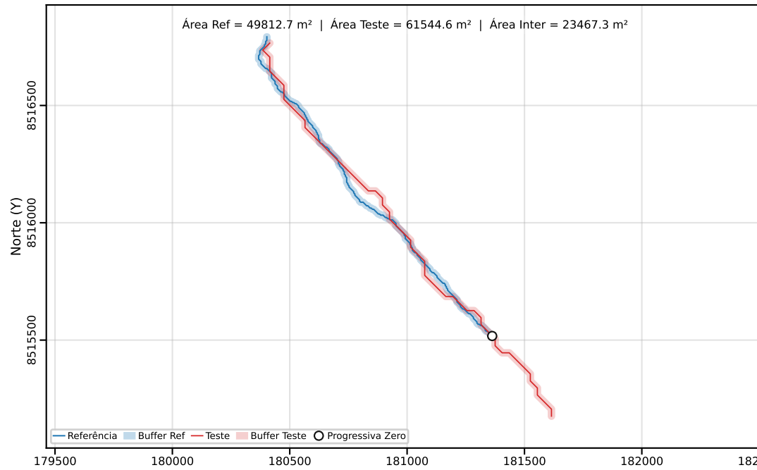
Classe C | PEC-PCD (Horizontal)=40.00 m | dm = 22.95
