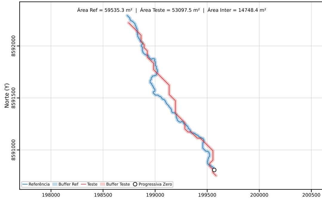
Classe C | PEC-PCD (Horizontal)=40.00 m | dm = 59.27
