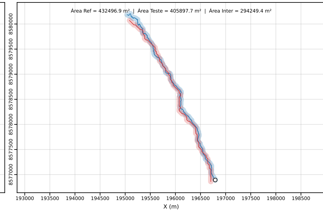
Classe D | PEC-PCD (Horizontal)=50.00 m | dm = 53.50
