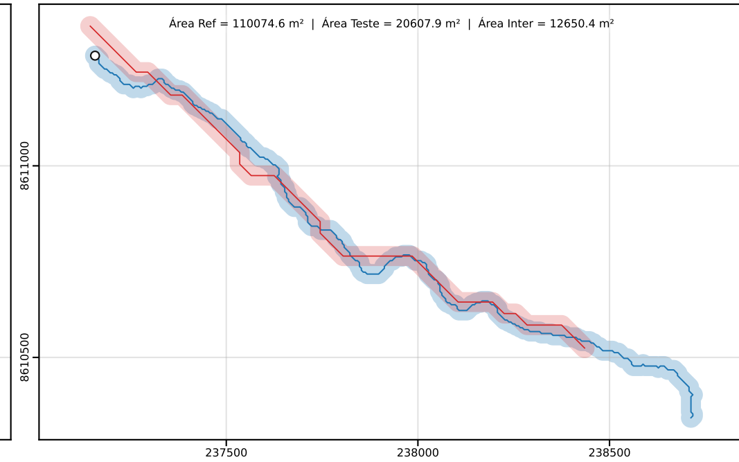
Classe D | PEC-PCD (Horizontal)=50.00 m | dm = 641.37
