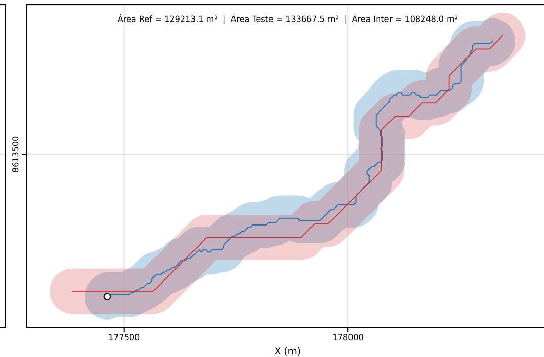
Classe D | PEC-PCD (Horizontal)=50.00 m | dm = 24.64
