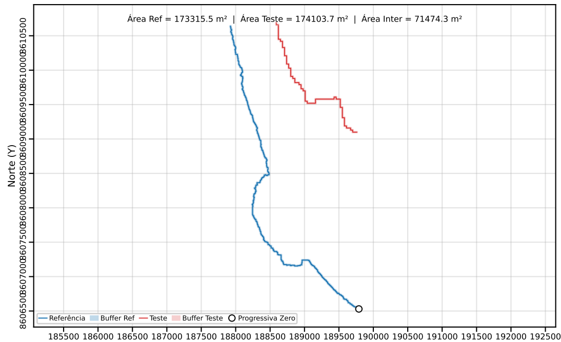
Classe C | PEC-PCD (Horizontal)=40.00 m | dm = 32.04
