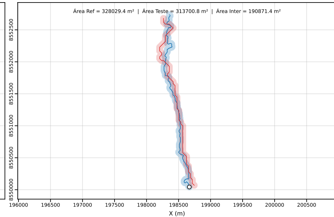
Classe D | PEC-PCD (Horizontal)=50.00 m | dm = 68.68
