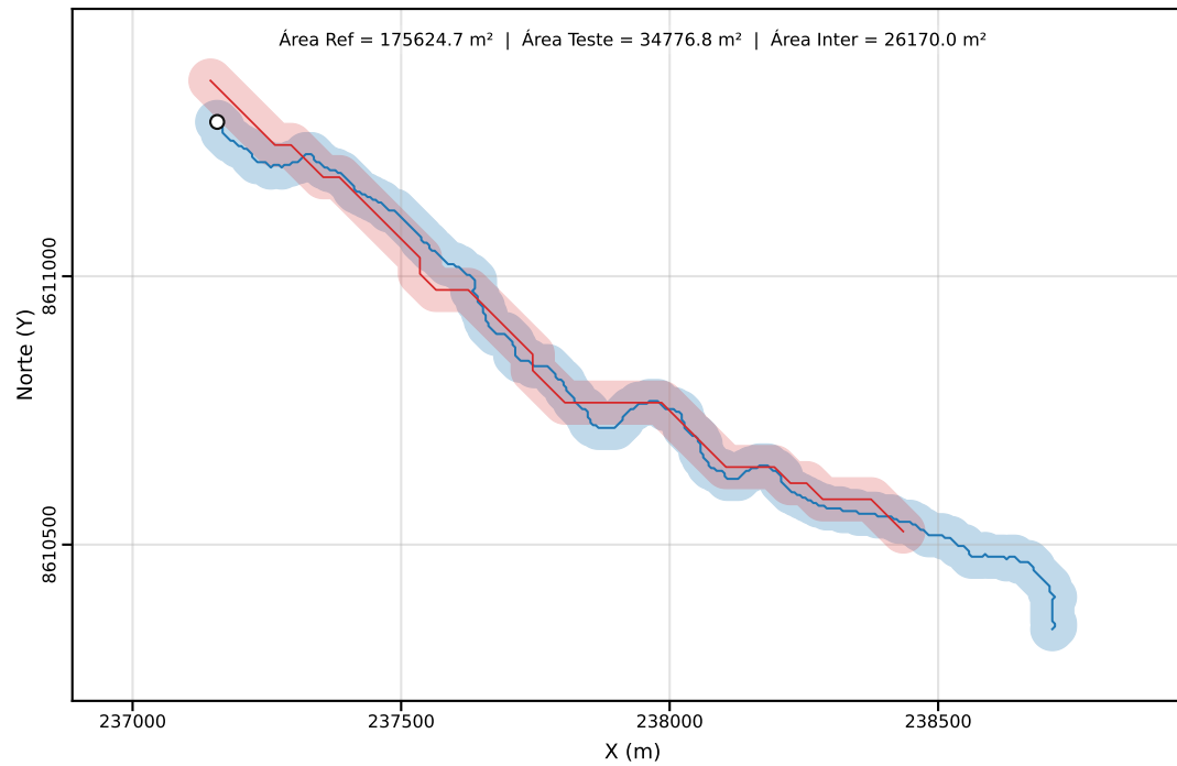
Classe C | PEC-PCD (Horizontal)=40.00 m | dm = 540.05
