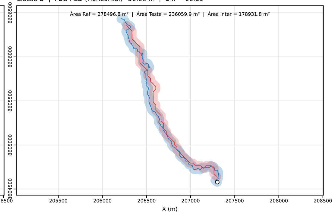
Classe D | PEC-PCD (Horizontal)=50.00 m | dm = 66.25
