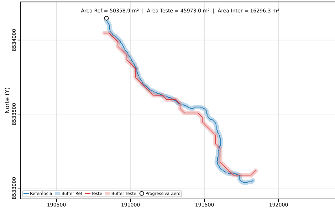
Classe C | PEC-PCD (Horizontal)=40.00 m | dm = 44.92
