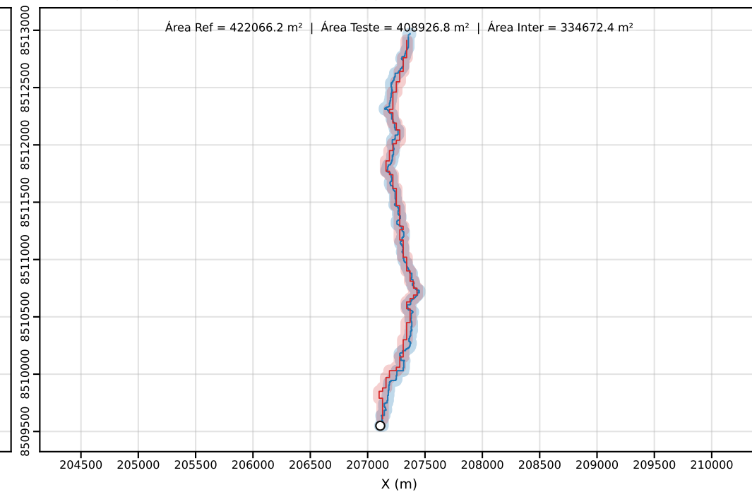
Classe D | PEC-PCD (Horizontal)=50.00 m | dm = 33.57
