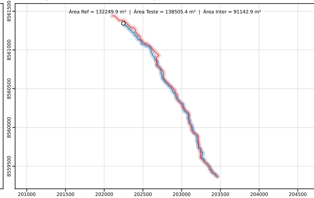
Classe D | PEC-PCD (Horizontal)=50.00 m | dm = 22.81
