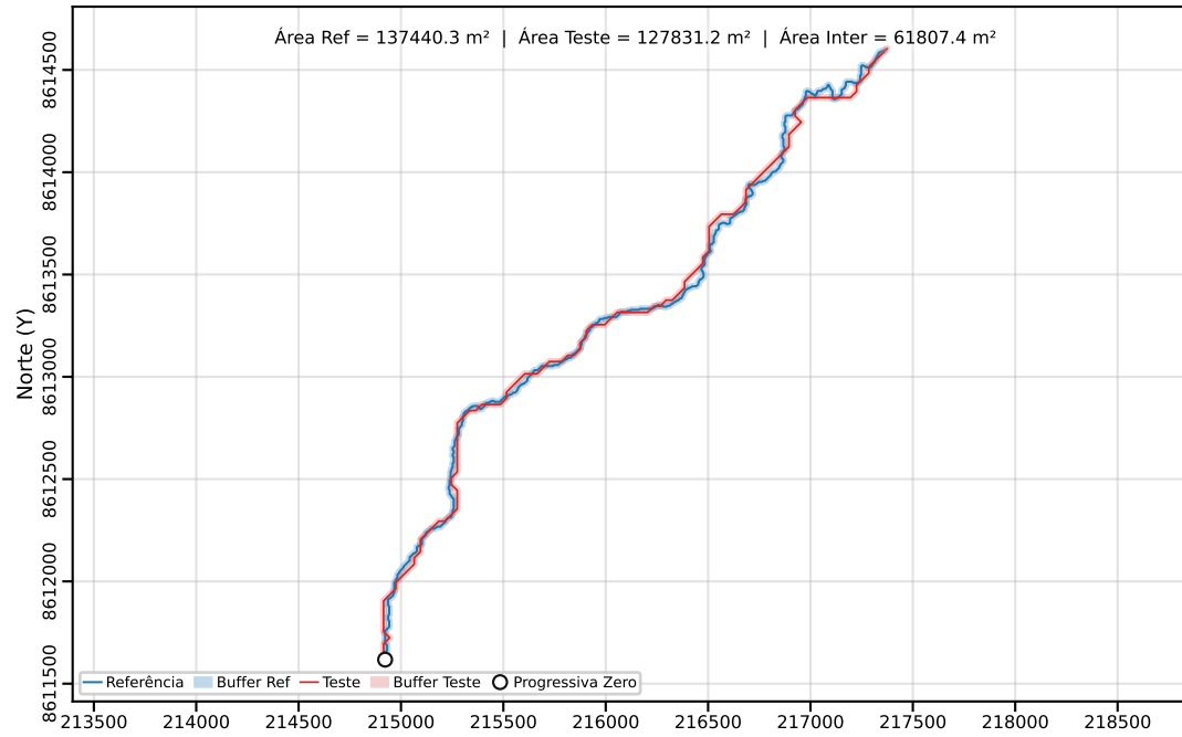
Classe C | PEC-PCD (Horizontal)=40.00 m | dm = 29.33
