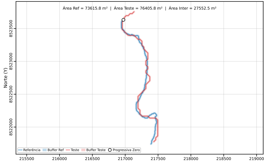
Classe C | PEC-PCD (Horizontal)=40.00 m | dm = 32.23
