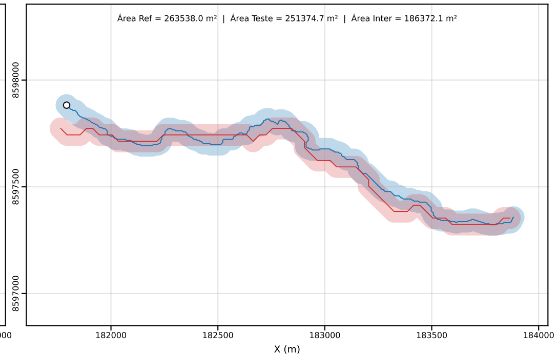
Classe D | PEC-PCD (Horizontal)=50.00 m | dm = 48.22
