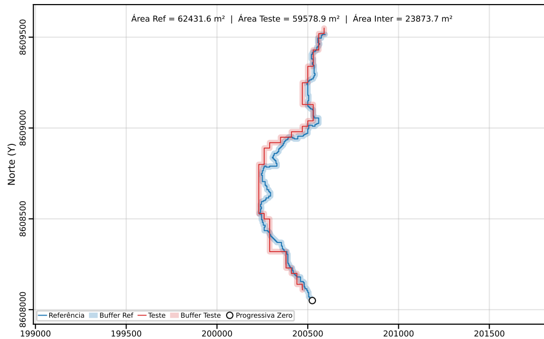
Classe C | PEC-PCD (Horizontal)=40.00 m | dm = 35.30
