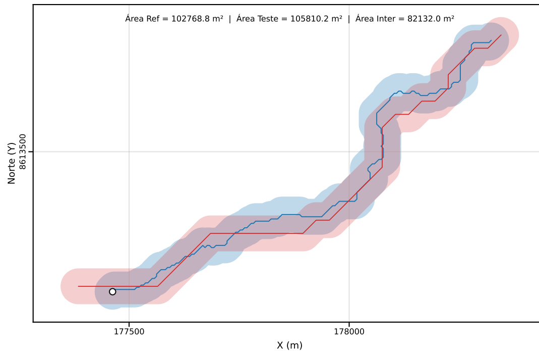
Classe C | PEC-PCD (Horizontal)=40.00 m | dm = 24.51
