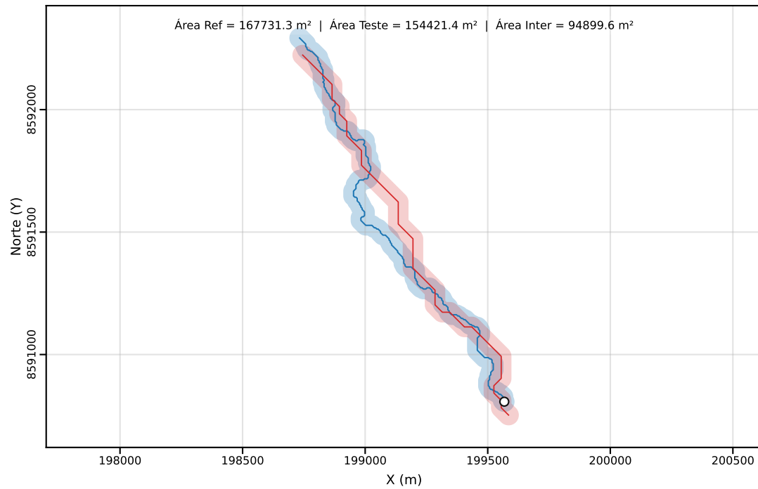
Classe C | PEC-PCD (Horizontal)=40.00 m | dm = 59.27
