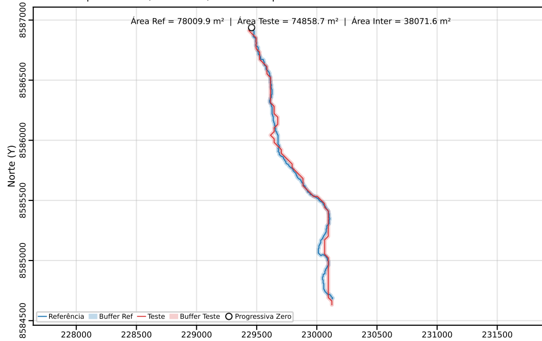
Classe C | PEC-PCD (Horizontal)=40.00 m | dm = 26.98
