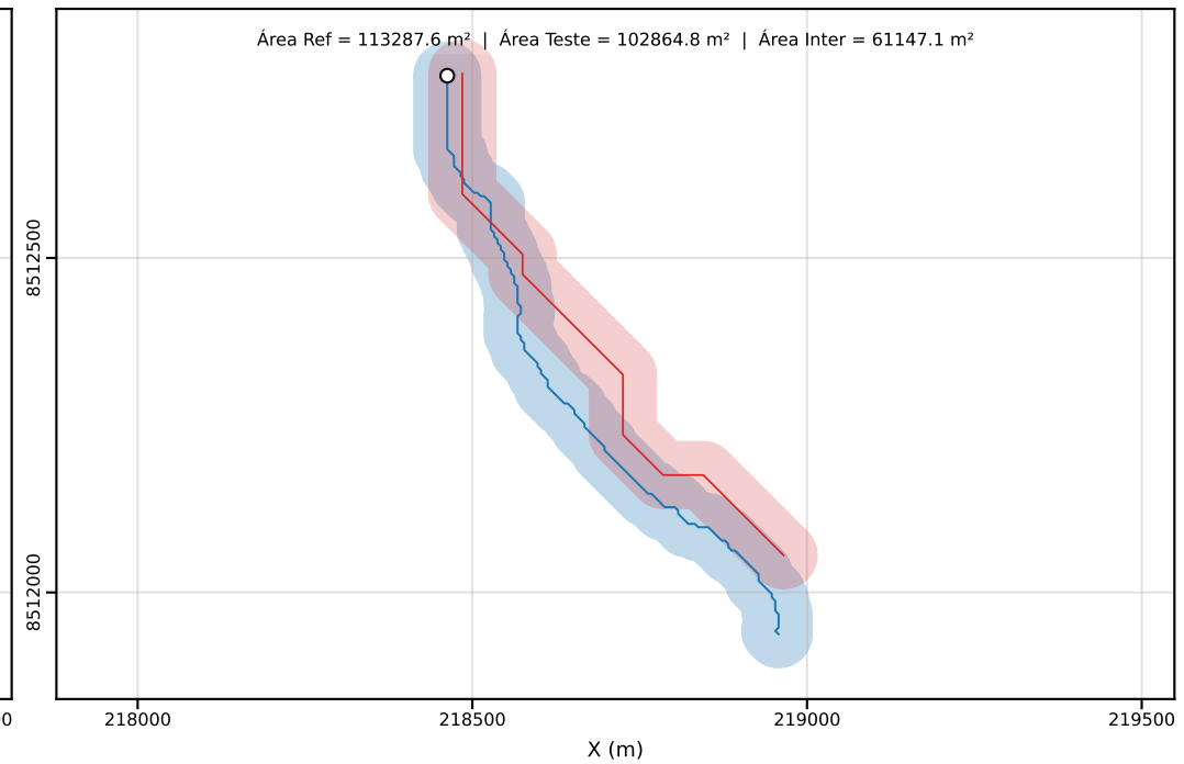
Classe D | PEC-PCD (Horizontal)=50.00 m | dm = 79.62
