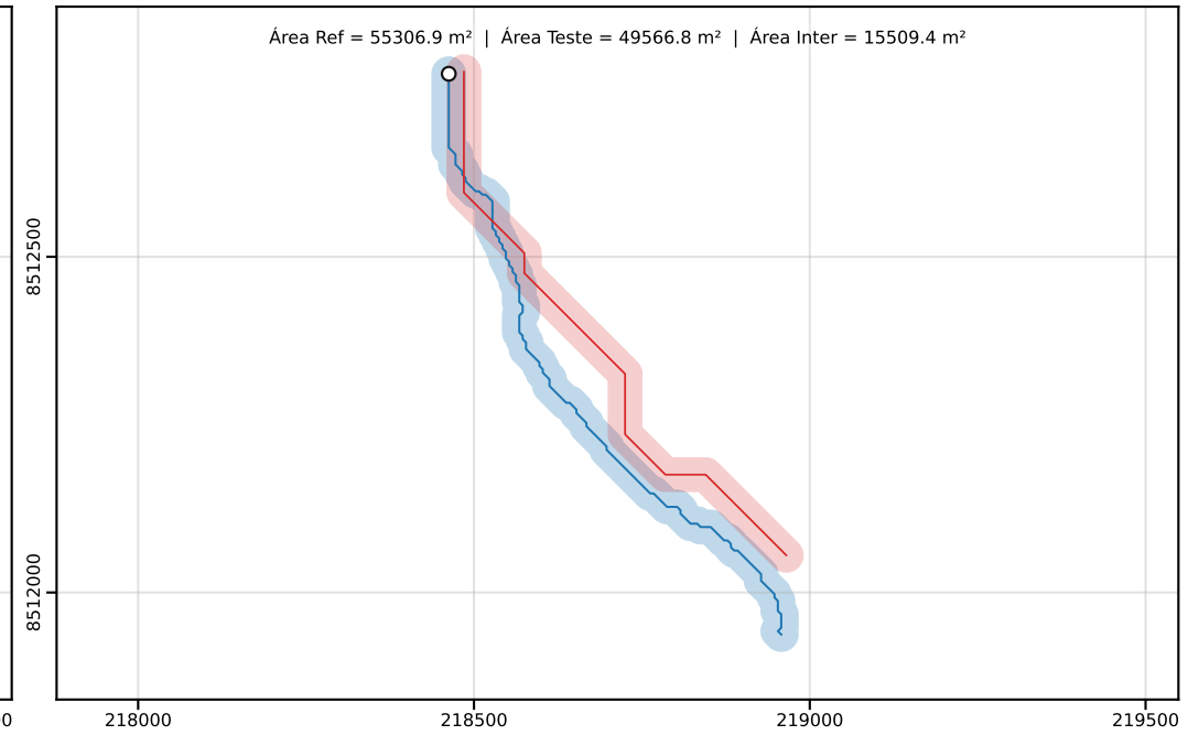
Classe D | PEC-PCD (Horizontal)=50.00 m | dm = 79.62
