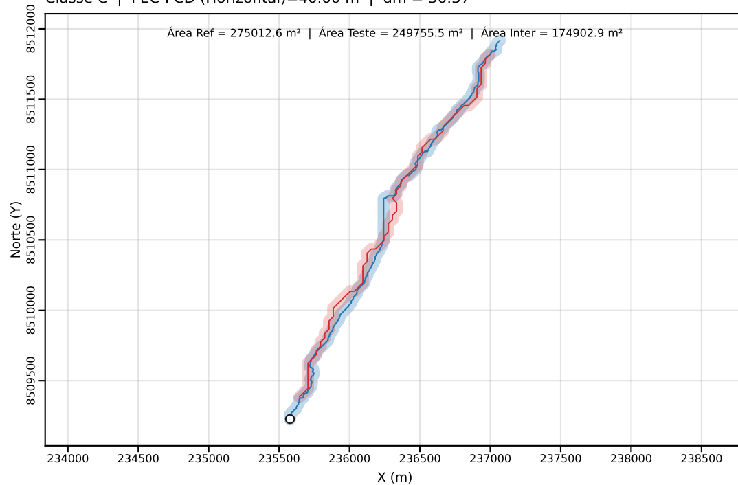
Classe C | PEC-PCD (Horizontal)=40.00 m | dm = 50.37
