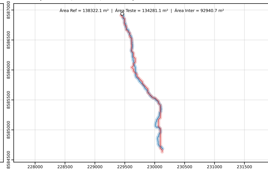
Classe D | PEC-PCD (Horizontal)=50.00 m | dm = 27.17
