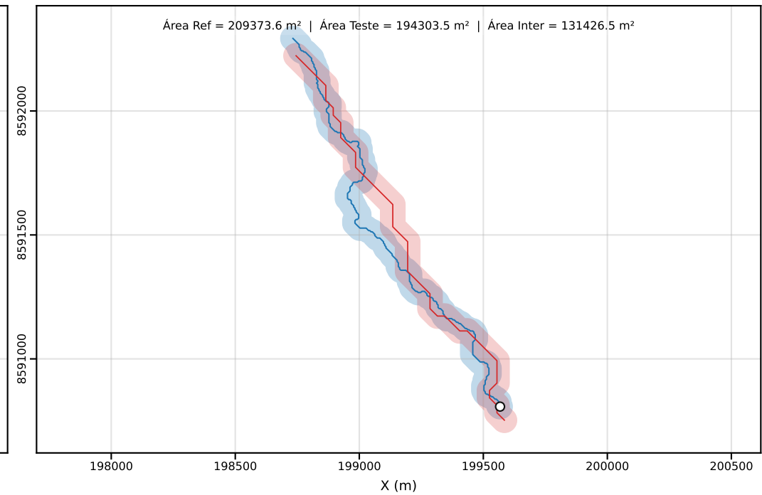
Classe D | PEC-PCD (Horizontal)=50.00 m | dm = 63.01
