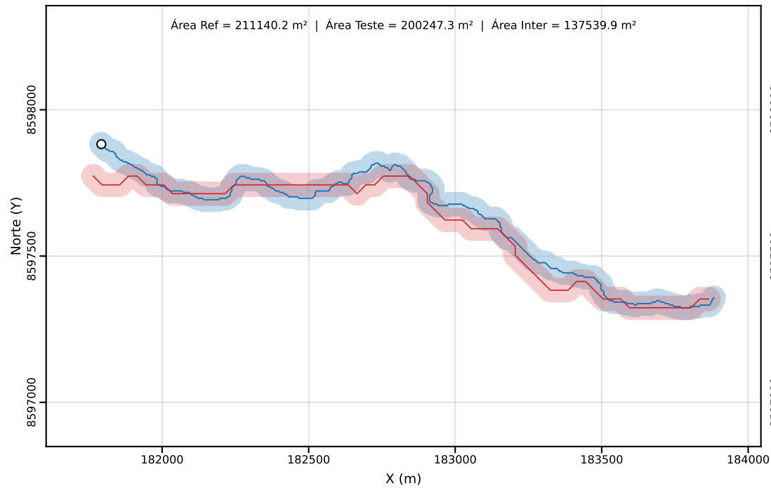
Classe C | PEC-PCD (Horizontal)=40.00 m | dm = 46.19
