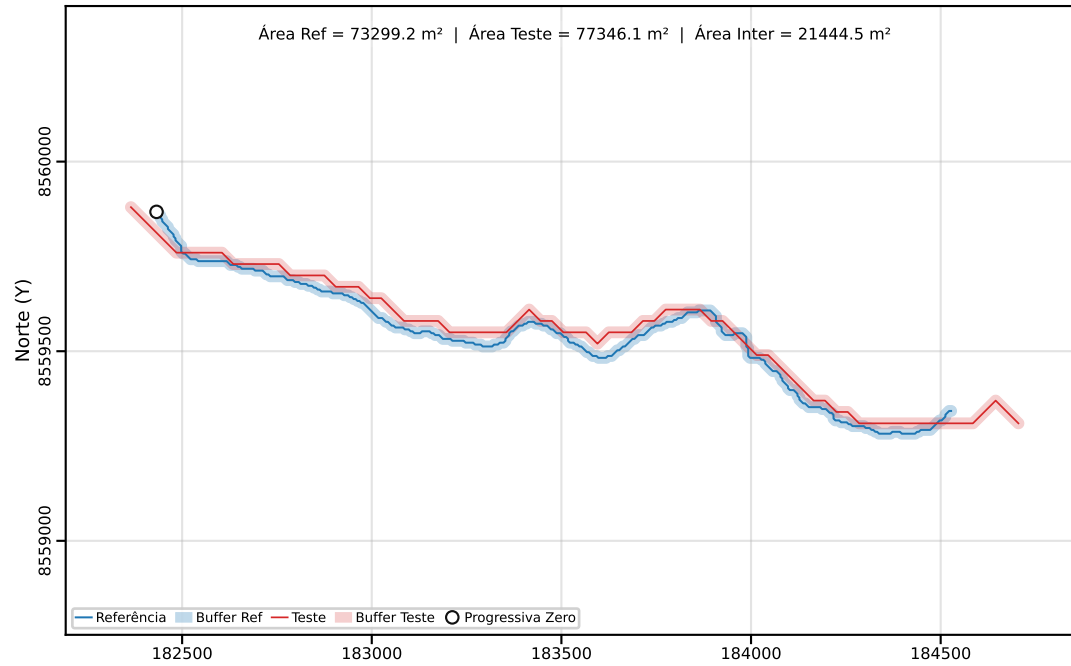
Classe C | PEC-PCD (Horizontal)=40.00 m | dm = 32.94
