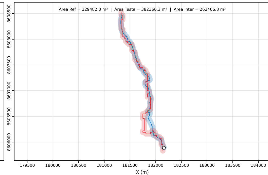
Classe D | PEC-PCD (Horizontal)=50.00 m | dm = 27.53
