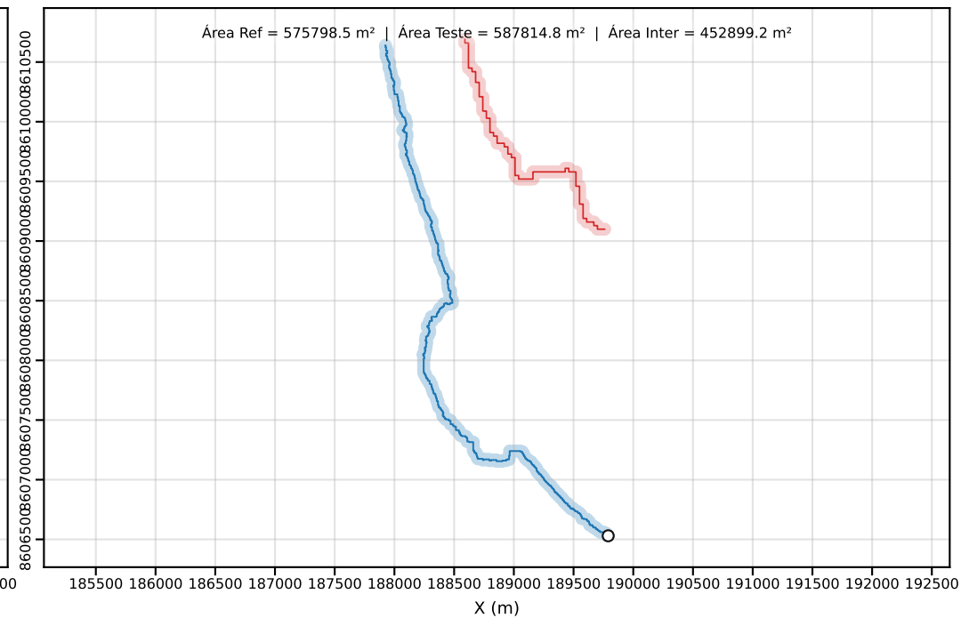
Classe D | PEC-PCD (Horizontal)=50.00 m | dm = 32.84
