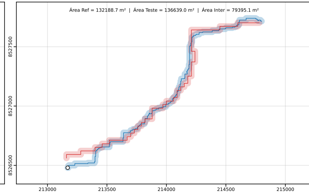
Classe D | PEC-PCD (Horizontal)=50.00 m | dm = 37.06
