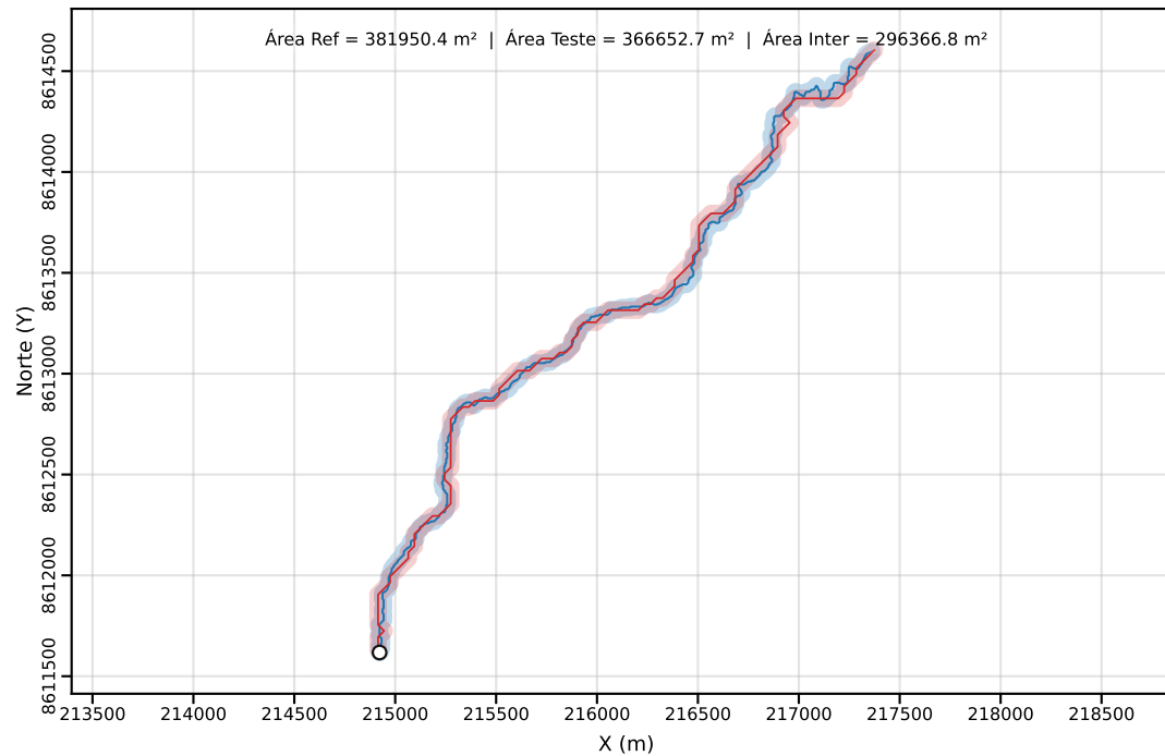
Classe C | PEC-PCD (Horizontal)=40.00 m | dm = 29.33
