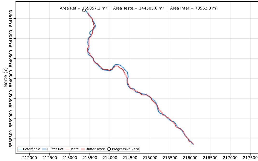
Classe C | PEC-PCD (Horizontal)=40.00 m | dm = 31.70
