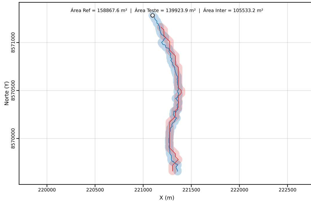
Classe C | PEC-PCD (Horizontal)=40.00 m | dm = 47.90
