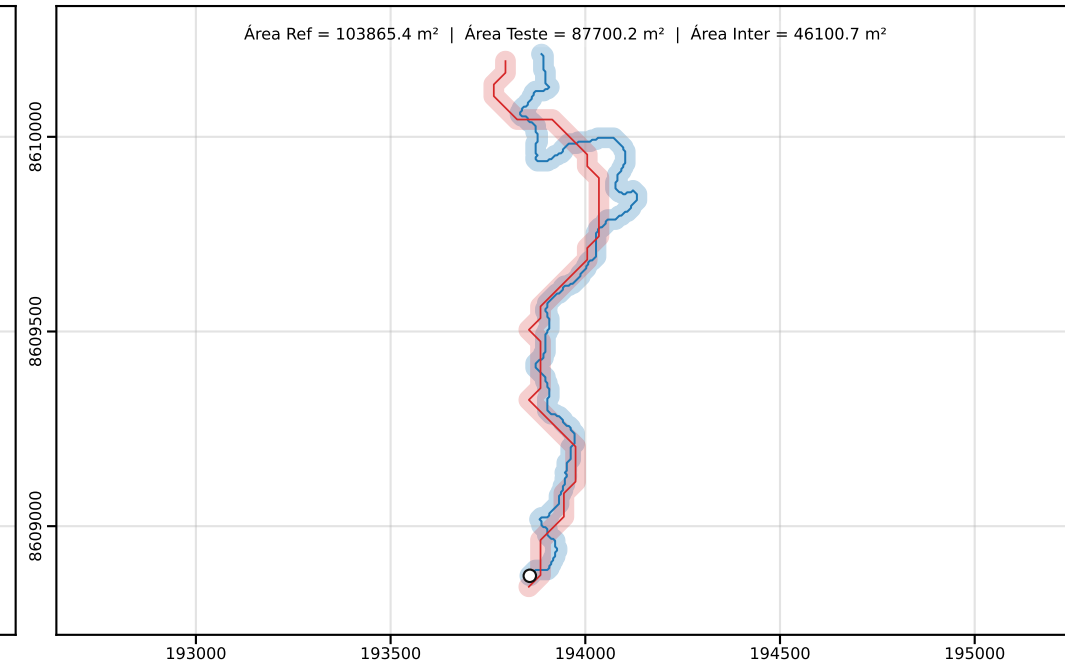
Classe D | PEC-PCD (Horizontal)=50.00 m | dm = 65.27
