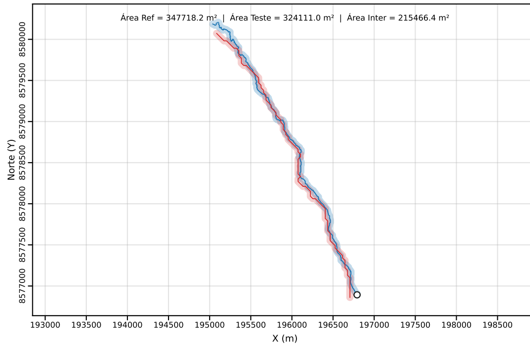
Classe C | PEC-PCD (Horizontal)=40.00 m | dm = 51.28
