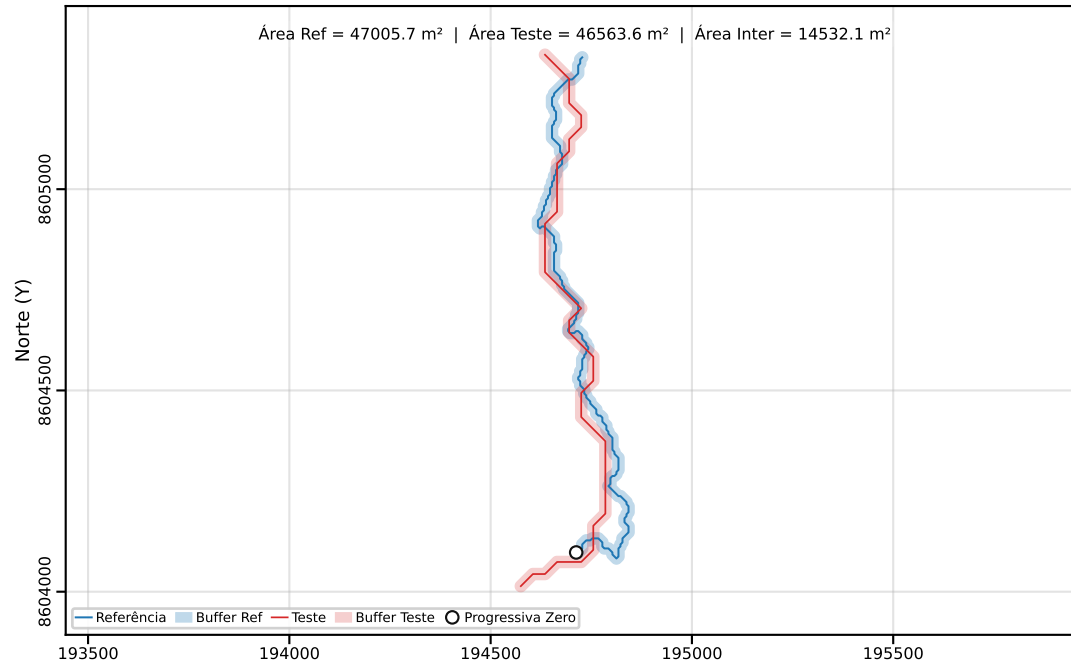
Classe C | PEC-PCD (Horizontal)=40.00 m | dm = 40.16
