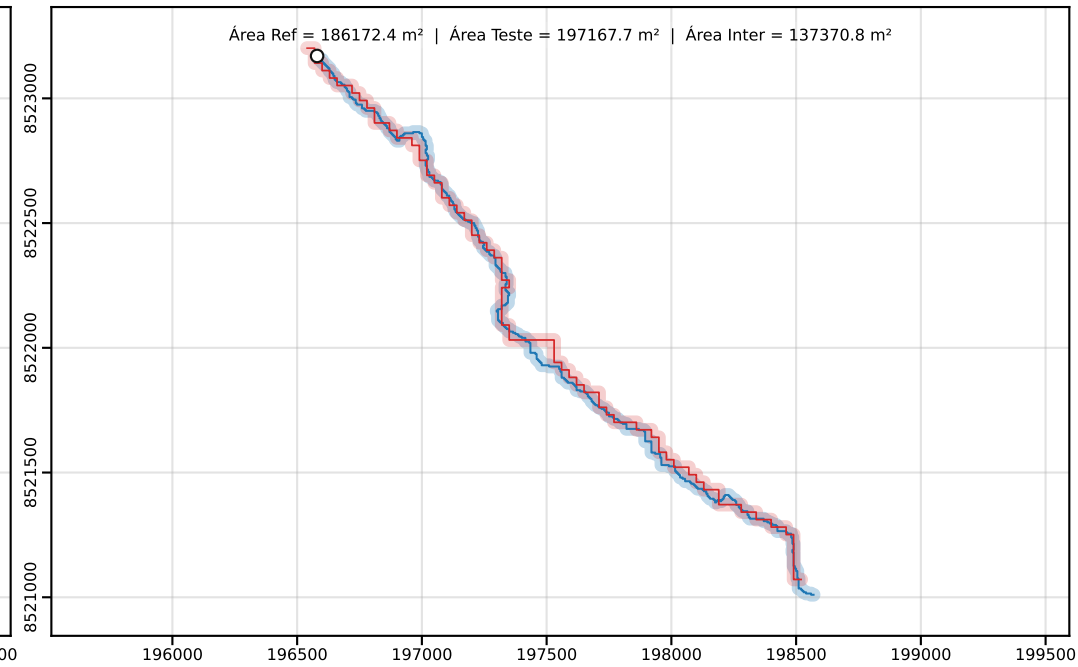
Classe D | PEC-PCD (Horizontal)=50.00 m | dm = 20.65
