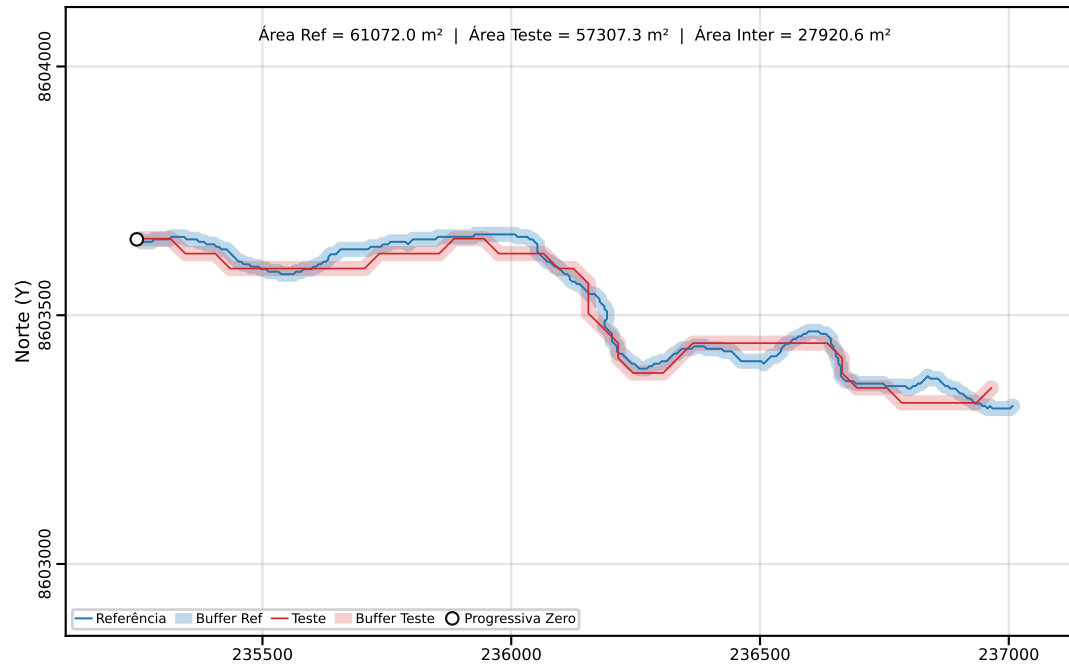
Classe C | PEC-PCD (Horizontal)=40.00 m | dm = 29.57
