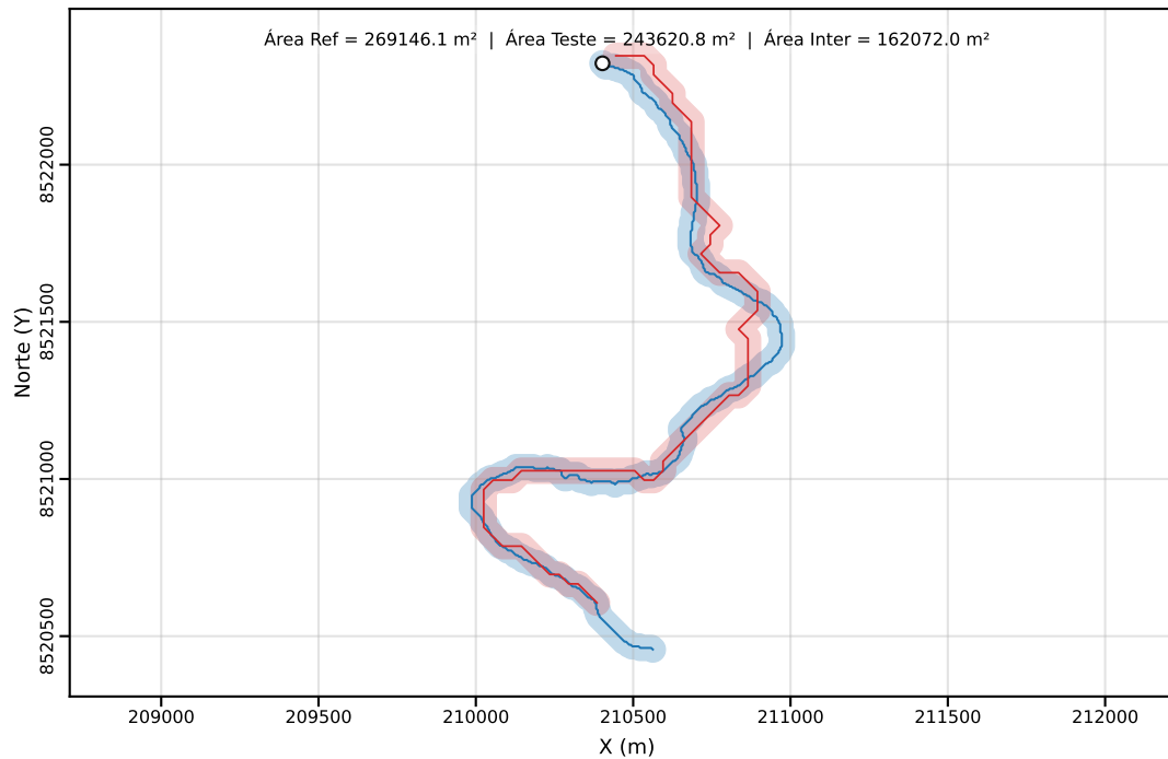
Classe C | PEC-PCD (Horizontal)=40.00 m | dm = 55.23
