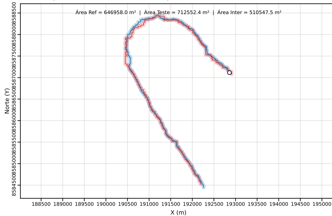
Classe C | PEC-PCD (Horizontal)=40.00 m | dm = 24.06
