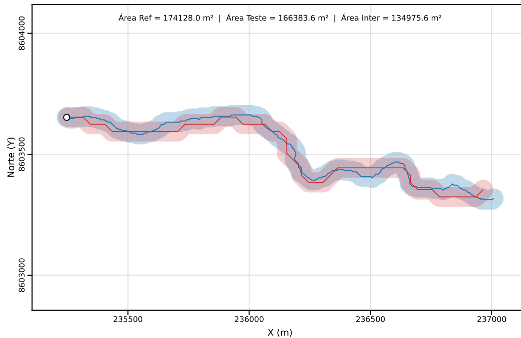
Classe C | PEC-PCD (Horizontal)=40.00 m | dm = 29.57
