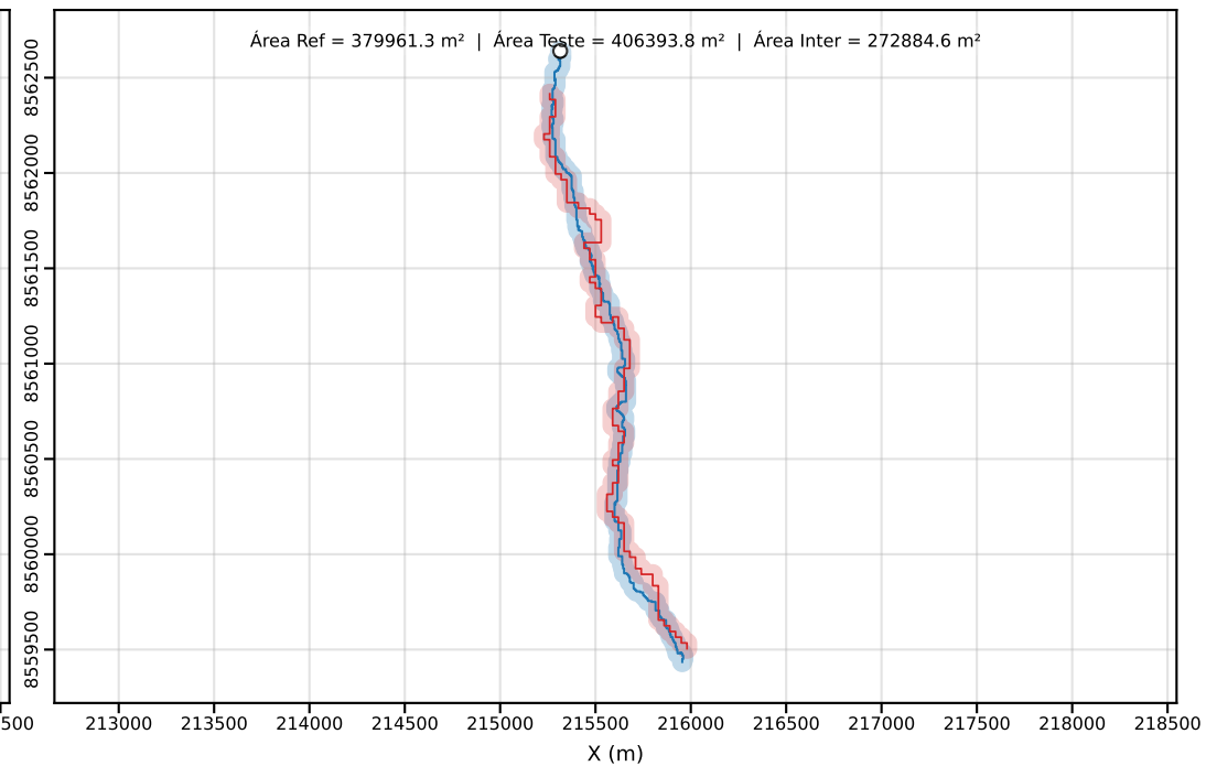
Classe D | PEC-PCD (Horizontal)=50.00 m | dm = 41.39
