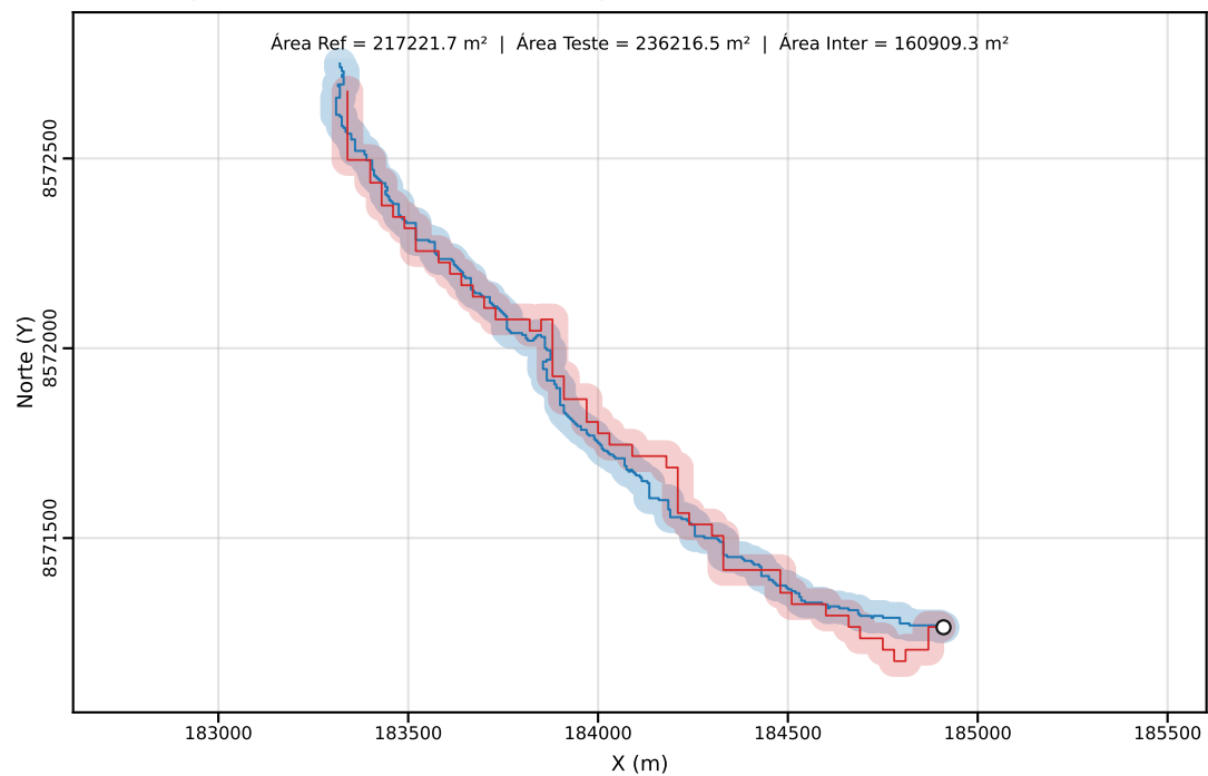
Classe C | PEC-PCD (Horizontal)=40.00 m | dm = 29.96
