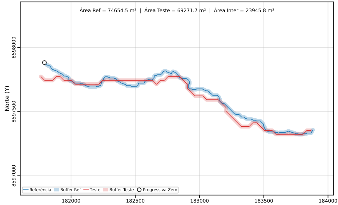
Classe C | PEC-PCD (Horizontal)=40.00 m | dm = 46.19
