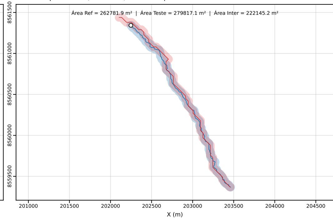
Classe D | PEC-PCD (Horizontal)=50.00 m | dm = 22.81
