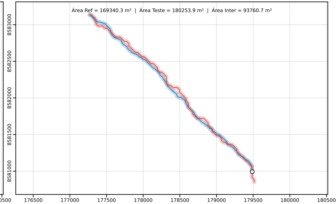
Classe D | PEC-PCD (Horizontal)=50.00 m | dm = 31.60
