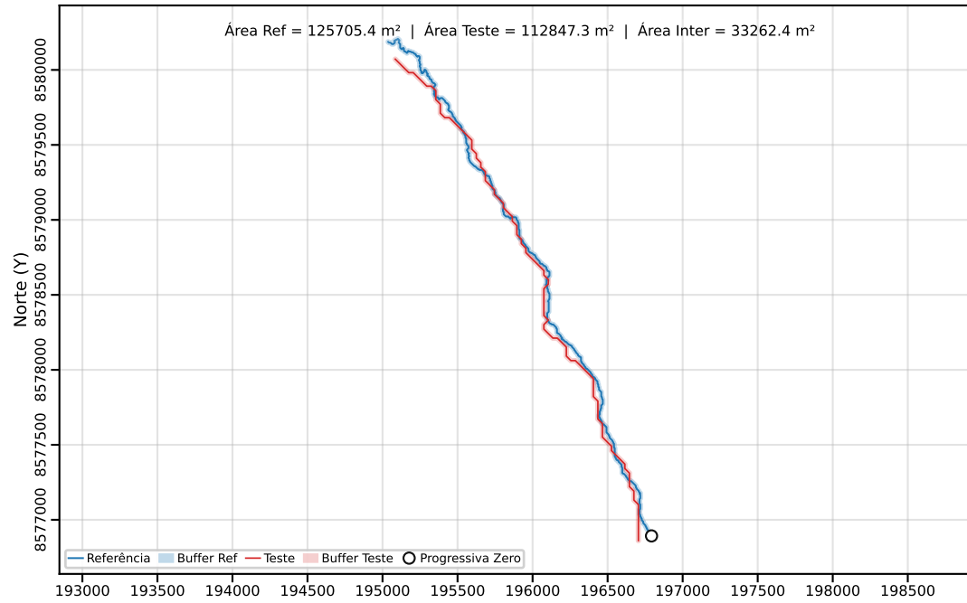
Classe C | PEC-PCD (Horizontal)=40.00 m | dm = 51.28
