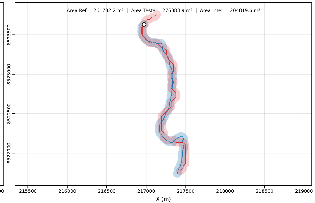
Classe D | PEC-PCD (Horizontal)=50.00 m | dm = 32.29
