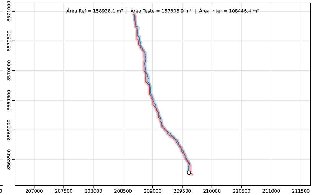
Classe D | PEC-PCD (Horizontal)=50.00 m | dm = 24.86
