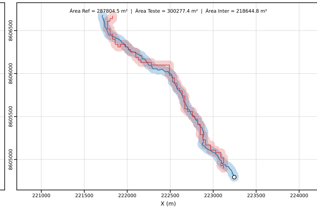
Classe D | PEC-PCD (Horizontal)=50.00 m | dm = 36.18
