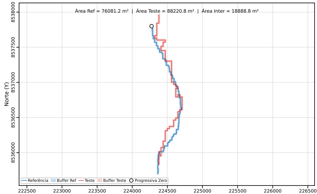
Classe C | PEC-PCD (Horizontal)=40.00 m | dm = 48.48
