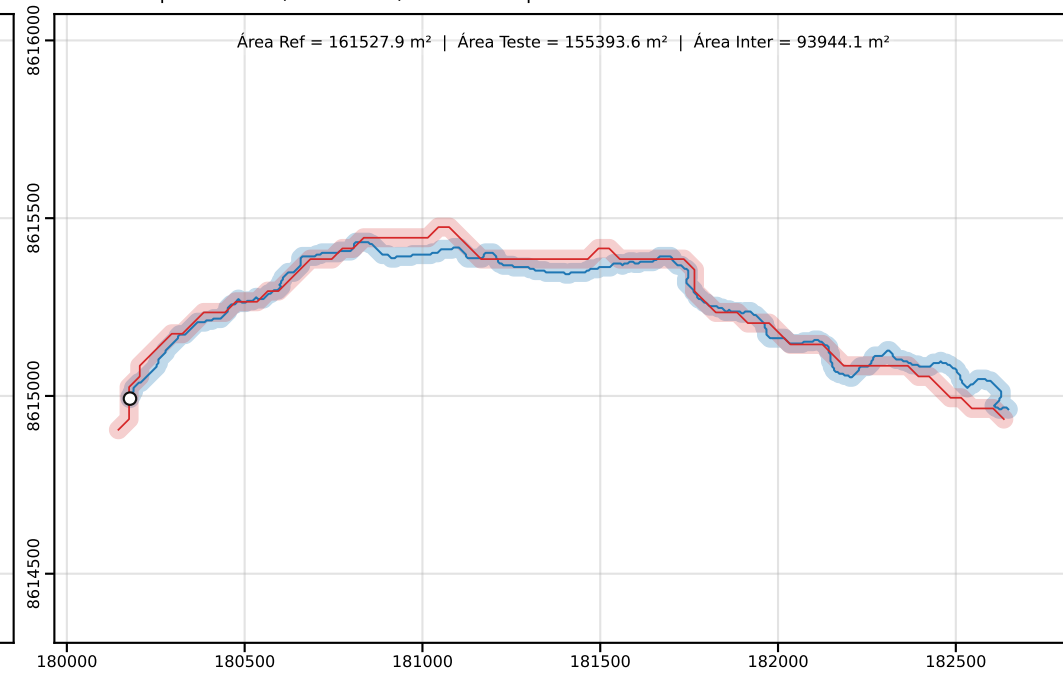
Classe D | PEC-PCD (Horizontal)=50.00 m | dm = 36.12
