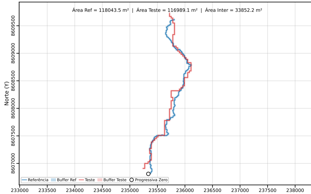
Classe C | PEC-PCD (Horizontal)=40.00 m | dm = 51.56
