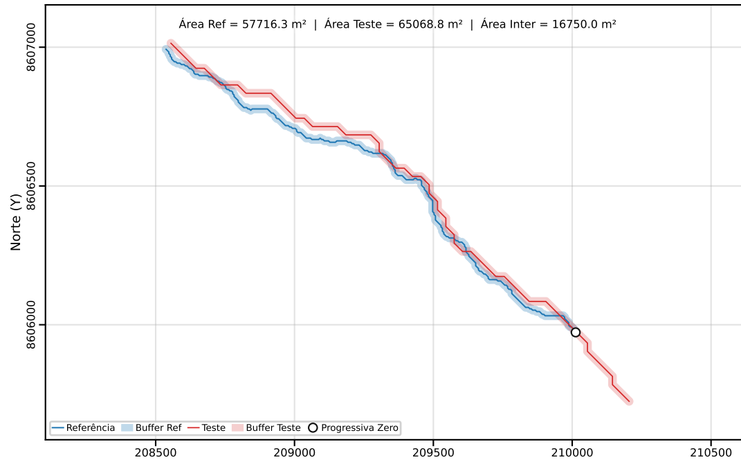
Classe C | PEC-PCD (Horizontal)=40.00 m | dm = 34.65
