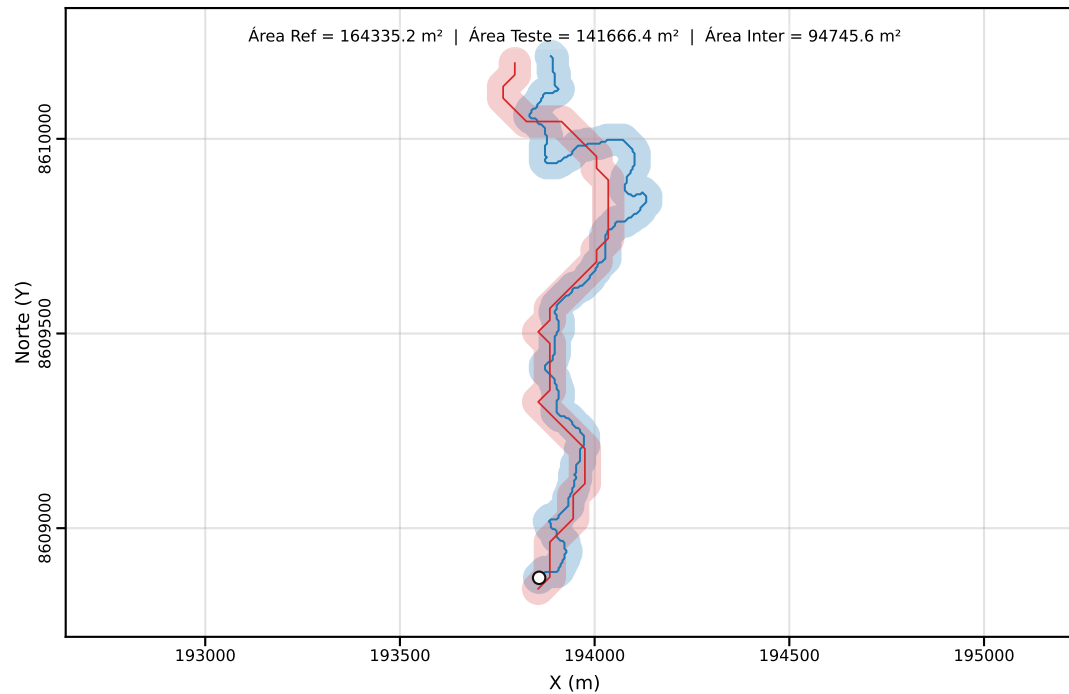
Classe C | PEC-PCD (Horizontal)=40.00 m | dm = 61.73
