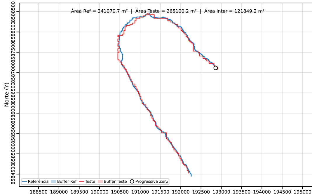
Classe C | PEC-PCD (Horizontal)=40.00 m | dm = 24.06
