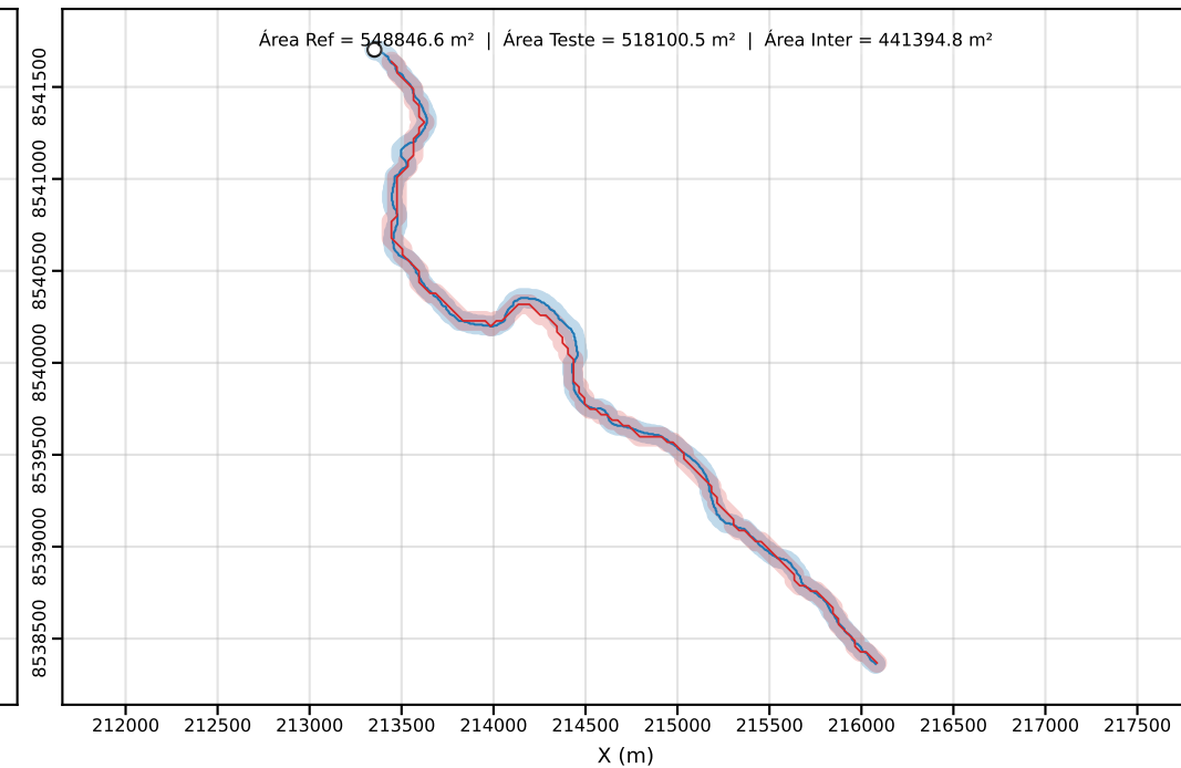
Classe D | PEC-PCD (Horizontal)=50.00 m | dm = 32.58
