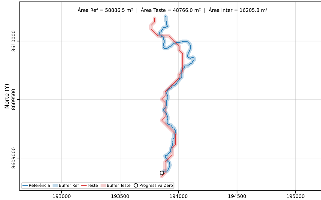
Classe C | PEC-PCD (Horizontal)=40.00 m | dm = 61.73
