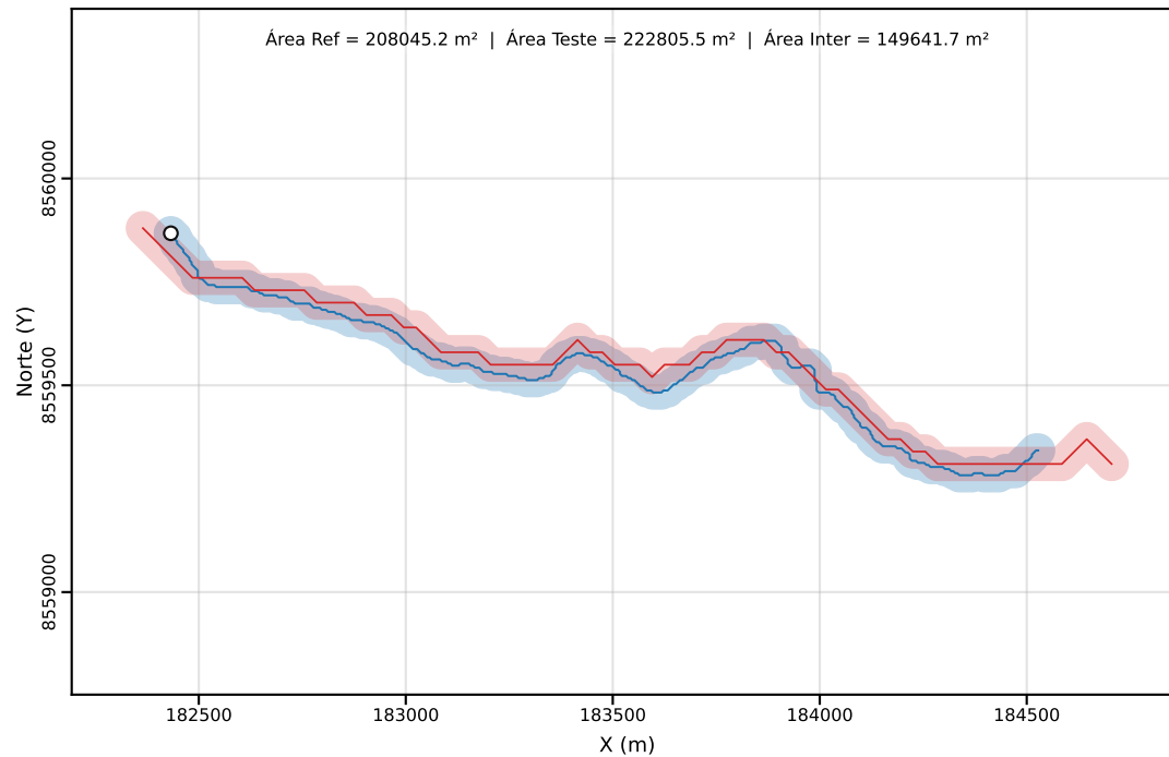
Classe C | PEC-PCD (Horizontal)=40.00 m | dm = 32.94
