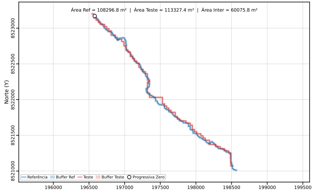
Classe C | PEC-PCD (Horizontal)=40.00 m | dm = 20.16
