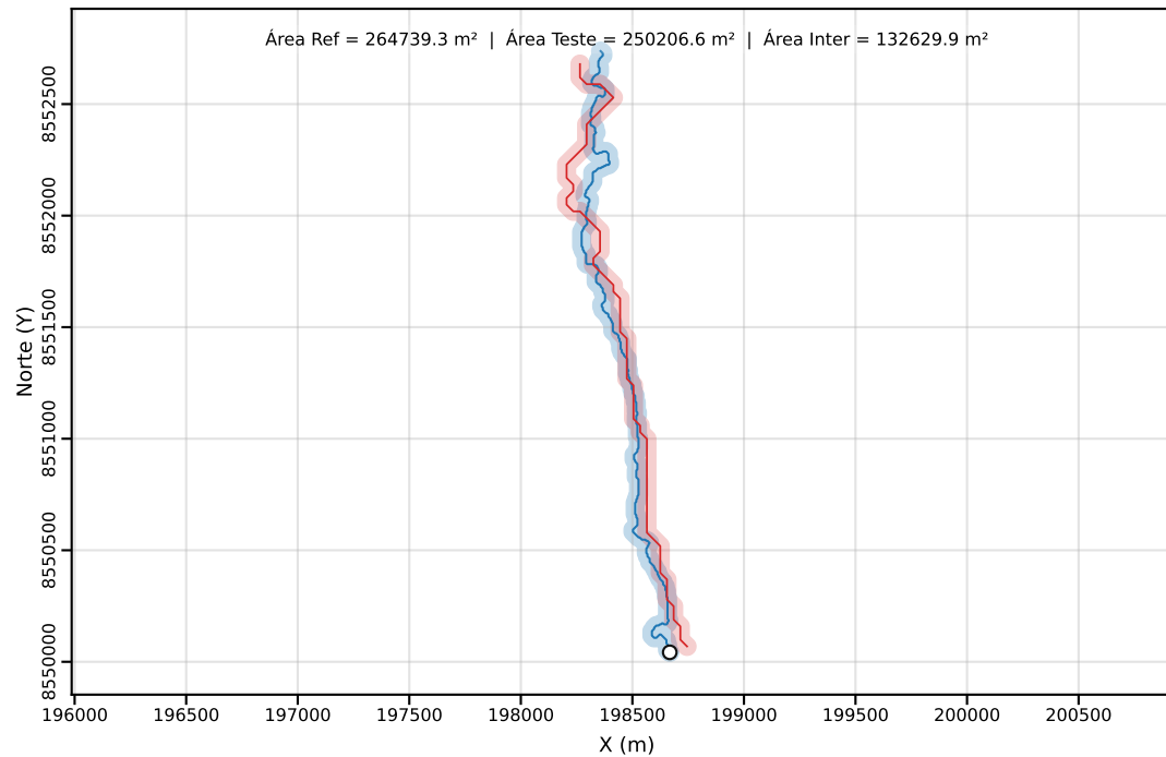
Classe C | PEC-PCD (Horizontal)=40.00 m | dm = 66.35
