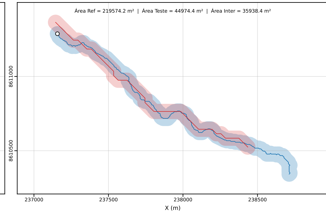
Classe D | PEC-PCD (Horizontal)=50.00 m | dm = 641.37
