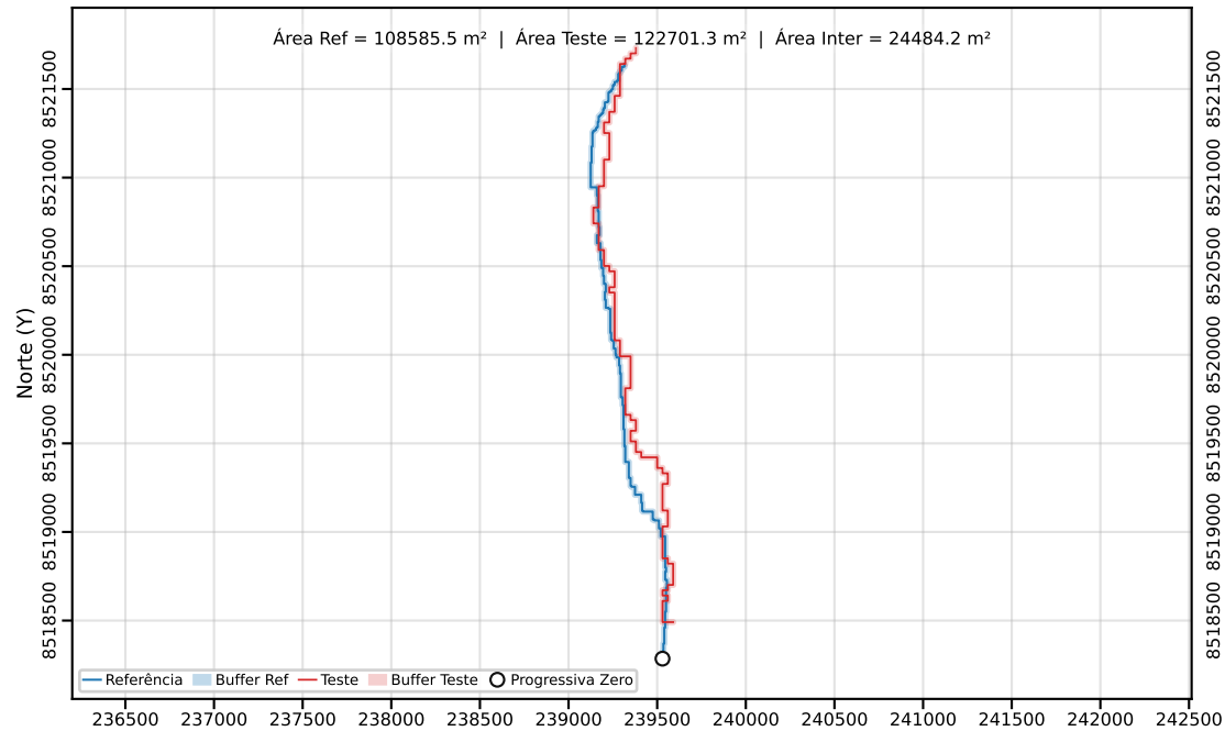
Classe C | PEC-PCD (Horizontal)=40.00 m | dm = 52.75
