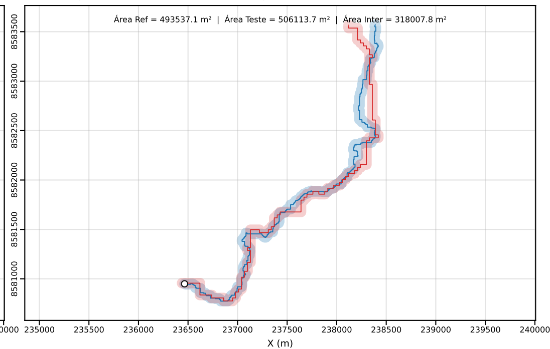
Classe D | PEC-PCD (Horizontal)=50.00 m | dm = 54.48
