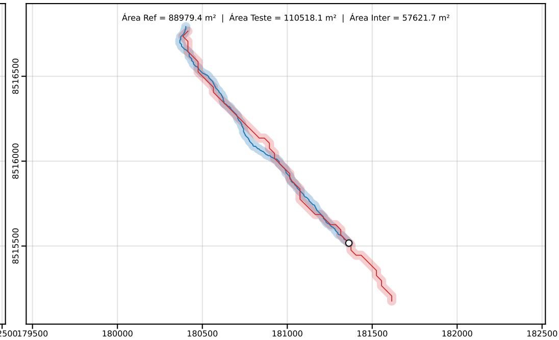
Classe D | PEC-PCD (Horizontal)=50.00 m | dm = 22.97
