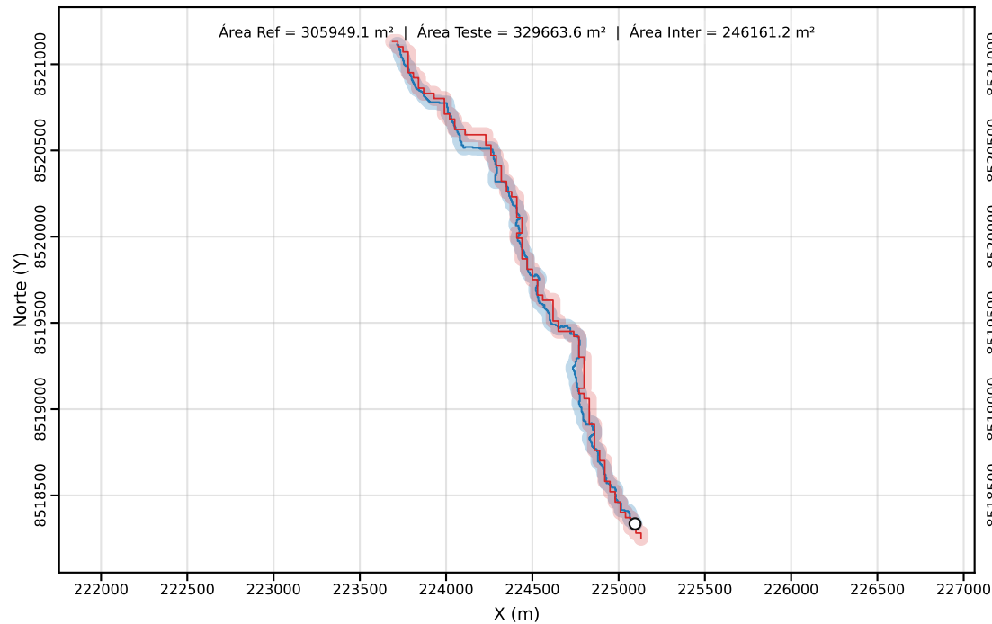
Classe C | PEC-PCD (Horizontal)=40.00 m | dm = 22.79
