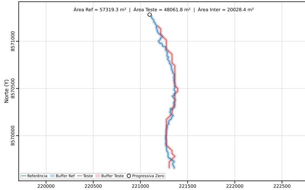
Classe C | PEC-PCD (Horizontal)=40.00 m | dm = 47.90
