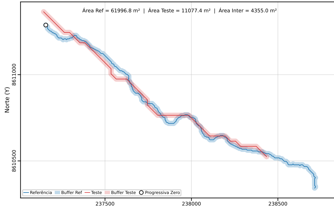
Classe C | PEC-PCD (Horizontal)=40.00 m | dm = 540.05
