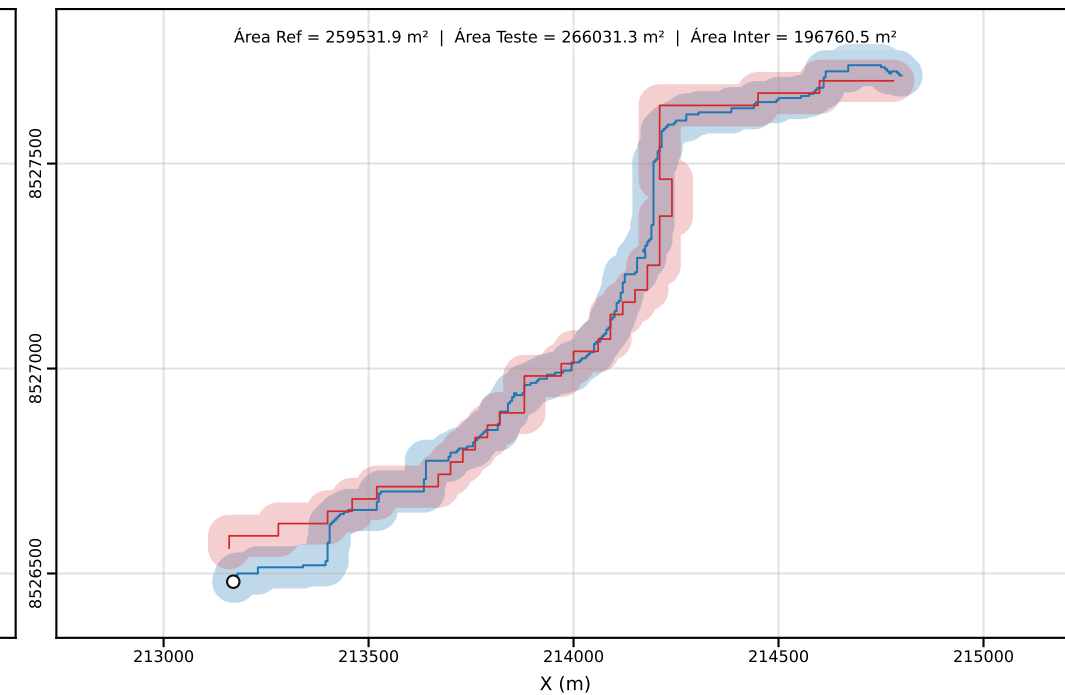
Classe D | PEC-PCD (Horizontal)=50.00 m | dm = 37.06
