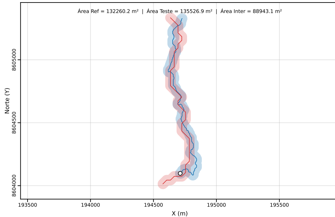
Classe C | PEC-PCD (Horizontal)=40.00 m | dm = 40.16
