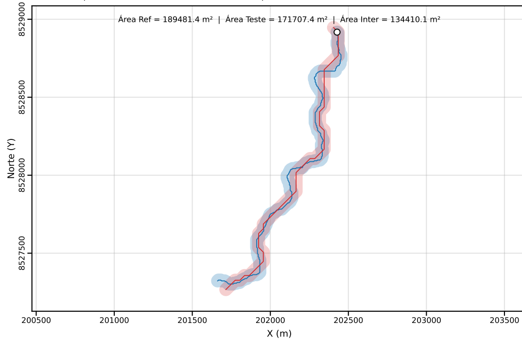
Classe C | PEC-PCD (Horizontal)=40.00 m | dm = 40.30
