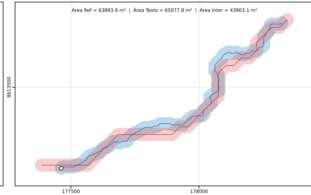
Classe D | PEC-PCD (Horizontal)=50.00 m | dm = 24.64
