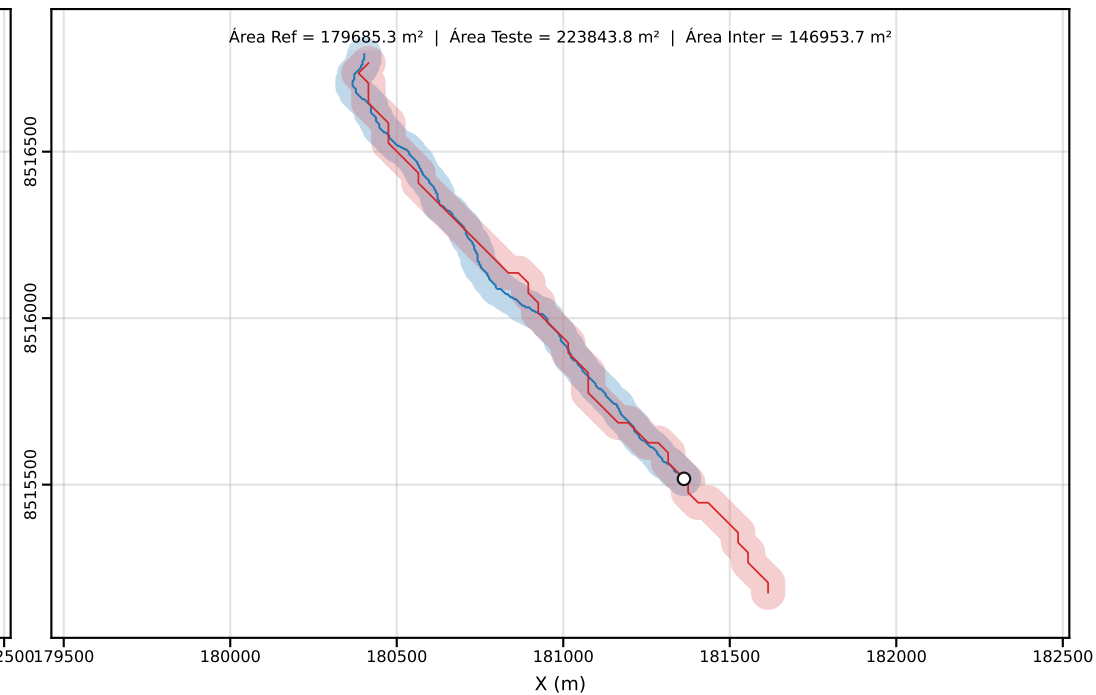
Classe D | PEC-PCD (Horizontal)=50.00 m | dm = 22.97
