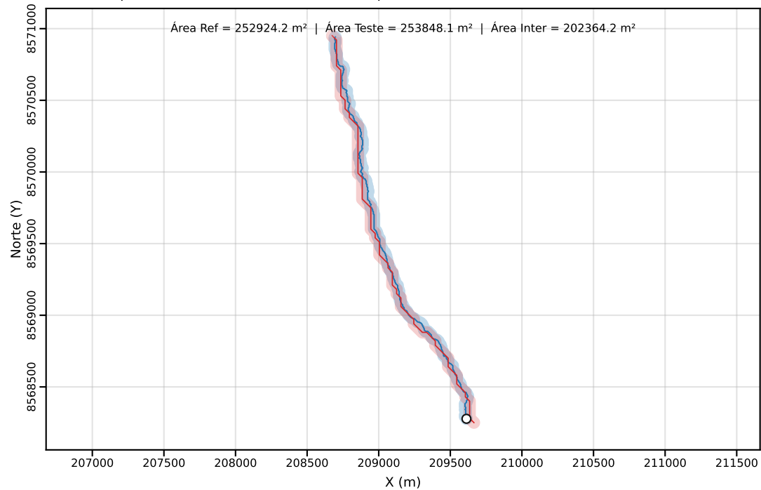
Classe C | PEC-PCD (Horizontal)=40.00 m | dm = 25.03
