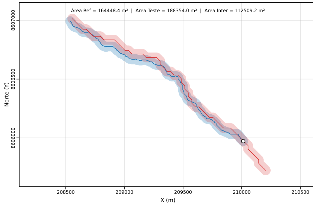
Classe C | PEC-PCD (Horizontal)=40.00 m | dm = 34.65
