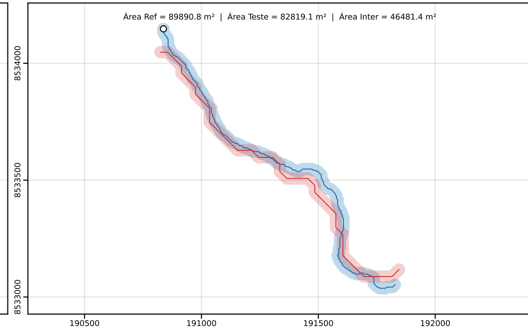
Classe D | PEC-PCD (Horizontal)=50.00 m | dm = 47.05
