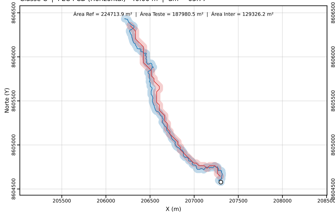
Classe C | PEC-PCD (Horizontal)=40.00 m | dm = 63.77
