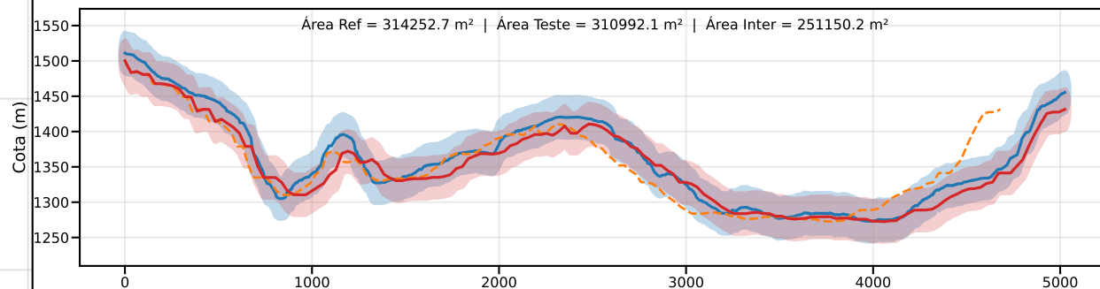
Classe D | PEC-PCD (Vertical)=37.5 m | EQ = 50m | dm = 19.25
