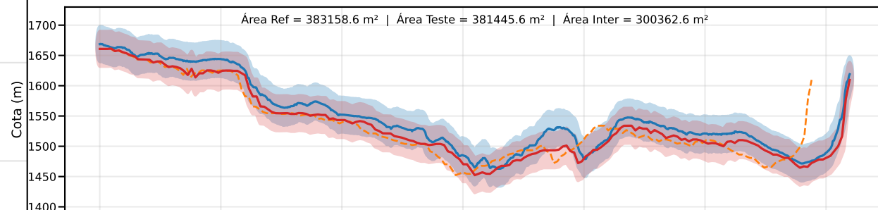
Classe D | PEC-PCD (Vertical)=37.5 m | EQ = 50m | dm = 20.48
