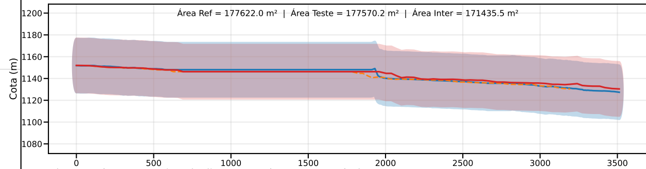
Classe C | PEC-PCD (Vertical)=30.0 m | EQ = 50m | dm = 2.74
