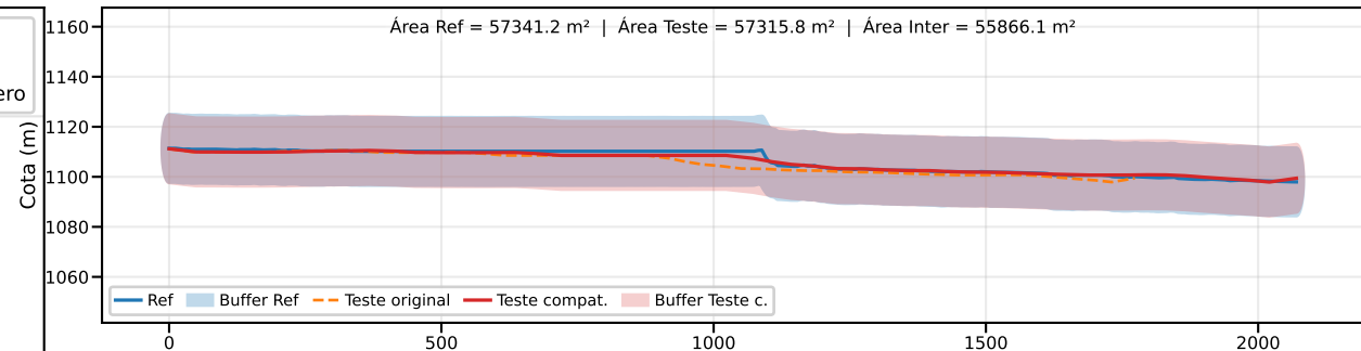
Classe B | PEC-PCD (Vertical)=25.0 m | EQ = 50m | dm = 1.12
