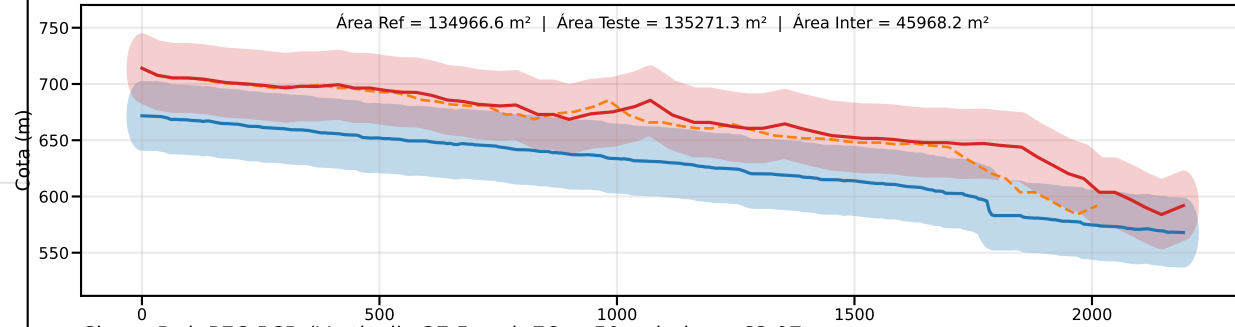
Classe D | PEC-PCD (Vertical)=37.5 m | EQ = 50m | dm = 62.07
