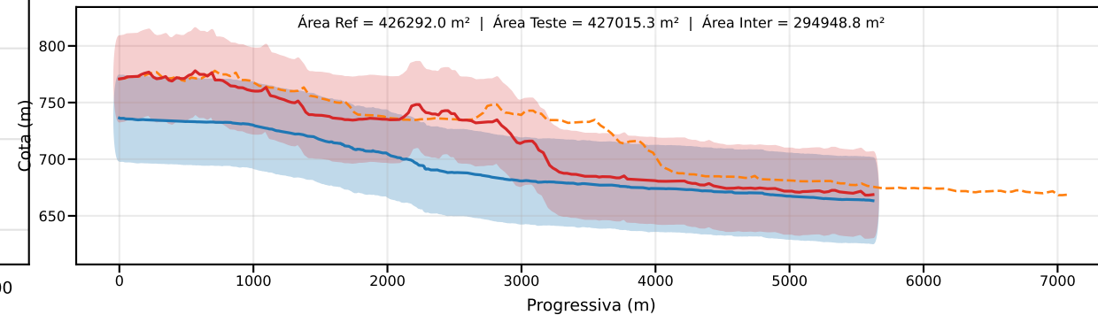
Classe D | PEC-PCD (Vertical)=37.5 m | EQ = 50m | dm = 36.24
