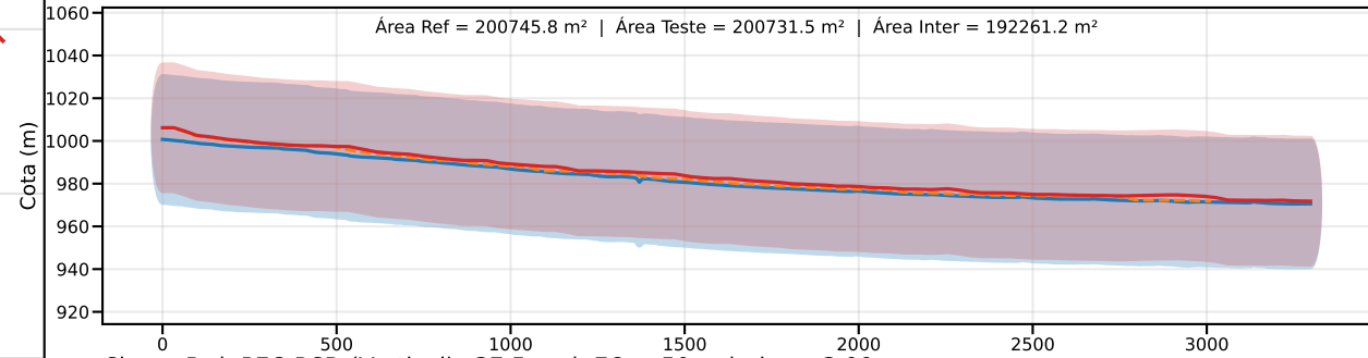
Classe D | PEC-PCD (Vertical)=37.5 m | EQ = 50m | dm = 3.99
