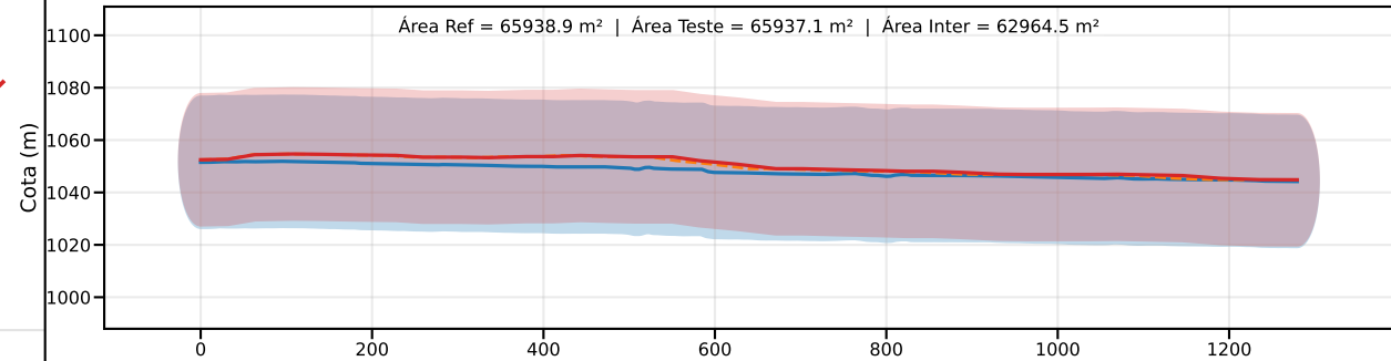
Classe C | PEC-PCD (Vertical)=30.0 m | EQ = 50m | dm = 3.53
