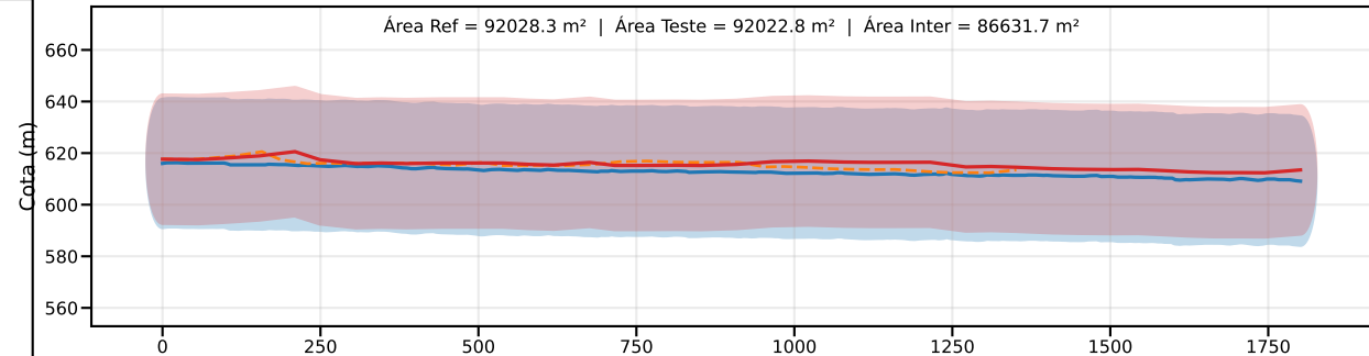
Classe C | PEC-PCD (Vertical)=30.0 m | EQ = 50m | dm = 4.61
