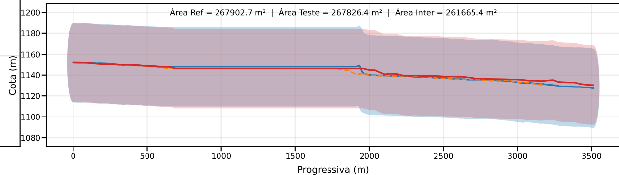
Classe D | PEC-PCD (Vertical)=37.5 m | EQ = 50m | dm = 2.74
