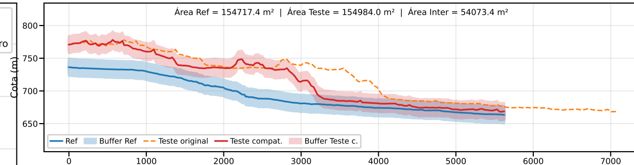
Classe B | PEC-PCD (Vertical)=25.0 m | EQ = 50m | dm = 36.12
