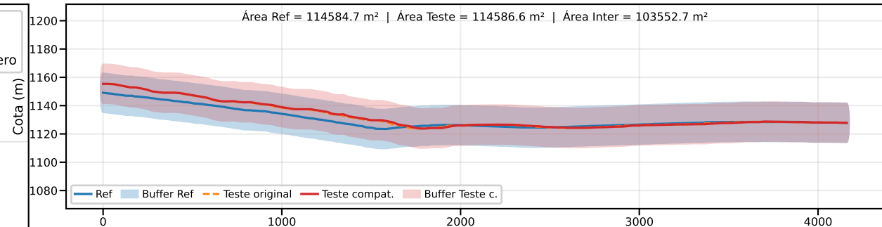
Classe B | PEC-PCD (Vertical)=25.0 m | EQ = 50m | dm = 4.15
