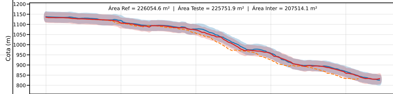
Classe C | PEC-PCD (Vertical)=30.0 m | EQ = 50m | dm = 6.46
