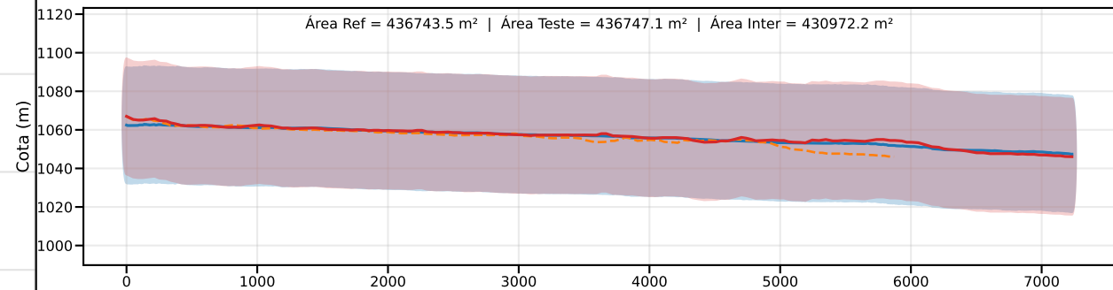
Classe D | PEC-PCD (Vertical)=37.5 m | EQ = 50m | dm = 1.25
