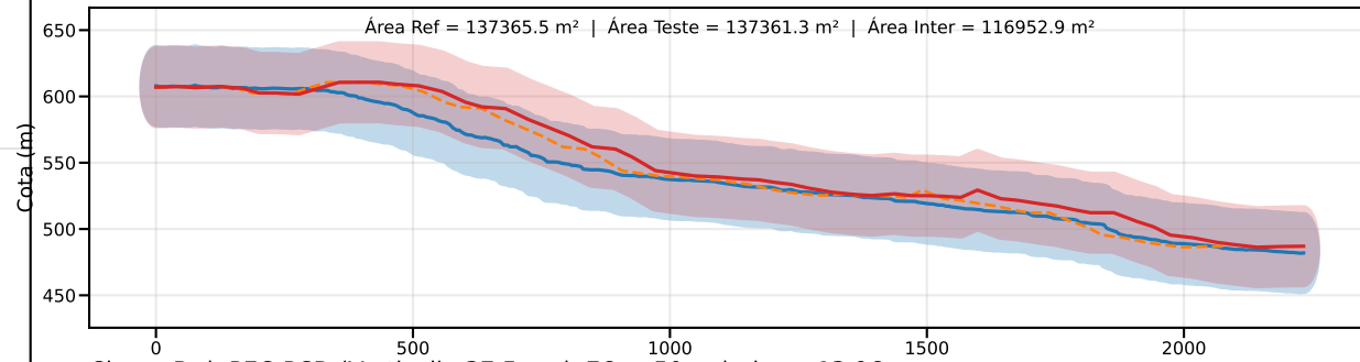
Classe D | PEC-PCD (Vertical)=37.5 m | EQ = 50m | dm = 13.96
