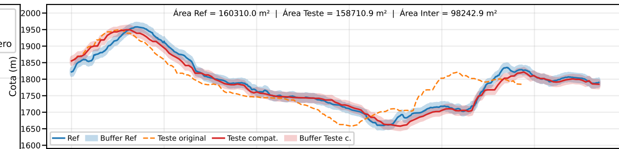
Classe B | PEC-PCD (Vertical)=25.0 m | EQ = 50m | dm = 17.74
