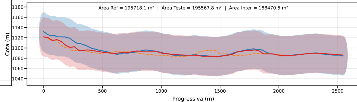
Classe D | PEC-PCD (Vertical)=37.5 m | EQ = 50m | dm = 4.37
