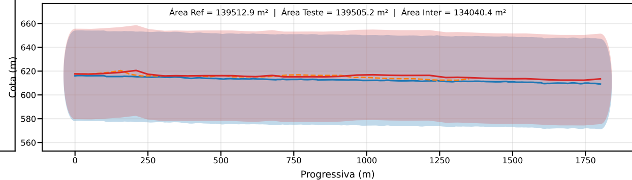
Classe D | PEC-PCD (Vertical)=37.5 m | EQ = 50m | dm = 4.62
