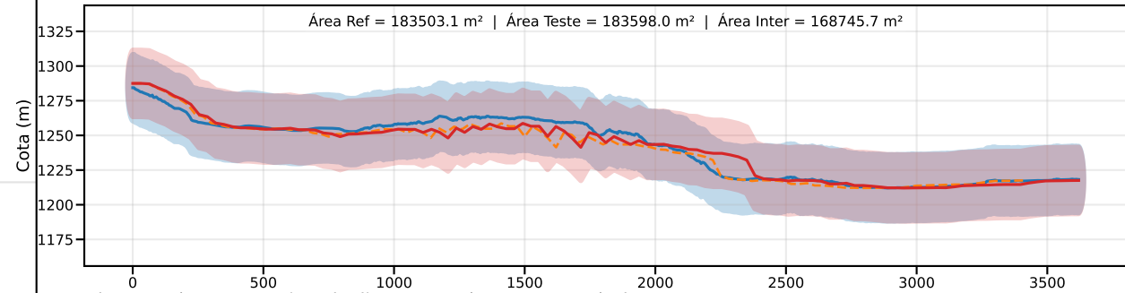
Classe C | PEC-PCD (Vertical)=30.0 m | EQ = 50m | dm = 6.30
