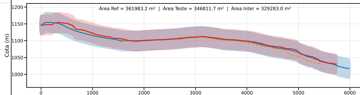
Classe D | PEC-PCD (Vertical)=37.5 m | EQ = 50m | dm = 9.90
