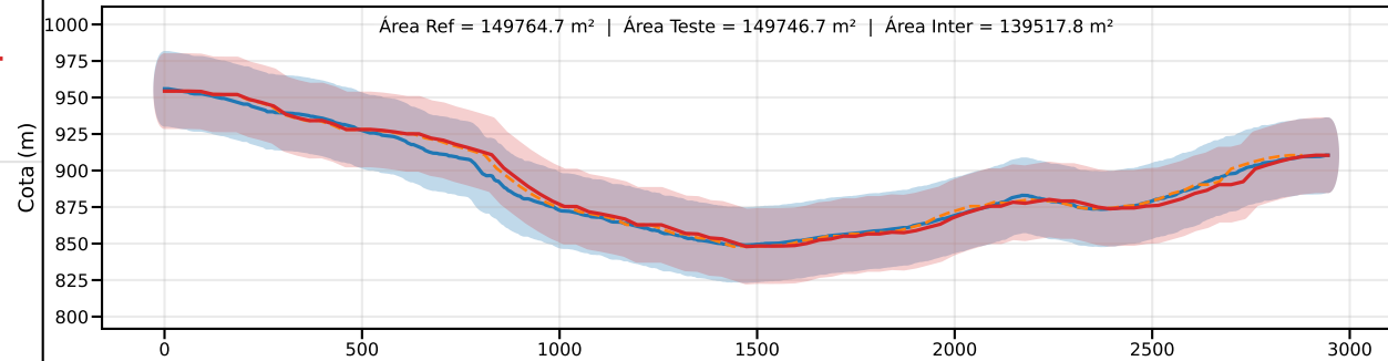
Classe C | PEC-PCD (Vertical)=30.0 m | EQ = 50m | dm = 5.36
