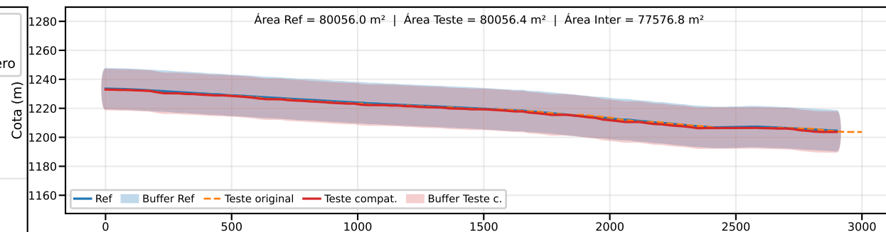
Classe B | PEC-PCD (Vertical)=25.0 m | EQ = 50m | dm = 1.33
