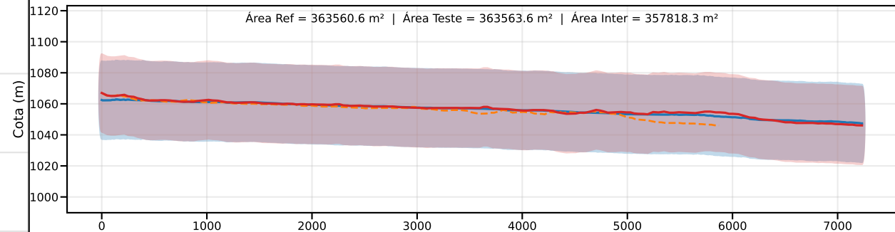
Classe C | PEC-PCD (Vertical)=30.0 m | EQ = 50m | dm = 1.25
