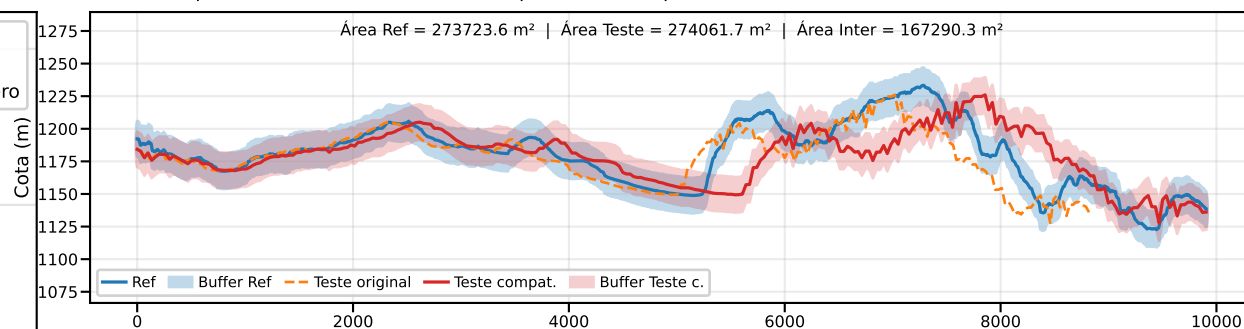
Classe B | PEC-PCD (Vertical)=25.0 m | EQ = 50m | dm = 19.71
