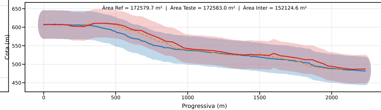
Classe D | PEC-PCD (Vertical)=37.5 m | EQ = 50m | dm = 13.96
