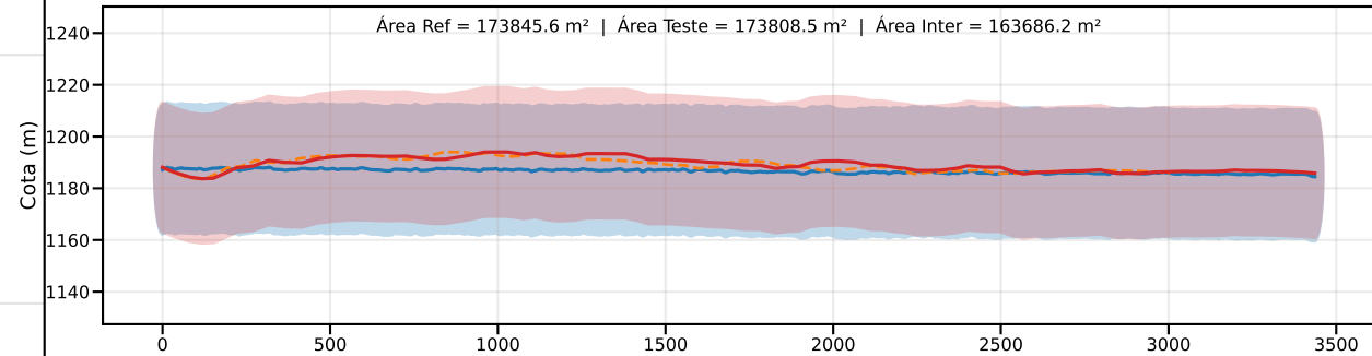
Classe C | PEC-PCD (Vertical)=30.0 m | EQ = 50m | dm = 4.59
