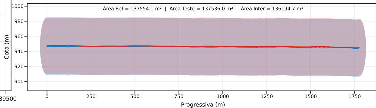
Classe D | PEC-PCD (Vertical)=37.5 m | EQ = 50m | dm = 1.16
