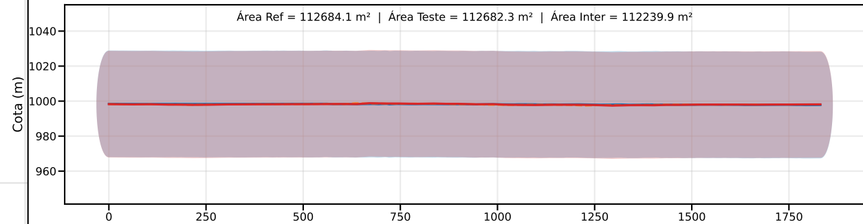
Classe D | PEC-PCD (Vertical)=37.5 m | EQ = 50m | dm = 0.37
