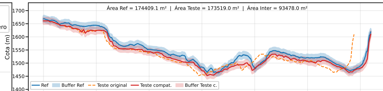
Classe B | PEC-PCD (Vertical)=25.0 m | EQ = 50m | dm = 20.44
