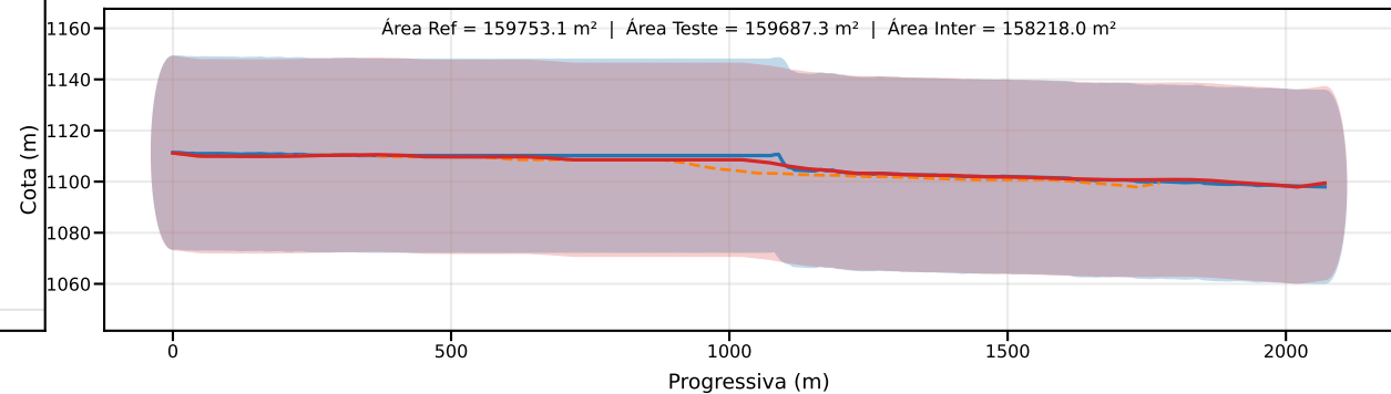
Classe D | PEC-PCD (Vertical)=37.5 m | EQ = 50m | dm = 1.13
