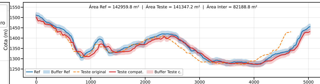
Classe B | PEC-PCD (Vertical)=25.0 m | EQ = 50m | dm = 19.03
