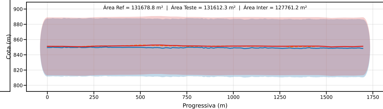
Classe D | PEC-PCD (Vertical)=37.5 m | EQ = 50m | dm = 3.51
