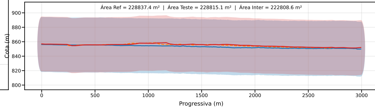
Classe D | PEC-PCD (Vertical)=37.5 m | EQ = 50m | dm = 3.10
