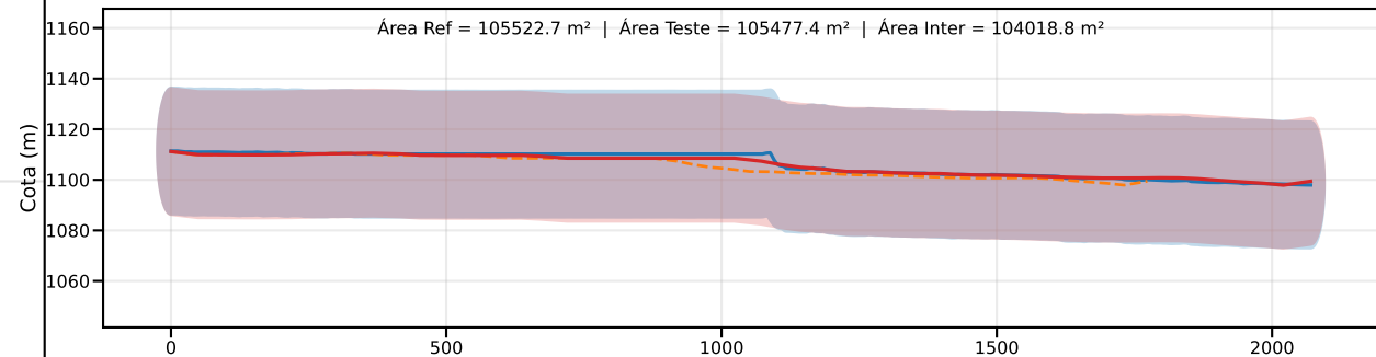
Classe C | PEC-PCD (Vertical)=30.0 m | EQ = 50m | dm = 1.12
