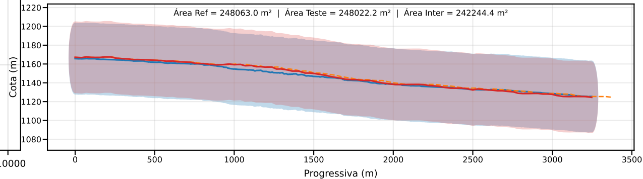
Classe D | PEC-PCD (Vertical)=37.5 m | EQ = 50m | dm = 2.76
