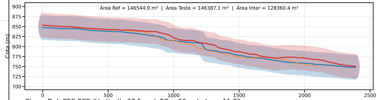
Classe D | PEC-PCD (Vertical)=37.5 m | EQ = 50m | dm = 11.70
