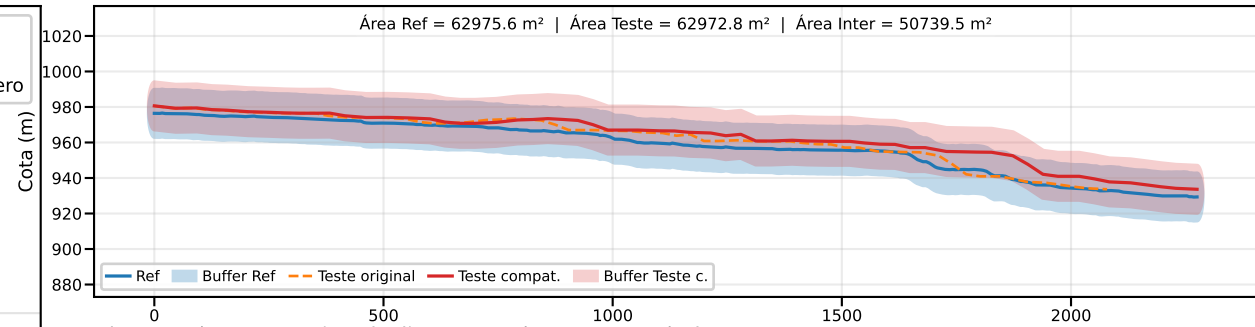
Classe B | PEC-PCD (Vertical)=25.0 m | EQ = 50m | dm = 8.36
