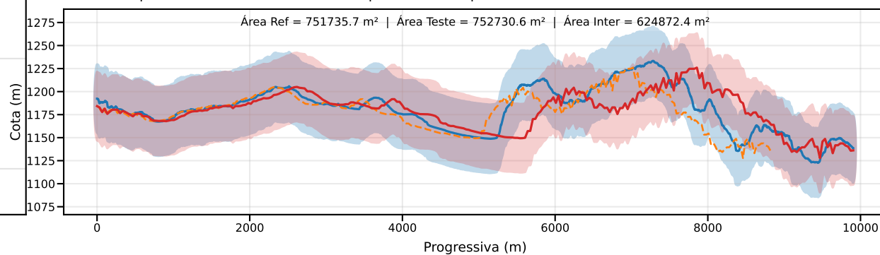
Classe D | PEC-PCD (Vertical)=37.5 m | EQ = 50m | dm = 19.86
