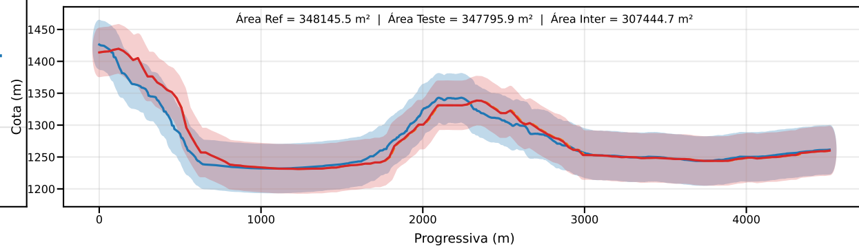
Classe D | PEC-PCD (Vertical)=37.5 m | EQ = 50m | dm = 13.79
