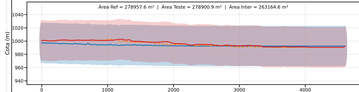
Classe D | PEC-PCD (Vertical)=37.5 m | EQ = 50m | dm = 5.34
