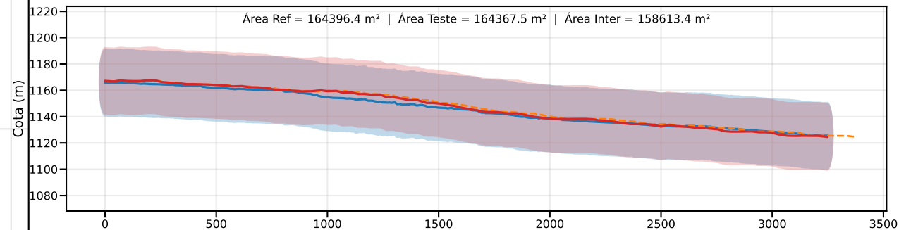
Classe C | PEC-PCD (Vertical)=30.0 m | EQ = 50m | dm = 2.76
