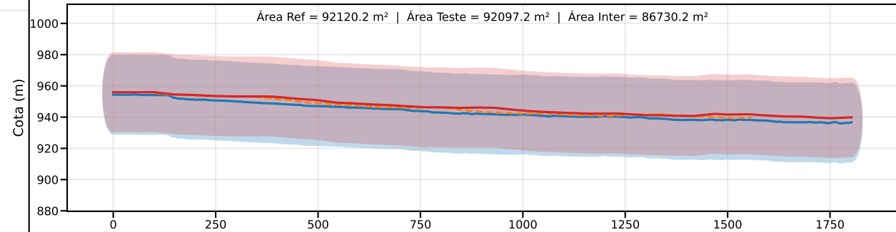
Classe C | PEC-PCD (Vertical)=30.0 m | EQ = 50m | dm = 4.60
