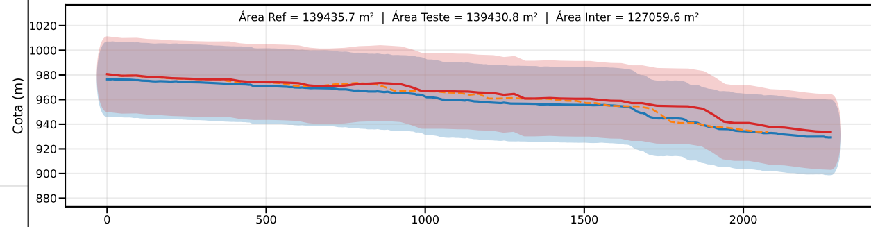
Classe D | PEC-PCD (Vertical)=37.5 m | EQ = 50m | dm = 8.37
