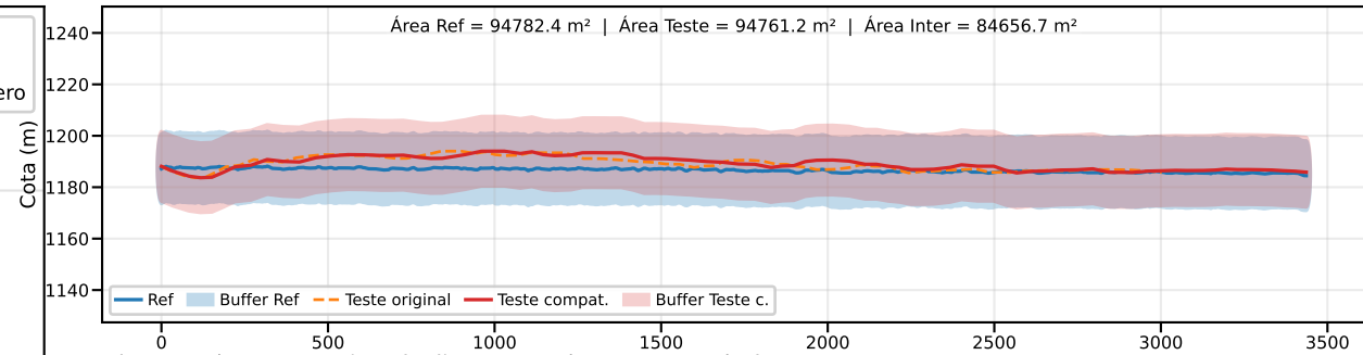
Classe B | PEC-PCD (Vertical)=25.0 m | EQ = 50m | dm = 4.59
