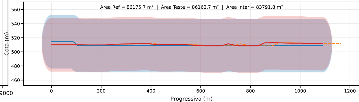
Classe D | PEC-PCD (Vertical)=37.5 m | EQ = 50m | dm = 3.26
