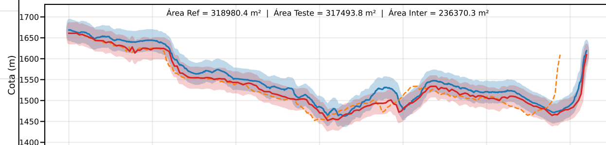
Classe C | PEC-PCD (Vertical)=30.0 m | EQ = 50m | dm = 20.46
