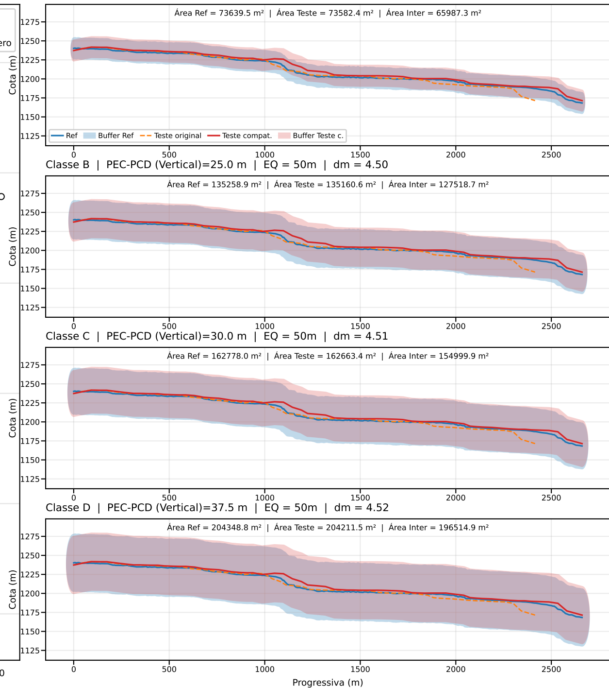
Classe A | PEC-PCD (Vertical)=13.7 m | EQ = 50m | dm = 4.48
