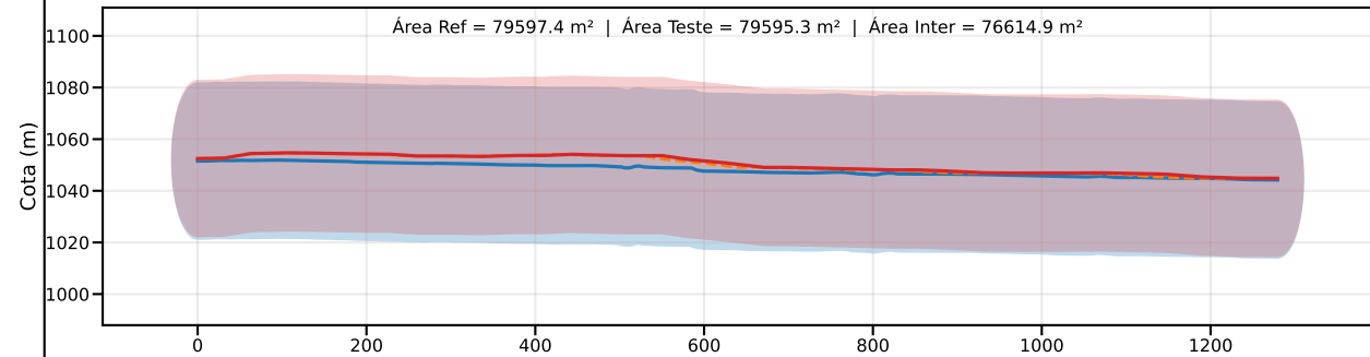
Classe D | PEC-PCD (Vertical)=37.5 m | EQ = 50m | dm = 3.51
