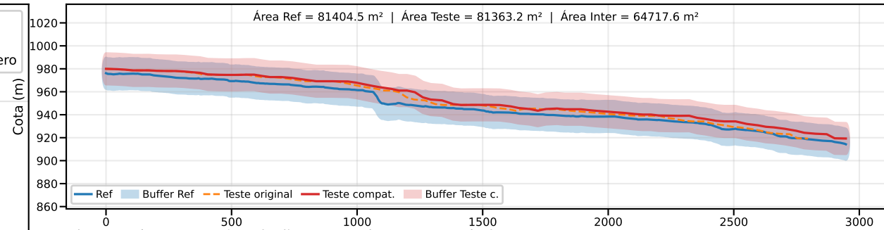
Classe B | PEC-PCD (Vertical)=25.0 m | EQ = 50m | dm = 8.84
