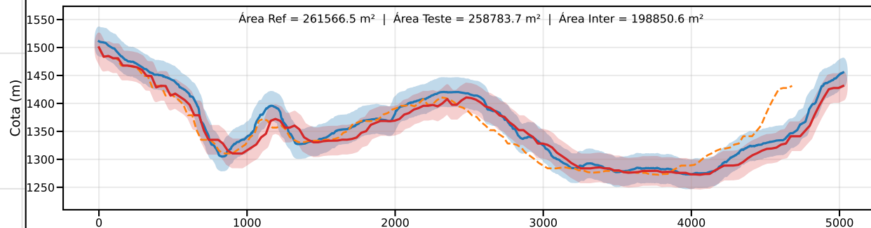
Classe C | PEC-PCD (Vertical)=30.0 m | EQ = 50m | dm = 19.12
