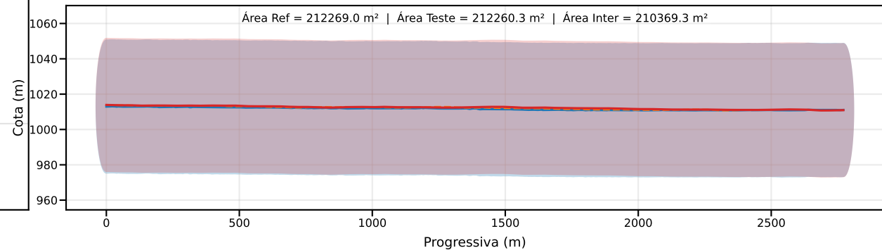
Classe D | PEC-PCD (Vertical)=37.5 m | EQ = 50m | dm = 1.05
