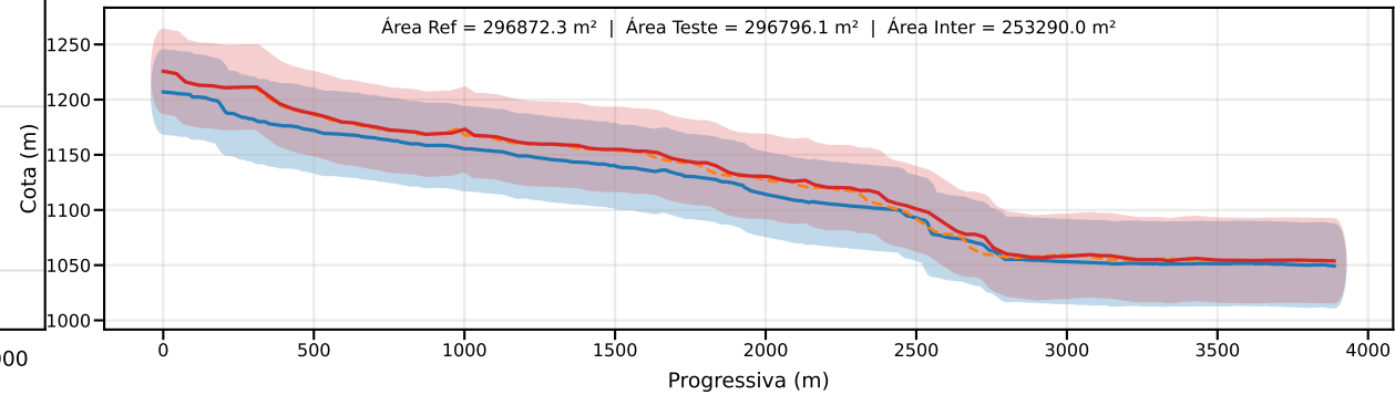
Classe D | PEC-PCD (Vertical)=37.5 m | EQ = 50m | dm = 17.30
