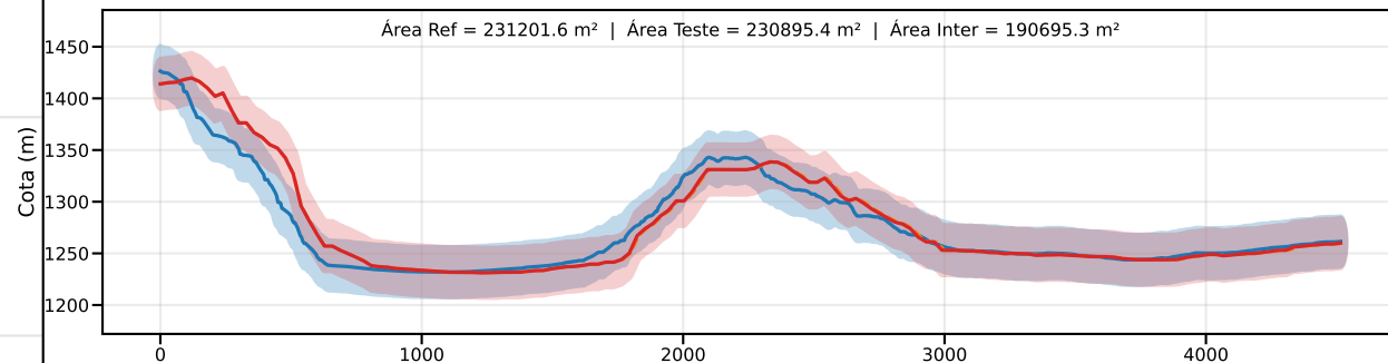
Classe C | PEC-PCD (Vertical)=30.0 m | EQ = 50m | dm = 13.78
