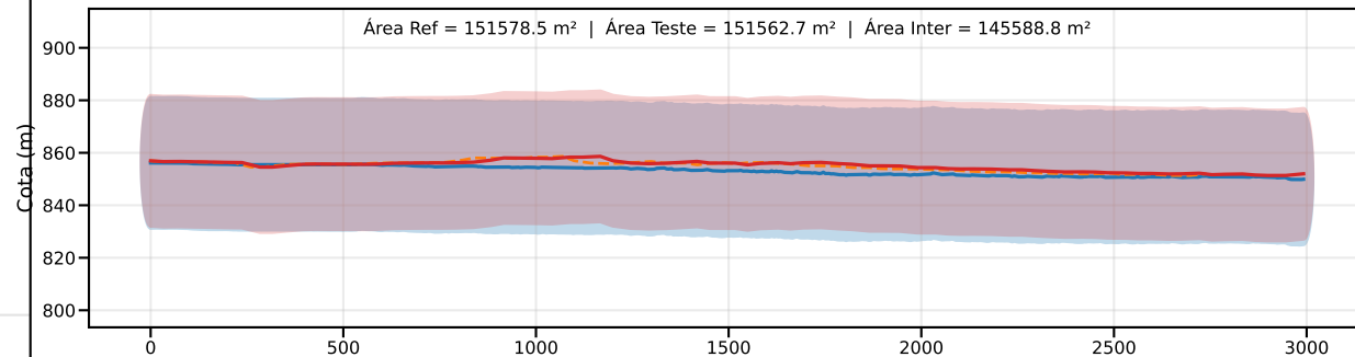
Classe C | PEC-PCD (Vertical)=30.0 m | EQ = 50m | dm = 3.10
