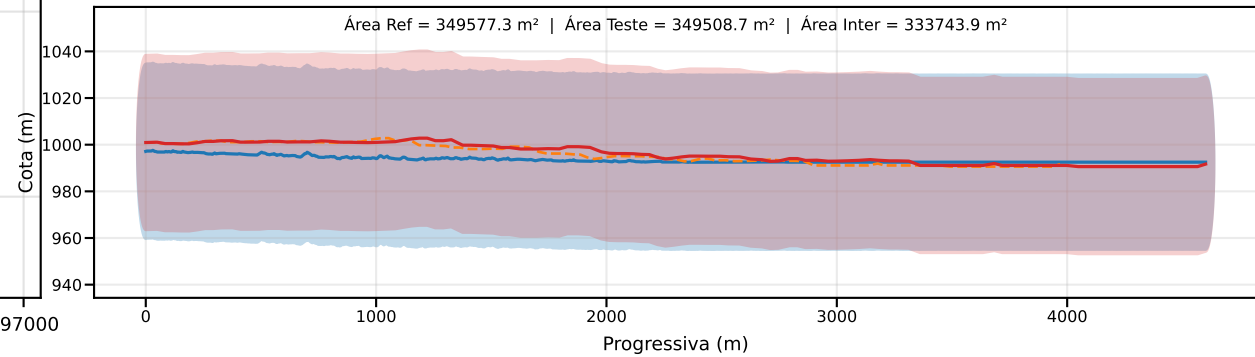
Classe D | PEC-PCD (Vertical)=37.5 m | EQ = 50m | dm = 5.34
