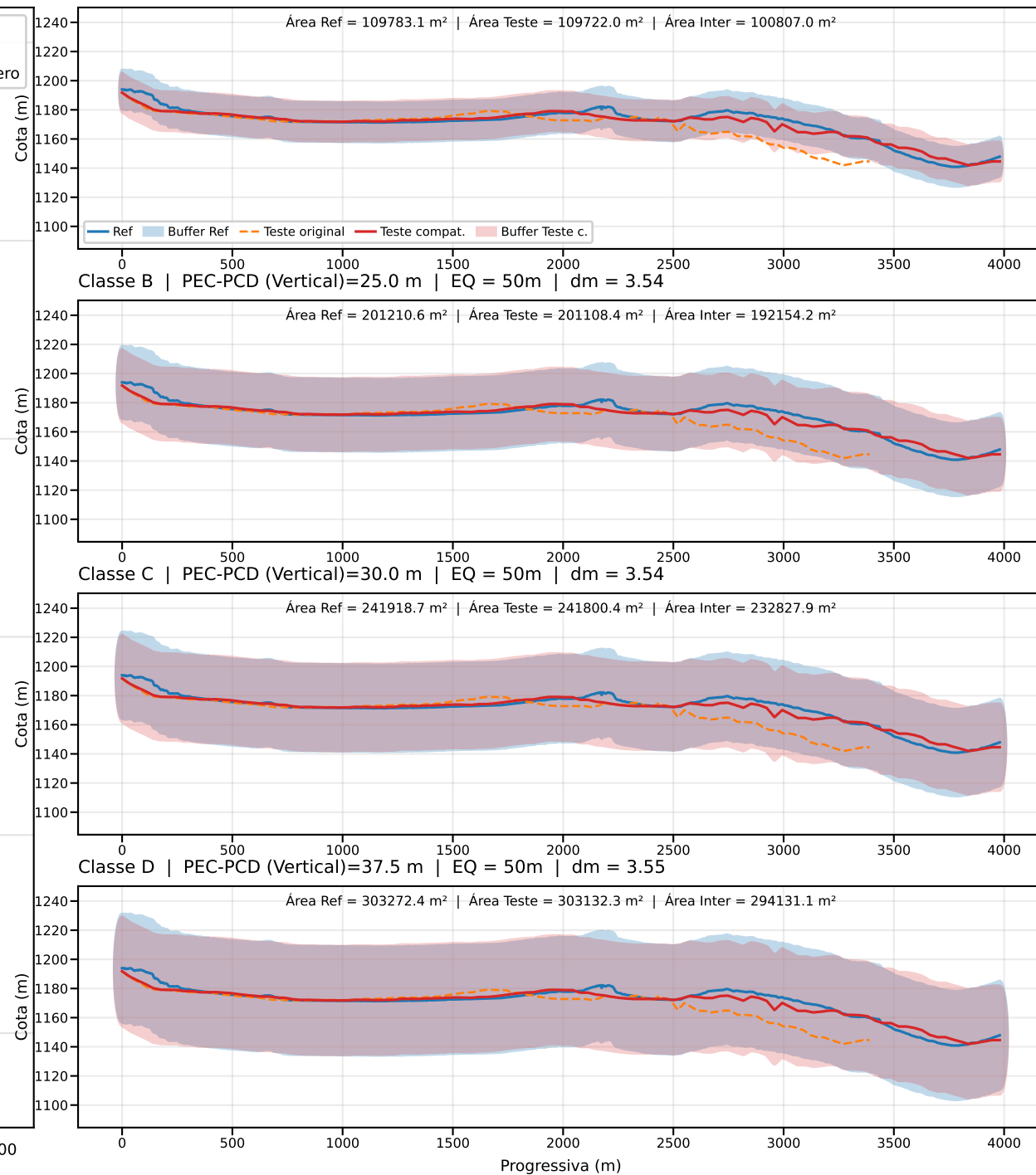
Classe A | PEC-PCD (Vertical)=13.7 m | EQ = 50m | dm = 3.52
