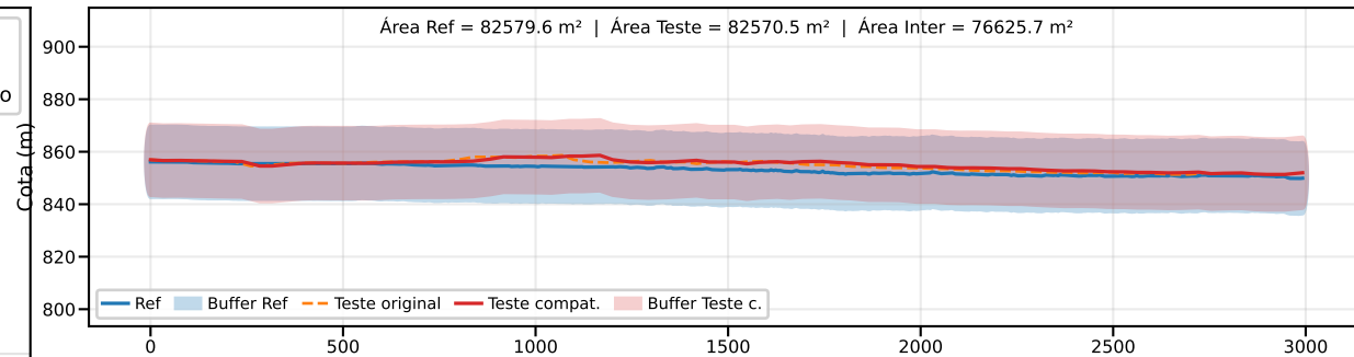
Classe B | PEC-PCD (Vertical)=25.0 m | EQ = 50m | dm = 3.10
