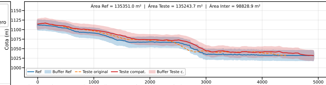
Classe B | PEC-PCD (Vertical)=25.0 m | EQ = 50m | dm = 11.61
