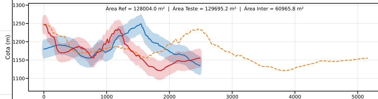
Classe C | PEC-PCD (Vertical)=30.0 m | EQ = 50m | dm = 44.30
