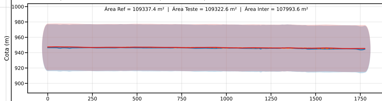
Classe D | PEC-PCD (Vertical)=37.5 m | EQ = 50m | dm = 1.16
