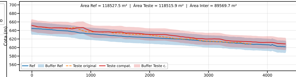
Classe B | PEC-PCD (Vertical)=25.0 m | EQ = 50m | dm = 10.53
