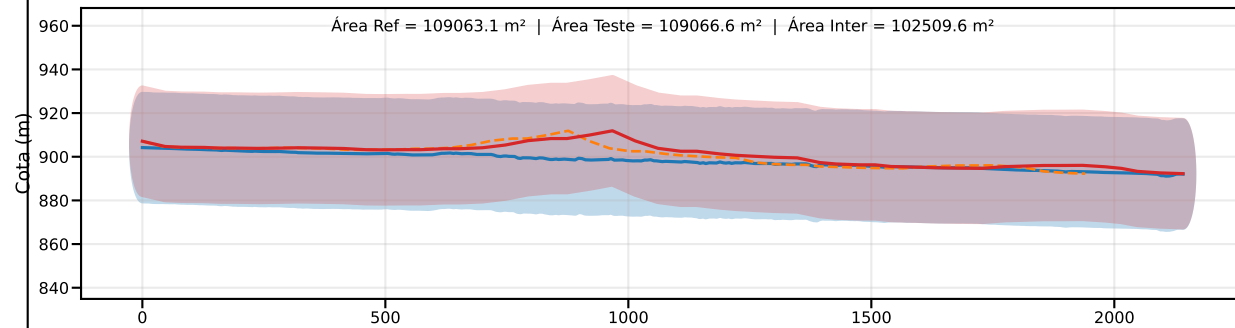
Classe C | PEC-PCD (Vertical)=30.0 m | EQ = 50m | dm = 4.71
