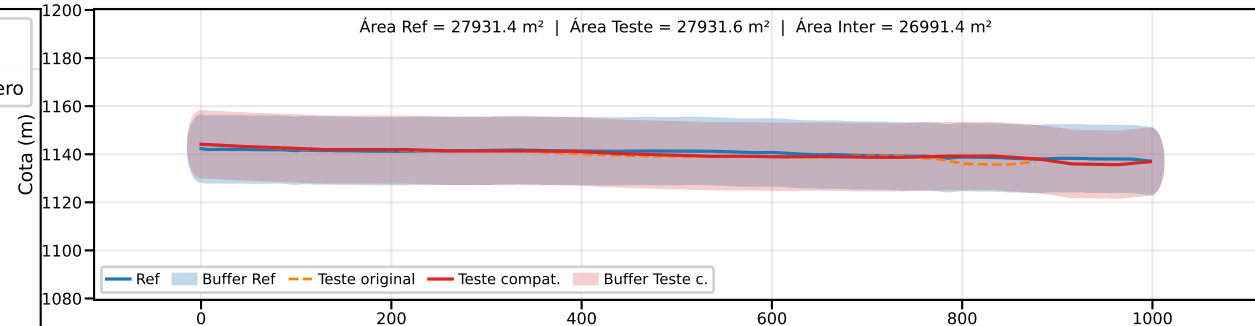
Classe B | PEC-PCD (Vertical)=25.0 m | EQ = 50m | dm = 1.46
