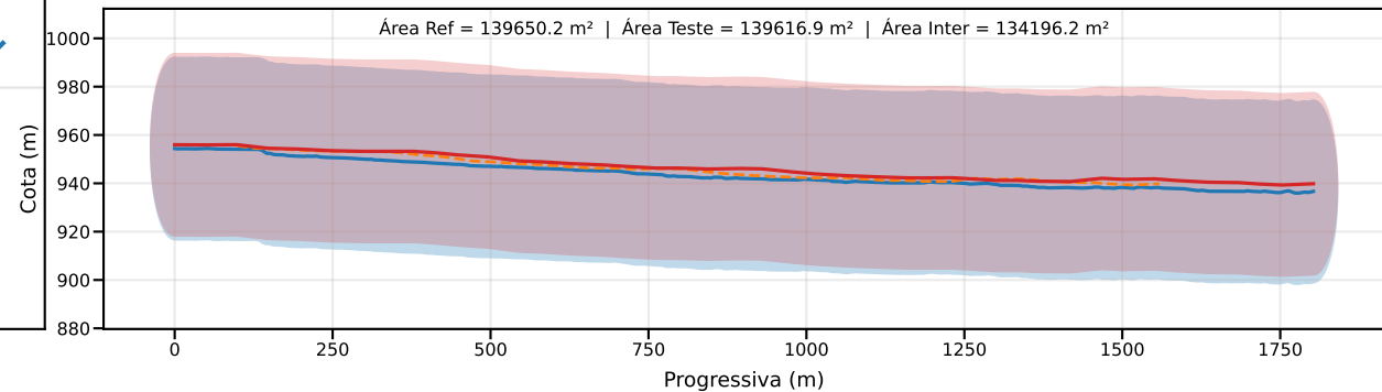
Classe D | PEC-PCD (Vertical)=37.5 m | EQ = 50m | dm = 4.60
