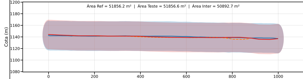
Classe C | PEC-PCD (Vertical)=30.0 m | EQ = 50m | dm = 1.46
