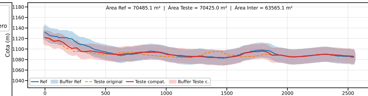
Classe B | PEC-PCD (Vertical)=25.0 m | EQ = 50m | dm = 4.30
