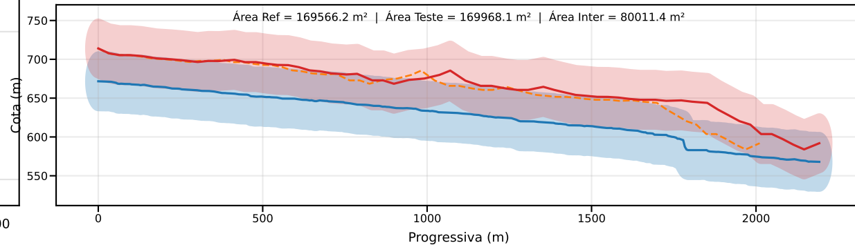
Classe D | PEC-PCD (Vertical)=37.5 m | EQ = 50m | dm = 62.07
