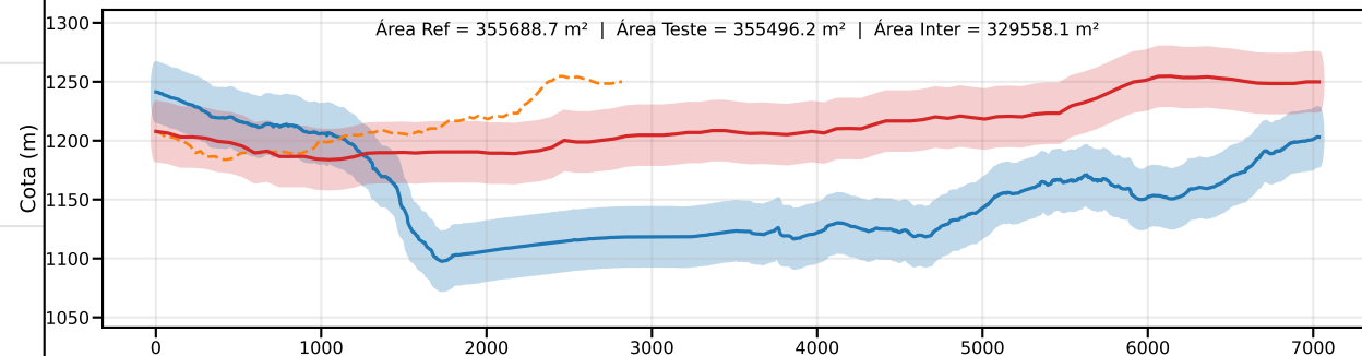
Classe C | PEC-PCD (Vertical)=30.0 m | EQ = 50m | dm = 5.77
