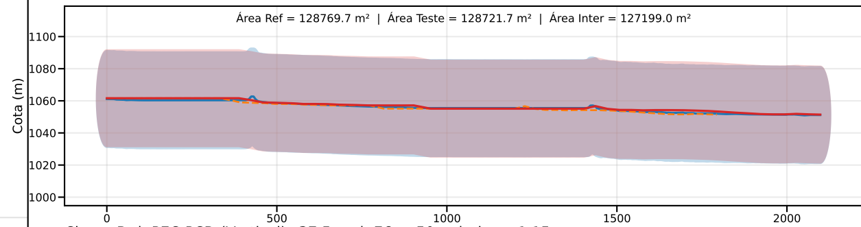
Classe D | PEC-PCD (Vertical)=37.5 m | EQ = 50m | dm = 1.15
