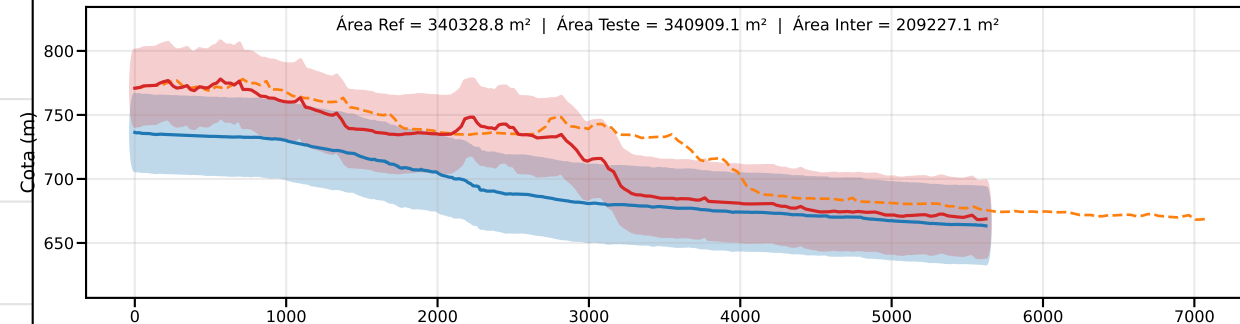
Classe D | PEC-PCD (Vertical)=37.5 m | EQ = 50m | dm = 36.24
