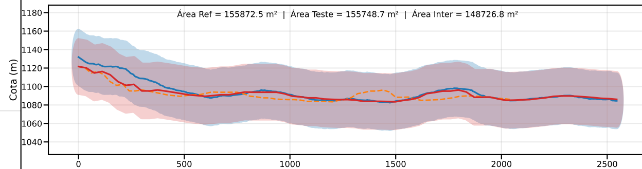
Classe D | PEC-PCD (Vertical)=37.5 m | EQ = 50m | dm = 4.37
