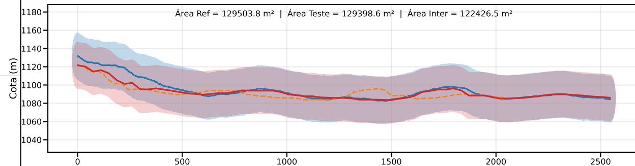
Classe C | PEC-PCD (Vertical)=30.0 m | EQ = 50m | dm = 4.32
