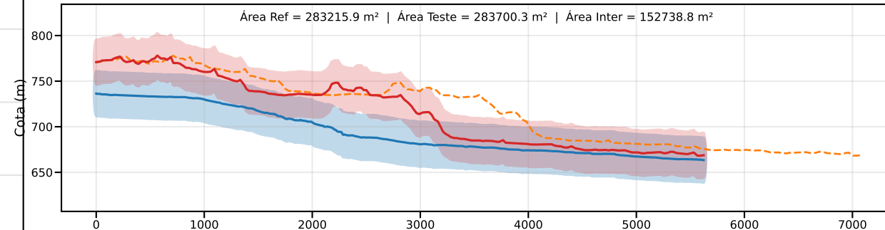
Classe C | PEC-PCD (Vertical)=30.0 m | EQ = 50m | dm = 36.24
