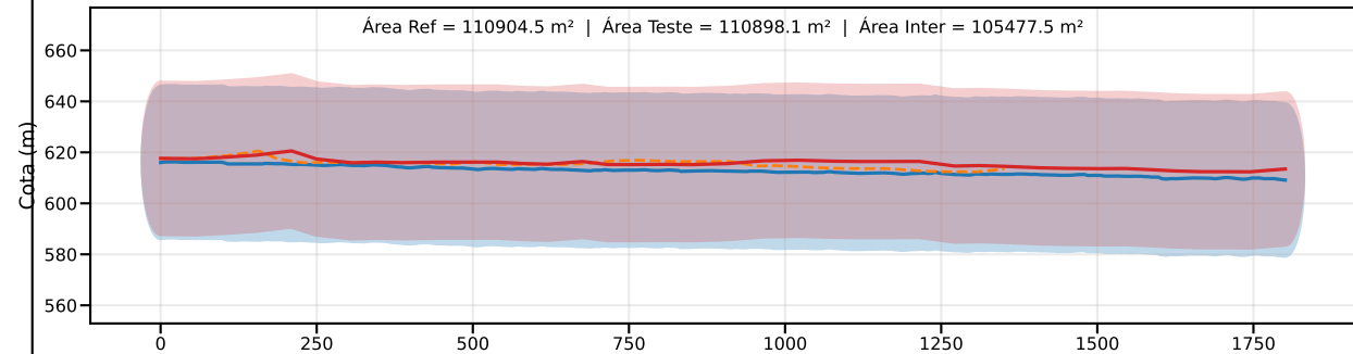
Classe D | PEC-PCD (Vertical)=37.5 m | EQ = 50m | dm = 4.62
