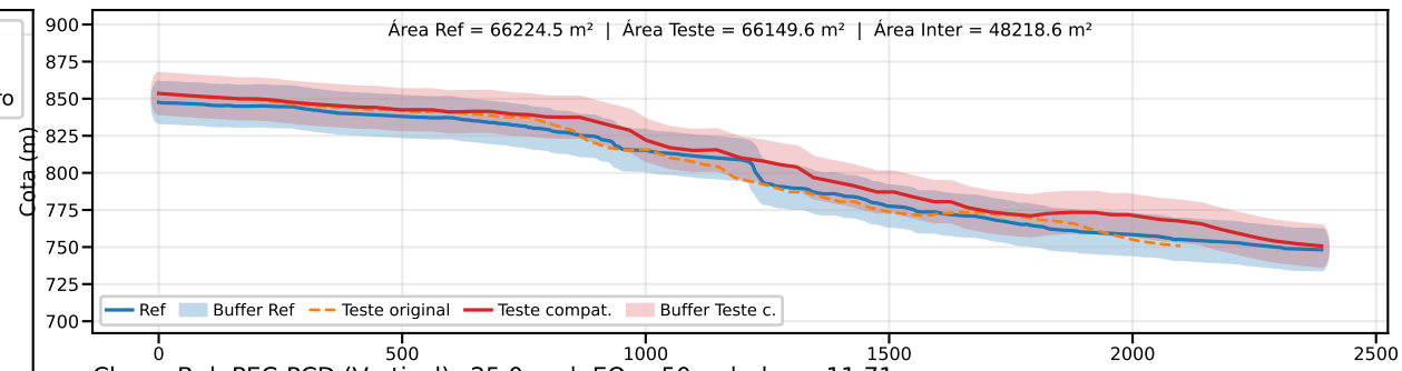
Classe B | PEC-PCD (Vertical)=25.0 m | EQ = 50m | dm = 11.71
