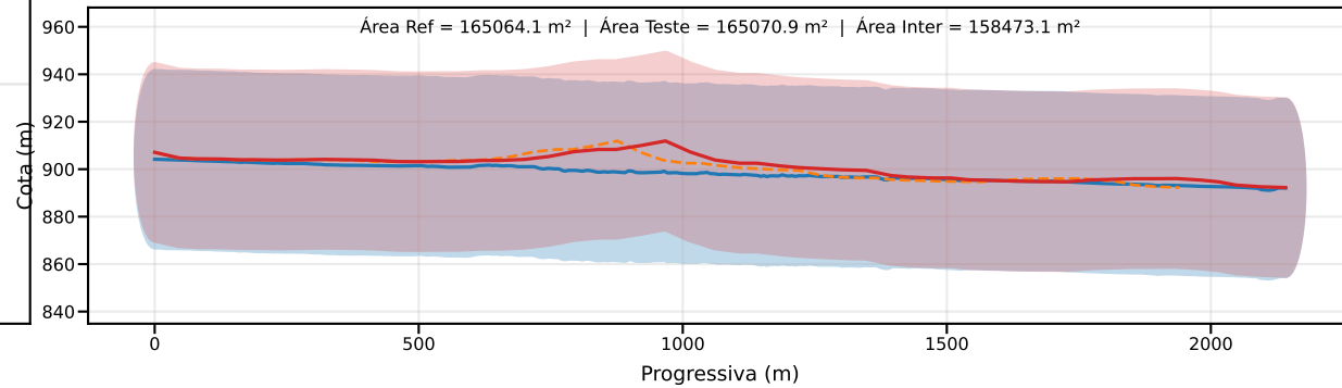
Classe D | PEC-PCD (Vertical)=37.5 m | EQ = 50m | dm = 4.70
