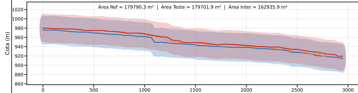
Classe D | PEC-PCD (Vertical)=37.5 m | EQ = 50m | dm = 8.85
