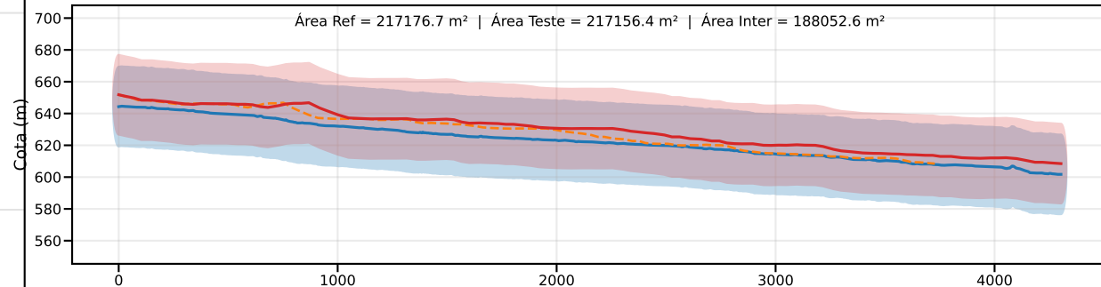
Classe C | PEC-PCD (Vertical)=30.0 m | EQ = 50m | dm = 10.54
