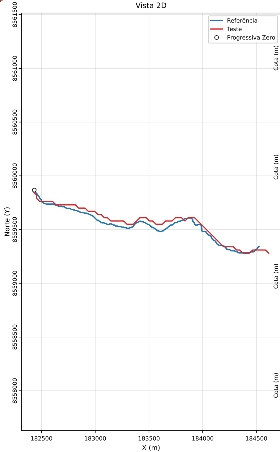
Classe A | PEC-PCD (Vertical)=13.7 m | EQ = 50m | dm = 11.03
