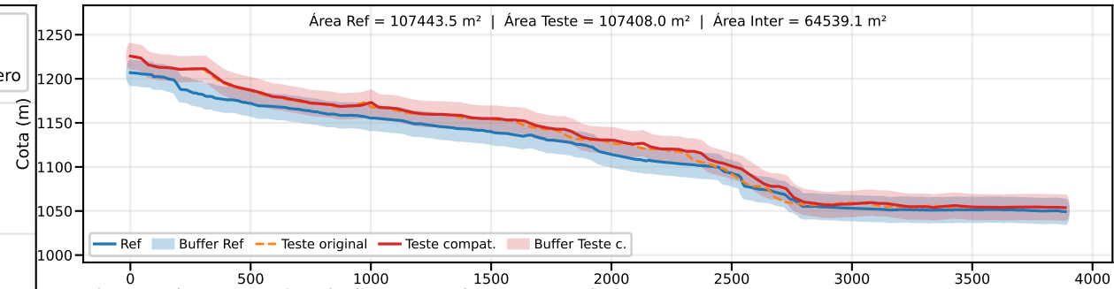
Classe B | PEC-PCD (Vertical)=25.0 m | EQ = 50m | dm = 17.26
