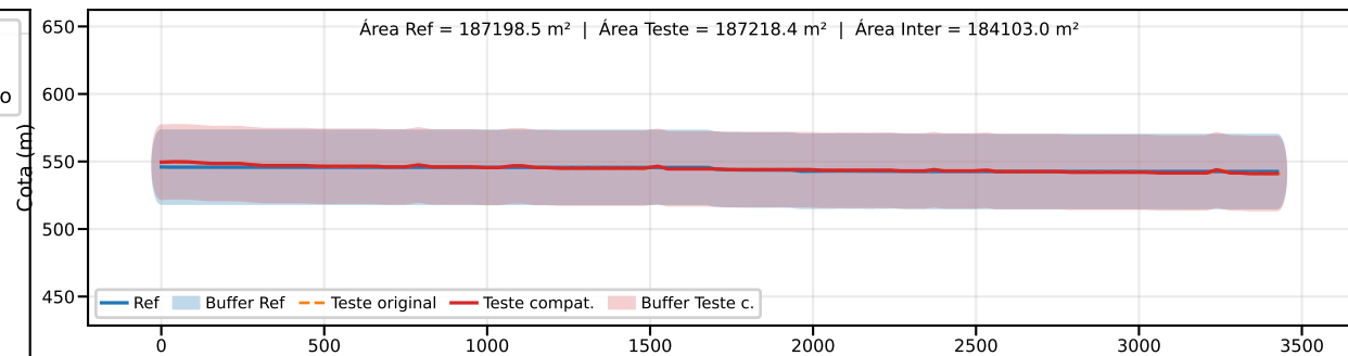
Classe B | PEC-PCD (Vertical)=50.0 m | EQ = 100m | dm = 1.44
