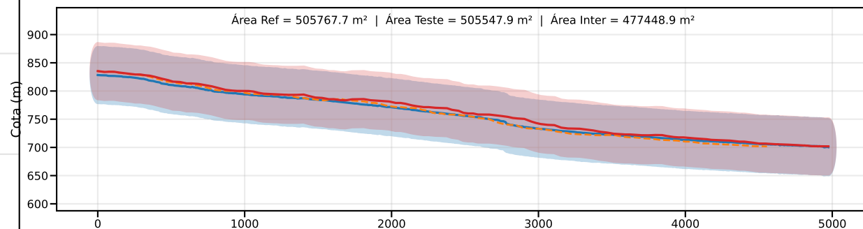
Classe C | PEC-PCD (Vertical)=60.0 m | EQ = 100m | dm = 8.80
