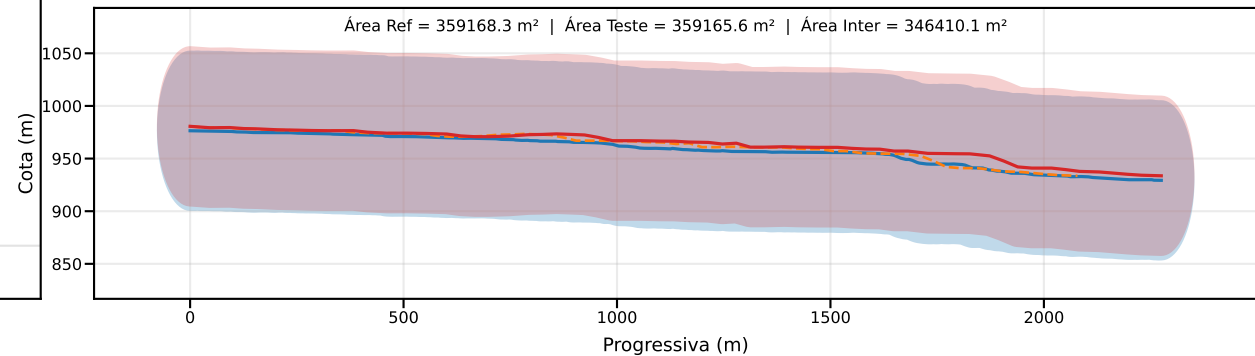
Classe D | PEC-PCD (Vertical)=75.0 m | EQ = 100m | dm = 8.37
