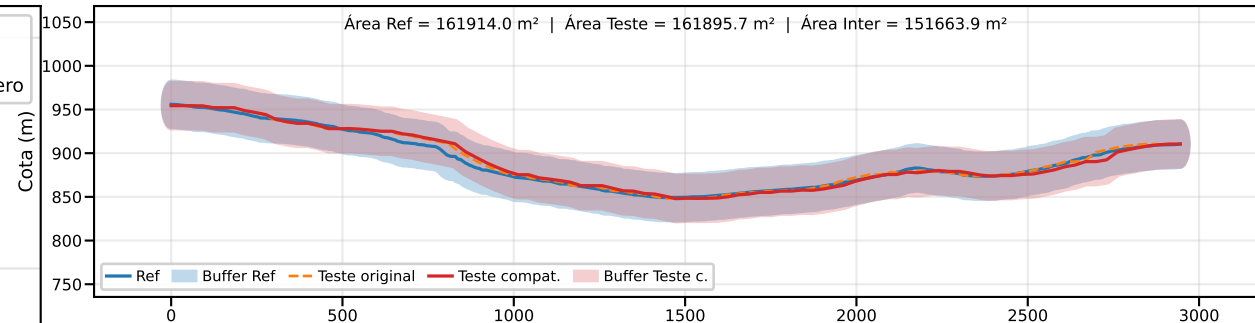
Classe B | PEC-PCD (Vertical)=50.0 m | EQ = 100m | dm = 5.32
