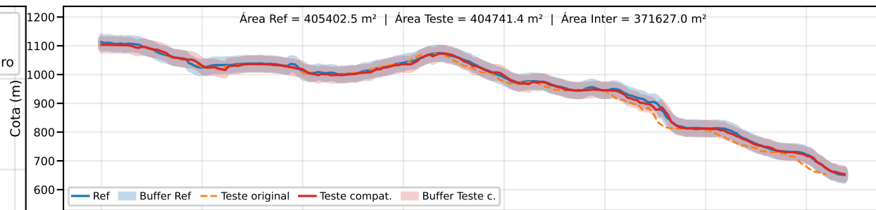
Classe B | PEC-PCD (Vertical)=50.0 m | EQ = 100m | dm = 7.11
