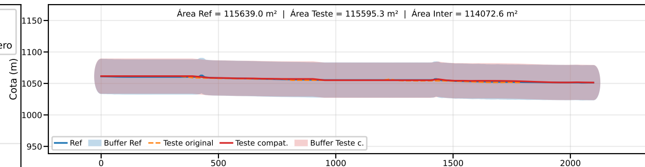
Classe B | PEC-PCD (Vertical)=50.0 m | EQ = 100m | dm = 1.15
