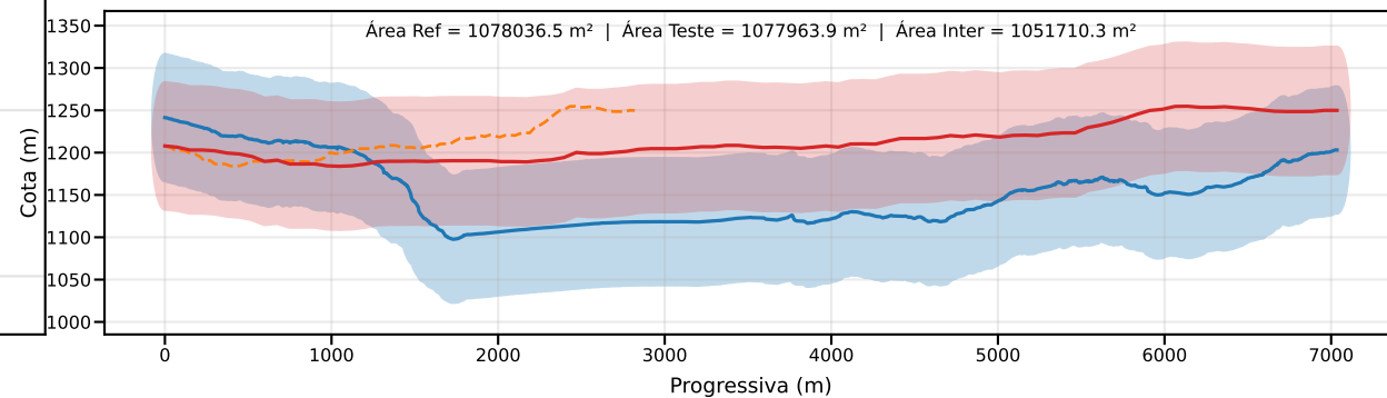
Classe D | PEC-PCD (Vertical)=75.0 m | EQ = 100m | dm = 5.75
