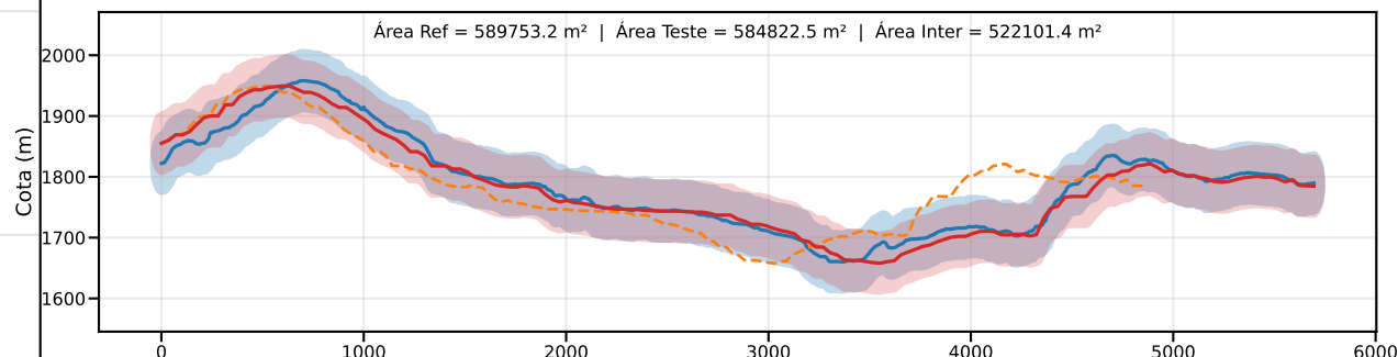
Classe C | PEC-PCD (Vertical)=60.0 m | EQ = 100m | dm = 18.32
