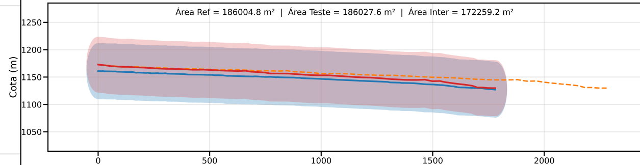
Classe C | PEC-PCD (Vertical)=60.0 m | EQ = 100m | dm = 11.63
