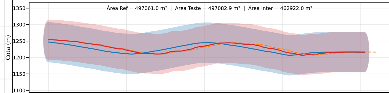
Classe D | PEC-PCD (Vertical)=75.0 m | EQ = 100m | dm = 12.91
