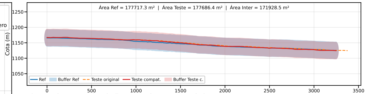
Classe B | PEC-PCD (Vertical)=50.0 m | EQ = 100m | dm = 2.76
