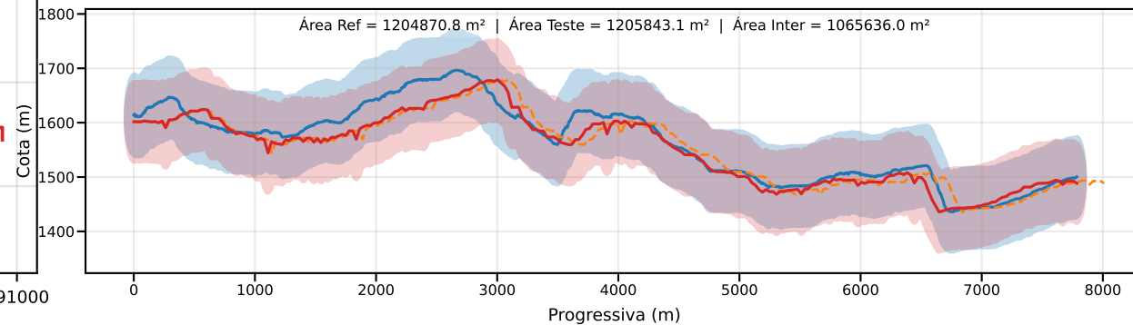
Classe D | PEC-PCD (Vertical)=75.0 m | EQ = 100m | dm = 27.21
