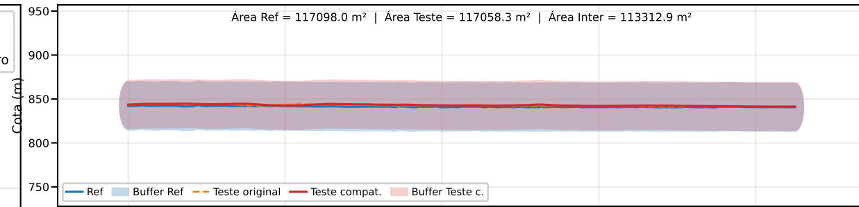
Classe B | PEC-PCD (Vertical)=50.0 m | EQ = 100m | dm = 2.74
