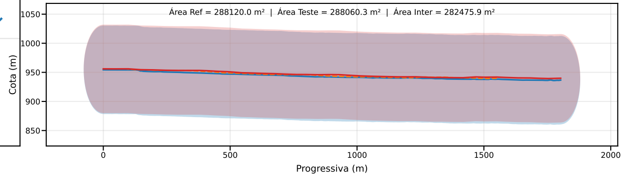
Classe D | PEC-PCD (Vertical)=75.0 m | EQ = 100m | dm = 4.62
