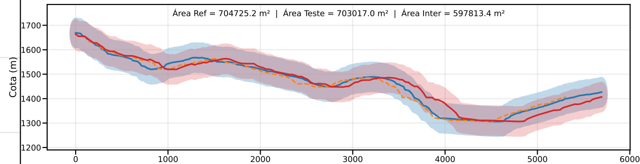
Classe D | PEC-PCD (Vertical)=75.0 m | EQ = 100m | dm = 28.68
