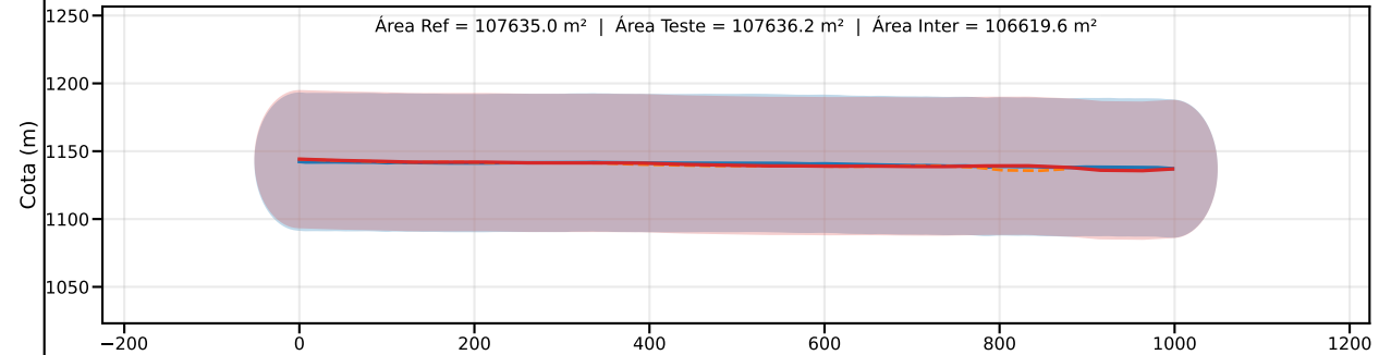
Classe C | PEC-PCD (Vertical)=60.0 m | EQ = 100m | dm = 1.49
