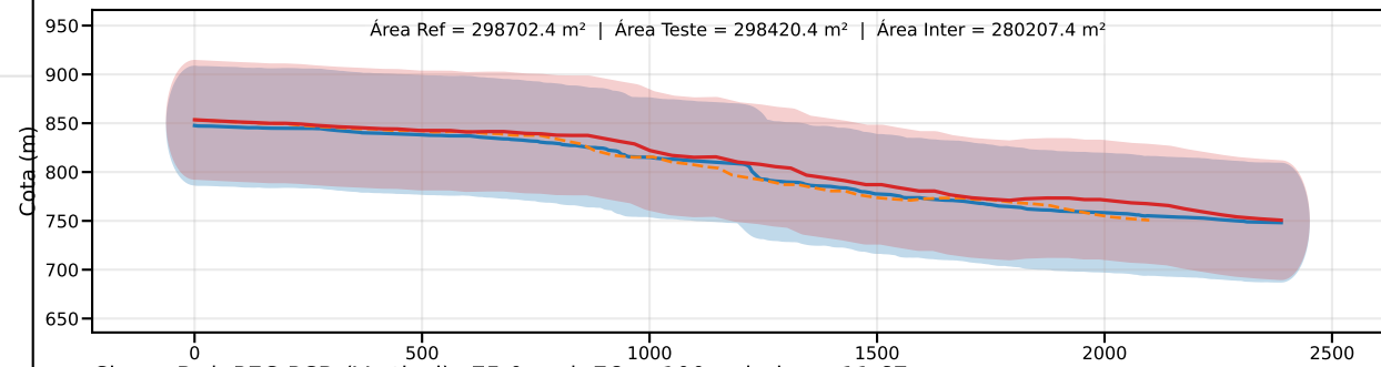
Classe D | PEC-PCD (Vertical)=75.0 m | EQ = 100m | dm = 11.67
