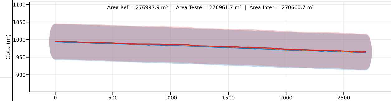
Classe C | PEC-PCD (Vertical)=60.0 m | EQ = 100m | dm = 3.60
