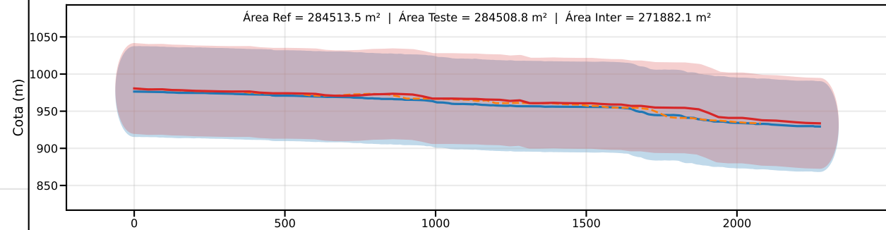
Classe D | PEC-PCD (Vertical)=75.0 m | EQ = 100m | dm = 8.37
