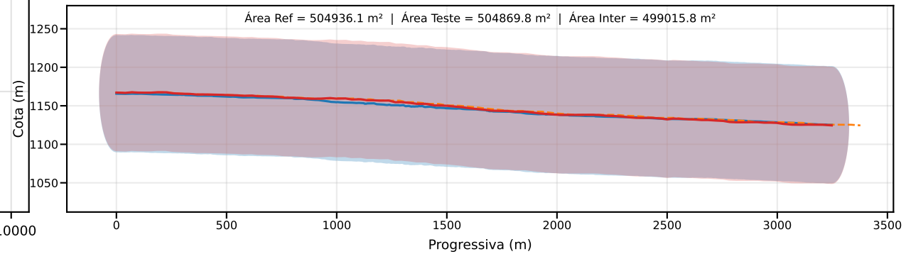
Classe D | PEC-PCD (Vertical)=75.0 m | EQ = 100m | dm = 2.76
