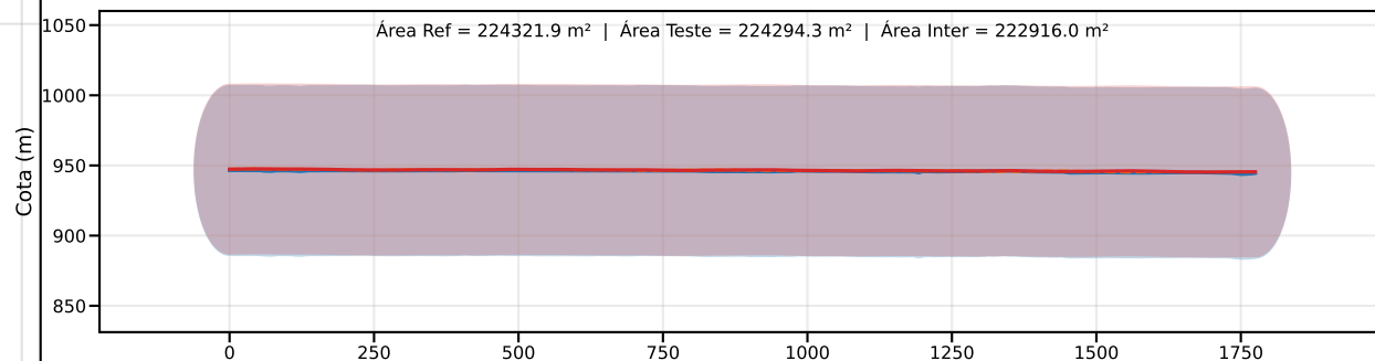
Classe D | PEC-PCD (Vertical)=75.0 m | EQ = 100m | dm = 1.19
