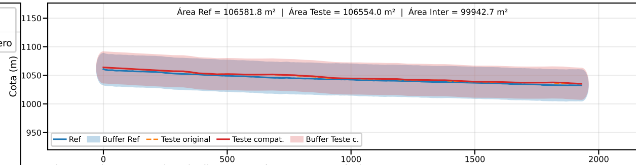
Classe B | PEC-PCD (Vertical)=50.0 m | EQ = 100m | dm = 5.30
