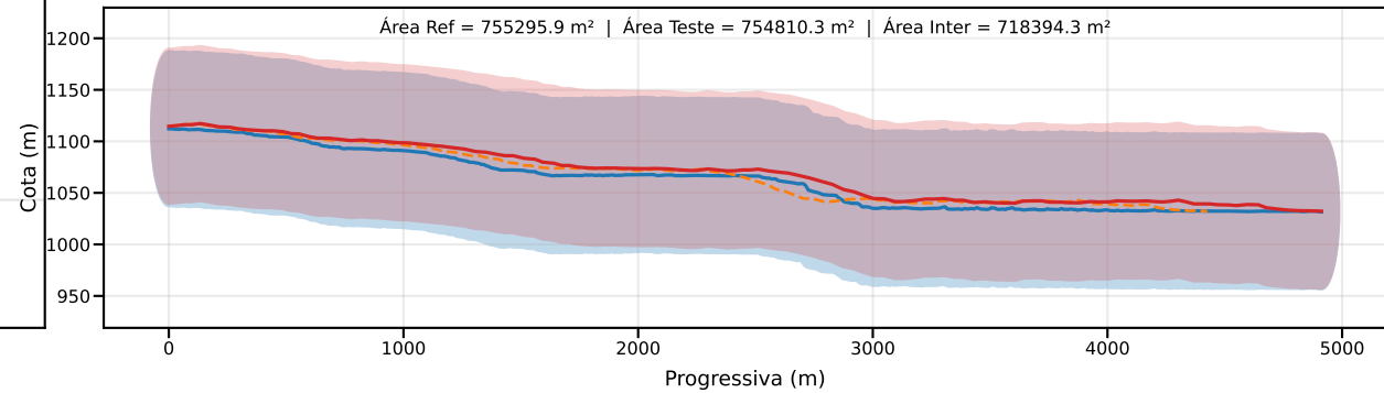
Classe D | PEC-PCD (Vertical)=75.0 m | EQ = 100m | dm = 11.52
