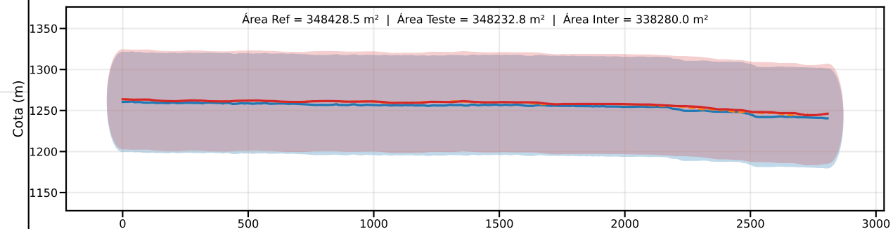
Classe D | PEC-PCD (Vertical)=75.0 m | EQ = 100m | dm = 5.53
