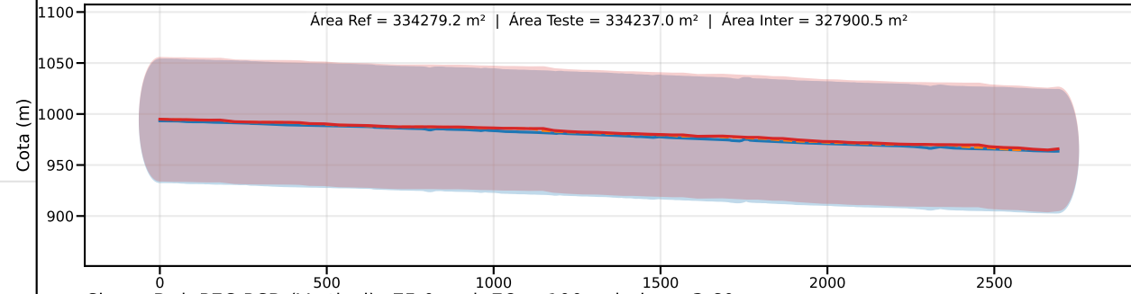
Classe D | PEC-PCD (Vertical)=75.0 m | EQ = 100m | dm = 3.60
