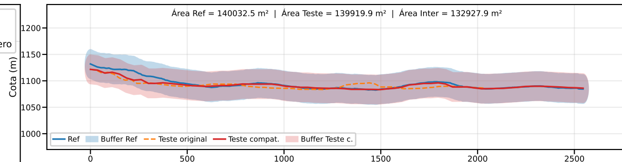
Classe B | PEC-PCD (Vertical)=50.0 m | EQ = 100m | dm = 4.43
