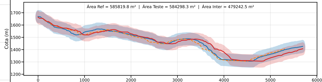
Classe C | PEC-PCD (Vertical)=60.0 m | EQ = 100m | dm = 28.67
