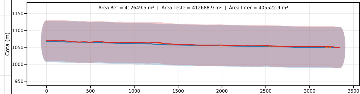
Classe D | PEC-PCD (Vertical)=75.0 m | EQ = 100m | dm = 3.24
