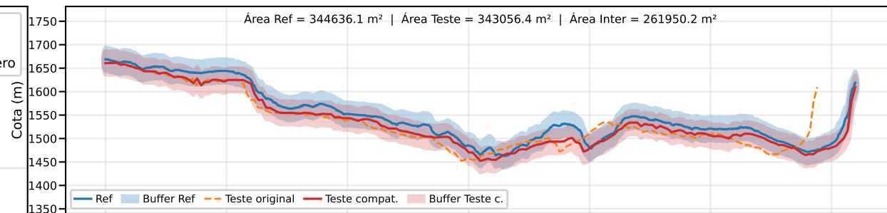
Classe B | PEC-PCD (Vertical)=50.0 m | EQ = 100m | dm = 20.52
