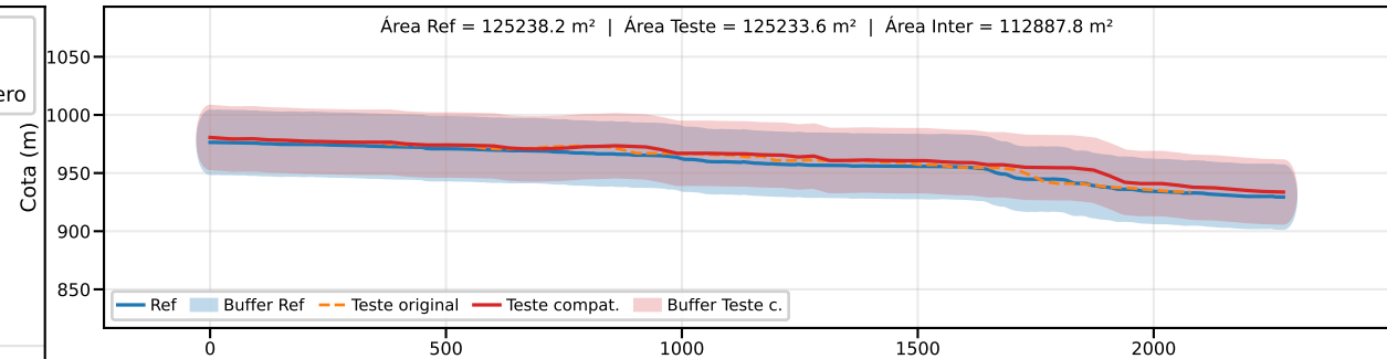
Classe B | PEC-PCD (Vertical)=50.0 m | EQ = 100m | dm = 8.37
