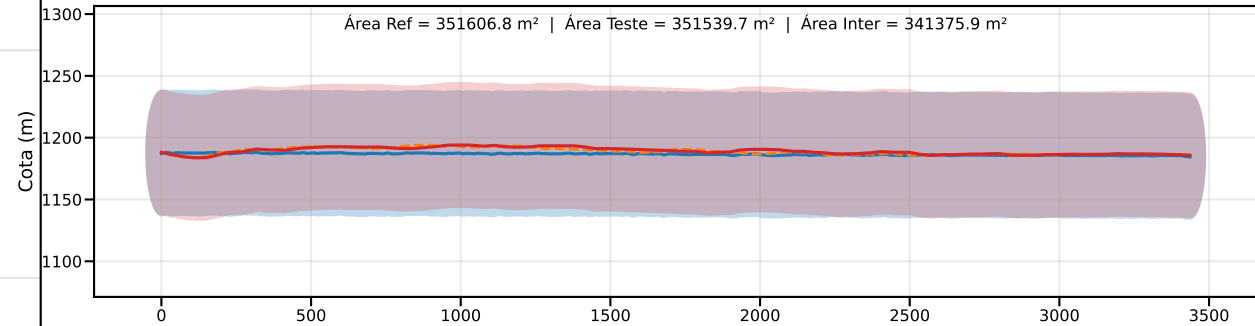
Classe C | PEC-PCD (Vertical)=60.0 m | EQ = 100m | dm = 4.56
