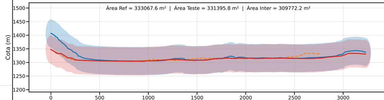
Classe C | PEC-PCD (Vertical)=60.0 m | EQ = 100m | dm = 11.38
