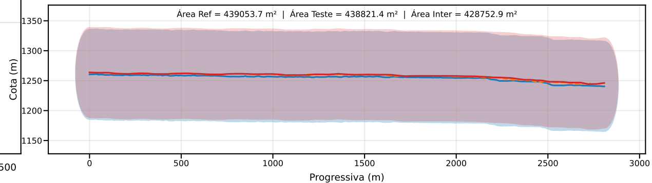
Classe D | PEC-PCD (Vertical)=75.0 m | EQ = 100m | dm = 5.53
