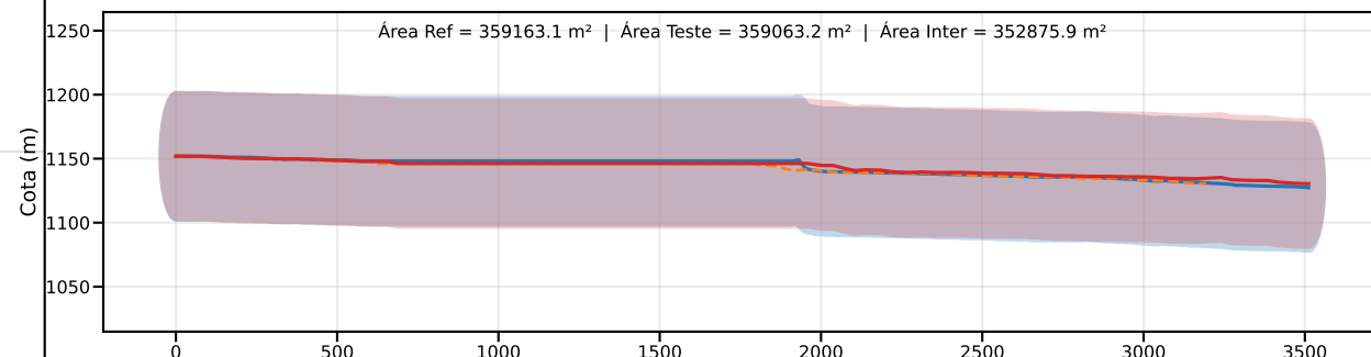
Classe C | PEC-PCD (Vertical)=60.0 m | EQ = 100m | dm = 2.76
