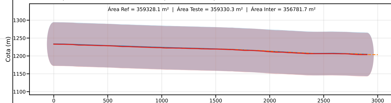
Classe D | PEC-PCD (Vertical)=75.0 m | EQ = 100m | dm = 1.34
