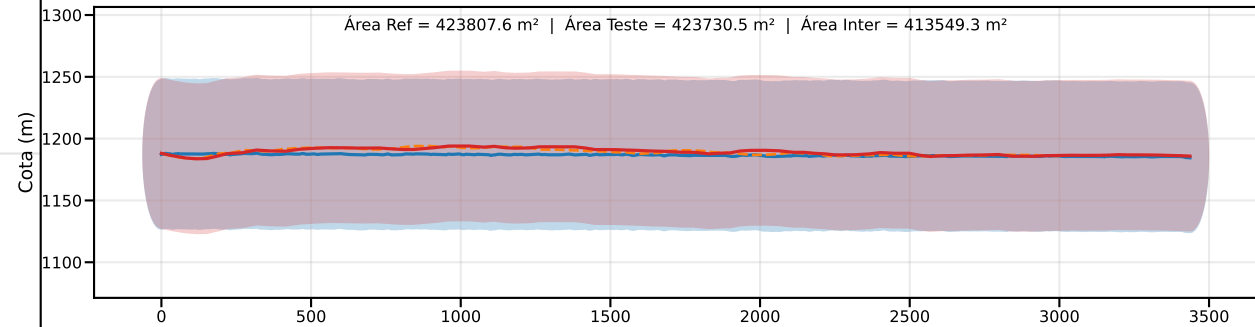
Classe D | PEC-PCD (Vertical)=75.0 m | EQ = 100m | dm = 4.55
