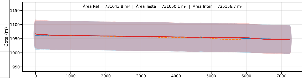
Classe C | PEC-PCD (Vertical)=60.0 m | EQ = 100m | dm = 1.27
