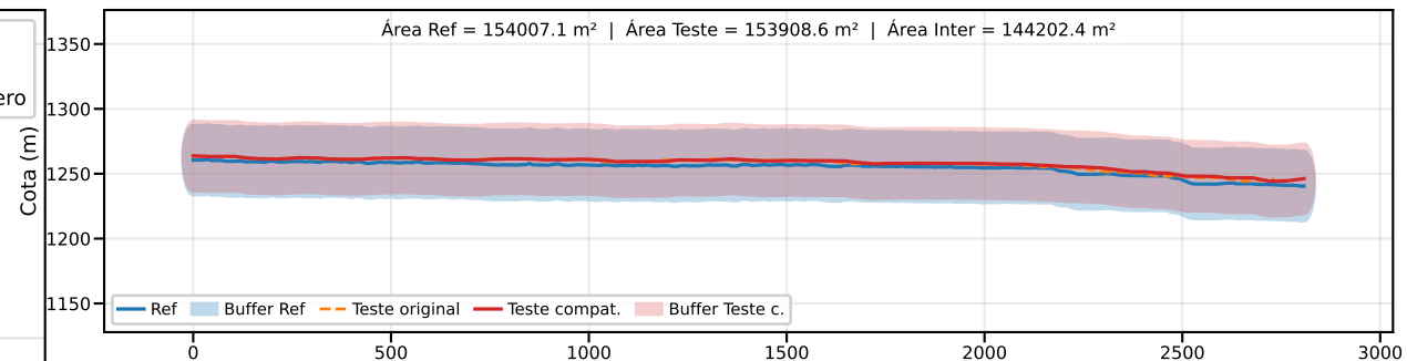
Classe B | PEC-PCD (Vertical)=50.0 m | EQ = 100m | dm = 5.47
