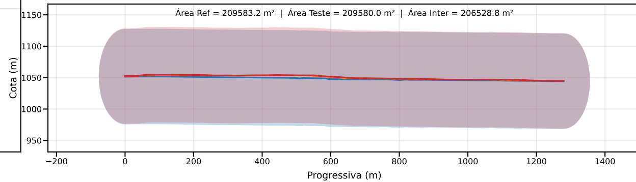
Classe D | PEC-PCD (Vertical)=75.0 m | EQ = 100m | dm = 3.43
