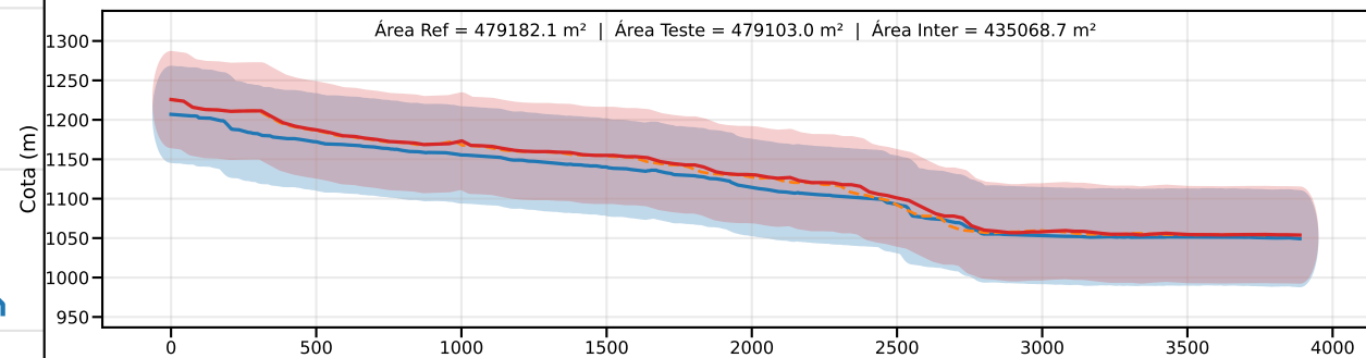
Classe D | PEC-PCD (Vertical)=75.0 m | EQ = 100m | dm = 17.39
