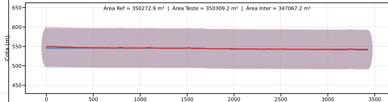
Classe C | PEC-PCD (Vertical)=60.0 m | EQ = 100m | dm = 1.45
