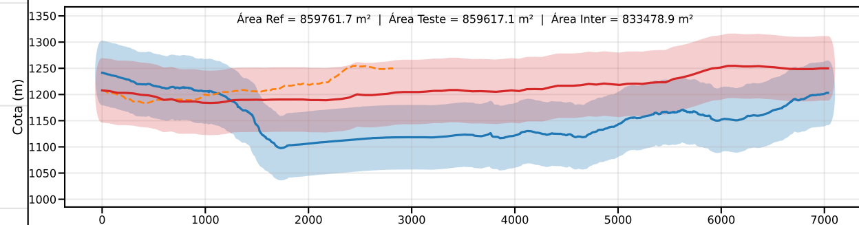
Classe D | PEC-PCD (Vertical)=75.0 m | EQ = 100m | dm = 5.75
