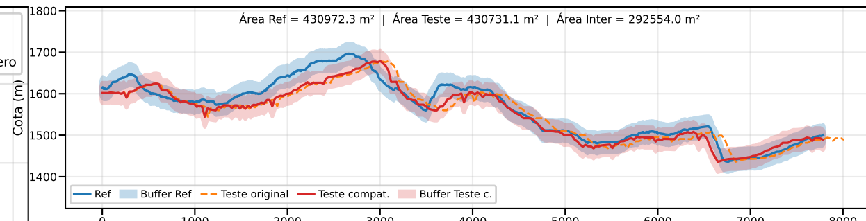
Classe B | PEC-PCD (Vertical)=50.0 m | EQ = 100m | dm = 27.23
