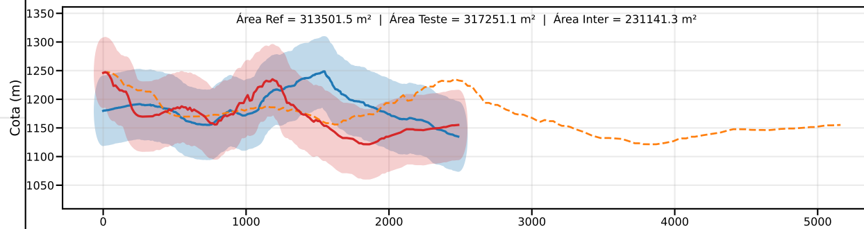
Classe D | PEC-PCD (Vertical)=75.0 m | EQ = 100m | dm = 49.02
