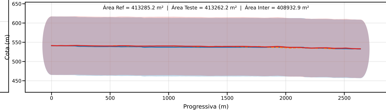
Classe D | PEC-PCD (Vertical)=75.0 m | EQ = 100m | dm = 2.48
