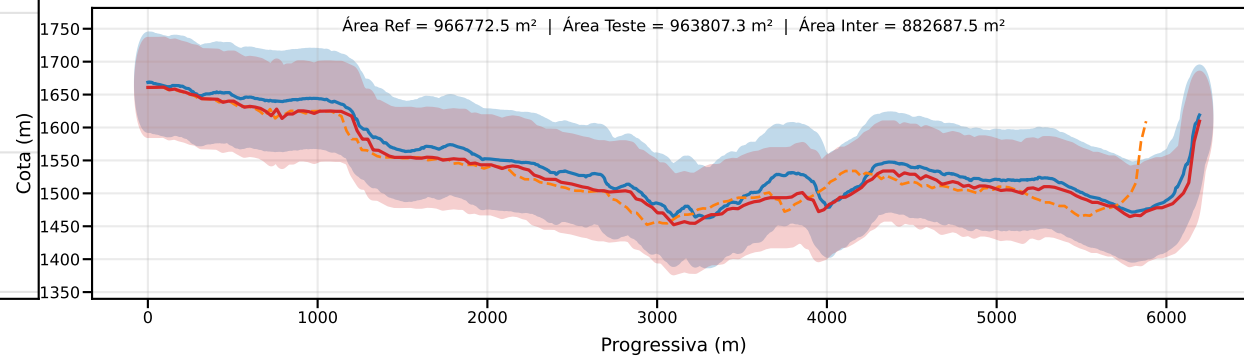
Classe D | PEC-PCD (Vertical)=75.0 m | EQ = 100m | dm = 20.56
