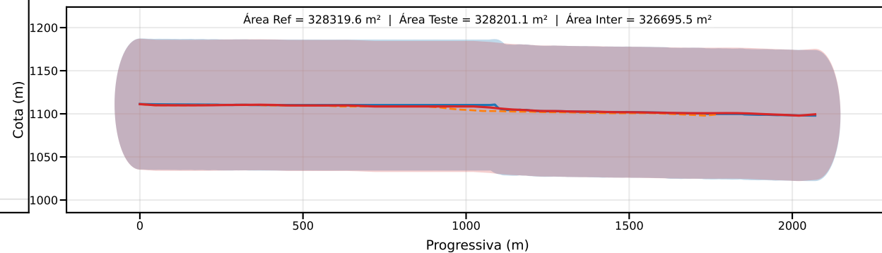
Classe D | PEC-PCD (Vertical)=75.0 m | EQ = 100m | dm = 1.17
