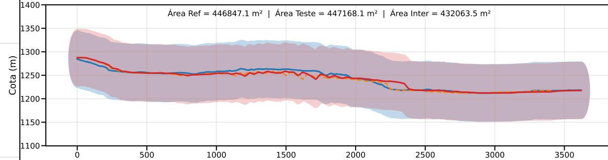
Classe D | PEC-PCD (Vertical)=75.0 m | EQ = 100m | dm = 6.20
