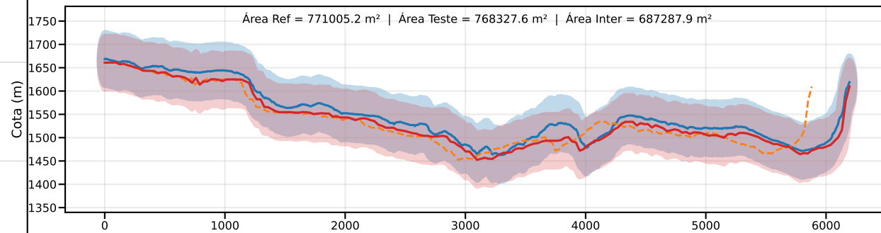
Classe D | PEC-PCD (Vertical)=75.0 m | EQ = 100m | dm = 20.56
