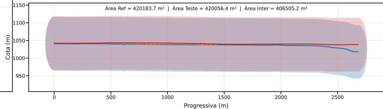
Classe D | PEC-PCD (Vertical)=75.0 m | EQ = 100m | dm = 7.67
