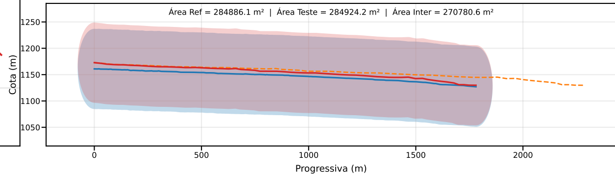
Classe D | PEC-PCD (Vertical)=75.0 m | EQ = 100m | dm = 11.66
