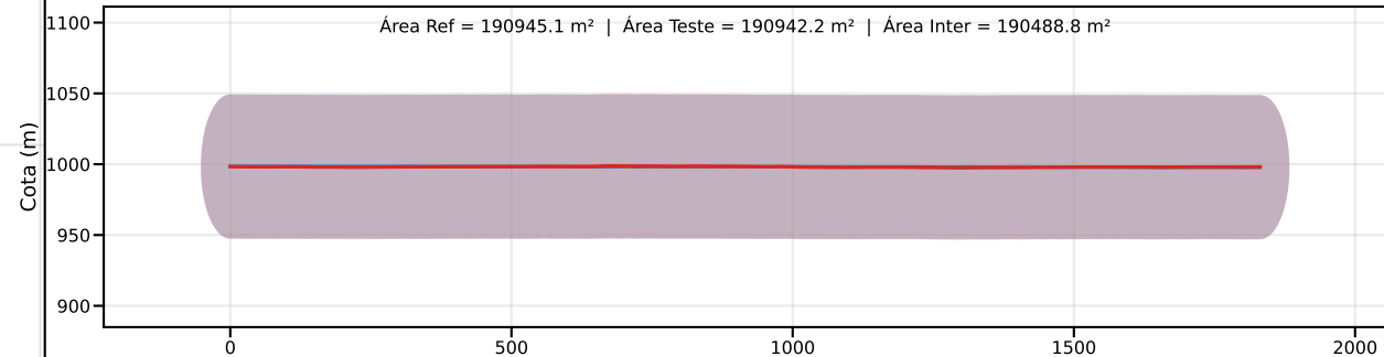
Classe C | PEC-PCD (Vertical)=60.0 m | EQ = 100m | dm = 0.38
