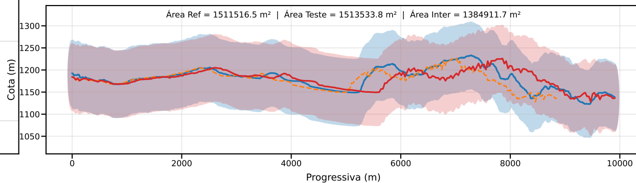
Classe D | PEC-PCD (Vertical)=75.0 m | EQ = 100m | dm = 19.71
