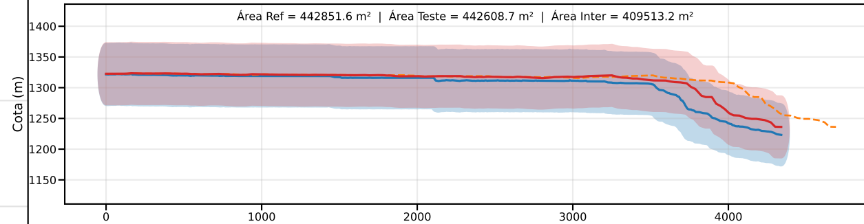
Classe C | PEC-PCD (Vertical)=60.0 m | EQ = 100m | dm = 11.85
