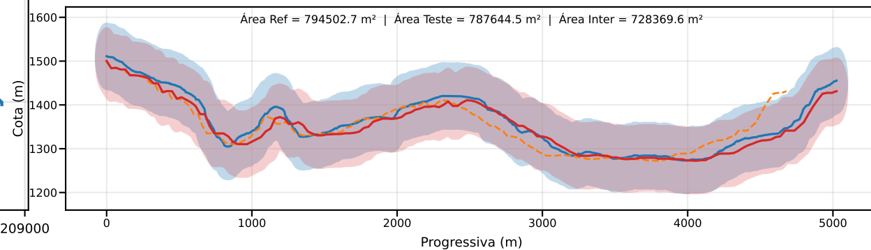
Classe D | PEC-PCD (Vertical)=75.0 m | EQ = 100m | dm = 19.78
