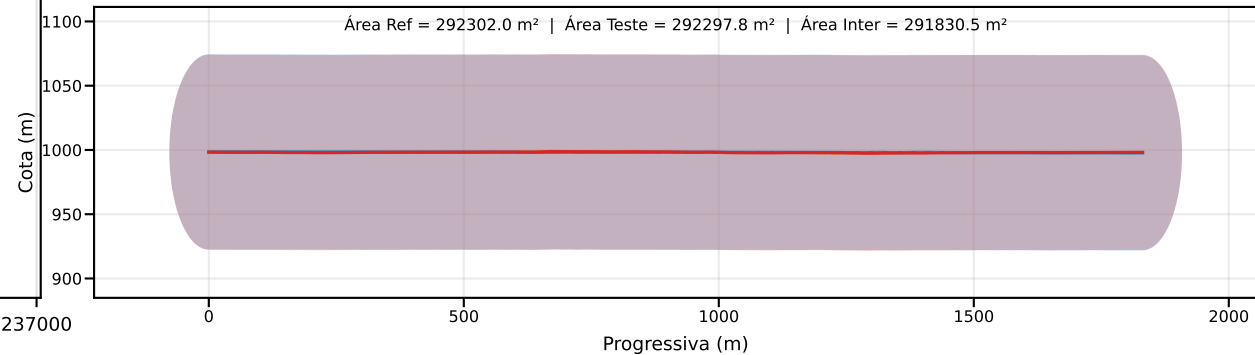
Classe D | PEC-PCD (Vertical)=75.0 m | EQ = 100m | dm = 0.38
