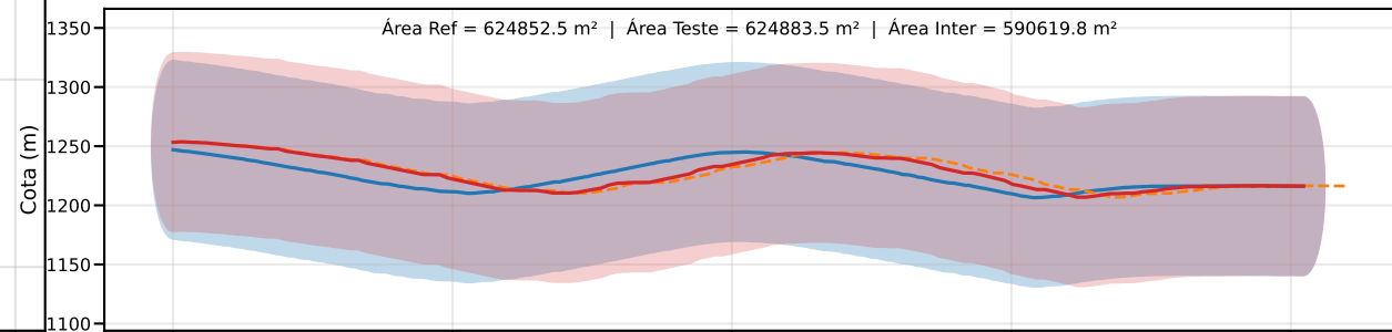
Classe D | PEC-PCD (Vertical)=75.0 m | EQ = 100m | dm = 12.91
