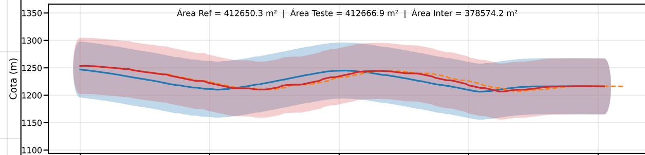
Classe C | PEC-PCD (Vertical)=60.0 m | EQ = 100m | dm = 12.95
