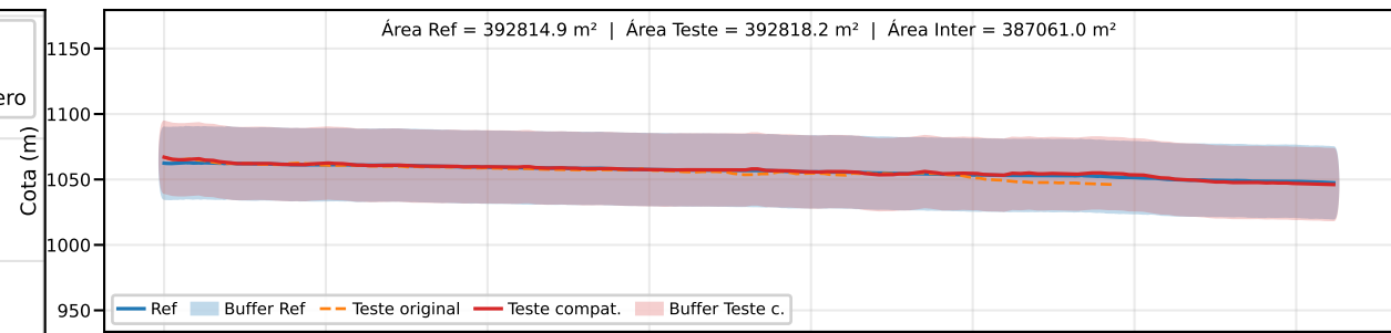
Classe B | PEC-PCD (Vertical)=50.0 m | EQ = 100m | dm = 1.26
