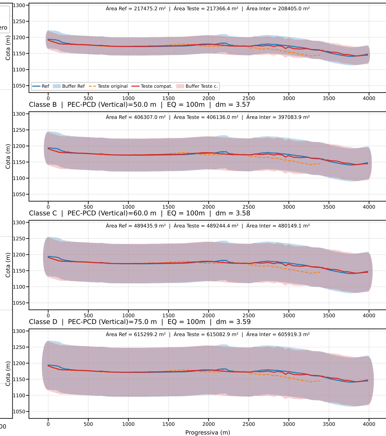
Classe A | PEC-PCD (Vertical)=27.0 m | EQ = 100m | dm = 3.54
