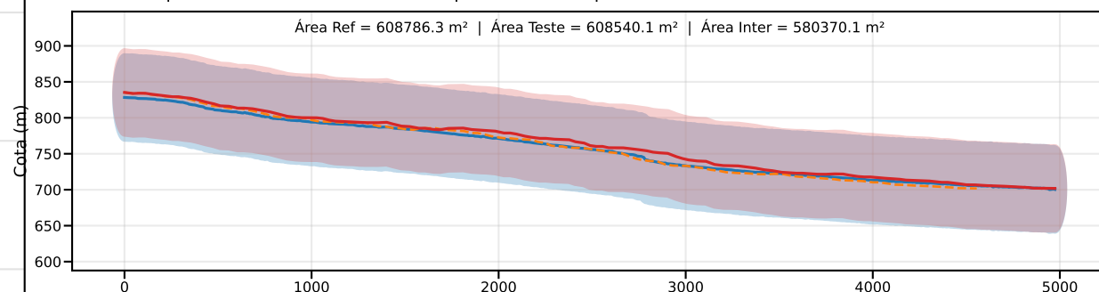
Classe D | PEC-PCD (Vertical)=75.0 m | EQ = 100m | dm = 8.80
