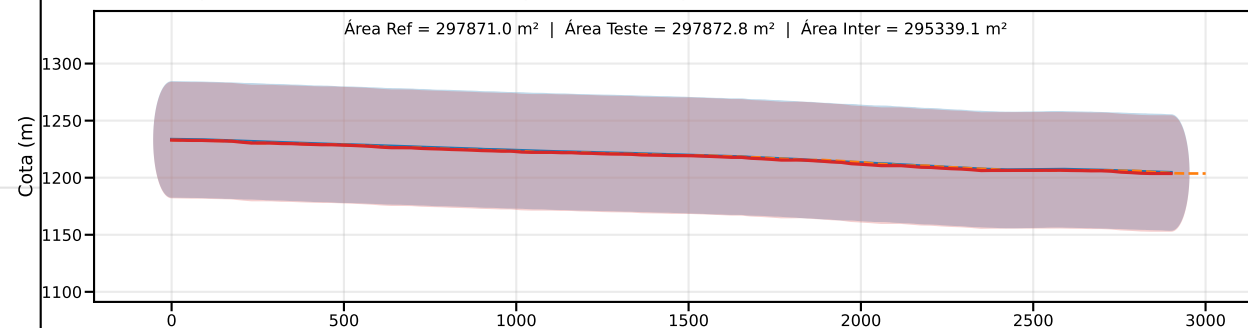
Classe C | PEC-PCD (Vertical)=60.0 m | EQ = 100m | dm = 1.34
