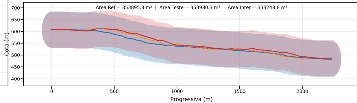
Classe D | PEC-PCD (Vertical)=75.0 m | EQ = 100m | dm = 13.74
