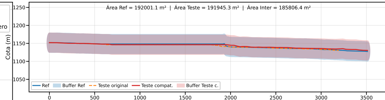
Classe B | PEC-PCD (Vertical)=50.0 m | EQ = 100m | dm = 2.75
