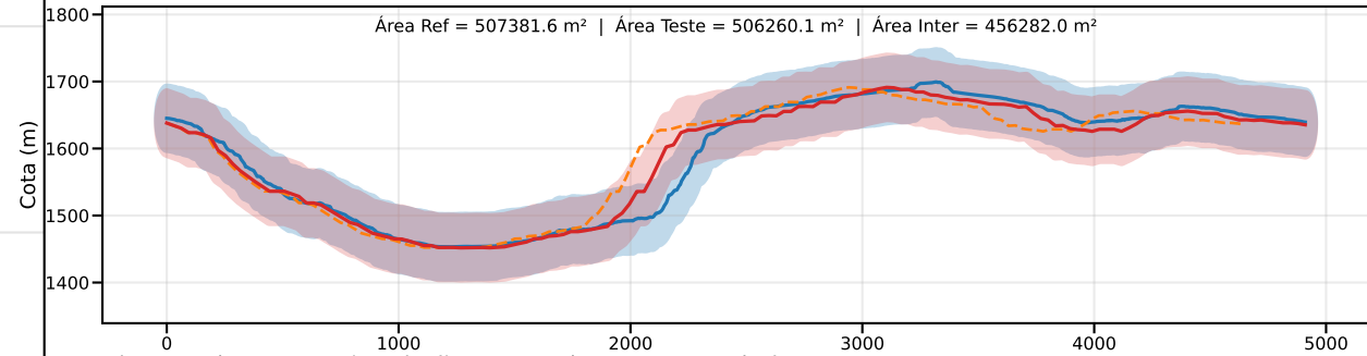
Classe C | PEC-PCD (Vertical)=60.0 m | EQ = 100m | dm = 15.85
