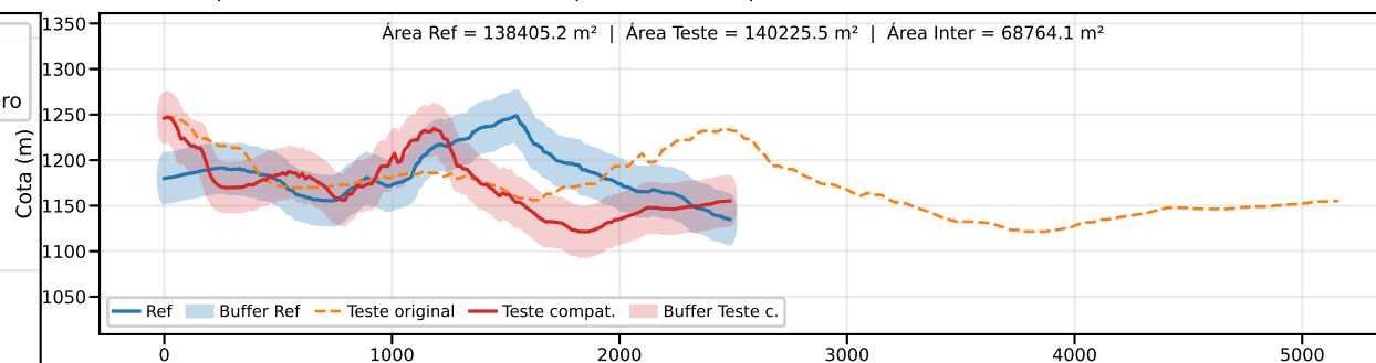
Classe B | PEC-PCD (Vertical)=50.0 m | EQ = 100m | dm = 48.86
