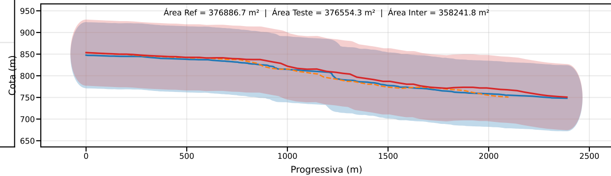
Classe D | PEC-PCD (Vertical)=75.0 m | EQ = 100m | dm = 11.67
