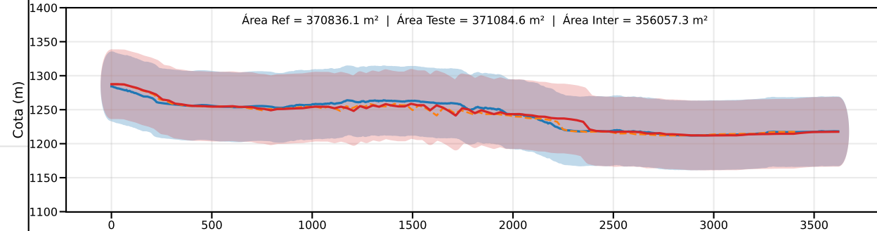
Classe C | PEC-PCD (Vertical)=60.0 m | EQ = 100m | dm = 6.23
