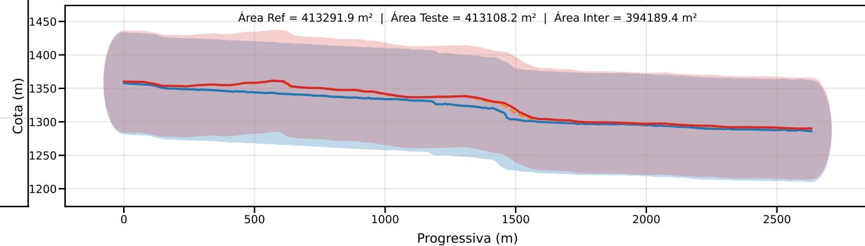
Classe D | PEC-PCD (Vertical)=75.0 m | EQ = 100m | dm = 10.90
