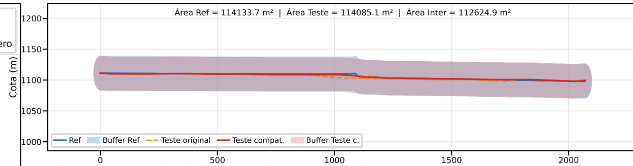
Classe B | PEC-PCD (Vertical)=50.0 m | EQ = 100m | dm = 1.14
