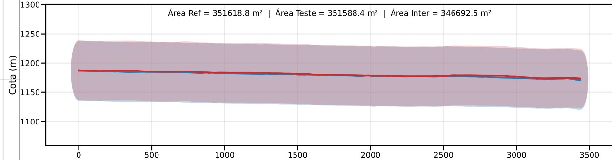
Classe C | PEC-PCD (Vertical)=60.0 m | EQ = 100m | dm = 2.21
