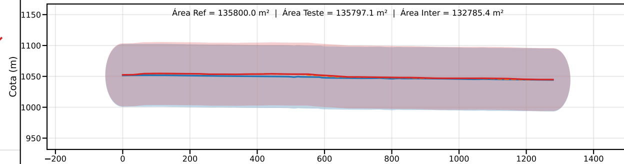
Classe C | PEC-PCD (Vertical)=60.0 m | EQ = 100m | dm = 3.47
