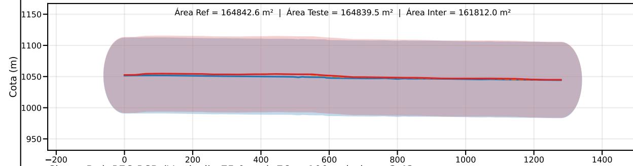
Classe D | PEC-PCD (Vertical)=75.0 m | EQ = 100m | dm = 3.43
