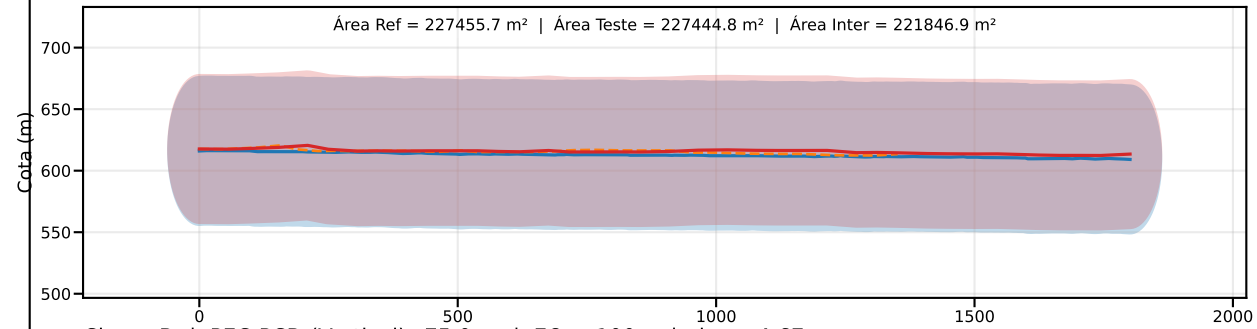
Classe D | PEC-PCD (Vertical)=75.0 m | EQ = 100m | dm = 4.67
