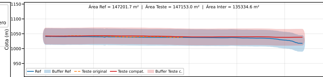
Classe B | PEC-PCD (Vertical)=50.0 m | EQ = 100m | dm = 7.25
