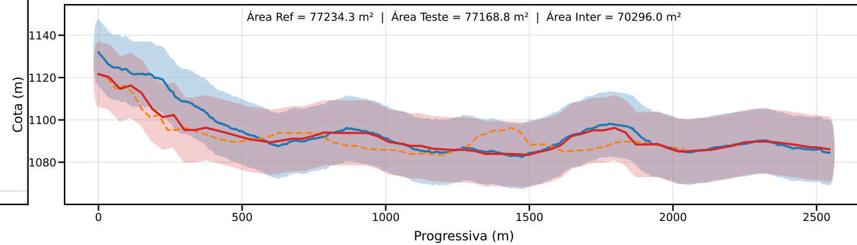
Classe D | PEC-PCD (Vertical)=15.0 m | EQ = 20m | dm = 4.24
