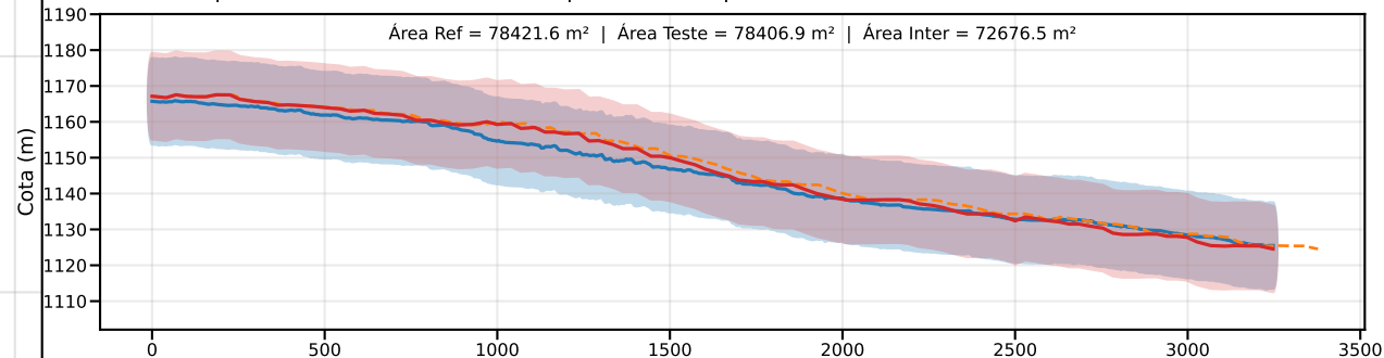
Classe D | PEC-PCD (Vertical)=15.0 m | EQ = 20m | dm = 2.76
