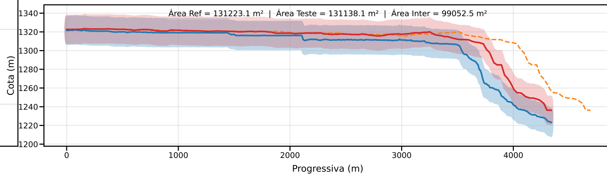
Classe D | PEC-PCD (Vertical)=15.0 m | EQ = 20m | dm = 11.56
