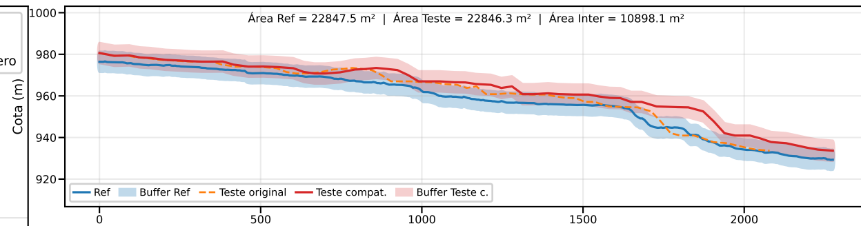
Classe B | PEC-PCD (Vertical)=10.0 m | EQ = 20m | dm = 8.36
