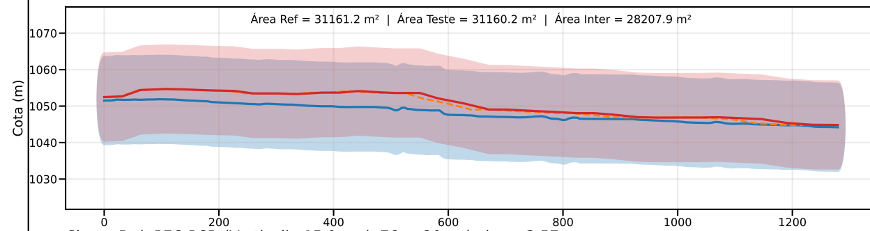
Classe D | PEC-PCD (Vertical)=15.0 m | EQ = 20m | dm = 3.57
