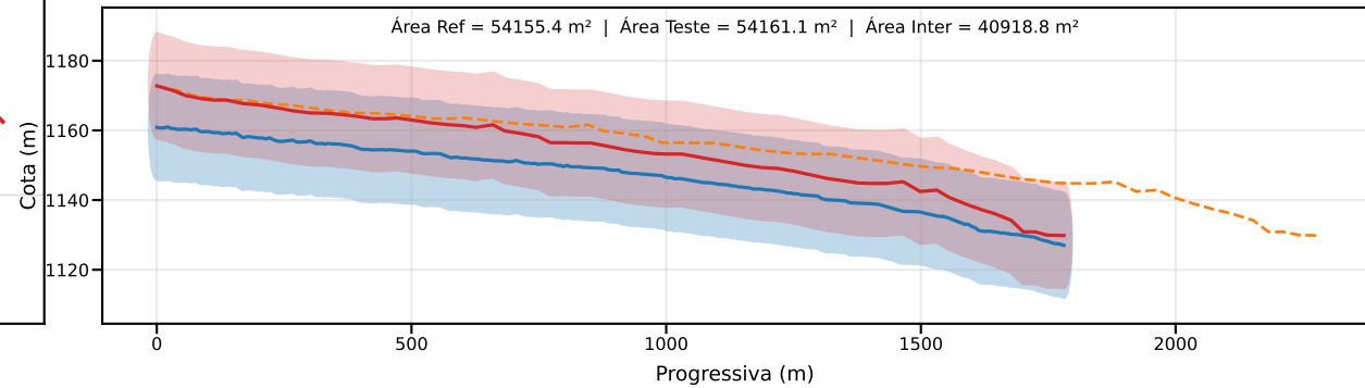
Classe D | PEC-PCD (Vertical)=15.0 m | EQ = 20m | dm = 11.52
