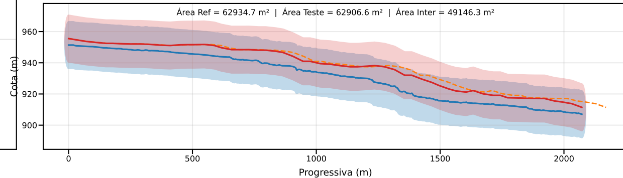
Classe D | PEC-PCD (Vertical)=15.0 m | EQ = 20m | dm = 10.33
