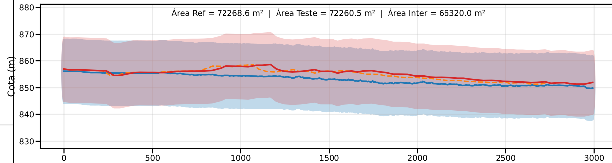
Classe D | PEC-PCD (Vertical)=15.0 m | EQ = 20m | dm = 3.10
