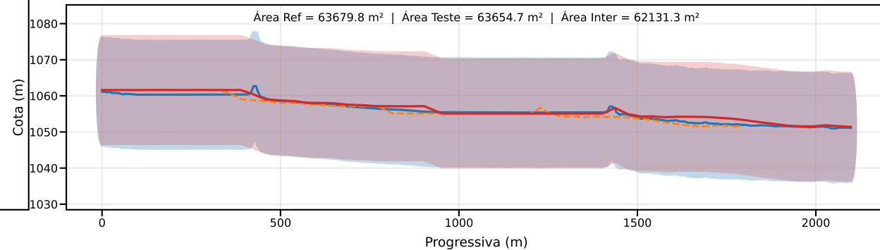
Classe D | PEC-PCD (Vertical)=15.0 m | EQ = 20m | dm = 1.15
