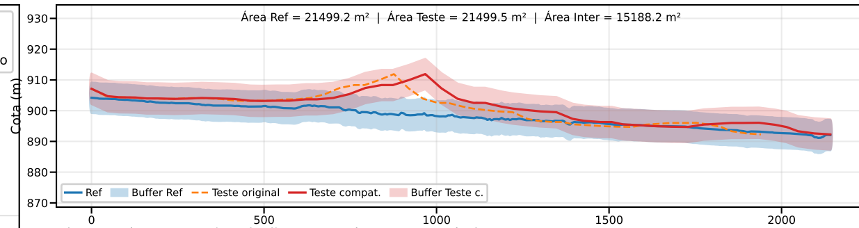
Classe B | PEC-PCD (Vertical)=10.0 m | EQ = 20m | dm = 4.74
