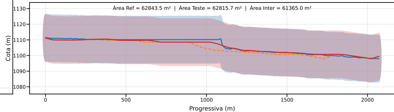
Classe D | PEC-PCD (Vertical)=15.0 m | EQ = 20m | dm = 1.11
