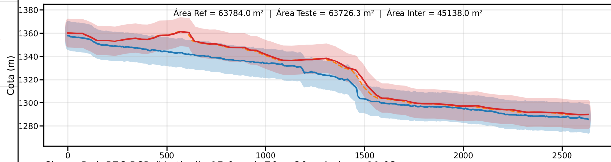
Classe D | PEC-PCD (Vertical)=15.0 m | EQ = 20m | dm = 11.03
