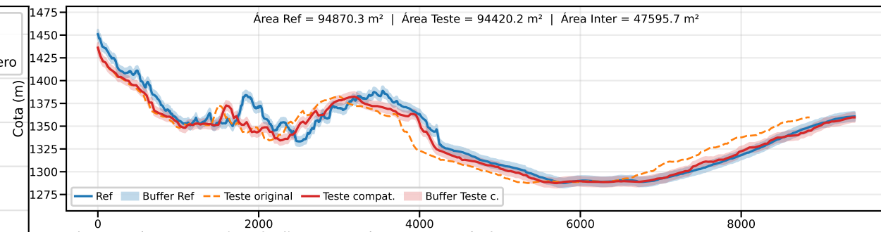
Classe B | PEC-PCD (Vertical)=10.0 m | EQ = 20m | dm = 9.65
