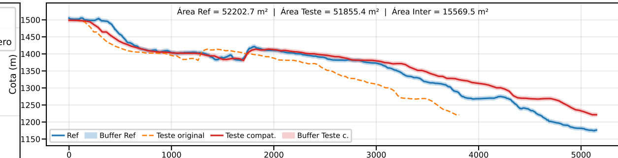
Classe B | PEC-PCD (Vertical)=10.0 m | EQ = 20m | dm = 18.18
