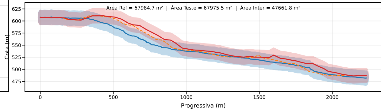
Classe D | PEC-PCD (Vertical)=15.0 m | EQ = 20m | dm = 14.09
