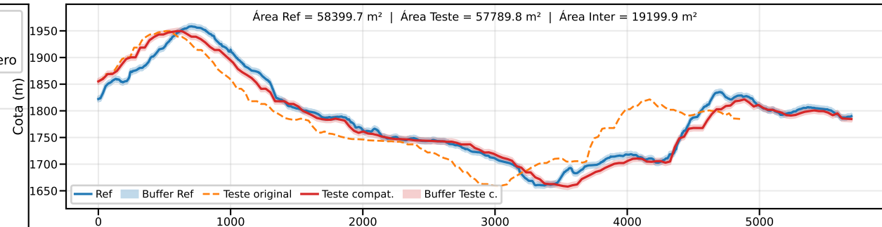
Classe B | PEC-PCD (Vertical)=10.0 m | EQ = 20m | dm = 15.32
