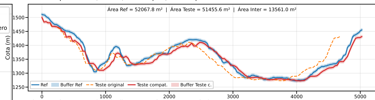
Classe B | PEC-PCD (Vertical)=10.0 m | EQ = 20m | dm = 17.46
