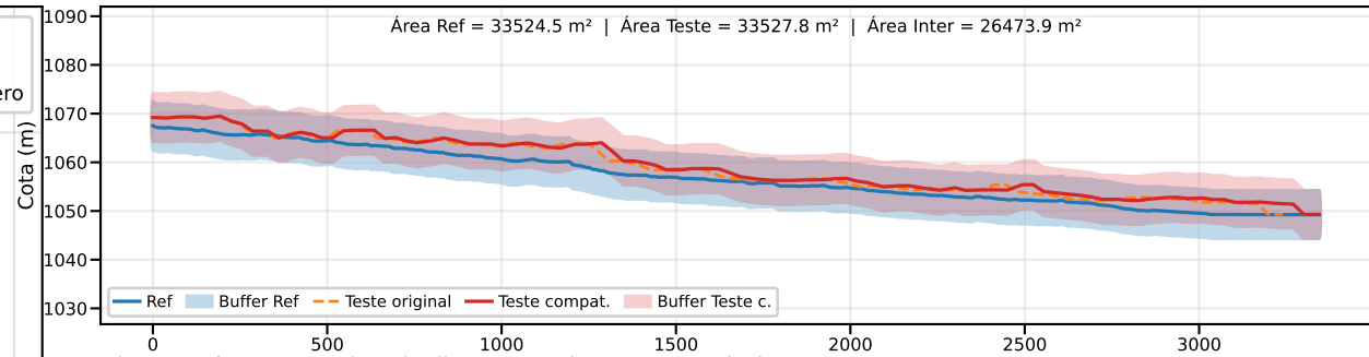
Classe B | PEC-PCD (Vertical)=10.0 m | EQ = 20m | dm = 3.30
