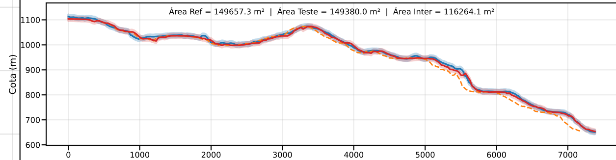
Classe C | PEC-PCD (Vertical)=12.0 m | EQ = 20m | dm = 7.04
