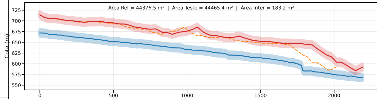
Classe C | PEC-PCD (Vertical)=12.0 m | EQ = 20m | dm = 37.26
