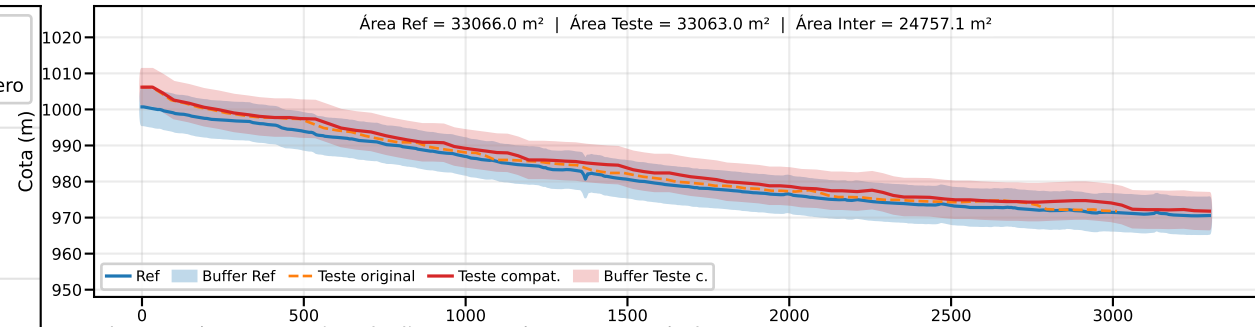
Classe B | PEC-PCD (Vertical)=10.0 m | EQ = 20m | dm = 3.96
