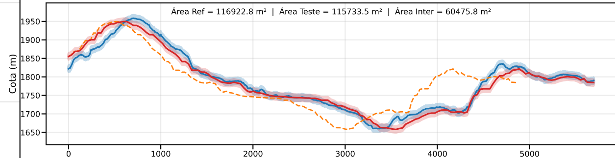
Classe C | PEC-PCD (Vertical)=12.0 m | EQ = 20m | dm = 16.26
