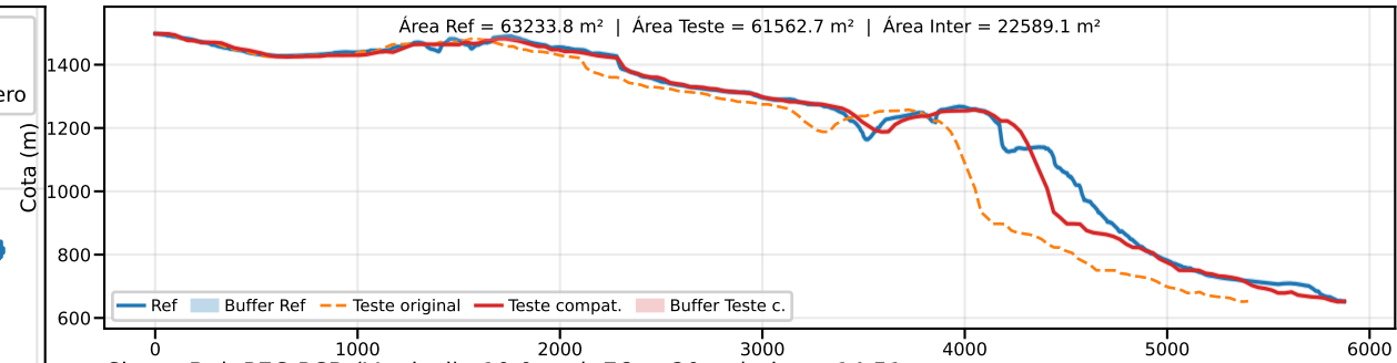
Classe B | PEC-PCD (Vertical)=10.0 m | EQ = 20m | dm = 14.51
