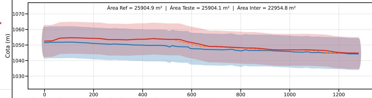
Classe C | PEC-PCD (Vertical)=12.0 m | EQ = 20m | dm = 3.57
