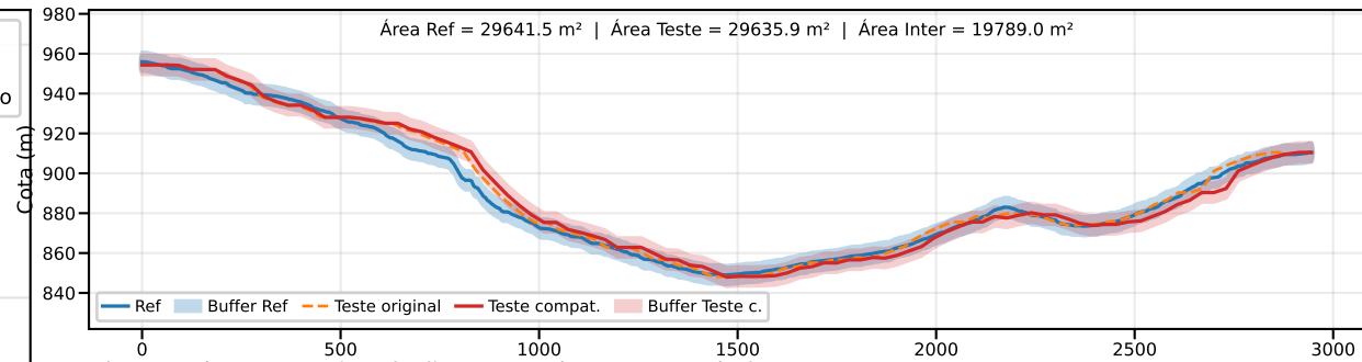
Classe B | PEC-PCD (Vertical)=10.0 m | EQ = 20m | dm = 5.40
