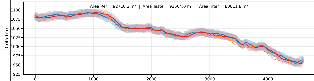
Classe C | PEC-PCD (Vertical)=12.0 m | EQ = 20m | dm = 4.32
