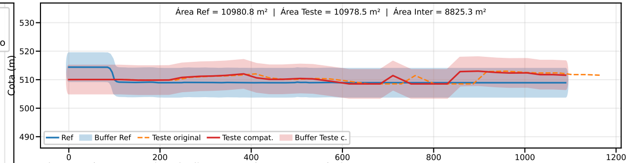
Classe B | PEC-PCD (Vertical)=10.0 m | EQ = 20m | dm = 3.11
