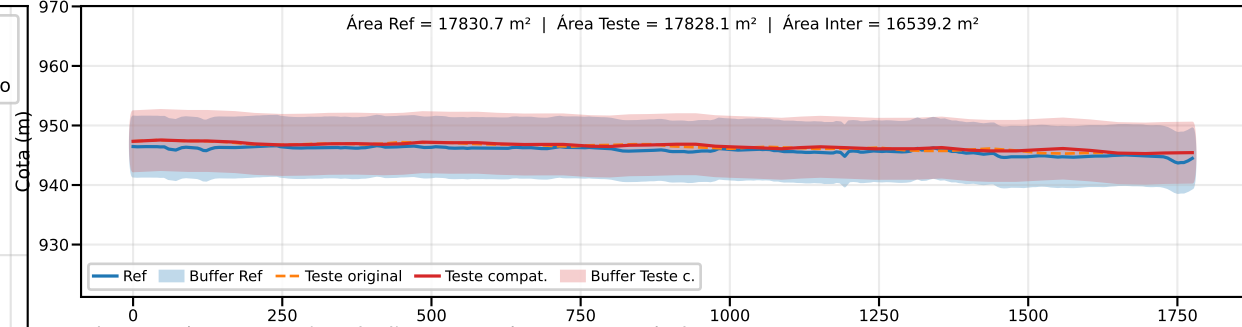
Classe B | PEC-PCD (Vertical)=10.0 m | EQ = 20m | dm = 1.14
