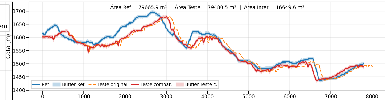
Classe B | PEC-PCD (Vertical)=10.0 m | EQ = 20m | dm = 19.23
