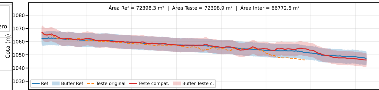
Classe B | PEC-PCD (Vertical)=10.0 m | EQ = 20m | dm = 1.23
