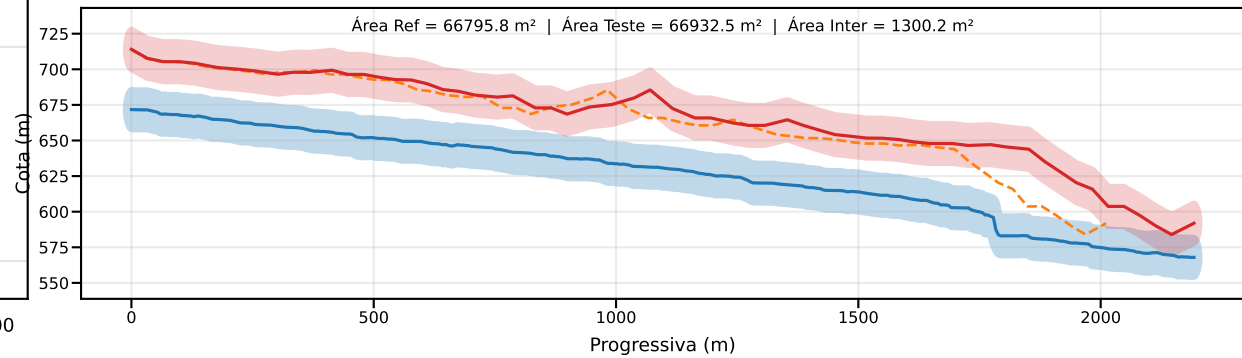
Classe D | PEC-PCD (Vertical)=15.0 m | EQ = 20m | dm = 46.11
