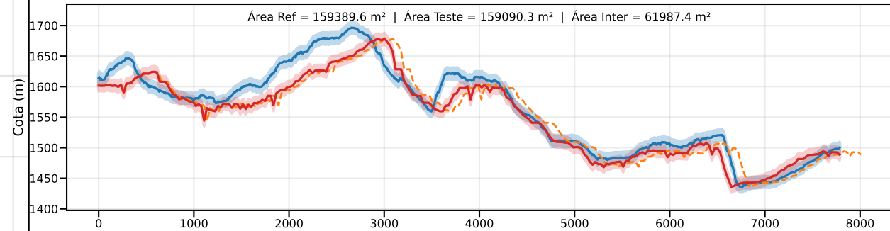
Classe C | PEC-PCD (Vertical)=12.0 m | EQ = 20m | dm = 21.15
