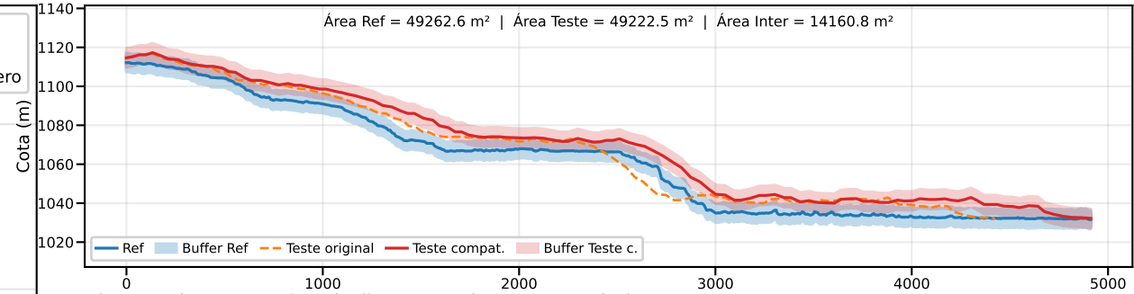
Classe B | PEC-PCD (Vertical)=10.0 m | EQ = 20m | dm = 11.63
