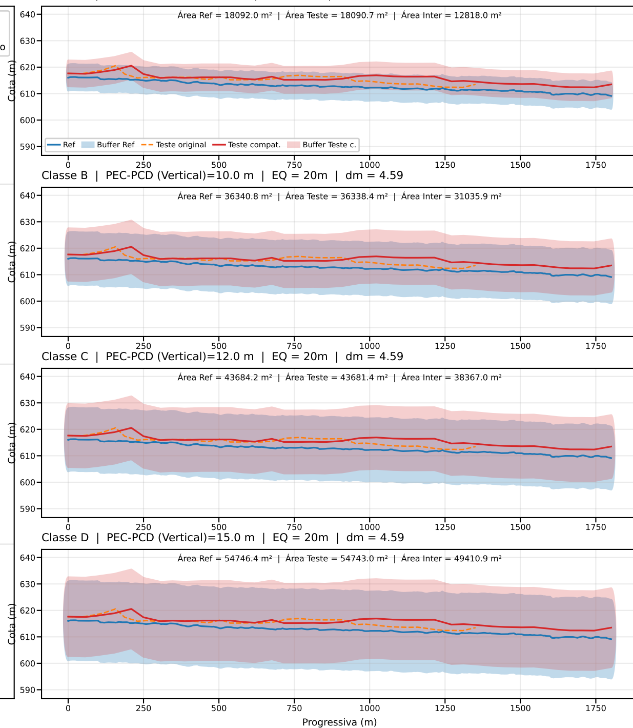
Classe A | PEC-PCD (Vertical)=5.0 m | EQ = 20m | dm = 4.58
