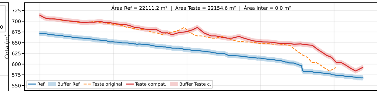
Classe B | PEC-PCD (Vertical)=10.0 m | EQ = 20m | dm = 31.22
