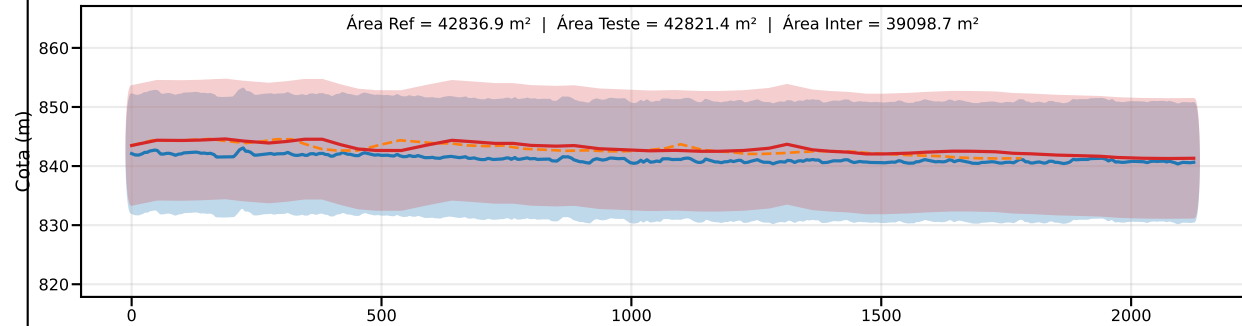
Classe C | PEC-PCD (Vertical)=12.0 m | EQ = 20m | dm = 2.74
