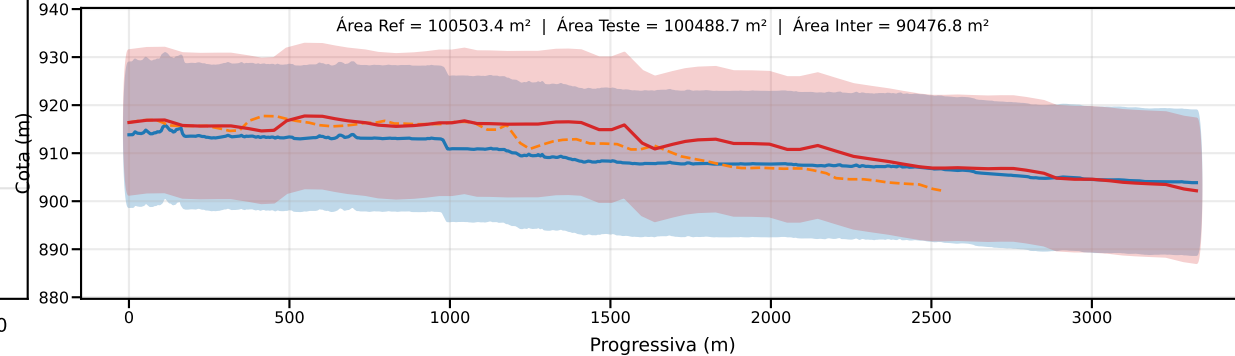
Classe D | PEC-PCD (Vertical)=15.0 m | EQ = 20m | dm = 4.70
