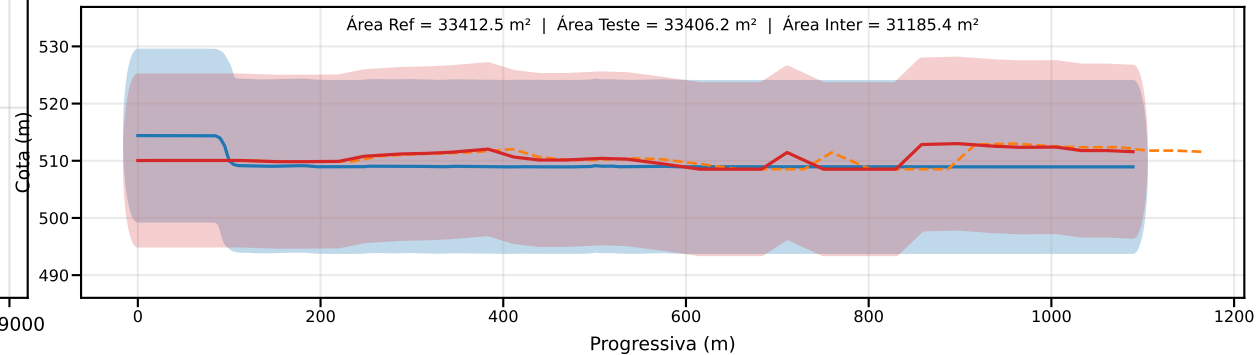
Classe D | PEC-PCD (Vertical)=15.0 m | EQ = 20m | dm = 3.14
