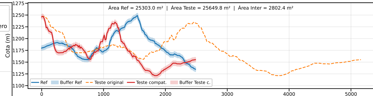
Classe B | PEC-PCD (Vertical)=10.0 m | EQ = 20m | dm = 24.70
