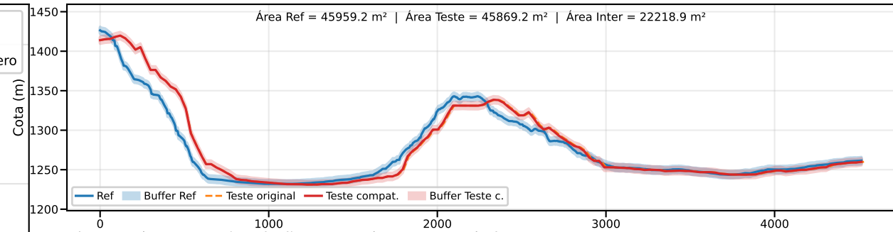
Classe B | PEC-PCD (Vertical)=10.0 m | EQ = 20m | dm = 11.46
