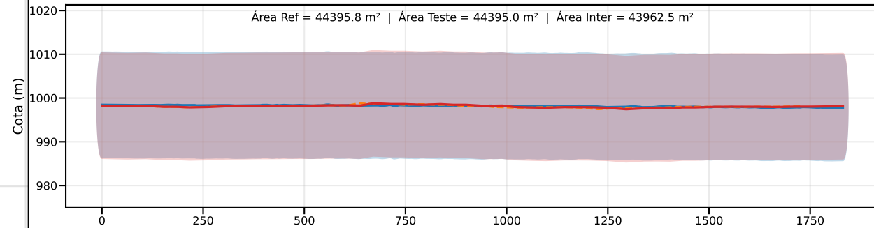
Classe D | PEC-PCD (Vertical)=15.0 m | EQ = 20m | dm = 0.37
