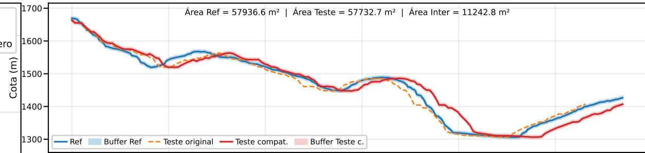
Classe B | PEC-PCD (Vertical)=10.0 m | EQ = 20m | dm = 20.20
