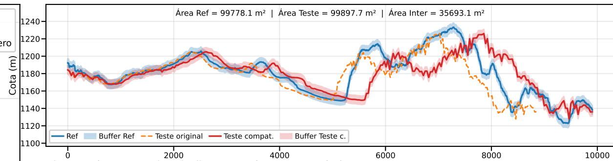
Classe B | PEC-PCD (Vertical)=10.0 m | EQ = 20m | dm = 14.38
