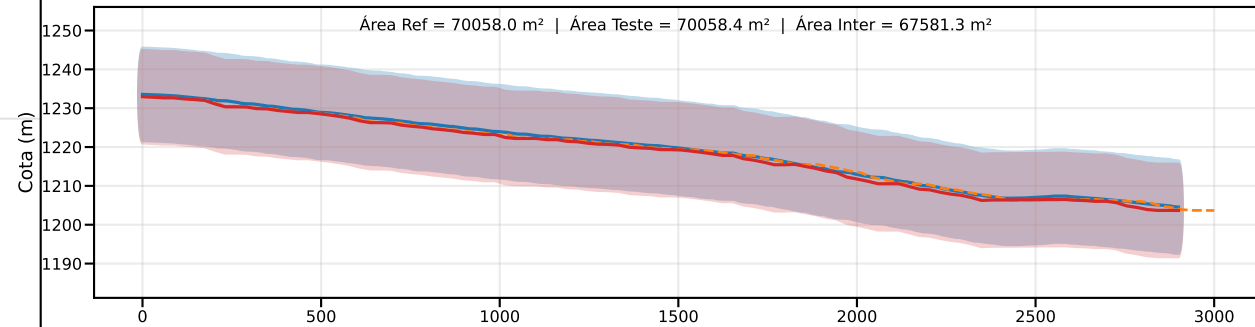
Classe D | PEC-PCD (Vertical)=15.0 m | EQ = 20m | dm = 1.33
