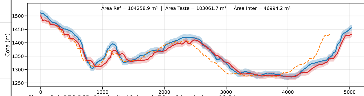
Classe C | PEC-PCD (Vertical)=12.0 m | EQ = 20m | dm = 18.24
