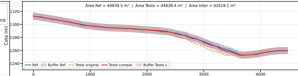
Classe B | PEC-PCD (Vertical)=10.0 m | EQ = 20m | dm = 0.78
