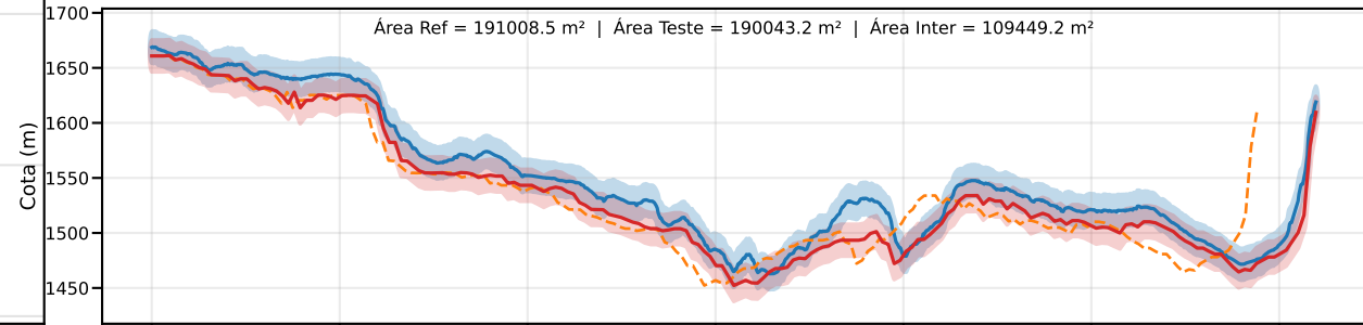
Classe D | PEC-PCD (Vertical)=15.0 m | EQ = 20m | dm = 20.22
