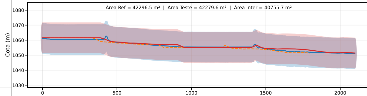
Classe C | PEC-PCD (Vertical)=12.0 m | EQ = 20m | dm = 1.15
