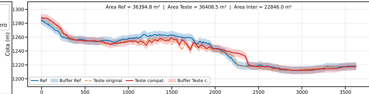
Classe B | PEC-PCD (Vertical)=10.0 m | EQ = 20m | dm = 6.34
