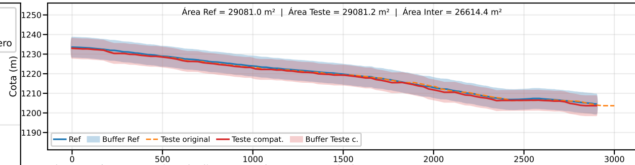
Classe B | PEC-PCD (Vertical)=10.0 m | EQ = 20m | dm = 1.33
