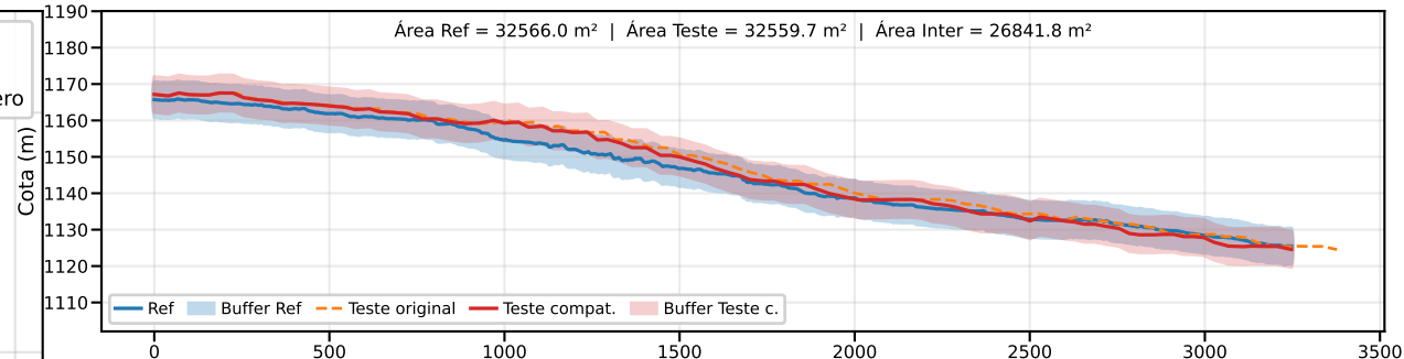
Classe B | PEC-PCD (Vertical)=10.0 m | EQ = 20m | dm = 2.76
