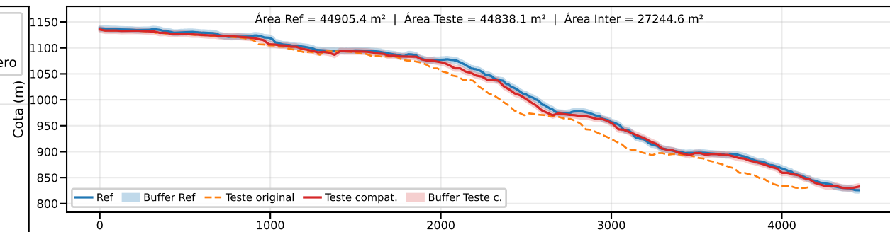
Classe B | PEC-PCD (Vertical)=10.0 m | EQ = 20m | dm = 6.41
