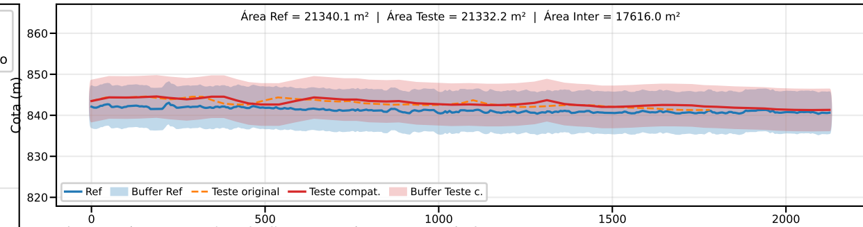
Classe B | PEC-PCD (Vertical)=10.0 m | EQ = 20m | dm = 2.74
