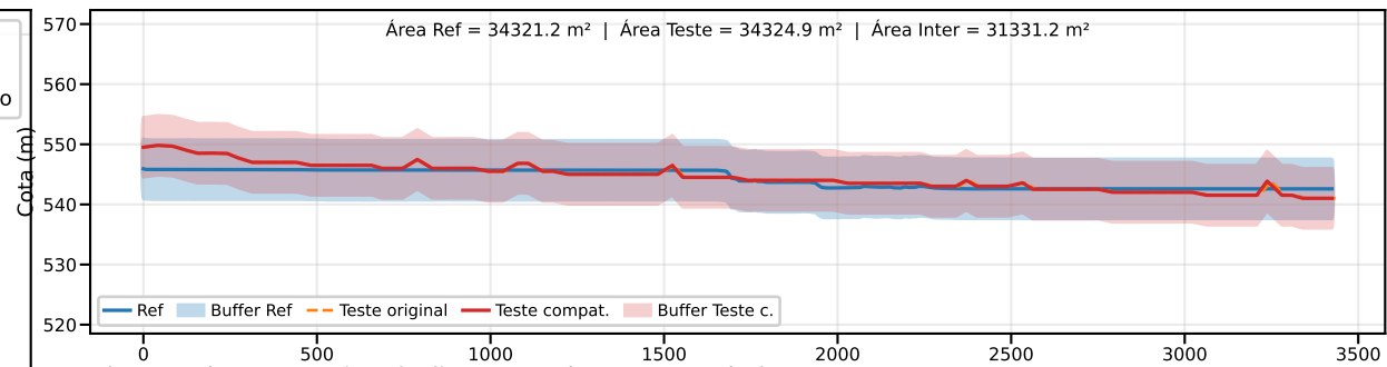
Classe B | PEC-PCD (Vertical)=10.0 m | EQ = 20m | dm = 1.38
