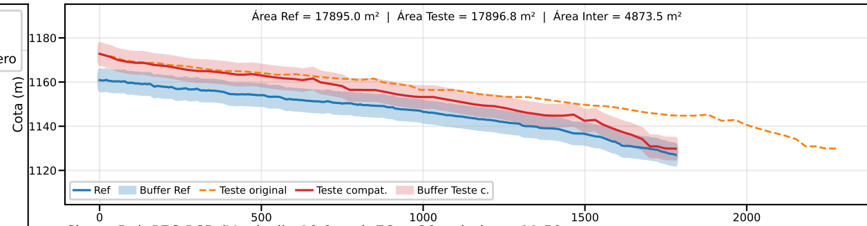
Classe B | PEC-PCD (Vertical)=10.0 m | EQ = 20m | dm = 11.50
