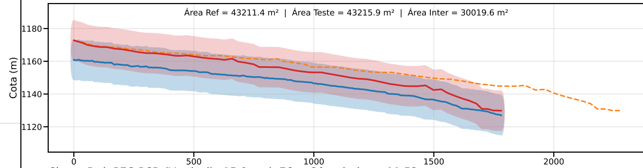
Classe D | PEC-PCD (Vertical)=15.0 m | EQ = 20m | dm = 11.52
