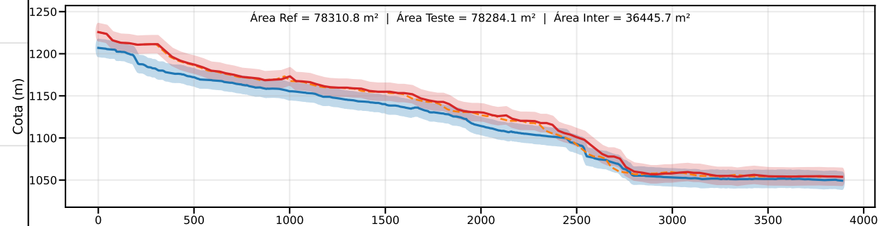
Classe C | PEC-PCD (Vertical)=12.0 m | EQ = 20m | dm = 17.06
