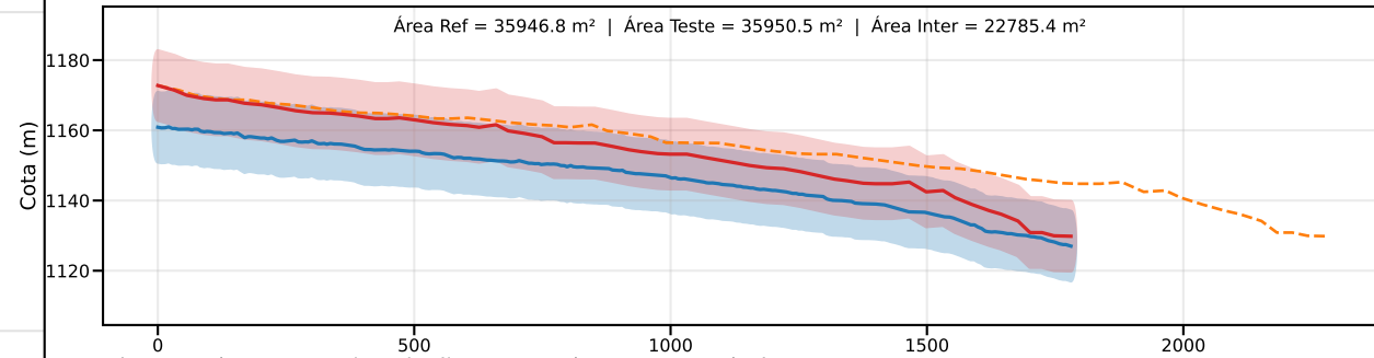
Classe C | PEC-PCD (Vertical)=12.0 m | EQ = 20m | dm = 11.51
