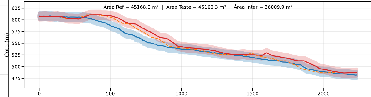
Classe C | PEC-PCD (Vertical)=12.0 m | EQ = 20m | dm = 14.01
