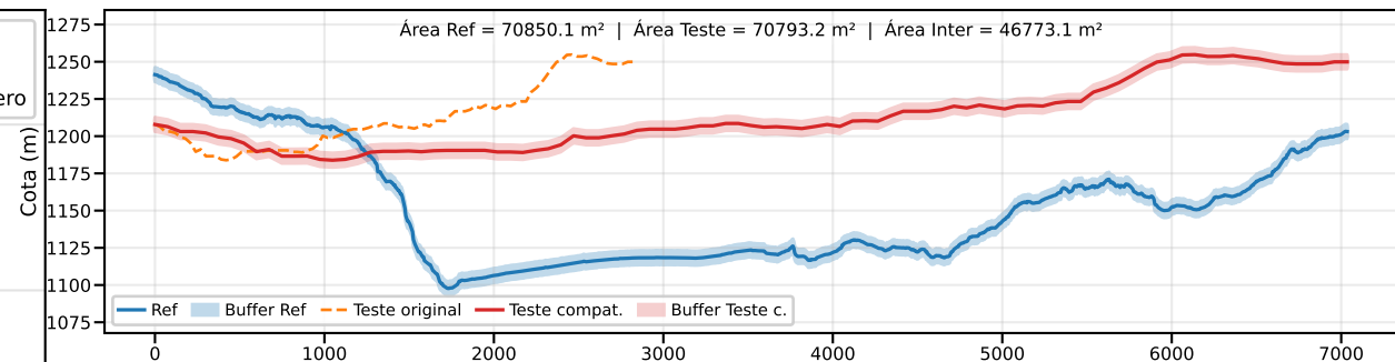
Classe B | PEC-PCD (Vertical)=10.0 m | EQ = 20m | dm = 5.77
