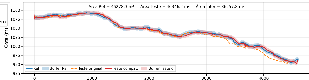
Classe B | PEC-PCD (Vertical)=10.0 m | EQ = 20m | dm = 3.41
