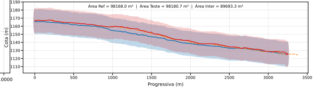
Classe D | PEC-PCD (Vertical)=15.0 m | EQ = 20m | dm = 4.07
