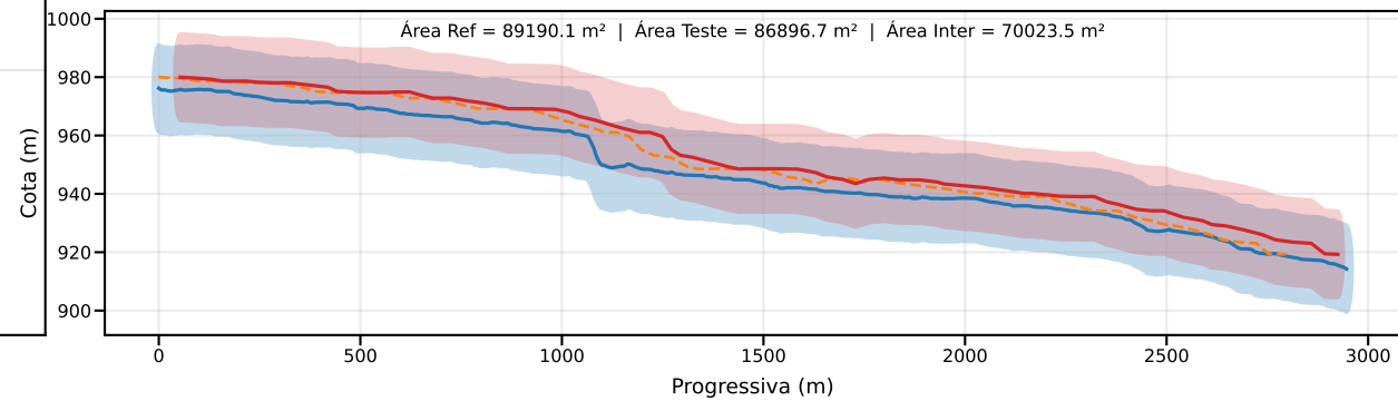
Classe D | PEC-PCD (Vertical)=15.0 m | EQ = 20m | dm = 10.39
