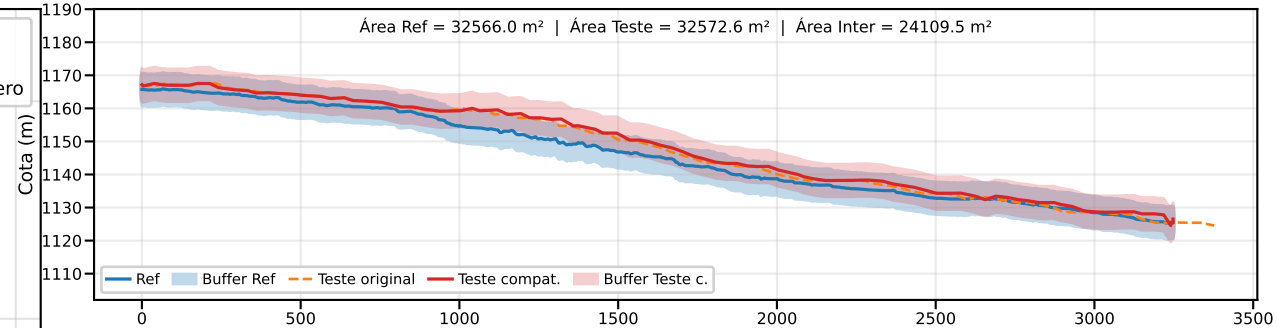
Classe B | PEC-PCD (Vertical)=10.0 m | EQ = 20m | dm = 4.07
