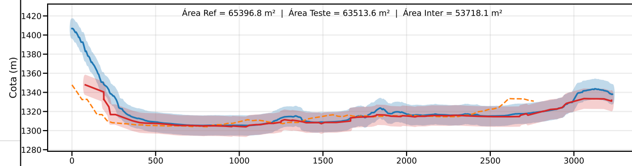
Classe C | PEC-PCD (Vertical)=12.0 m | EQ = 20m | dm = 6.11
