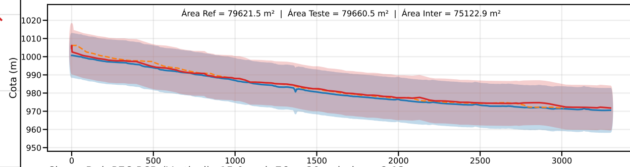
Classe D | PEC-PCD (Vertical)=15.0 m | EQ = 20m | dm = 2.13
