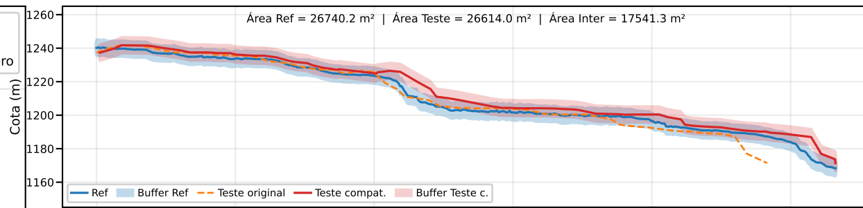
Classe B | PEC-PCD (Vertical)=10.0 m | EQ = 20m | dm = 5.55
