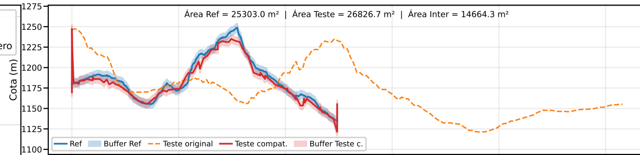
Classe B | PEC-PCD (Vertical)=10.0 m | EQ = 20m | dm = 6.43
