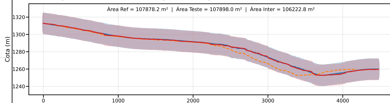
Classe D | PEC-PCD (Vertical)=15.0 m | EQ = 20m | dm = 0.58
