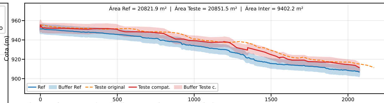
Classe B | PEC-PCD (Vertical)=10.0 m | EQ = 20m | dm = 8.65
