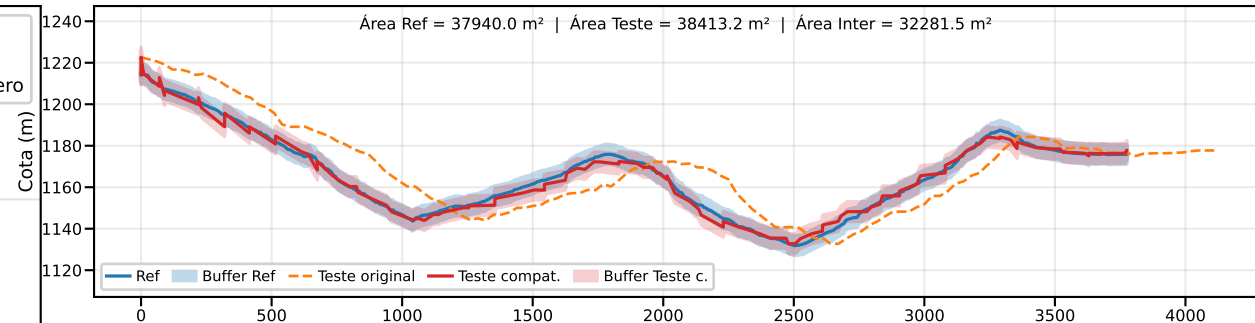
Classe B | PEC-PCD (Vertical)=10.0 m | EQ = 20m | dm = 2.28
