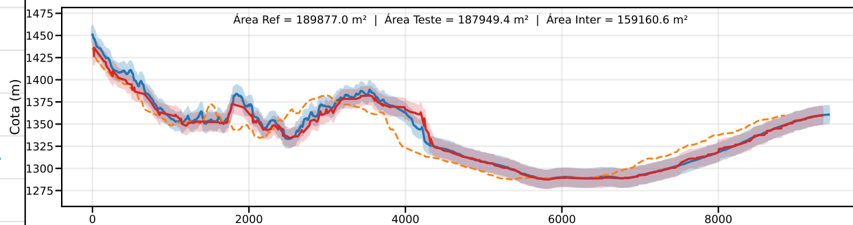
Classe C | PEC-PCD (Vertical)=12.0 m | EQ = 20m | dm = 5.21
