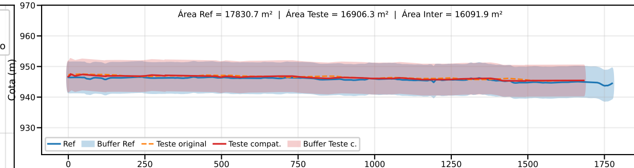
Classe B | PEC-PCD (Vertical)=10.0 m | EQ = 20m | dm = 2.47
