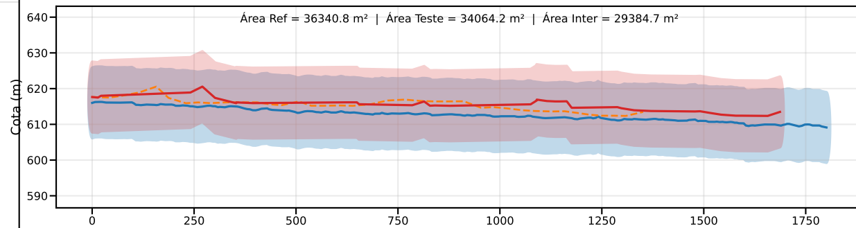
Classe C | PEC-PCD (Vertical)=12.0 m | EQ = 20m | dm = 6.83
