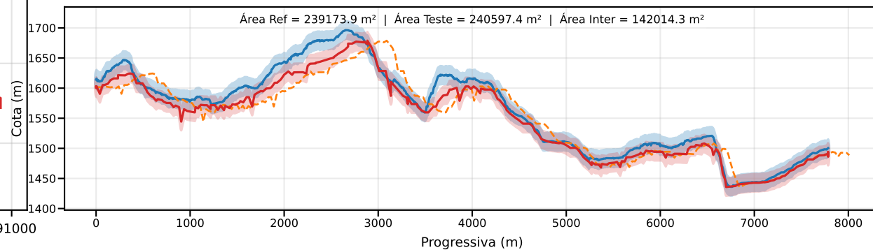
Classe D | PEC-PCD (Vertical)=15.0 m | EQ = 20m | dm = 19.03
