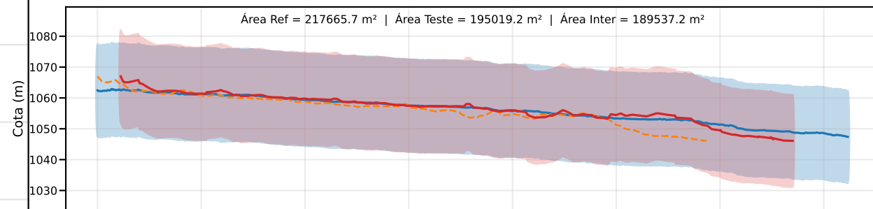
Classe D | PEC-PCD (Vertical)=15.0 m | EQ = 20m | dm = 6.80
