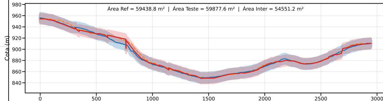
Classe C | PEC-PCD (Vertical)=12.0 m | EQ = 20m | dm = 2.55
