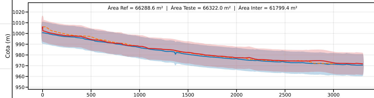
Classe C | PEC-PCD (Vertical)=12.0 m | EQ = 20m | dm = 2.13
