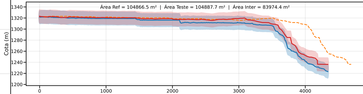
Classe D | PEC-PCD (Vertical)=15.0 m | EQ = 20m | dm = 7.52
