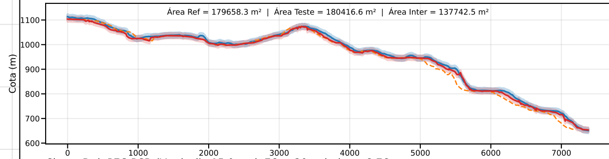
Classe D | PEC-PCD (Vertical)=15.0 m | EQ = 20m | dm = 8.76
