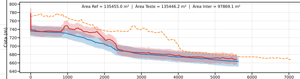
Classe D | PEC-PCD (Vertical)=15.0 m | EQ = 20m | dm = 10.55
