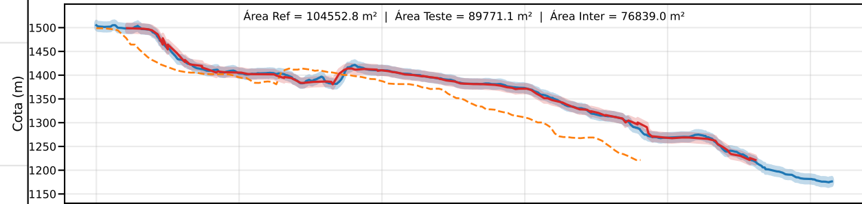
Classe C | PEC-PCD (Vertical)=12.0 m | EQ = 20m | dm = 10.76
