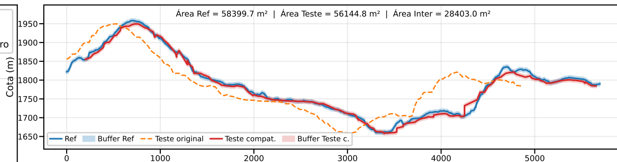
Classe B | PEC-PCD (Vertical)=10.0 m | EQ = 20m | dm = 10.06
