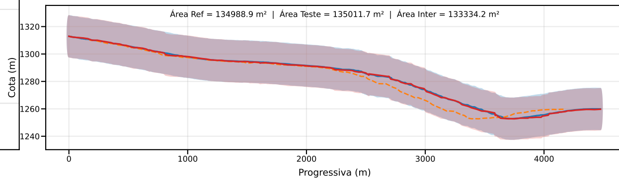
Classe D | PEC-PCD (Vertical)=15.0 m | EQ = 20m | dm = 0.58
