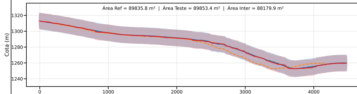
Classe C | PEC-PCD (Vertical)=12.0 m | EQ = 20m | dm = 0.58
