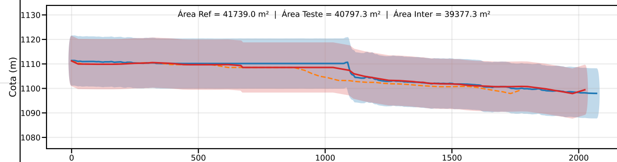
Classe C | PEC-PCD (Vertical)=12.0 m | EQ = 20m | dm = 1.96
