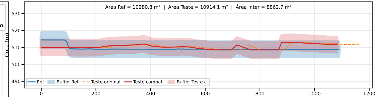
Classe B | PEC-PCD (Vertical)=10.0 m | EQ = 20m | dm = 3.16
