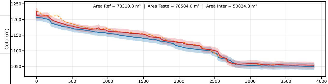
Classe C | PEC-PCD (Vertical)=12.0 m | EQ = 20m | dm = 10.99
