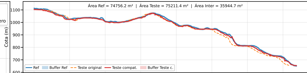
Classe B | PEC-PCD (Vertical)=10.0 m | EQ = 20m | dm = 8.76
