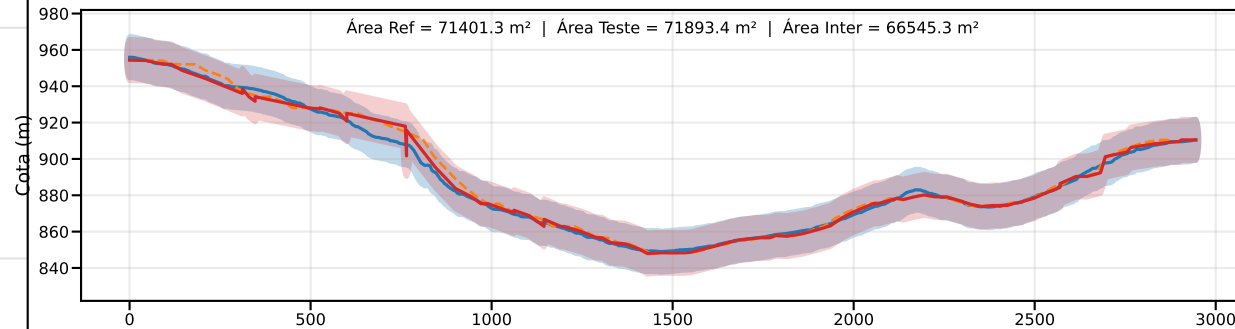
Classe D | PEC-PCD (Vertical)=15.0 m | EQ = 20m | dm = 2.52
