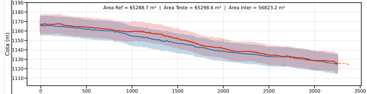
Classe C | PEC-PCD (Vertical)=12.0 m | EQ = 20m | dm = 4.07
