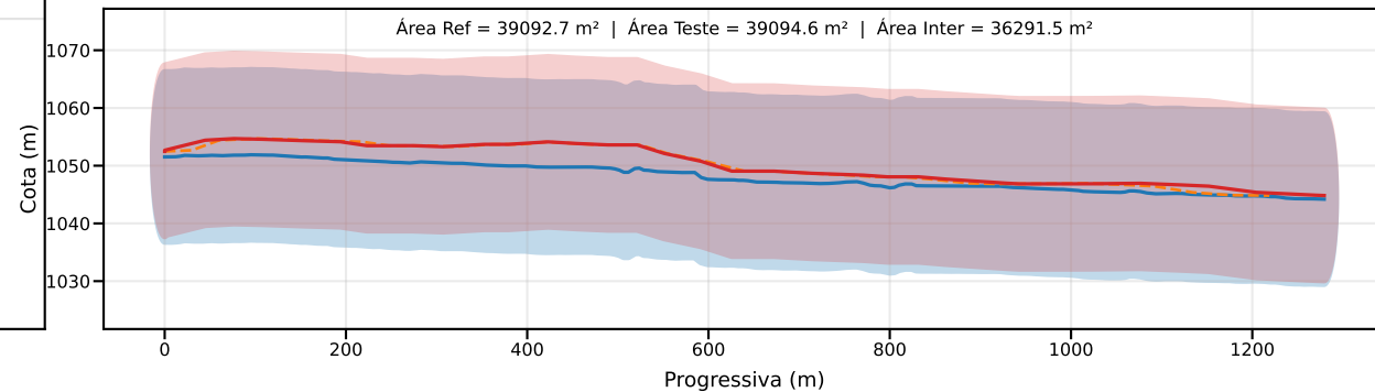
Classe D | PEC-PCD (Vertical)=15.0 m | EQ = 20m | dm = 3.38
