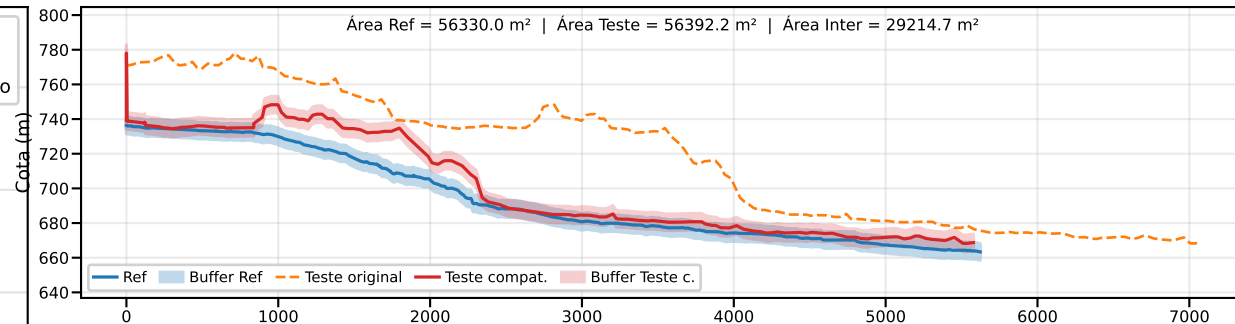
Classe B | PEC-PCD (Vertical)=10.0 m | EQ = 20m | dm = 10.26
