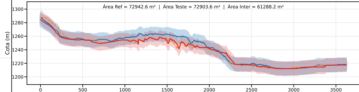
Classe C | PEC-PCD (Vertical)=12.0 m | EQ = 20m | dm = 5.03
