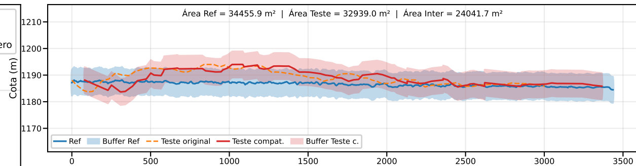
Classe B | PEC-PCD (Vertical)=10.0 m | EQ = 20m | dm = 5.68
