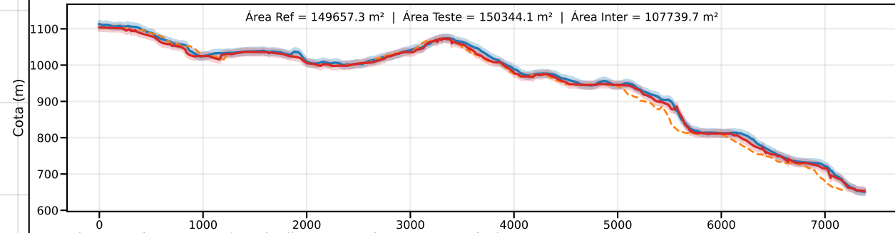
Classe C | PEC-PCD (Vertical)=12.0 m | EQ = 20m | dm = 8.76
