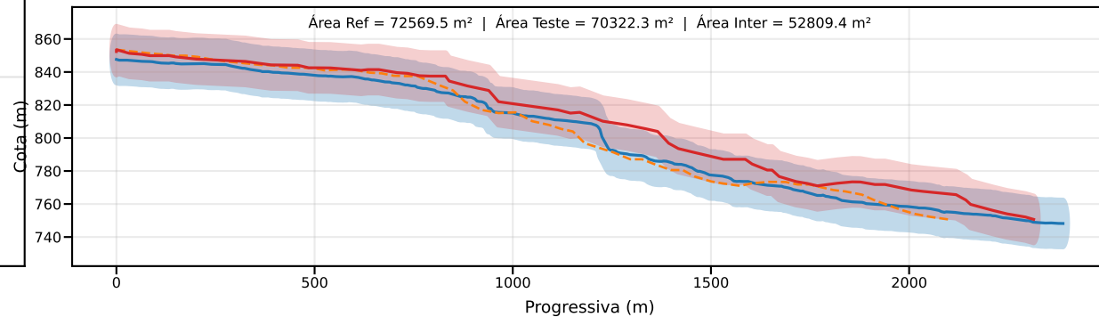
Classe D | PEC-PCD (Vertical)=15.0 m | EQ = 20m | dm = 13.24
