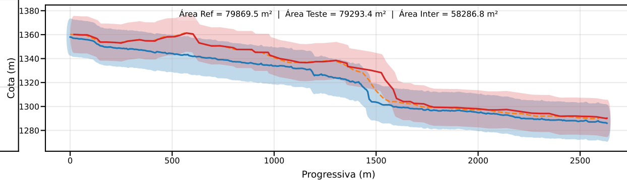
Classe D | PEC-PCD (Vertical)=15.0 m | EQ = 20m | dm = 12.83
