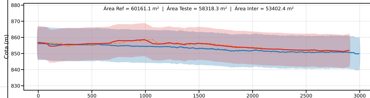
Classe C | PEC-PCD (Vertical)=12.0 m | EQ = 20m | dm = 3.84
