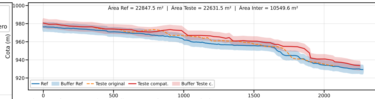
Classe B | PEC-PCD (Vertical)=10.0 m | EQ = 20m | dm = 8.76
