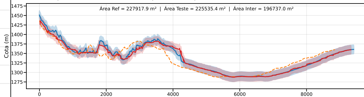
Classe D | PEC-PCD (Vertical)=15.0 m | EQ = 20m | dm = 5.33
