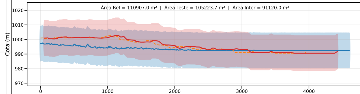
Classe D | PEC-PCD (Vertical)=15.0 m | EQ = 20m | dm = 7.59
