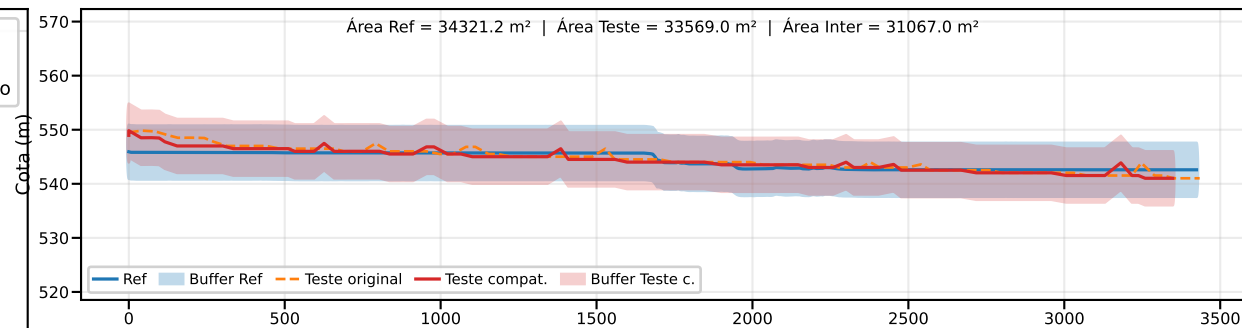
Classe B | PEC-PCD (Vertical)=10.0 m | EQ = 20m | dm = 1.88
