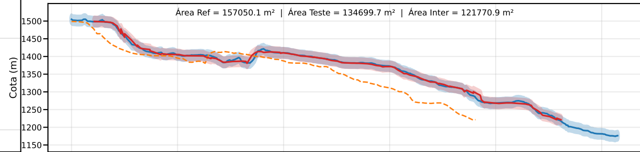
Classe D | PEC-PCD (Vertical)=15.0 m | EQ = 20m | dm = 12.34
