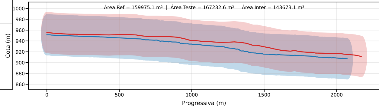
Classe D | PEC-PCD (Vertical)=37.5 m | EQ = 50m | dm = 11.48
