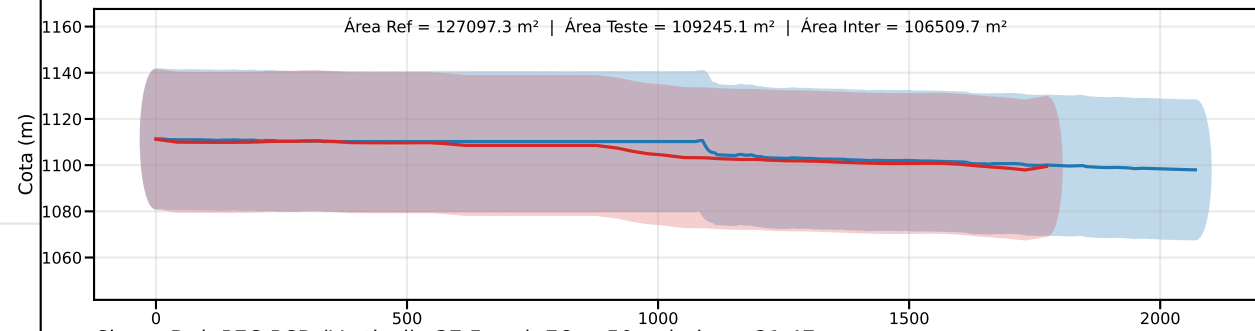
Classe D | PEC-PCD (Vertical)=37.5 m | EQ = 50m | dm = 21.47
