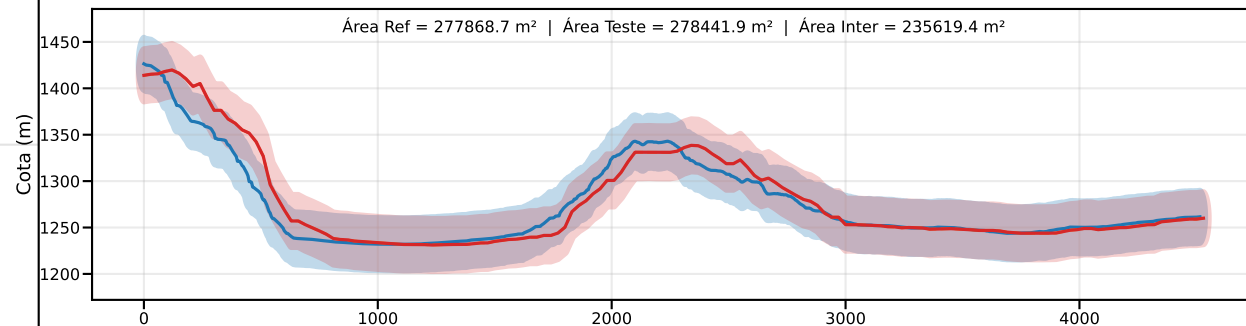
Classe D | PEC-PCD (Vertical)=37.5 m | EQ = 50m | dm = 14.30
