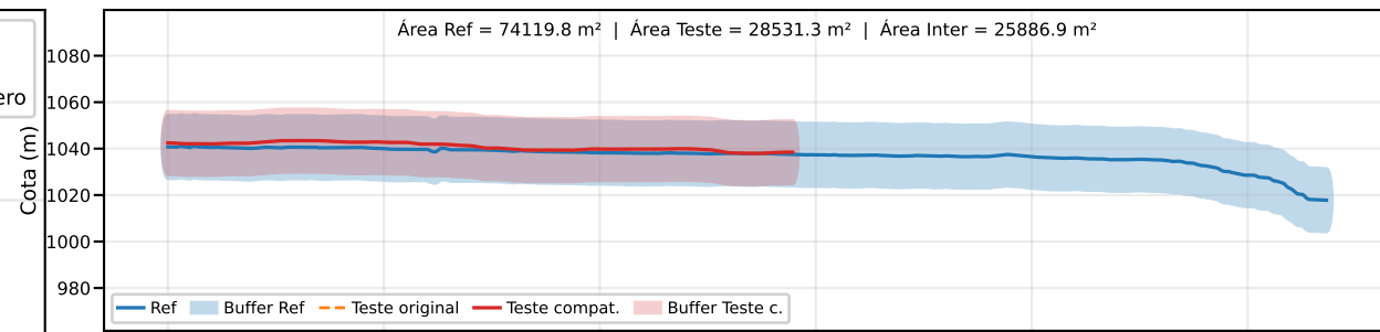
Classe B | PEC-PCD (Vertical)=25.0 m | EQ = 50m | dm = 127.60
