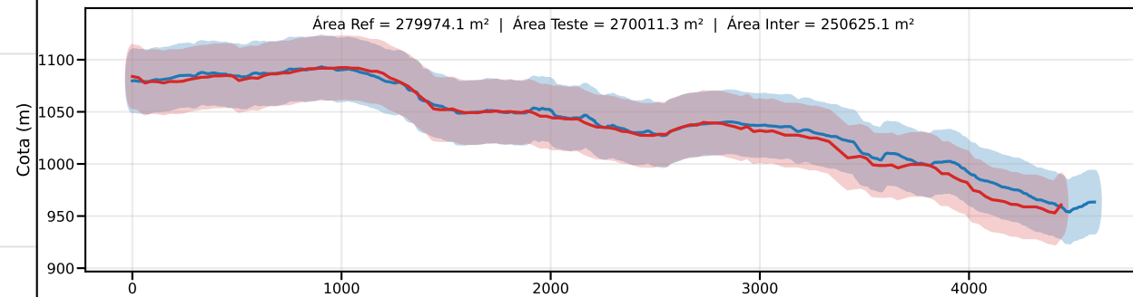
Classe D | PEC-PCD (Vertical)=37.5 m | EQ = 50m | dm = 11.08
