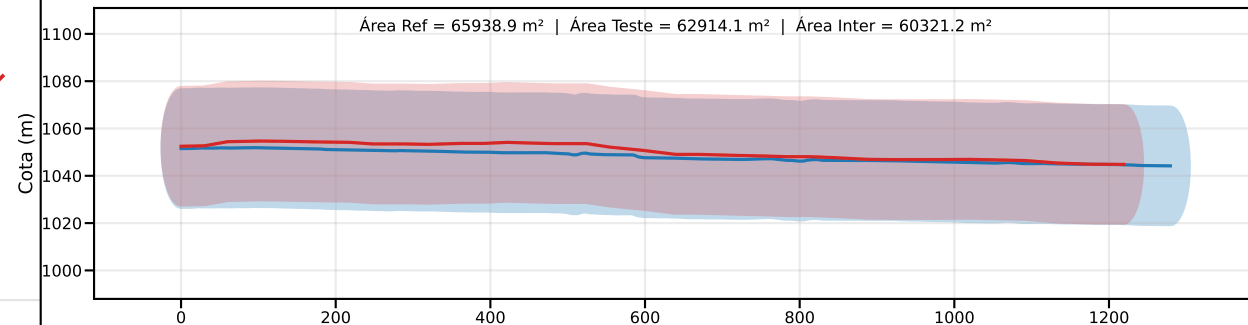
Classe C | PEC-PCD (Vertical)=30.0 m | EQ = 50m | dm = 7.73
