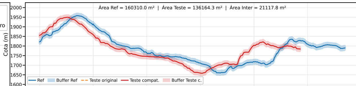
Classe B | PEC-PCD (Vertical)=25.0 m | EQ = 50m | dm = 65.26
