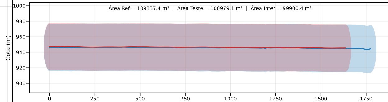
Classe D | PEC-PCD (Vertical)=37.5 m | EQ = 50m | dm = 10.69
