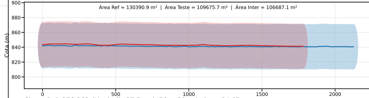
Classe D | PEC-PCD (Vertical)=37.5 m | EQ = 50m | dm = 24.67
