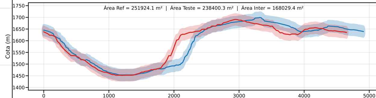
Classe C | PEC-PCD (Vertical)=30.0 m | EQ = 50m | dm = 29.48
