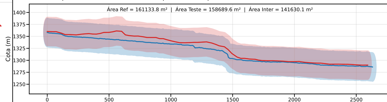
Classe D | PEC-PCD (Vertical)=37.5 m | EQ = 50m | dm = 11.89
