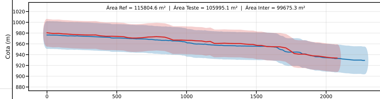
Classe C | PEC-PCD (Vertical)=30.0 m | EQ = 50m | dm = 13.37
