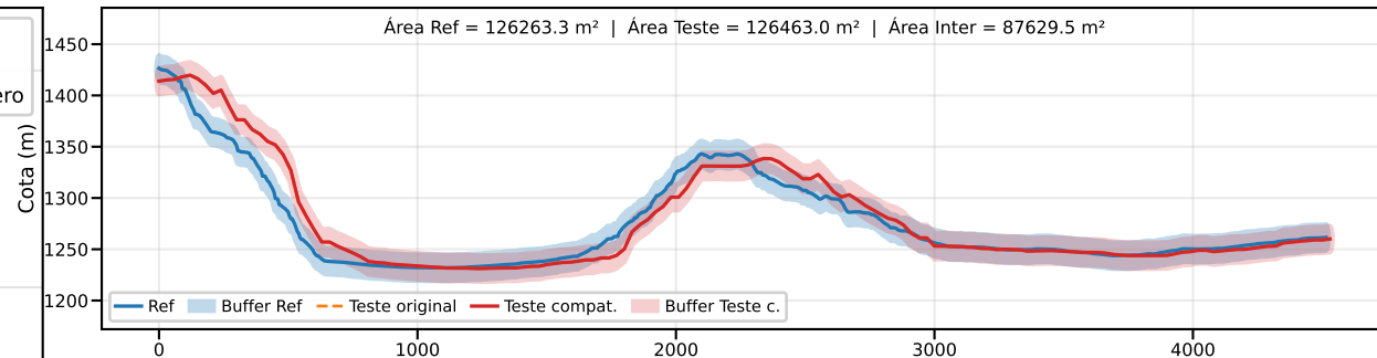
Classe B | PEC-PCD (Vertical)=25.0 m | EQ = 50m | dm = 14.30
