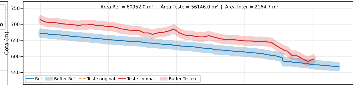
Classe B | PEC-PCD (Vertical)=25.0 m | EQ = 50m | dm = 61.09
