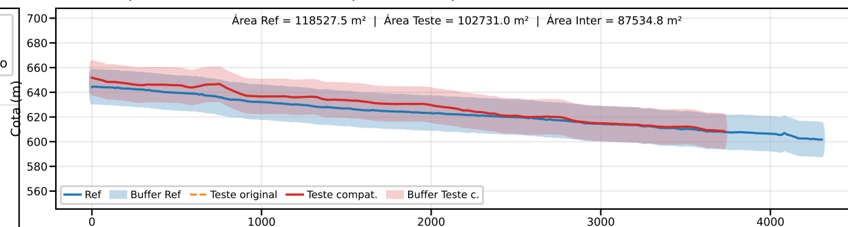
Classe B | PEC-PCD (Vertical)=25.0 m | EQ = 50m | dm = 18.39
