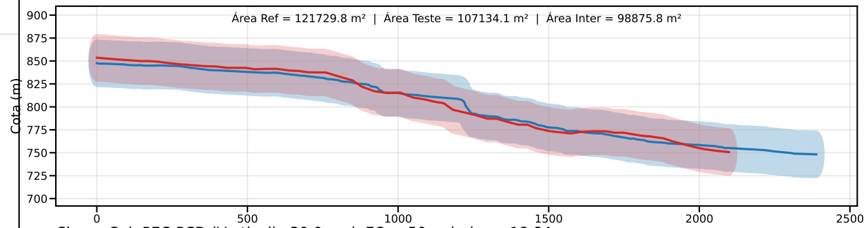
Classe C | PEC-PCD (Vertical)=30.0 m | EQ = 50m | dm = 18.84
