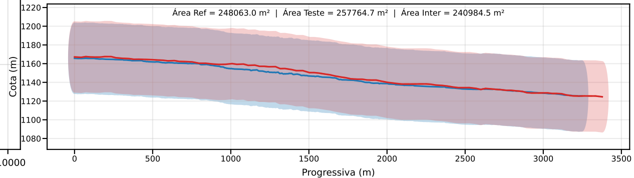
Classe D | PEC-PCD (Vertical)=37.5 m | EQ = 50m | dm = 3.24
