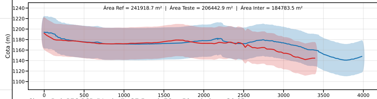
Classe D | PEC-PCD (Vertical)=37.5 m | EQ = 50m | dm = 30.05
