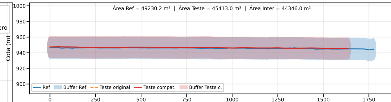
Classe B | PEC-PCD (Vertical)=25.0 m | EQ = 50m | dm = 7.54
