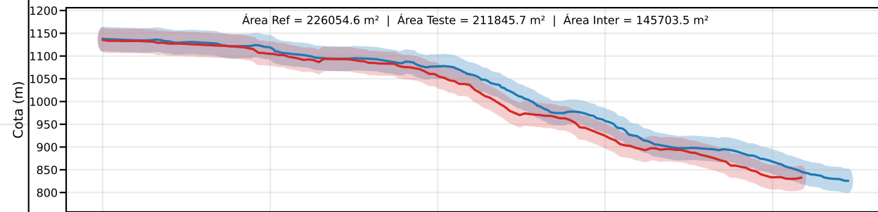
Classe C | PEC-PCD (Vertical)=30.0 m | EQ = 50m | dm = 30.79
