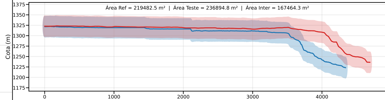
Classe C | PEC-PCD (Vertical)=30.0 m | EQ = 50m | dm = 18.22
