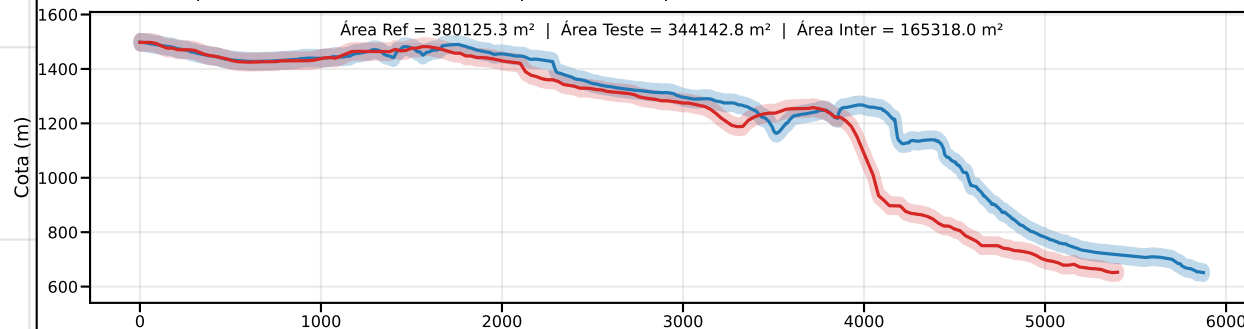
Classe D | PEC-PCD (Vertical)=37.5 m | EQ = 50m | dm = 67.52
