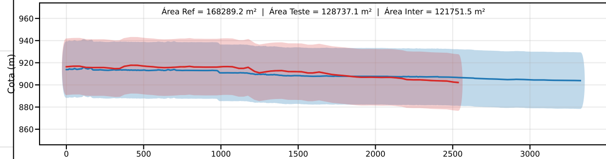
Classe C | PEC-PCD (Vertical)=30.0 m | EQ = 50m | dm = 33.13
