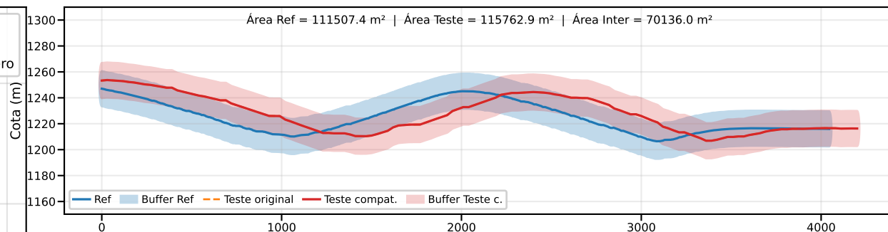
Classe B | PEC-PCD (Vertical)=25.0 m | EQ = 50m | dm = 15.34
