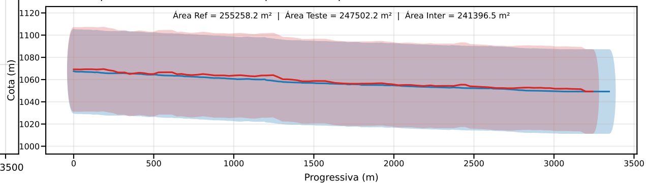
Classe D | PEC-PCD (Vertical)=37.5 m | EQ = 50m | dm = 6.60
