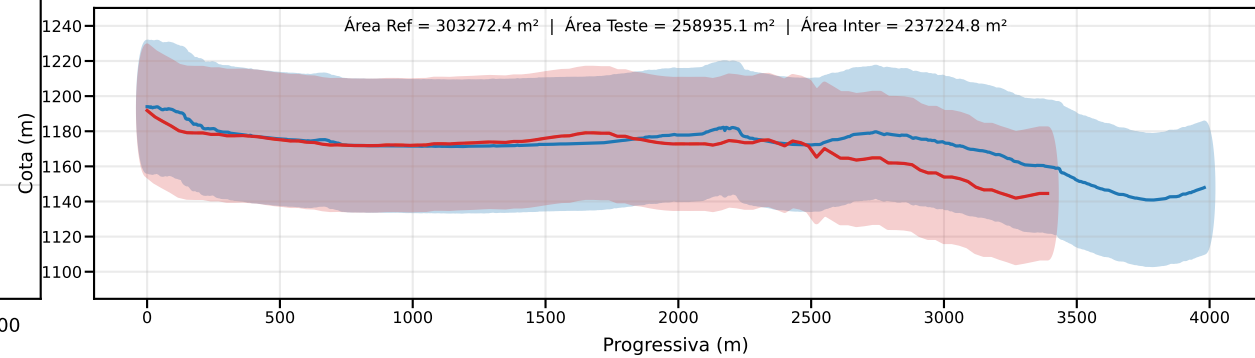
Classe D | PEC-PCD (Vertical)=37.5 m | EQ = 50m | dm = 30.05
