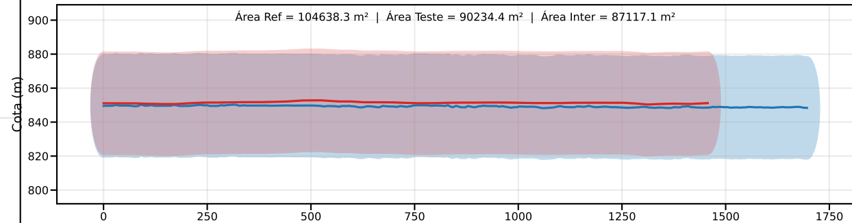
Classe D | PEC-PCD (Vertical)=37.5 m | EQ = 50m | dm = 21.90
