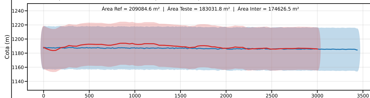
Classe D | PEC-PCD (Vertical)=37.5 m | EQ = 50m | dm = 21.02
