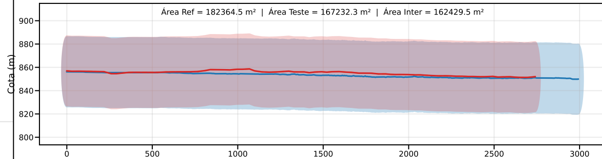
Classe D | PEC-PCD (Vertical)=37.5 m | EQ = 50m | dm = 13.31
