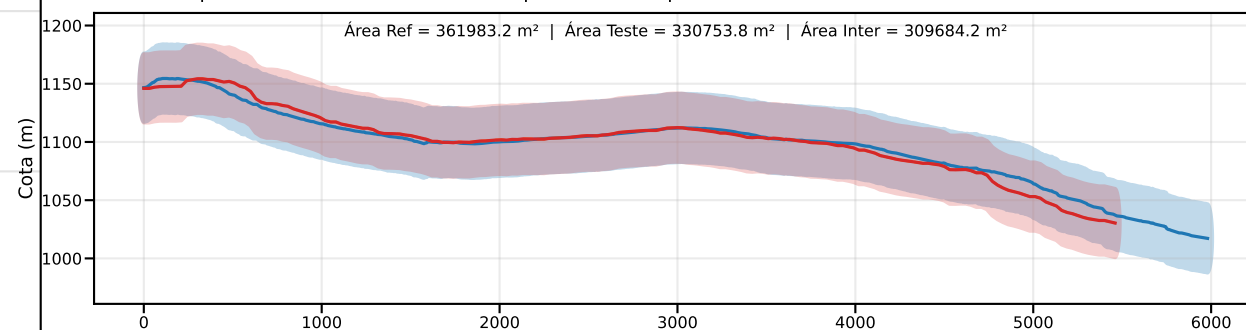
Classe D | PEC-PCD (Vertical)=37.5 m | EQ = 50m | dm = 17.09
