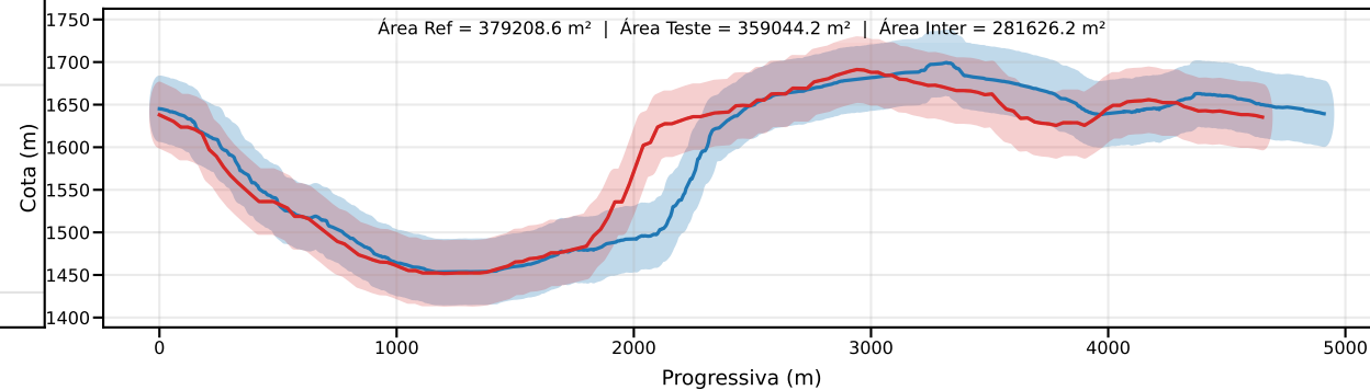
Classe D | PEC-PCD (Vertical)=37.5 m | EQ = 50m | dm = 32.02
