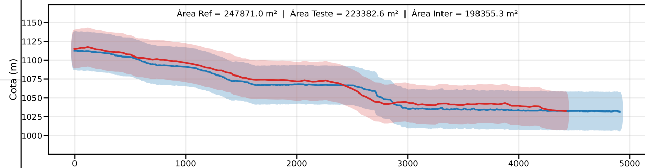
Classe C | PEC-PCD (Vertical)=30.0 m | EQ = 50m | dm = 19.10
