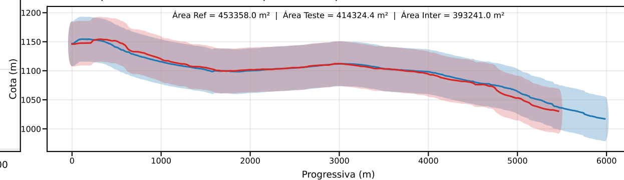
Classe D | PEC-PCD (Vertical)=37.5 m | EQ = 50m | dm = 17.09
