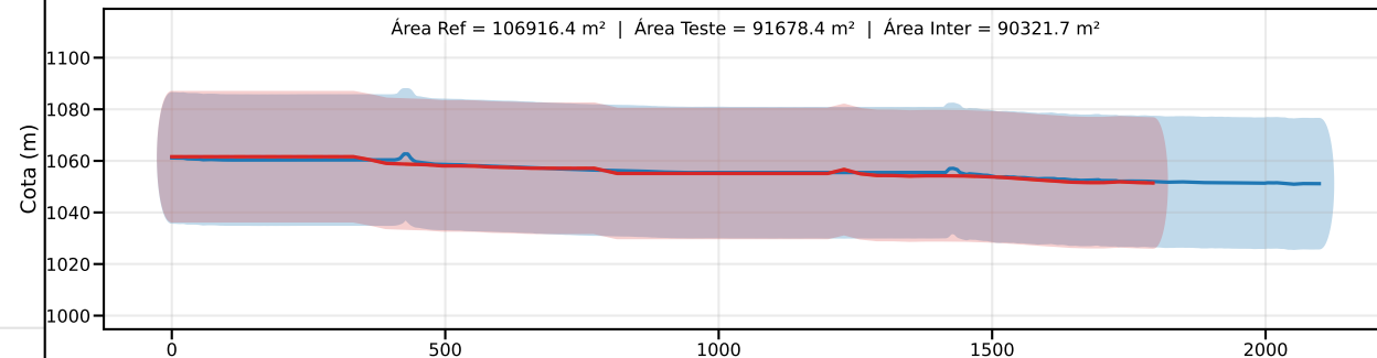
Classe C | PEC-PCD (Vertical)=30.0 m | EQ = 50m | dm = 16.75
