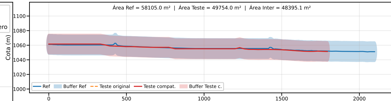
Classe B | PEC-PCD (Vertical)=25.0 m | EQ = 50m | dm = 14.22
