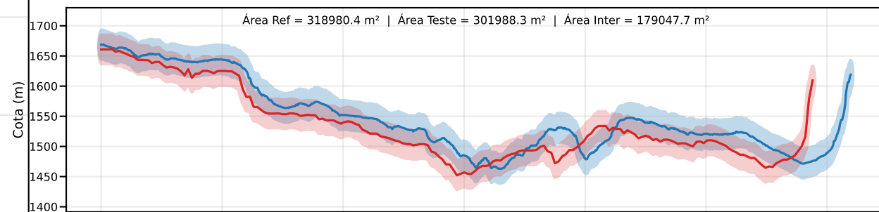
Classe C | PEC-PCD (Vertical)=30.0 m | EQ = 50m | dm = 37.58
