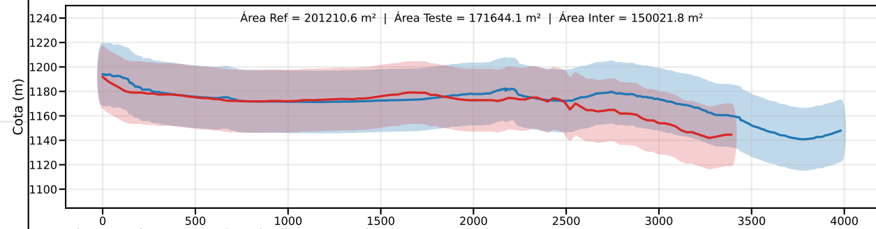
Classe C | PEC-PCD (Vertical)=30.0 m | EQ = 50m | dm = 26.08
