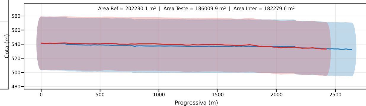
Classe D | PEC-PCD (Vertical)=37.5 m | EQ = 50m | dm = 12.64
