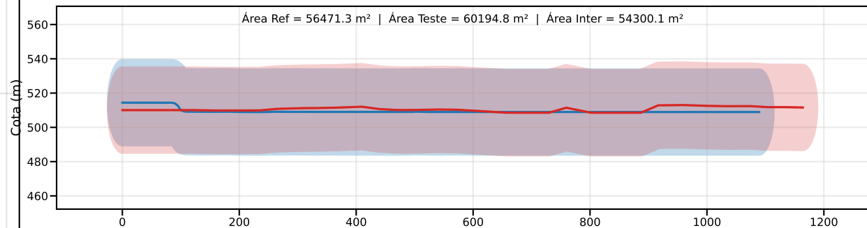
Classe C | PEC-PCD (Vertical)=30.0 m | EQ = 50m | dm = 2.85
