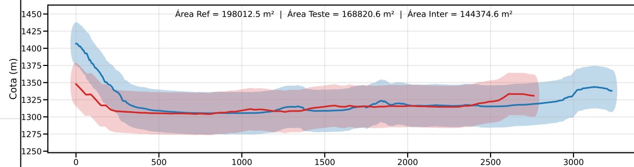
Classe D | PEC-PCD (Vertical)=37.5 m | EQ = 50m | dm = 34.13
