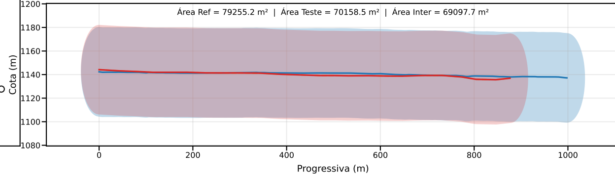
Classe D | PEC-PCD (Vertical)=37.5 m | EQ = 50m | dm = 17.06
