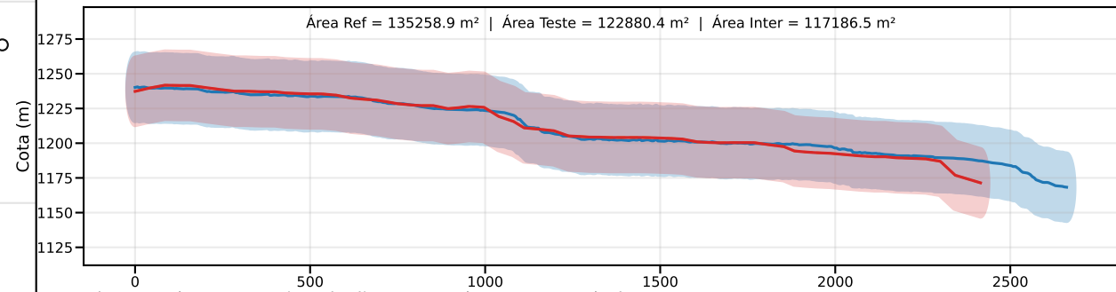
Classe C | PEC-PCD (Vertical)=30.0 m | EQ = 50m | dm = 13.12
