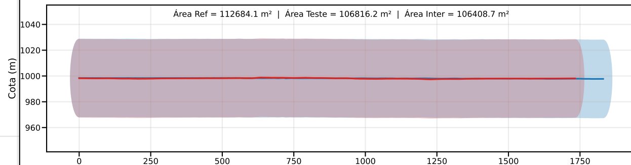
Classe D | PEC-PCD (Vertical)=37.5 m | EQ = 50m | dm = 6.79
