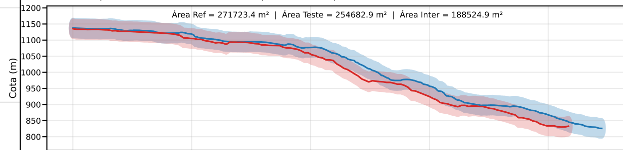
Classe D | PEC-PCD (Vertical)=37.5 m | EQ = 50m | dm = 32.28
