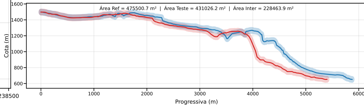
Classe D | PEC-PCD (Vertical)=37.5 m | EQ = 50m | dm = 67.52
