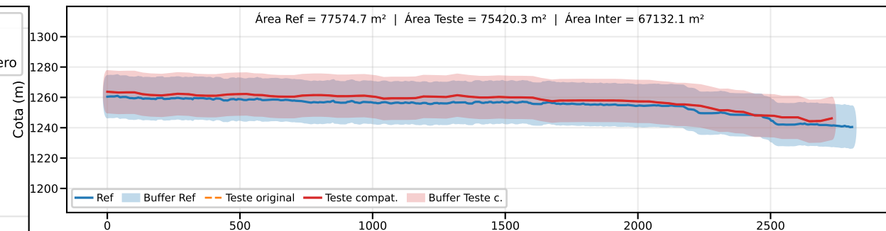
Classe B | PEC-PCD (Vertical)=25.0 m | EQ = 50m | dm = 6.94
