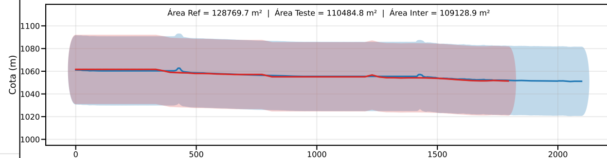
Classe D | PEC-PCD (Vertical)=37.5 m | EQ = 50m | dm = 20.52
