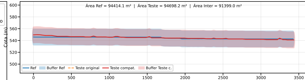
Classe B | PEC-PCD (Vertical)=25.0 m | EQ = 50m | dm = 1.38
