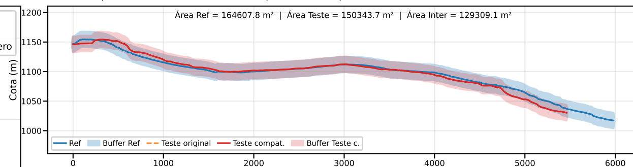
Classe B | PEC-PCD (Vertical)=25.0 m | EQ = 50m | dm = 13.44
