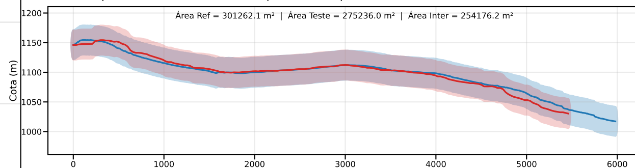
Classe C | PEC-PCD (Vertical)=30.0 m | EQ = 50m | dm = 14.90
