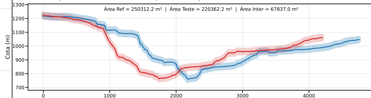
Classe C | PEC-PCD (Vertical)=30.0 m | EQ = 50m | dm = 74.21
