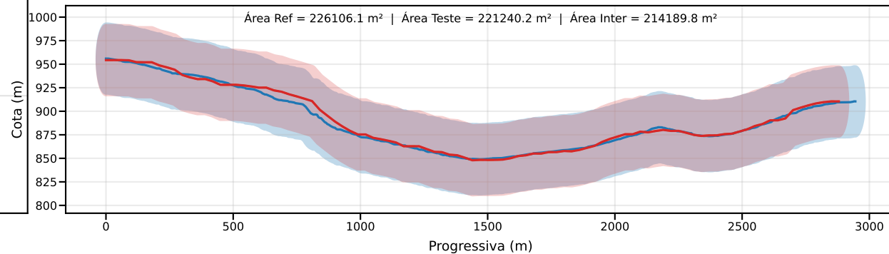
Classe D | PEC-PCD (Vertical)=37.5 m | EQ = 50m | dm = 6.35
