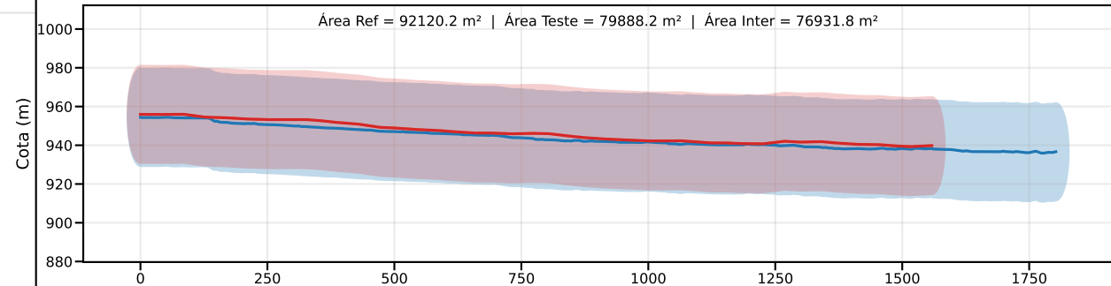
Classe C | PEC-PCD (Vertical)=30.0 m | EQ = 50m | dm = 17.26
