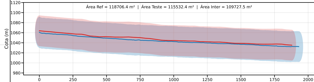
Classe D | PEC-PCD (Vertical)=37.5 m | EQ = 50m | dm = 7.94
