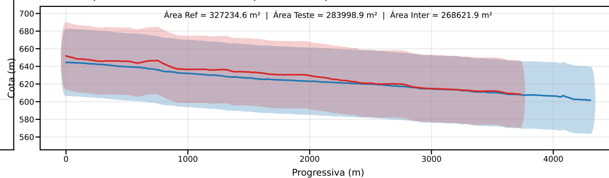
Classe D | PEC-PCD (Vertical)=37.5 m | EQ = 50m | dm = 24.31
