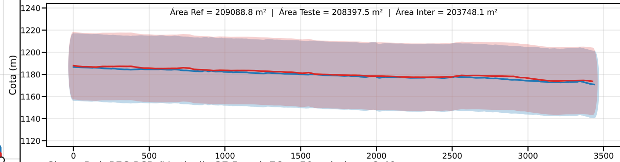
Classe D | PEC-PCD (Vertical)=37.5 m | EQ = 50m | dm = 2.49
