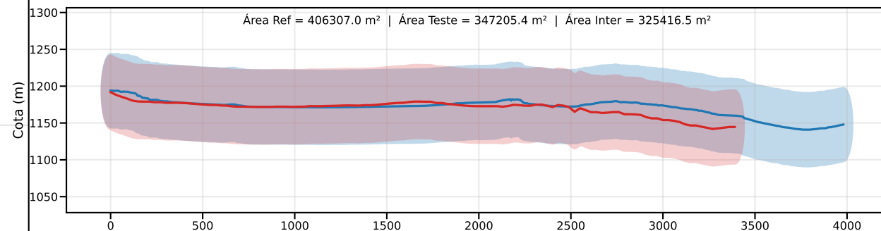
Classe C | PEC-PCD (Vertical)=60.0 m | EQ = 100m | dm = 41.78
