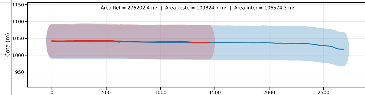
Classe C | PEC-PCD (Vertical)=60.0 m | EQ = 100m | dm = 286.35
