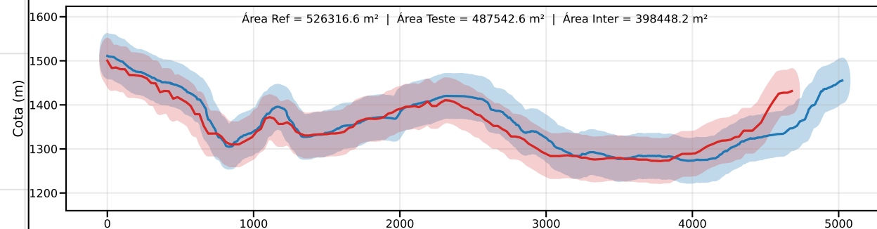
Classe C | PEC-PCD (Vertical)=60.0 m | EQ = 100m | dm = 43.63
