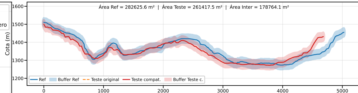
Classe B | PEC-PCD (Vertical)=50.0 m | EQ = 100m | dm = 41.20
