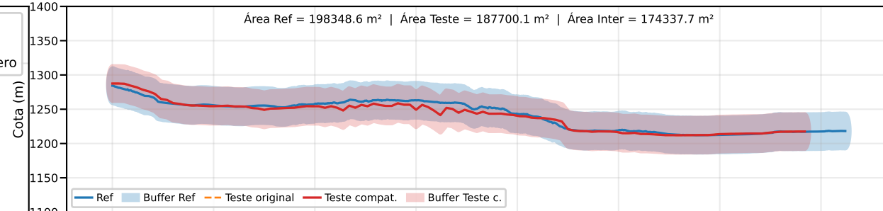
Classe B | PEC-PCD (Vertical)=50.0 m | EQ = 100m | dm = 14.85
