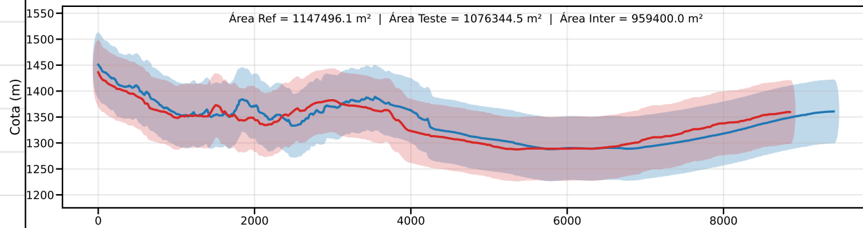
Classe D | PEC-PCD (Vertical)=75.0 m | EQ = 100m | dm = 35.89
