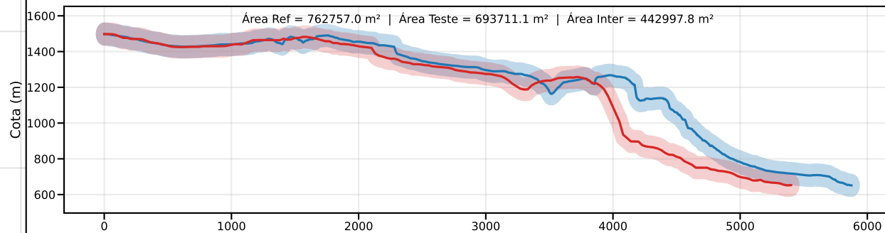
Classe D | PEC-PCD (Vertical)=75.0 m | EQ = 100m | dm = 97.87
