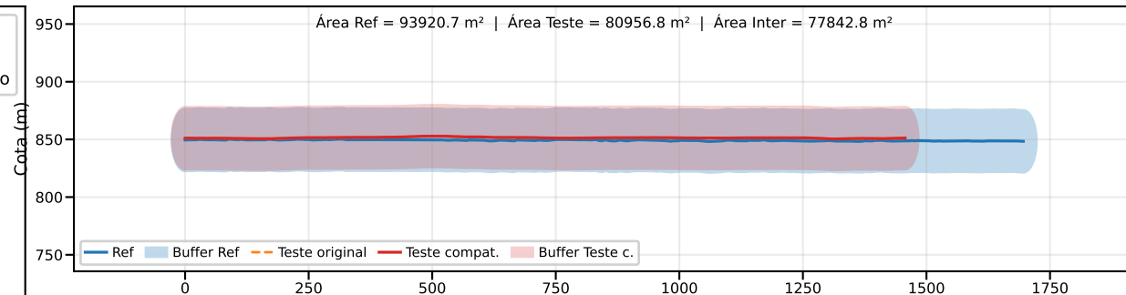
Classe B | PEC-PCD (Vertical)=50.0 m | EQ = 100m | dm = 27.77
