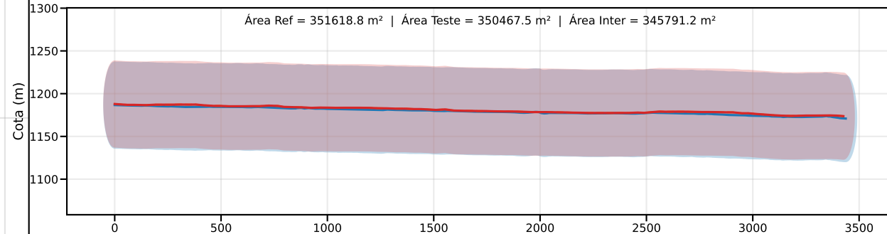
Classe C | PEC-PCD (Vertical)=60.0 m | EQ = 100m | dm = 2.71
