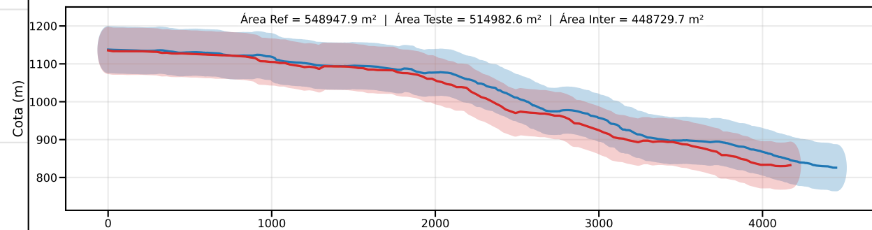
Classe D | PEC-PCD (Vertical)=75.0 m | EQ = 100m | dm = 39.57
