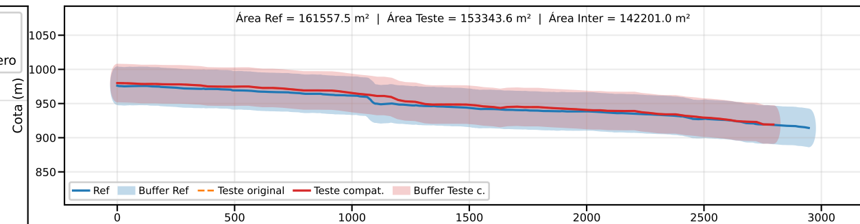
Classe B | PEC-PCD (Vertical)=50.0 m | EQ = 100m | dm = 14.43
