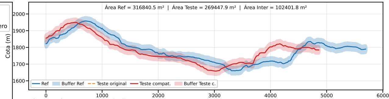
Classe B | PEC-PCD (Vertical)=50.0 m | EQ = 100m | dm = 85.09
