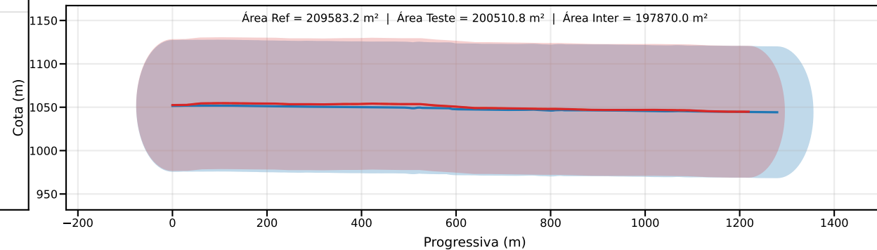
Classe D | PEC-PCD (Vertical)=75.0 m | EQ = 100m | dm = 13.76
