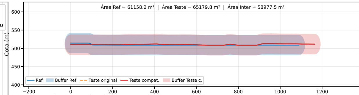
Classe B | PEC-PCD (Vertical)=50.0 m | EQ = 100m | dm = 2.89
