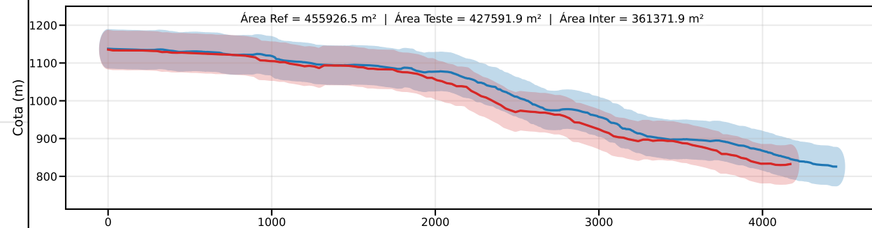
Classe C | PEC-PCD (Vertical)=60.0 m | EQ = 100m | dm = 36.68
