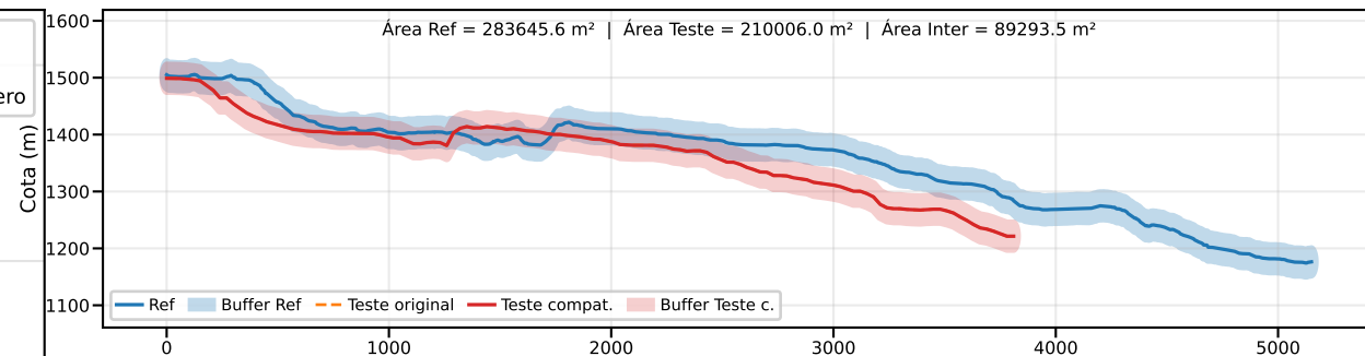
Classe B | PEC-PCD (Vertical)=50.0 m | EQ = 100m | dm = 106.75
