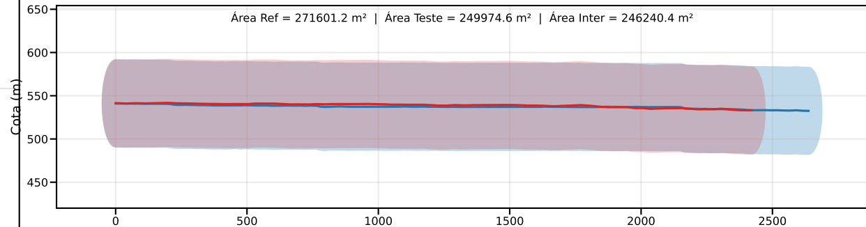
Classe C | PEC-PCD (Vertical)=60.0 m | EQ = 100m | dm = 18.54
