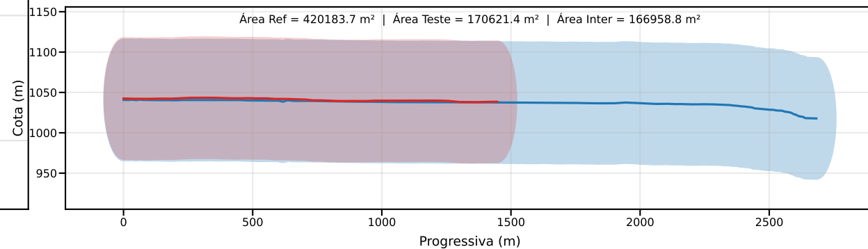
Classe D | PEC-PCD (Vertical)=75.0 m | EQ = 100m | dm = 349.69
