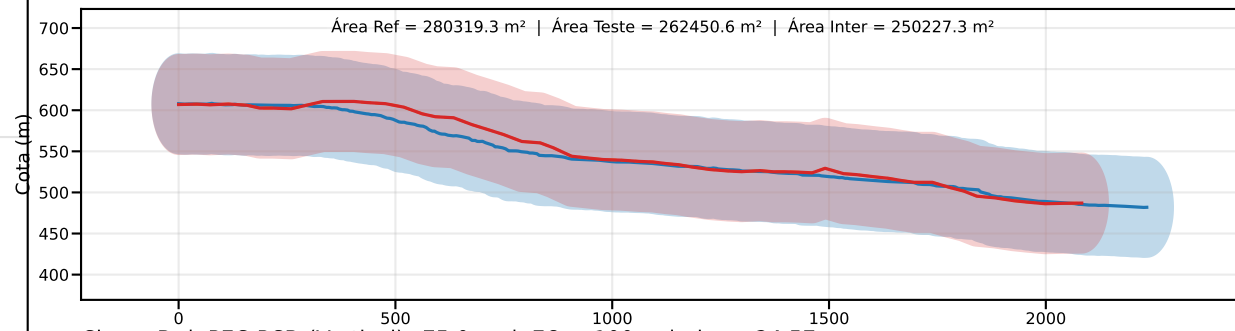
Classe D | PEC-PCD (Vertical)=75.0 m | EQ = 100m | dm = 24.57
