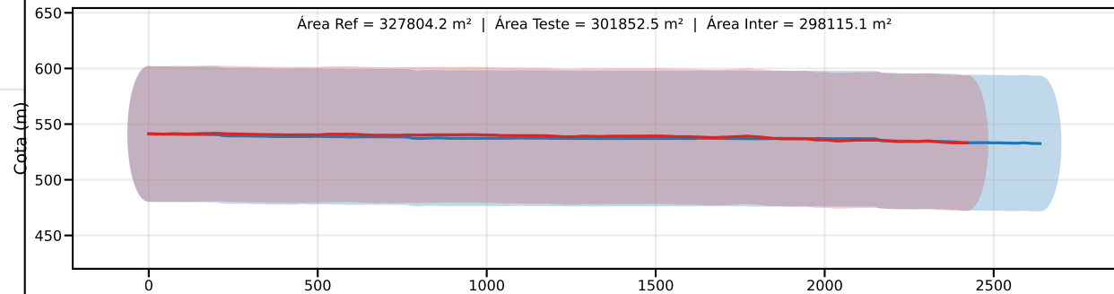
Classe D | PEC-PCD (Vertical)=75.0 m | EQ = 100m | dm = 22.38
