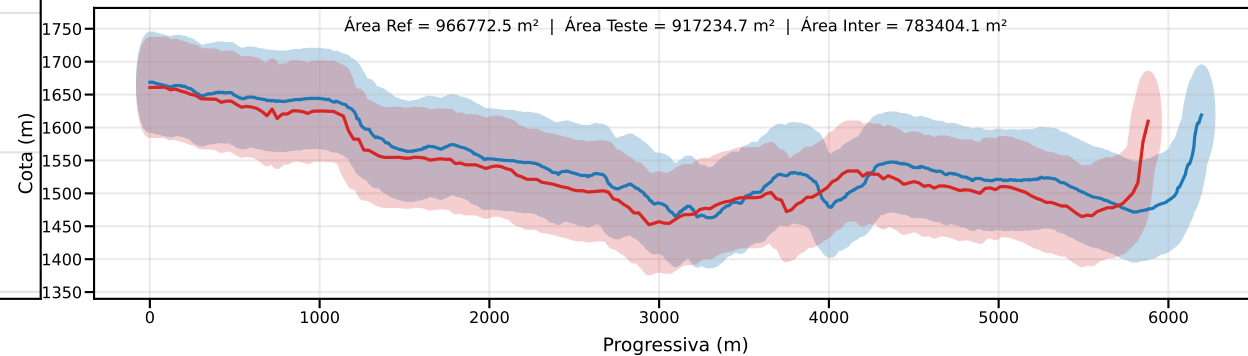
Classe D | PEC-PCD (Vertical)=75.0 m | EQ = 100m | dm = 47.10
