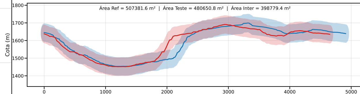
Classe C | PEC-PCD (Vertical)=60.0 m | EQ = 100m | dm = 37.44
