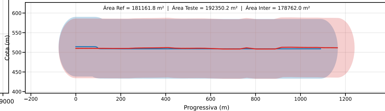
Classe D | PEC-PCD (Vertical)=75.0 m | EQ = 100m | dm = 2.94
