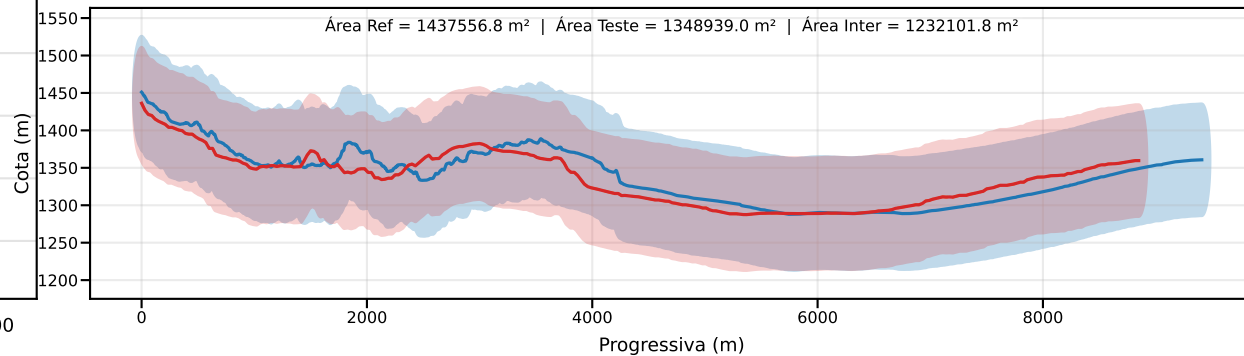
Classe D | PEC-PCD (Vertical)=75.0 m | EQ = 100m | dm = 35.89
