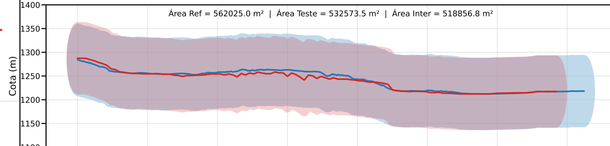
Classe D | PEC-PCD (Vertical)=75.0 m | EQ = 100m | dm = 19.10
