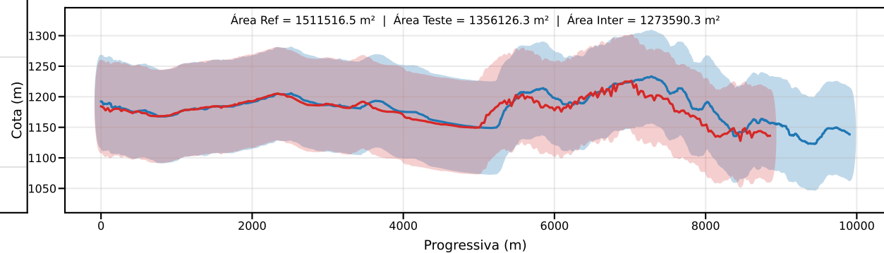
Classe D | PEC-PCD (Vertical)=75.0 m | EQ = 100m | dm = 41.34
