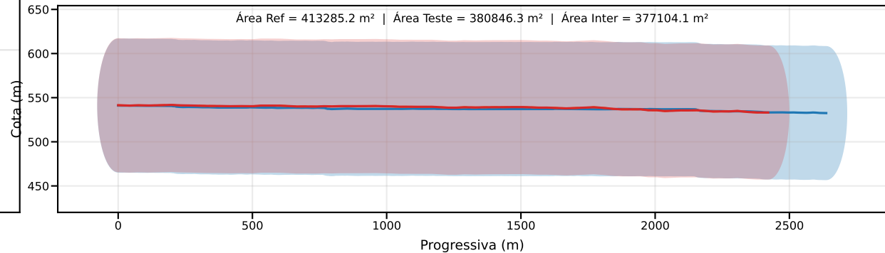
Classe D | PEC-PCD (Vertical)=75.0 m | EQ = 100m | dm = 22.38
