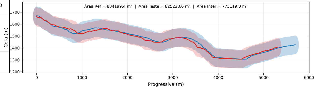
Classe D | PEC-PCD (Vertical)=75.0 m | EQ = 100m | dm = 31.72
