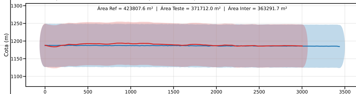
Classe D | PEC-PCD (Vertical)=75.0 m | EQ = 100m | dm = 37.01
