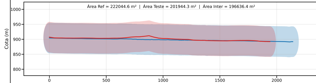
Classe C | PEC-PCD (Vertical)=60.0 m | EQ = 100m | dm = 22.74
