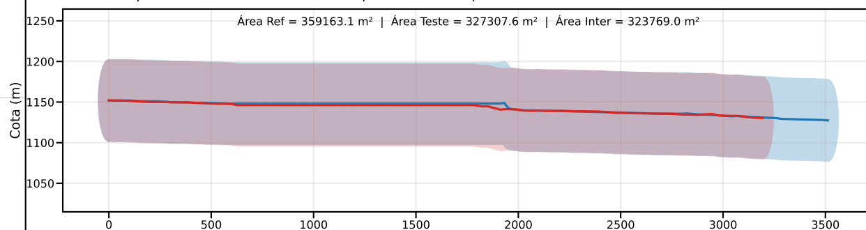
Classe C | PEC-PCD (Vertical)=60.0 m | EQ = 100m | dm = 19.94
