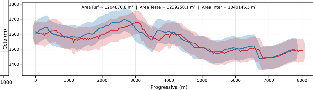
Classe D | PEC-PCD (Vertical)=75.0 m | EQ = 100m | dm = 31.32
