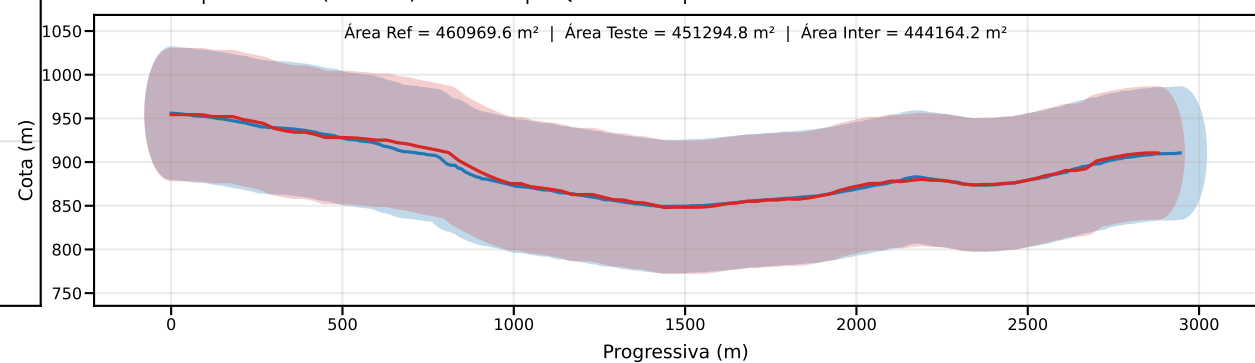
Classe D | PEC-PCD (Vertical)=75.0 m | EQ = 100m | dm = 8.77
