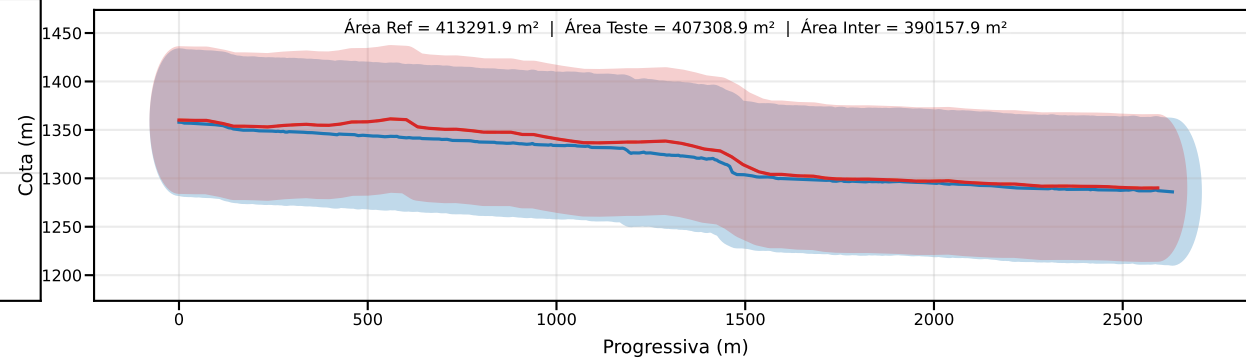
Classe D | PEC-PCD (Vertical)=75.0 m | EQ = 100m | dm = 13.38
