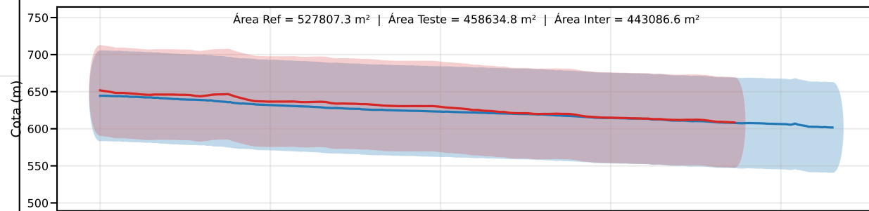
Classe D | PEC-PCD (Vertical)=75.0 m | EQ = 100m | dm = 41.72
