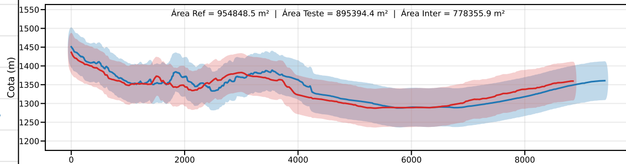
Classe C | PEC-PCD (Vertical)=60.0 m | EQ = 100m | dm = 32.94
