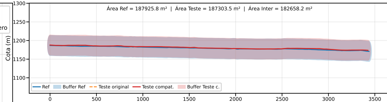
Classe B | PEC-PCD (Vertical)=50.0 m | EQ = 100m | dm = 2.61
