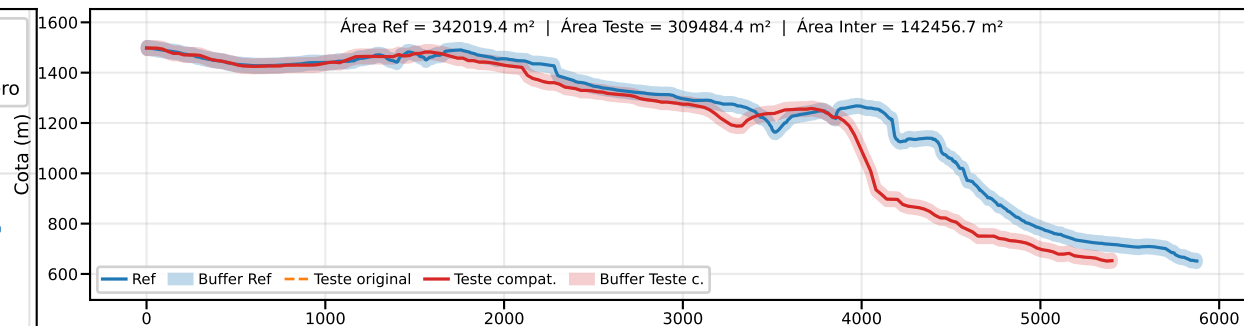
Classe B | PEC-PCD (Vertical)=50.0 m | EQ = 100m | dm = 78.76
