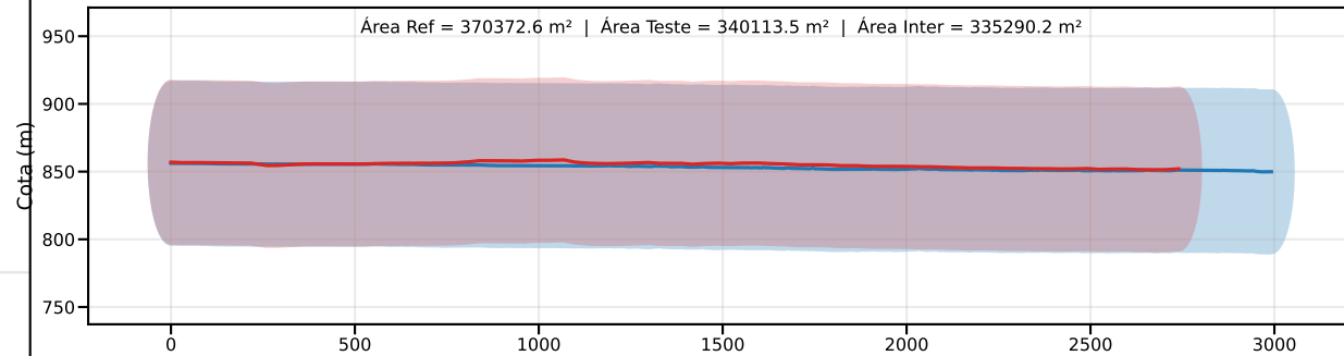
Classe D | PEC-PCD (Vertical)=75.0 m | EQ = 100m | dm = 23.45
