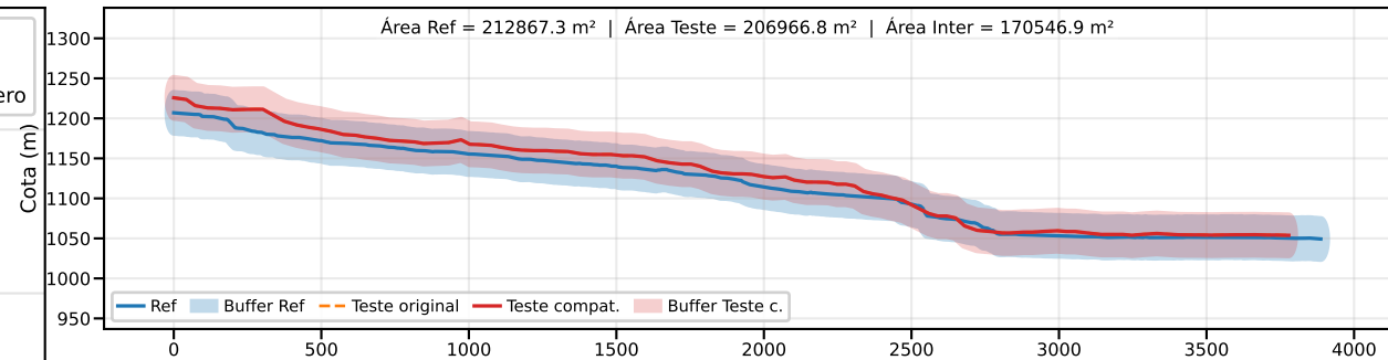
Classe B | PEC-PCD (Vertical)=50.0 m | EQ = 100m | dm = 19.39
