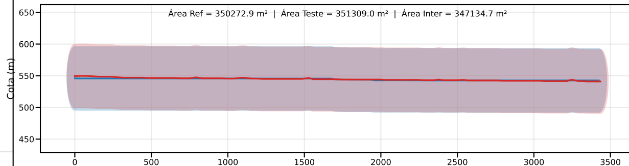
Classe C | PEC-PCD (Vertical)=60.0 m | EQ = 100m | dm = 1.41
