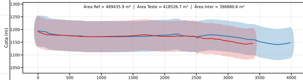
Classe D | PEC-PCD (Vertical)=75.0 m | EQ = 100m | dm = 49.45
