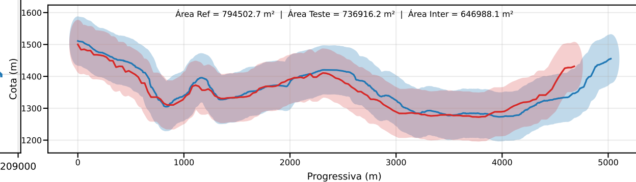
Classe D | PEC-PCD (Vertical)=75.0 m | EQ = 100m | dm = 47.17
