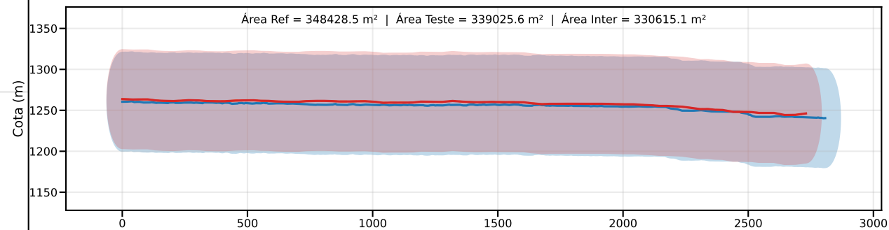
Classe D | PEC-PCD (Vertical)=75.0 m | EQ = 100m | dm = 11.13
