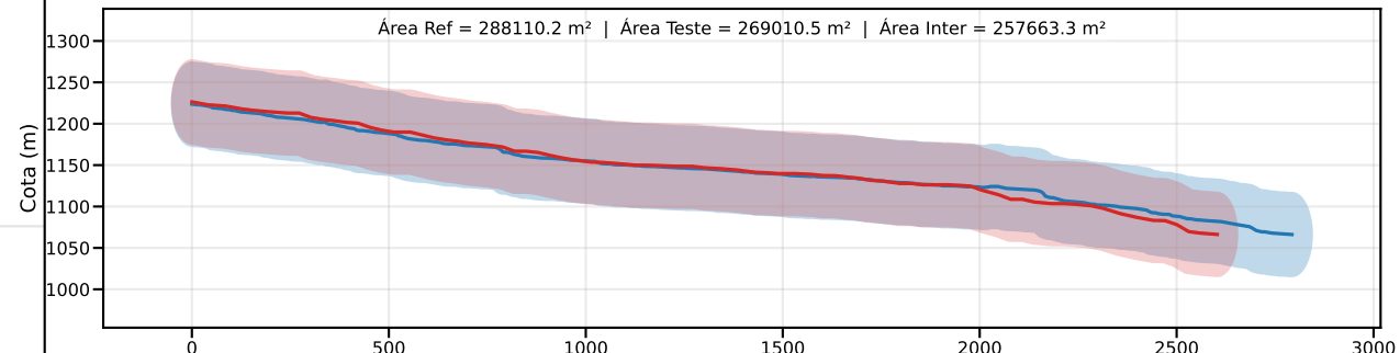
Classe C | PEC-PCD (Vertical)=60.0 m | EQ = 100m | dm = 19.92
