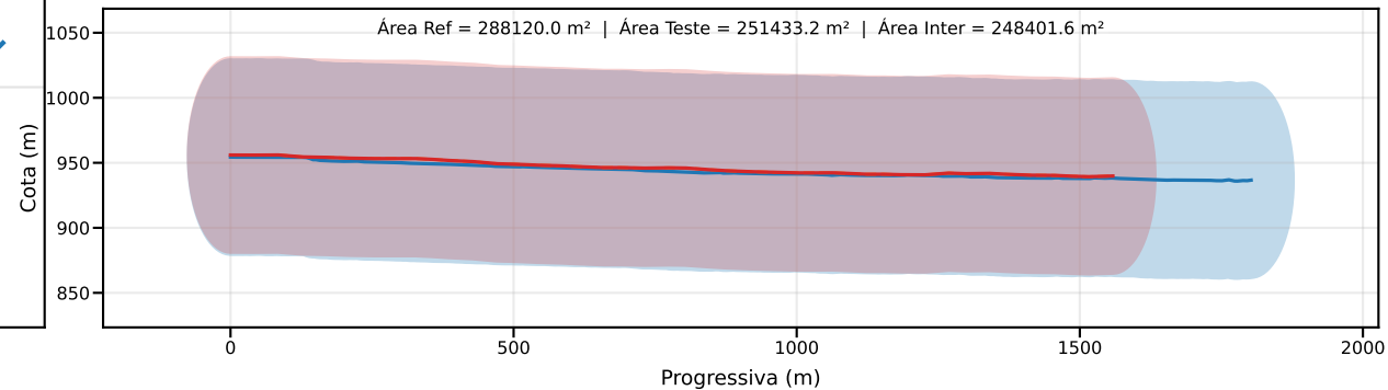
Classe D | PEC-PCD (Vertical)=75.0 m | EQ = 100m | dm = 37.22
