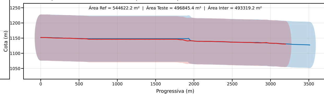
Classe D | PEC-PCD (Vertical)=75.0 m | EQ = 100m | dm = 24.33
