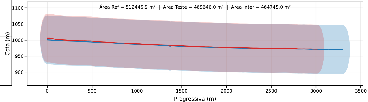
Classe D | PEC-PCD (Vertical)=75.0 m | EQ = 100m | dm = 23.93
