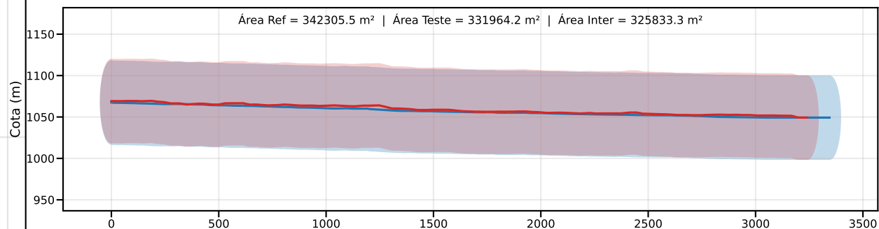
Classe C | PEC-PCD (Vertical)=60.0 m | EQ = 100m | dm = 8.74
