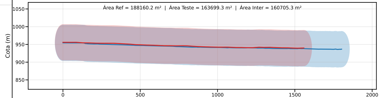
Classe C | PEC-PCD (Vertical)=60.0 m | EQ = 100m | dm = 30.76
