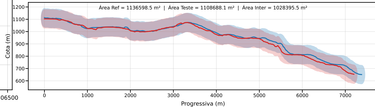
Classe D | PEC-PCD (Vertical)=75.0 m | EQ = 100m | dm = 23.00
