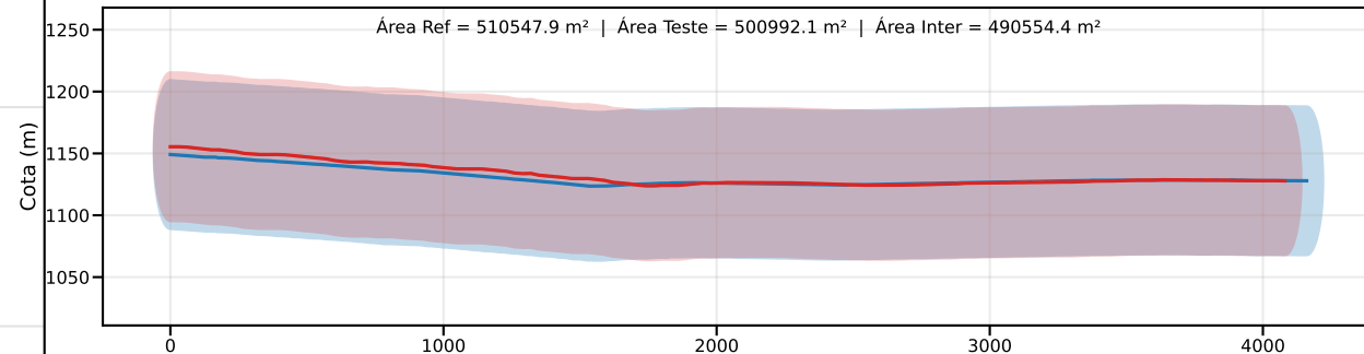
Classe D | PEC-PCD (Vertical)=75.0 m | EQ = 100m | dm = 8.41
