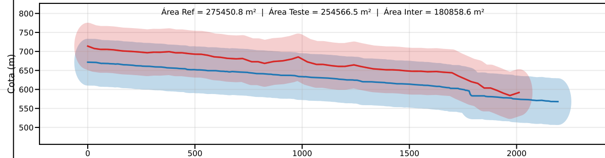
Classe D | PEC-PCD (Vertical)=75.0 m | EQ = 100m | dm = 73.70
