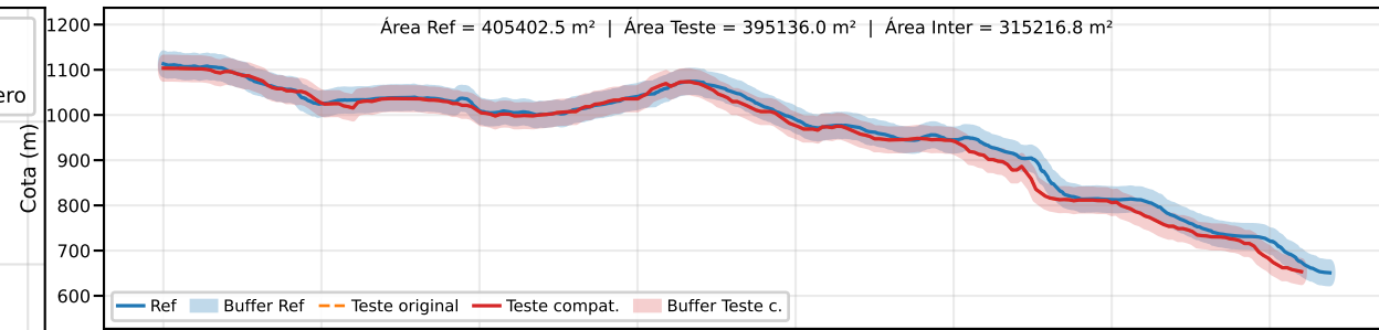
Classe B | PEC-PCD (Vertical)=50.0 m | EQ = 100m | dm = 21.12
