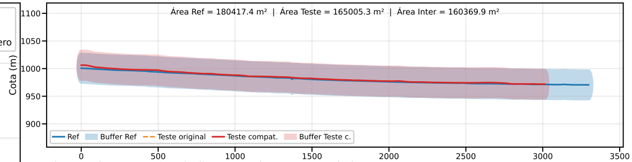
Classe B | PEC-PCD (Vertical)=50.0 m | EQ = 100m | dm = 16.92
