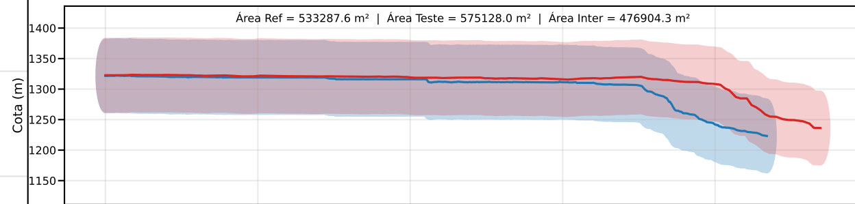
Classe D | PEC-PCD (Vertical)=75.0 m | EQ = 100m | dm = 18.46
