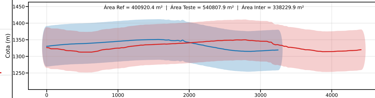
Classe D | PEC-PCD (Vertical)=75.0 m | EQ = 100m | dm = 21.77
