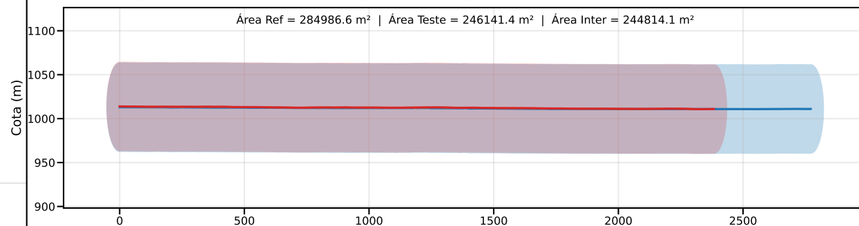
Classe C | PEC-PCD (Vertical)=60.0 m | EQ = 100m | dm = 30.41
