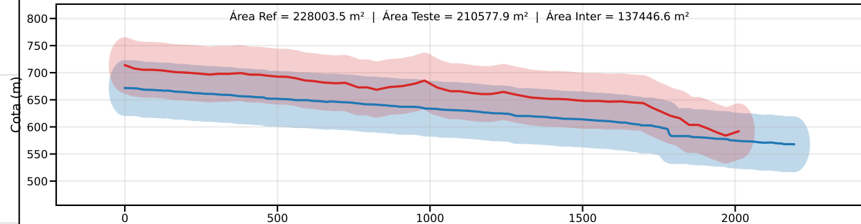
Classe C | PEC-PCD (Vertical)=60.0 m | EQ = 100m | dm = 70.04
