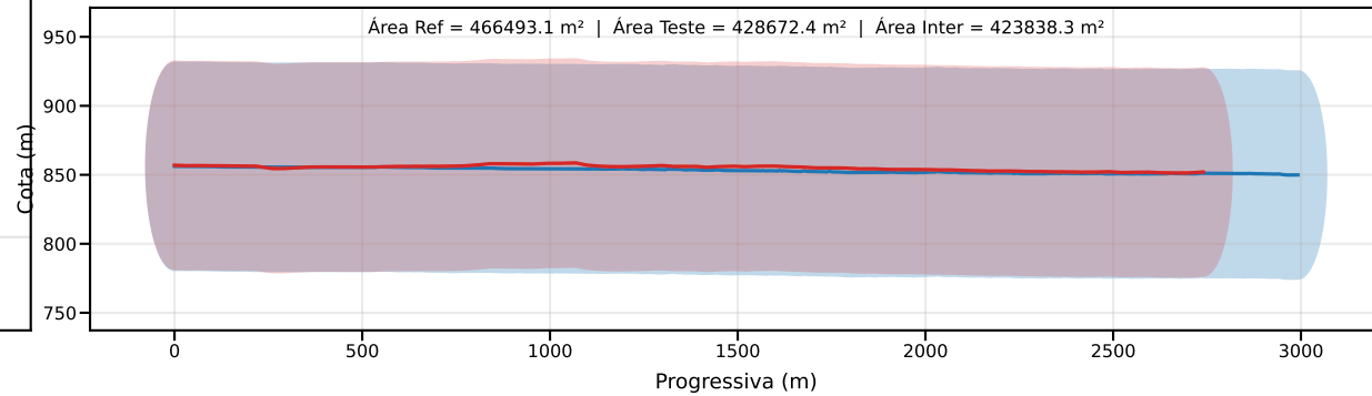
Classe D | PEC-PCD (Vertical)=75.0 m | EQ = 100m | dm = 23.45
