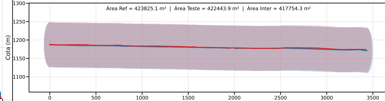
Classe D | PEC-PCD (Vertical)=75.0 m | EQ = 100m | dm = 2.85
