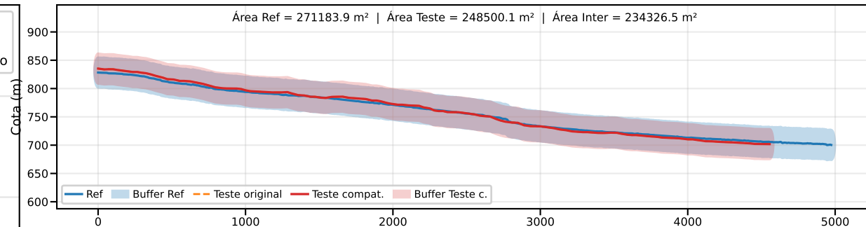
Classe B | PEC-PCD (Vertical)=50.0 m | EQ = 100m | dm = 19.07
