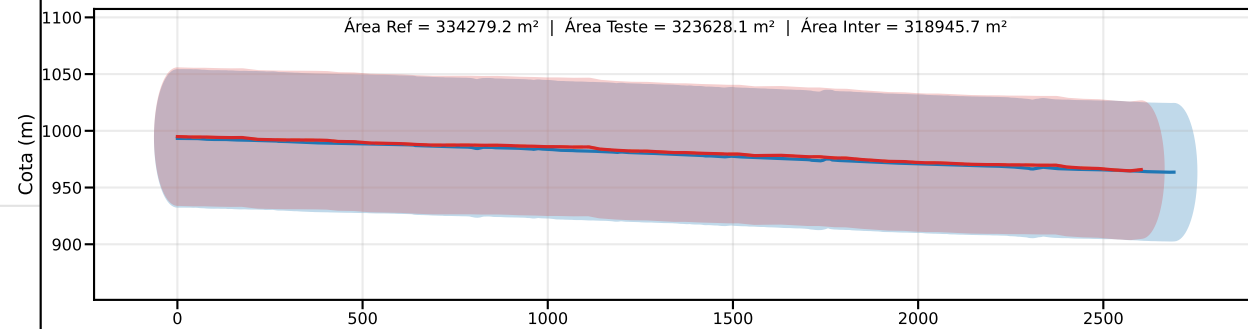
Classe D | PEC-PCD (Vertical)=75.0 m | EQ = 100m | dm = 10.40
