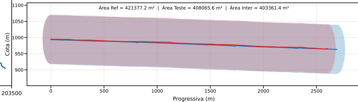
Classe D | PEC-PCD (Vertical)=75.0 m | EQ = 100m | dm = 10.40
