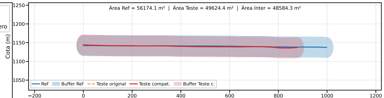
Classe B | PEC-PCD (Vertical)=50.0 m | EQ = 100m | dm = 21.73
