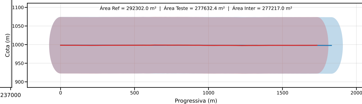
Classe D | PEC-PCD (Vertical)=75.0 m | EQ = 100m | dm = 12.80
