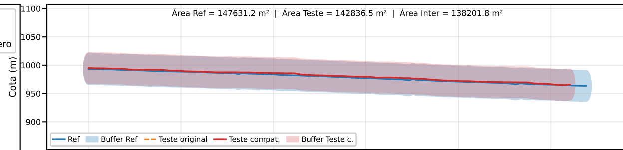
Classe B | PEC-PCD (Vertical)=50.0 m | EQ = 100m | dm = 7.94
