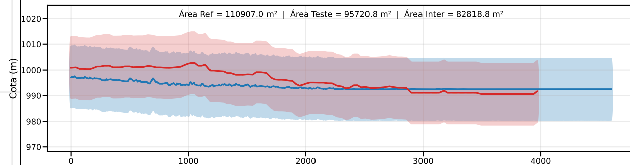
Classe D | PEC-PCD (Vertical)=15.0 m | EQ = 20m | dm = 12.55
