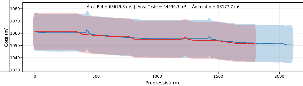
Classe D | PEC-PCD (Vertical)=15.0 m | EQ = 20m | dm = 9.07
