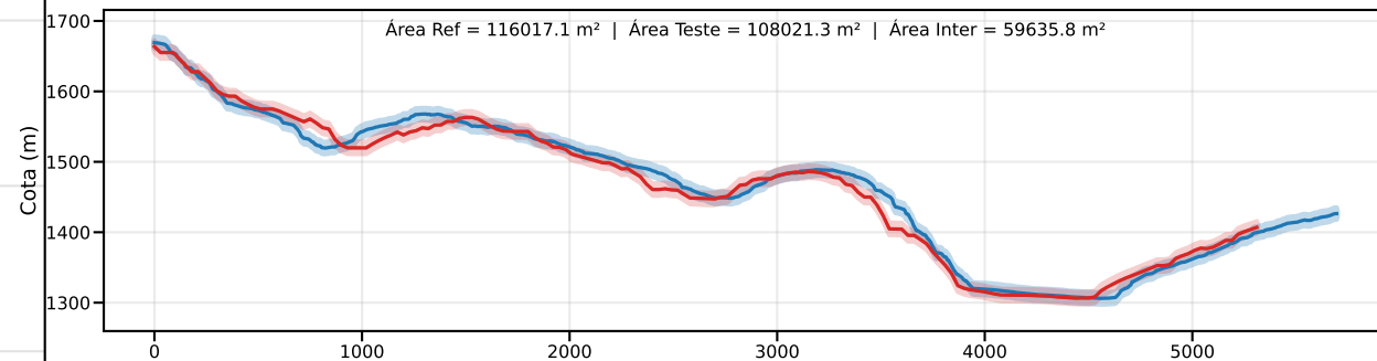
Classe C | PEC-PCD (Vertical)=12.0 m | EQ = 20m | dm = 17.43
