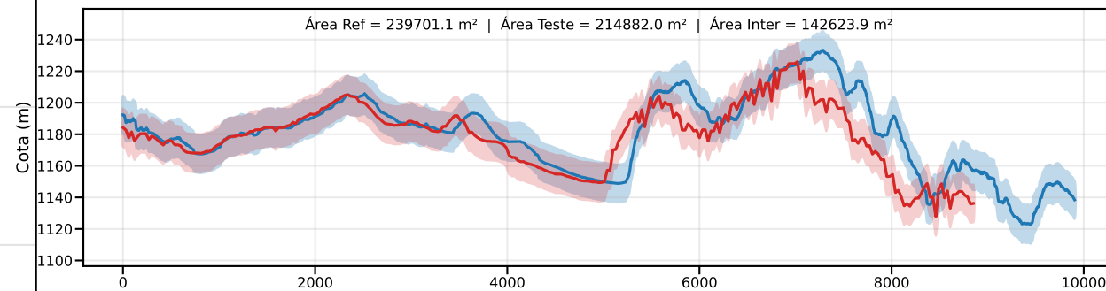
Classe D | PEC-PCD (Vertical)=15.0 m | EQ = 20m | dm = 18.98
