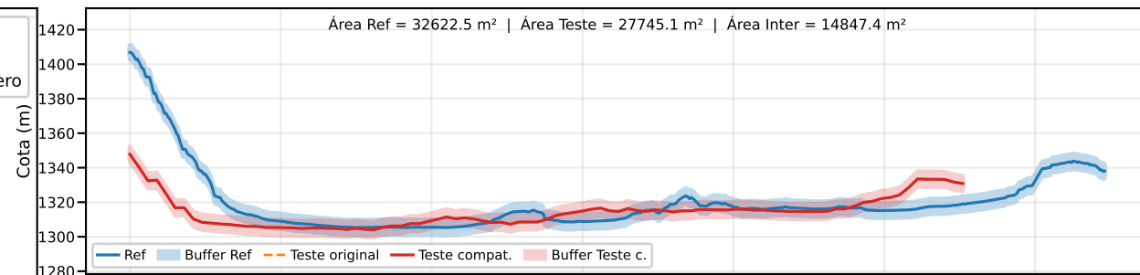
Classe B | PEC-PCD (Vertical)=10.0 m | EQ = 20m | dm = 15.10
