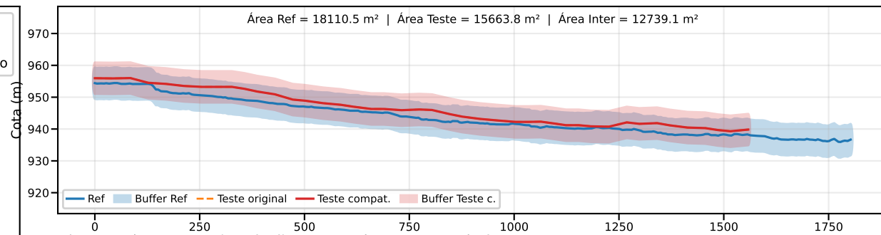
Classe B | PEC-PCD (Vertical)=10.0 m | EQ = 20m | dm = 7.81
