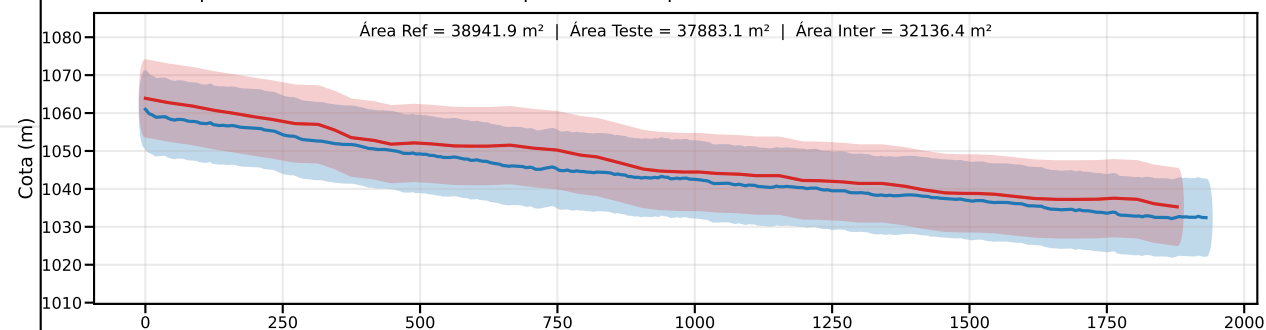
Classe C | PEC-PCD (Vertical)=12.0 m | EQ = 20m | dm = 5.81
