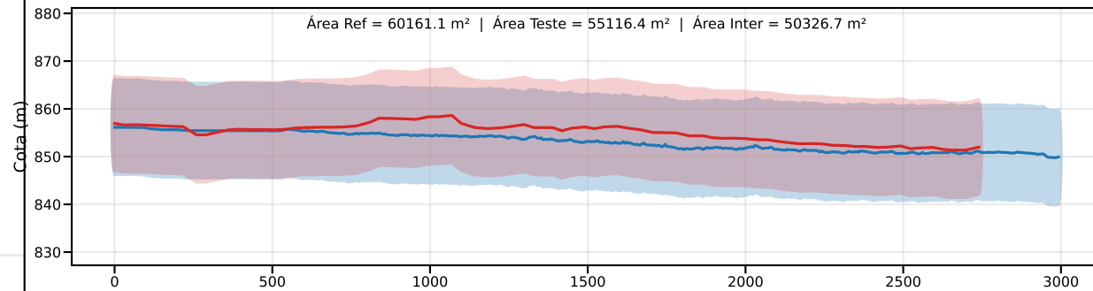
Classe C | PEC-PCD (Vertical)=12.0 m | EQ = 20m | dm = 6.17
