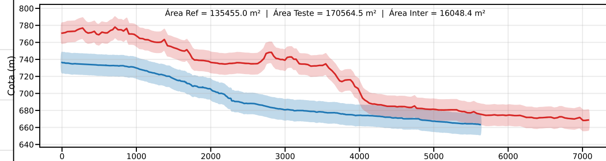
Classe D | PEC-PCD (Vertical)=15.0 m | EQ = 20m | dm = 31.72
