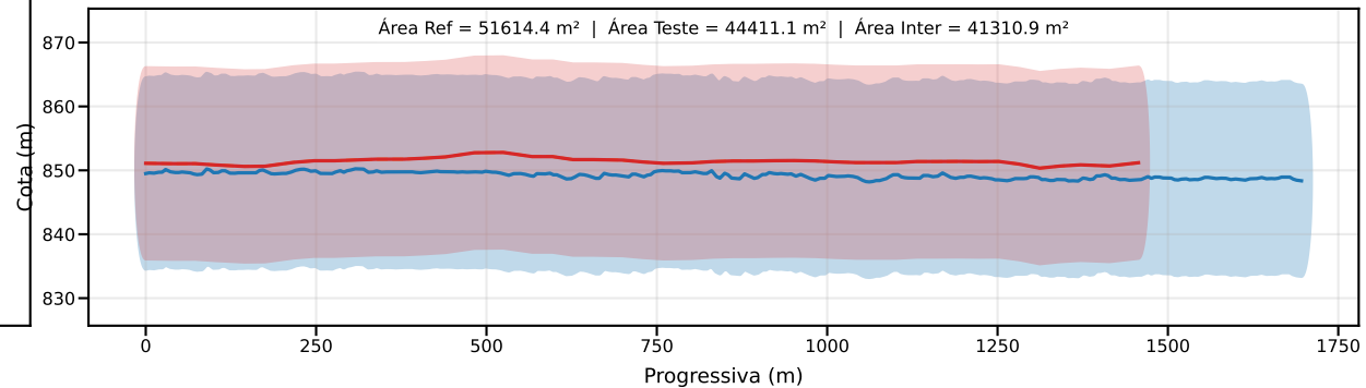
Classe D | PEC-PCD (Vertical)=15.0 m | EQ = 20m | dm = 10.93
