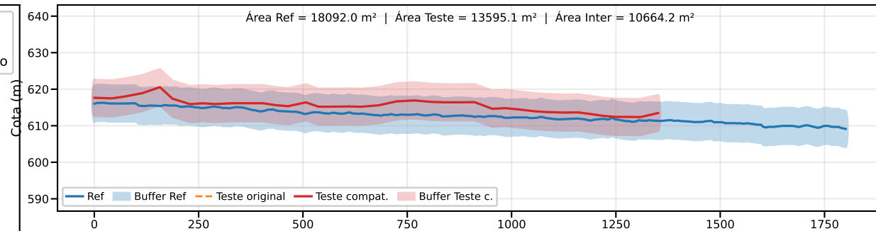
Classe B | PEC-PCD (Vertical)=10.0 m | EQ = 20m | dm = 13.71
