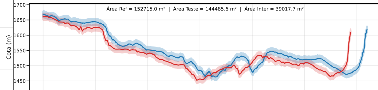
Classe D | PEC-PCD (Vertical)=15.0 m | EQ = 20m | dm = 32.44
