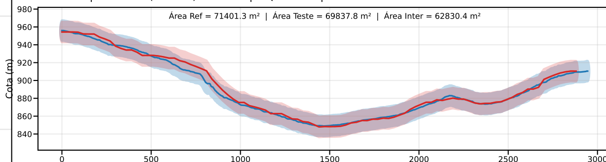
Classe D | PEC-PCD (Vertical)=15.0 m | EQ = 20m | dm = 4.83
