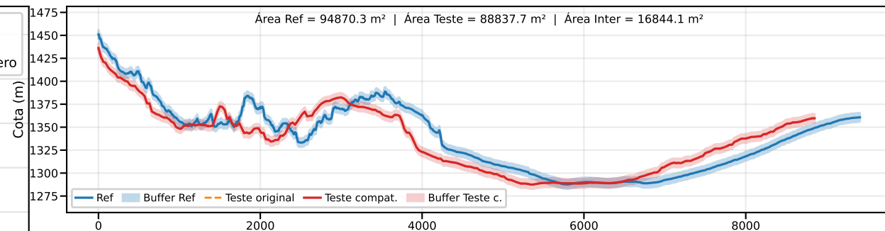
Classe B | PEC-PCD (Vertical)=10.0 m | EQ = 20m | dm = 21.14
