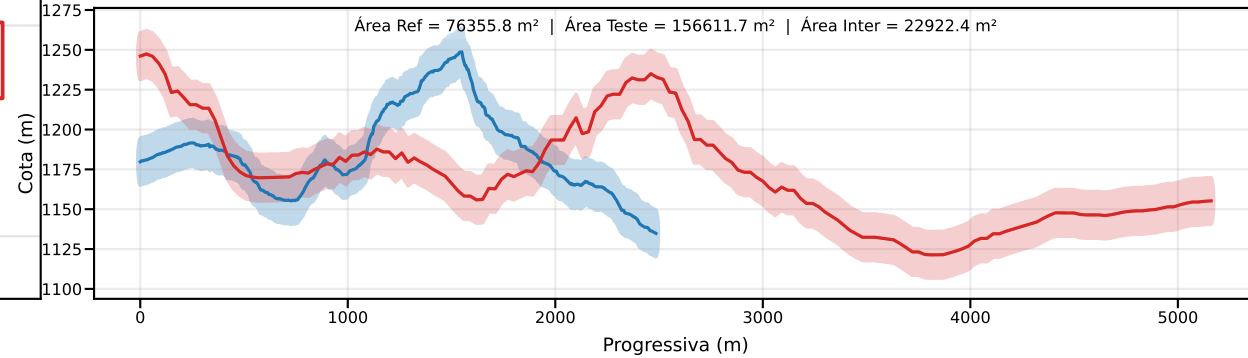
Classe D | PEC-PCD (Vertical)=15.0 m | EQ = 20m | dm = 16.08
