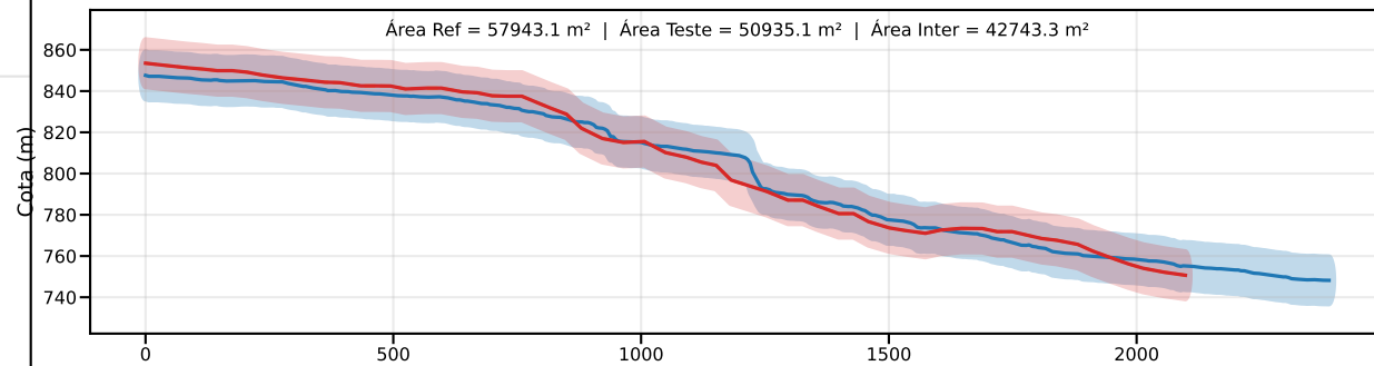
Classe D | PEC-PCD (Vertical)=15.0 m | EQ = 20m | dm = 12.53
