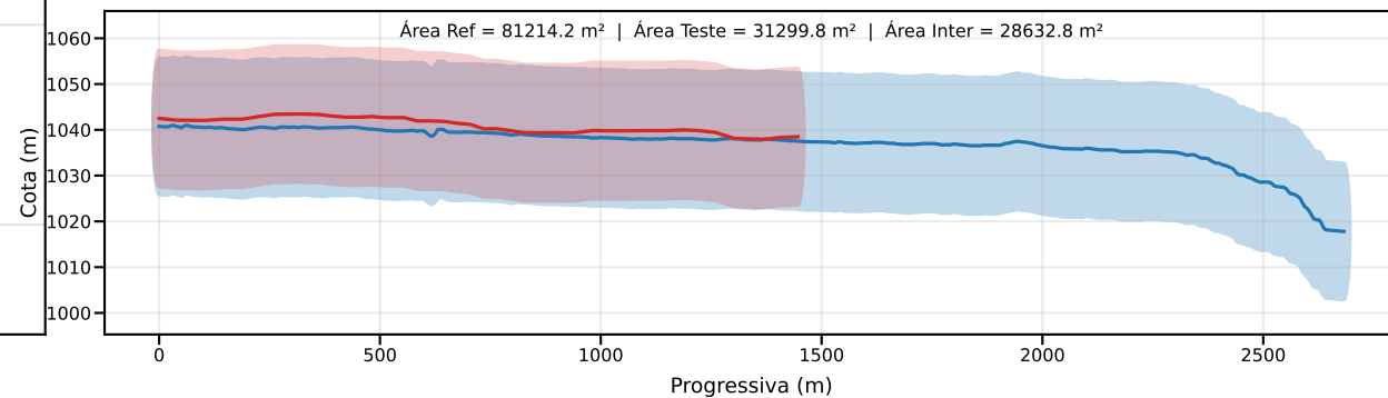
Classe D | PEC-PCD (Vertical)=15.0 m | EQ = 20m | dm = 79.16
