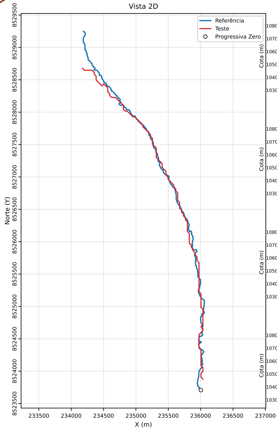
Classe A | PEC-PCD (Vertical)=5.0 m | EQ = 20m | dm = 6.11
