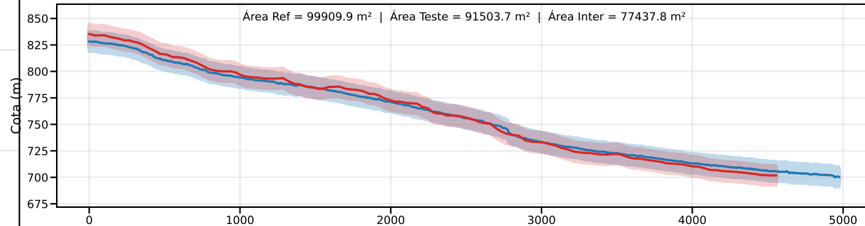
Classe C | PEC-PCD (Vertical)=12.0 m | EQ = 20m | dm = 8.29
