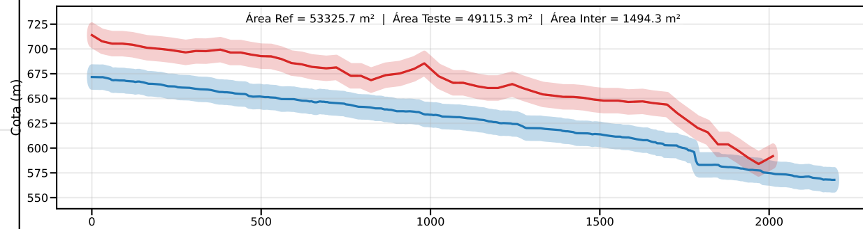
Classe D | PEC-PCD (Vertical)=15.0 m | EQ = 20m | dm = 48.98
