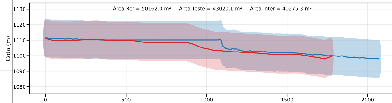
Classe D | PEC-PCD (Vertical)=15.0 m | EQ = 20m | dm = 10.20
