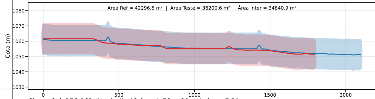
Classe C | PEC-PCD (Vertical)=12.0 m | EQ = 20m | dm = 7.51
