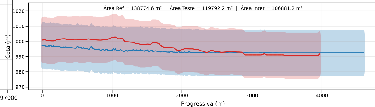
Classe D | PEC-PCD (Vertical)=15.0 m | EQ = 20m | dm = 12.55
