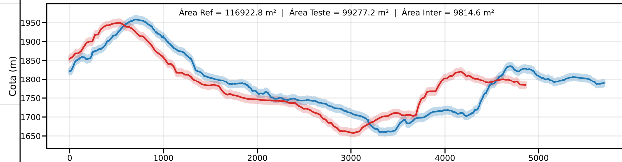
Classe C | PEC-PCD (Vertical)=12.0 m | EQ = 20m | dm = 39.53
