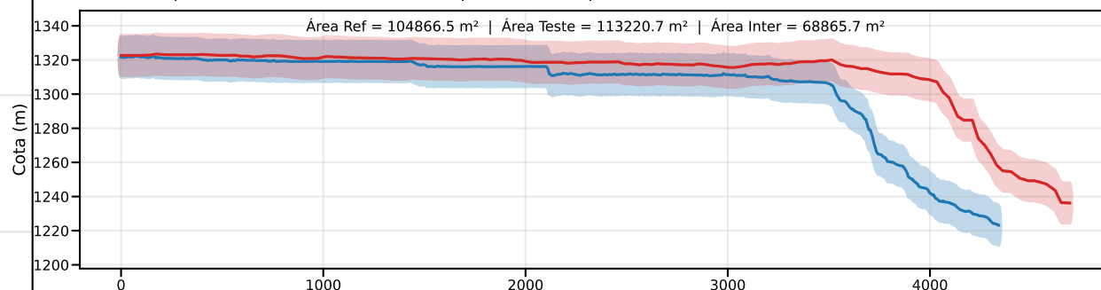
Classe D | PEC-PCD (Vertical)=15.0 m | EQ = 20m | dm = 13.41
