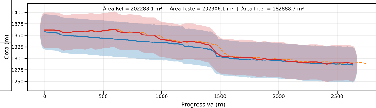
Classe D | PEC-PCD (Vertical)=37.5 m | EQ = 50m | dm = 11.30
