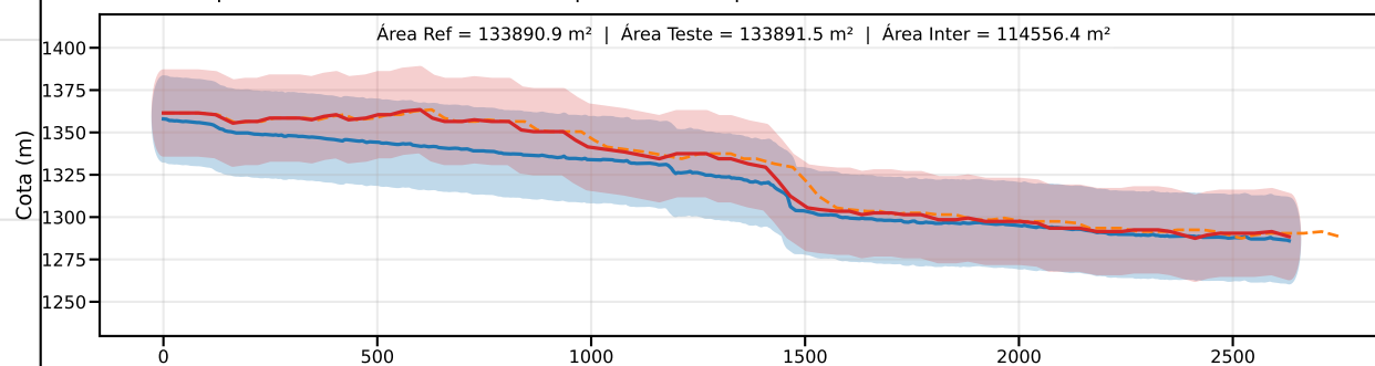
Classe C | PEC-PCD (Vertical)=30.0 m | EQ = 50m | dm = 11.32
