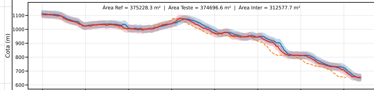
Classe C | PEC-PCD (Vertical)=30.0 m | EQ = 50m | dm = 13.14
