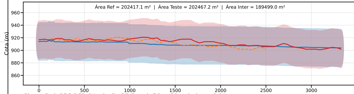
Classe D | PEC-PCD (Vertical)=37.5 m | EQ = 50m | dm = 6.01
