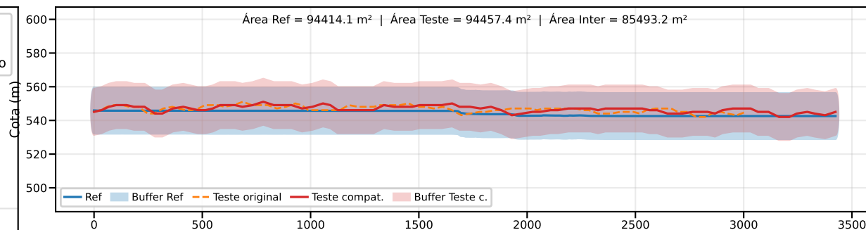
Classe B | PEC-PCD (Vertical)=25.0 m | EQ = 50m | dm = 4.05
