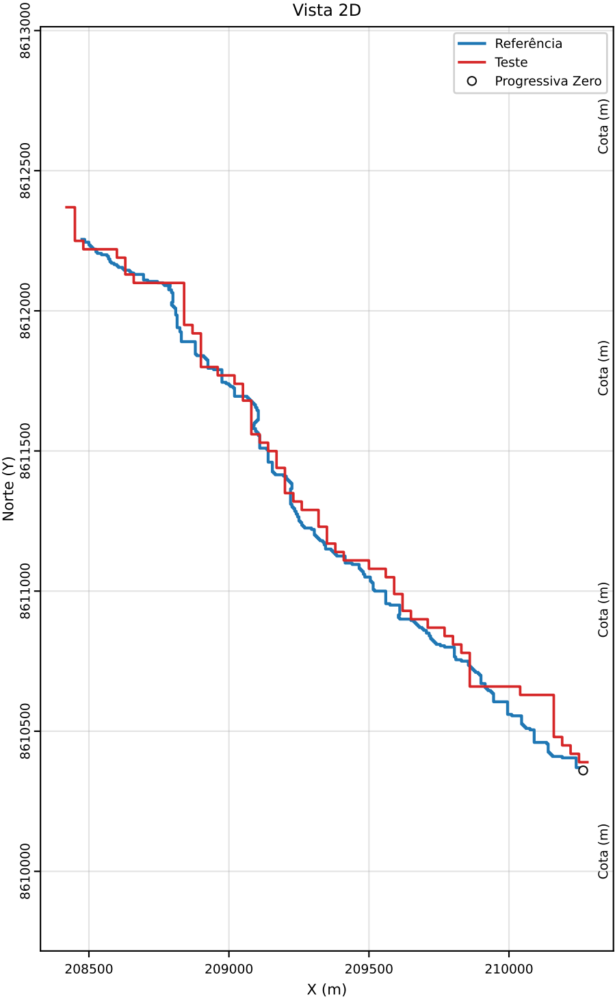
Classe A | PEC-PCD (Vertical)=13.7 m | EQ = 50m | dm = 6.83
