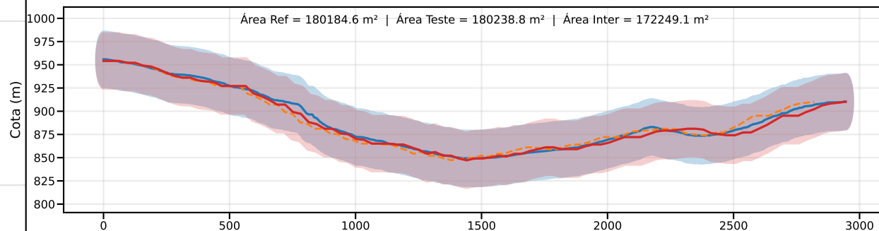
Classe D | PEC-PCD (Vertical)=37.5 m | EQ = 50m | dm = 4.14
