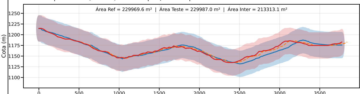
Classe D | PEC-PCD (Vertical)=37.5 m | EQ = 50m | dm = 6.82
