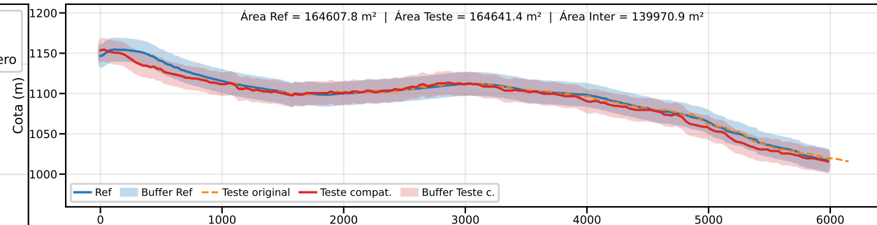
Classe B | PEC-PCD (Vertical)=25.0 m | EQ = 50m | dm = 6.44
