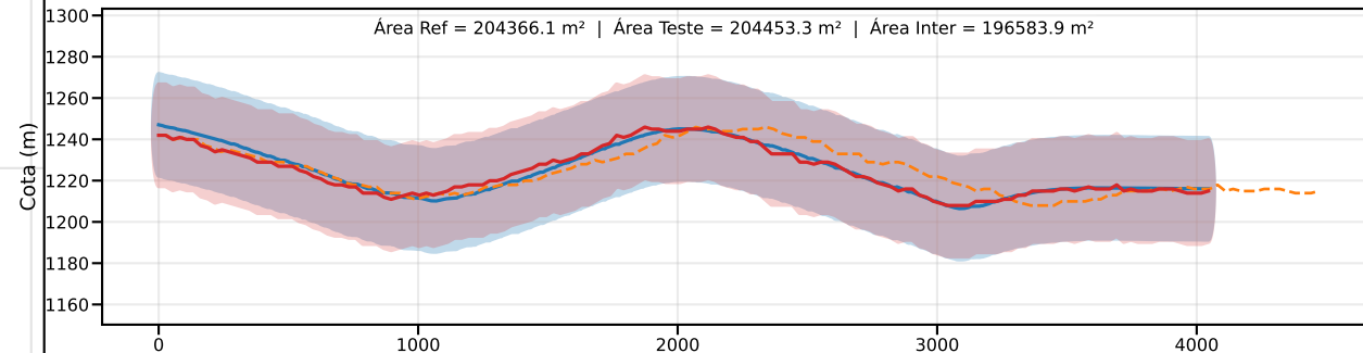
Classe C | PEC-PCD (Vertical)=30.0 m | EQ = 50m | dm = 2.99
