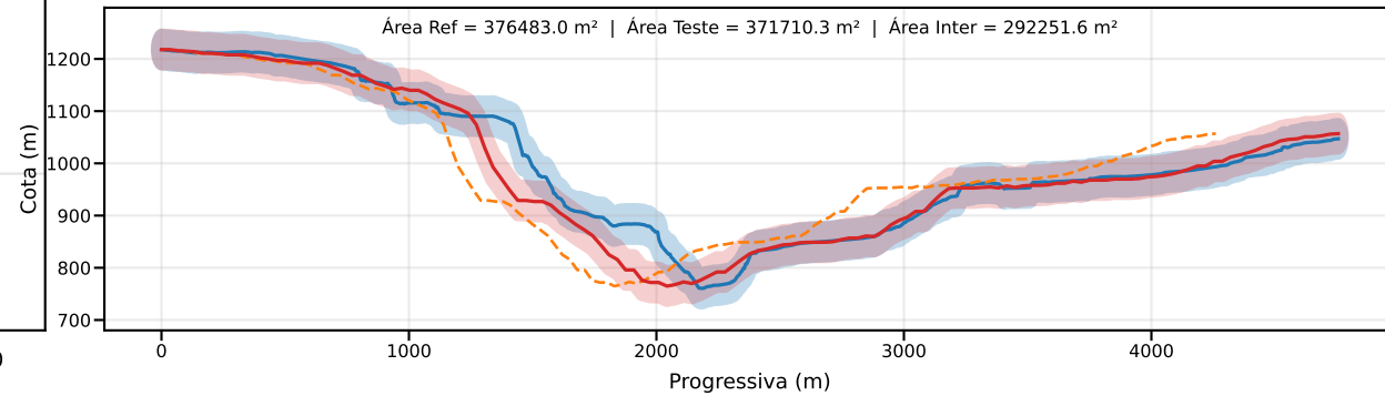
Classe D | PEC-PCD (Vertical)=37.5 m | EQ = 50m | dm = 26.70
