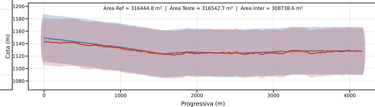
Classe D | PEC-PCD (Vertical)=37.5 m | EQ = 50m | dm = 2.87
