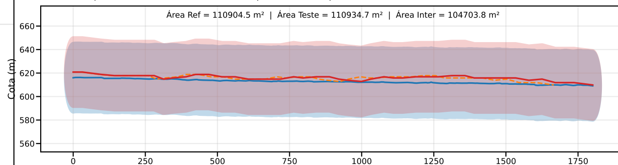
Classe D | PEC-PCD (Vertical)=37.5 m | EQ = 50m | dm = 5.27
