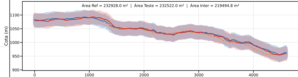
Classe C | PEC-PCD (Vertical)=30.0 m | EQ = 50m | dm = 4.55
