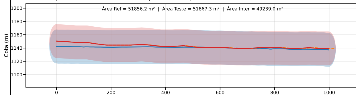
Classe C | PEC-PCD (Vertical)=30.0 m | EQ = 50m | dm = 4.01
