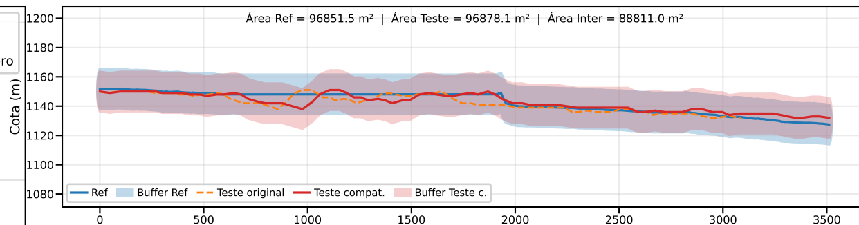
Classe B | PEC-PCD (Vertical)=25.0 m | EQ = 50m | dm = 3.58
