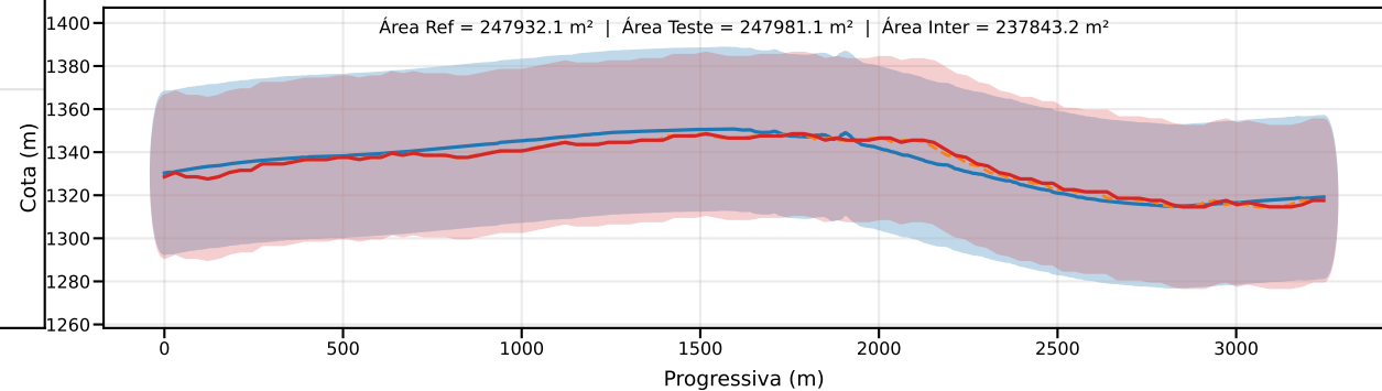
Classe D | PEC-PCD (Vertical)=37.5 m | EQ = 50m | dm = 4.79
