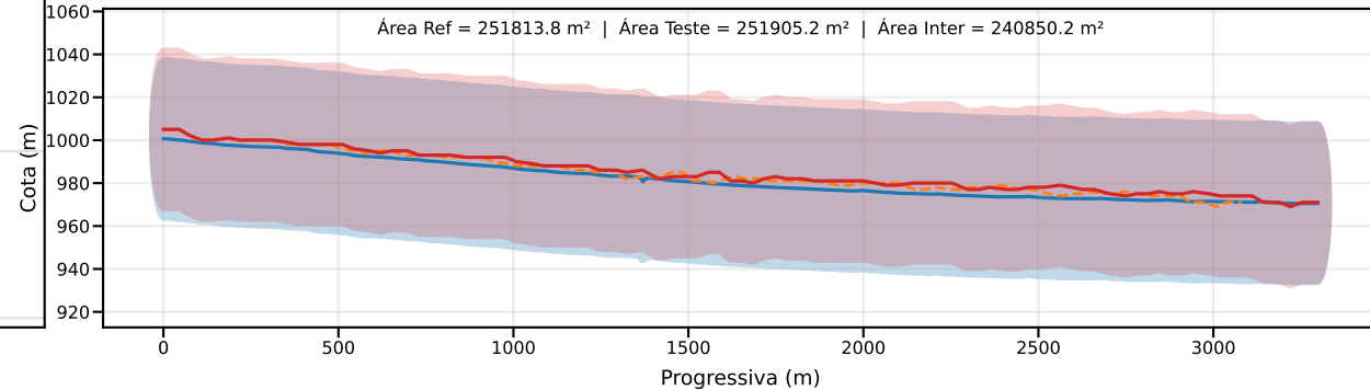
Classe D | PEC-PCD (Vertical)=37.5 m | EQ = 50m | dm = 5.13
