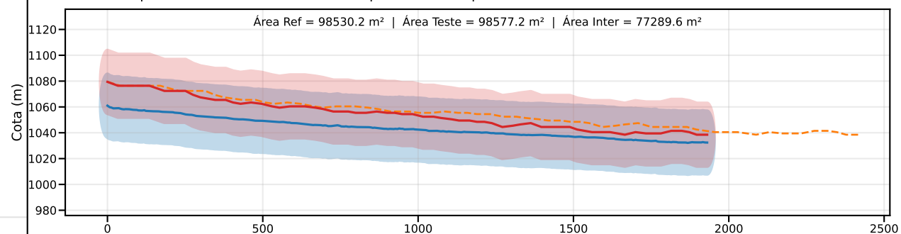
Classe C | PEC-PCD (Vertical)=30.0 m | EQ = 50m | dm = 16.95
