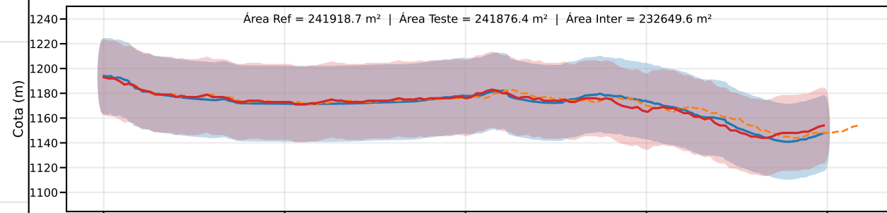
Classe D | PEC-PCD (Vertical)=37.5 m | EQ = 50m | dm = 3.62
