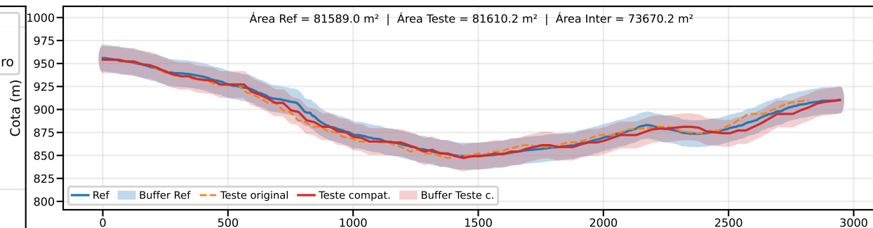
Classe B | PEC-PCD (Vertical)=25.0 m | EQ = 50m | dm = 4.16
