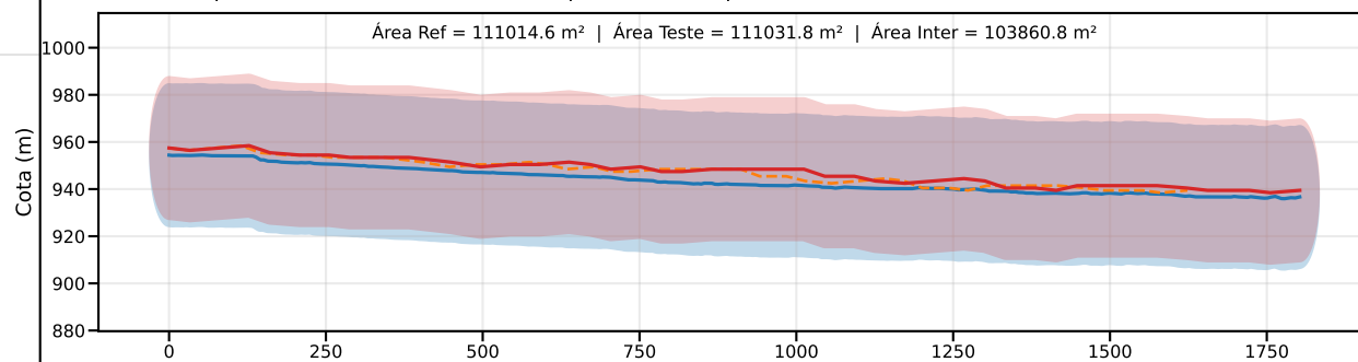
Classe D | PEC-PCD (Vertical)=37.5 m | EQ = 50m | dm = 6.07
