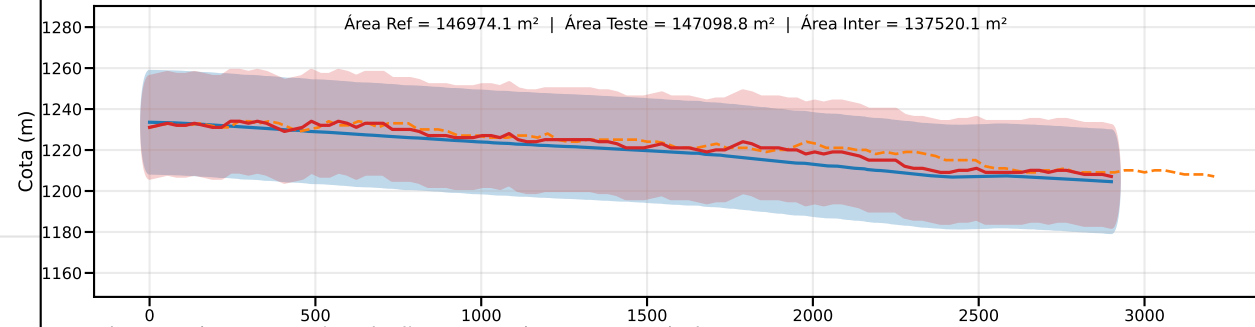
Classe C | PEC-PCD (Vertical)=30.0 m | EQ = 50m | dm = 5.04
