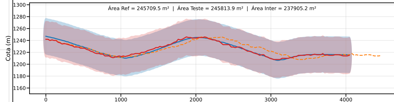
Classe D | PEC-PCD (Vertical)=37.5 m | EQ = 50m | dm = 3.00
