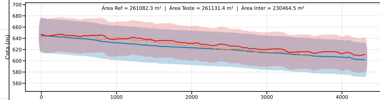
Classe D | PEC-PCD (Vertical)=37.5 m | EQ = 50m | dm = 11.05
