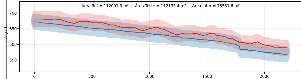
Classe C | PEC-PCD (Vertical)=30.0 m | EQ = 50m | dm = 25.62
