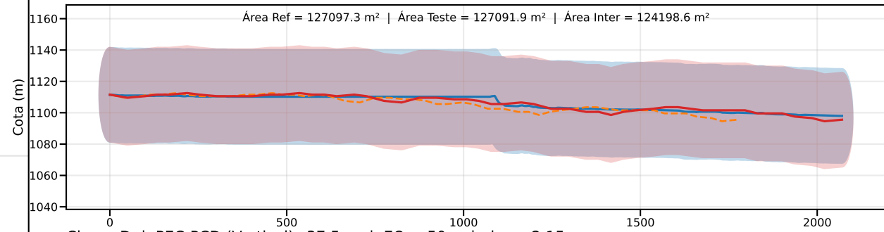
Classe D | PEC-PCD (Vertical)=37.5 m | EQ = 50m | dm = 2.15
