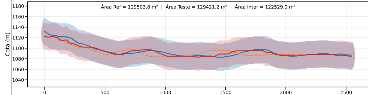
Classe C | PEC-PCD (Vertical)=30.0 m | EQ = 50m | dm = 4.26
