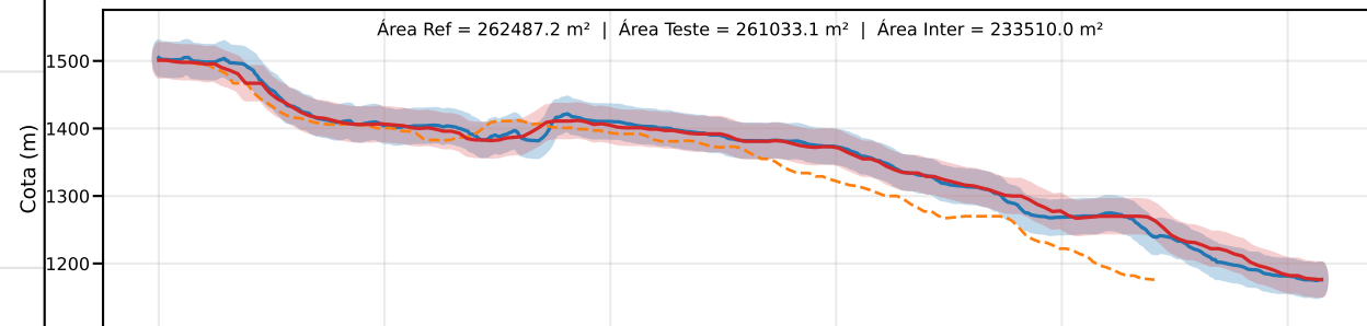
Classe C | PEC-PCD (Vertical)=30.0 m | EQ = 50m | dm = 8.75
