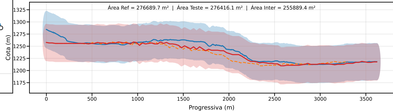
Classe D | PEC-PCD (Vertical)=37.5 m | EQ = 50m | dm = 8.87
