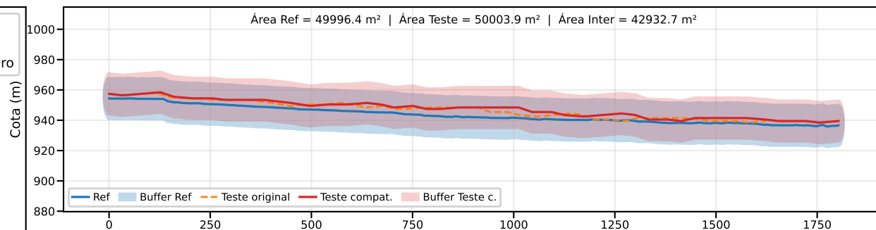
Classe B | PEC-PCD (Vertical)=25.0 m | EQ = 50m | dm = 6.07
