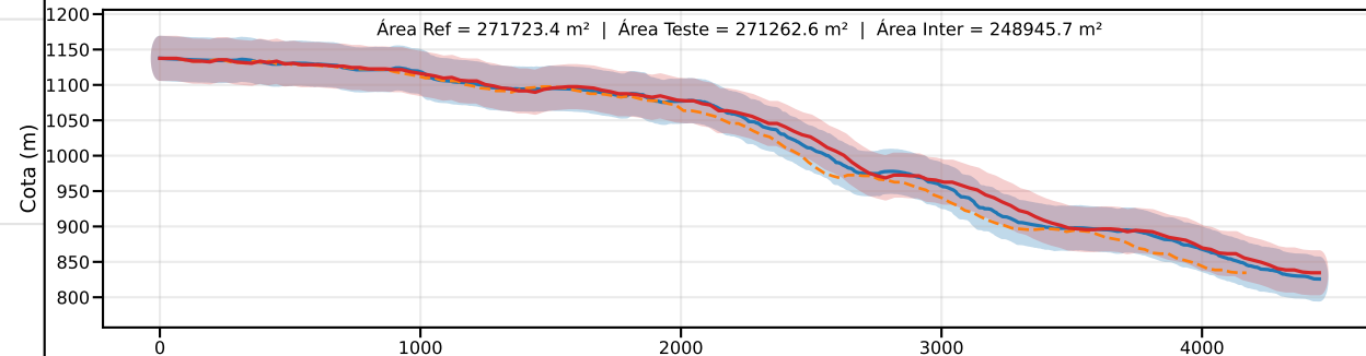
Classe D | PEC-PCD (Vertical)=37.5 m | EQ = 50m | dm = 7.93
