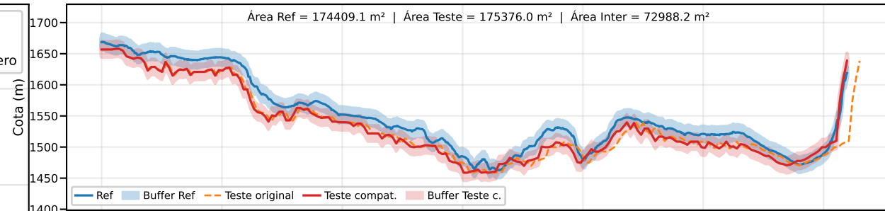
Classe B | PEC-PCD (Vertical)=25.0 m | EQ = 50m | dm = 25.16
