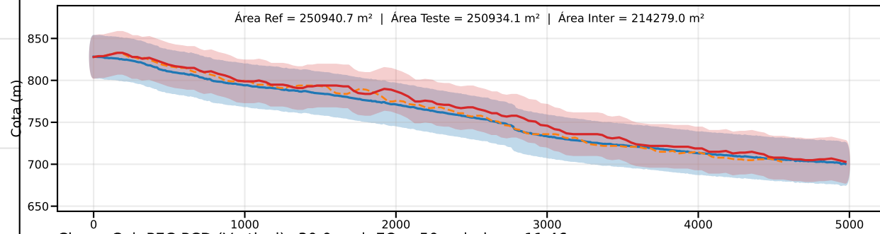
Classe C | PEC-PCD (Vertical)=30.0 m | EQ = 50m | dm = 11.46
