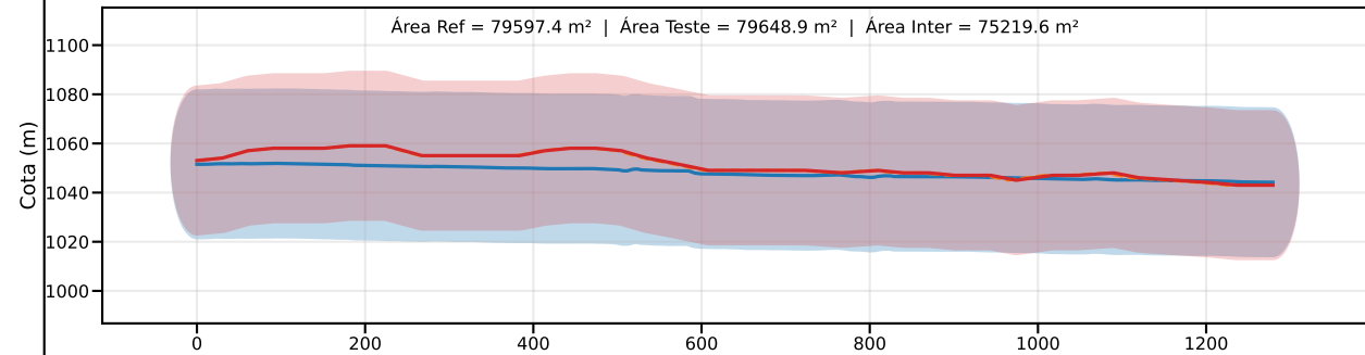
Classe D | PEC-PCD (Vertical)=37.5 m | EQ = 50m | dm = 5.15
