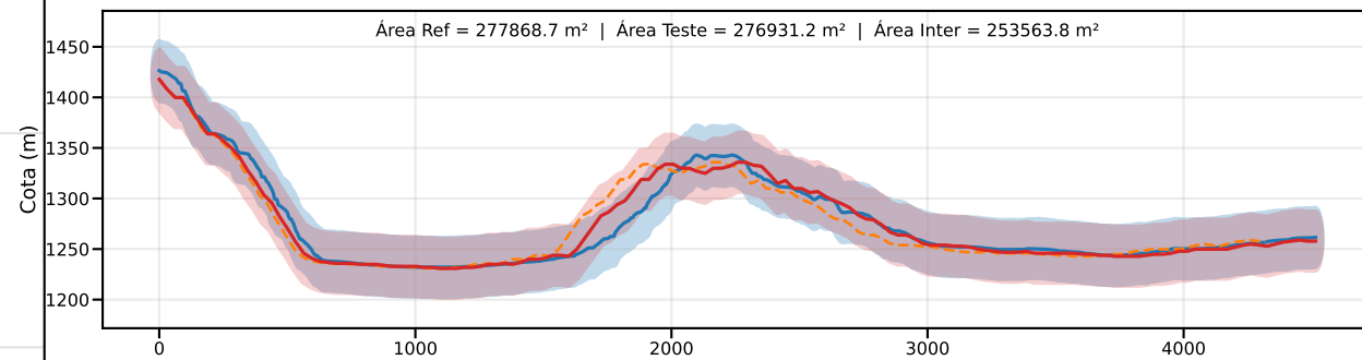
Classe D | PEC-PCD (Vertical)=37.5 m | EQ = 50m | dm = 8.31
