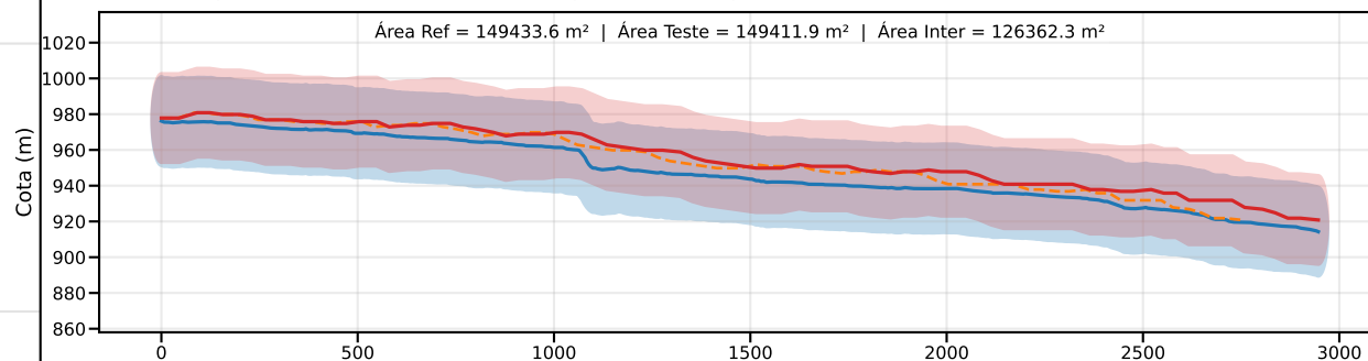
Classe C | PEC-PCD (Vertical)=30.0 m | EQ = 50m | dm = 12.12
