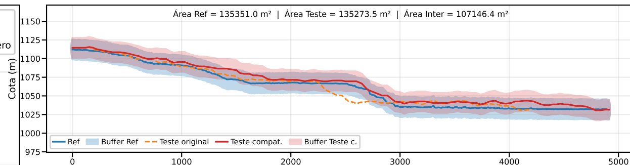
Classe B | PEC-PCD (Vertical)=25.0 m | EQ = 50m | dm = 8.96
