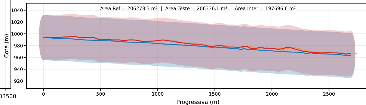
Classe D | PEC-PCD (Vertical)=37.5 m | EQ = 50m | dm = 4.90
