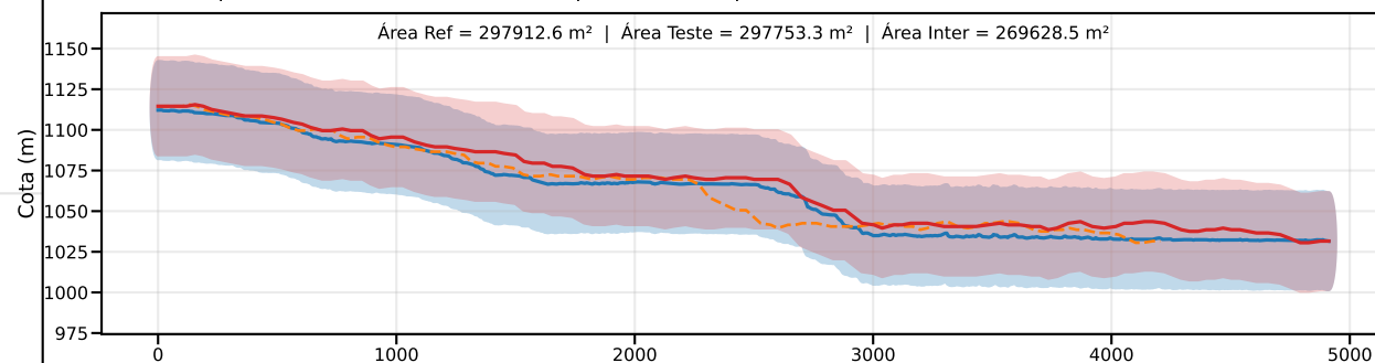
Classe D | PEC-PCD (Vertical)=37.5 m | EQ = 50m | dm = 8.94
