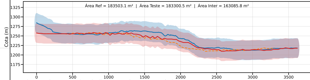
Classe C | PEC-PCD (Vertical)=30.0 m | EQ = 50m | dm = 8.80
