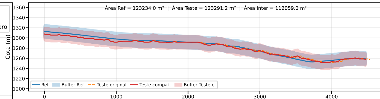
Classe B | PEC-PCD (Vertical)=25.0 m | EQ = 50m | dm = 3.91
