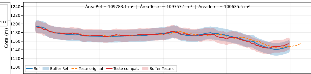
Classe B | PEC-PCD (Vertical)=25.0 m | EQ = 50m | dm = 3.60
