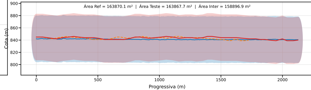
Classe D | PEC-PCD (Vertical)=37.5 m | EQ = 50m | dm = 3.58
