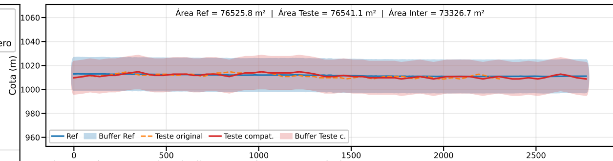
Classe B | PEC-PCD (Vertical)=25.0 m | EQ = 50m | dm = 1.82
