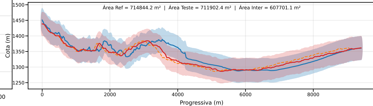
Classe D | PEC-PCD (Vertical)=37.5 m | EQ = 50m | dm = 17.73
