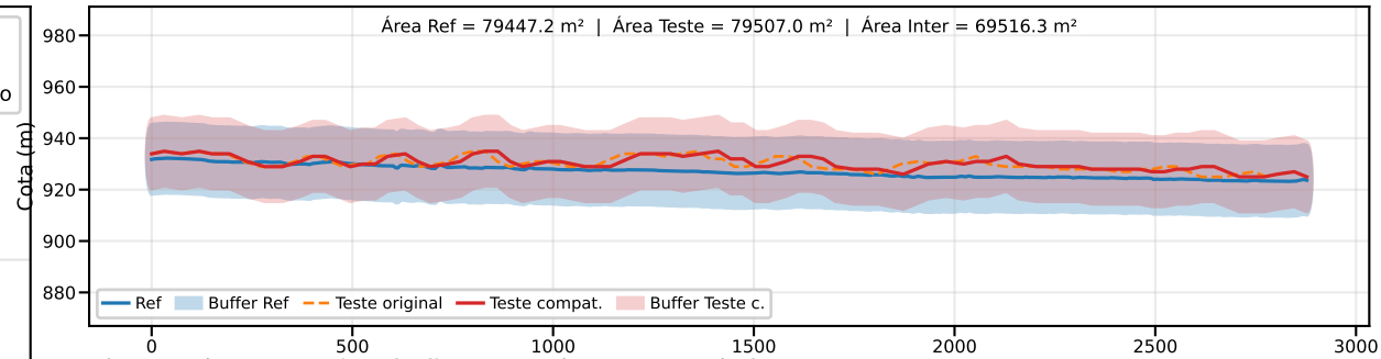
Classe B | PEC-PCD (Vertical)=25.0 m | EQ = 50m | dm = 5.35
