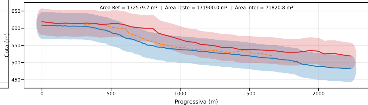
Classe D | PEC-PCD (Vertical)=37.5 m | EQ = 50m | dm = 69.05
