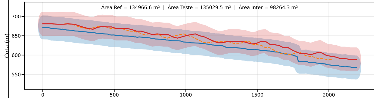
Classe D | PEC-PCD (Vertical)=37.5 m | EQ = 50m | dm = 25.63
