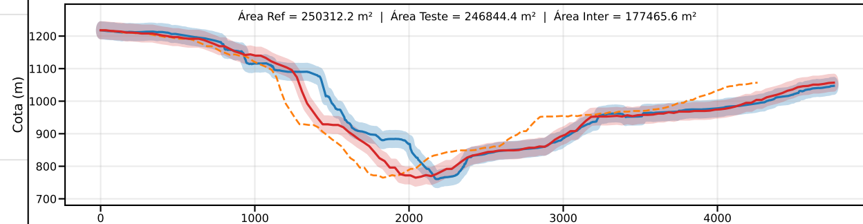
Classe C | PEC-PCD (Vertical)=30.0 m | EQ = 50m | dm = 24.83
