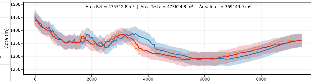
Classe C | PEC-PCD (Vertical)=30.0 m | EQ = 50m | dm = 17.70
