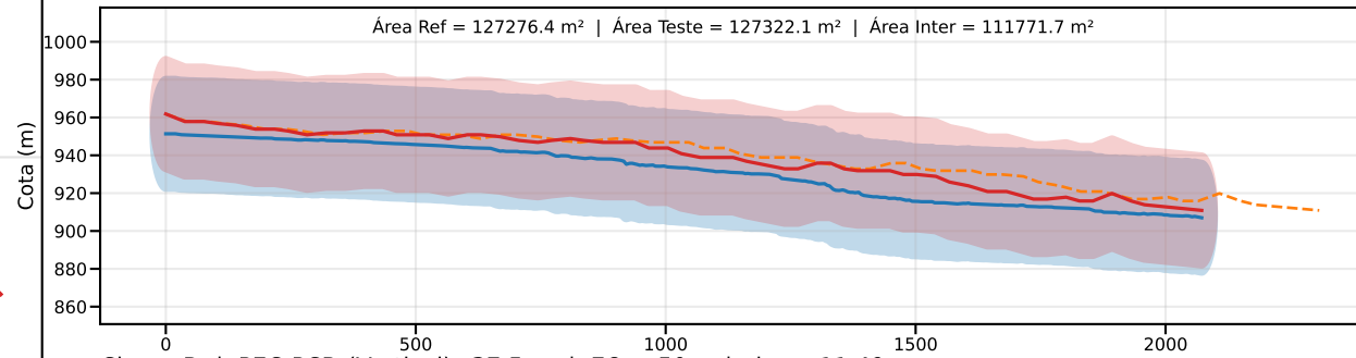
Classe D | PEC-PCD (Vertical)=37.5 m | EQ = 50m | dm = 11.49
