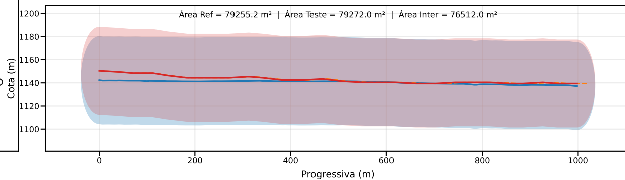
Classe D | PEC-PCD (Vertical)=37.5 m | EQ = 50m | dm = 4.08
