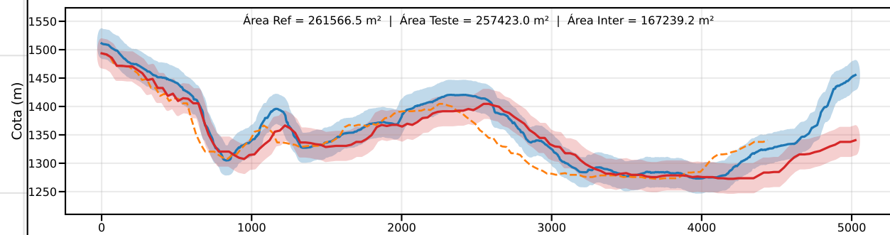
Classe C | PEC-PCD (Vertical)=30.0 m | EQ = 50m | dm = 29.75
