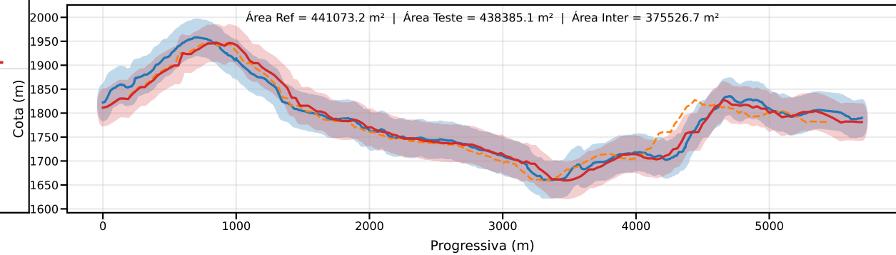
Classe D | PEC-PCD (Vertical)=37.5 m | EQ = 50m | dm = 17.61
