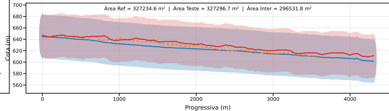
Classe D | PEC-PCD (Vertical)=37.5 m | EQ = 50m | dm = 11.05
