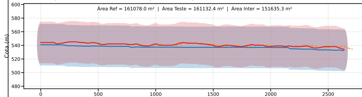
Classe D | PEC-PCD (Vertical)=37.5 m | EQ = 50m | dm = 5.52
