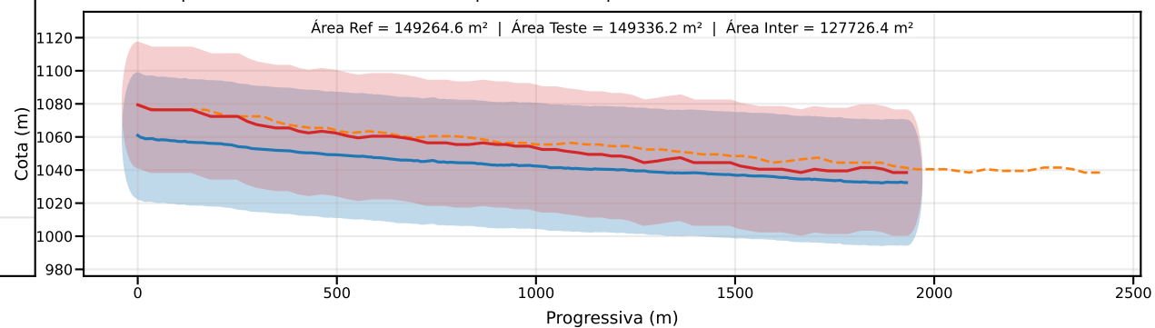
Classe D | PEC-PCD (Vertical)=37.5 m | EQ = 50m | dm = 16.99
