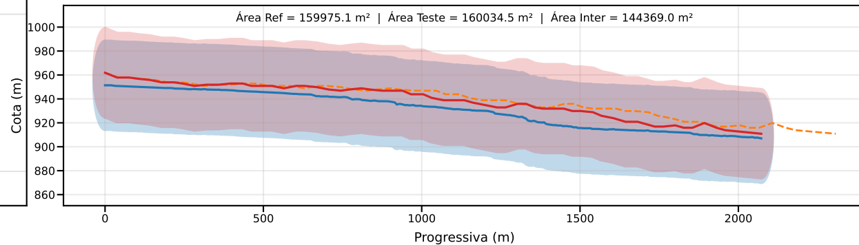
Classe D | PEC-PCD (Vertical)=37.5 m | EQ = 50m | dm = 11.49
