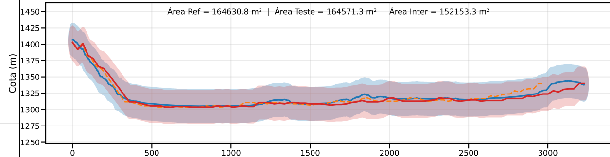
Classe C | PEC-PCD (Vertical)=30.0 m | EQ = 50m | dm = 5.95
