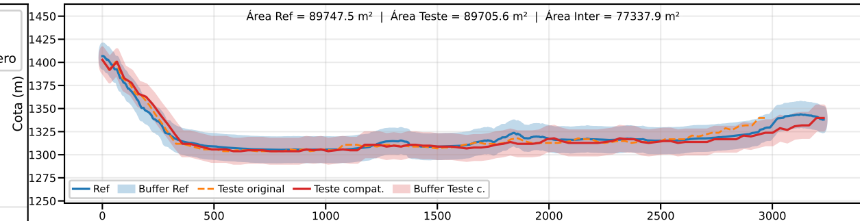
Classe B | PEC-PCD (Vertical)=25.0 m | EQ = 50m | dm = 5.95
