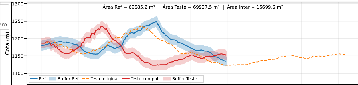
Classe B | PEC-PCD (Vertical)=25.0 m | EQ = 50m | dm = 48.61
