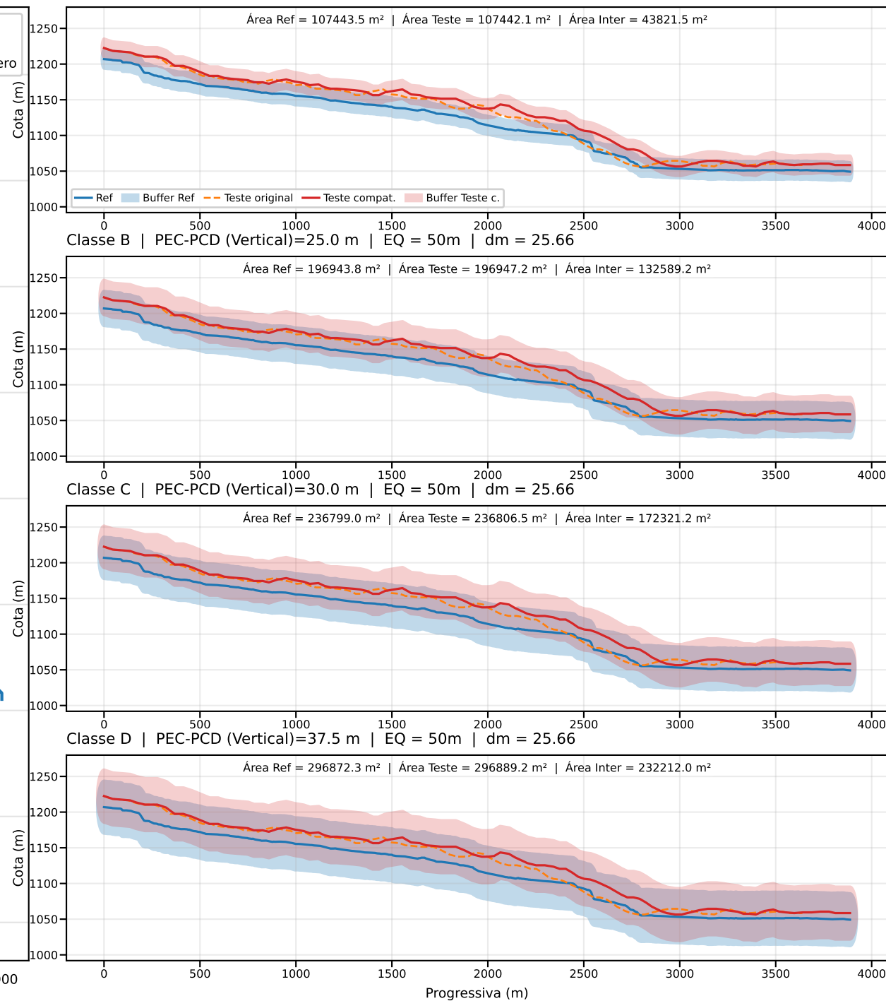
Classe A | PEC-PCD (Vertical)=13.7 m | EQ = 50m | dm = 25.49
