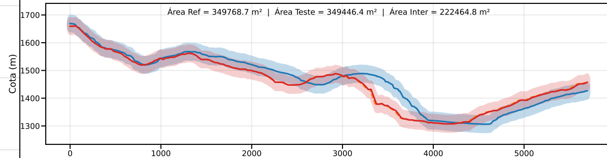
Classe D | PEC-PCD (Vertical)=37.5 m | EQ = 50m | dm = 35.93
