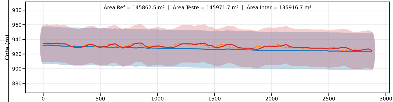
Classe C | PEC-PCD (Vertical)=30.0 m | EQ = 50m | dm = 5.34
