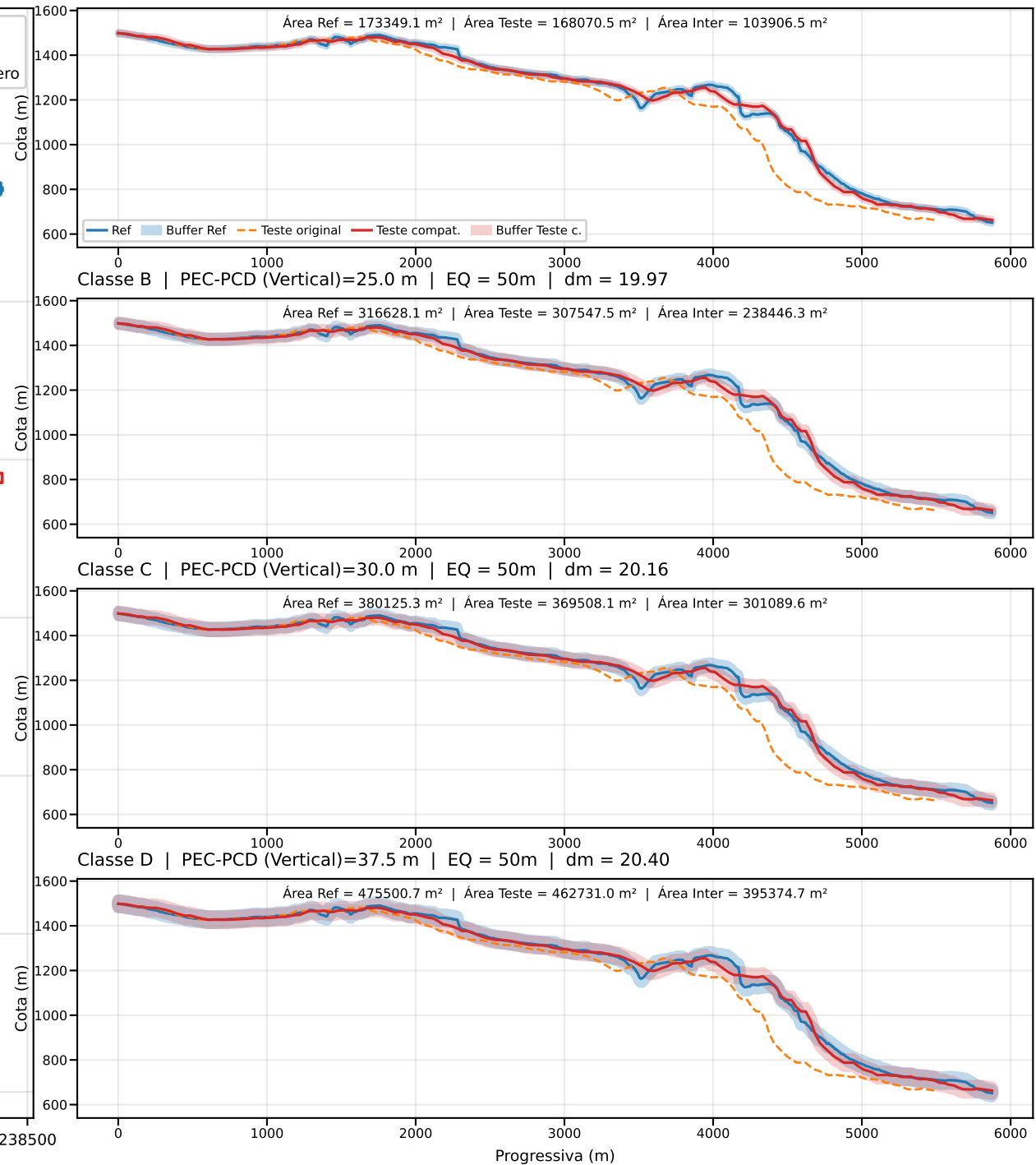
Classe A | PEC-PCD (Vertical)=13.7 m | EQ = 50m | dm = 17.78
