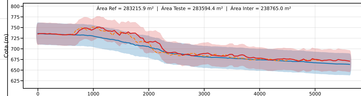
Classe C | PEC-PCD (Vertical)=30.0 m | EQ = 50m | dm = 12.30
