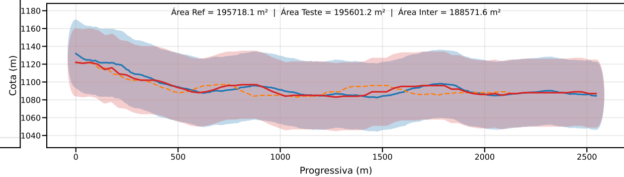
Classe D | PEC-PCD (Vertical)=37.5 m | EQ = 50m | dm = 4.30
