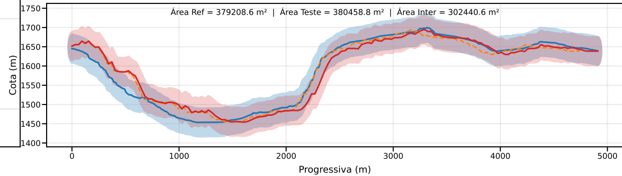
Classe D | PEC-PCD (Vertical)=37.5 m | EQ = 50m | dm = 23.77
