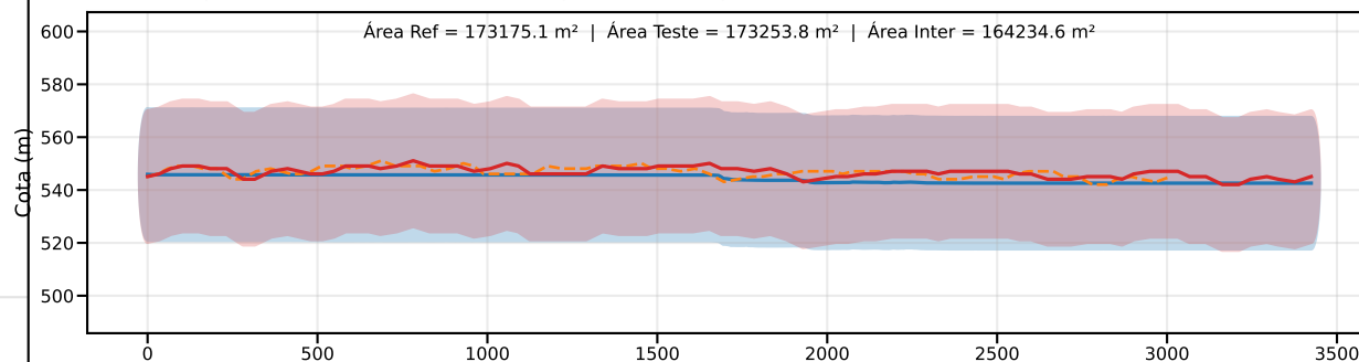
Classe C | PEC-PCD (Vertical)=30.0 m | EQ = 50m | dm = 4.05
