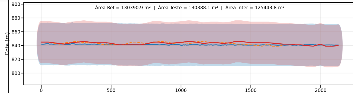
Classe D | PEC-PCD (Vertical)=37.5 m | EQ = 50m | dm = 3.58
