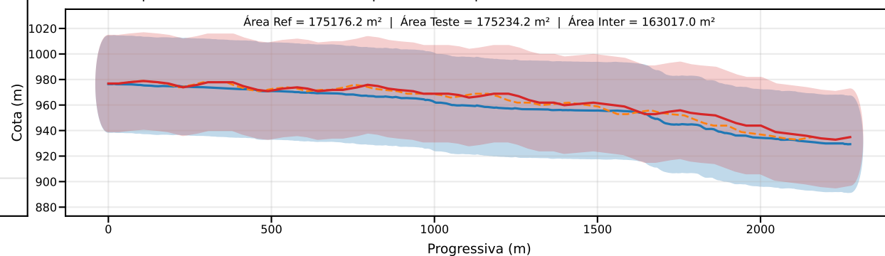
Classe D | PEC-PCD (Vertical)=37.5 m | EQ = 50m | dm = 8.17
