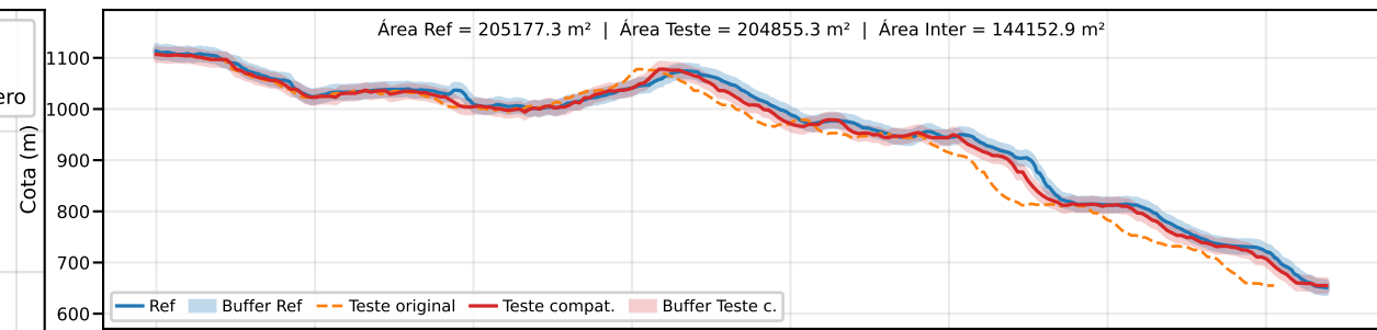
Classe B | PEC-PCD (Vertical)=25.0 m | EQ = 50m | dm = 13.13
