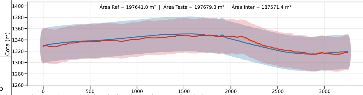
Classe D | PEC-PCD (Vertical)=37.5 m | EQ = 50m | dm = 4.79
