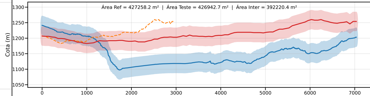
Classe D | PEC-PCD (Vertical)=37.5 m | EQ = 50m | dm = 7.74
