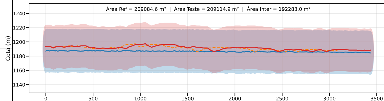
Classe D | PEC-PCD (Vertical)=37.5 m | EQ = 50m | dm = 7.58
