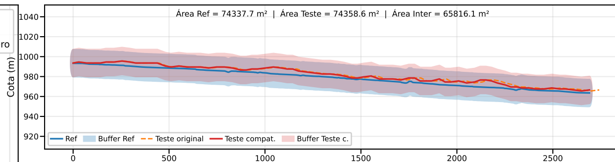
Classe B | PEC-PCD (Vertical)=25.0 m | EQ = 50m | dm = 4.92
