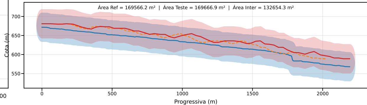
Classe D | PEC-PCD (Vertical)=37.5 m | EQ = 50m | dm = 25.63
