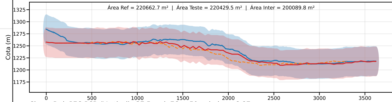
Classe D | PEC-PCD (Vertical)=37.5 m | EQ = 50m | dm = 8.87
