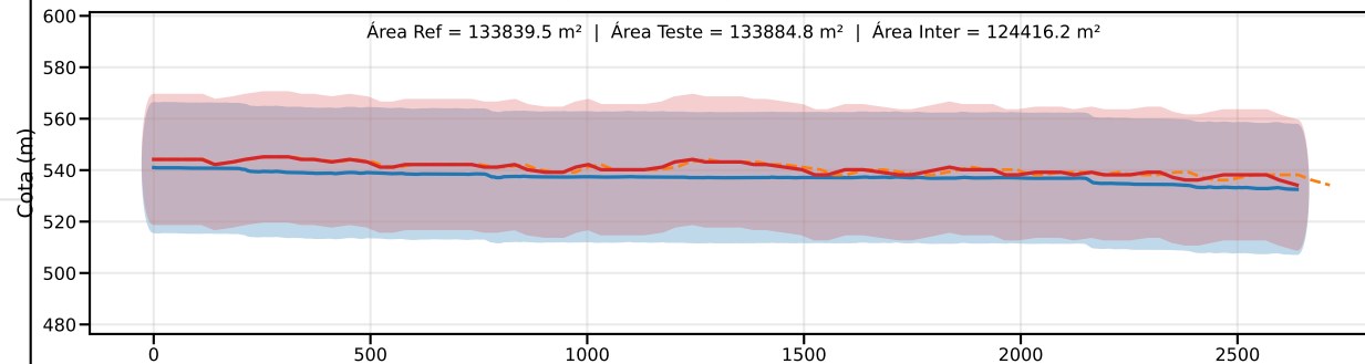
Classe C | PEC-PCD (Vertical)=30.0 m | EQ = 50m | dm = 5.52
