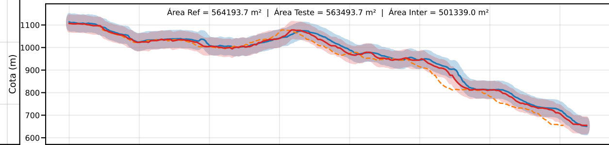
Classe D | PEC-PCD (Vertical)=37.5 m | EQ = 50m | dm = 13.14
