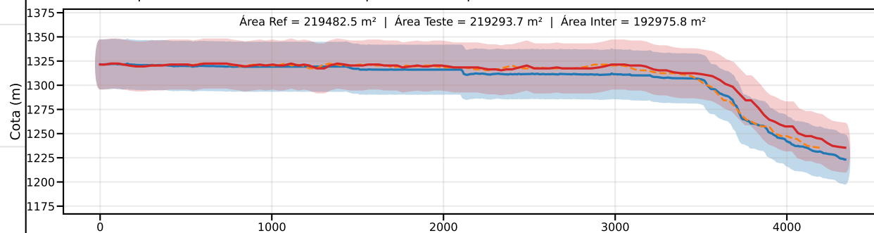
Classe C | PEC-PCD (Vertical)=30.0 m | EQ = 50m | dm = 9.50
