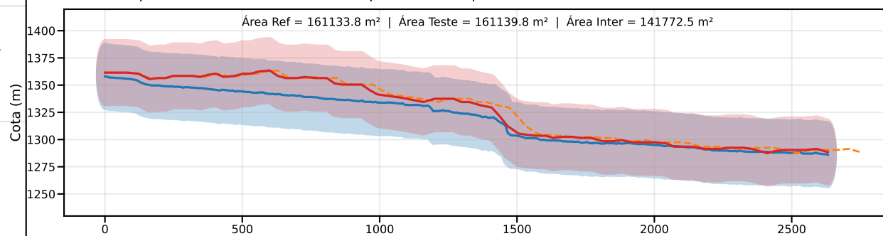
Classe D | PEC-PCD (Vertical)=37.5 m | EQ = 50m | dm = 11.30
