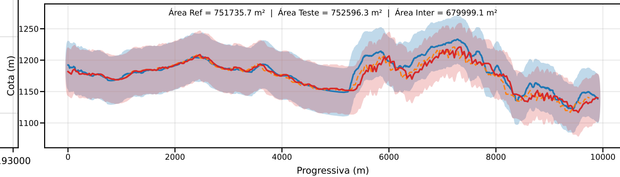
Classe D | PEC-PCD (Vertical)=37.5 m | EQ = 50m | dm = 11.23
