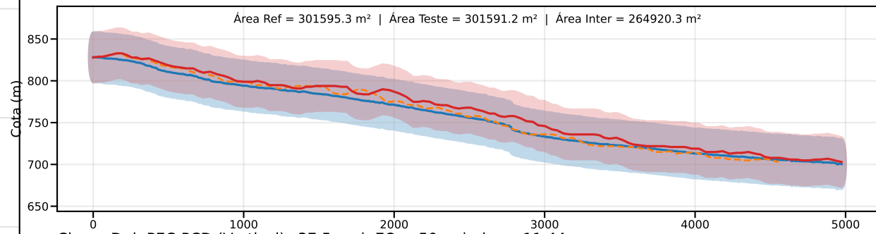
Classe D | PEC-PCD (Vertical)=37.5 m | EQ = 50m | dm = 11.44
