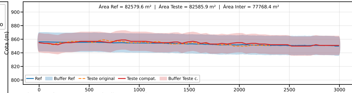
Classe B | PEC-PCD (Vertical)=25.0 m | EQ = 50m | dm = 2.50
