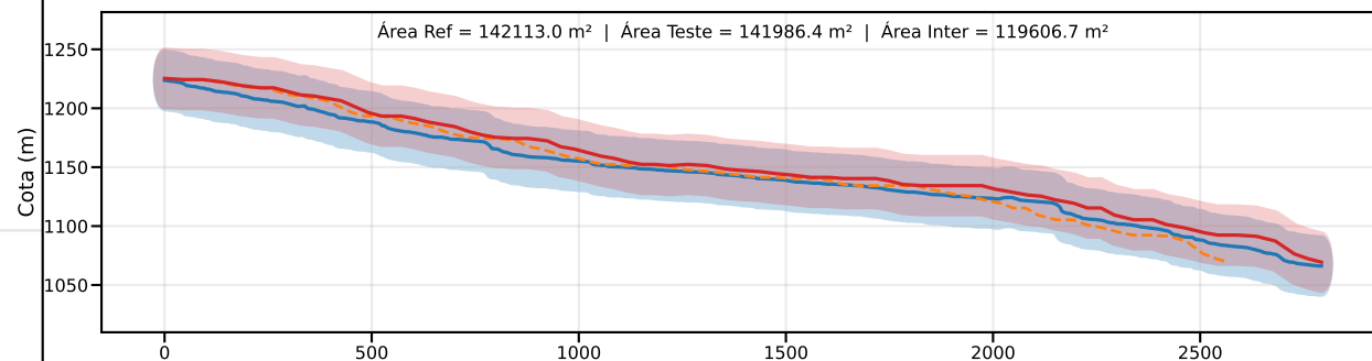
Classe C | PEC-PCD (Vertical)=30.0 m | EQ = 50m | dm = 12.43
