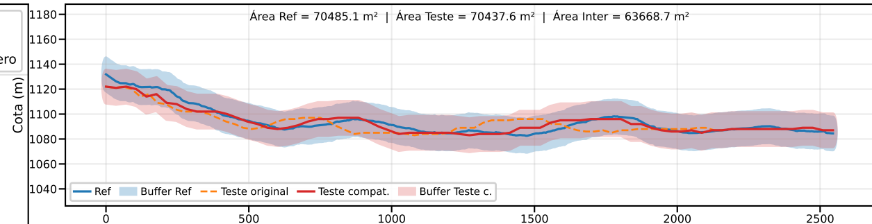
Classe B | PEC-PCD (Vertical)=25.0 m | EQ = 50m | dm = 4.23
