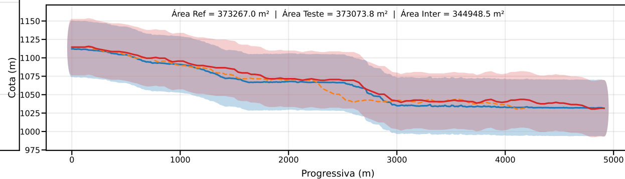
Classe D | PEC-PCD (Vertical)=37.5 m | EQ = 50m | dm = 8.94
