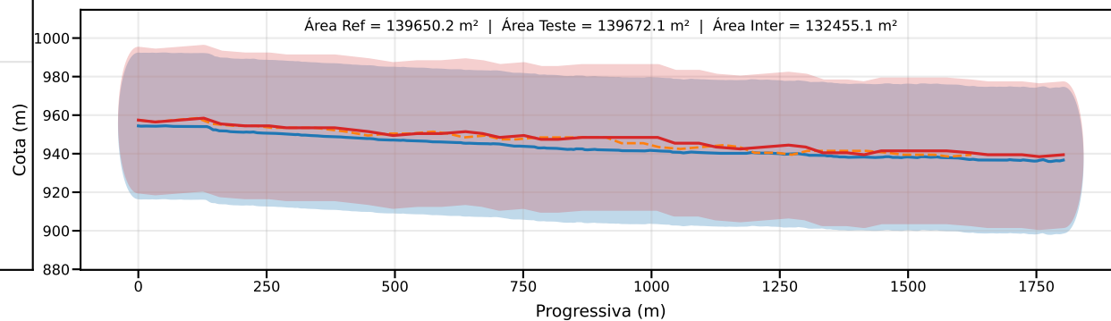
Classe D | PEC-PCD (Vertical)=37.5 m | EQ = 50m | dm = 6.07
