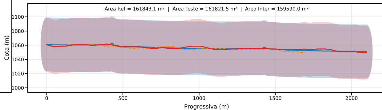
Classe D | PEC-PCD (Vertical)=37.5 m | EQ = 50m | dm = 1.64
