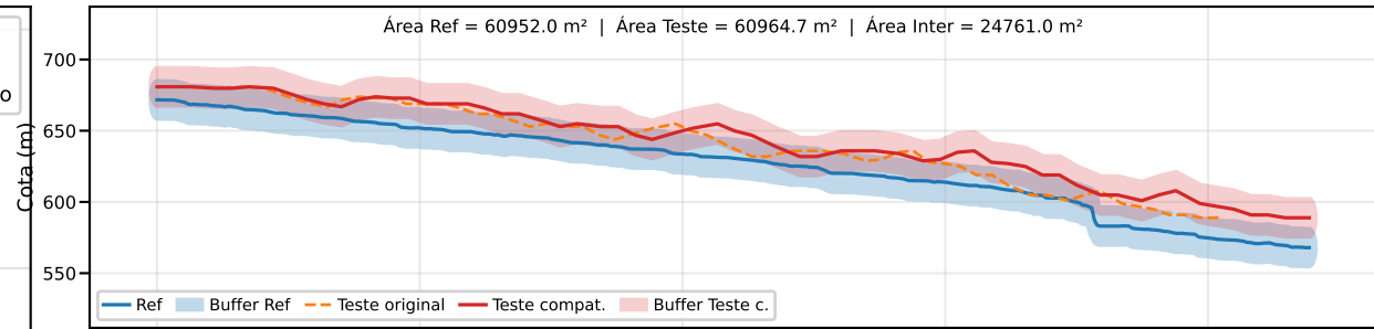
Classe B | PEC-PCD (Vertical)=25.0 m | EQ = 50m | dm = 25.61
