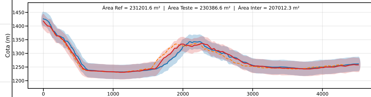
Classe C | PEC-PCD (Vertical)=30.0 m | EQ = 50m | dm = 8.27
