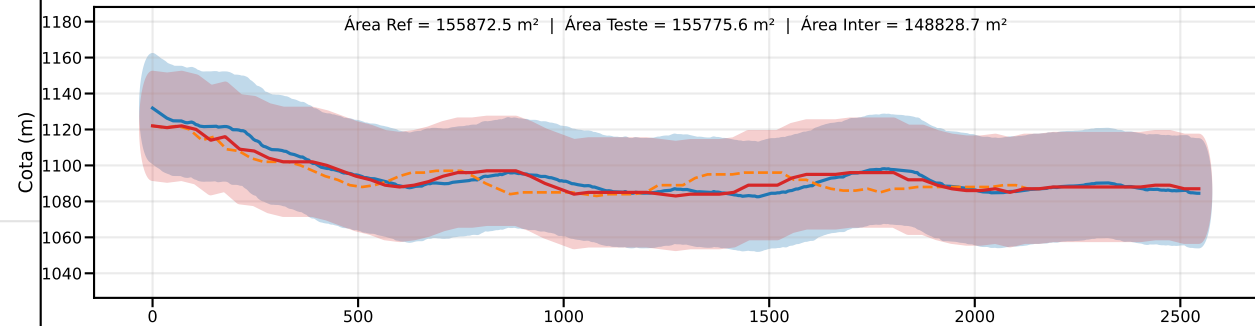
Classe D | PEC-PCD (Vertical)=37.5 m | EQ = 50m | dm = 4.30
