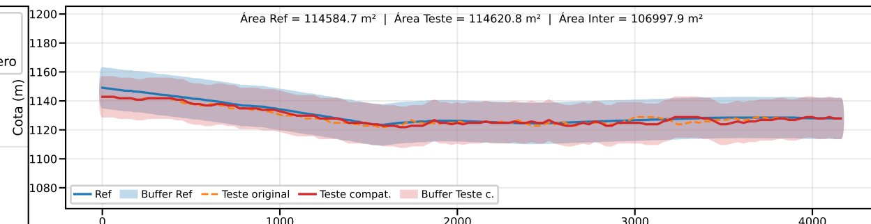
Classe B | PEC-PCD (Vertical)=25.0 m | EQ = 50m | dm = 2.86
