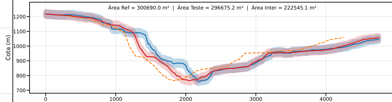
Classe D | PEC-PCD (Vertical)=37.5 m | EQ = 50m | dm = 26.70
