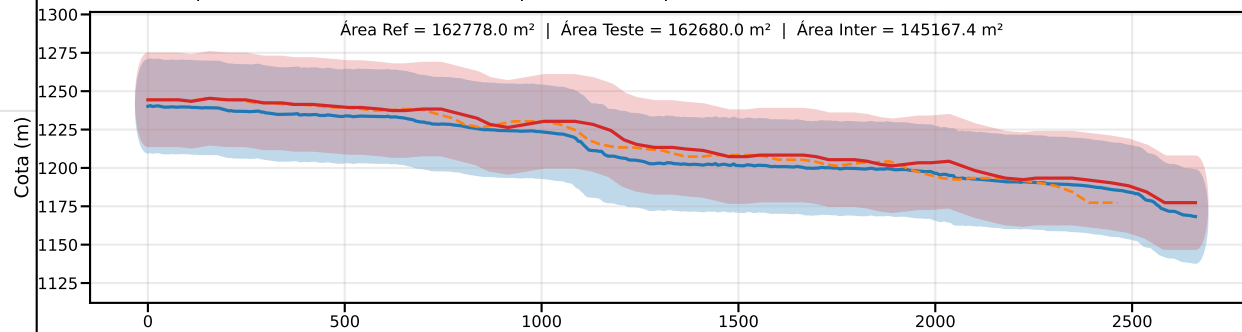
Classe D | PEC-PCD (Vertical)=37.5 m | EQ = 50m | dm = 10.22
