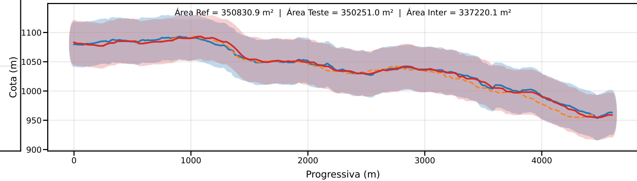
Classe D | PEC-PCD (Vertical)=37.5 m | EQ = 50m | dm = 4.58
