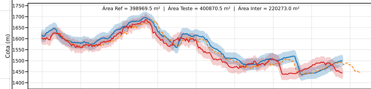
Classe C | PEC-PCD (Vertical)=30.0 m | EQ = 50m | dm = 36.08
