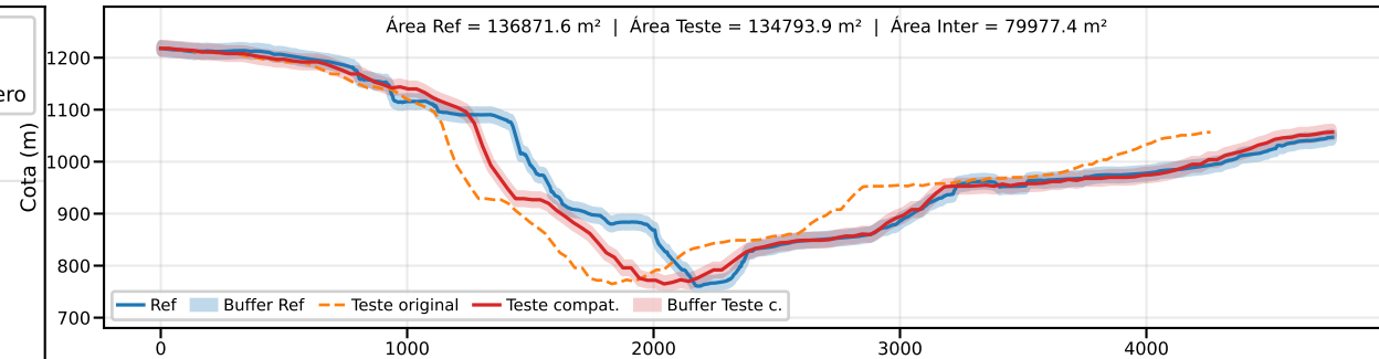
Classe B | PEC-PCD (Vertical)=25.0 m | EQ = 50m | dm = 23.18
