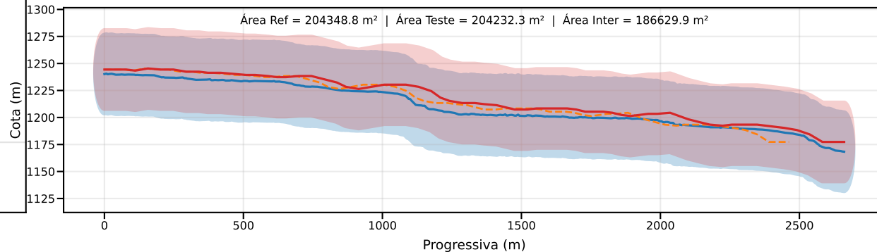
Classe D | PEC-PCD (Vertical)=37.5 m | EQ = 50m | dm = 10.22
