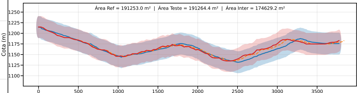
Classe C | PEC-PCD (Vertical)=30.0 m | EQ = 50m | dm = 6.83
