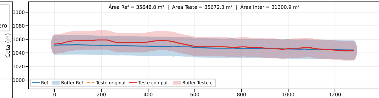
Classe B | PEC-PCD (Vertical)=25.0 m | EQ = 50m | dm = 5.20
