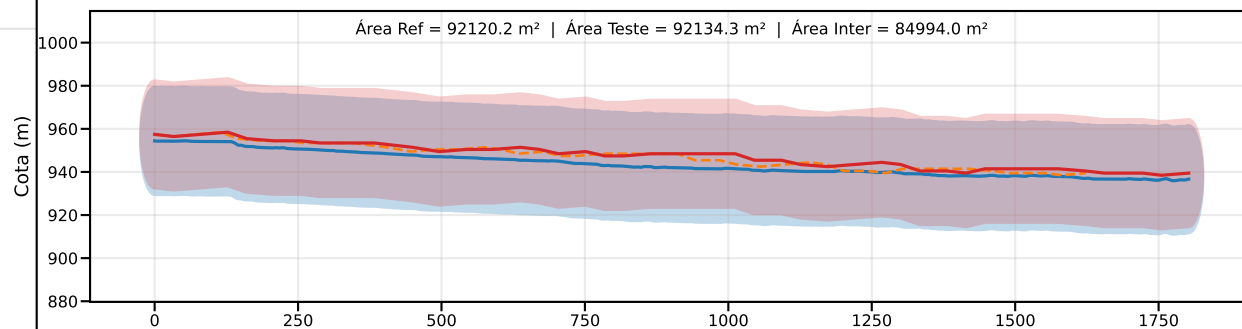
Classe C | PEC-PCD (Vertical)=30.0 m | EQ = 50m | dm = 6.07
