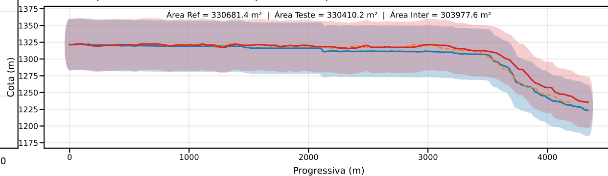
Classe D | PEC-PCD (Vertical)=37.5 m | EQ = 50m | dm = 9.52
