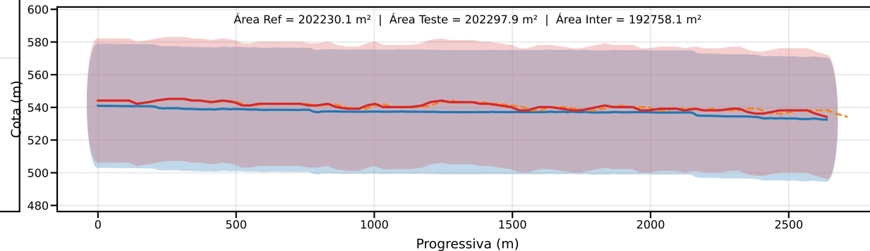
Classe D | PEC-PCD (Vertical)=37.5 m | EQ = 50m | dm = 5.52
