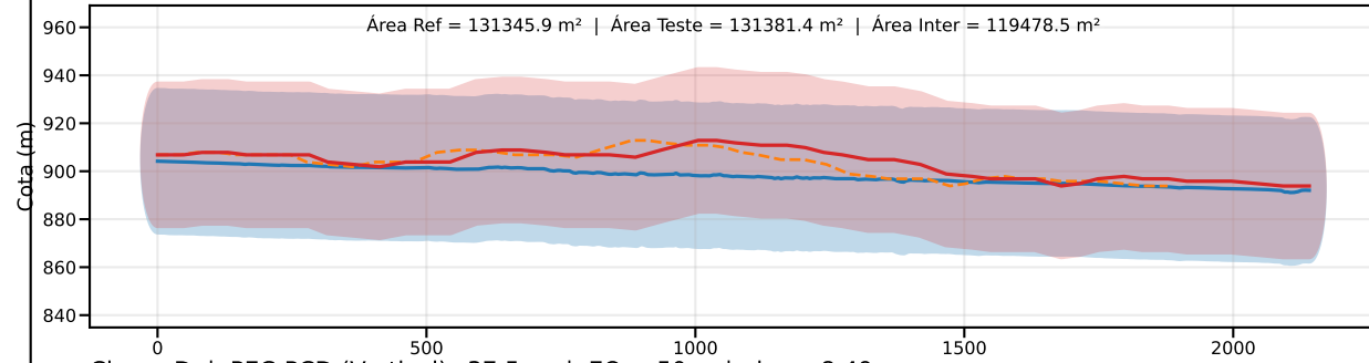
Classe D | PEC-PCD (Vertical)=37.5 m | EQ = 50m | dm = 8.49
