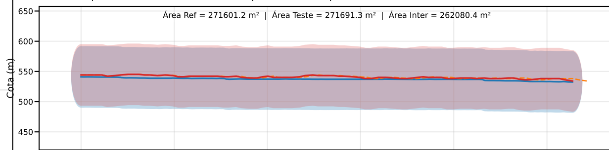
Classe C | PEC-PCD (Vertical)=60.0 m | EQ = 100m | dm = 5.50
