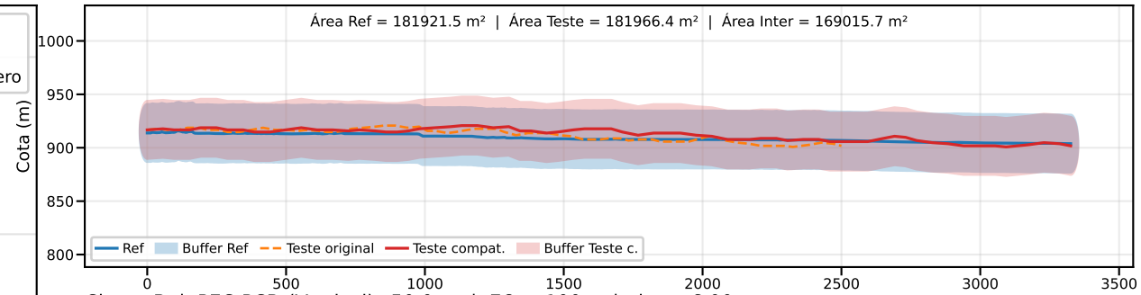
Classe B | PEC-PCD (Vertical)=50.0 m | EQ = 100m | dm = 6.00
