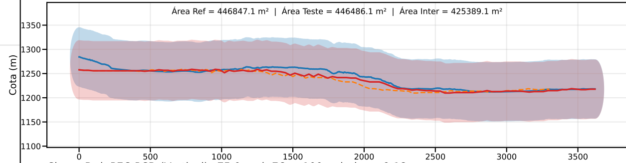
Classe D | PEC-PCD (Vertical)=75.0 m | EQ = 100m | dm = 9.18
