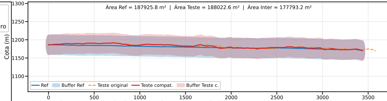
Classe B | PEC-PCD (Vertical)=50.0 m | EQ = 100m | dm = 4.53
