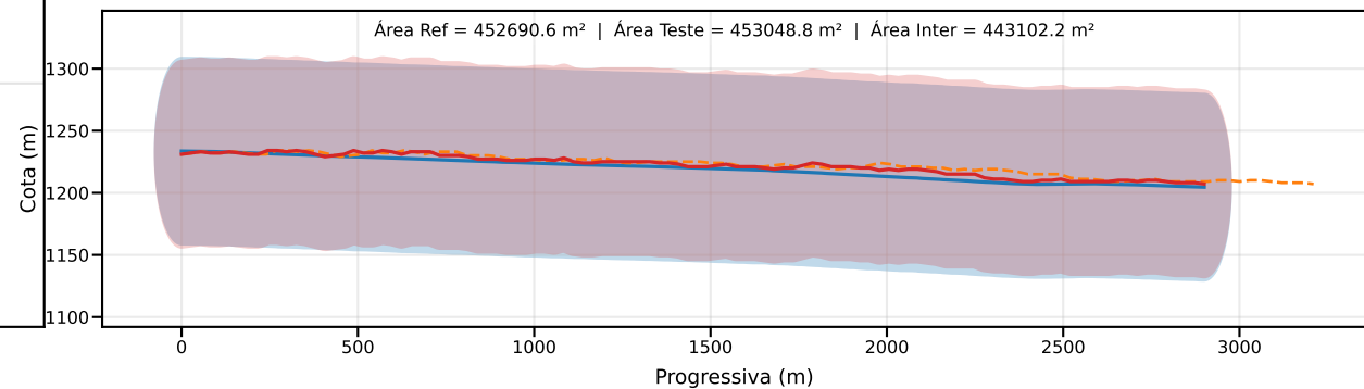
Classe D | PEC-PCD (Vertical)=75.0 m | EQ = 100m | dm = 4.99
