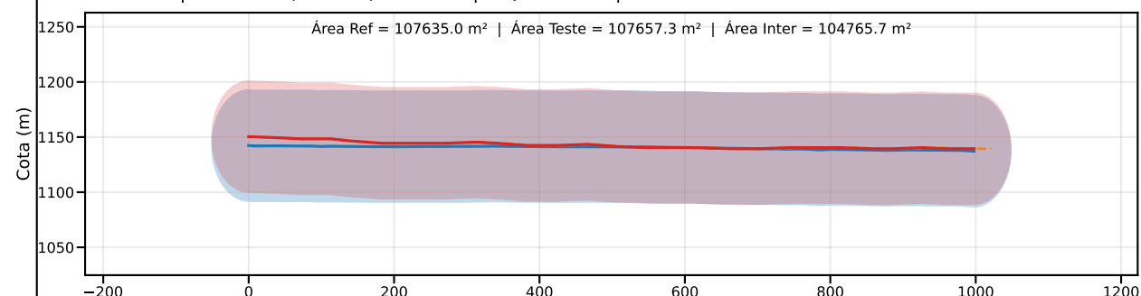
Classe C | PEC-PCD (Vertical)=60.0 m | EQ = 100m | dm = 4.27
