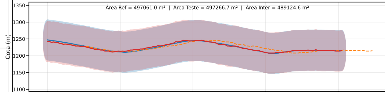
Classe D | PEC-PCD (Vertical)=75.0 m | EQ = 100m | dm = 3.02
