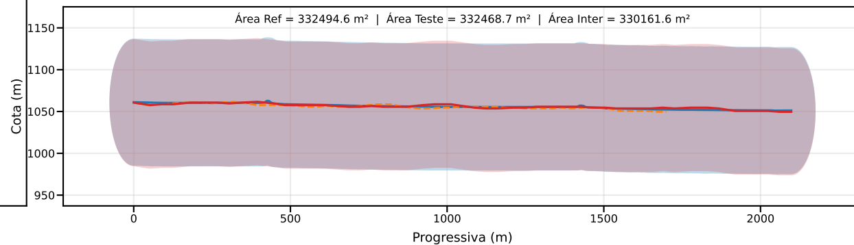
Classe D | PEC-PCD (Vertical)=75.0 m | EQ = 100m | dm = 1.65
