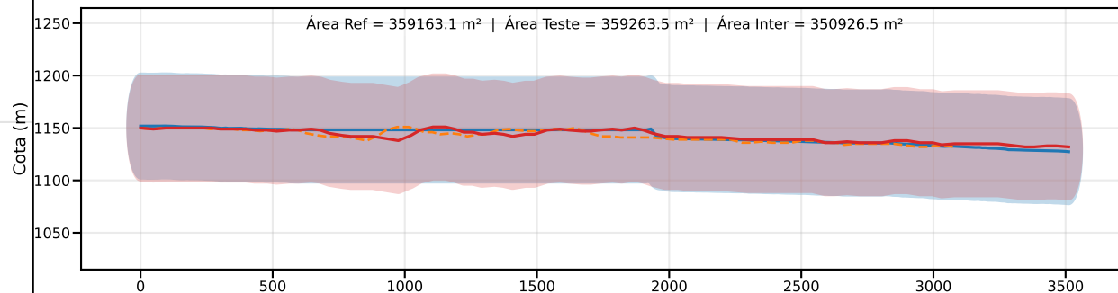
Classe C | PEC-PCD (Vertical)=60.0 m | EQ = 100m | dm = 3.61
