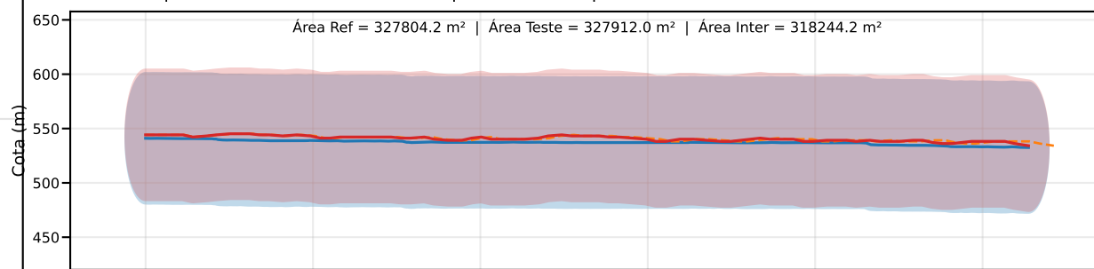
Classe D | PEC-PCD (Vertical)=75.0 m | EQ = 100m | dm = 5.48
