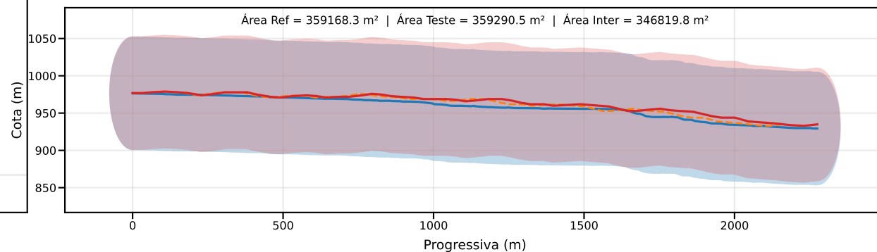
Classe D | PEC-PCD (Vertical)=75.0 m | EQ = 100m | dm = 8.10
