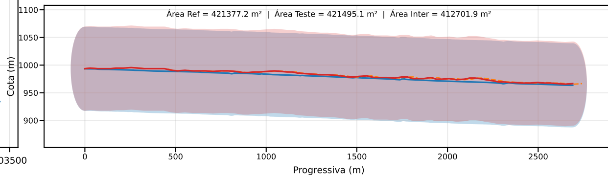
Classe D | PEC-PCD (Vertical)=75.0 m | EQ = 100m | dm = 4.85
