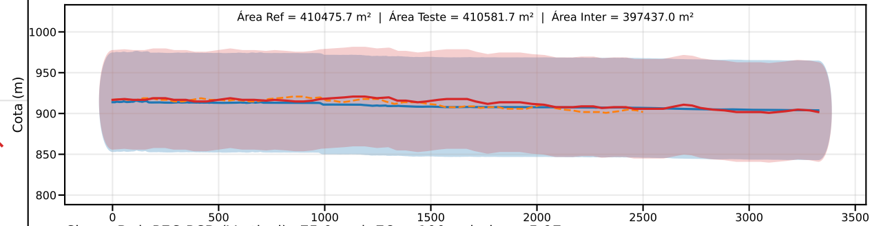
Classe D | PEC-PCD (Vertical)=75.0 m | EQ = 100m | dm = 5.97
