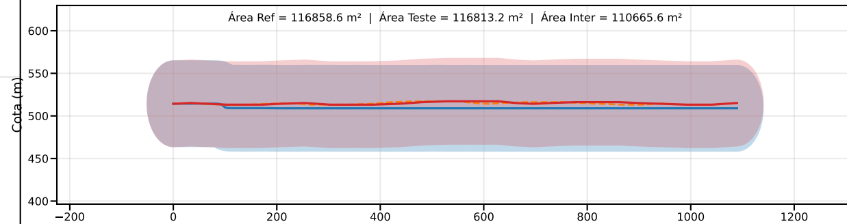
Classe C | PEC-PCD (Vertical)=60.0 m | EQ = 100m | dm = 8.31
