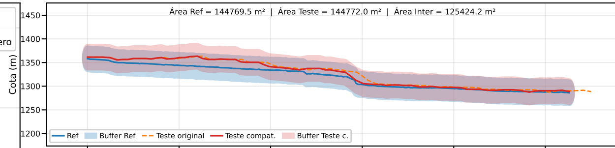
Classe B | PEC-PCD (Vertical)=50.0 m | EQ = 100m | dm = 11.25
