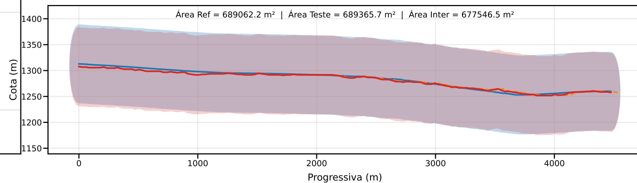
Classe D | PEC-PCD (Vertical)=75.0 m | EQ = 100m | dm = 3.94
