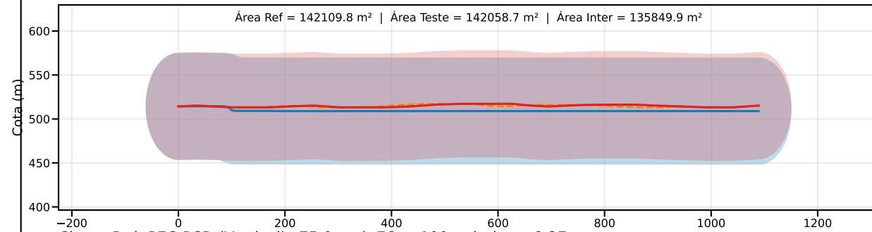
Classe D | PEC-PCD (Vertical)=75.0 m | EQ = 100m | dm = 8.27
