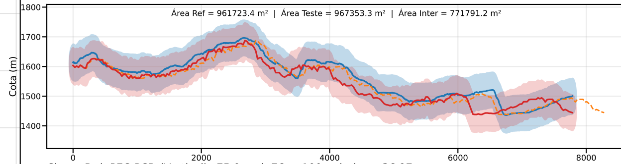
Classe D | PEC-PCD (Vertical)=75.0 m | EQ = 100m | dm = 36.97
