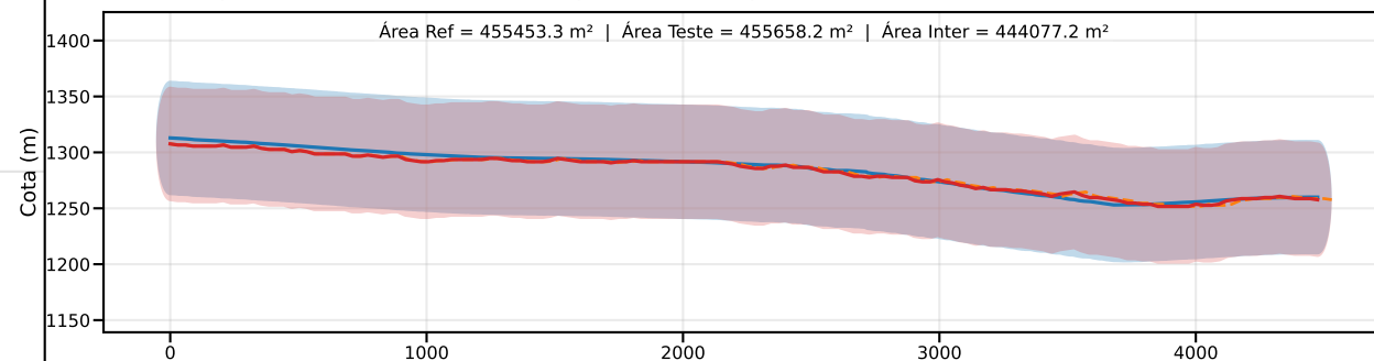
Classe C | PEC-PCD (Vertical)=60.0 m | EQ = 100m | dm = 3.93
