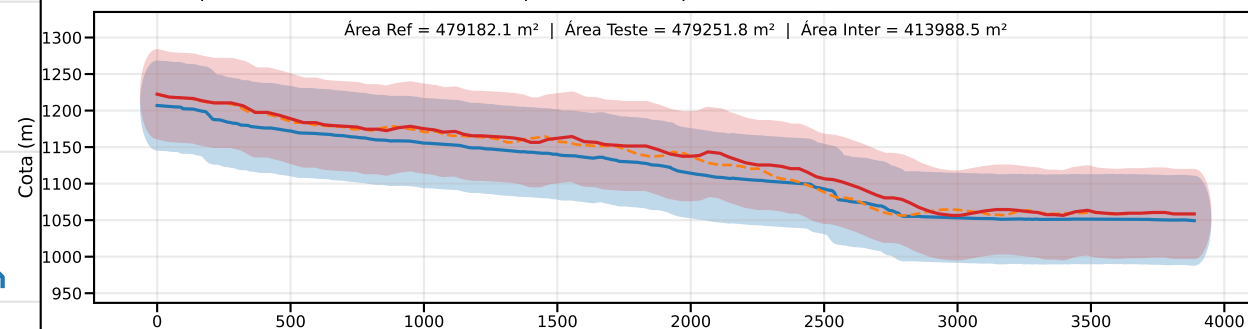
Classe D | PEC-PCD (Vertical)=75.0 m | EQ = 100m | dm = 25.63
