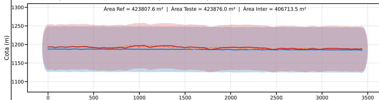
Classe D | PEC-PCD (Vertical)=75.0 m | EQ = 100m | dm = 7.62
