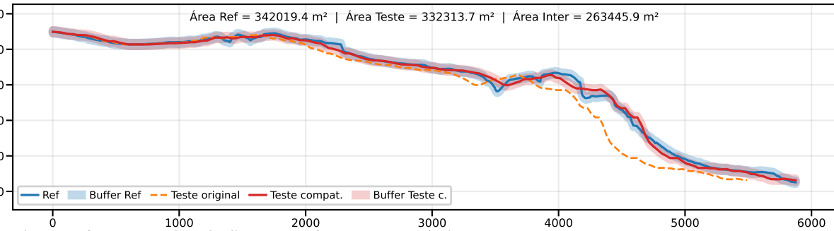
Classe B | PEC-PCD (Vertical)=50.0 m | EQ = 100m | dm = 20.75
