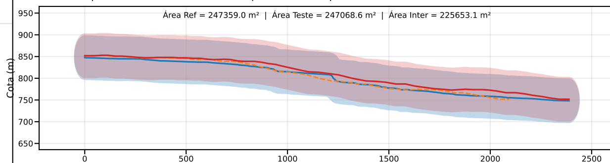
Classe C | PEC-PCD (Vertical)=60.0 m | EQ = 100m | dm = 13.78
