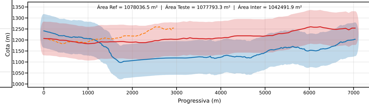
Classe D | PEC-PCD (Vertical)=75.0 m | EQ = 100m | dm = 7.77
