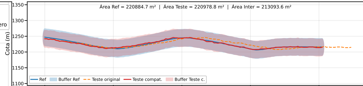
Classe B | PEC-PCD (Vertical)=50.0 m | EQ = 100m | dm = 3.00
