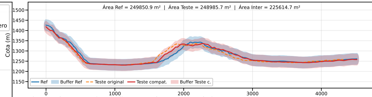
Classe B | PEC-PCD (Vertical)=50.0 m | EQ = 100m | dm = 8.36
