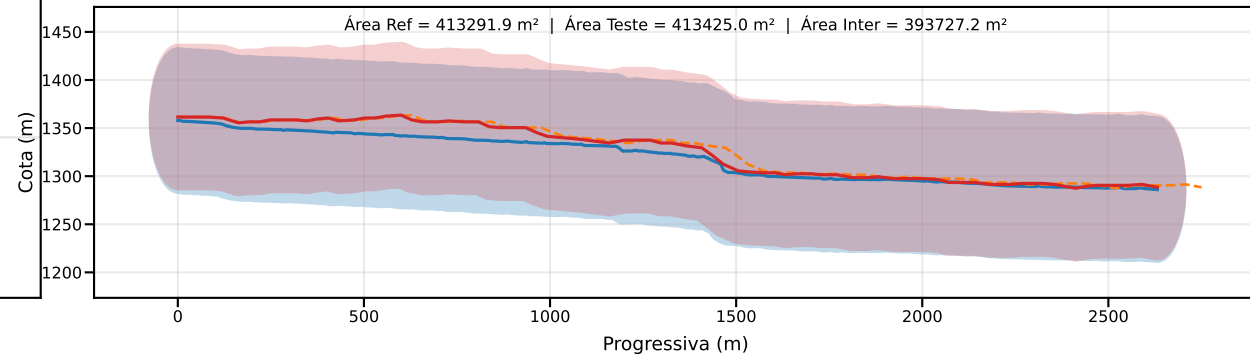
Classe D | PEC-PCD (Vertical)=75.0 m | EQ = 100m | dm = 11.15
