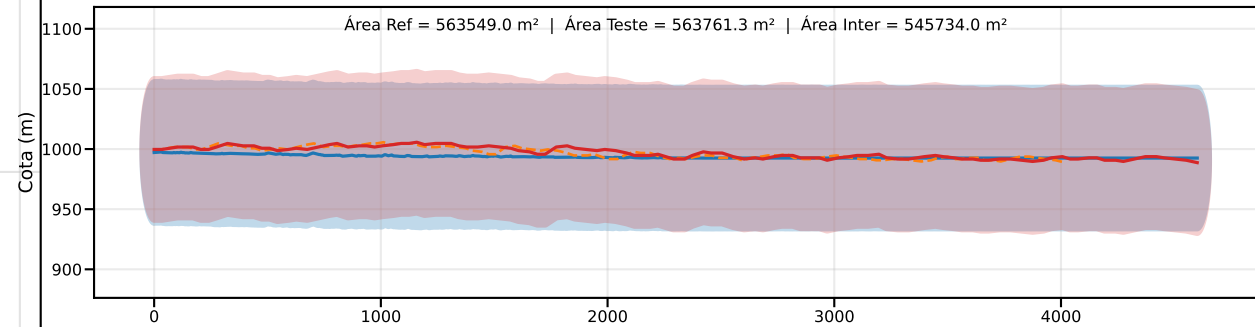
Classe D | PEC-PCD (Vertical)=75.0 m | EQ = 100m | dm = 5.95
