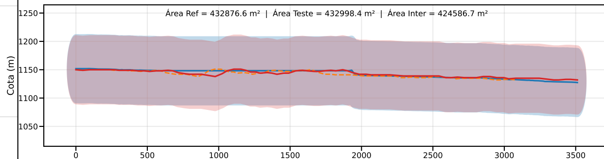
Classe D | PEC-PCD (Vertical)=75.0 m | EQ = 100m | dm = 3.62
