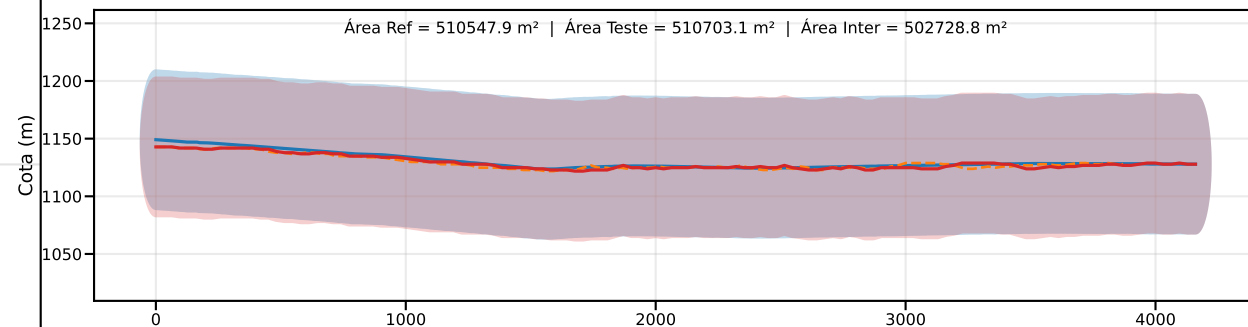
Classe D | PEC-PCD (Vertical)=75.0 m | EQ = 100m | dm = 2.90
