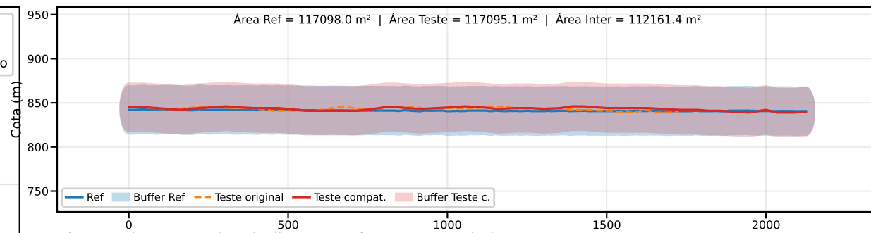
Classe B | PEC-PCD (Vertical)=50.0 m | EQ = 100m | dm = 3.57
