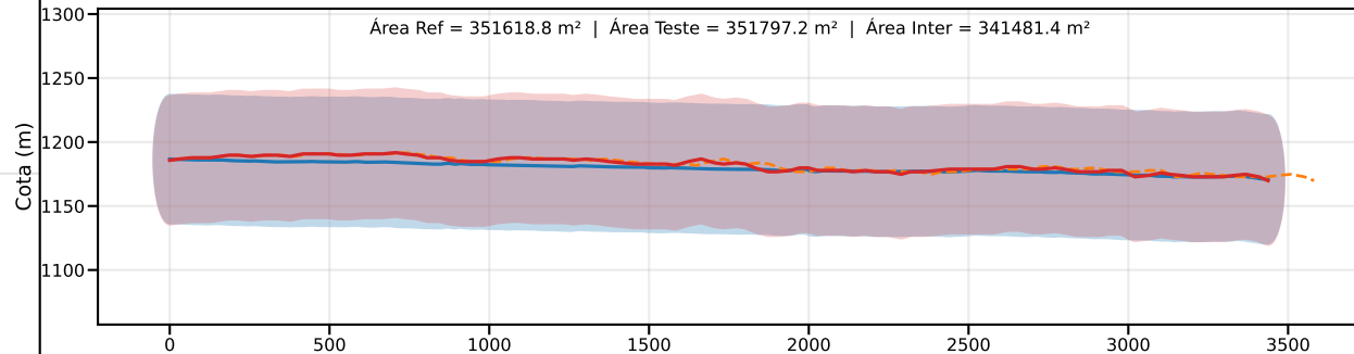
Classe C | PEC-PCD (Vertical)=60.0 m | EQ = 100m | dm = 4.51
