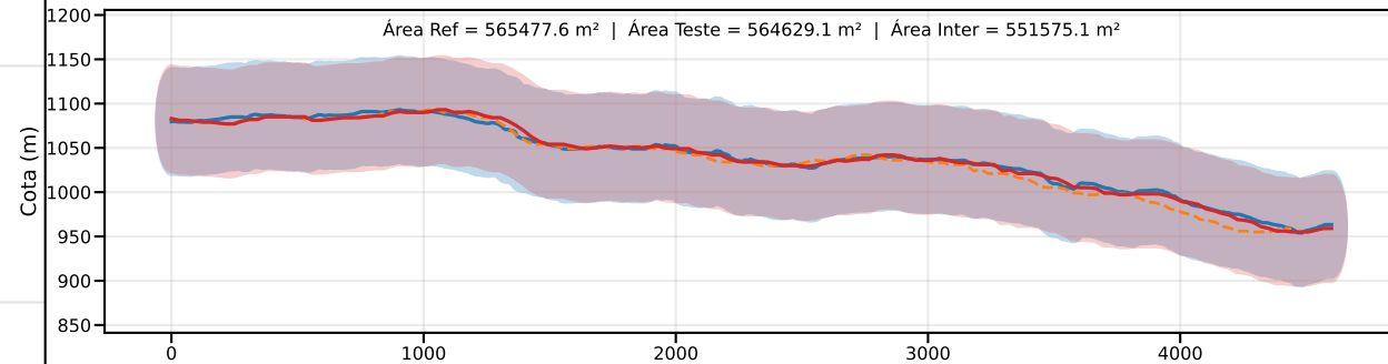
Classe D | PEC-PCD (Vertical)=75.0 m | EQ = 100m | dm = 4.68
