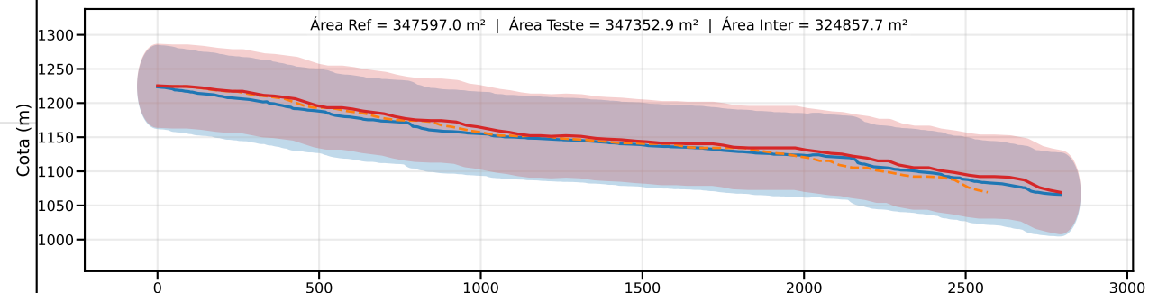
Classe D | PEC-PCD (Vertical)=75.0 m | EQ = 100m | dm = 12.29
