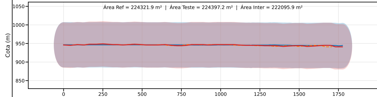
Classe D | PEC-PCD (Vertical)=75.0 m | EQ = 100m | dm = 1.89
