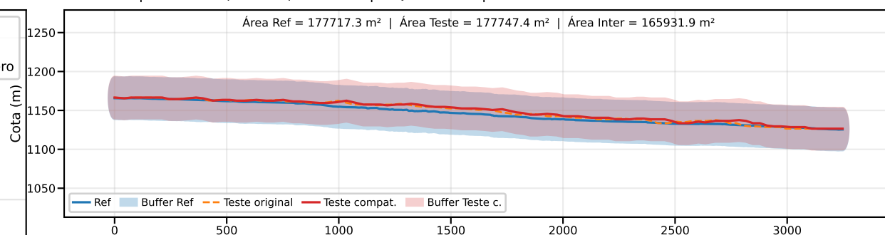
Classe B | PEC-PCD (Vertical)=50.0 m | EQ = 100m | dm = 5.58
