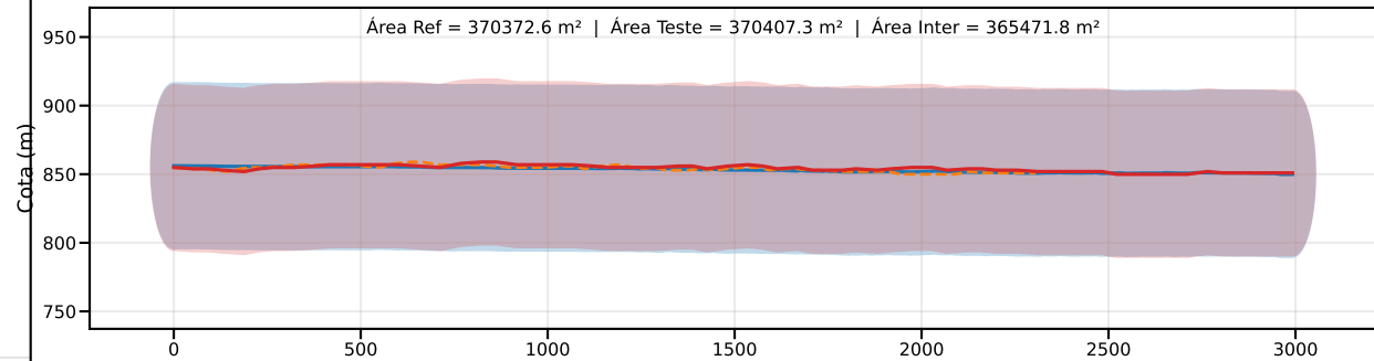
Classe D | PEC-PCD (Vertical)=75.0 m | EQ = 100m | dm = 2.49
