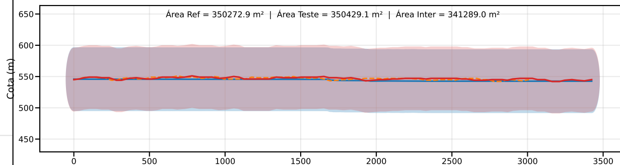
Classe C | PEC-PCD (Vertical)=60.0 m | EQ = 100m | dm = 4.02
