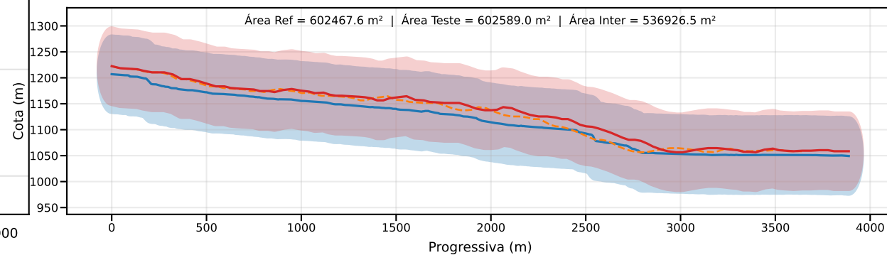
Classe D | PEC-PCD (Vertical)=75.0 m | EQ = 100m | dm = 25.63
