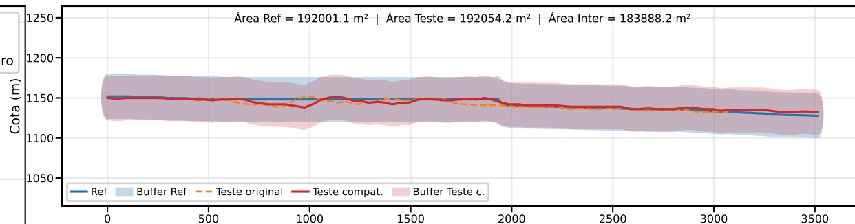
Classe B | PEC-PCD (Vertical)=50.0 m | EQ = 100m | dm = 3.60
