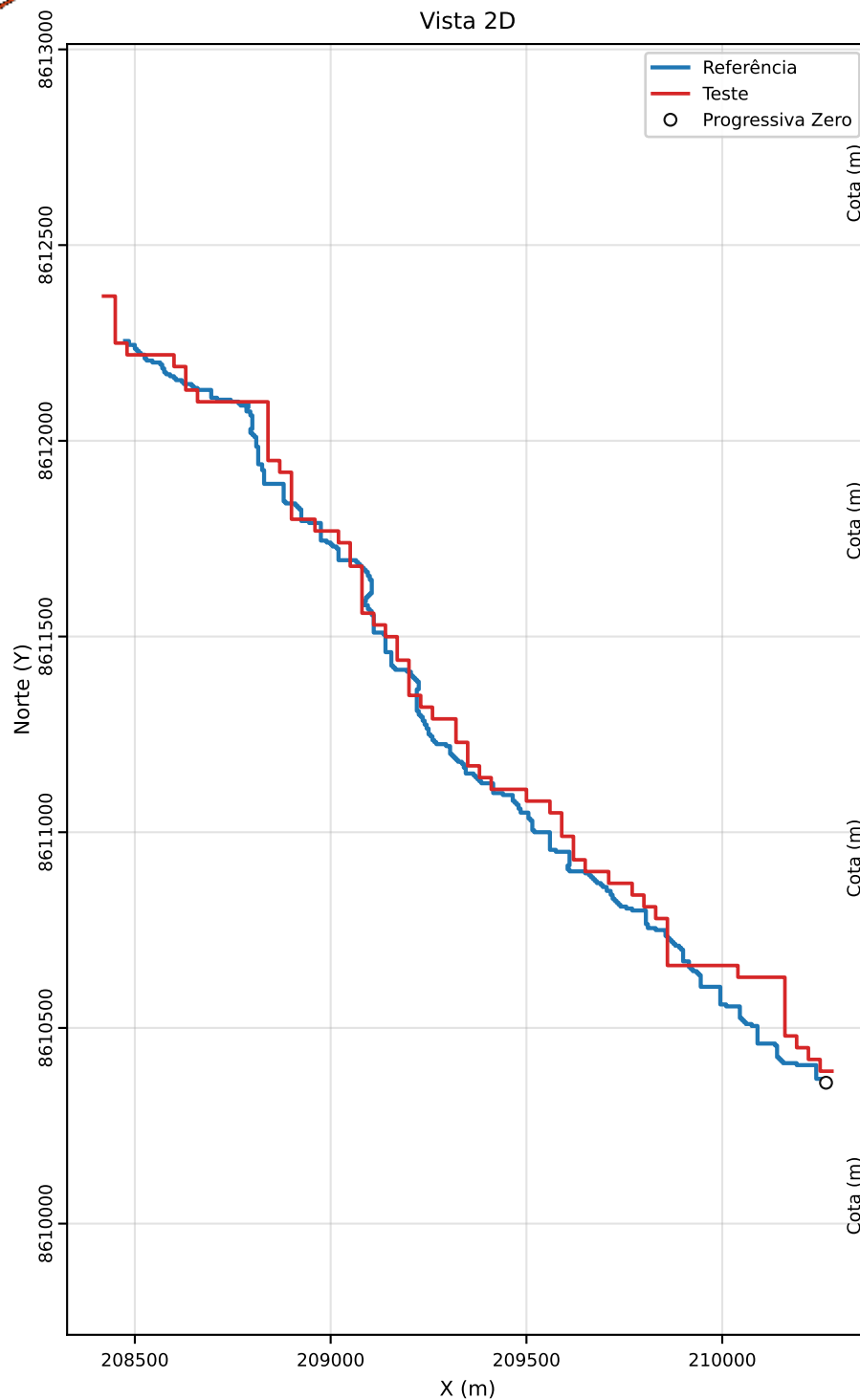
Classe A | PEC-PCD (Vertical)=27.0 m | EQ = 100m | dm = 6.83
