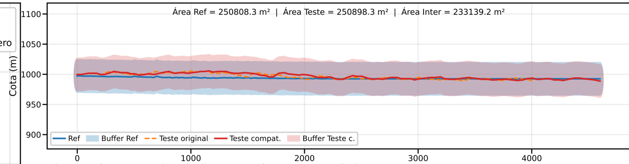
Classe B | PEC-PCD (Vertical)=50.0 m | EQ = 100m | dm = 5.96
