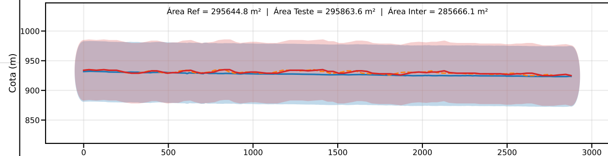
Classe C | PEC-PCD (Vertical)=60.0 m | EQ = 100m | dm = 5.28
