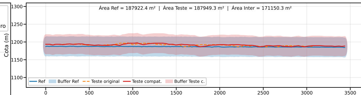
Classe B | PEC-PCD (Vertical)=50.0 m | EQ = 100m | dm = 7.59
