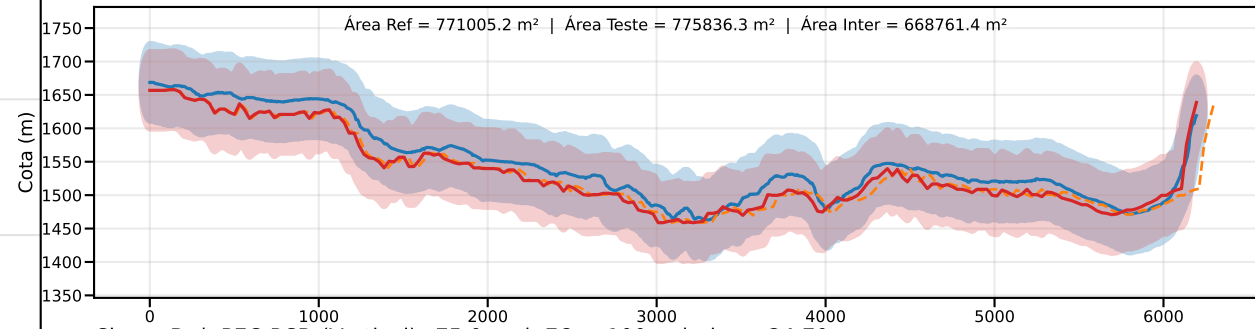
Classe D | PEC-PCD (Vertical)=75.0 m | EQ = 100m | dm = 24.70
