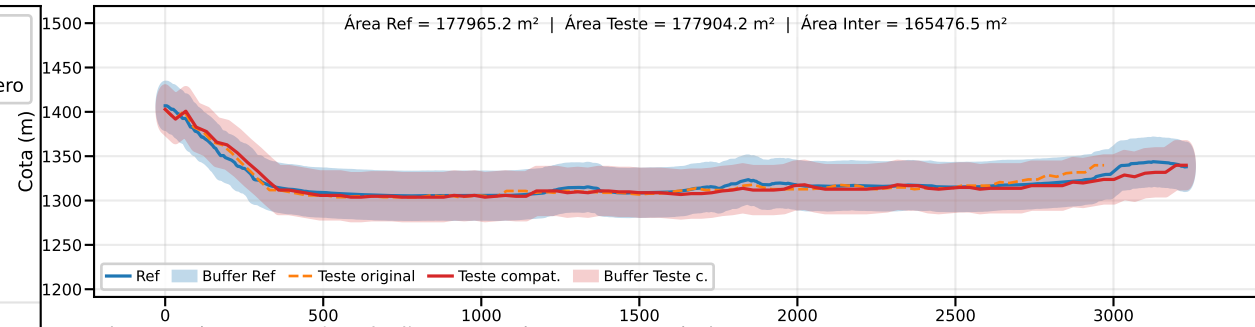
Classe B | PEC-PCD (Vertical)=50.0 m | EQ = 100m | dm = 5.95
