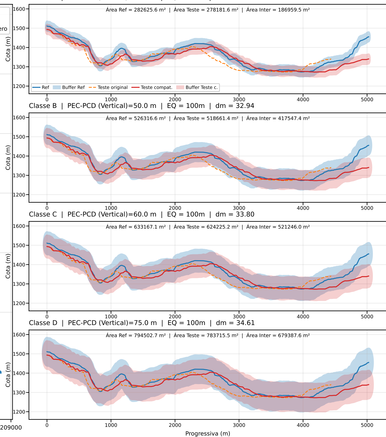
Classe A | PEC-PCD (Vertical)=27.0 m | EQ = 100m | dm = 29.17
