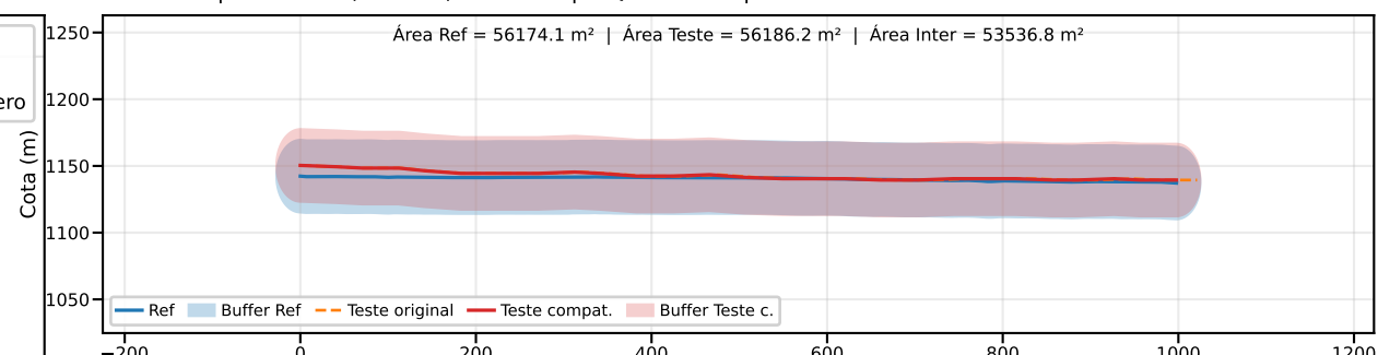
Classe B | PEC-PCD (Vertical)=50.0 m | EQ = 100m | dm = 4.19
