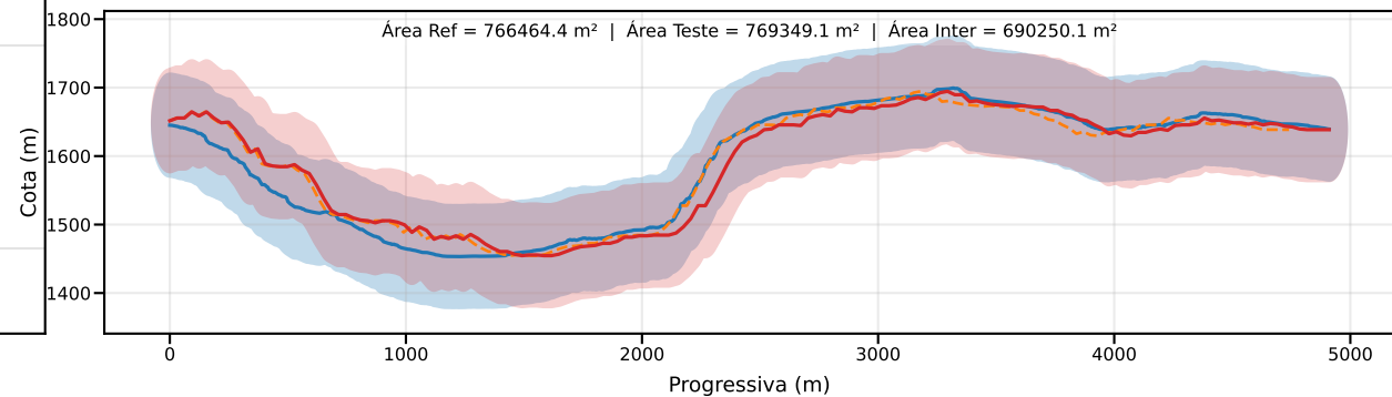
Classe D | PEC-PCD (Vertical)=75.0 m | EQ = 100m | dm = 23.34
