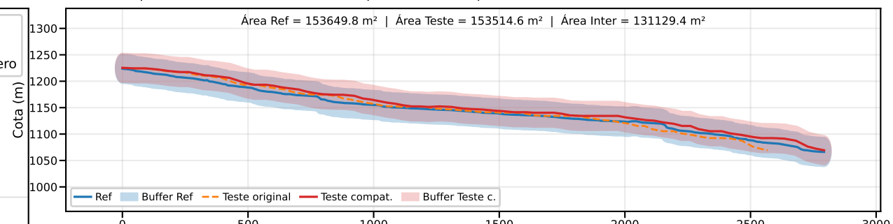
Classe B | PEC-PCD (Vertical)=50.0 m | EQ = 100m | dm = 12.37
