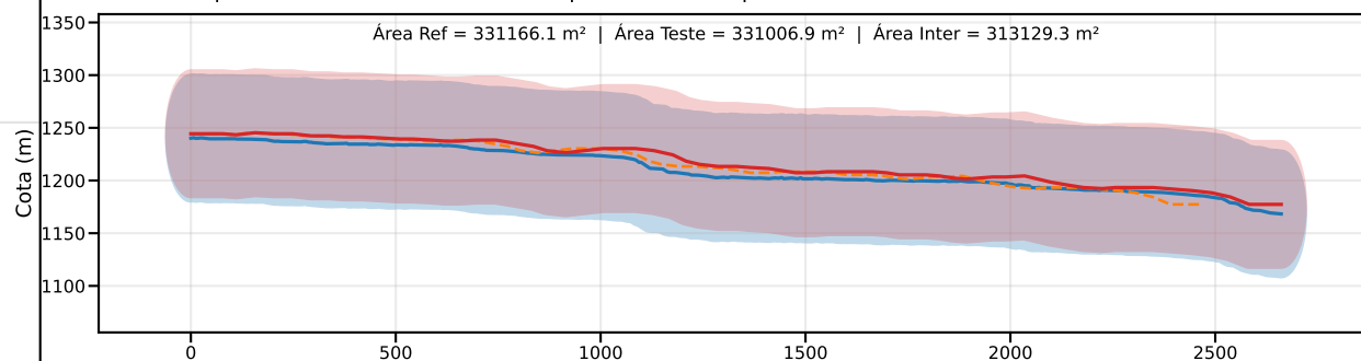
Classe D | PEC-PCD (Vertical)=75.0 m | EQ = 100m | dm = 10.30
