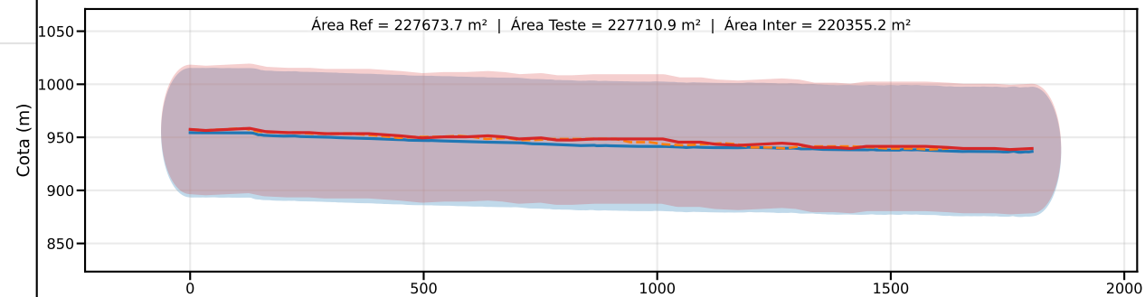
Classe D | PEC-PCD (Vertical)=75.0 m | EQ = 100m | dm = 6.05
