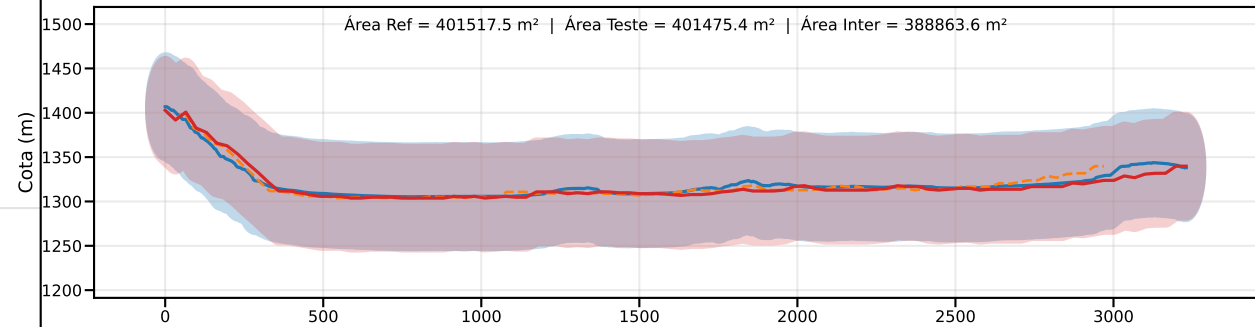
Classe D | PEC-PCD (Vertical)=75.0 m | EQ = 100m | dm = 5.93
