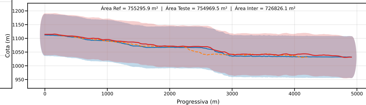
Classe D | PEC-PCD (Vertical)=75.0 m | EQ = 100m | dm = 8.89
