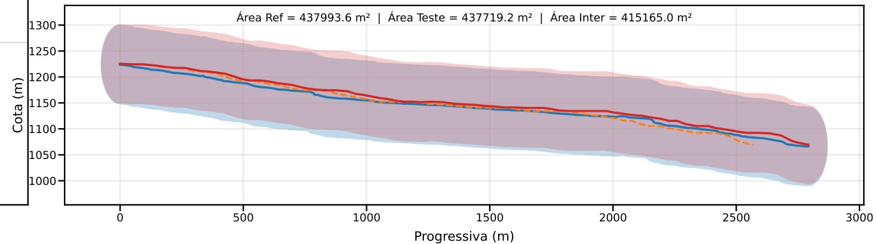
Classe D | PEC-PCD (Vertical)=75.0 m | EQ = 100m | dm = 12.29
