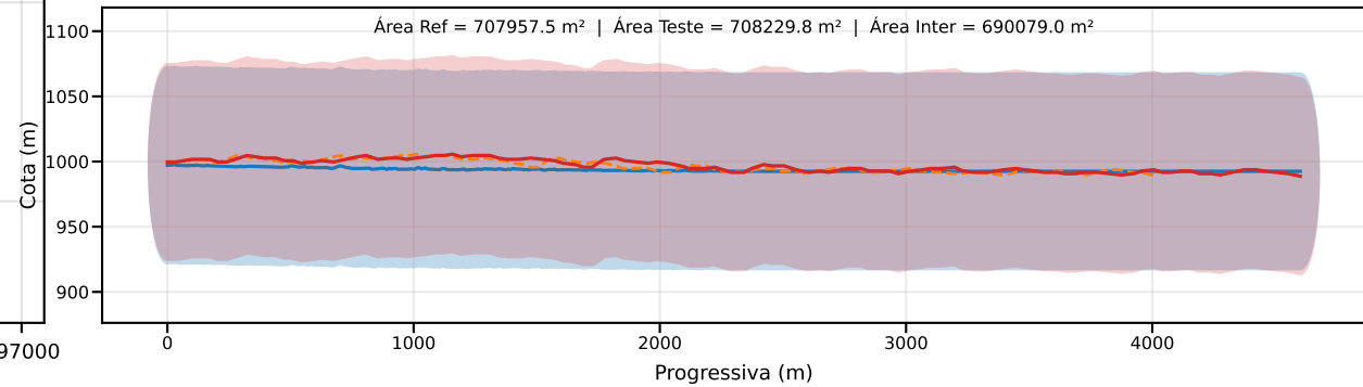
Classe D | PEC-PCD (Vertical)=75.0 m | EQ = 100m | dm = 5.95
