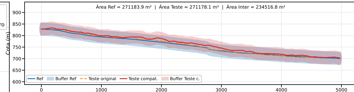
Classe B | PEC-PCD (Vertical)=50.0 m | EQ = 100m | dm = 11.40
