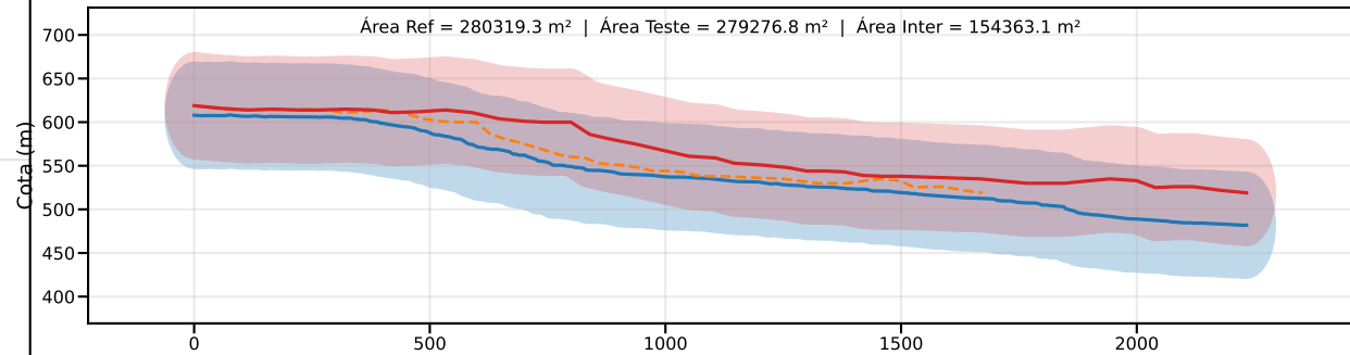
Classe D | PEC-PCD (Vertical)=75.0 m | EQ = 100m | dm = 86.05
