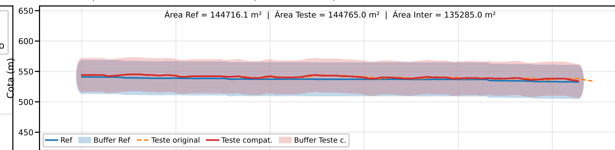
Classe B | PEC-PCD (Vertical)=50.0 m | EQ = 100m | dm = 5.50
