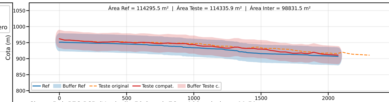
Classe B | PEC-PCD (Vertical)=50.0 m | EQ = 100m | dm = 11.51
