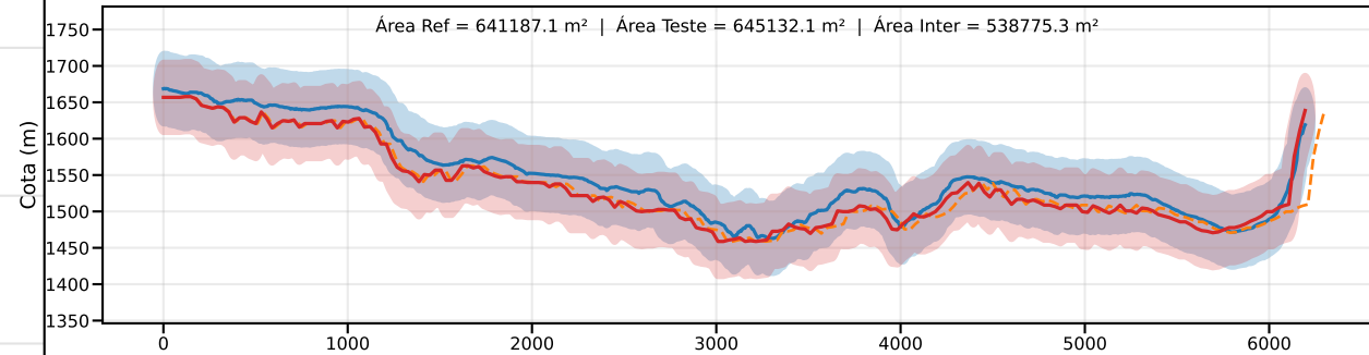
Classe C | PEC-PCD (Vertical)=60.0 m | EQ = 100m | dm = 24.84
