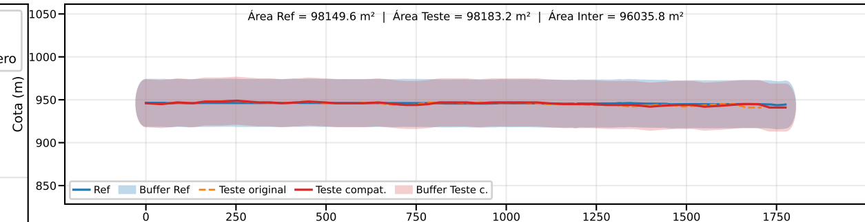
Classe B | PEC-PCD (Vertical)=50.0 m | EQ = 100m | dm = 1.86
