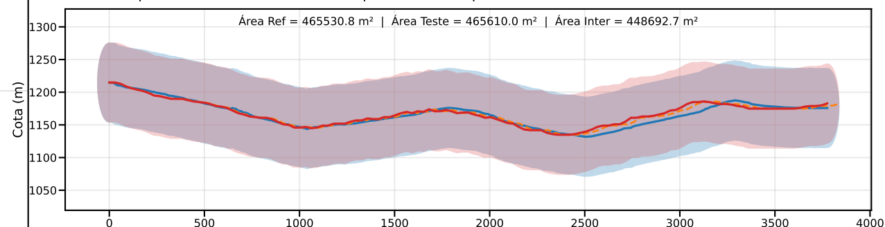
Classe D | PEC-PCD (Vertical)=75.0 m | EQ = 100m | dm = 6.81
