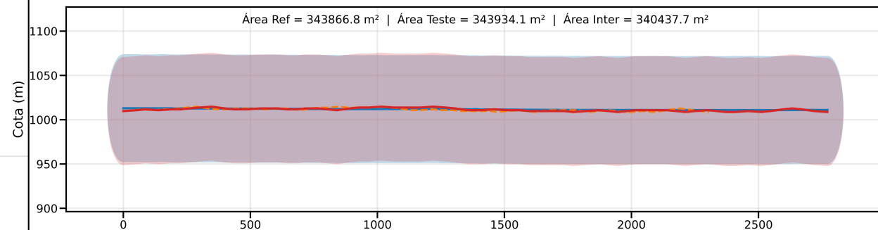
Classe D | PEC-PCD (Vertical)=75.0 m | EQ = 100m | dm = 1.90
