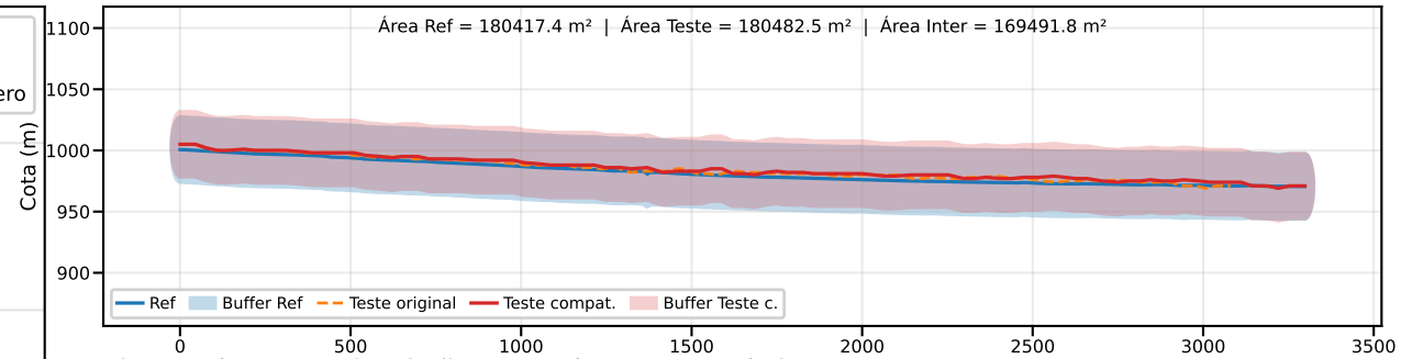
Classe B | PEC-PCD (Vertical)=50.0 m | EQ = 100m | dm = 5.12
