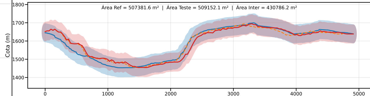
Classe C | PEC-PCD (Vertical)=60.0 m | EQ = 100m | dm = 23.52
