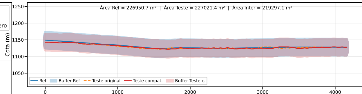
Classe B | PEC-PCD (Vertical)=50.0 m | EQ = 100m | dm = 2.88
