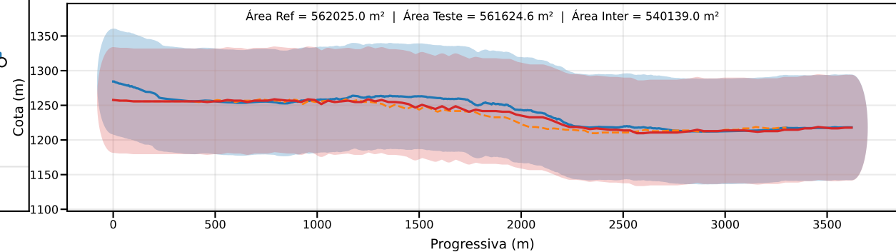
Classe D | PEC-PCD (Vertical)=75.0 m | EQ = 100m | dm = 9.18
