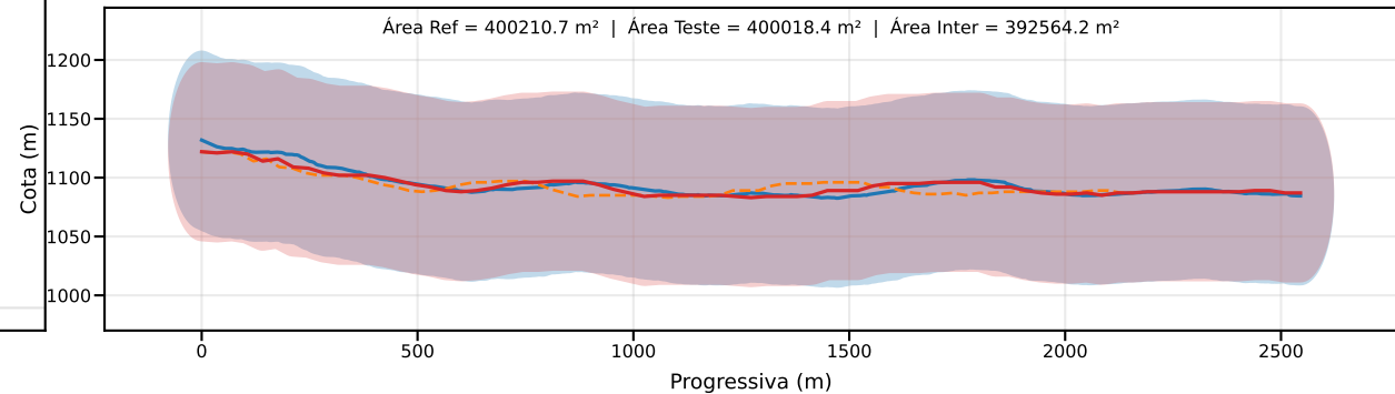
Classe D | PEC-PCD (Vertical)=75.0 m | EQ = 100m | dm = 4.50
