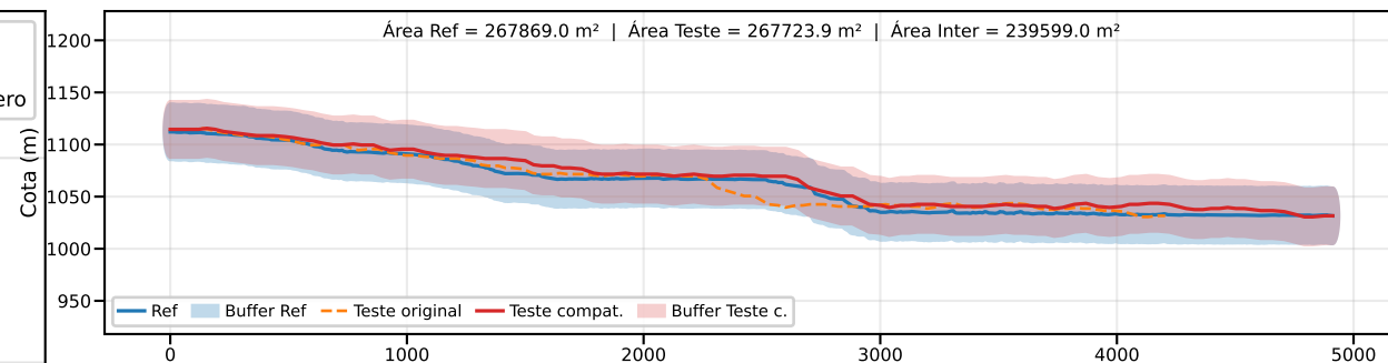
Classe B | PEC-PCD (Vertical)=50.0 m | EQ = 100m | dm = 8.92
