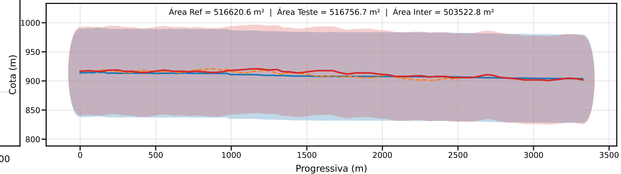
Classe D | PEC-PCD (Vertical)=75.0 m | EQ = 100m | dm = 5.97
