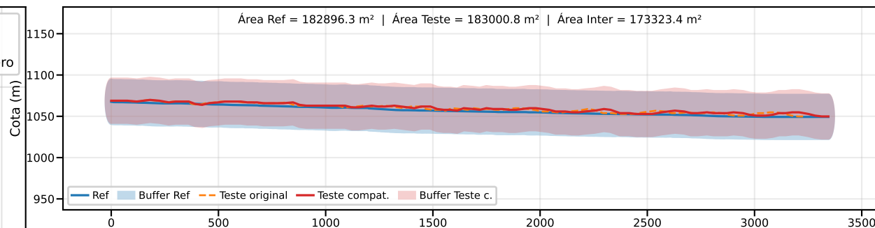
Classe B | PEC-PCD (Vertical)=50.0 m | EQ = 100m | dm = 4.39
