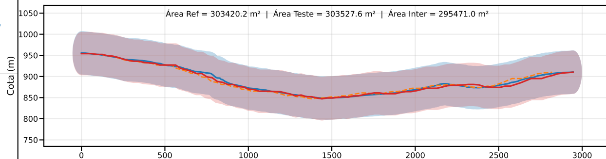
Classe C | PEC-PCD (Vertical)=60.0 m | EQ = 100m | dm = 4.10
