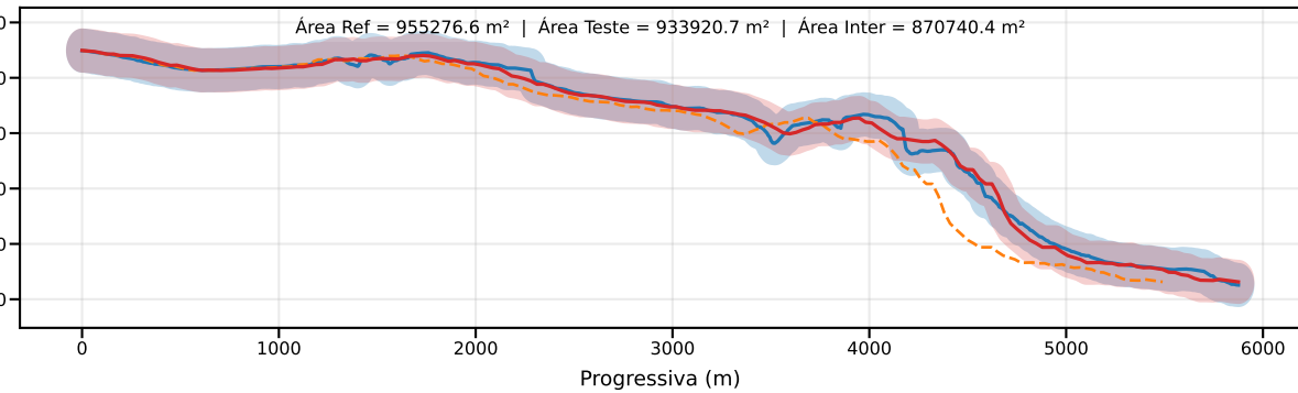
Classe D | PEC-PCD (Vertical)=75.0 m | EQ = 100m | dm = 21.33
