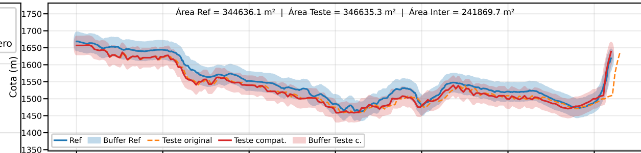
Classe B | PEC-PCD (Vertical)=50.0 m | EQ = 100m | dm = 24.94
