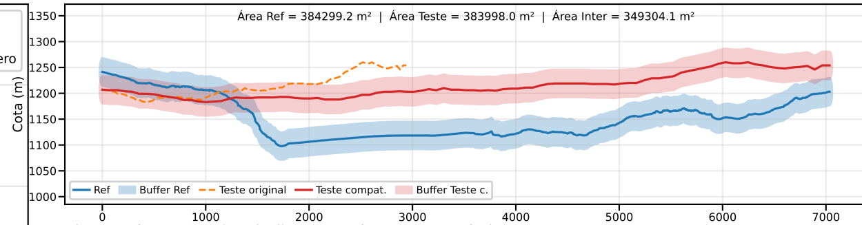
Classe B | PEC-PCD (Vertical)=50.0 m | EQ = 100m | dm = 7.76
