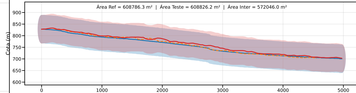
Classe D | PEC-PCD (Vertical)=75.0 m | EQ = 100m | dm = 11.33
