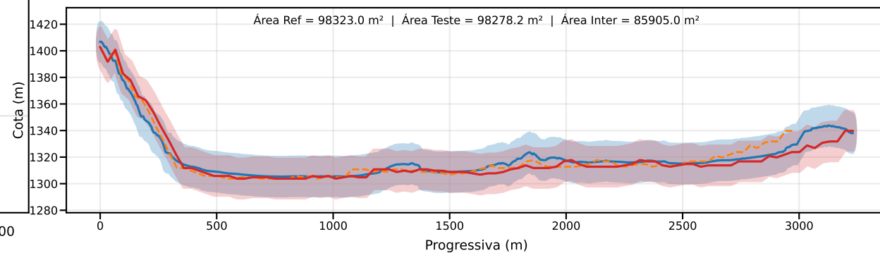
Classe D | PEC-PCD (Vertical)=15.0 m | EQ = 20m | dm = 5.95
