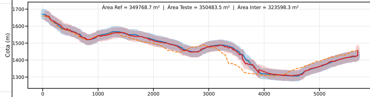
Classe D | PEC-PCD (Vertical)=37.5 m | EQ = 50m | dm = 7.21
