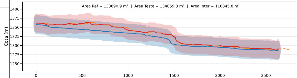
Classe C | PEC-PCD (Vertical)=30.0 m | EQ = 50m | dm = 13.47
