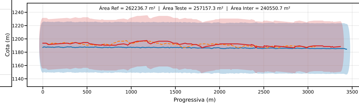
Classe D | PEC-PCD (Vertical)=37.5 m | EQ = 50m | dm = 9.93
