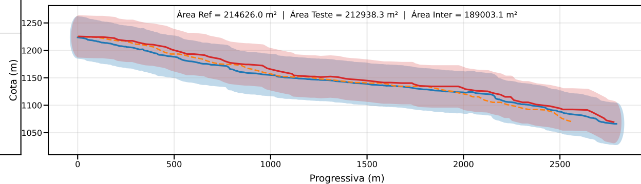
Classe D | PEC-PCD (Vertical)=37.5 m | EQ = 50m | dm = 14.18
