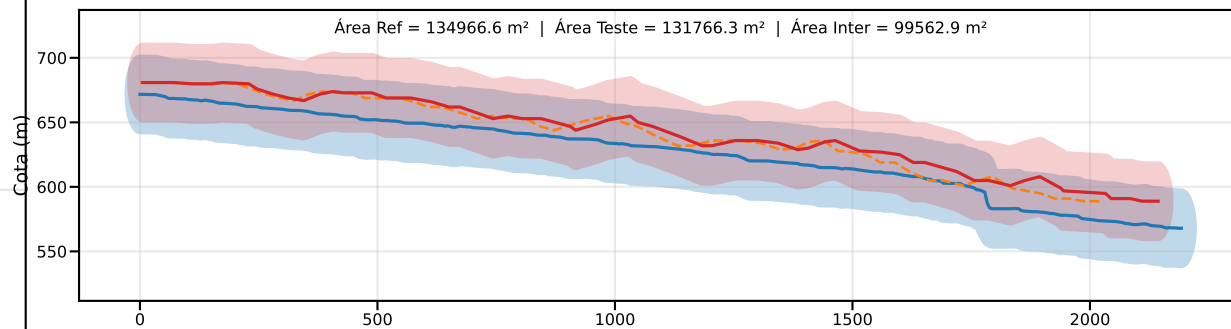
Classe D | PEC-PCD (Vertical)=37.5 m | EQ = 50m | dm = 25.83
