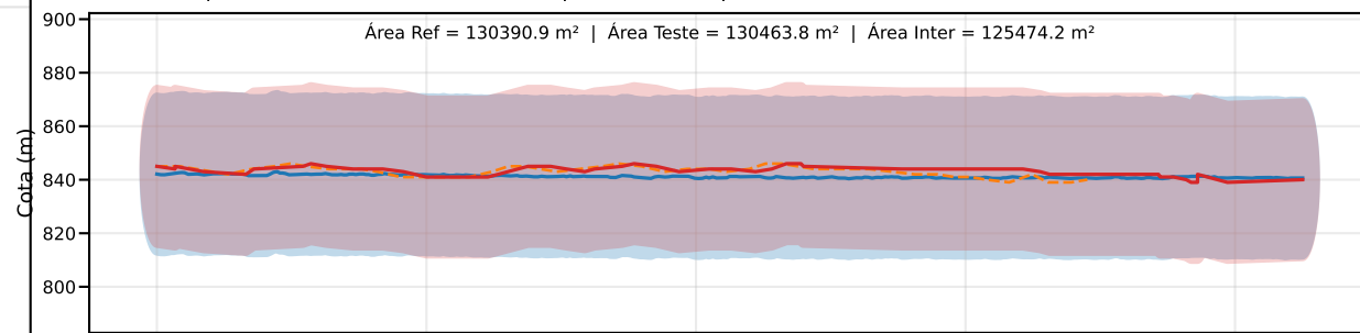
Classe D | PEC-PCD (Vertical)=37.5 m | EQ = 50m | dm = 3.55
