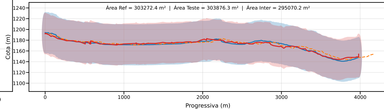
Classe D | PEC-PCD (Vertical)=37.5 m | EQ = 50m | dm = 3.18
