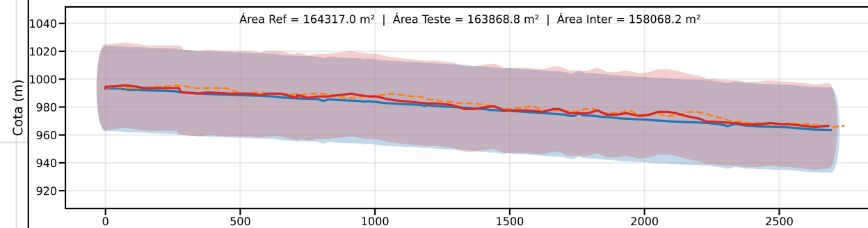
Classe D | PEC-PCD (Vertical)=37.5 m | EQ = 50m | dm = 3.66
