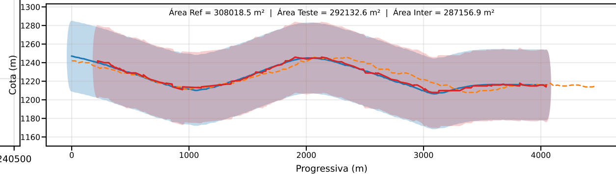
Classe D | PEC-PCD (Vertical)=37.5 m | EQ = 50m | dm = 8.41
