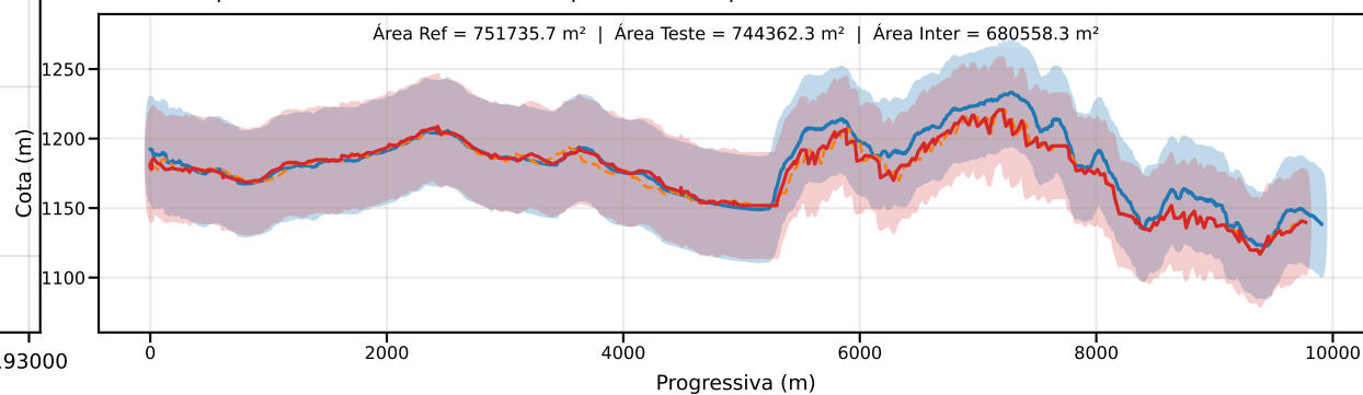
Classe D | PEC-PCD (Vertical)=37.5 m | EQ = 50m | dm = 11.27
