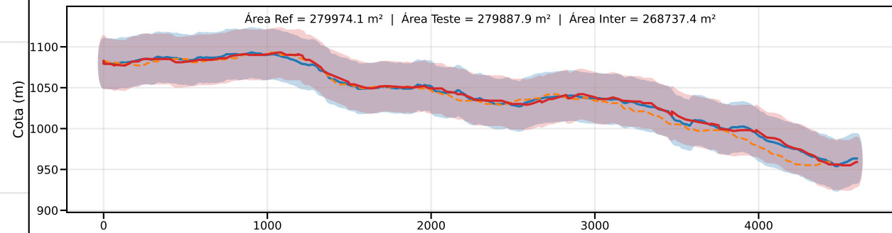
Classe D | PEC-PCD (Vertical)=37.5 m | EQ = 50m | dm = 3.79
