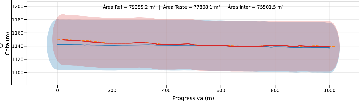
Classe D | PEC-PCD (Vertical)=37.5 m | EQ = 50m | dm = 5.68
