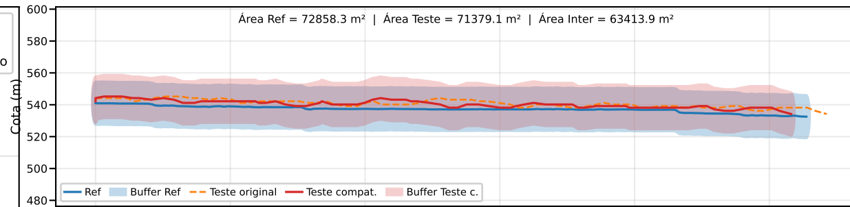
Classe B | PEC-PCD (Vertical)=25.0 m | EQ = 50m | dm = 6.42
