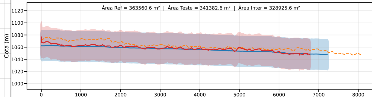
Classe C | PEC-PCD (Vertical)=30.0 m | EQ = 50m | dm = 9.01
