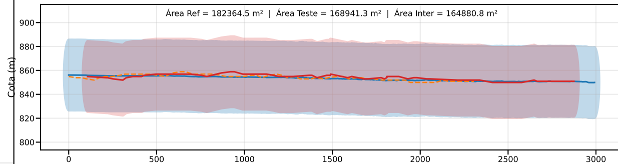
Classe D | PEC-PCD (Vertical)=37.5 m | EQ = 50m | dm = 11.58
