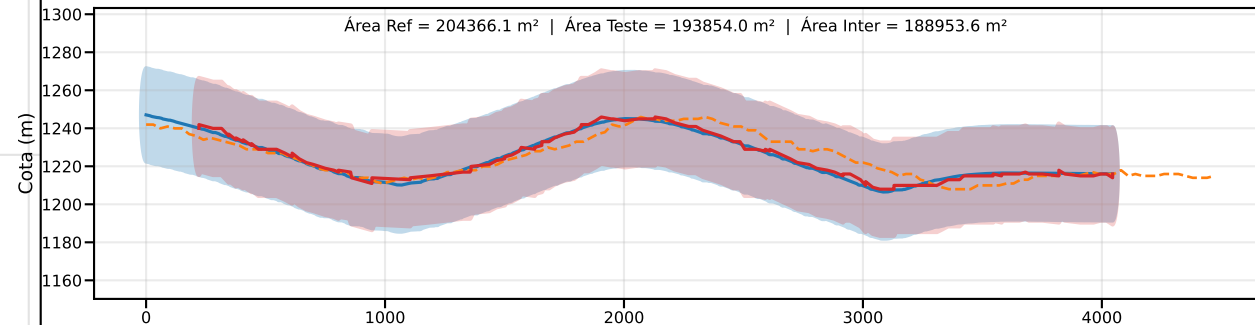
Classe C | PEC-PCD (Vertical)=30.0 m | EQ = 50m | dm = 7.11
