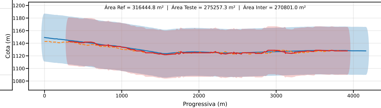
Classe D | PEC-PCD (Vertical)=37.5 m | EQ = 50m | dm = 19.54
