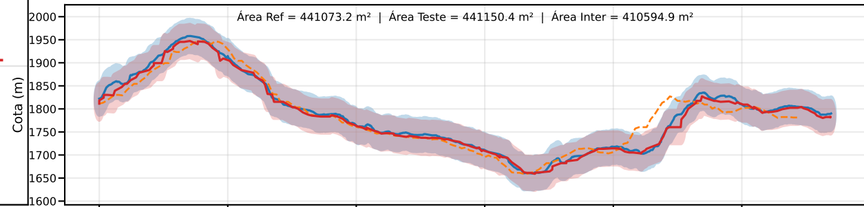
Classe D | PEC-PCD (Vertical)=37.5 m | EQ = 50m | dm = 8.14
