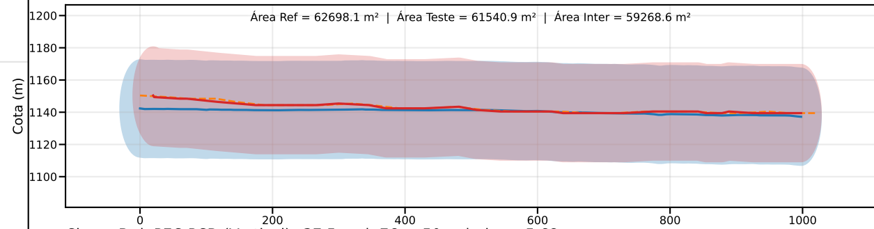
Classe D | PEC-PCD (Vertical)=37.5 m | EQ = 50m | dm = 5.68
