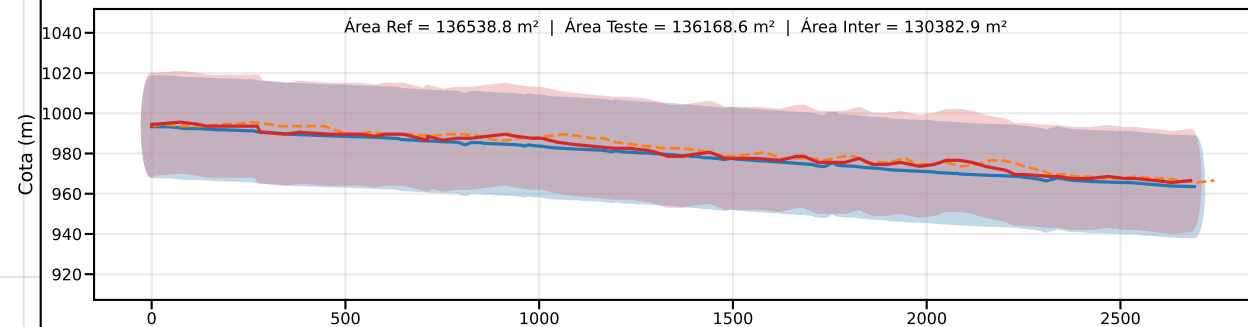
Classe C | PEC-PCD (Vertical)=30.0 m | EQ = 50m | dm = 3.59
