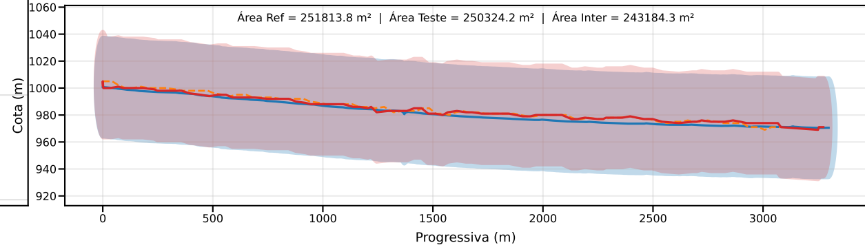
Classe D | PEC-PCD (Vertical)=37.5 m | EQ = 50m | dm = 4.06
