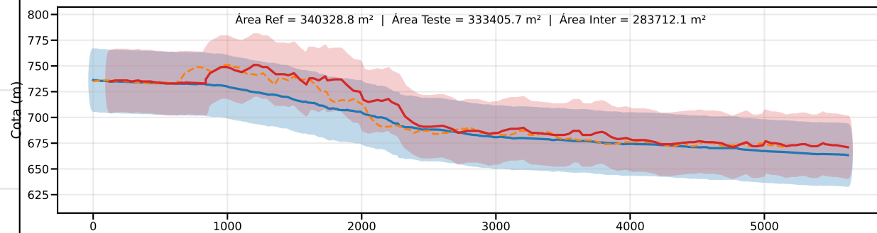
Classe D | PEC-PCD (Vertical)=37.5 m | EQ = 50m | dm = 16.50
