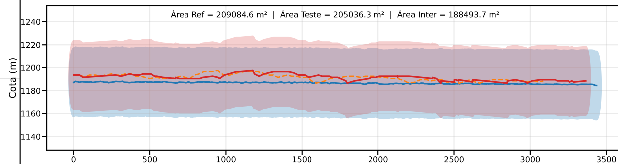
Classe D | PEC-PCD (Vertical)=37.5 m | EQ = 50m | dm = 9.93
