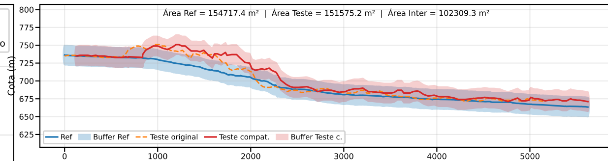
Classe B | PEC-PCD (Vertical)=25.0 m | EQ = 50m | dm = 15.67
