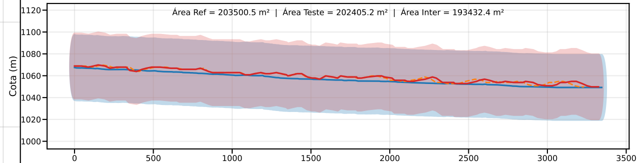
Classe D | PEC-PCD (Vertical)=37.5 m | EQ = 50m | dm = 4.81
