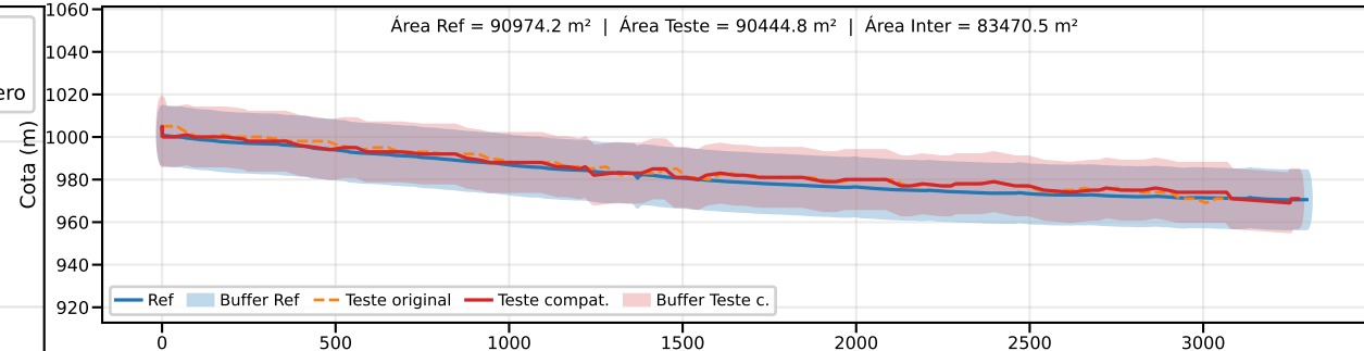
Classe B | PEC-PCD (Vertical)=25.0 m | EQ = 50m | dm = 3.80
