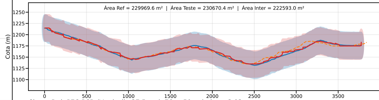
Classe D | PEC-PCD (Vertical)=37.5 m | EQ = 50m | dm = 3.03
