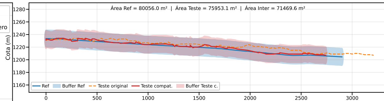
Classe B | PEC-PCD (Vertical)=25.0 m | EQ = 50m | dm = 6.85
