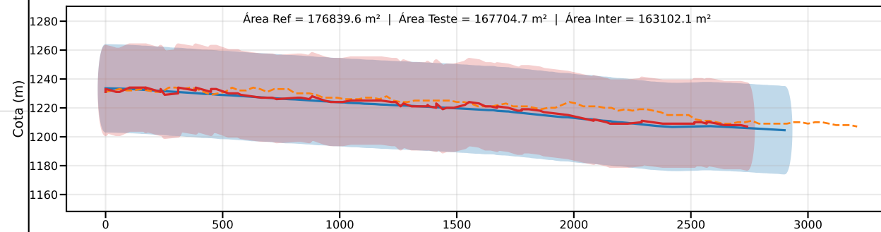
Classe D | PEC-PCD (Vertical)=37.5 m | EQ = 50m | dm = 9.02
