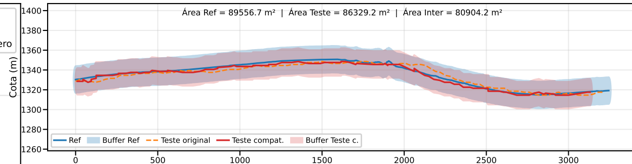
Classe B | PEC-PCD (Vertical)=25.0 m | EQ = 50m | dm = 5.67
