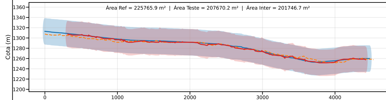
Classe C | PEC-PCD (Vertical)=30.0 m | EQ = 50m | dm = 10.46
