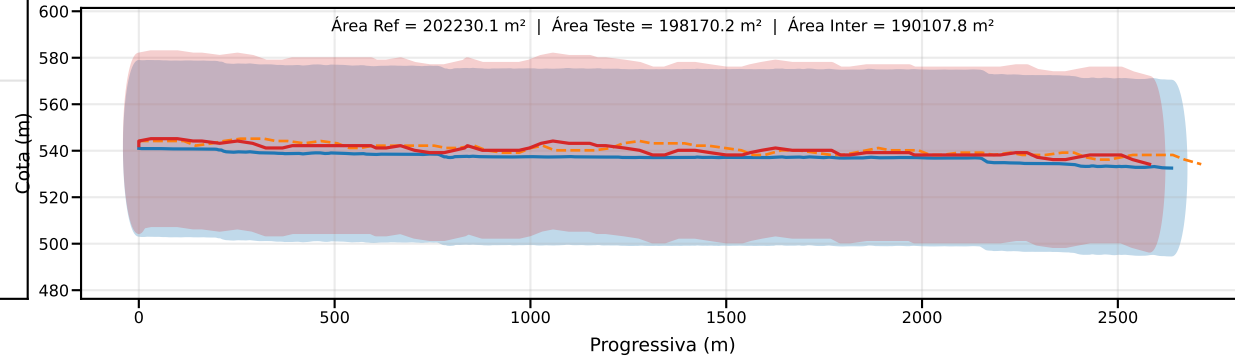
Classe D | PEC-PCD (Vertical)=37.5 m | EQ = 50m | dm = 7.21
