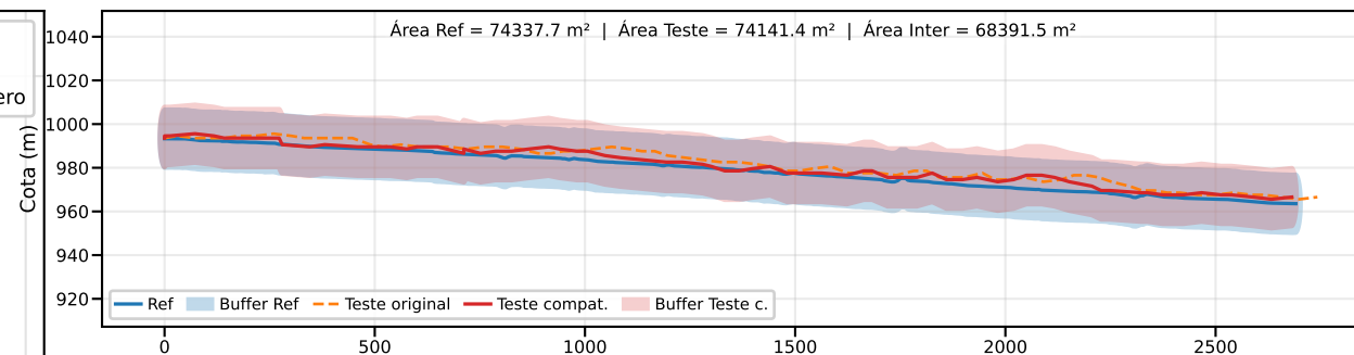
Classe B | PEC-PCD (Vertical)=25.0 m | EQ = 50m | dm = 3.55
