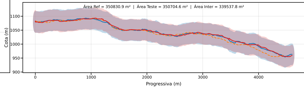
Classe D | PEC-PCD (Vertical)=37.5 m | EQ = 50m | dm = 3.79
