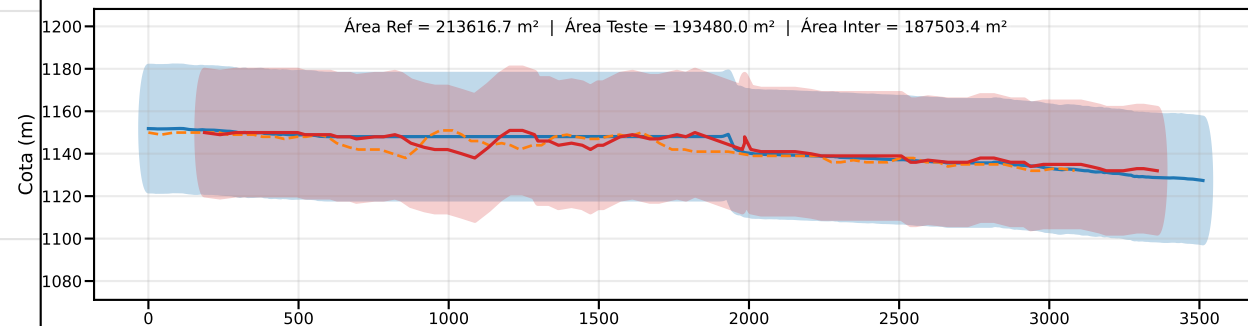
Classe D | PEC-PCD (Vertical)=37.5 m | EQ = 50m | dm = 15.14
