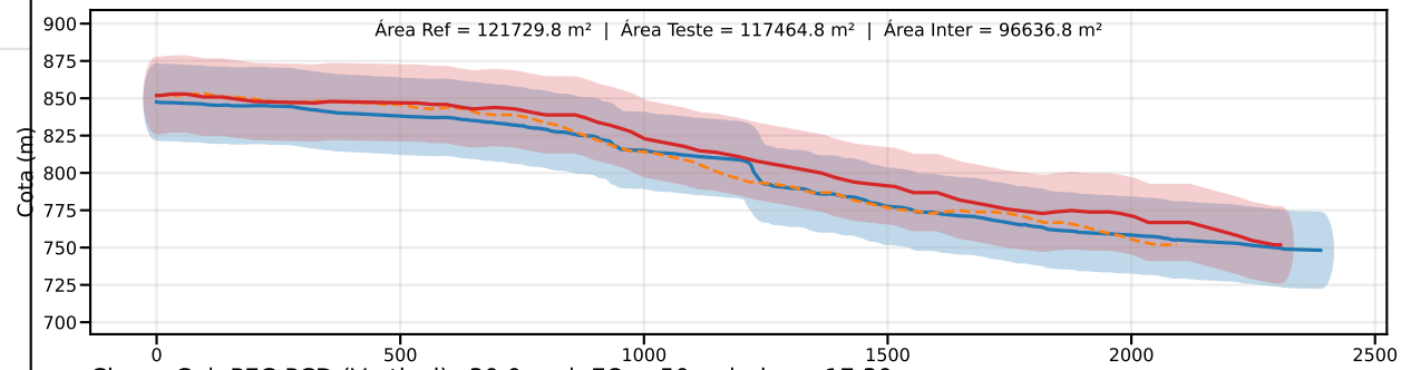
Classe C | PEC-PCD (Vertical)=30.0 m | EQ = 50m | dm = 17.30
