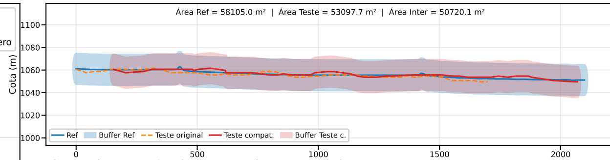
Classe B | PEC-PCD (Vertical)=25.0 m | EQ = 50m | dm = 9.26
