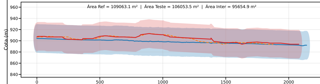
Classe C | PEC-PCD (Vertical)=30.0 m | EQ = 50m | dm = 10.36
