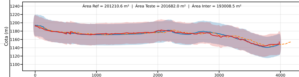
Classe C | PEC-PCD (Vertical)=30.0 m | EQ = 50m | dm = 3.19
