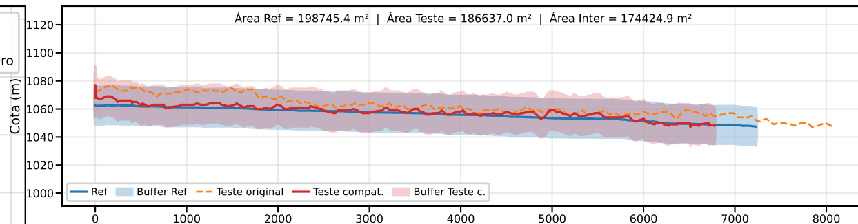
Classe B | PEC-PCD (Vertical)=25.0 m | EQ = 50m | dm = 7.97
