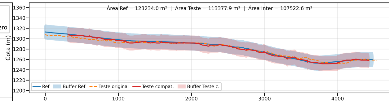
Classe B | PEC-PCD (Vertical)=25.0 m | EQ = 50m | dm = 9.08
