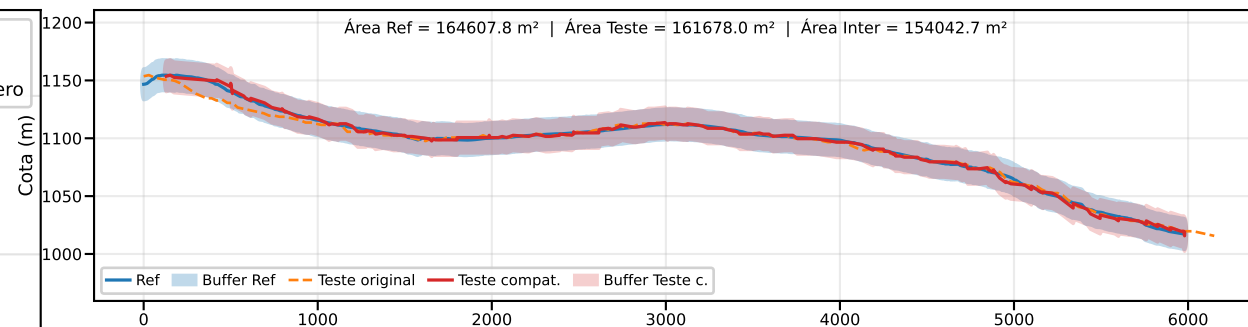
Classe B | PEC-PCD (Vertical)=25.0 m | EQ = 50m | dm = 3.56
