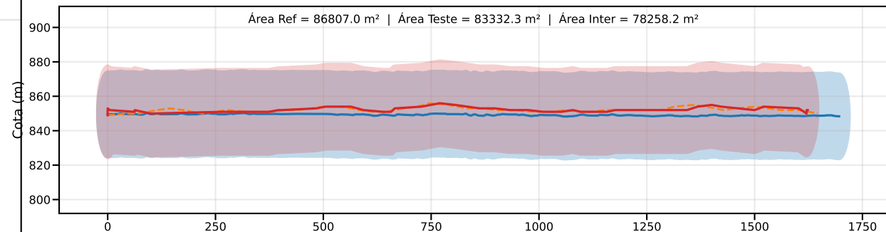
Classe C | PEC-PCD (Vertical)=30.0 m | EQ = 50m | dm = 8.70
