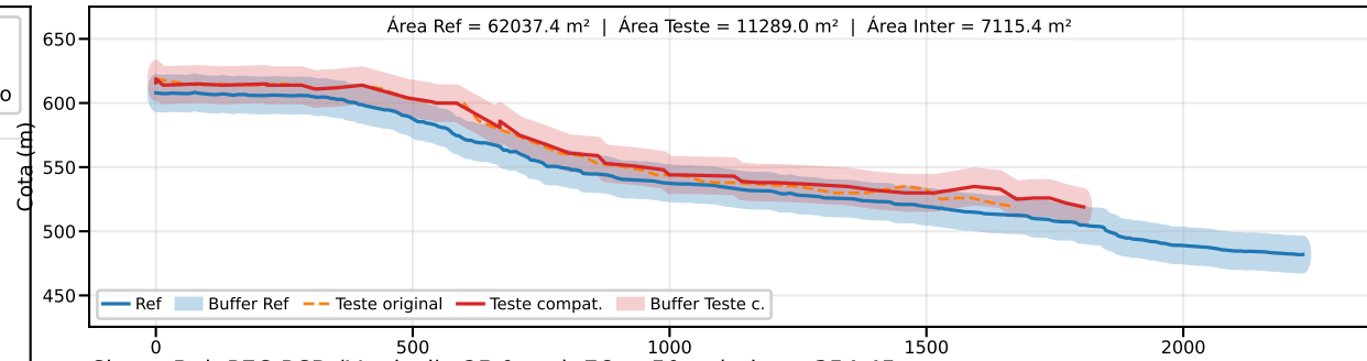
Classe B | PEC-PCD (Vertical)=25.0 m | EQ = 50m | dm = 354.45
