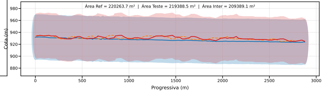
Classe D | PEC-PCD (Vertical)=37.5 m | EQ = 50m | dm = 5.84
