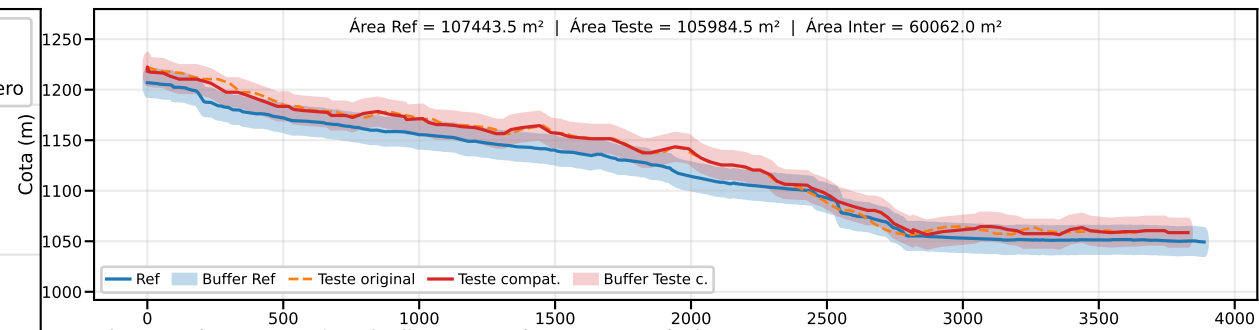
Classe B | PEC-PCD (Vertical)=25.0 m | EQ = 50m | dm = 19.75
