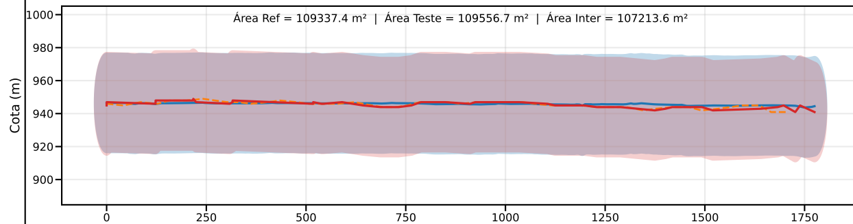
Classe D | PEC-PCD (Vertical)=37.5 m | EQ = 50m | dm = 1.83
