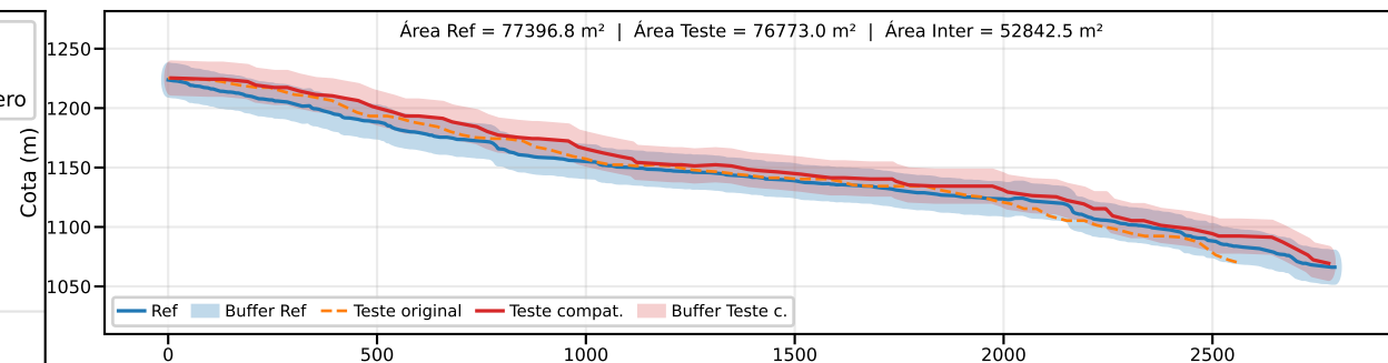
Classe B | PEC-PCD (Vertical)=25.0 m | EQ = 50m | dm = 13.96
