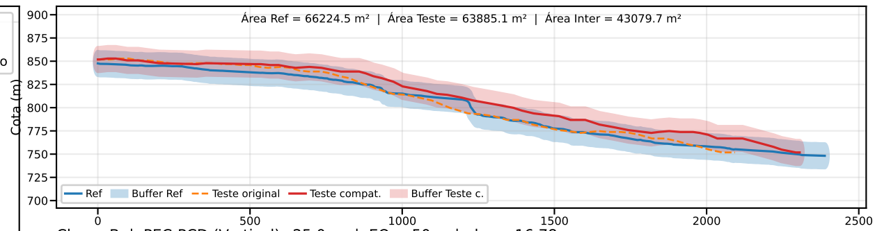
Classe B | PEC-PCD (Vertical)=25.0 m | EQ = 50m | dm = 16.78
