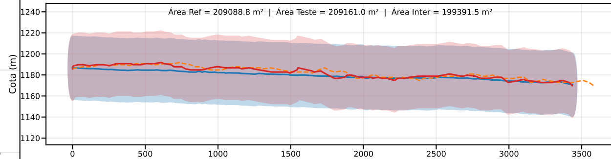
Classe D | PEC-PCD (Vertical)=37.5 m | EQ = 50m | dm = 4.36
