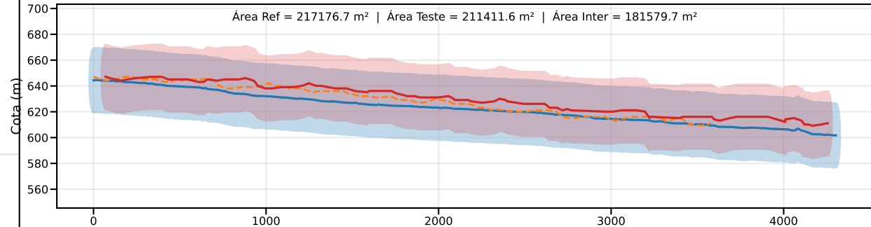
Classe C | PEC-PCD (Vertical)=30.0 m | EQ = 50m | dm = 13.64
