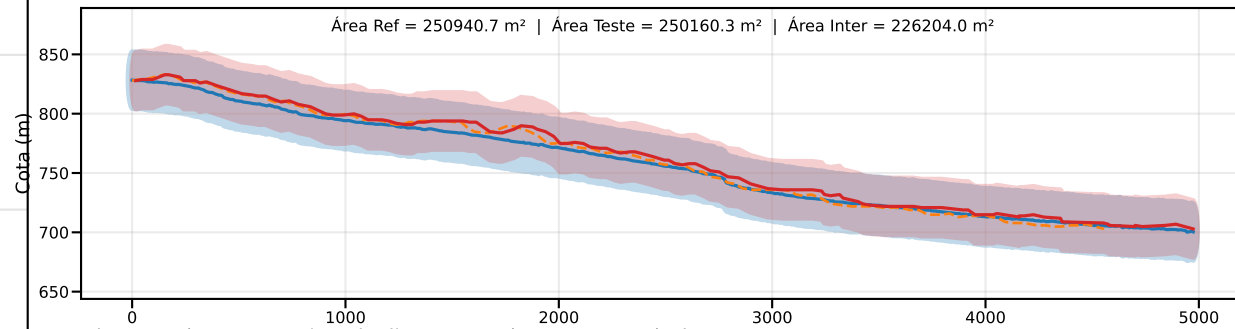
Classe C | PEC-PCD (Vertical)=30.0 m | EQ = 50m | dm = 7.81
