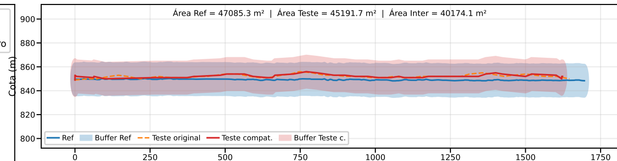
Classe B | PEC-PCD (Vertical)=25.0 m | EQ = 50m | dm = 8.06
