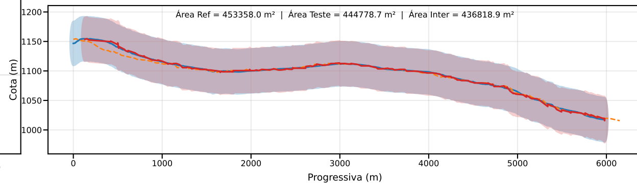
Classe D | PEC-PCD (Vertical)=37.5 m | EQ = 50m | dm = 4.38
