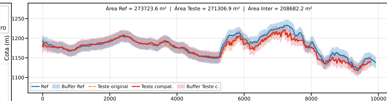
Classe B | PEC-PCD (Vertical)=25.0 m | EQ = 50m | dm = 10.77
