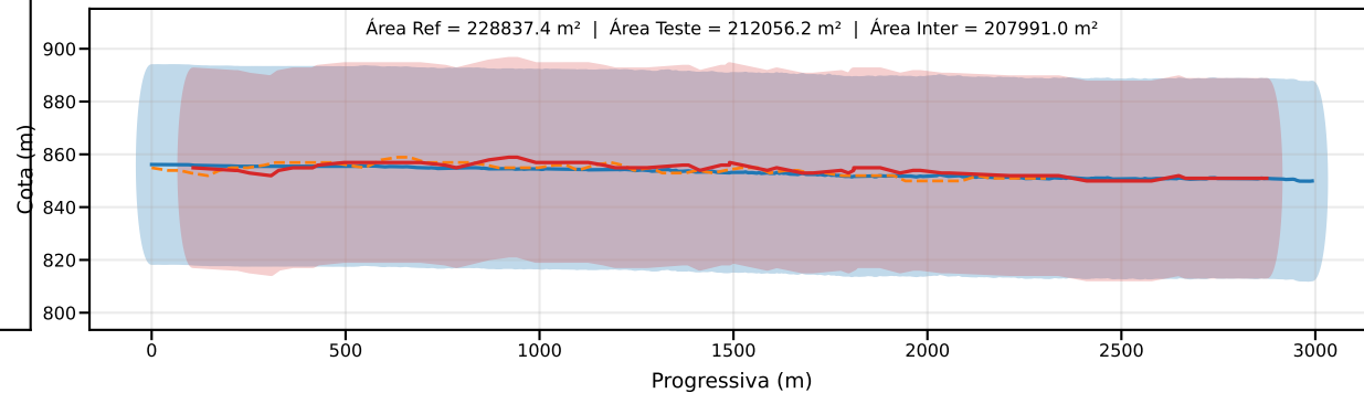
Classe D | PEC-PCD (Vertical)=37.5 m | EQ = 50m | dm = 11.58
