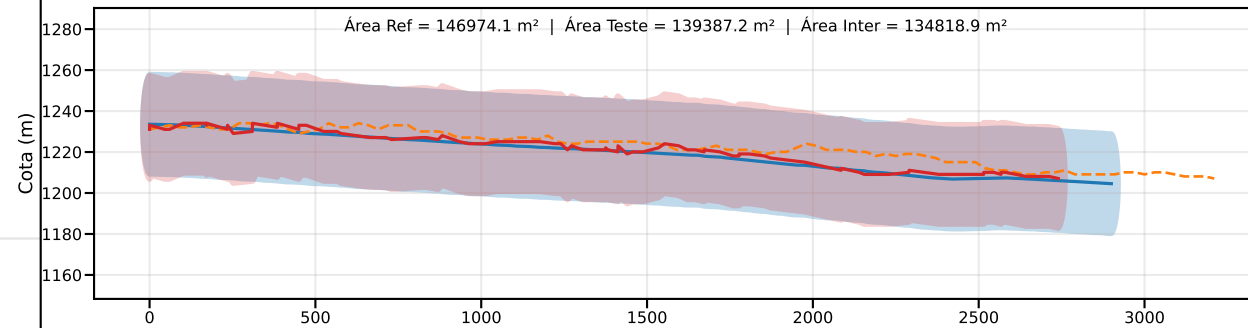
Classe C | PEC-PCD (Vertical)=30.0 m | EQ = 50m | dm = 7.72
