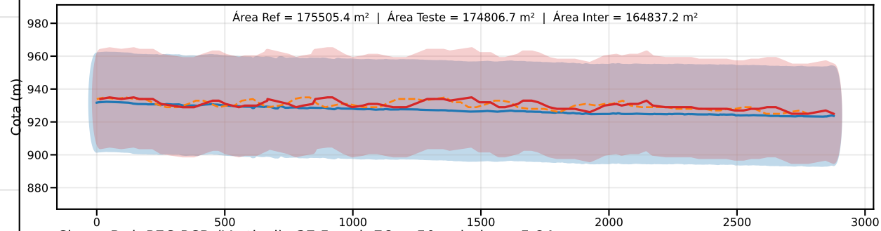
Classe D | PEC-PCD (Vertical)=37.5 m | EQ = 50m | dm = 5.84
