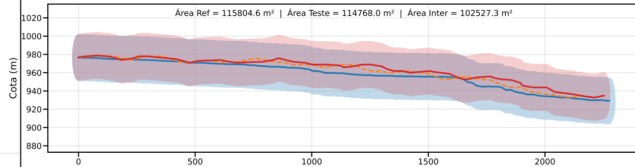
Classe C | PEC-PCD (Vertical)=30.0 m | EQ = 50m | dm = 9.21
