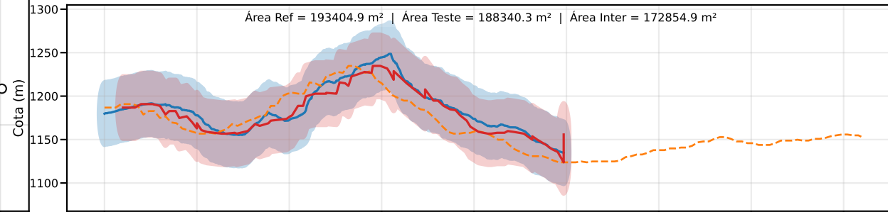
Classe D | PEC-PCD (Vertical)=37.5 m | EQ = 50m | dm = 12.85
