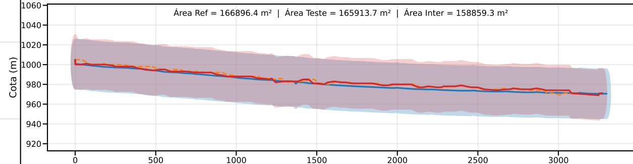
Classe C | PEC-PCD (Vertical)=30.0 m | EQ = 50m | dm = 3.91
