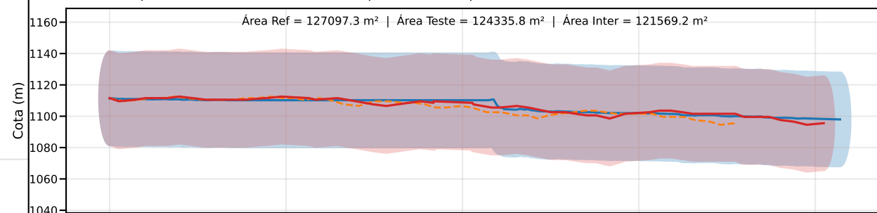
Classe D | PEC-PCD (Vertical)=37.5 m | EQ = 50m | dm = 4.69
