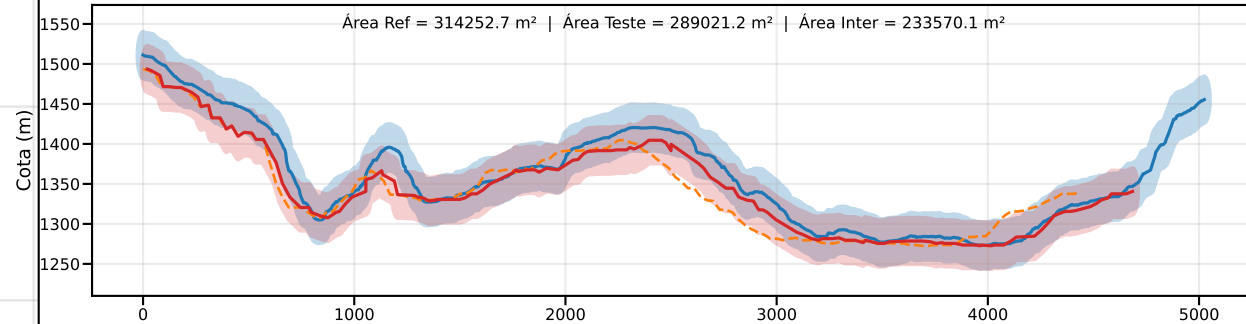
Classe D | PEC-PCD (Vertical)=37.5 m | EQ = 50m | dm = 28.24
