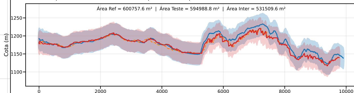
Classe D | PEC-PCD (Vertical)=37.5 m | EQ = 50m | dm = 11.27
