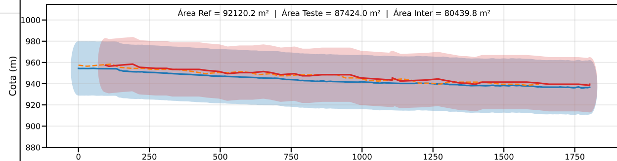
Classe C | PEC-PCD (Vertical)=30.0 m | EQ = 50m | dm = 11.31
