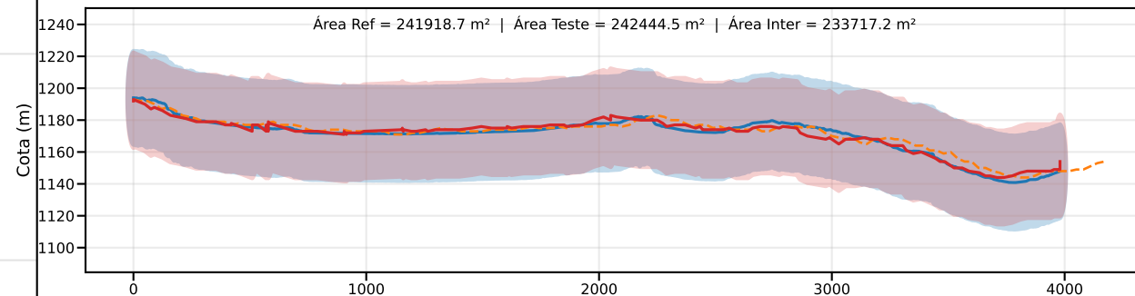
Classe D | PEC-PCD (Vertical)=37.5 m | EQ = 50m | dm = 3.18
