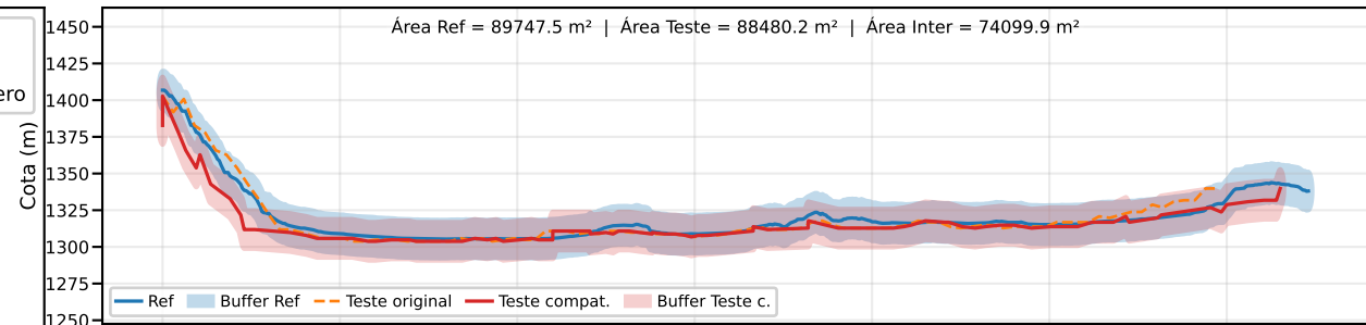
Classe B | PEC-PCD (Vertical)=25.0 m | EQ = 50m | dm = 8.41
