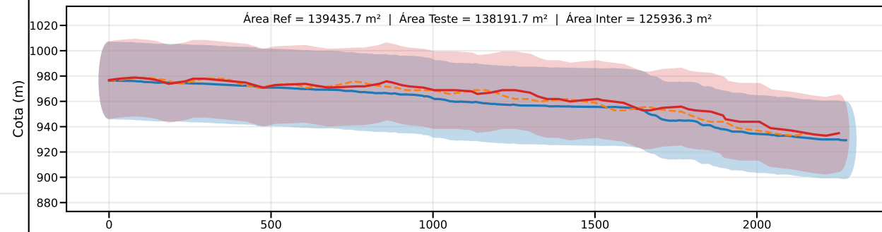
Classe D | PEC-PCD (Vertical)=37.5 m | EQ = 50m | dm = 9.39
