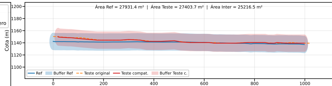
Classe B | PEC-PCD (Vertical)=25.0 m | EQ = 50m | dm = 4.96
