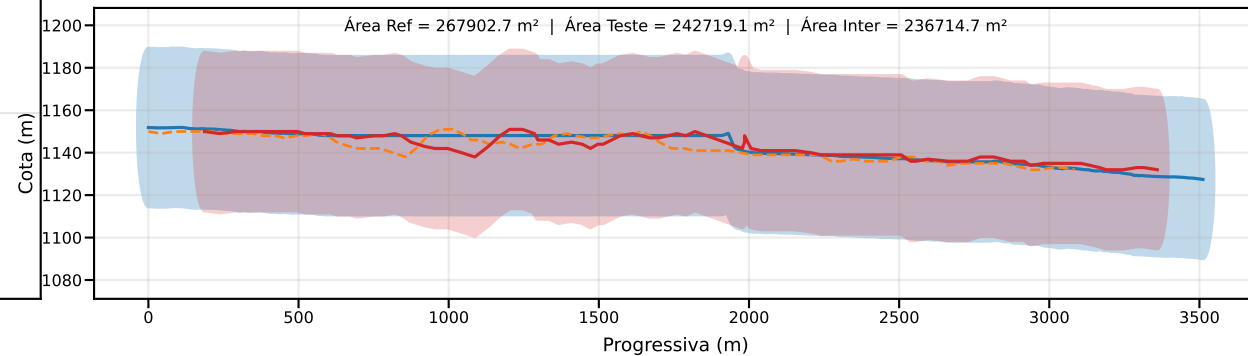
Classe D | PEC-PCD (Vertical)=37.5 m | EQ = 50m | dm = 15.14
