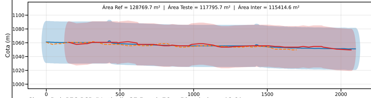
Classe D | PEC-PCD (Vertical)=37.5 m | EQ = 50m | dm = 12.81
