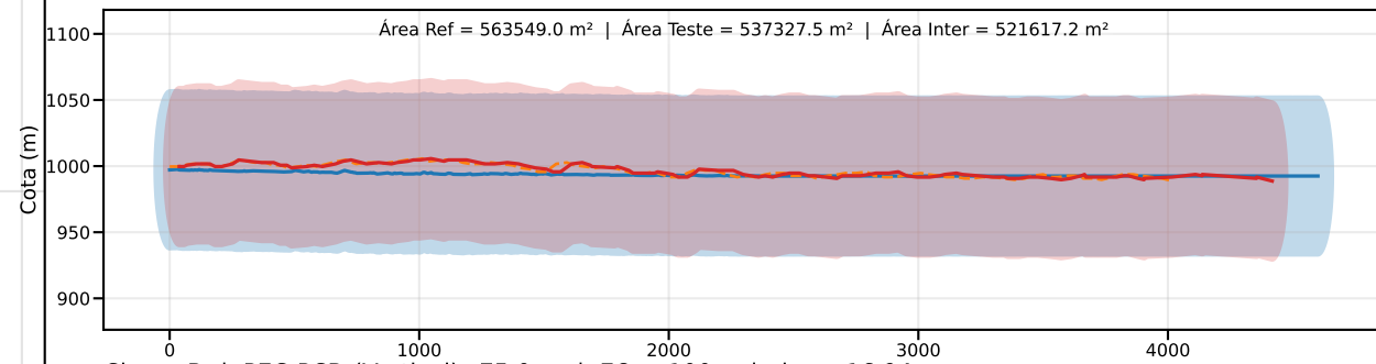
Classe D | PEC-PCD (Vertical)=75.0 m | EQ = 100m | dm = 16.94
