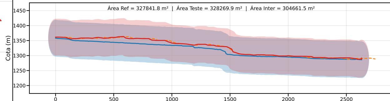
Classe D | PEC-PCD (Vertical)=75.0 m | EQ = 100m | dm = 13.23
