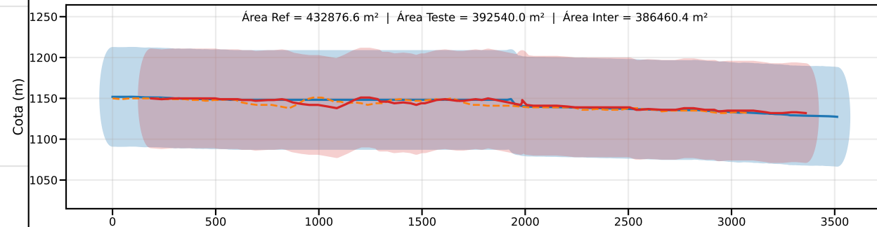
Classe D | PEC-PCD (Vertical)=75.0 m | EQ = 100m | dm = 26.97
