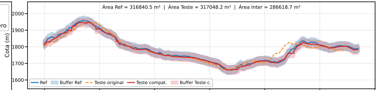
Classe B | PEC-PCD (Vertical)=50.0 m | EQ = 100m | dm = 8.21
