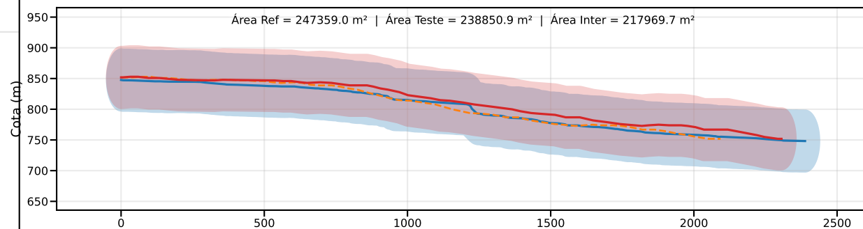
Classe C | PEC-PCD (Vertical)=60.0 m | EQ = 100m | dm = 20.32
