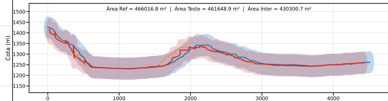
Classe C | PEC-PCD (Vertical)=60.0 m | EQ = 100m | dm = 12.76
