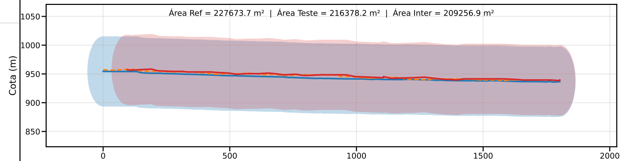
Classe D | PEC-PCD (Vertical)=75.0 m | EQ = 100m | dm = 18.32
