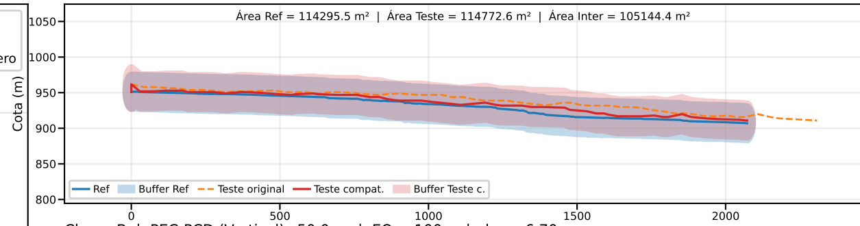
Classe B | PEC-PCD (Vertical)=50.0 m | EQ = 100m | dm = 6.70
