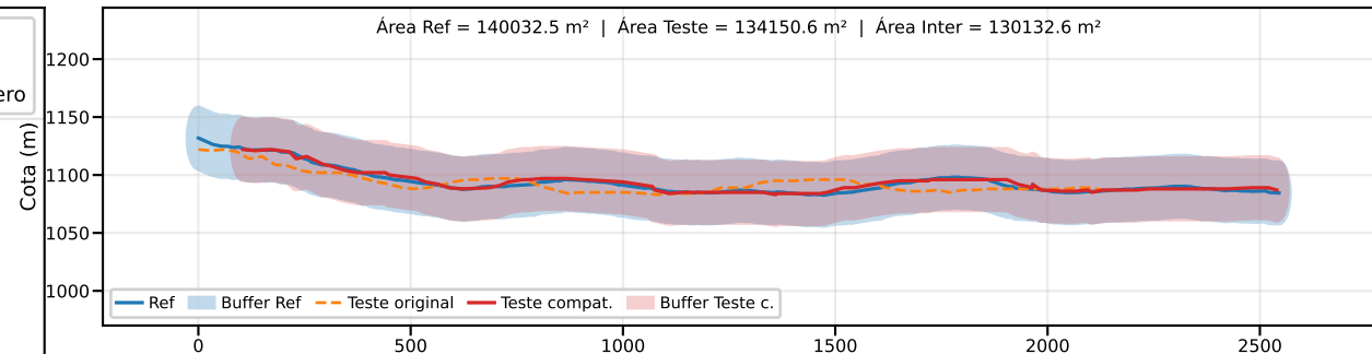
Classe B | PEC-PCD (Vertical)=50.0 m | EQ = 100m | dm = 9.34
