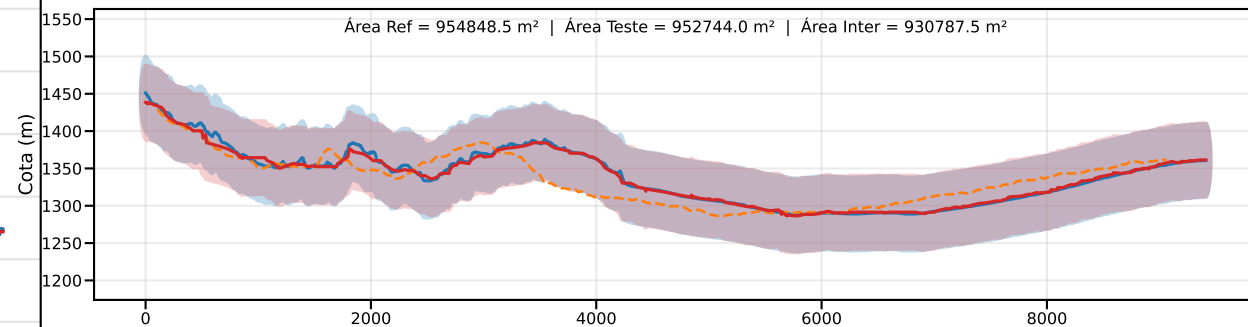
Classe C | PEC-PCD (Vertical)=60.0 m | EQ = 100m | dm = 4.02
