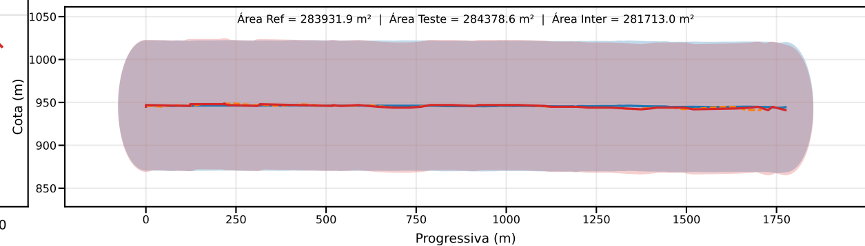
Classe D | PEC-PCD (Vertical)=75.0 m | EQ = 100m | dm = 1.84
