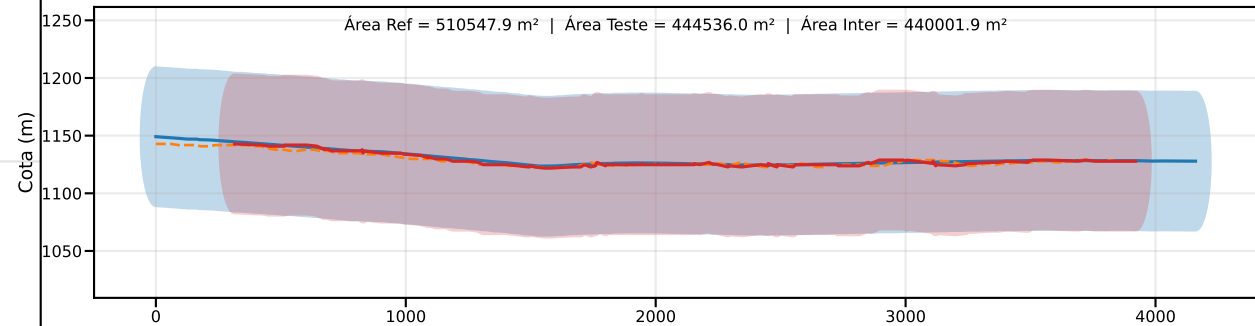
Classe D | PEC-PCD (Vertical)=75.0 m | EQ = 100m | dm = 36.73
