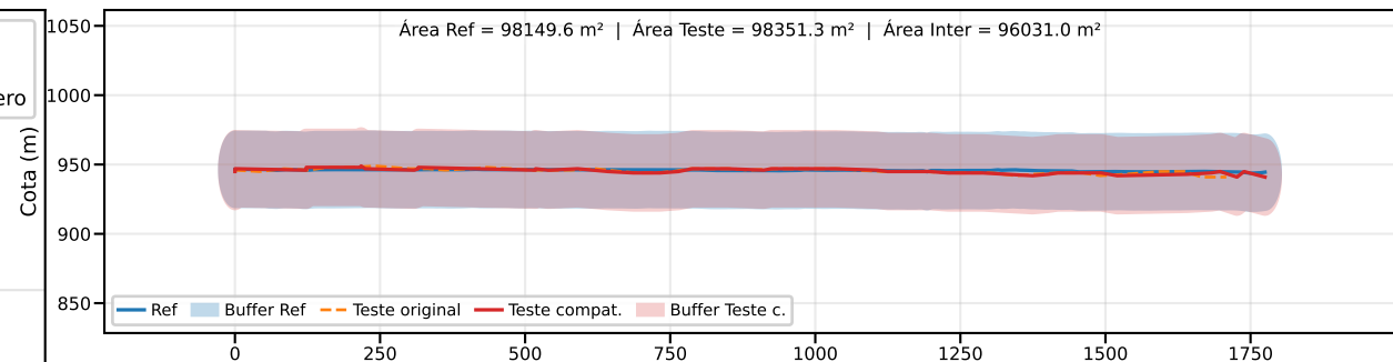
Classe B | PEC-PCD (Vertical)=50.0 m | EQ = 100m | dm = 1.83
