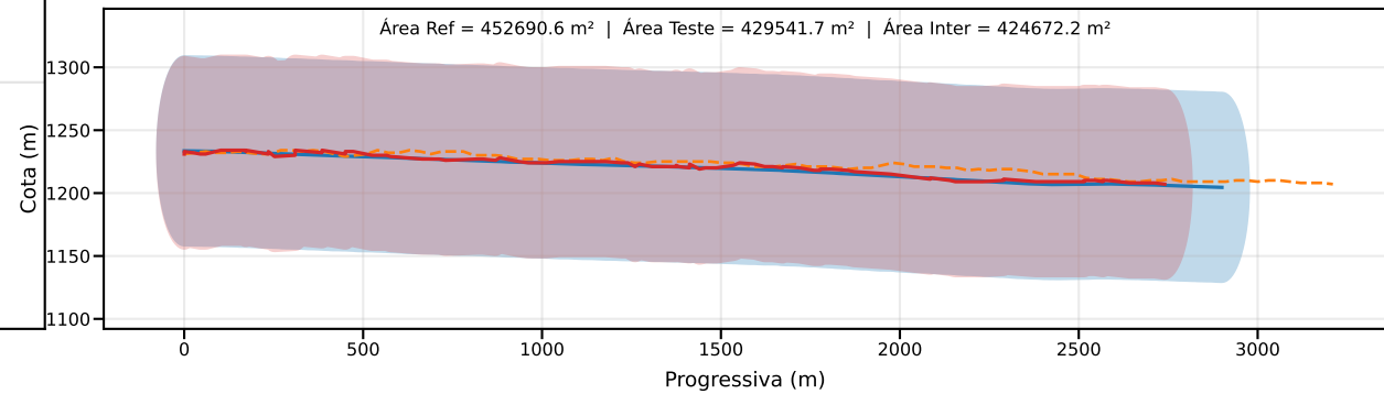
Classe D | PEC-PCD (Vertical)=75.0 m | EQ = 100m | dm = 15.37
