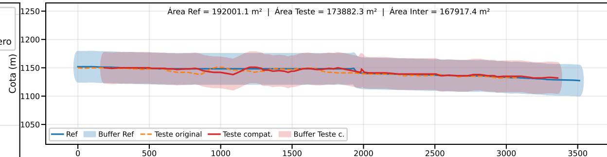
Classe B | PEC-PCD (Vertical)=50.0 m | EQ = 100m | dm = 19.13
