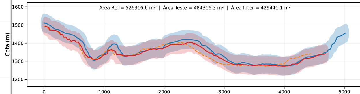
Classe C | PEC-PCD (Vertical)=60.0 m | EQ = 100m | dm = 33.94
