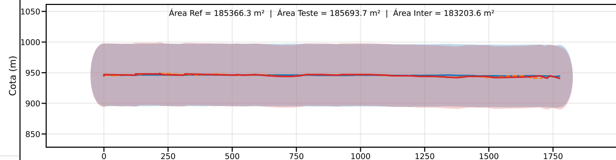
Classe C | PEC-PCD (Vertical)=60.0 m | EQ = 100m | dm = 1.83
