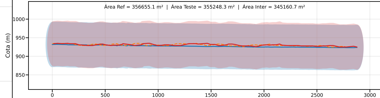
Classe D | PEC-PCD (Vertical)=75.0 m | EQ = 100m | dm = 6.27
