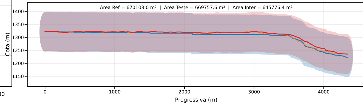
Classe D | PEC-PCD (Vertical)=75.0 m | EQ = 100m | dm = 8.56
