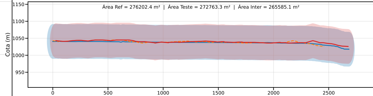
Classe C | PEC-PCD (Vertical)=60.0 m | EQ = 100m | dm = 6.50
