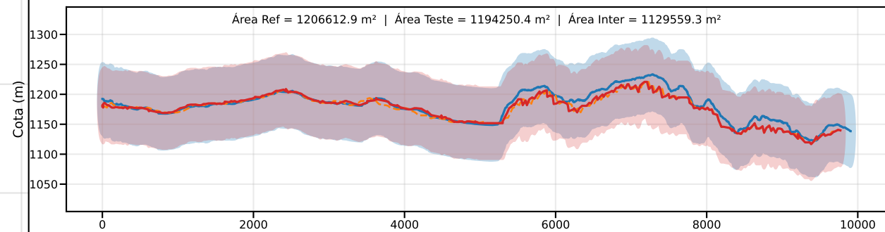
Classe D | PEC-PCD (Vertical)=75.0 m | EQ = 100m | dm = 12.77
