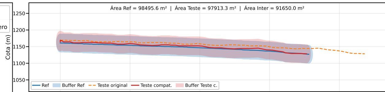
Classe B | PEC-PCD (Vertical)=50.0 m | EQ = 100m | dm = 6.45
