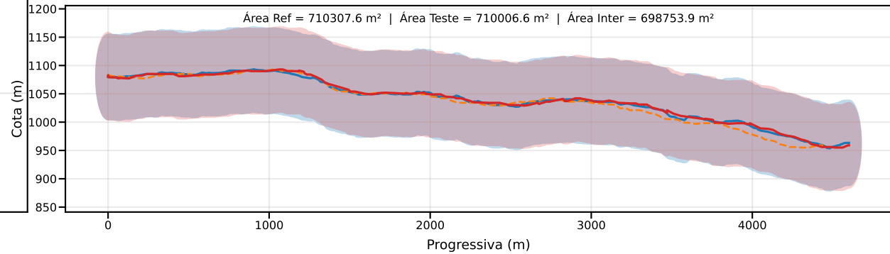
Classe D | PEC-PCD (Vertical)=75.0 m | EQ = 100m | dm = 3.83
