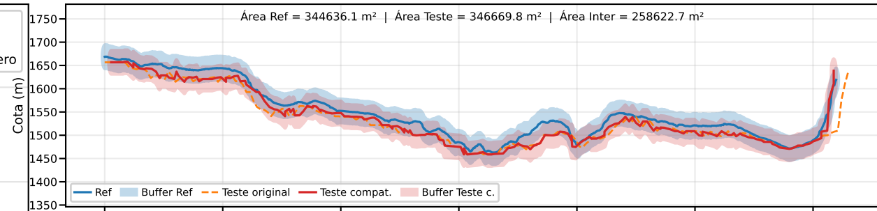
Classe B | PEC-PCD (Vertical)=50.0 m | EQ = 100m | dm = 21.47
