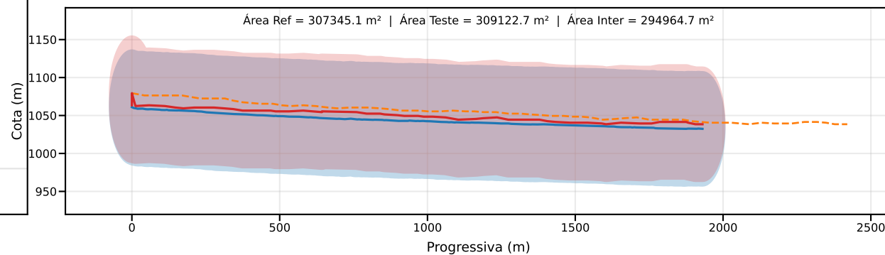
Classe D | PEC-PCD (Vertical)=75.0 m | EQ = 100m | dm = 9.44
