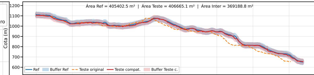
Classe B | PEC-PCD (Vertical)=50.0 m | EQ = 100m | dm = 7.50
