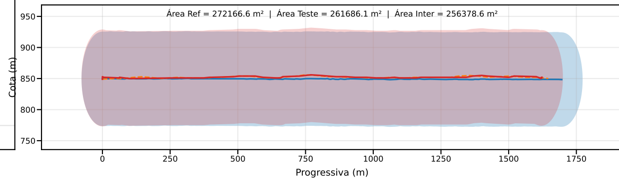
Classe D | PEC-PCD (Vertical)=75.0 m | EQ = 100m | dm = 14.22
