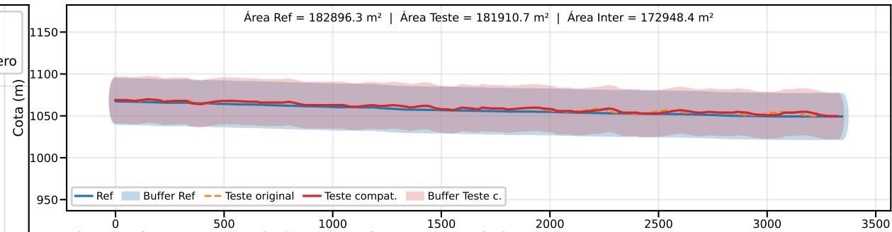
Classe B | PEC-PCD (Vertical)=50.0 m | EQ = 100m | dm = 5.01
