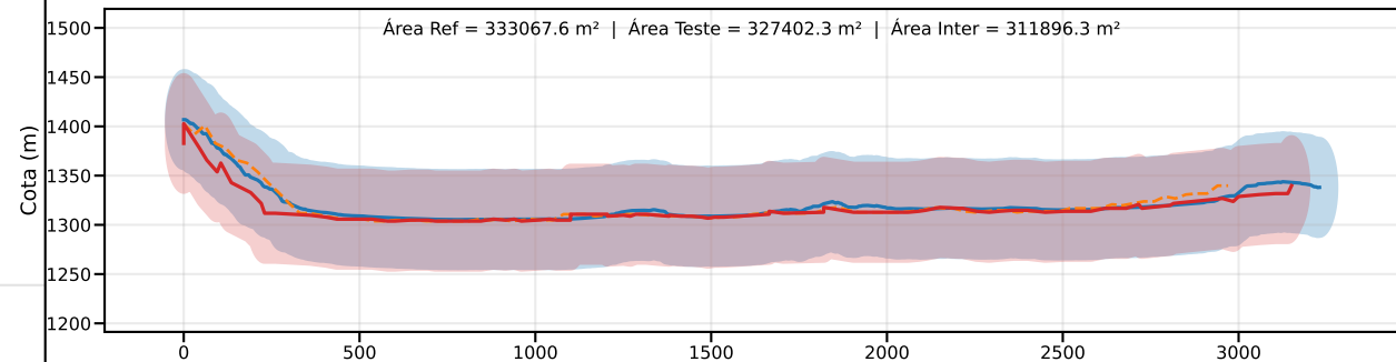
Classe C | PEC-PCD (Vertical)=60.0 m | EQ = 100m | dm = 10.85
