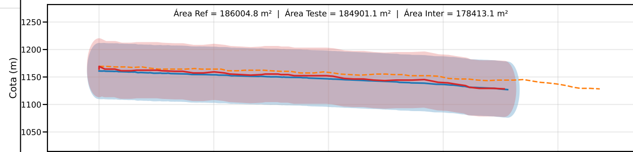
Classe C | PEC-PCD (Vertical)=60.0 m | EQ = 100m | dm = 6.67
