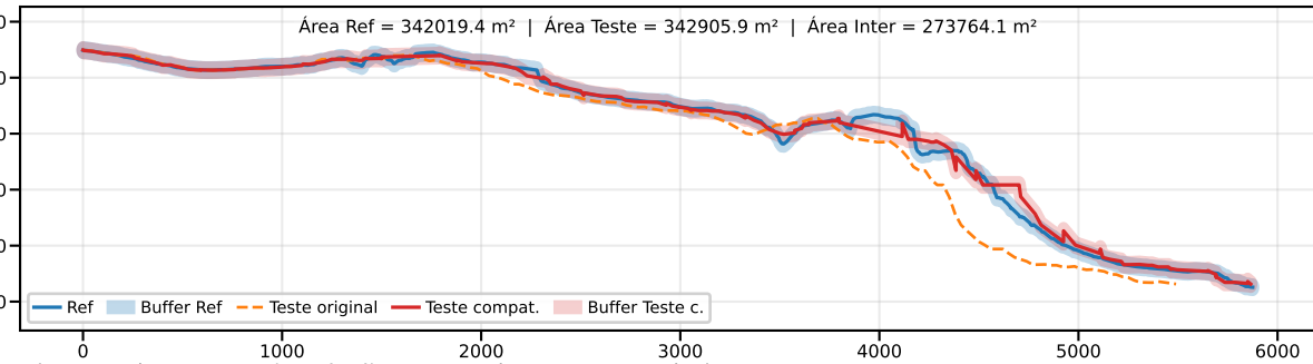
Classe B | PEC-PCD (Vertical)=50.0 m | EQ = 100m | dm = 17.59
