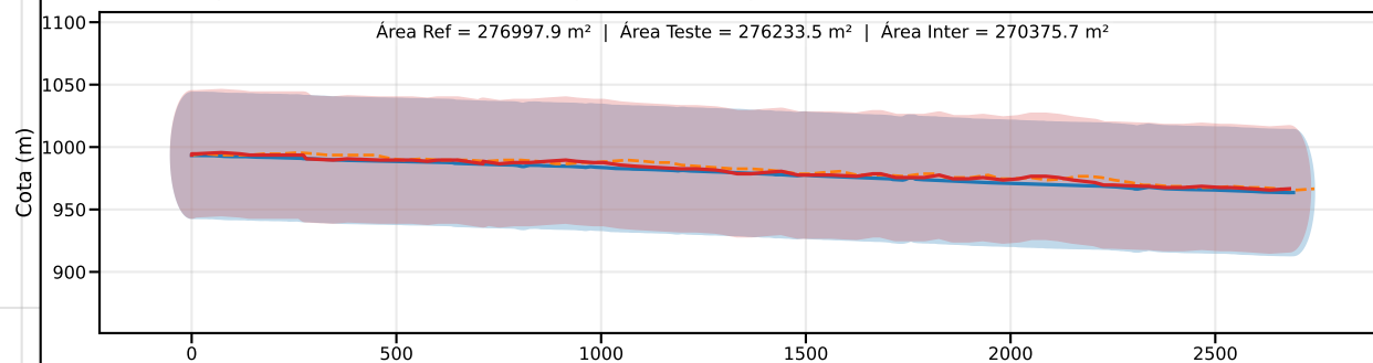
Classe C | PEC-PCD (Vertical)=60.0 m | EQ = 100m | dm = 3.85
