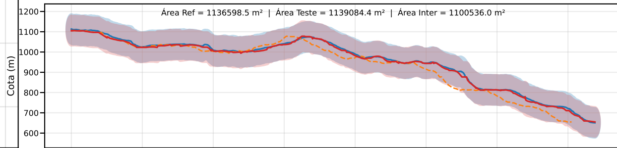
Classe D | PEC-PCD (Vertical)=75.0 m | EQ = 100m | dm = 7.46
