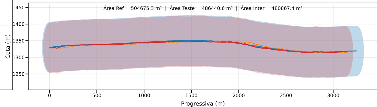
Classe D | PEC-PCD (Vertical)=75.0 m | EQ = 100m | dm = 11.53
