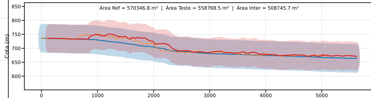
Classe C | PEC-PCD (Vertical)=60.0 m | EQ = 100m | dm = 17.97
