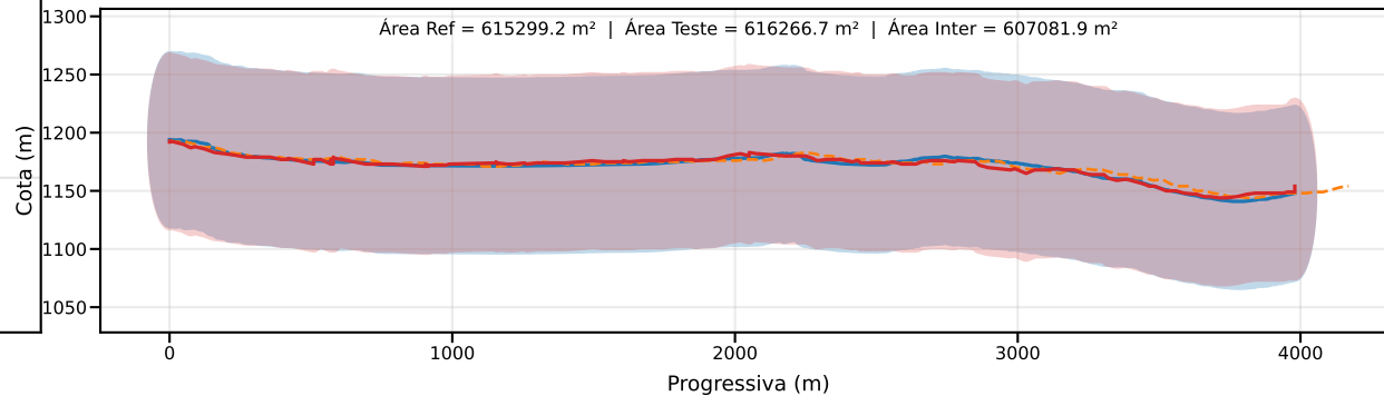
Classe D | PEC-PCD (Vertical)=75.0 m | EQ = 100m | dm = 3.14
