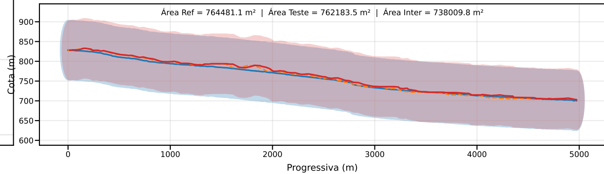
Classe D | PEC-PCD (Vertical)=75.0 m | EQ = 100m | dm = 8.18
