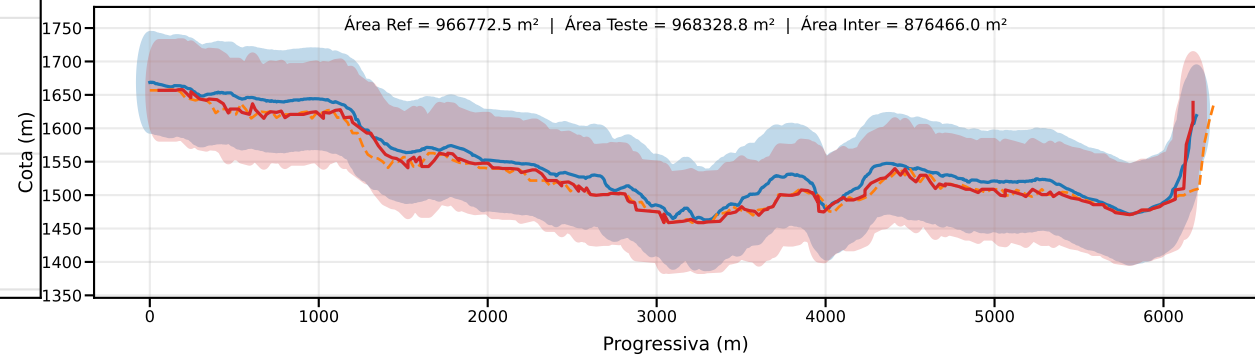
Classe D | PEC-PCD (Vertical)=75.0 m | EQ = 100m | dm = 21.97
