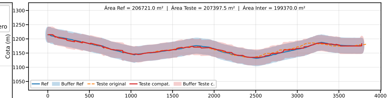
Classe B | PEC-PCD (Vertical)=50.0 m | EQ = 100m | dm = 3.07
