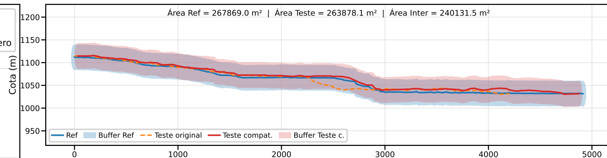
Classe B | PEC-PCD (Vertical)=50.0 m | EQ = 100m | dm = 9.93
