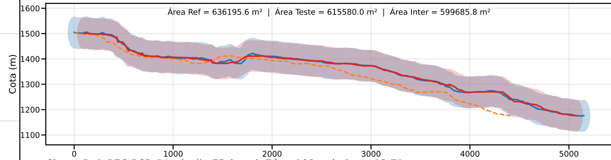
Classe D | PEC-PCD (Vertical)=75.0 m | EQ = 100m | dm = 12.71
