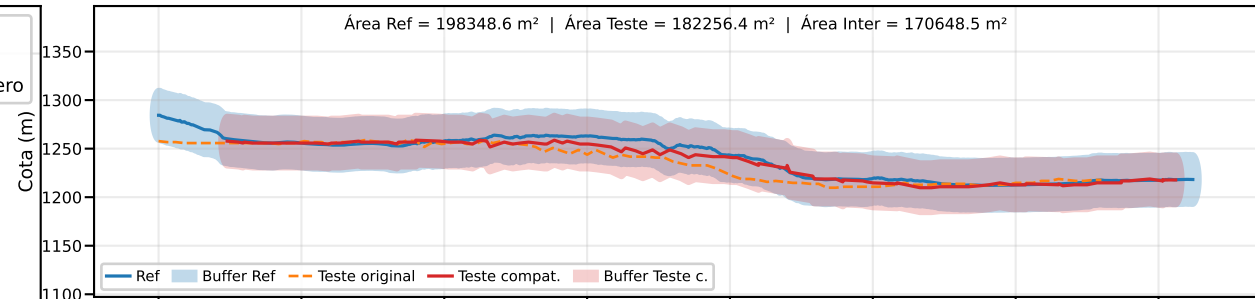
Classe B | PEC-PCD (Vertical)=50.0 m | EQ = 100m | dm = 19.15
