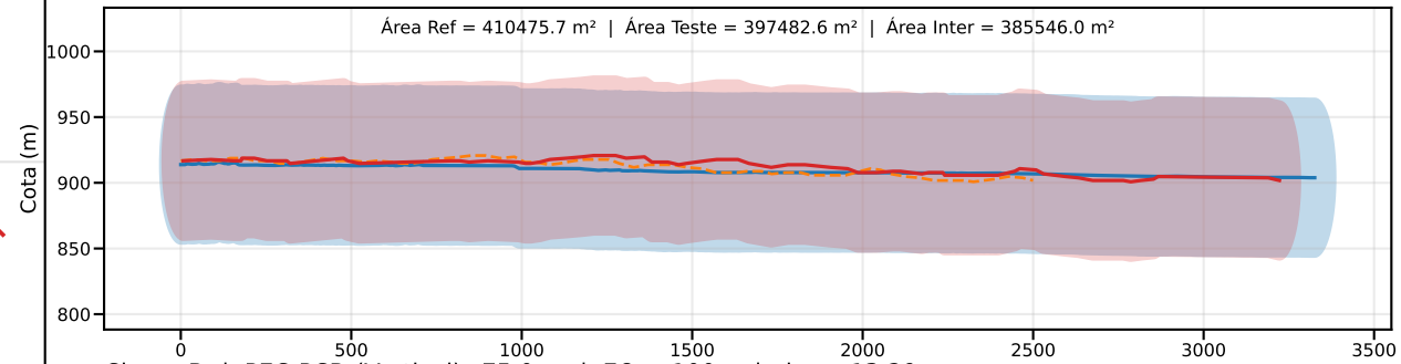
Classe D | PEC-PCD (Vertical)=75.0 m | EQ = 100m | dm = 13.29
