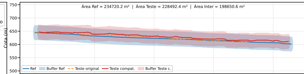
Classe B | PEC-PCD (Vertical)=50.0 m | EQ = 100m | dm = 15.27
