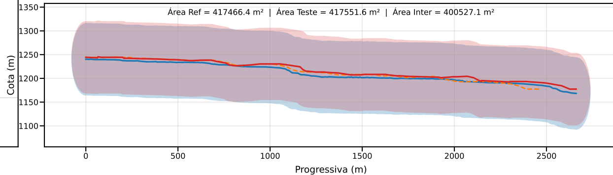
Classe D | PEC-PCD (Vertical)=75.0 m | EQ = 100m | dm = 9.56
