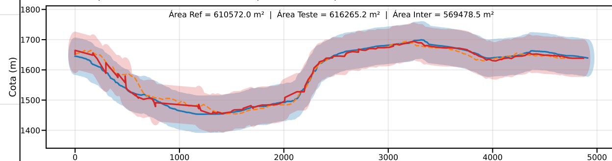
Classe D | PEC-PCD (Vertical)=75.0 m | EQ = 100m | dm = 12.75
