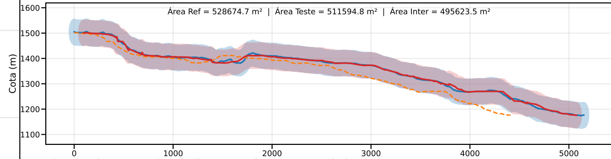
Classe C | PEC-PCD (Vertical)=60.0 m | EQ = 100m | dm = 11.18
