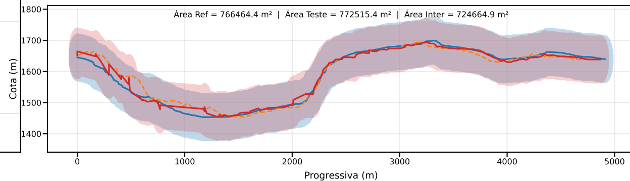
Classe D | PEC-PCD (Vertical)=75.0 m | EQ = 100m | dm = 12.75
