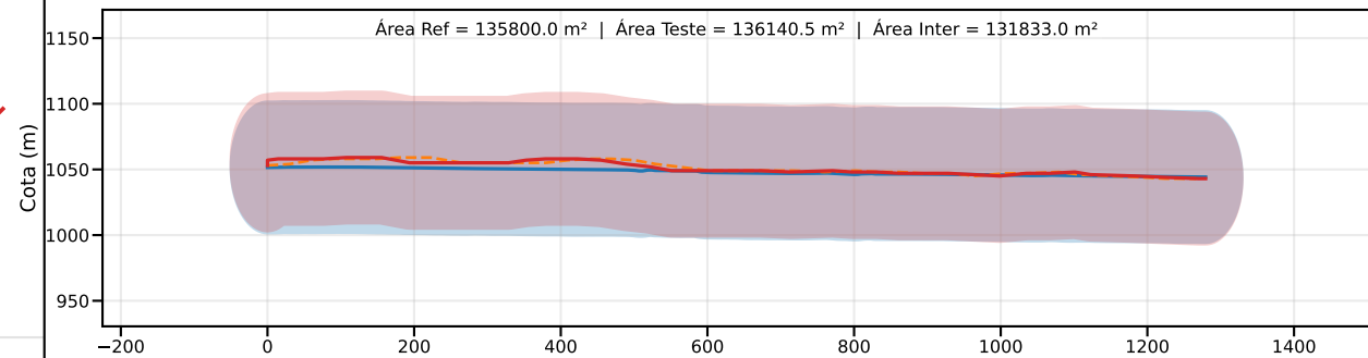
Classe C | PEC-PCD (Vertical)=60.0 m | EQ = 100m | dm = 4.54
