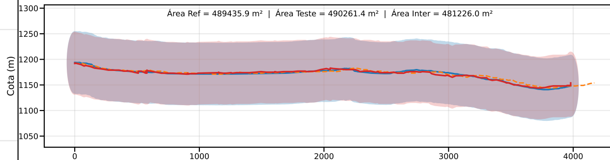
Classe D | PEC-PCD (Vertical)=75.0 m | EQ = 100m | dm = 3.14
