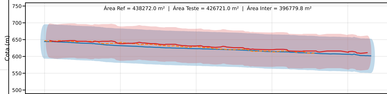
Classe C | PEC-PCD (Vertical)=60.0 m | EQ = 100m | dm = 16.08
