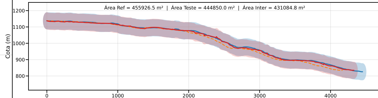
Classe C | PEC-PCD (Vertical)=60.0 m | EQ = 100m | dm = 9.58
