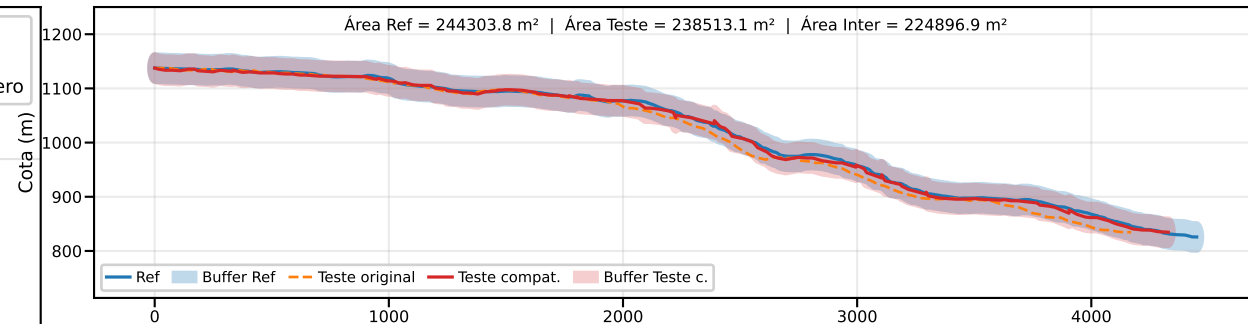
Classe B | PEC-PCD (Vertical)=50.0 m | EQ = 100m | dm = 8.77
