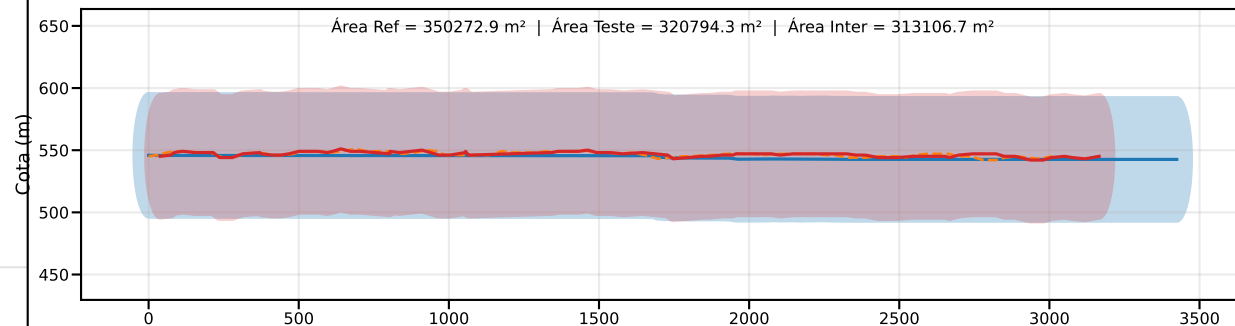
Classe C | PEC-PCD (Vertical)=60.0 m | EQ = 100m | dm = 21.00
