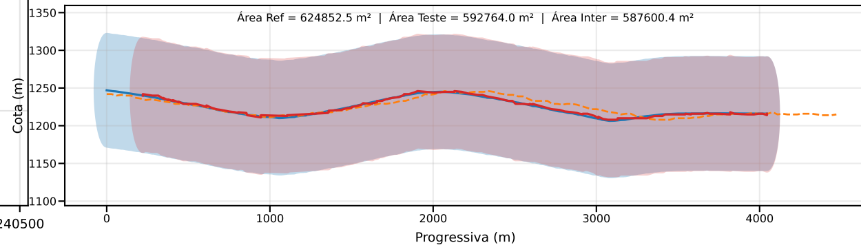
Classe D | PEC-PCD (Vertical)=75.0 m | EQ = 100m | dm = 14.81
