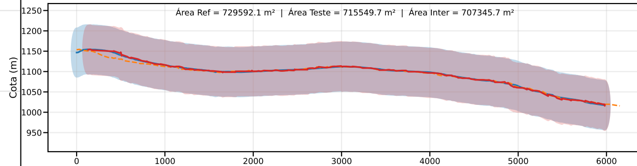
Classe D | PEC-PCD (Vertical)=75.0 m | EQ = 100m | dm = 6.84
