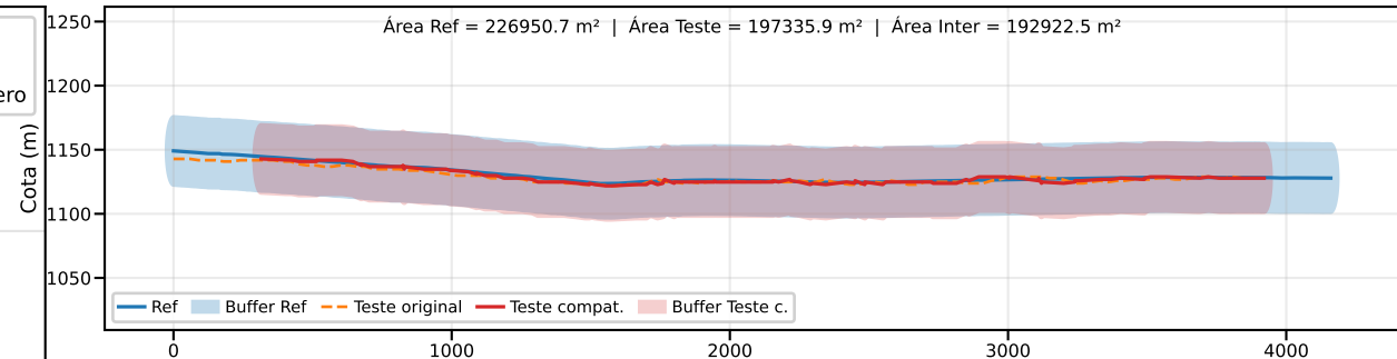
Classe B | PEC-PCD (Vertical)=50.0 m | EQ = 100m | dm = 25.32
