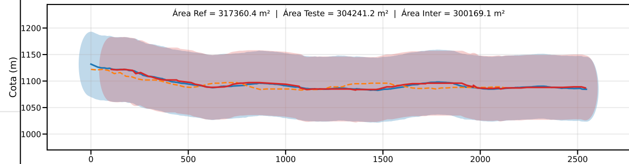
Classe D | PEC-PCD (Vertical)=75.0 m | EQ = 100m | dm = 12.59
