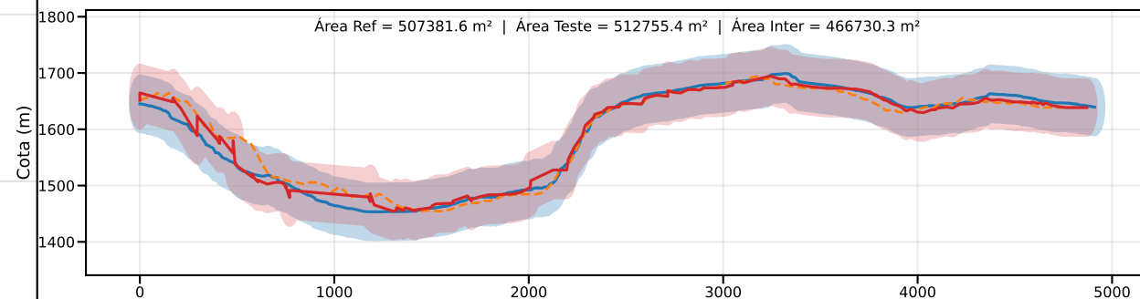
Classe C | PEC-PCD (Vertical)=60.0 m | EQ = 100m | dm = 12.57
