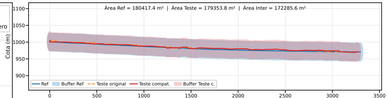
Classe B | PEC-PCD (Vertical)=50.0 m | EQ = 100m | dm = 4.32
