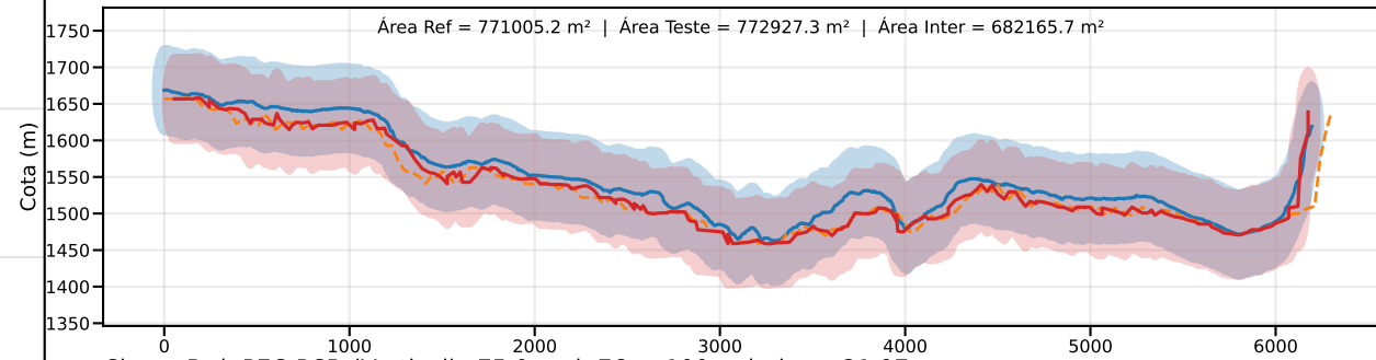
Classe D | PEC-PCD (Vertical)=75.0 m | EQ = 100m | dm = 21.97
