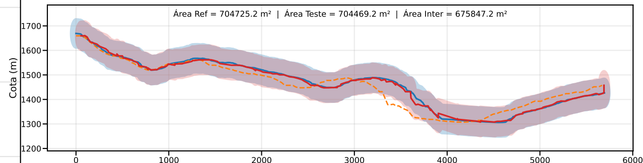
Classe D | PEC-PCD (Vertical)=75.0 m | EQ = 100m | dm = 8.08
