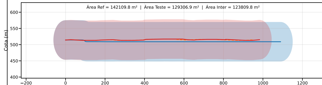
Classe D | PEC-PCD (Vertical)=75.0 m | EQ = 100m | dm = 30.69
