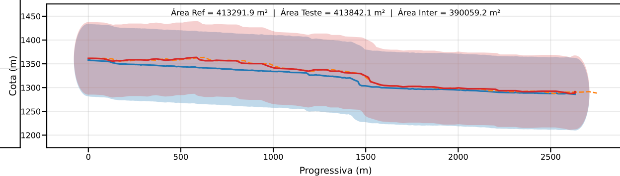
Classe D | PEC-PCD (Vertical)=75.0 m | EQ = 100m | dm = 13.23
