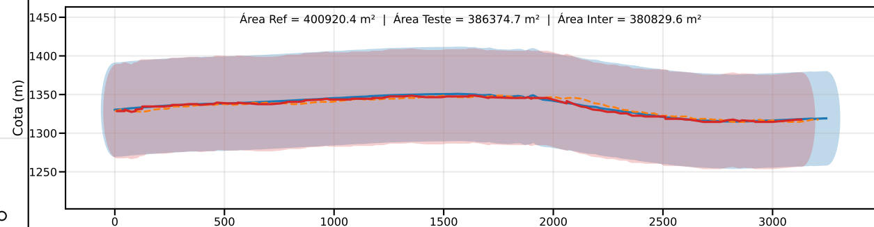
Classe D | PEC-PCD (Vertical)=75.0 m | EQ = 100m | dm = 11.53
