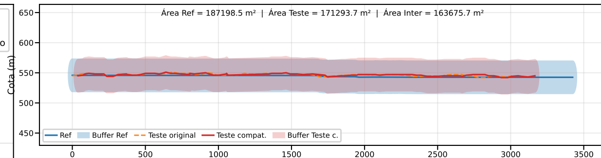
Classe B | PEC-PCD (Vertical)=50.0 m | EQ = 100m | dm = 18.20
