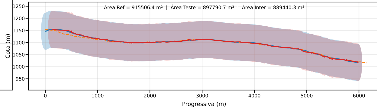
Classe D | PEC-PCD (Vertical)=75.0 m | EQ = 100m | dm = 6.84
