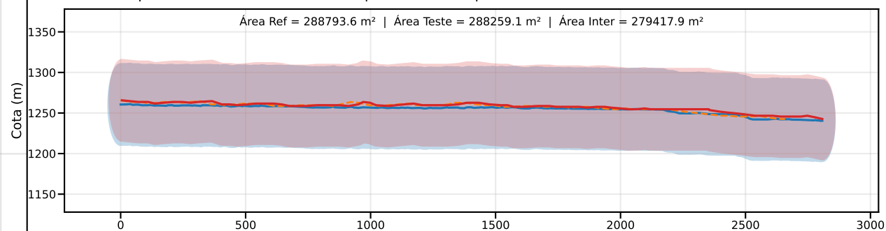
Classe C | PEC-PCD (Vertical)=60.0 m | EQ = 100m | dm = 5.16
