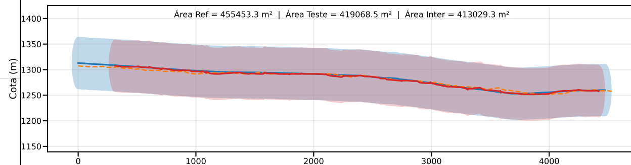
Classe C | PEC-PCD (Vertical)=60.0 m | EQ = 100m | dm = 18.60
