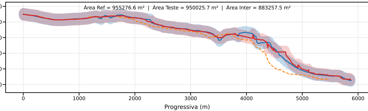
Classe D | PEC-PCD (Vertical)=75.0 m | EQ = 100m | dm = 17.86
