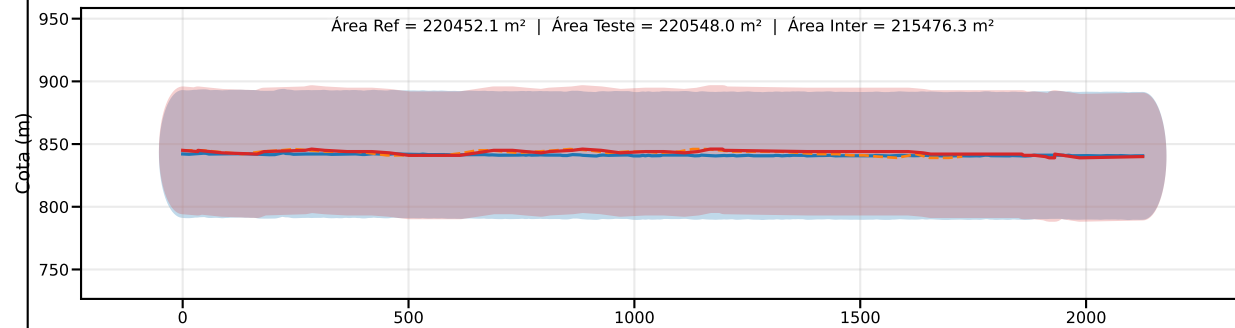
Classe C | PEC-PCD (Vertical)=60.0 m | EQ = 100m | dm = 3.54
