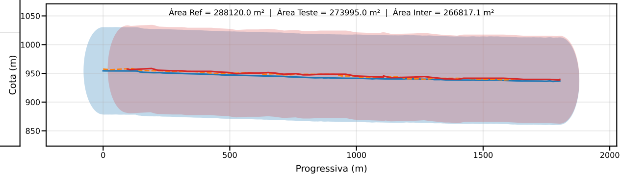
Classe D | PEC-PCD (Vertical)=75.0 m | EQ = 100m | dm = 18.32
