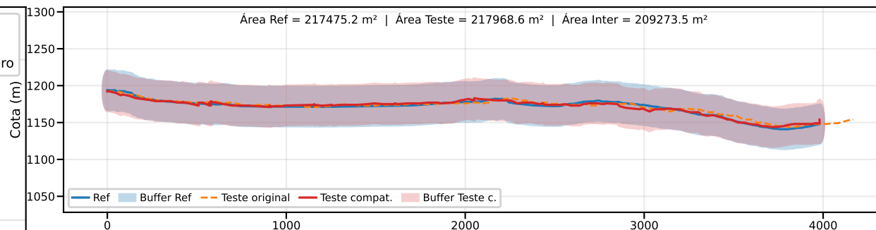
Classe B | PEC-PCD (Vertical)=50.0 m | EQ = 100m | dm = 3.17
