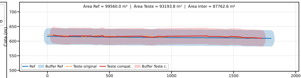
Classe B | PEC-PCD (Vertical)=50.0 m | EQ = 100m | dm = 15.47
