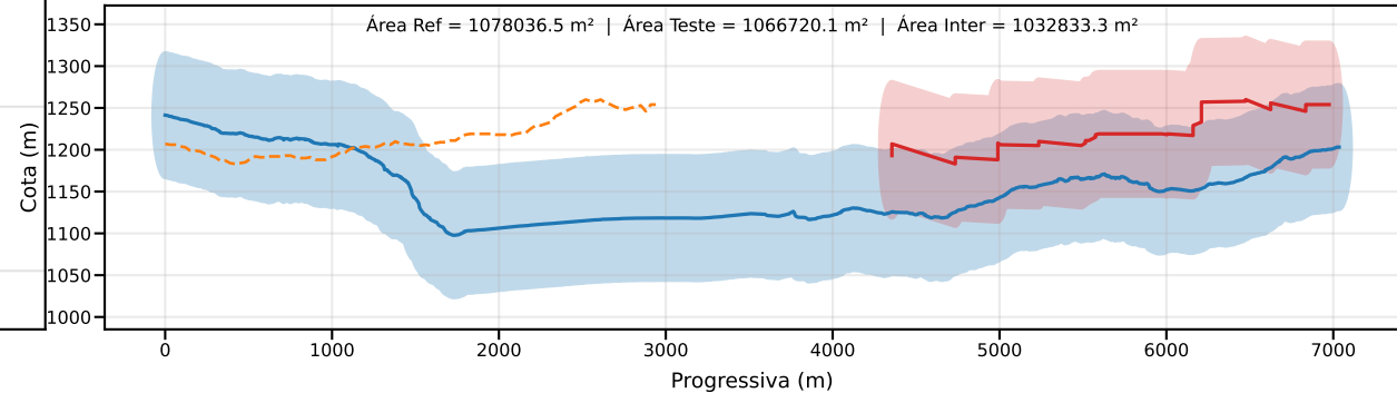
Classe D | PEC-PCD (Vertical)=75.0 m | EQ = 100m | dm = 9.98
