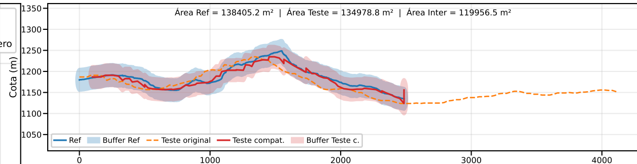
Classe B | PEC-PCD (Vertical)=50.0 m | EQ = 100m | dm = 14.34
