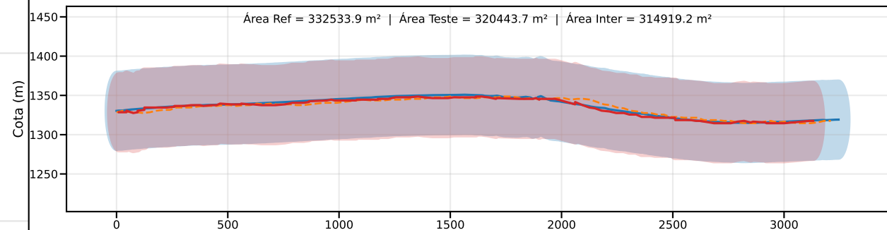
Classe C | PEC-PCD (Vertical)=60.0 m | EQ = 100m | dm = 9.80
