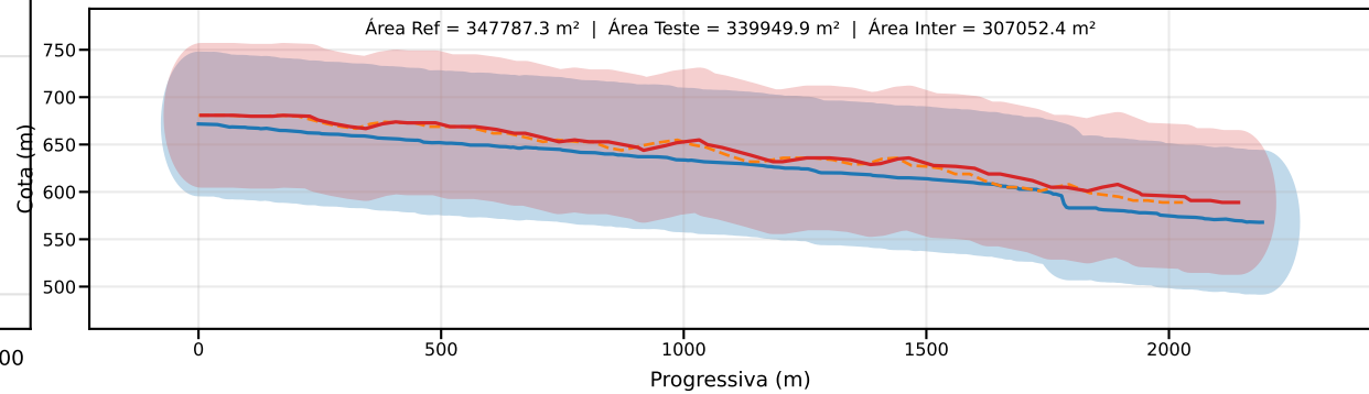
Classe D | PEC-PCD (Vertical)=75.0 m | EQ = 100m | dm = 28.23
