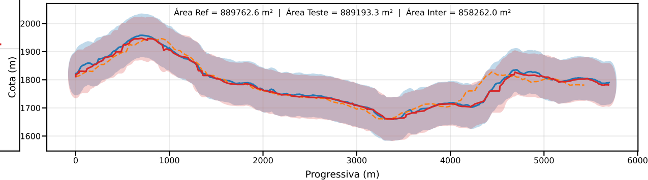
Classe D | PEC-PCD (Vertical)=75.0 m | EQ = 100m | dm = 8.35
