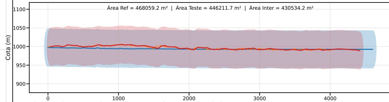
Classe C | PEC-PCD (Vertical)=60.0 m | EQ = 100m | dm = 14.71
