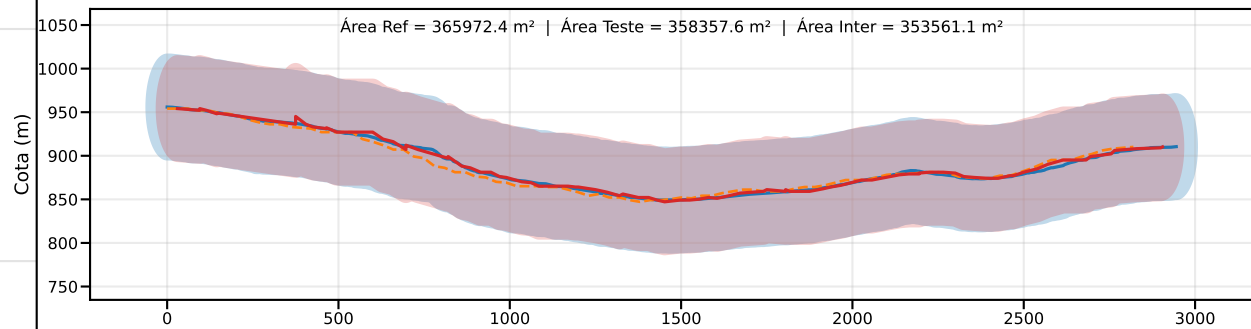
Classe D | PEC-PCD (Vertical)=75.0 m | EQ = 100m | dm = 7.55
