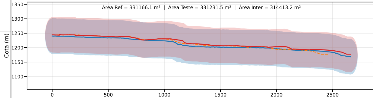
Classe D | PEC-PCD (Vertical)=75.0 m | EQ = 100m | dm = 9.56
