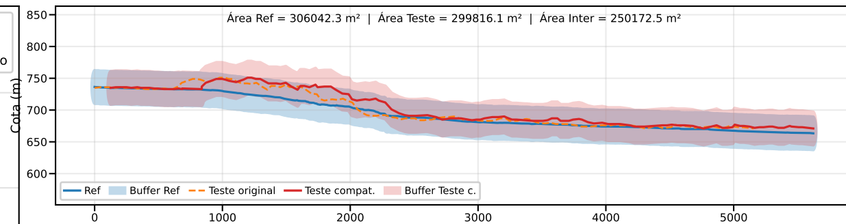
Classe B | PEC-PCD (Vertical)=50.0 m | EQ = 100m | dm = 17.32
