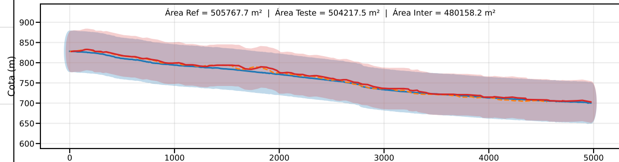
Classe C | PEC-PCD (Vertical)=60.0 m | EQ = 100m | dm = 8.06
