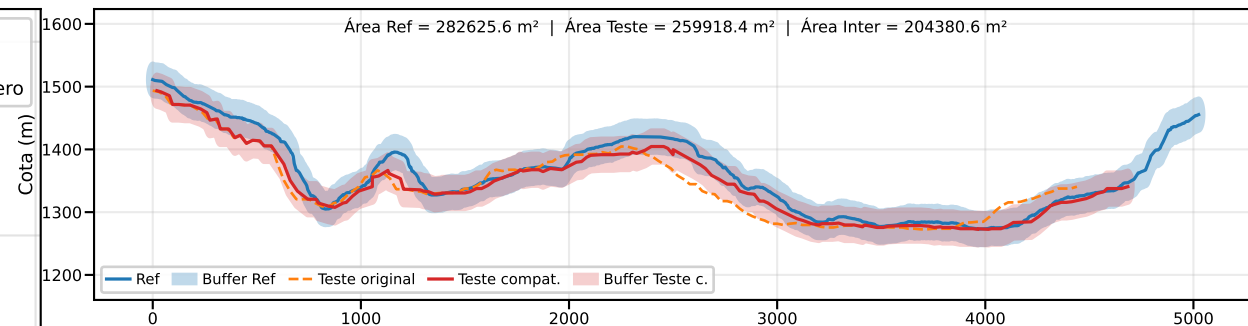
Classe B | PEC-PCD (Vertical)=50.0 m | EQ = 100m | dm = 31.42
