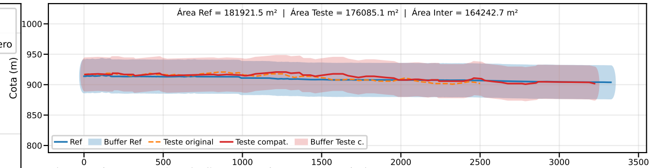
Classe B | PEC-PCD (Vertical)=50.0 m | EQ = 100m | dm = 10.83
