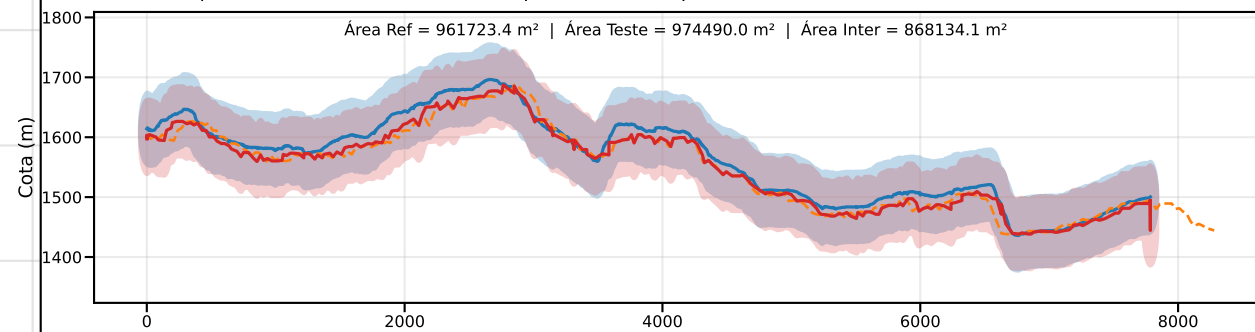
Classe D | PEC-PCD (Vertical)=75.0 m | EQ = 100m | dm = 18.02
