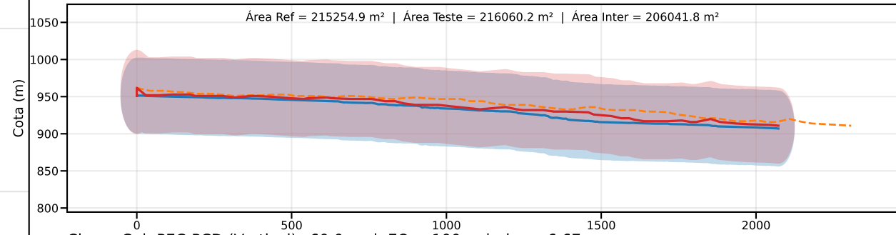
Classe C | PEC-PCD (Vertical)=60.0 m | EQ = 100m | dm = 6.67
