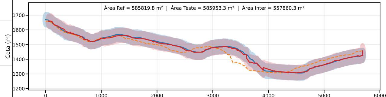
Classe C | PEC-PCD (Vertical)=60.0 m | EQ = 100m | dm = 7.73
