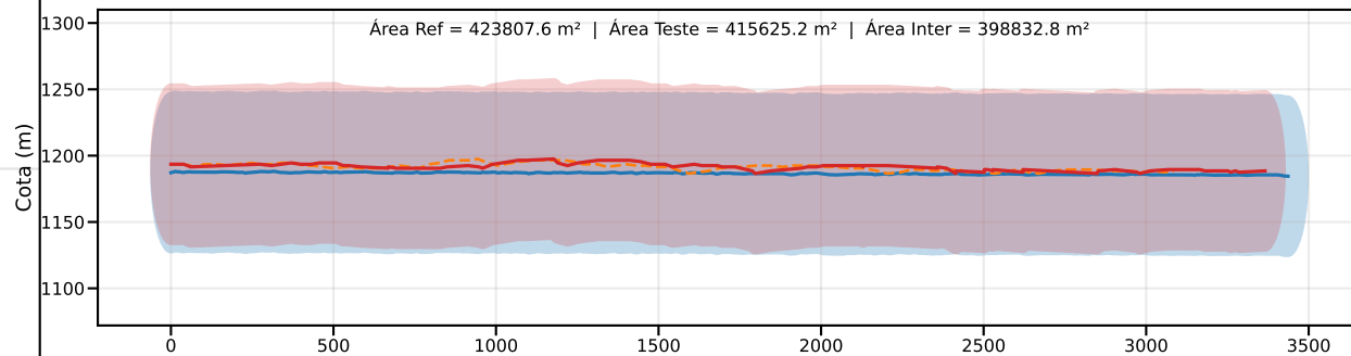
Classe D | PEC-PCD (Vertical)=75.0 m | EQ = 100m | dm = 12.24
