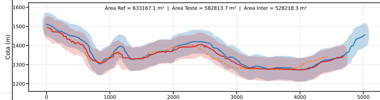
Classe D | PEC-PCD (Vertical)=75.0 m | EQ = 100m | dm = 37.69
