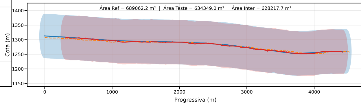
Classe D | PEC-PCD (Vertical)=75.0 m | EQ = 100m | dm = 22.60
