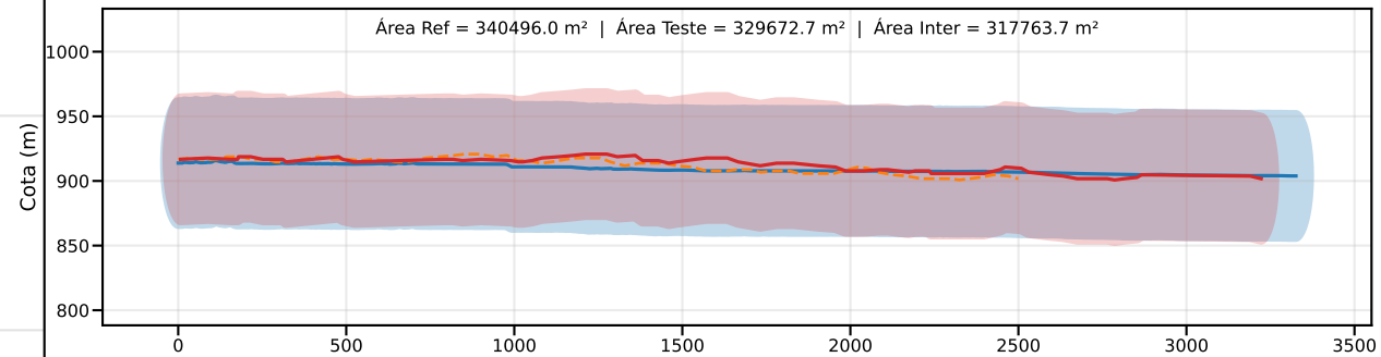
Classe C | PEC-PCD (Vertical)=60.0 m | EQ = 100m | dm = 11.82
