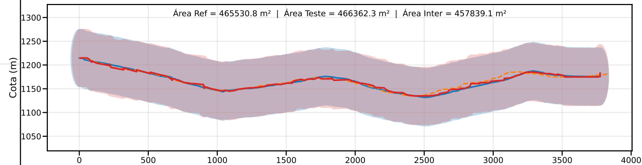
Classe D | PEC-PCD (Vertical)=75.0 m | EQ = 100m | dm = 3.16
