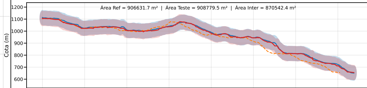
Classe D | PEC-PCD (Vertical)=75.0 m | EQ = 100m | dm = 7.46
