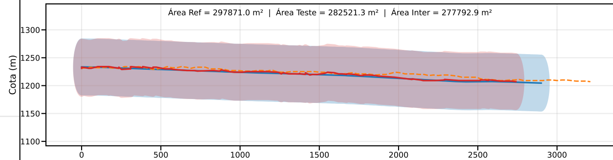
Classe C | PEC-PCD (Vertical)=60.0 m | EQ = 100m | dm = 12.86
