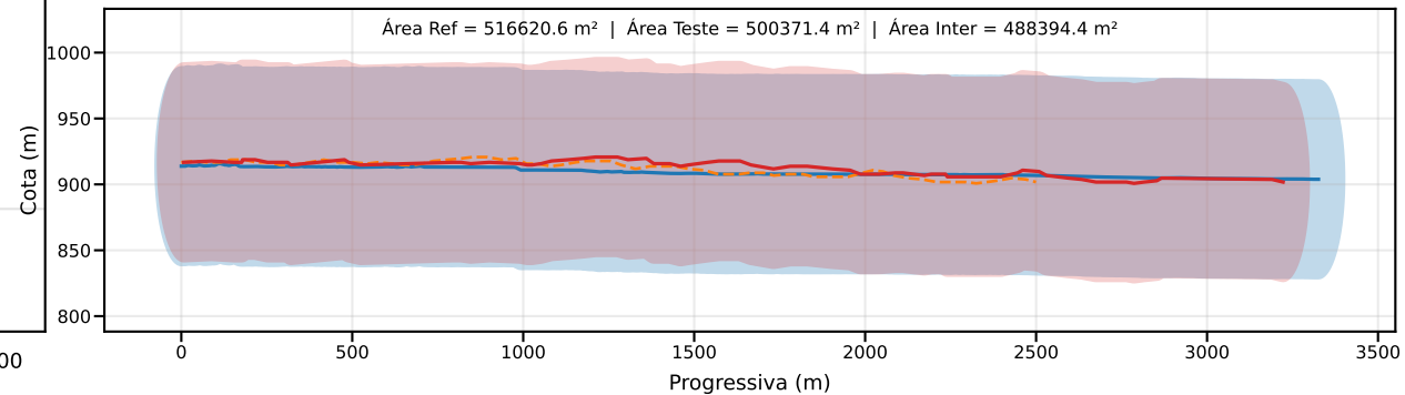
Classe D | PEC-PCD (Vertical)=75.0 m | EQ = 100m | dm = 13.29
