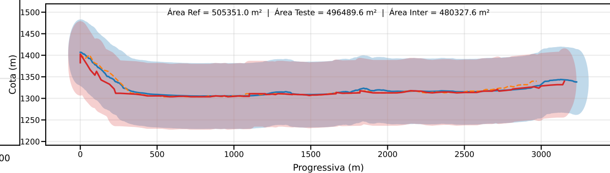
Classe D | PEC-PCD (Vertical)=75.0 m | EQ = 100m | dm = 11.88
