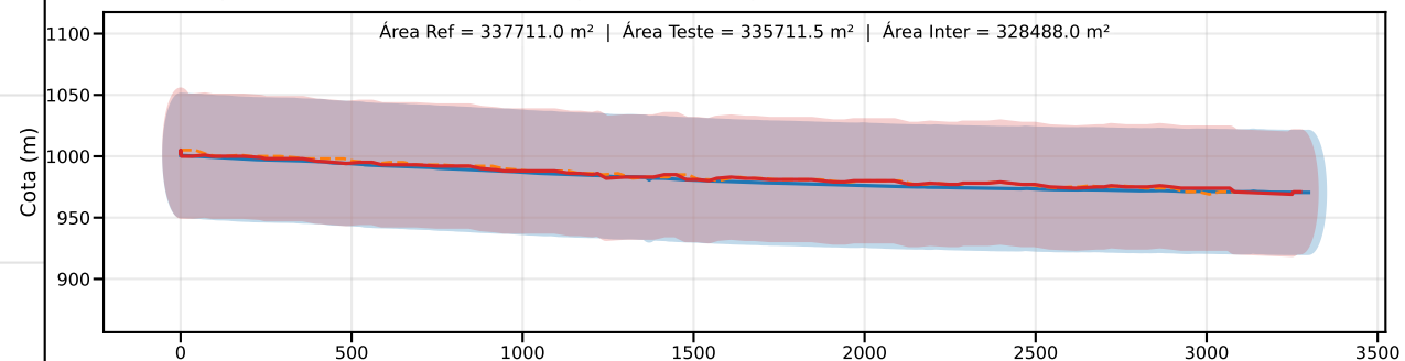
Classe C | PEC-PCD (Vertical)=60.0 m | EQ = 100m | dm = 4.52
