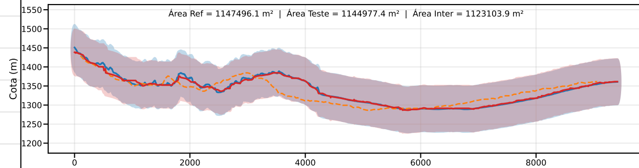
Classe D | PEC-PCD (Vertical)=75.0 m | EQ = 100m | dm = 4.09
