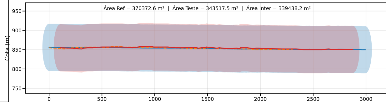
Classe D | PEC-PCD (Vertical)=75.0 m | EQ = 100m | dm = 20.50
