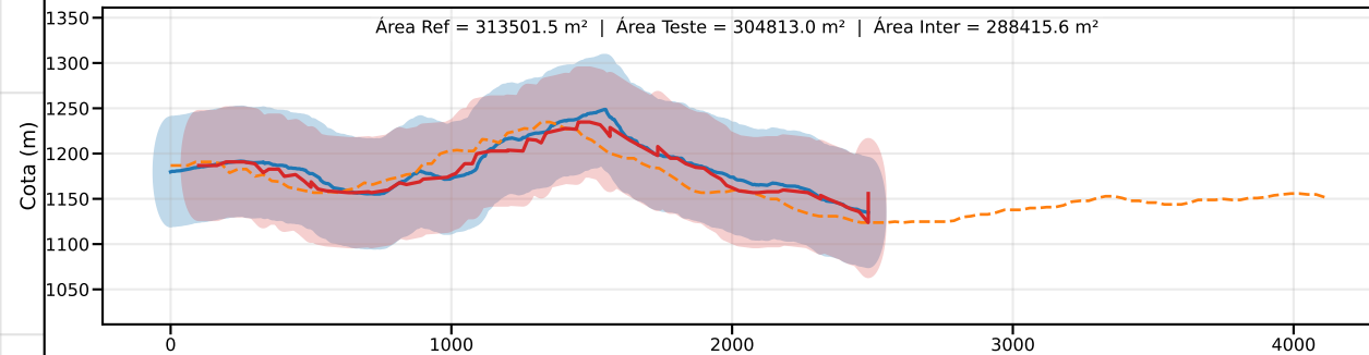
Classe D | PEC-PCD (Vertical)=75.0 m | EQ = 100m | dm = 17.25
