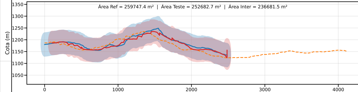
Classe C | PEC-PCD (Vertical)=60.0 m | EQ = 100m | dm = 15.51
