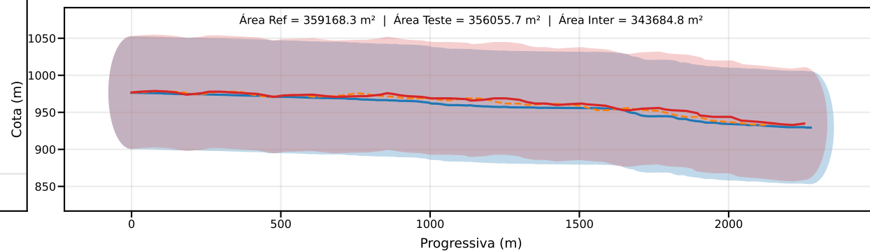
Classe D | PEC-PCD (Vertical)=75.0 m | EQ = 100m | dm = 10.25
