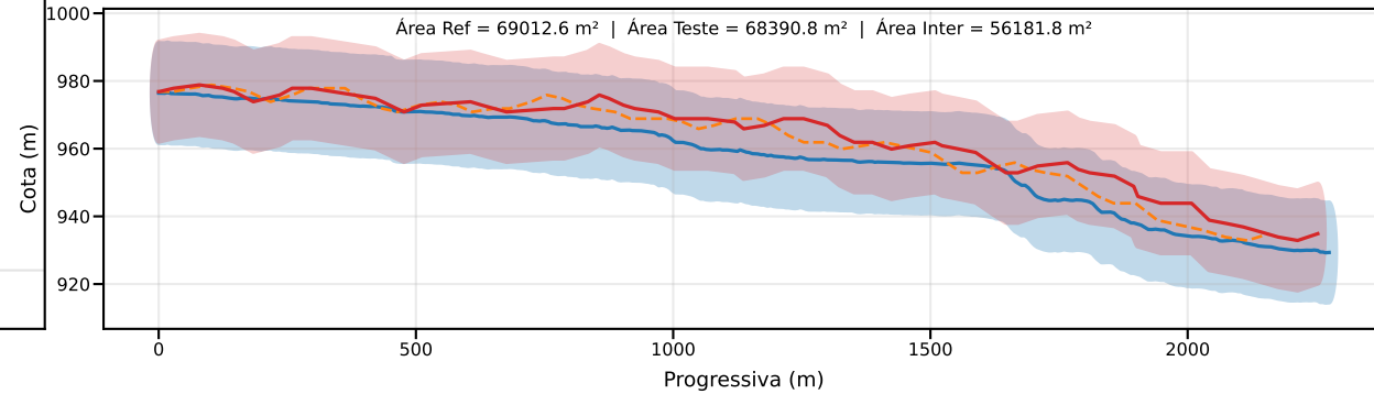
Classe D | PEC-PCD (Vertical)=15.0 m | EQ = 20m | dm = 8.84
