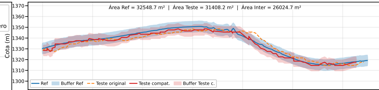
Classe B | PEC-PCD (Vertical)=10.0 m | EQ = 20m | dm = 3.87
