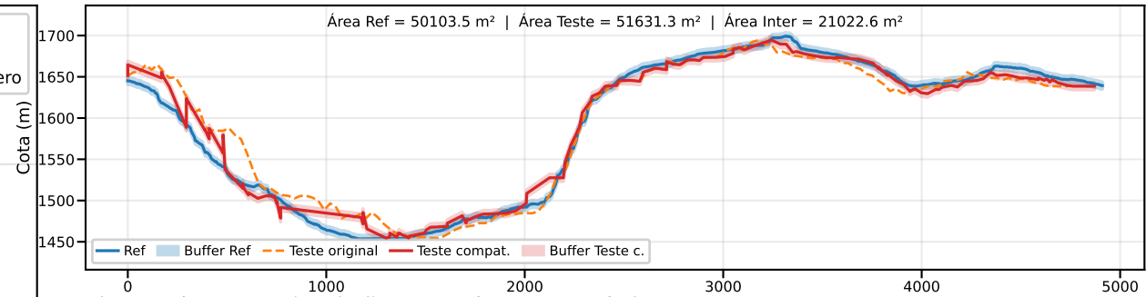
Classe B | PEC-PCD (Vertical)=10.0 m | EQ = 20m | dm = 11.45
