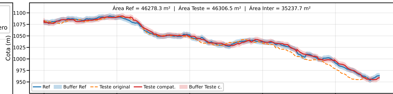
Classe B | PEC-PCD (Vertical)=10.0 m | EQ = 20m | dm = 3.75
