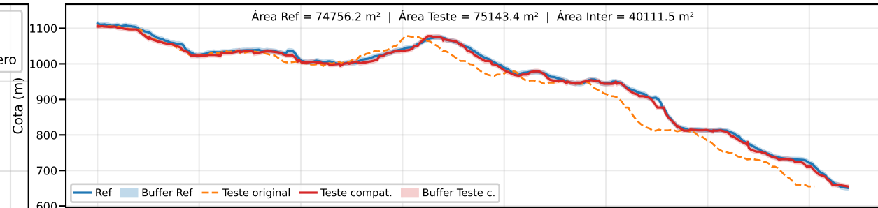
Classe B | PEC-PCD (Vertical)=10.0 m | EQ = 20m | dm = 7.58
