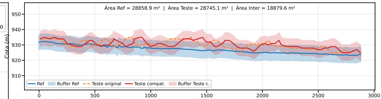
Classe B | PEC-PCD (Vertical)=10.0 m | EQ = 20m | dm = 5.51
