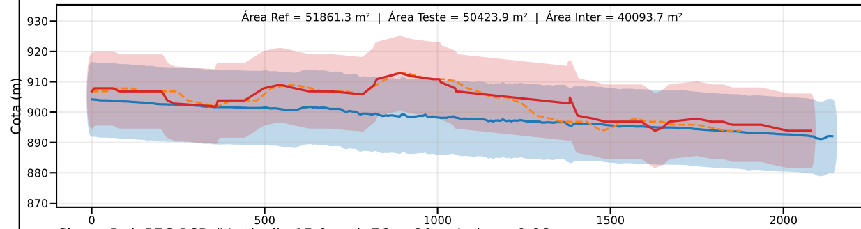
Classe D | PEC-PCD (Vertical)=15.0 m | EQ = 20m | dm = 9.06
