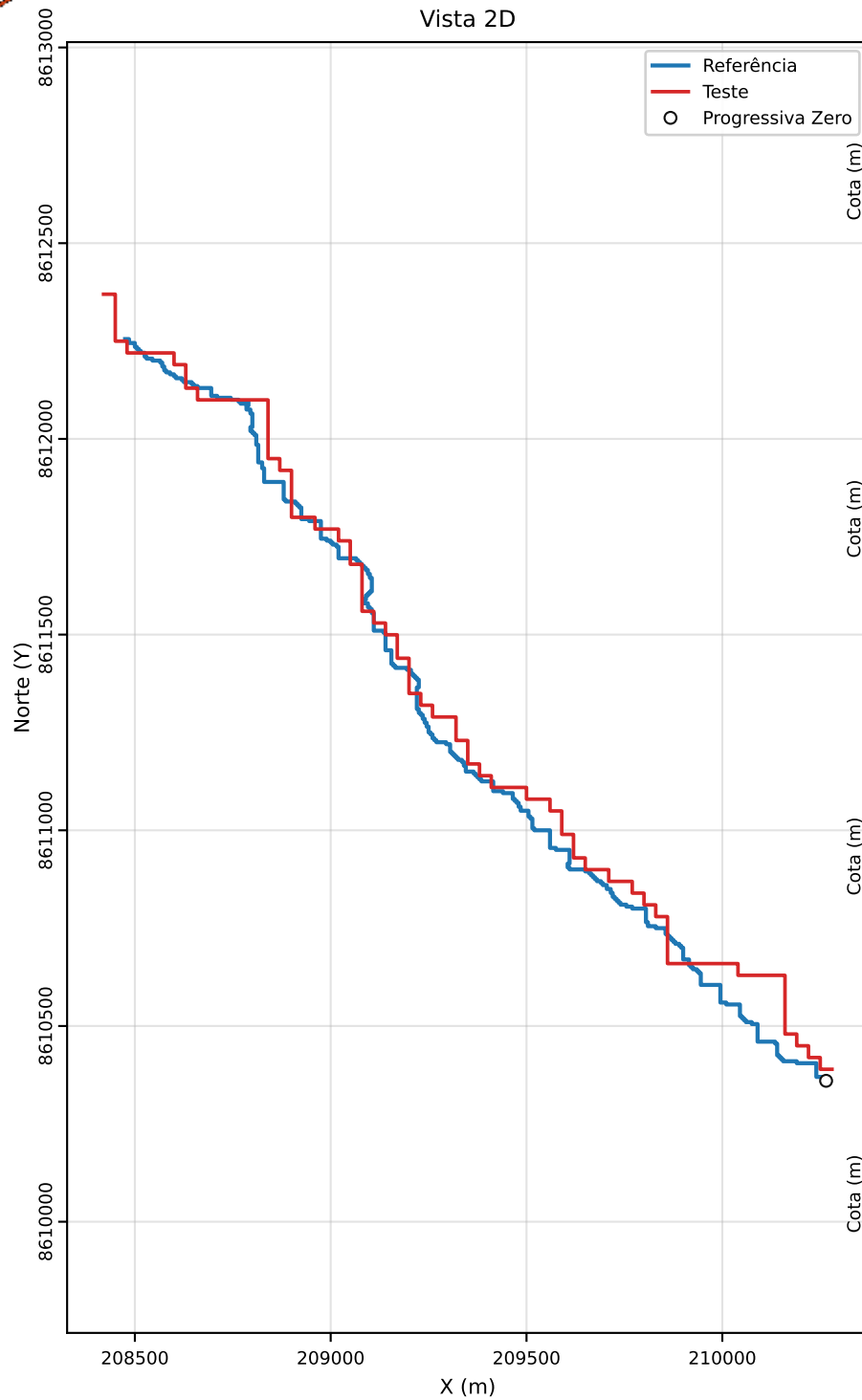
Classe A | PEC-PCD (Vertical)=5.0 m | EQ = 20m | dm = 2.98
