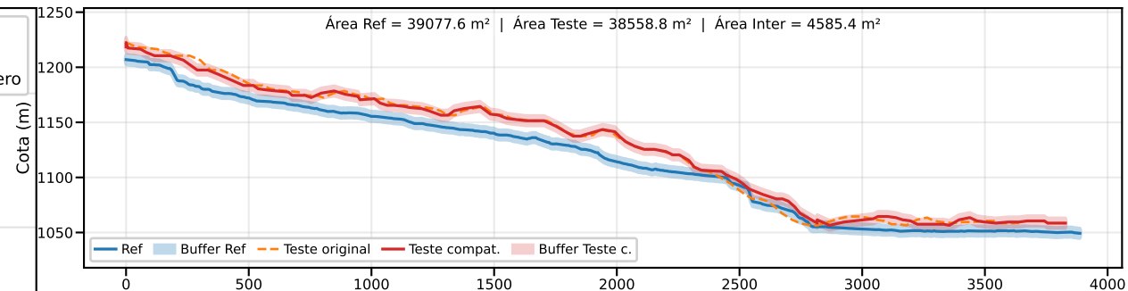
Classe B | PEC-PCD (Vertical)=10.0 m | EQ = 20m | dm = 18.83
