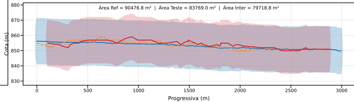
Classe D | PEC-PCD (Vertical)=15.0 m | EQ = 20m | dm = 6.05
