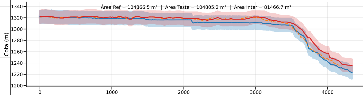
Classe D | PEC-PCD (Vertical)=15.0 m | EQ = 20m | dm = 8.42
