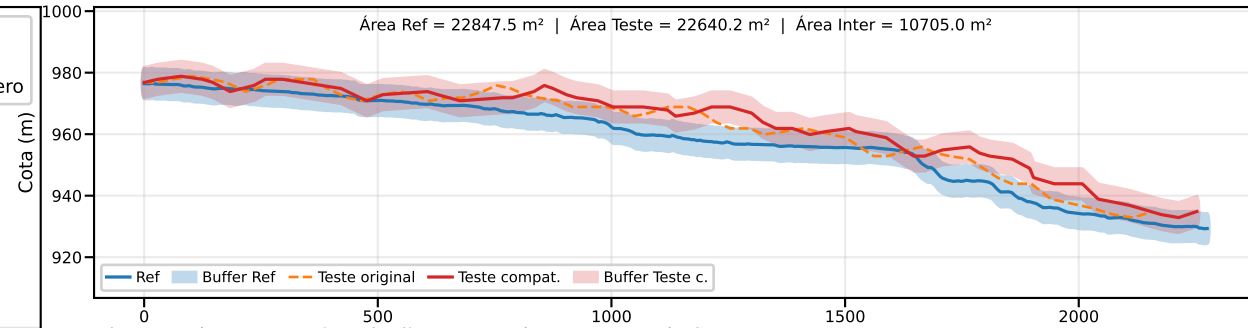
Classe B | PEC-PCD (Vertical)=10.0 m | EQ = 20m | dm = 8.72
