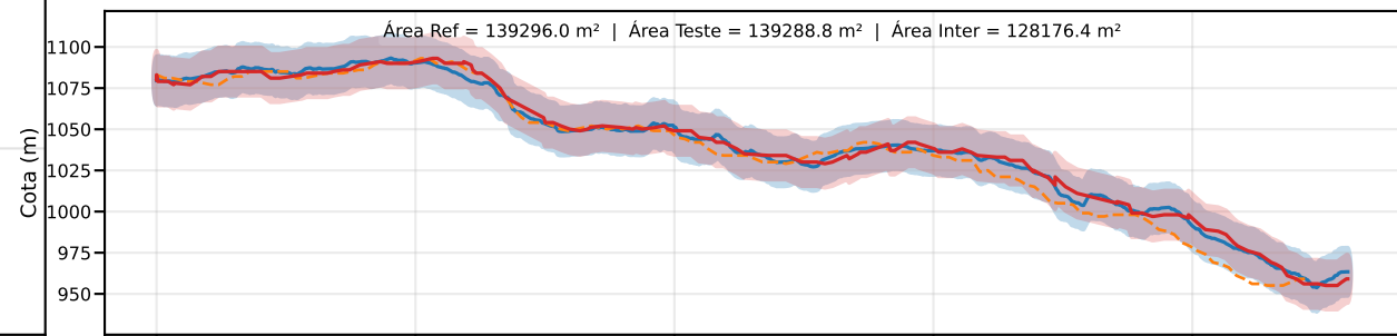
Classe D | PEC-PCD (Vertical)=15.0 m | EQ = 20m | dm = 3.76
