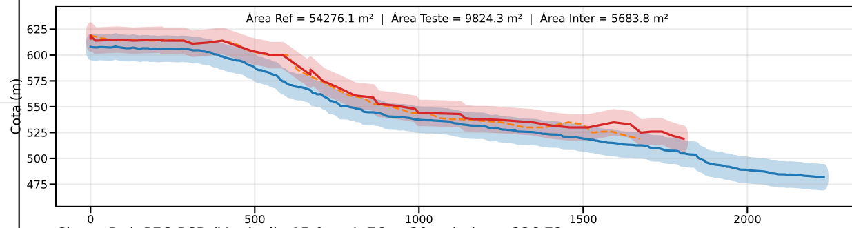
Classe D | PEC-PCD (Vertical)=15.0 m | EQ = 20m | dm = 226.72
