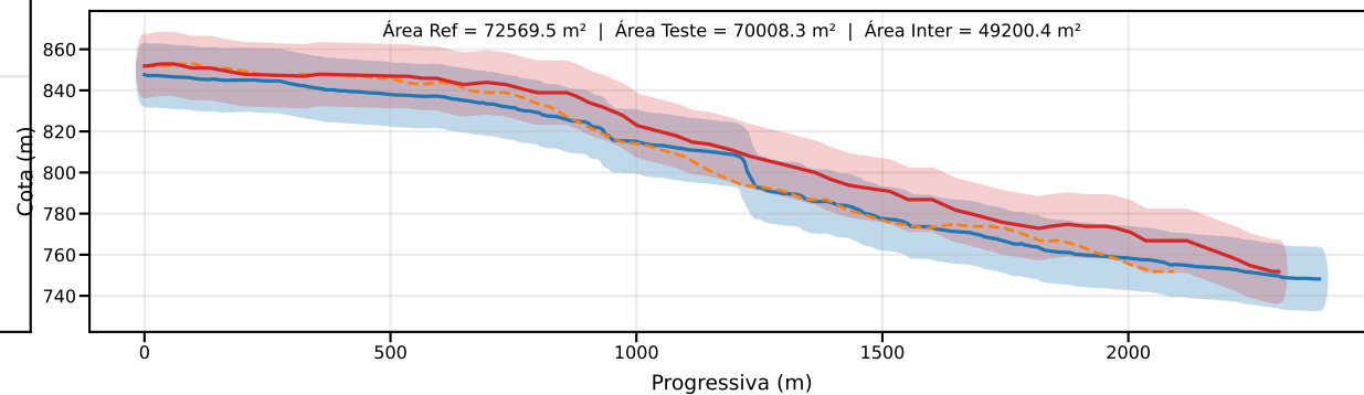
Classe D | PEC-PCD (Vertical)=15.0 m | EQ = 20m | dm = 15.73
