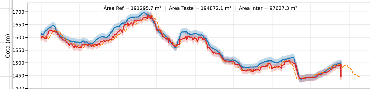
Classe D | PEC-PCD (Vertical)=15.0 m | EQ = 20m | dm = 18.42
