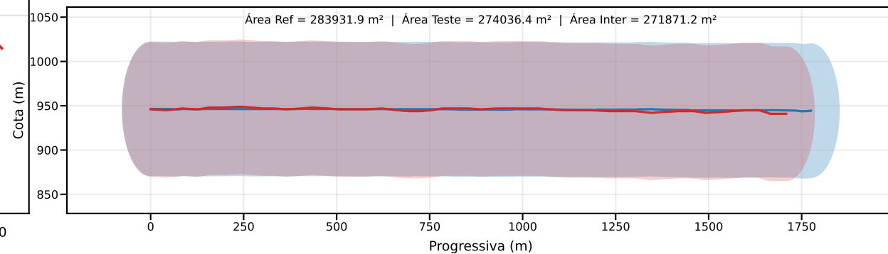
Classe D | PEC-PCD (Vertical)=75.0 m | EQ = 100m | dm = 10.37
