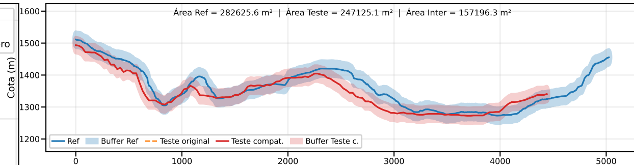
Classe B | PEC-PCD (Vertical)=50.0 m | EQ = 100m | dm = 52.97
