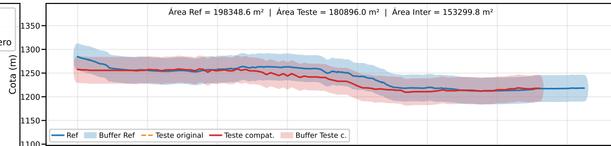
Classe B | PEC-PCD (Vertical)=50.0 m | EQ = 100m | dm = 28.03
