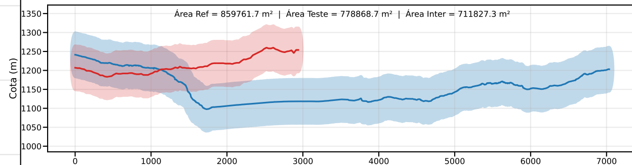
Classe D | PEC-PCD (Vertical)=75.0 m | EQ = 100m | dm = 40.62
