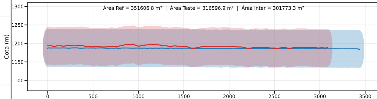
Classe C | PEC-PCD (Vertical)=60.0 m | EQ = 100m | dm = 28.10
