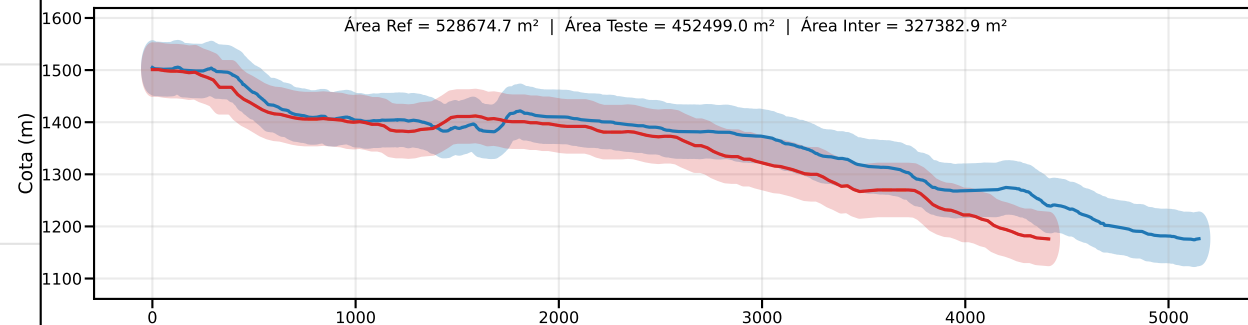
Classe C | PEC-PCD (Vertical)=60.0 m | EQ = 100m | dm = 74.98
