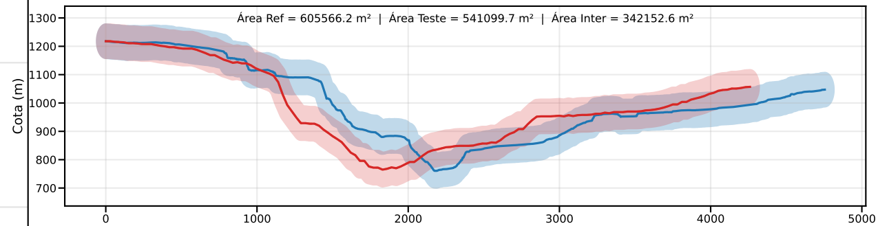
Classe D | PEC-PCD (Vertical)=75.0 m | EQ = 100m | dm = 98.07
