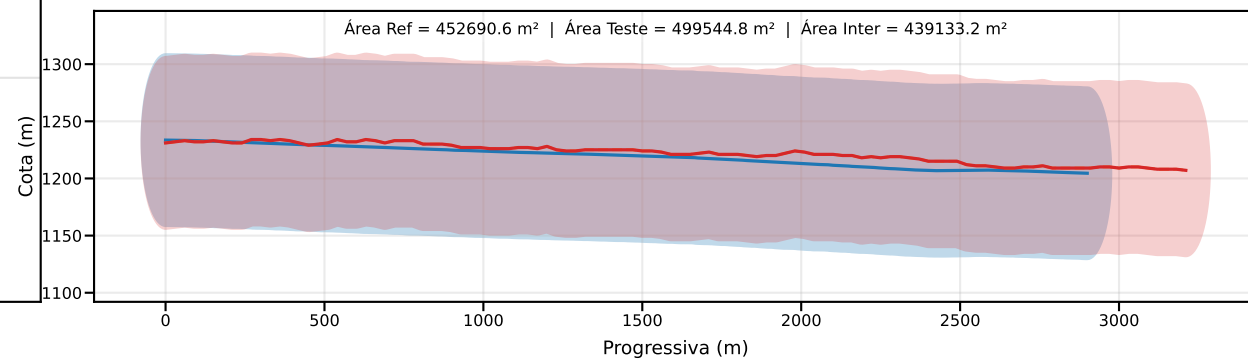
Classe D | PEC-PCD (Vertical)=75.0 m | EQ = 100m | dm = 6.39
