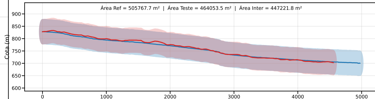
Classe C | PEC-PCD (Vertical)=60.0 m | EQ = 100m | dm = 22.57
