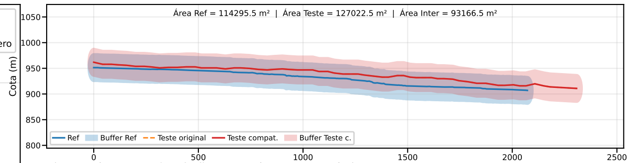
Classe B | PEC-PCD (Vertical)=50.0 m | EQ = 100m | dm = 14.10
