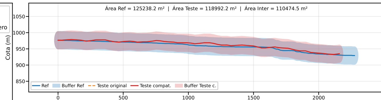
Classe B | PEC-PCD (Vertical)=50.0 m | EQ = 100m | dm = 14.12
