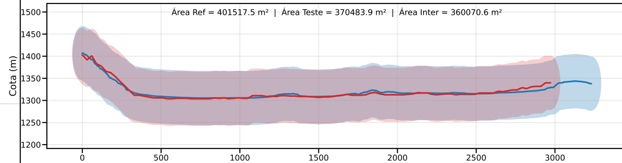
Classe D | PEC-PCD (Vertical)=75.0 m | EQ = 100m | dm = 24.90
