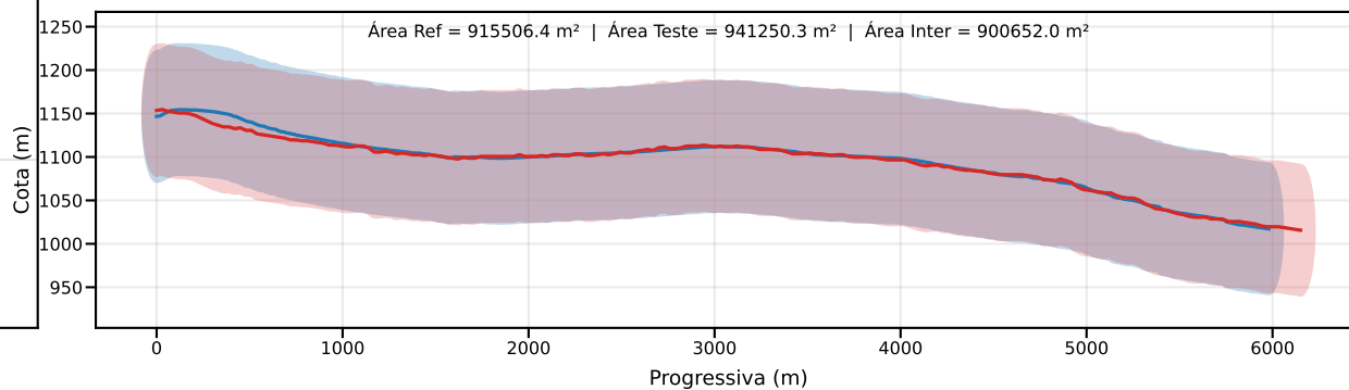
Classe D | PEC-PCD (Vertical)=75.0 m | EQ = 100m | dm = 3.72
