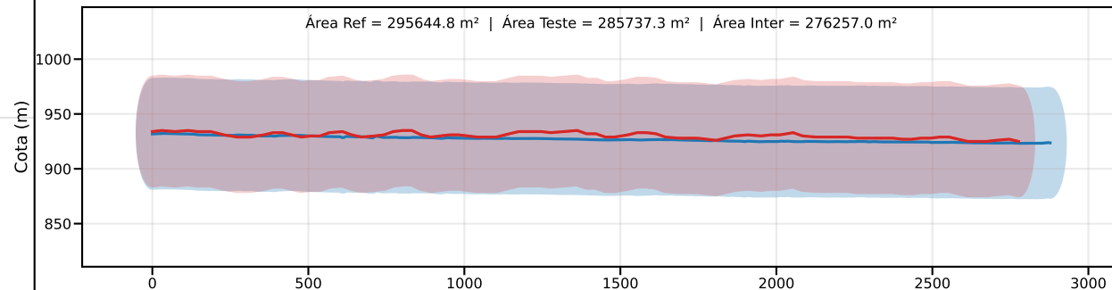
Classe C | PEC-PCD (Vertical)=60.0 m | EQ = 100m | dm = 11.71
