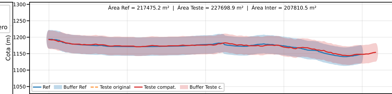
Classe B | PEC-PCD (Vertical)=50.0 m | EQ = 100m | dm = 3.58
