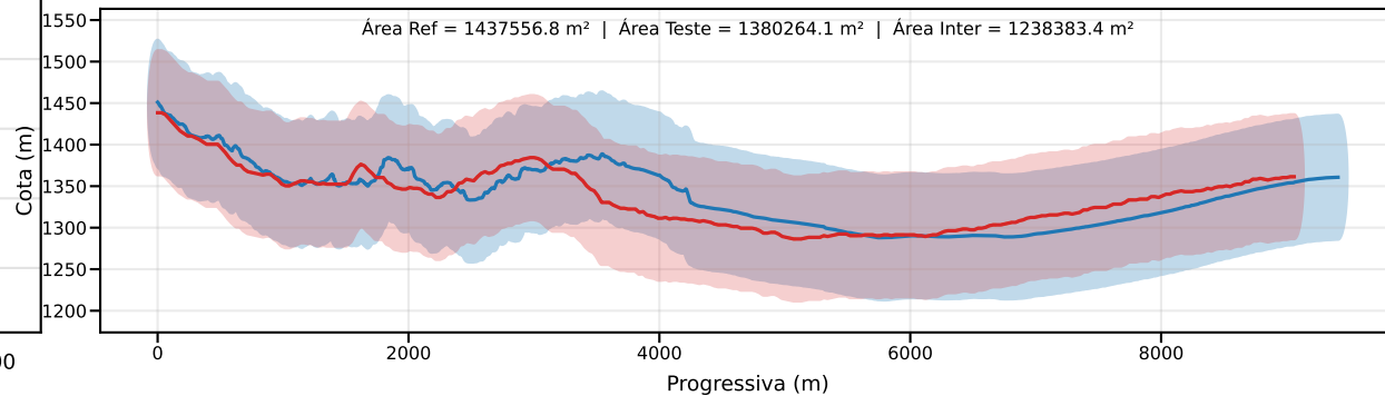
Classe D | PEC-PCD (Vertical)=75.0 m | EQ = 100m | dm = 34.00
