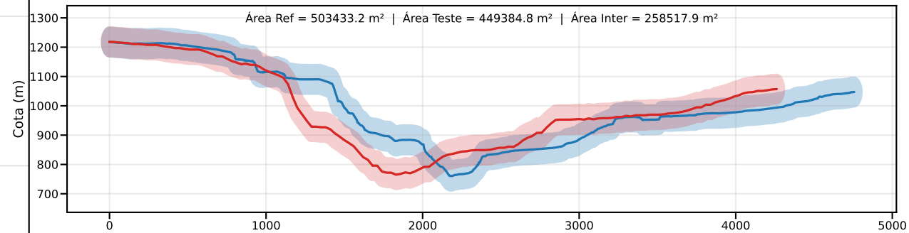
Classe C | PEC-PCD (Vertical)=60.0 m | EQ = 100m | dm = 91.76
