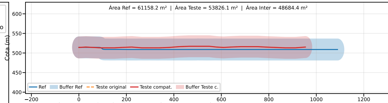
Classe B | PEC-PCD (Vertical)=50.0 m | EQ = 100m | dm = 28.49
