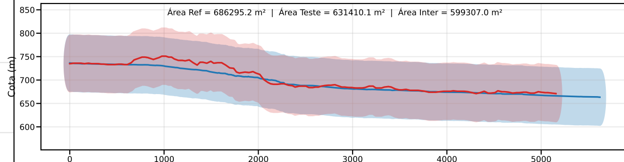
Classe D | PEC-PCD (Vertical)=75.0 m | EQ = 100m | dm = 29.98
