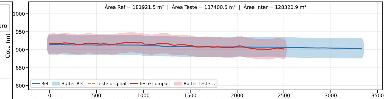
Classe B | PEC-PCD (Vertical)=50.0 m | EQ = 100m | dm = 55.78
