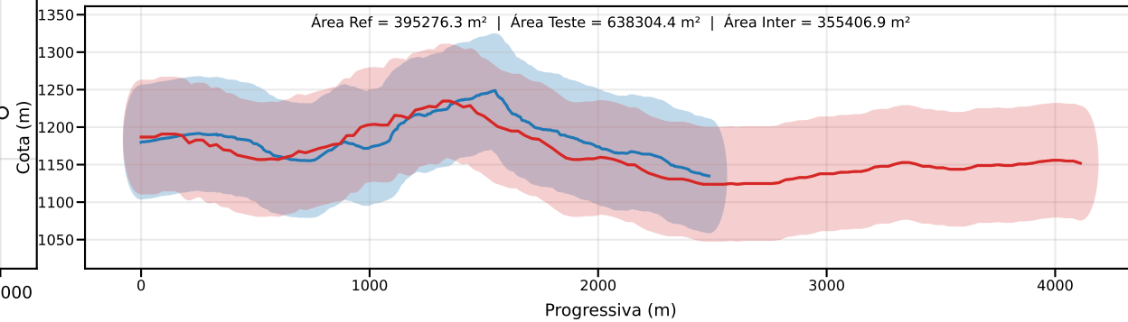
Classe D | PEC-PCD (Vertical)=75.0 m | EQ = 100m | dm = 14.72
