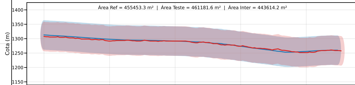
Classe C | PEC-PCD (Vertical)=60.0 m | EQ = 100m | dm = 4.03
