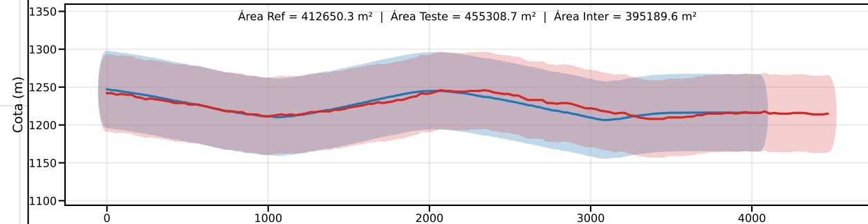
Classe C | PEC-PCD (Vertical)=60.0 m | EQ = 100m | dm = 6.02
