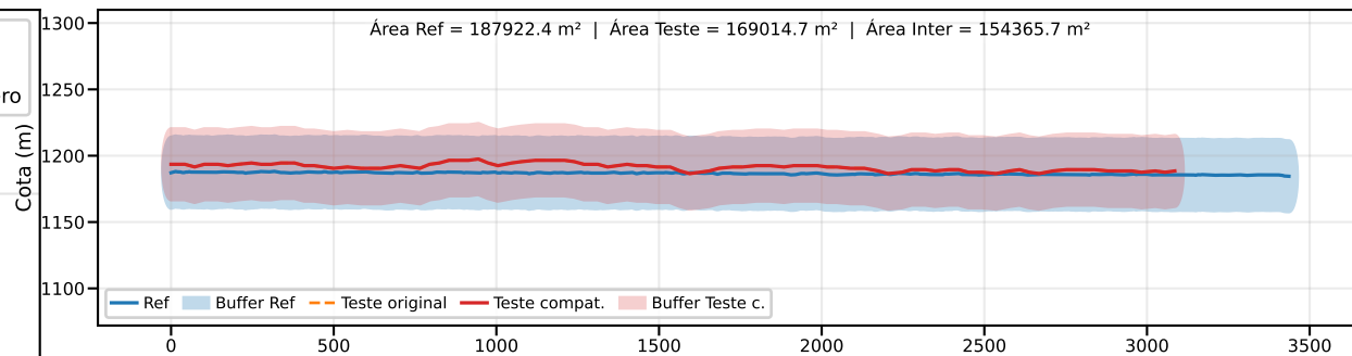
Classe B | PEC-PCD (Vertical)=50.0 m | EQ = 100m | dm = 24.72
