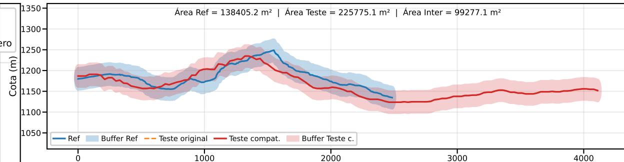
Classe B | PEC-PCD (Vertical)=50.0 m | EQ = 100m | dm = 14.72
