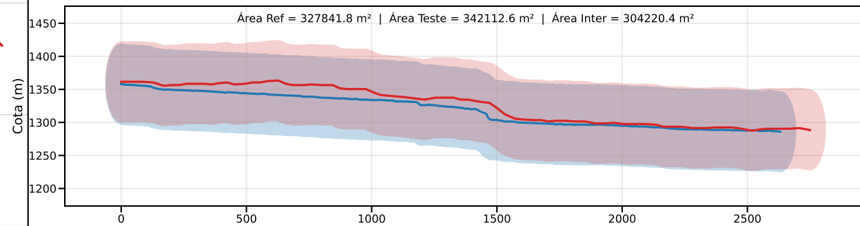
Classe D | PEC-PCD (Vertical)=75.0 m | EQ = 100m | dm = 12.93
