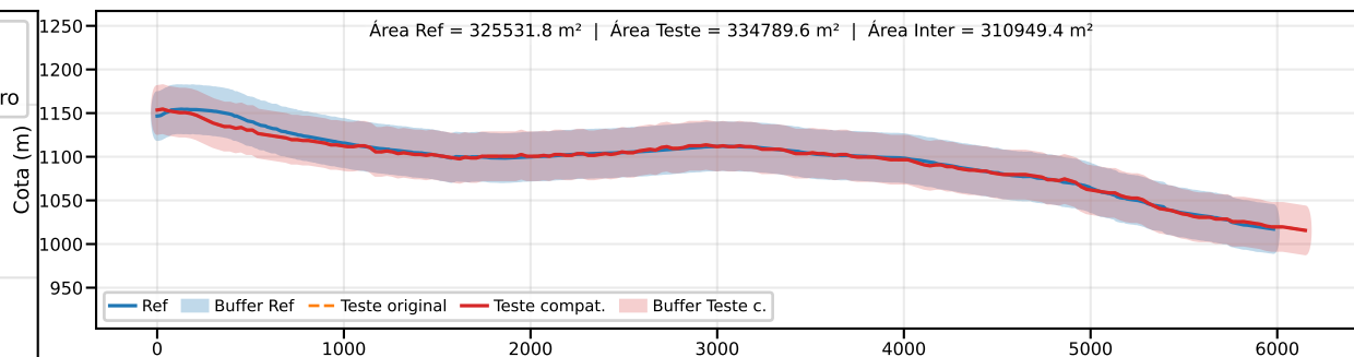
Classe B | PEC-PCD (Vertical)=50.0 m | EQ = 100m | dm = 3.71
