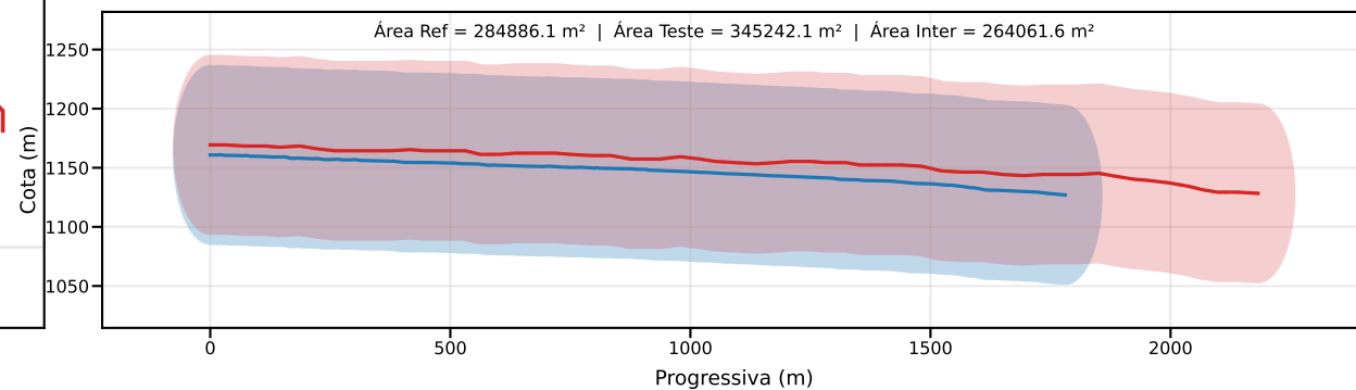
Classe D | PEC-PCD (Vertical)=75.0 m | EQ = 100m | dm = 14.21
