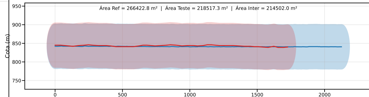
Classe D | PEC-PCD (Vertical)=75.0 m | EQ = 100m | dm = 54.45
