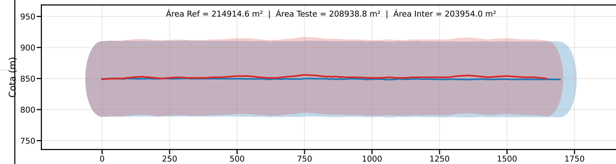
Classe D | PEC-PCD (Vertical)=75.0 m | EQ = 100m | dm = 11.09
