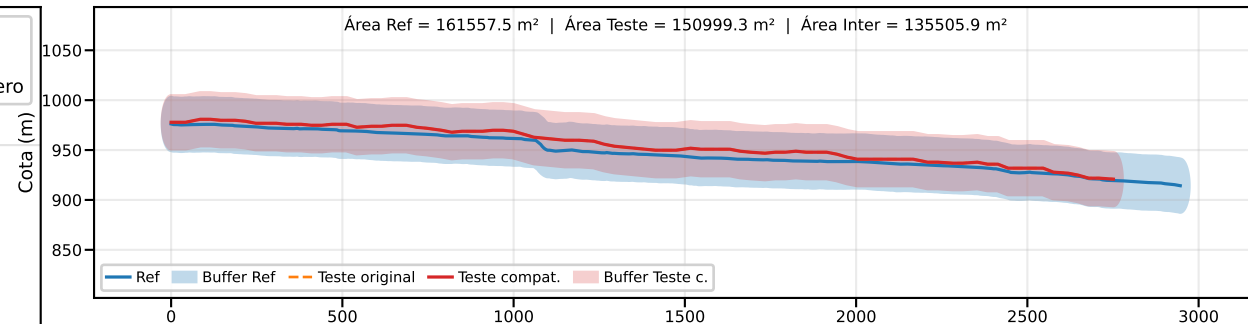
Classe B | PEC-PCD (Vertical)=50.0 m | EQ = 100m | dm = 19.46
