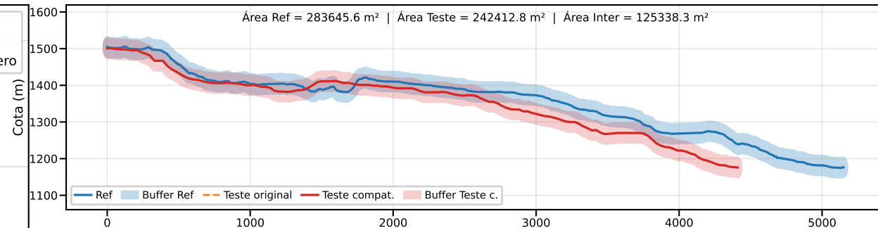
Classe B | PEC-PCD (Vertical)=50.0 m | EQ = 100m | dm = 69.88
