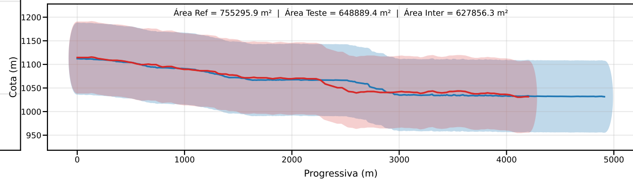
Classe D | PEC-PCD (Vertical)=75.0 m | EQ = 100m | dm = 46.27
