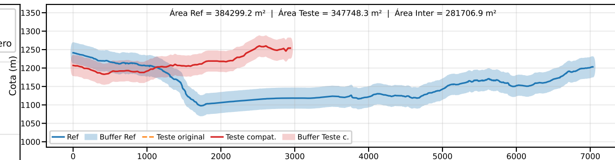
Classe B | PEC-PCD (Vertical)=50.0 m | EQ = 100m | dm = 32.57
