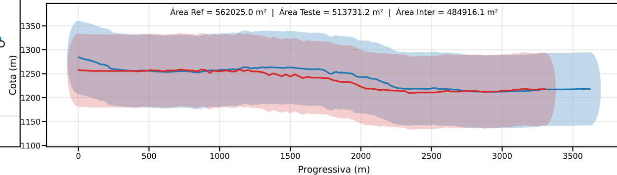
Classe D | PEC-PCD (Vertical)=75.0 m | EQ = 100m | dm = 35.37
