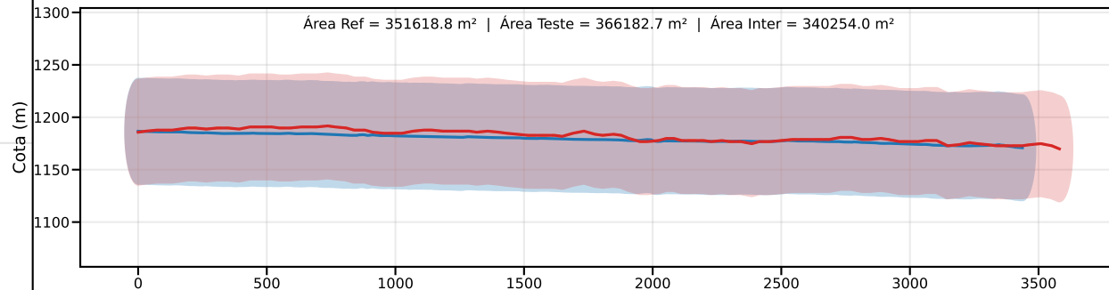
Classe C | PEC-PCD (Vertical)=60.0 m | EQ = 100m | dm = 4.85
