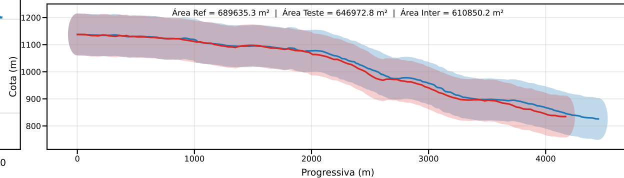
Classe D | PEC-PCD (Vertical)=75.0 m | EQ = 100m | dm = 28.69
