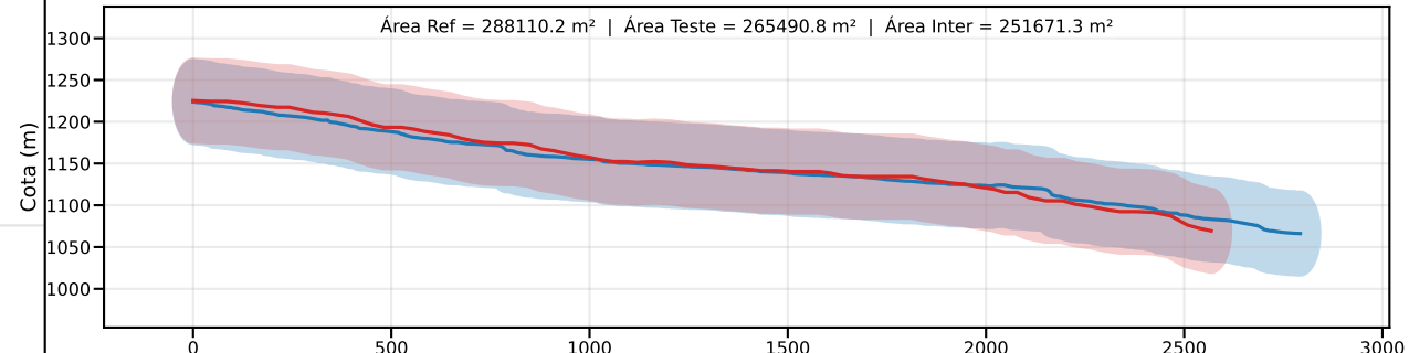
Classe C | PEC-PCD (Vertical)=60.0 m | EQ = 100m | dm = 24.11
