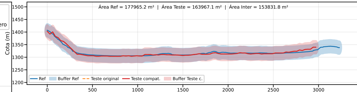
Classe B | PEC-PCD (Vertical)=50.0 m | EQ = 100m | dm = 18.51
