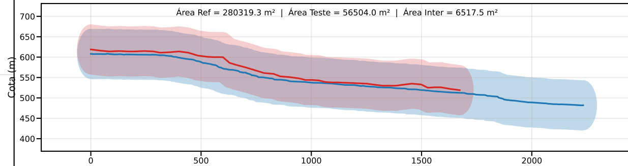
Classe D | PEC-PCD (Vertical)=75.0 m | EQ = 100m | dm = 1056.75
