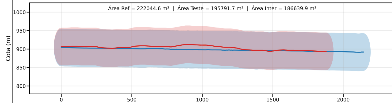
Classe C | PEC-PCD (Vertical)=60.0 m | EQ = 100m | dm = 32.38
