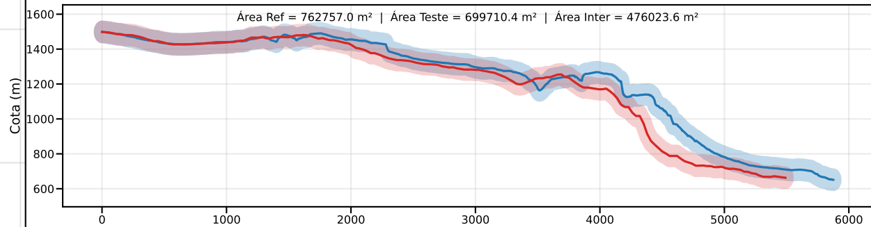
Classe D | PEC-PCD (Vertical)=75.0 m | EQ = 100m | dm = 84.17
