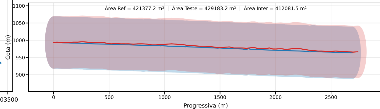
Classe D | PEC-PCD (Vertical)=75.0 m | EQ = 100m | dm = 5.10
