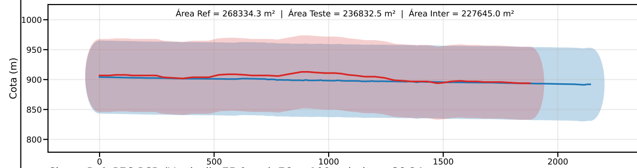
Classe D | PEC-PCD (Vertical)=75.0 m | EQ = 100m | dm = 38.24
