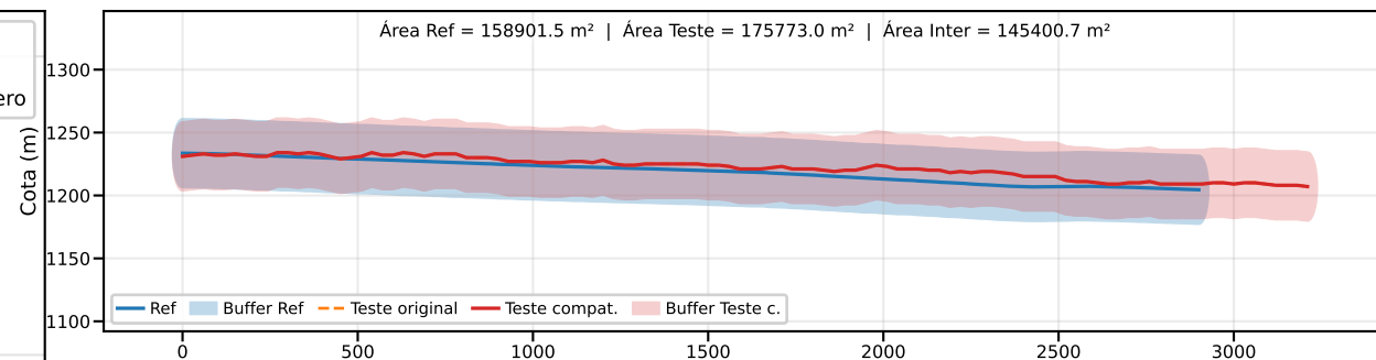
Classe B | PEC-PCD (Vertical)=50.0 m | EQ = 100m | dm = 6.46
