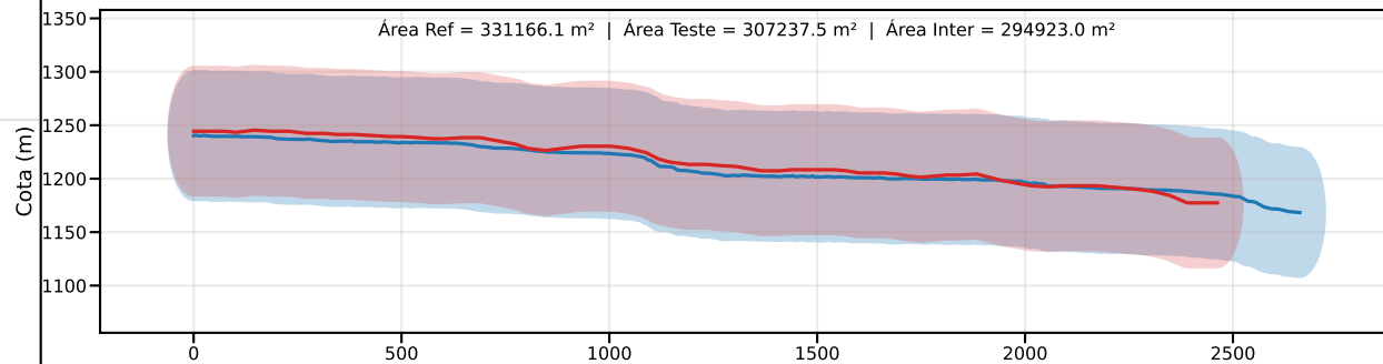
Classe D | PEC-PCD (Vertical)=75.0 m | EQ = 100m | dm = 25.71
