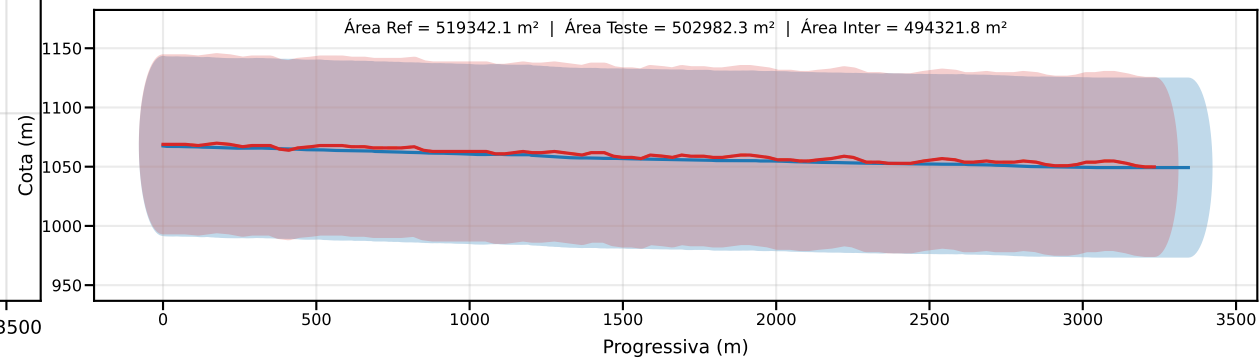
Classe D | PEC-PCD (Vertical)=75.0 m | EQ = 100m | dm = 11.72
