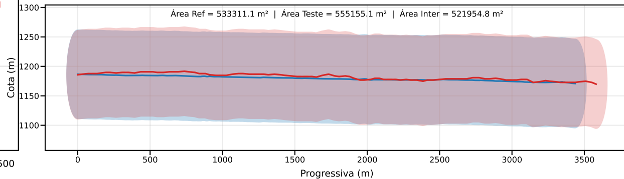
Classe D | PEC-PCD (Vertical)=75.0 m | EQ = 100m | dm = 4.82
