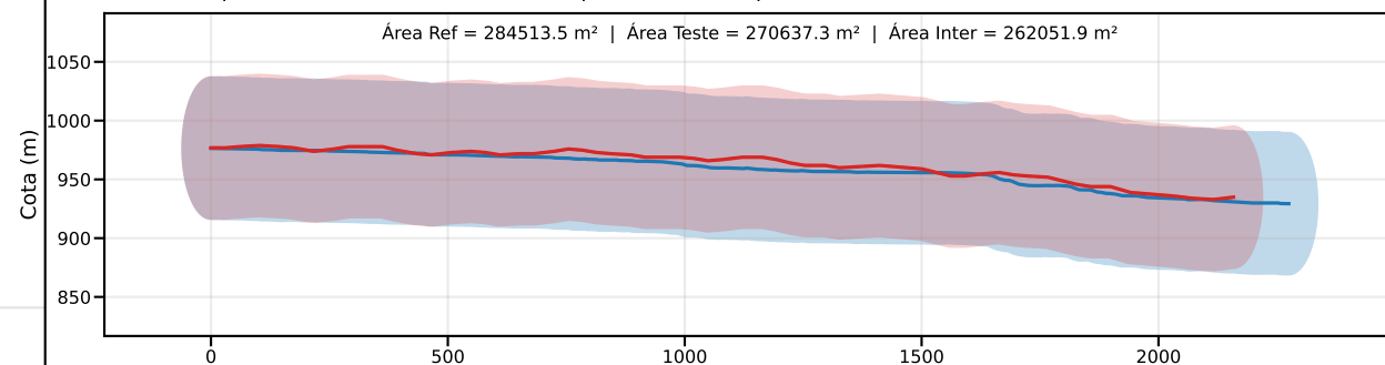
Classe D | PEC-PCD (Vertical)=75.0 m | EQ = 100m | dm = 17.89
