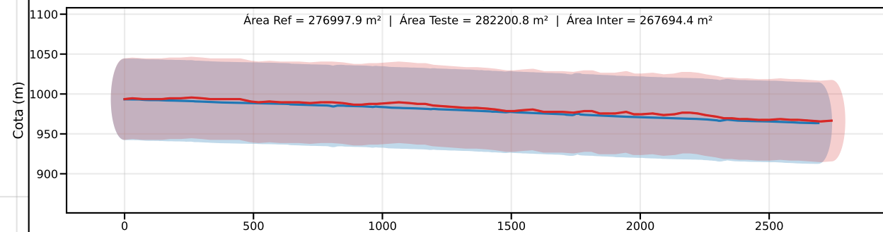
Classe C | PEC-PCD (Vertical)=60.0 m | EQ = 100m | dm = 5.15
