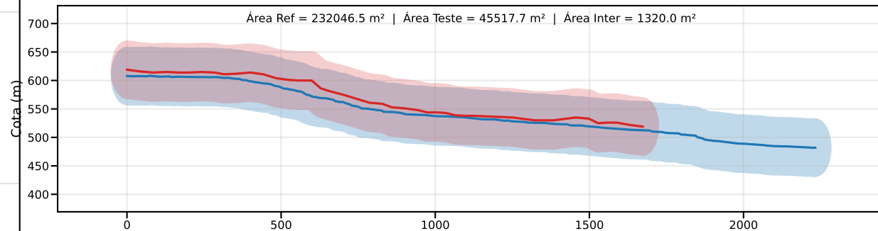
Classe C | PEC-PCD (Vertical)=60.0 m | EQ = 100m | dm = 913.40
