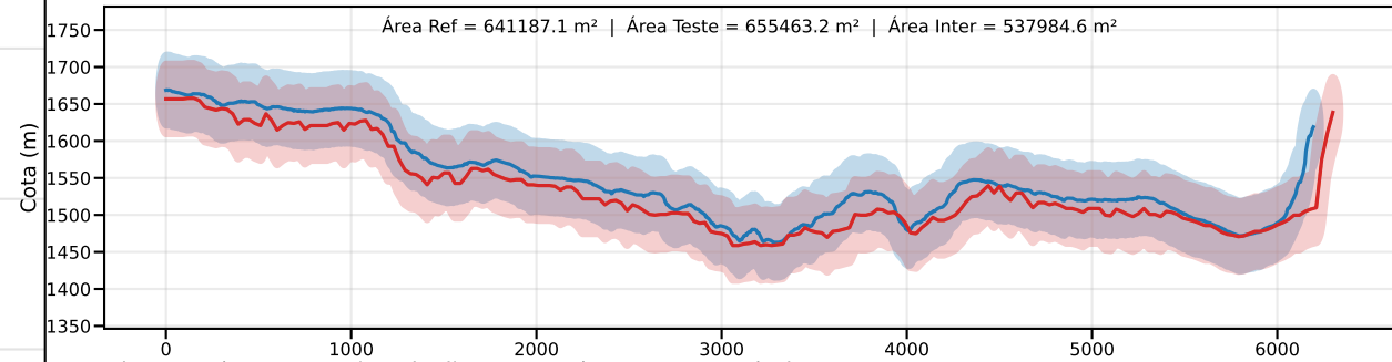
Classe C | PEC-PCD (Vertical)=60.0 m | EQ = 100m | dm = 24.65
