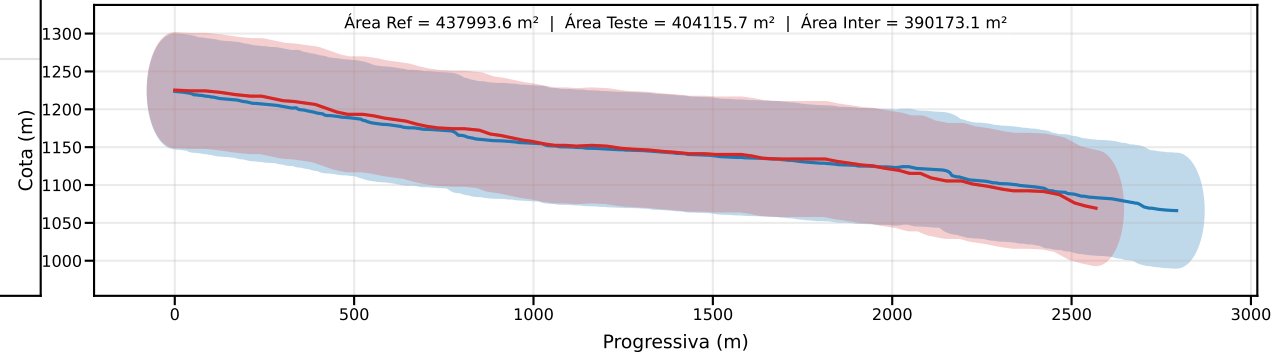
Classe D | PEC-PCD (Vertical)=75.0 m | EQ = 100m | dm = 27.88
