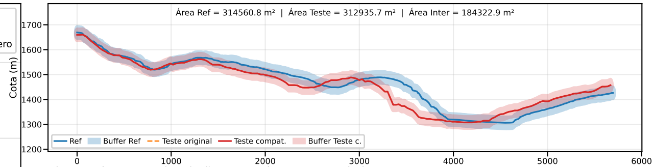
Classe B | PEC-PCD (Vertical)=50.0 m | EQ = 100m | dm = 39.09
