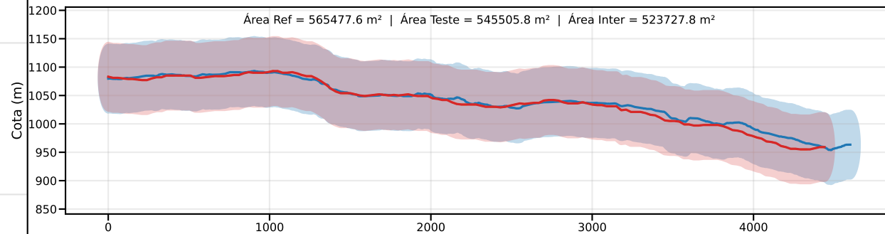
Classe D | PEC-PCD (Vertical)=75.0 m | EQ = 100m | dm = 16.05
