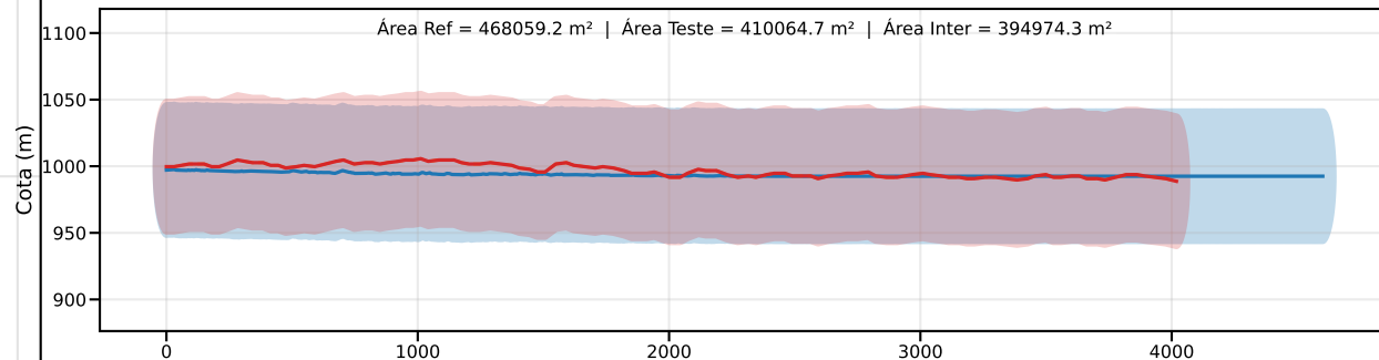
Classe C | PEC-PCD (Vertical)=60.0 m | EQ = 100m | dm = 32.33
