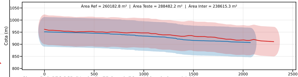
Classe D | PEC-PCD (Vertical)=75.0 m | EQ = 100m | dm = 14.08
