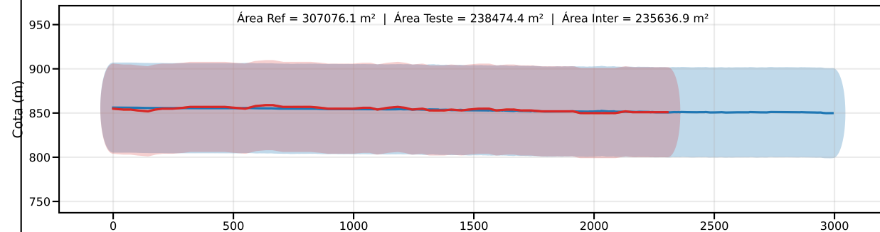
Classe C | PEC-PCD (Vertical)=60.0 m | EQ = 100m | dm = 55.74
