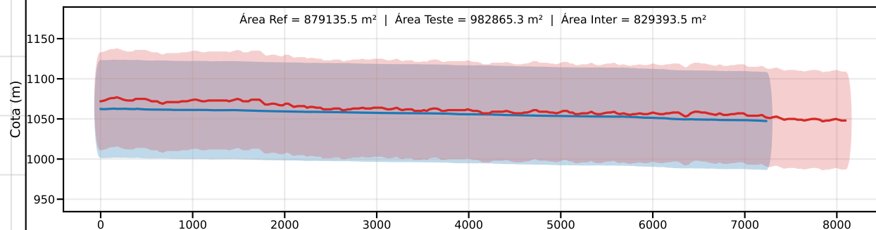
Classe D | PEC-PCD (Vertical)=75.0 m | EQ = 100m | dm = 9.53
