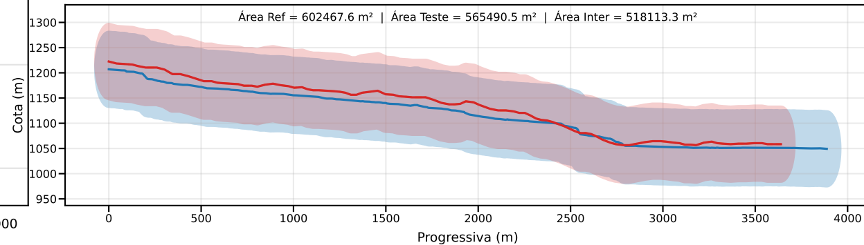
Classe D | PEC-PCD (Vertical)=75.0 m | EQ = 100m | dm = 35.15
