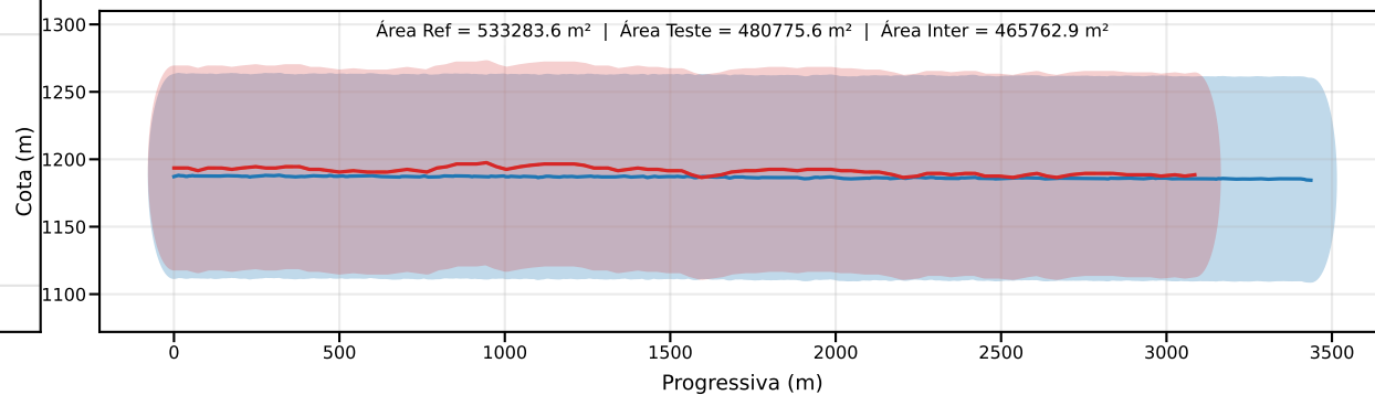
Classe D | PEC-PCD (Vertical)=75.0 m | EQ = 100m | dm = 33.09
