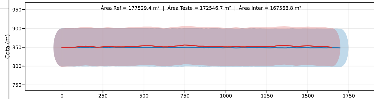
Classe C | PEC-PCD (Vertical)=60.0 m | EQ = 100m | dm = 9.89
