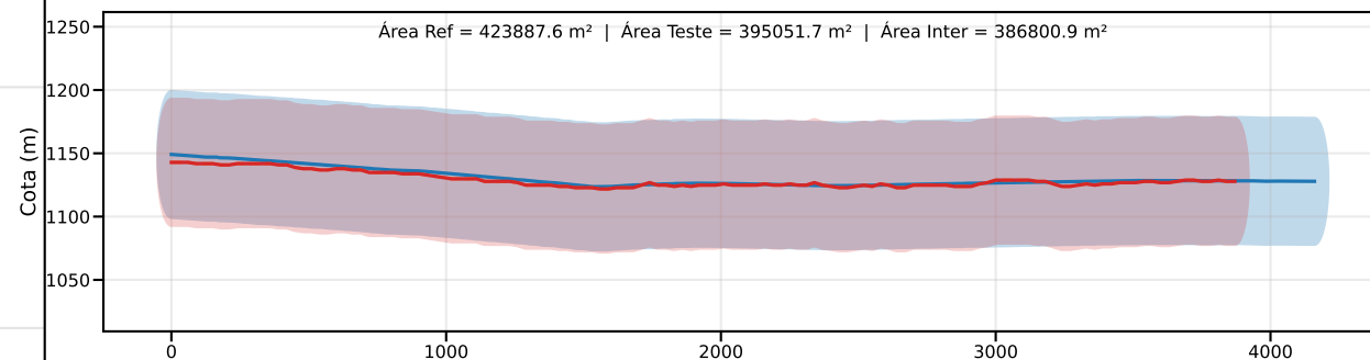
Classe C | PEC-PCD (Vertical)=60.0 m | EQ = 100m | dm = 17.00
