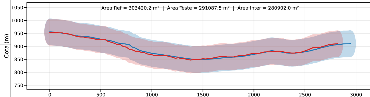
Classe C | PEC-PCD (Vertical)=60.0 m | EQ = 100m | dm = 13.43
