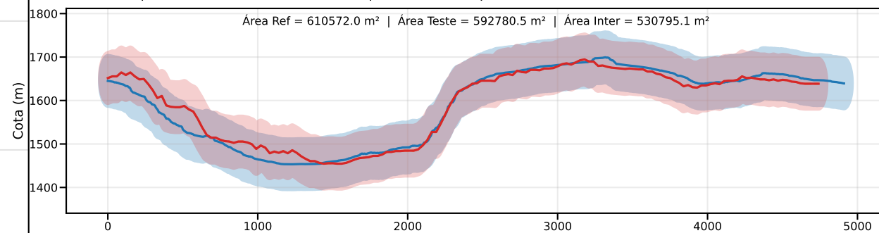
Classe D | PEC-PCD (Vertical)=75.0 m | EQ = 100m | dm = 26.78
