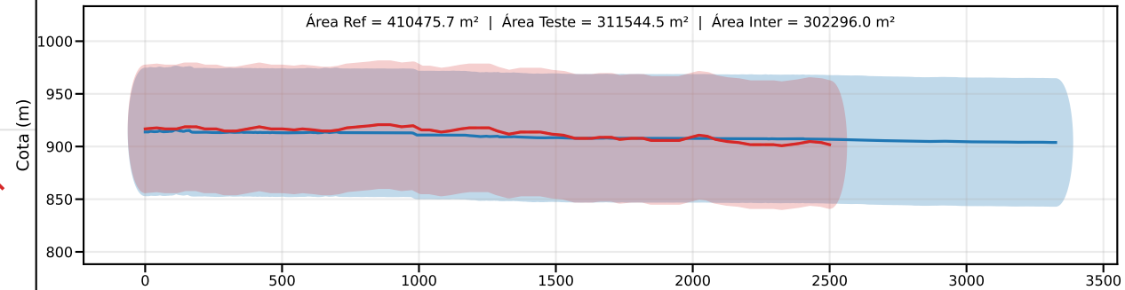
Classe D | PEC-PCD (Vertical)=75.0 m | EQ = 100m | dm = 79.74
