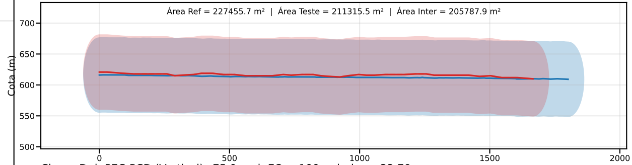
Classe D | PEC-PCD (Vertical)=75.0 m | EQ = 100m | dm = 22.70
