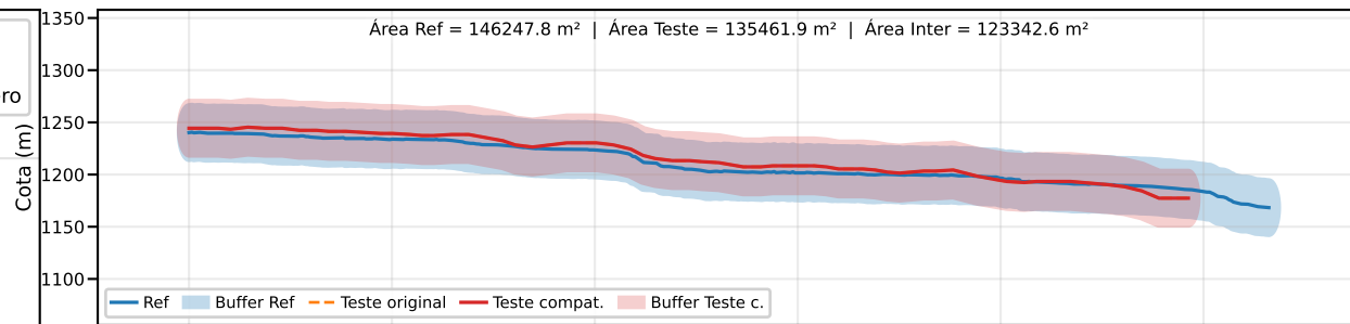
Classe B | PEC-PCD (Vertical)=50.0 m | EQ = 100m | dm = 19.88
