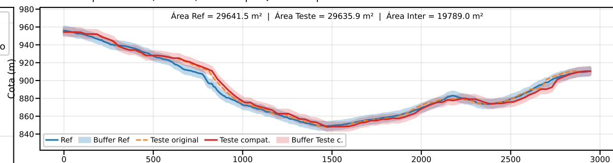
Classe B | PEC-PCD (Vertical)=10.0 m | EQ = 20m | dm = 5.40
