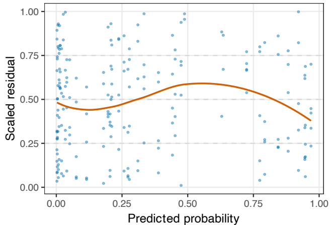
Algal plug: residual vs. predicted
