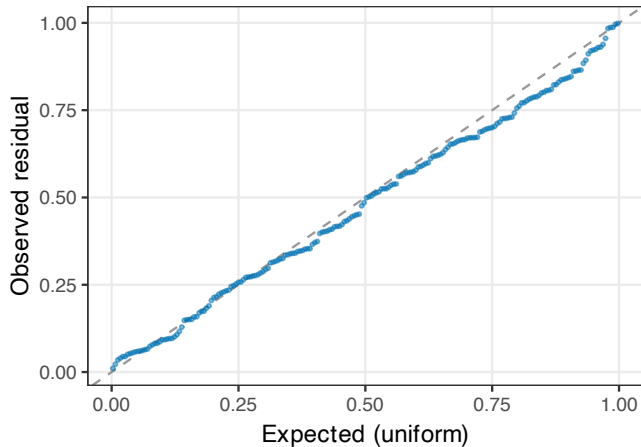
Algal plug: QQ uniformity
