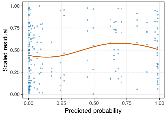
Polyp regeneration: residual vs. predicted
