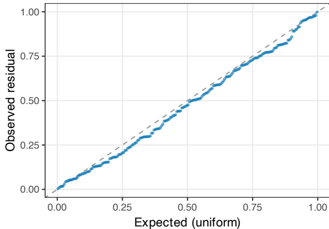
Polyp regeneration: QQ uniformity
