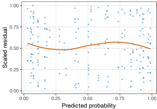
RFP: residual vs. predicted
