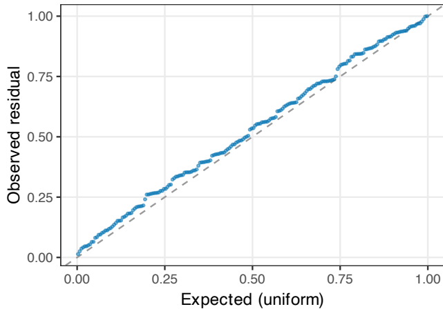
RFP: QQ uniformity
