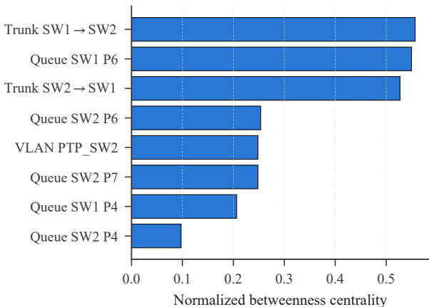
(a) BC, N=10 , base, steady state
