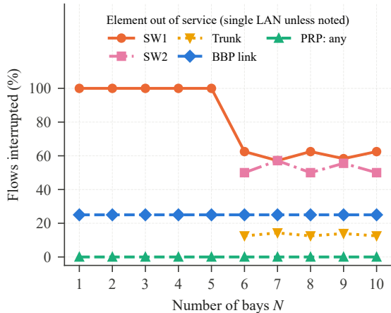
(b) Exposure during maintenance of one element
