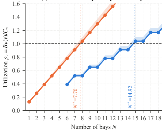
(a) 2 SV streams per bay, 100 Mbps
