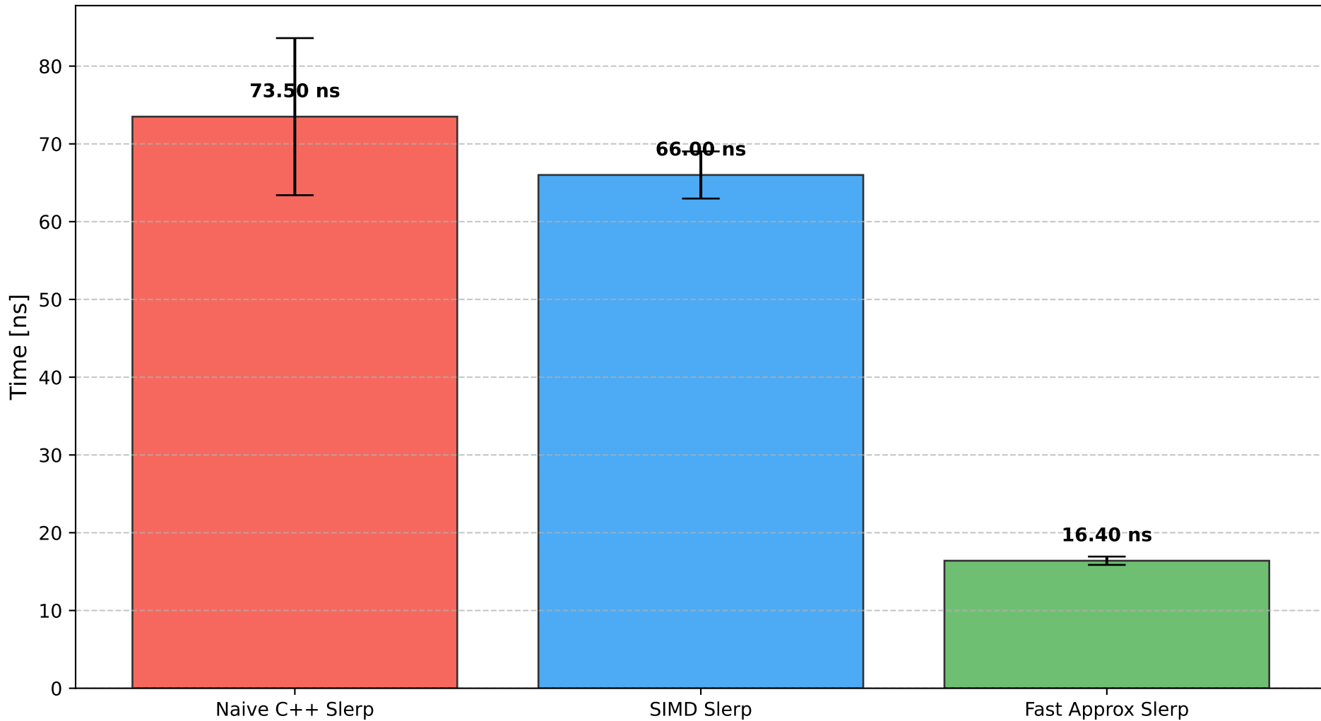
Comparison of Quaternion Slerp Implementations
