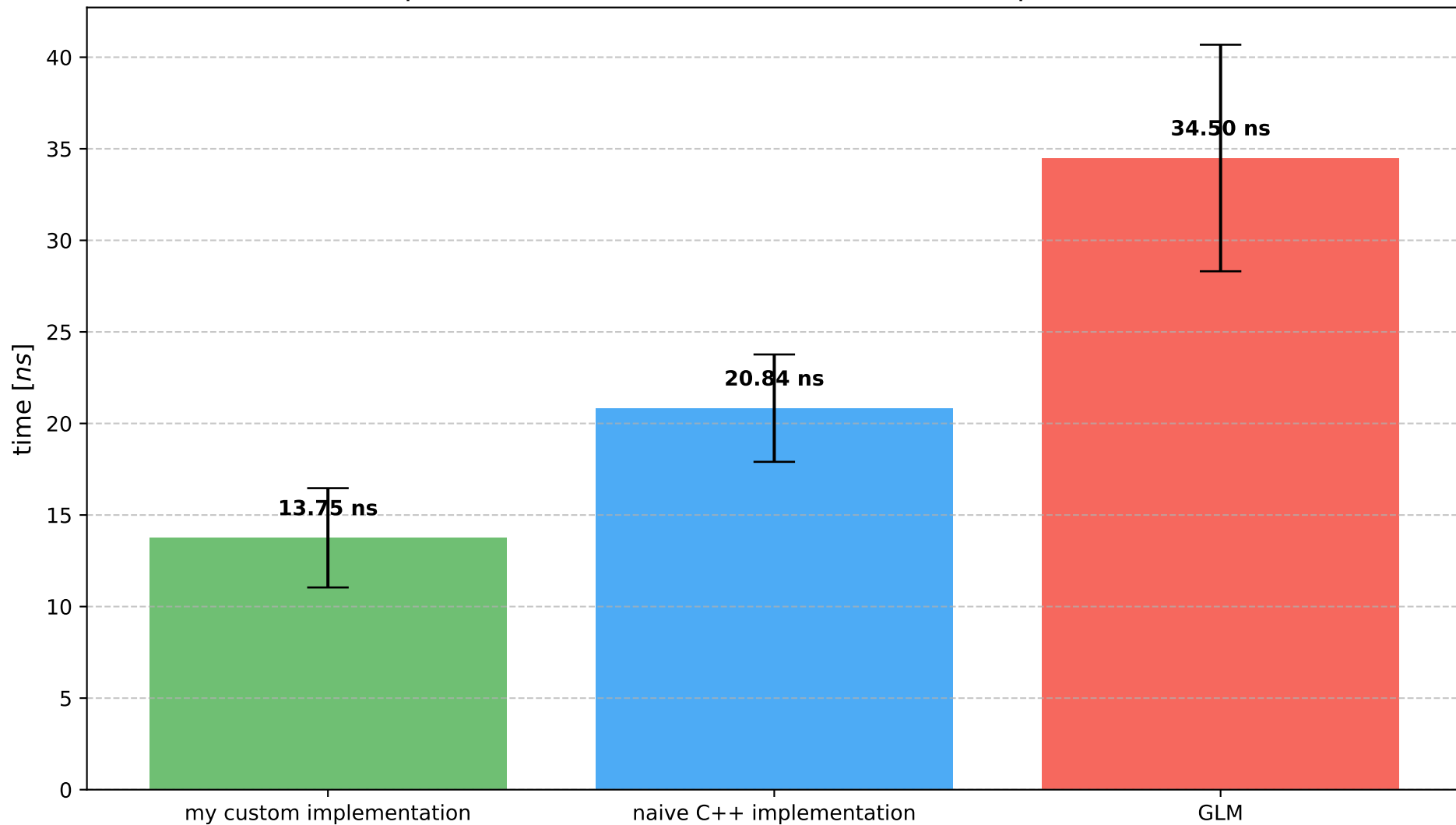
Comparison of different 4x4 matrix matmul implementation
