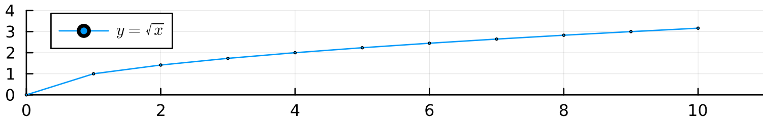
root of x
