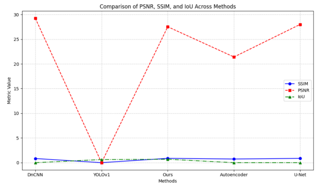
Fig. 4. Comparison of PSNR [4], SSIM [3], and IoU Across Methods
