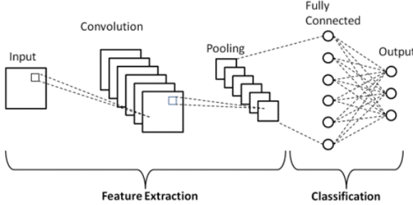
Fig. 1. Convolution Architecture Visualization
