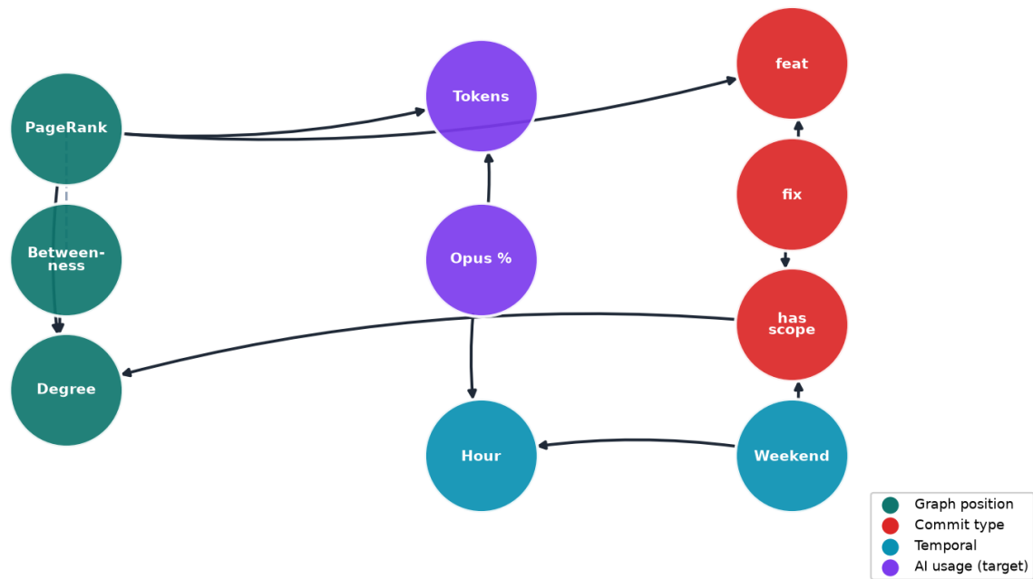
Causal DAG (PC algorithm, Fisher's Z, \alpha = 0.05 ) — 11 directed edges discovered
