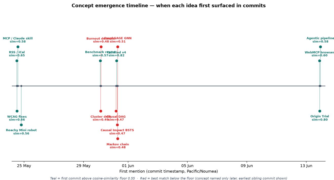
Figure 5: Each label is a key project concept. Its position on the x-axis is the timestamp of the first commit whose subject is semantically close to the concept description (cosine \geq 0.55 on BAAI/bge-m3). Teal = clear above-floor match (the concept was named in the subject). Red = best match below the floor (the concept’s foundation existed but it was not yet named — the timestamp marks the *forerunner* commit). Multi-level vertical layout chosen to keep neighbours legible.
