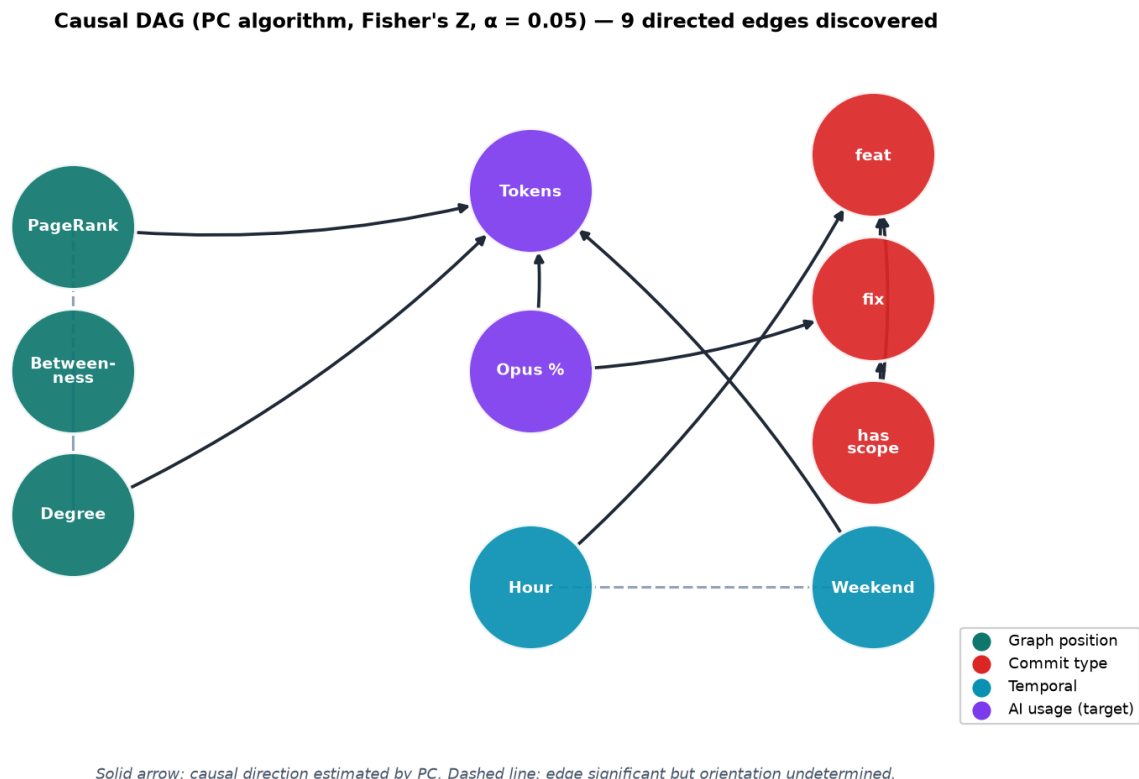
Figure 5: Causal DAG learnt by the PC algorithm with Fisher’s Z conditional independence test ( \alpha = 0.05 ) on 178 commit-level observations of 10 features. Solid arrows = direction estimated. Dashed lines = edge significant but orientation undetermined (a Markov-equivalence-class artefact).
