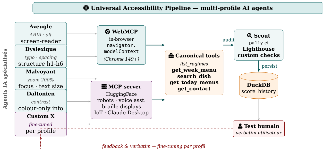
Figure 8: Universal Accessibility Pipeline: each AI agent simulates a specific WCAG profile and consumes the same canonical tools through either WebMCP (in-browser) or the MCP server (robots, voice assistants, braille displays, IoT). Scout audits the responses against multi-criterion rules; human verbatim closes the loop by fine-tuning each agent profile.
